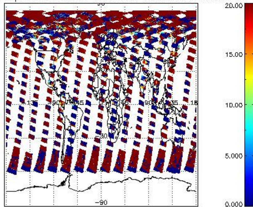
cL_opt_depth for 03JUL2009 00:00:00 to 04JUL2009 00:00:00
