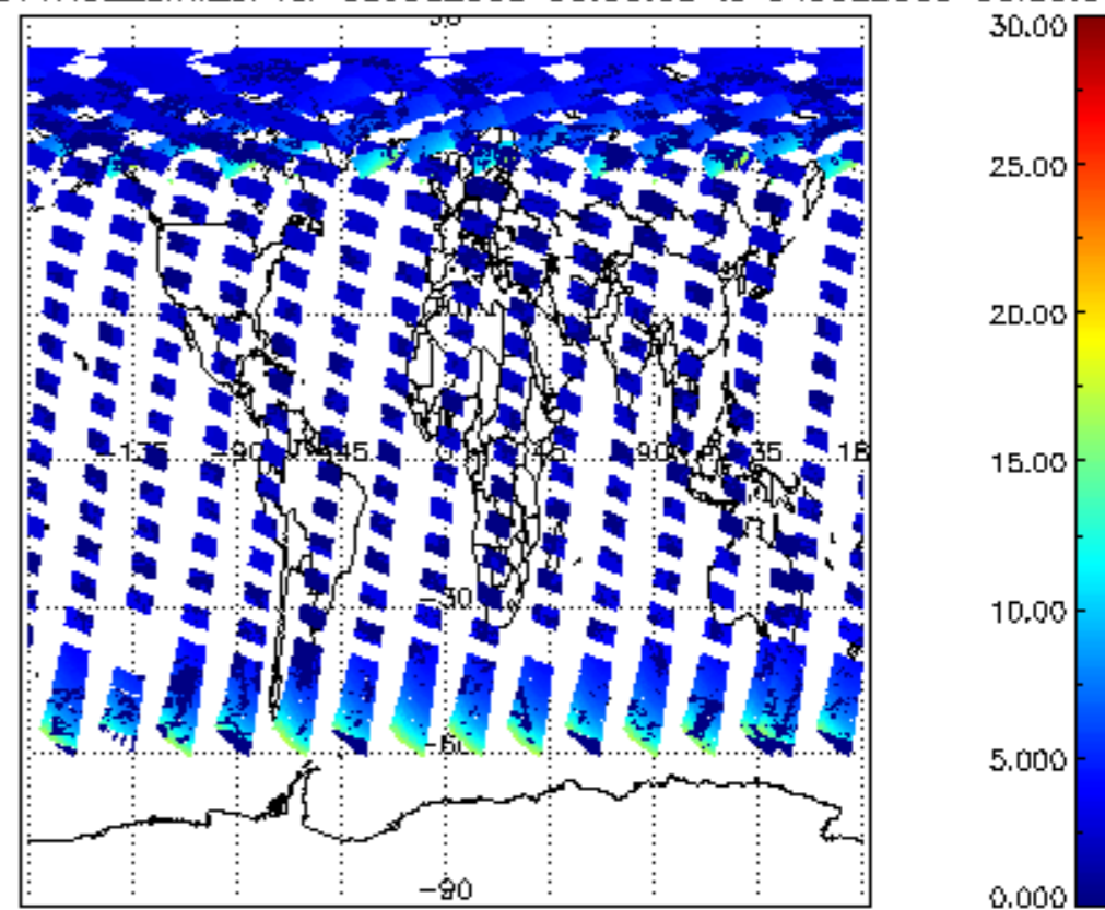
SCIOL2P_NADUV1NO2_amf_cl for 03JUL2009 00:00:00 to 04JUL2009 00:00:00
