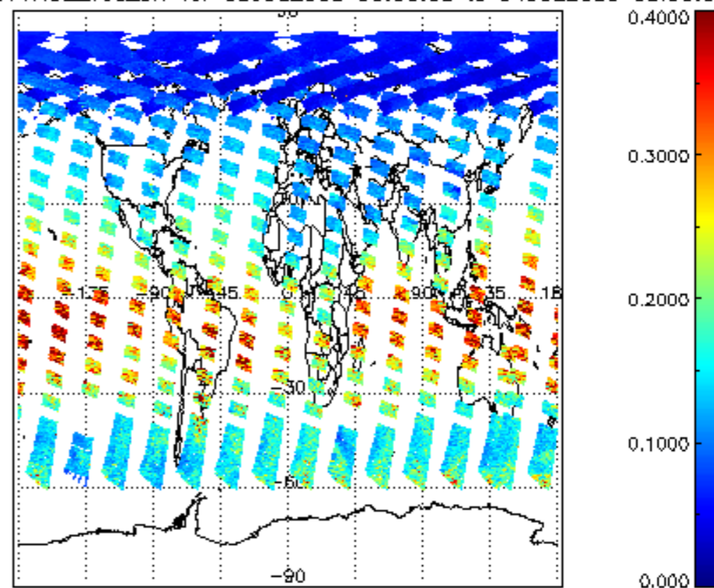
SCIOL2P_NADUV1NO2_vcd_err for 03JUL2009 00:00:00 to 04JUL2009 00:00:00
