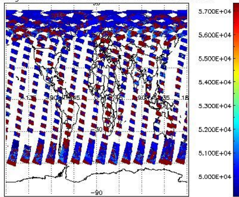
cloud_flags for 03JUL2009 00:00:00 to 04JUL2009 00:00:00
