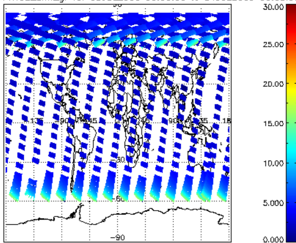
SCIOL2P_NADUV1NO2_amf_gr for 03JUL2009 00:00:00 to 04JUL2009 00:00:00
