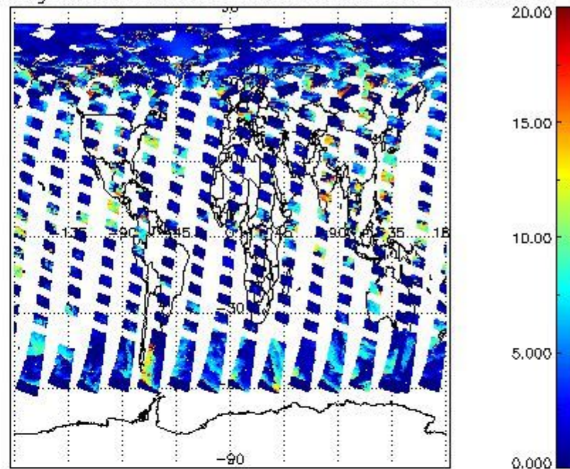
cL_top_height for 03JUL2009 00:00:00 to 04JUL2009 00:00:00
