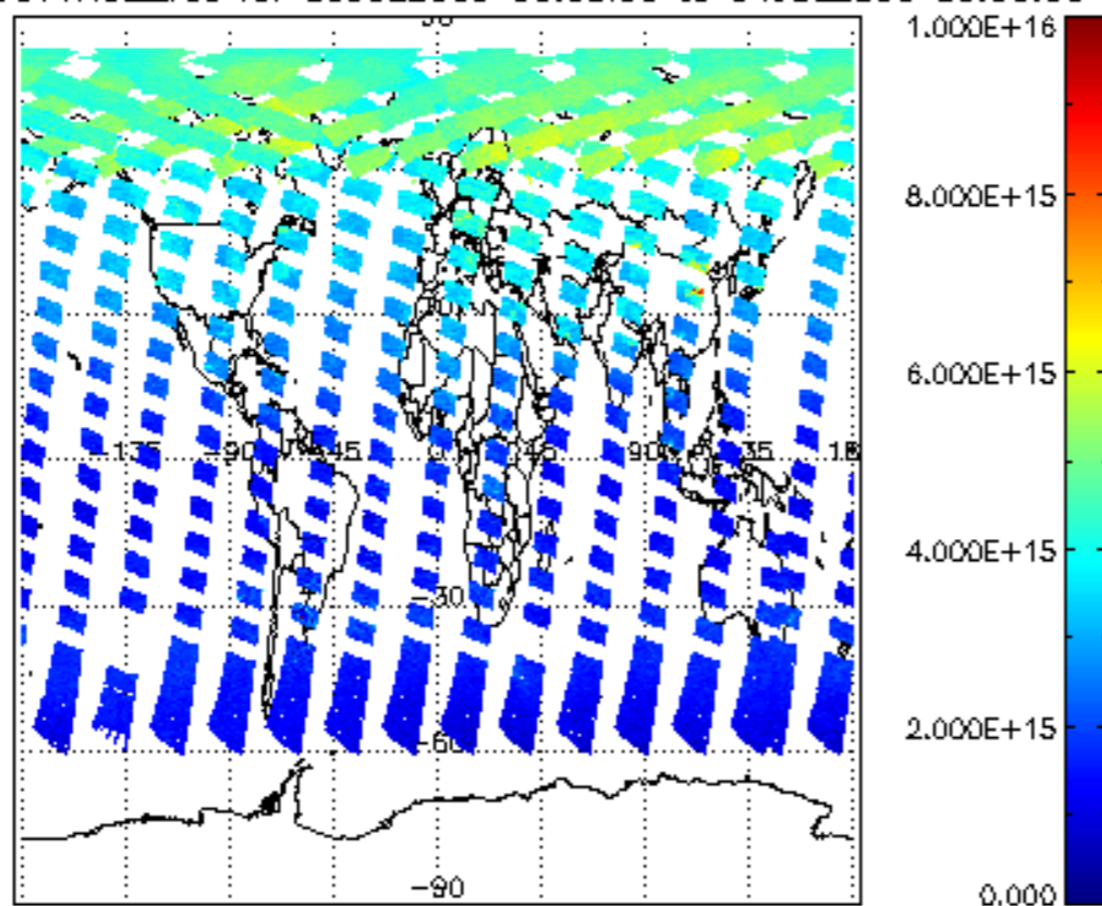
SCIOL2P_NADUV1NO2_vcd for 03JUL2009 00:00:00 to 04JUL2009 00:00:00
