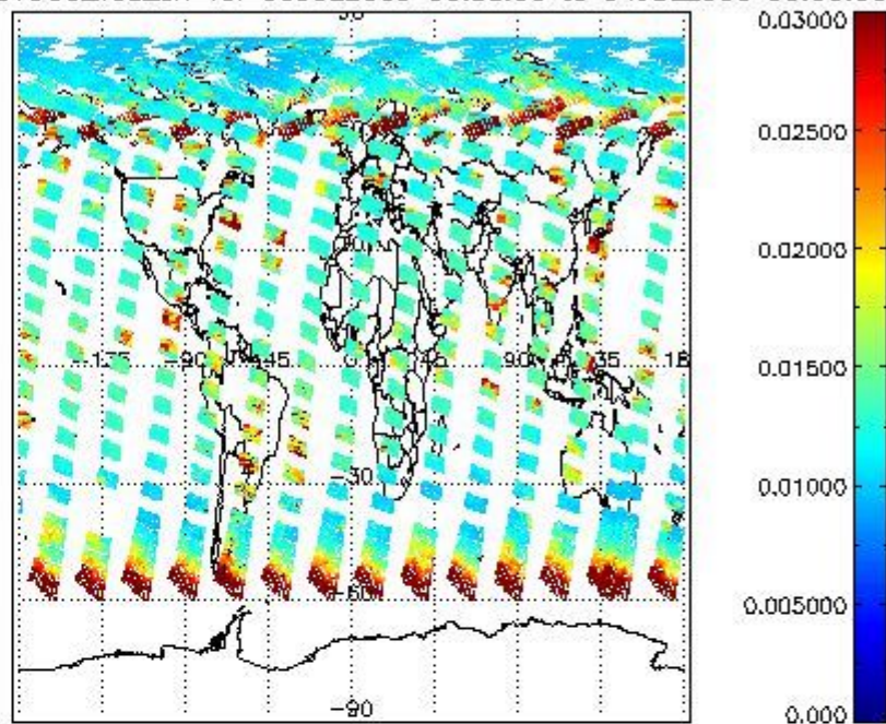
SCIOL2P_NADUV003_vcd_err for 03JUL2009 00:00:00 to 04JUL2009 00:00:00
