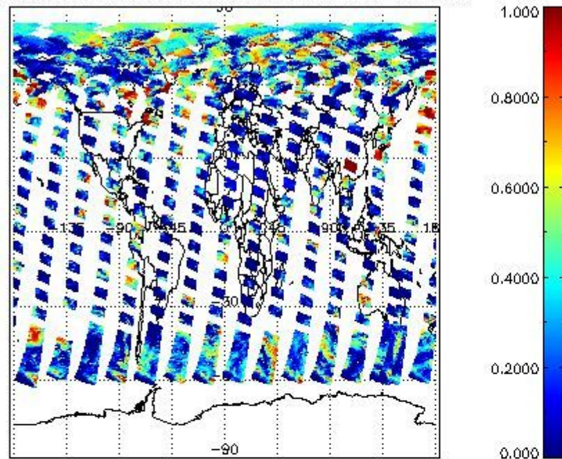
cL_frac for 03JUL2009 00:00:00 to 04JUL2009 00:00:00
