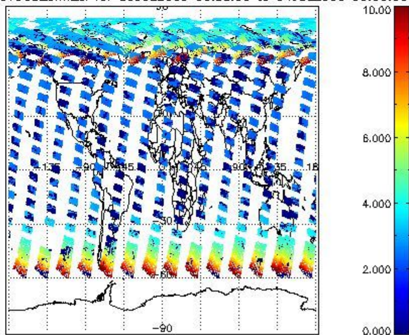
SCIOL2P_NADUV003_amf_cl for 03JUL2009 00:00:00 to 04JUL2009 00:00:00
