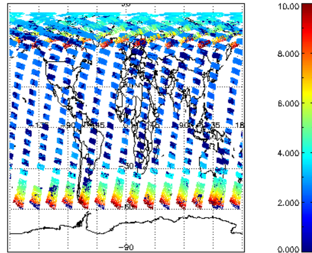
SCIOL2P_NADUV003_amf_cl for 03JUL2009 00:00:00 to 04JUL2009 00:00:00
