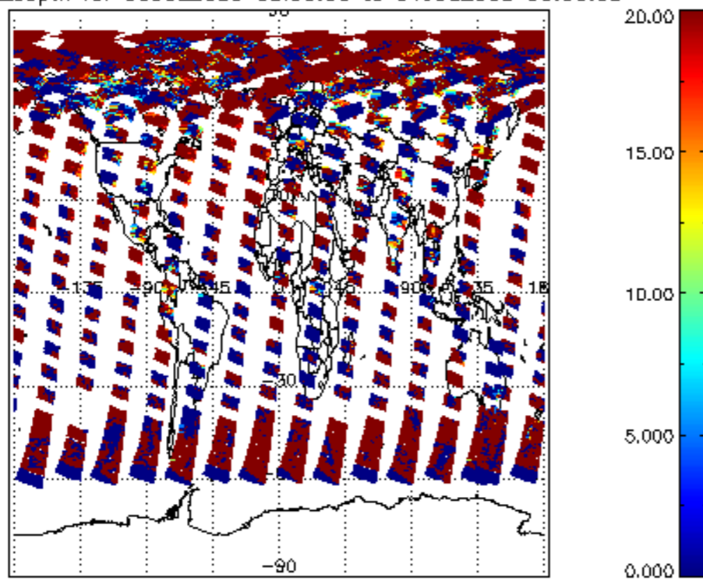
cl_lopt_depth for 03JUL2009 00:00:00 to 04JUL2009 00:00:00
