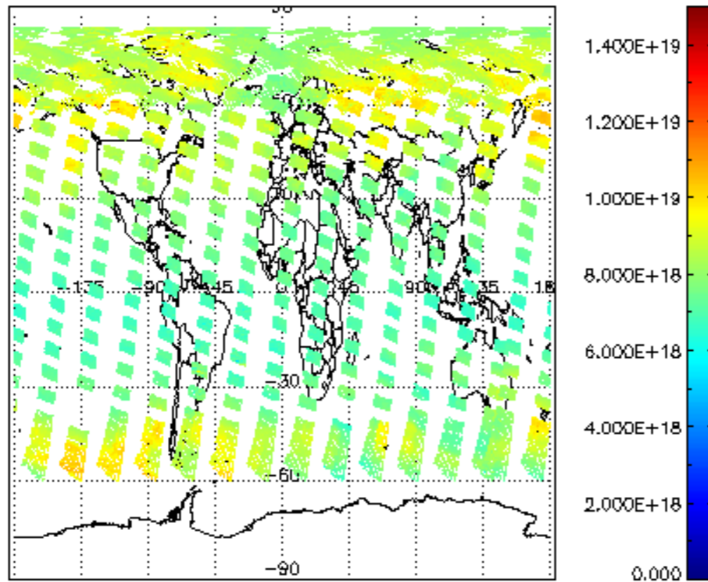
SCIOL2P_NADUV003_vcd for 03JUL2009 00:00:00 to 04JUL2009 00:00:00
