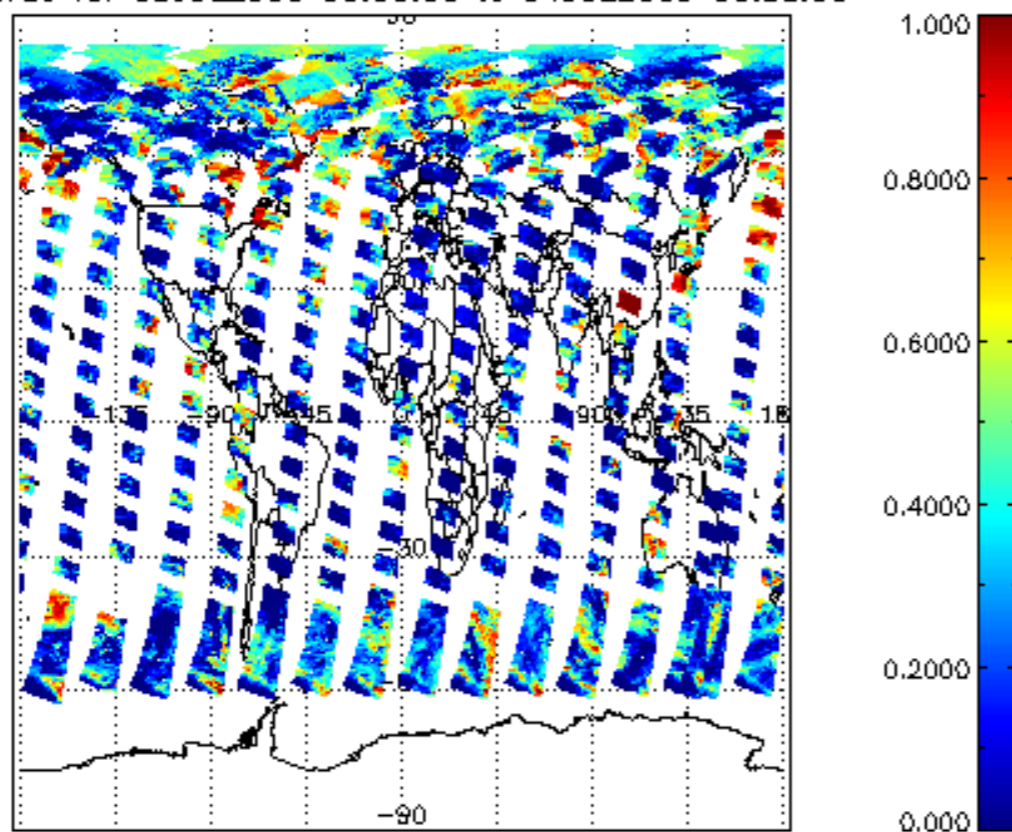
cl_frac for 03JUL2009 00:00:00 to 04JUL2009 00:00:00
