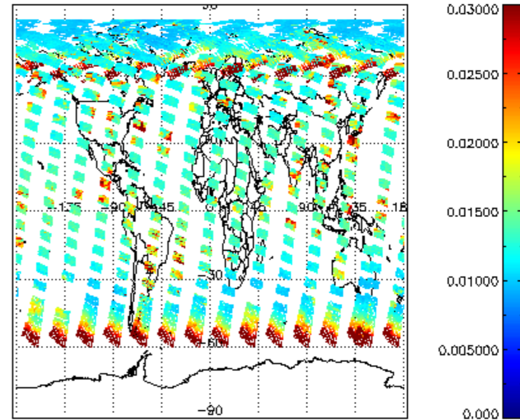
SCIOL2P_NADUV003_vcd_err for 03JUL2009 00:00:00 to 04JUL2009 00:00:00
