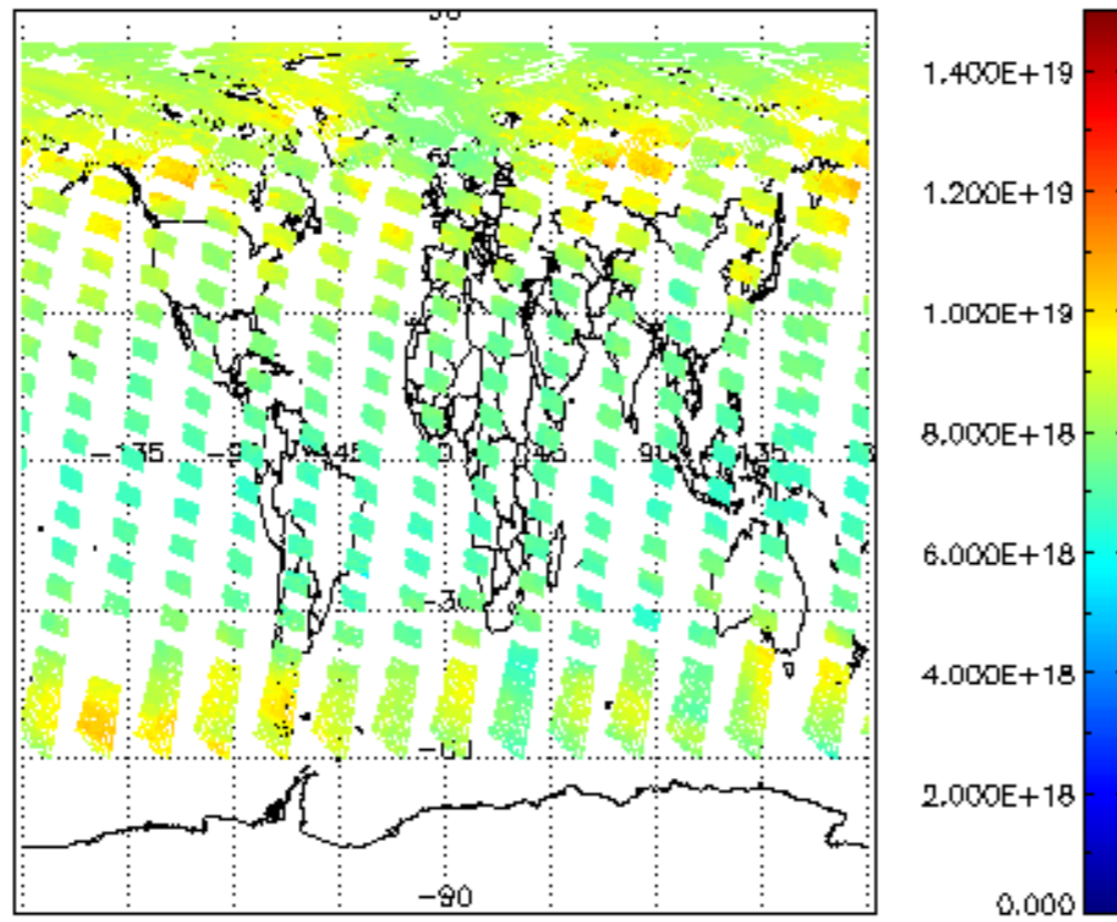
SCIOL2P_NADUV003_vcd for 02JUL2009 00:00:00 to 03JUL2009 00:00:00
