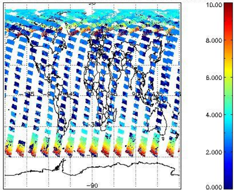
SCIOL2P_NADUV003_amf_cl for 02JUL2009 00:00:00 to 03JUL2009 00:00:00
