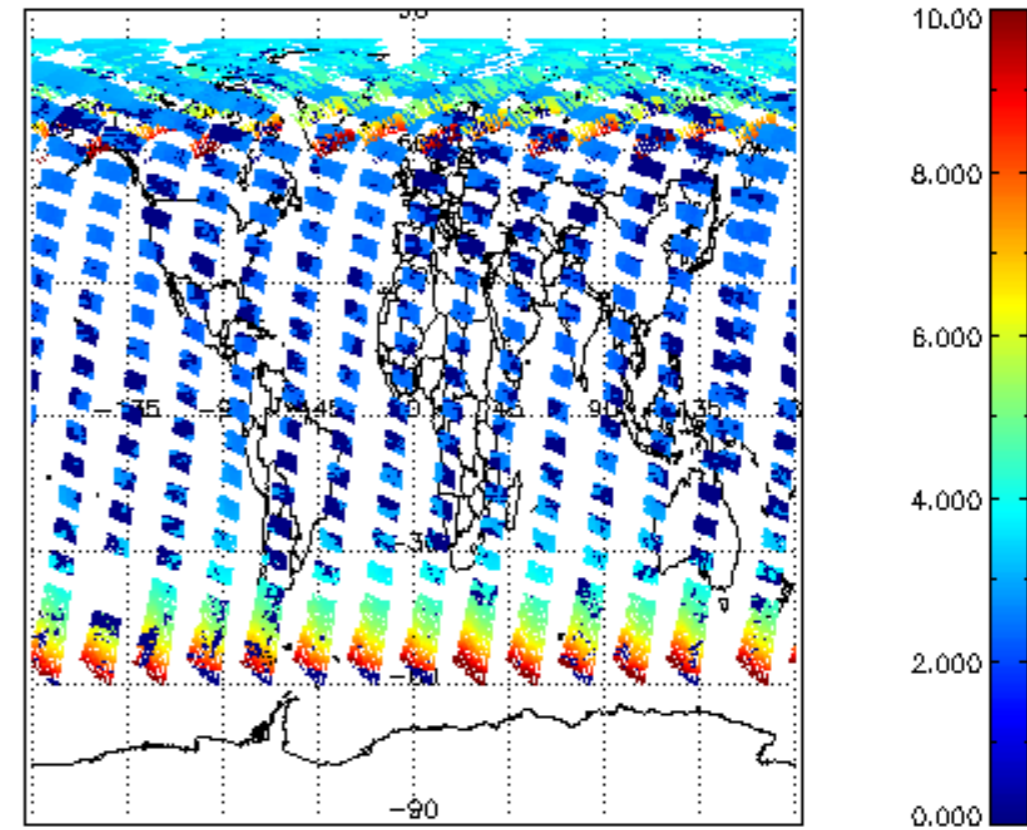
SCIOL2P_NADUV003_amf_cl for 02JUL2009 00:00:00 to 03JUL2009 00:00:00
