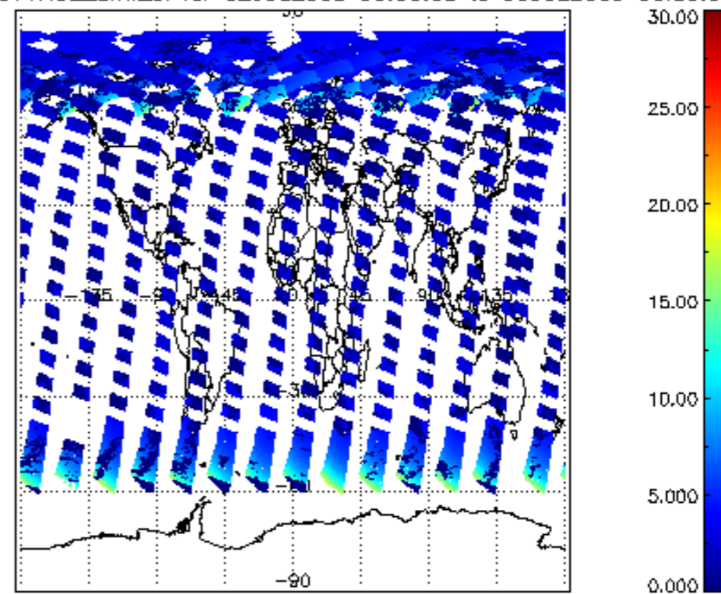
SCIOL2P_NADUV1NO2_amf_cl for 02JUL2009 00:00:00 to 03JUL2009 00:00:00
