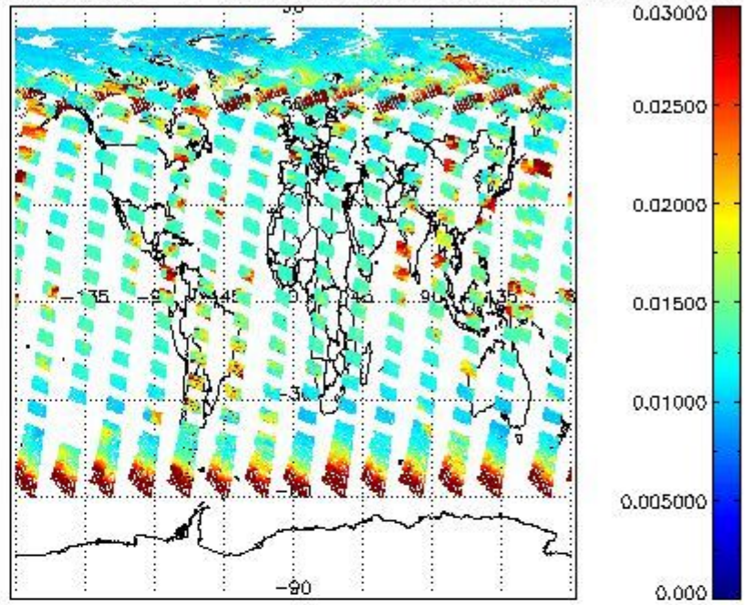
SCIOL2P_NADUV003_vcd_err for 02JUL2009 00:00:00 to 03JUL2009 00:00:00
