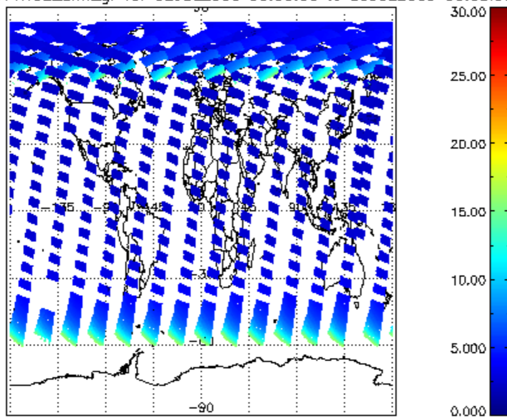
SCIOL2P_NADUV1NO2_amf_gr for 02JUL2009 00:00:00 to 03JUL2009 00:00:00
