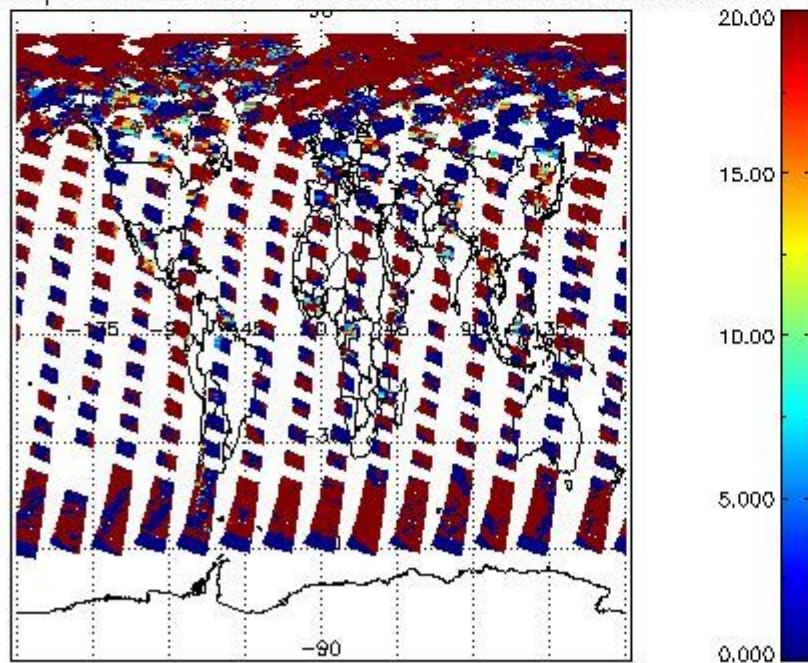
cL_opt_depth for 02JUL2009 00:00:00 to 03JUL2009 00:00:00
