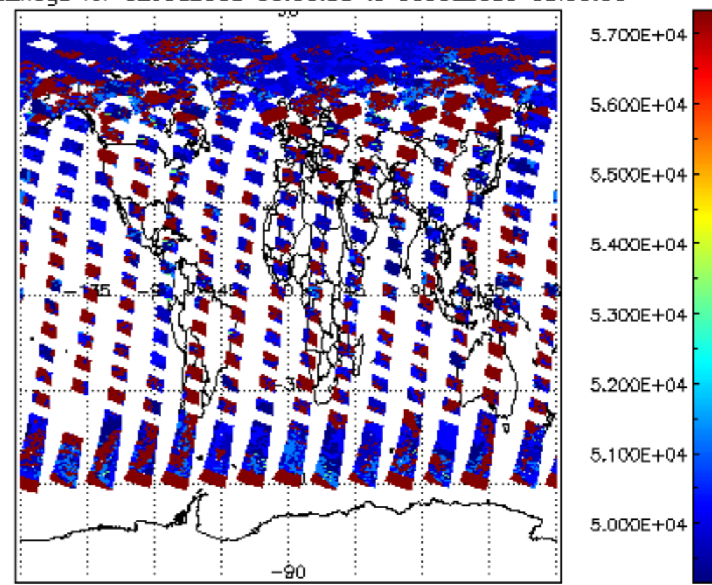
cloud_flags for 02JUL2009 00:00:00 to 03JUL2009 00:00:00
