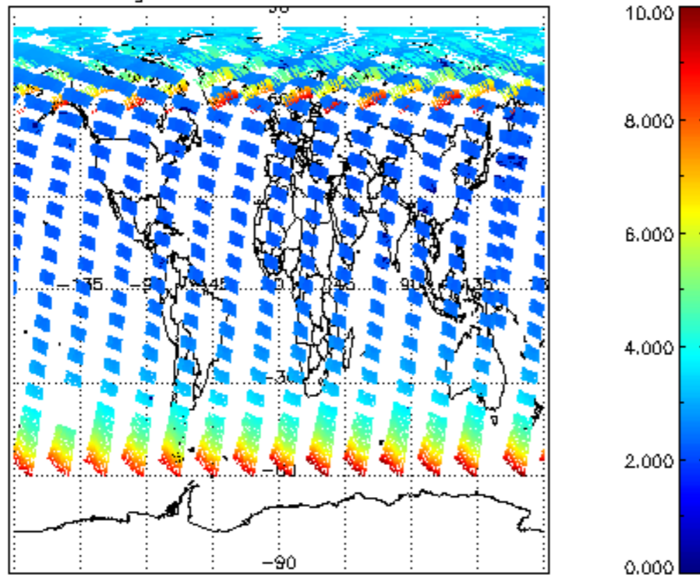
SCIOL2P_NADUV003_amf_gr for 02JUL2009 00:00:00 to 03JUL2009 00:00:00
