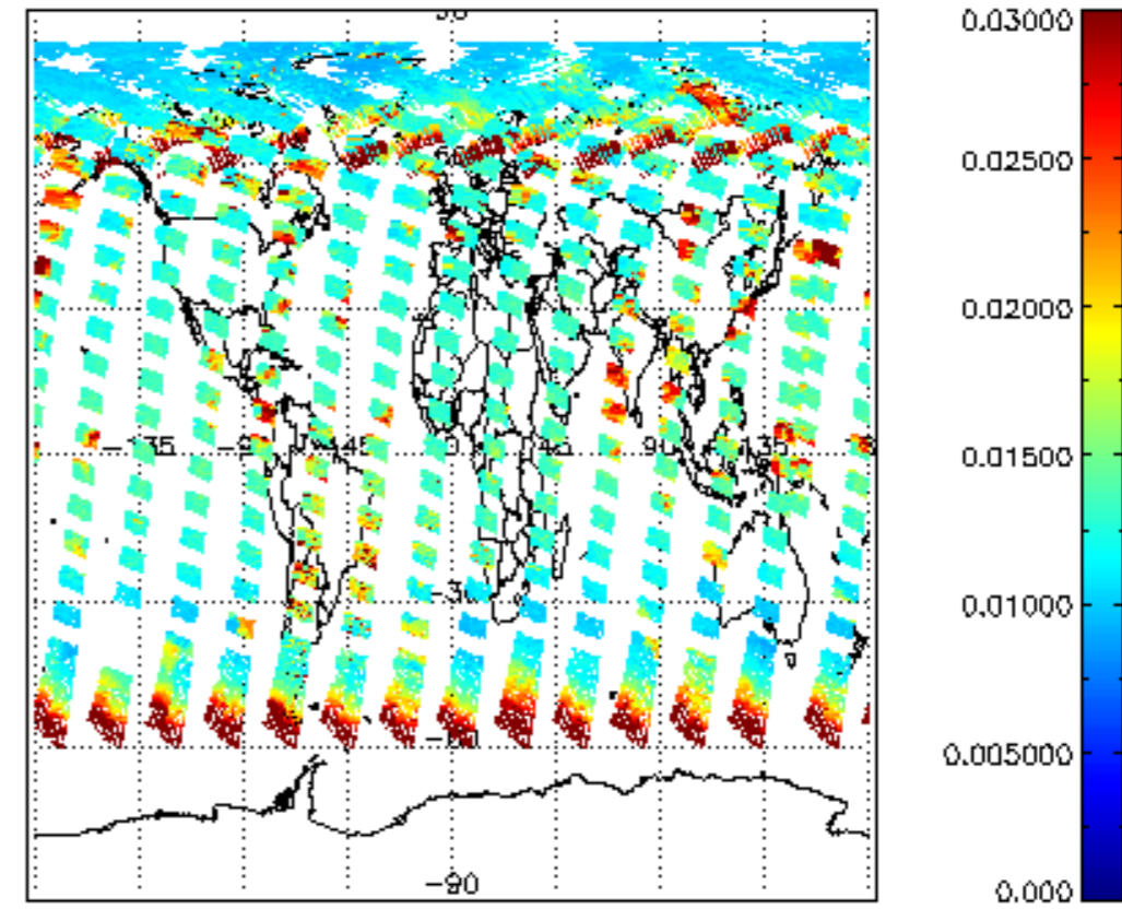
SCIOL2P_NADUV003_vcd_err for 02JUL2009 00:00:00 to 03JUL2009 00:00:00
