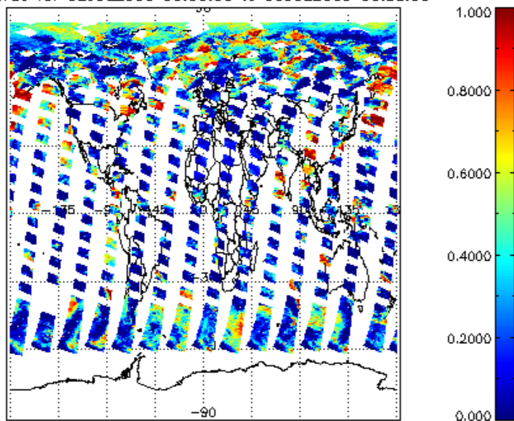
cl_frac for 02JUL2009 00:00:00 to 03JUL2009 00:00:00
