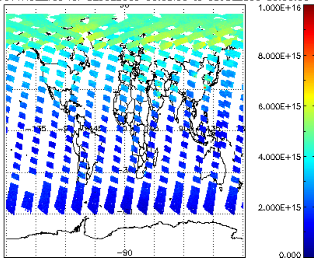
SCIOL2P_NADUV1NO2_vcd for 02JUL2009 00:00:00 to 03JUL2009 00:00:00
