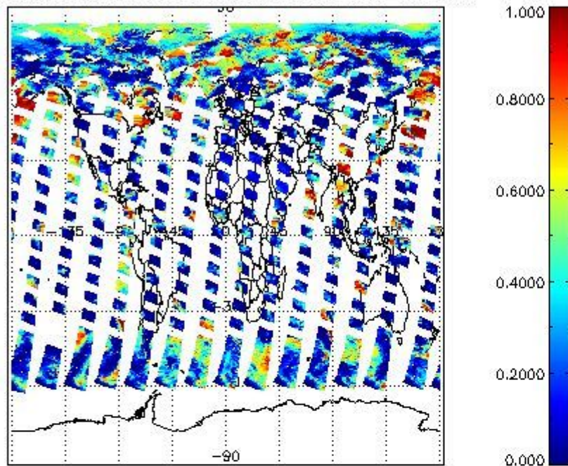
cL_frac for 02JUL2009 00:00:00 to 03JUL2009 00:00:00
