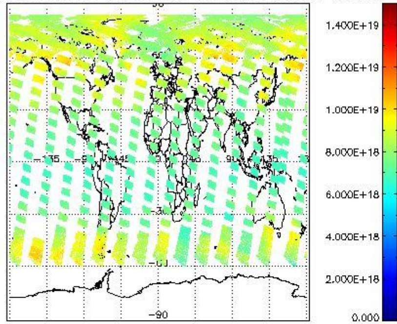
SCIOL2P_NADUV003_vcd for 02JUL2009 00:00:00 to 03JUL2009 00:00:00
