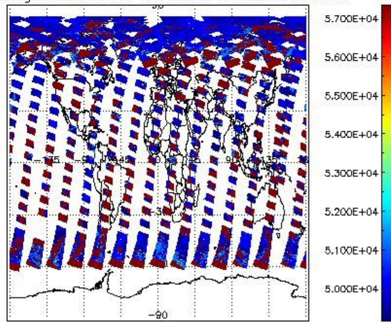
cloud_flags for 02JUL2009 00:00:00 to 03JUL2009 00:00:00
