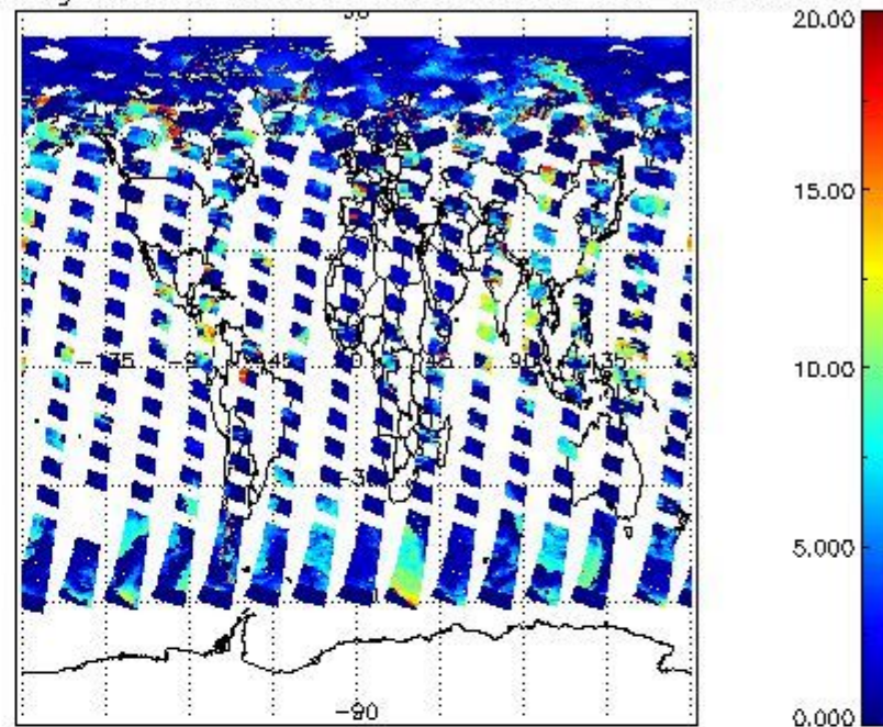
cL_top_height for 02JUL2009 00:00:00 to 03JUL2009 00:00:00
