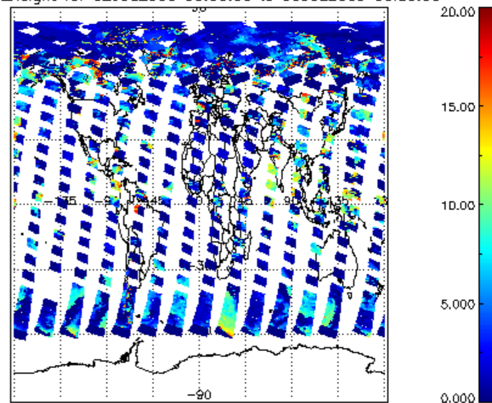
cl_top_height for 02JUL2009 00:00:00 to 03JUL2009 00:00:00
