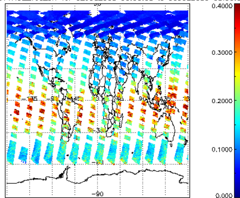
SCIOL2P_NADUV1NO2_vcd_err for 02JUL2009 00:00:00 to 03JUL2009 00:00:00
