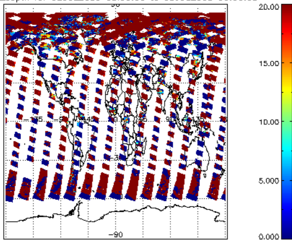
cl_opt_depth for 02JUL2009 00:00:00 to 03JUL2009 00:00:00
