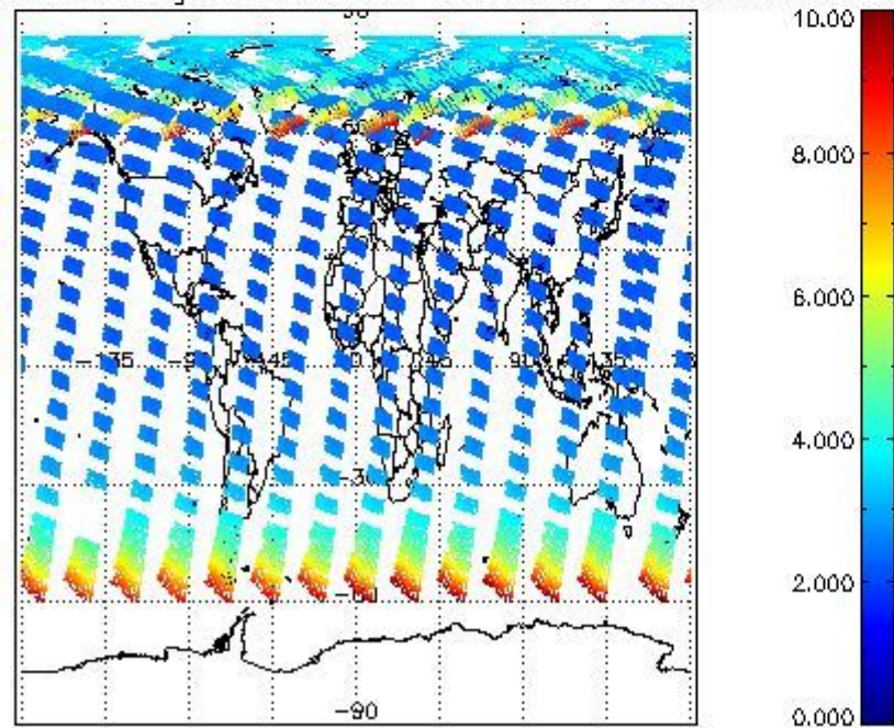
SCIOL2P_NADUV003_amf_gr for 02JUL2009 00:00:00 to 03JUL2009 00:00:00
