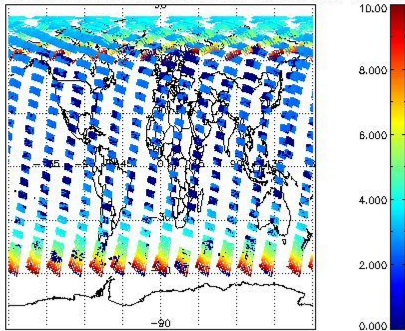
SCIOL2P_NADUV003_amf_cl for 31MAY2009 00:00:00 to 01JUN2009 00:00:00
