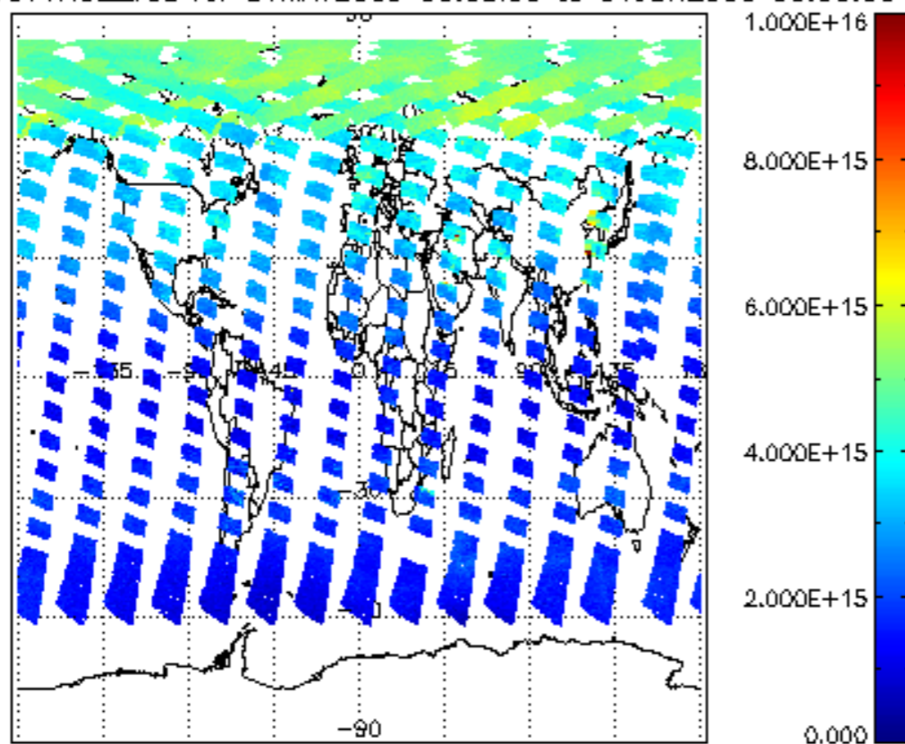
SCIOL2P_NADUV1NO2_vcd for 31MAY2009 00:00:00 to 01JUN2009 00:00:00
