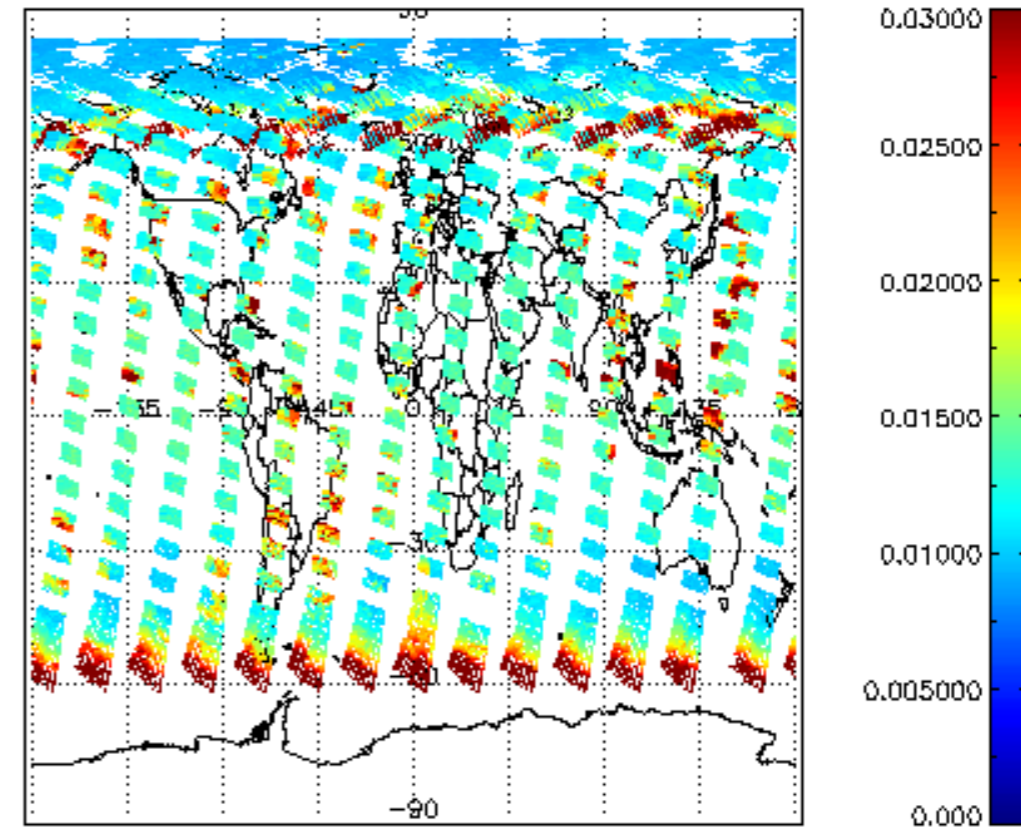
SCIOL2P_NADUV003_vcd_err for 31MAY2009 00:00:00 to 01JUN2009 00:00:00
