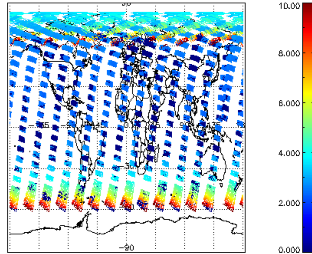
SCIOL2P_NADUV003_amf_cl for 31MAY2009 00:00:00 to 01JUN2009 00:00:00
