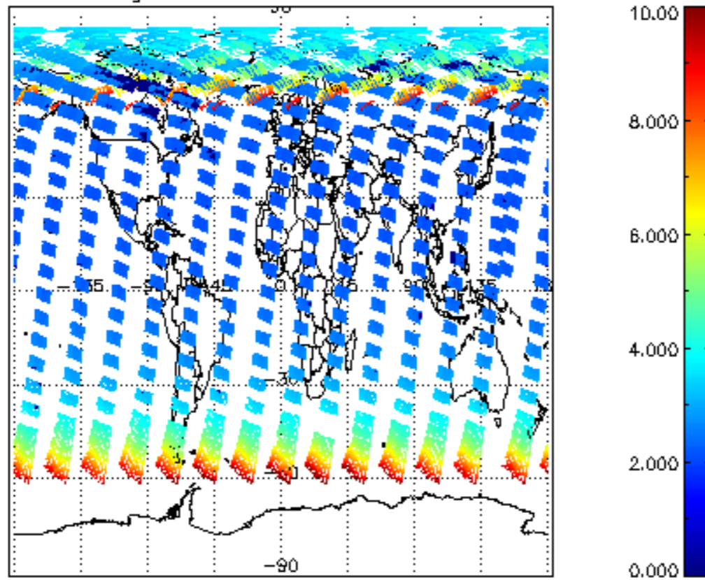
SCIOL2P_NADUV003_amf_gr for 31MAY2009 00:00:00 to 01JUN2009 00:00:00
