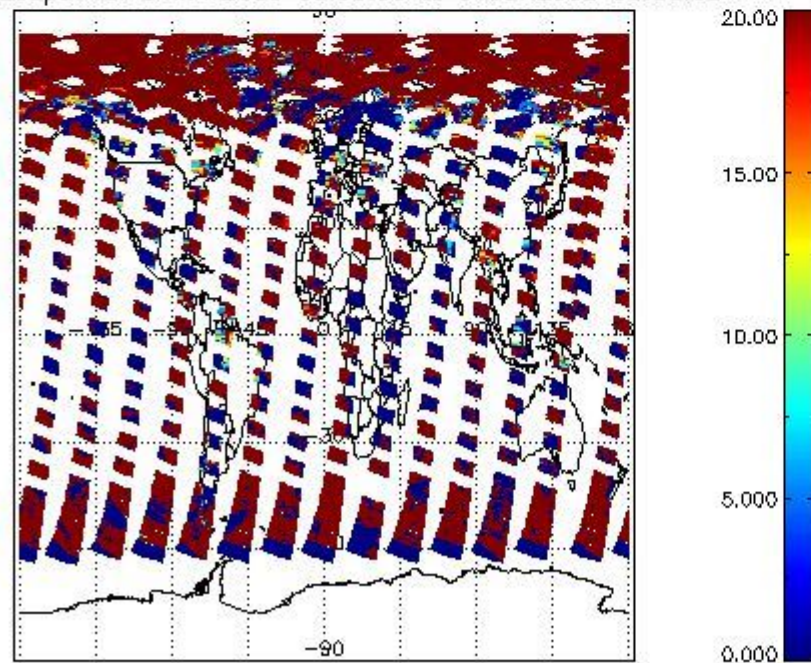
cL_opt_depth for 31MAY2009 00:00:00 to 01JUN2009 00:00:00
