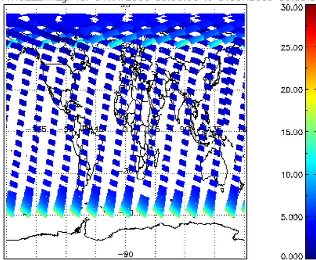
iCIOL2P_NADUV1NO2_amf_gr for 31MAY2009 00:00:00 to 01JUN2009 00:00:00
