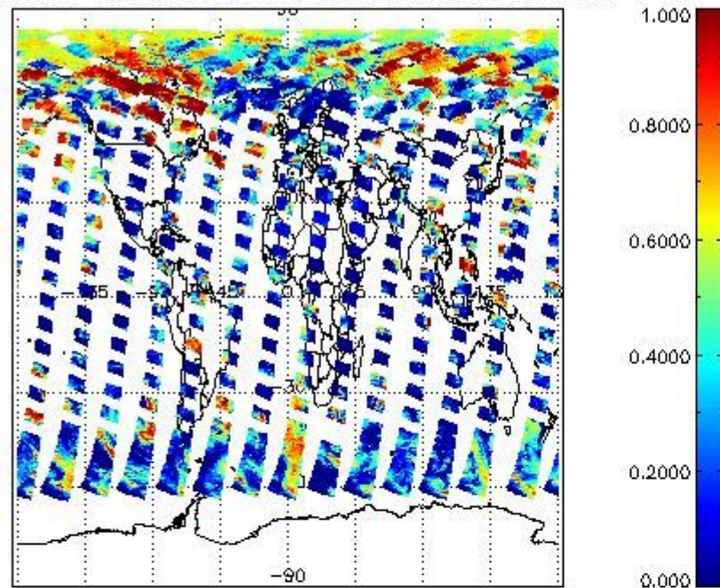
cL_frac for 31MAY2009 00:00:00 to 01JUN2009 00:00:00
