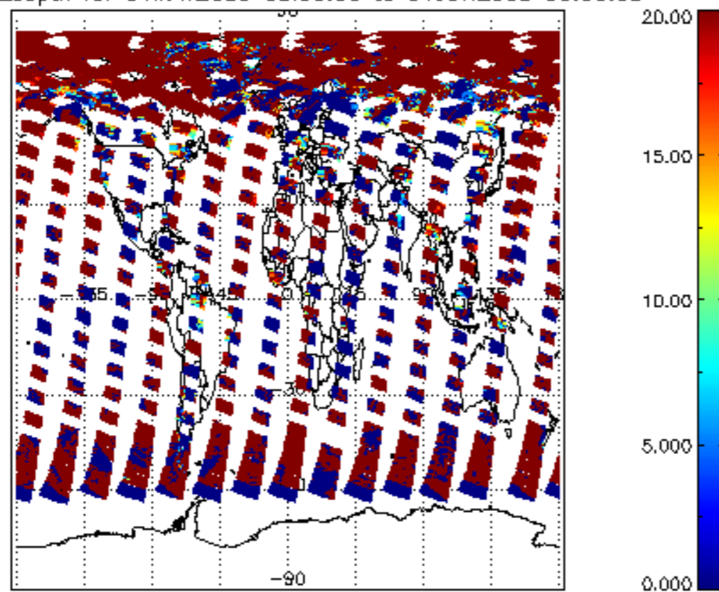
cl_opt_depth for 31MAY2009 00:00:00 to 01JUN2009 00:00:00
