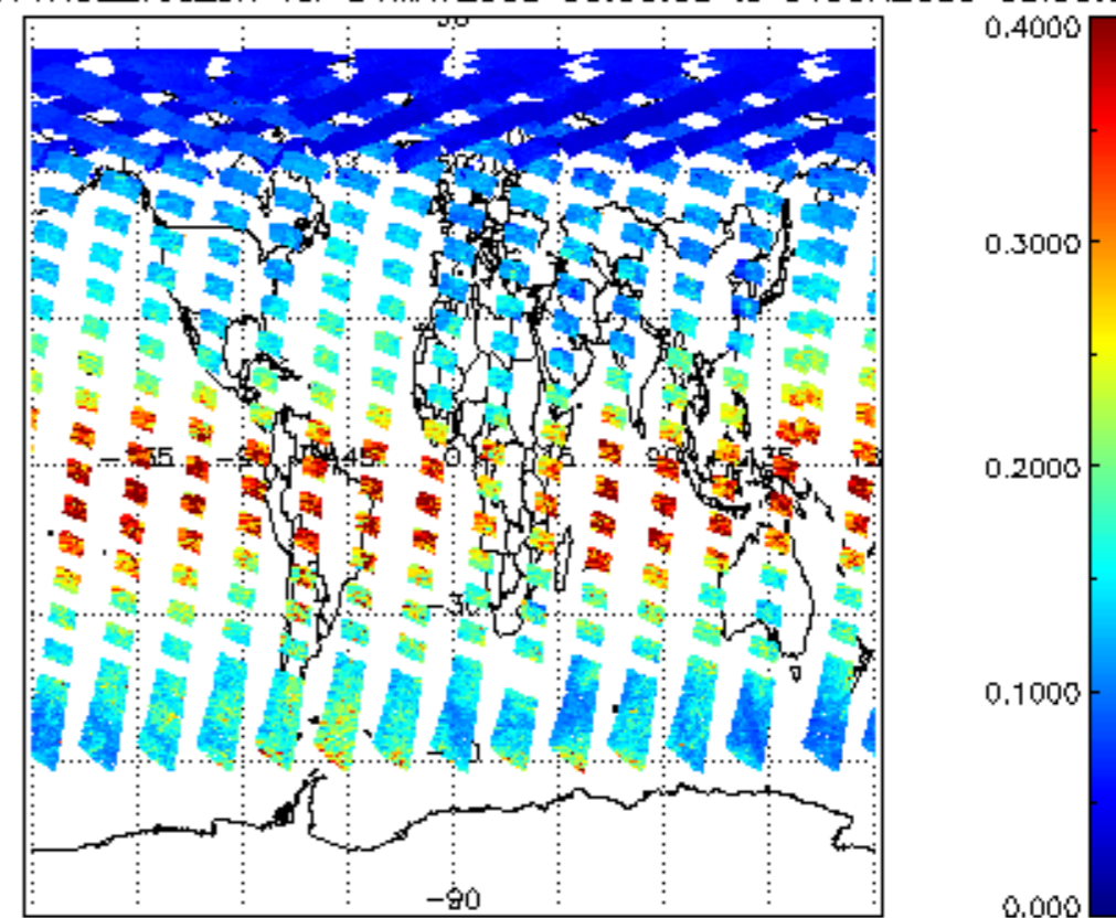
iCIOL2P_NADUV1NO2_vcd_err for 31MAY2009 00:00:00 to 01JUN2009 00:00:00
