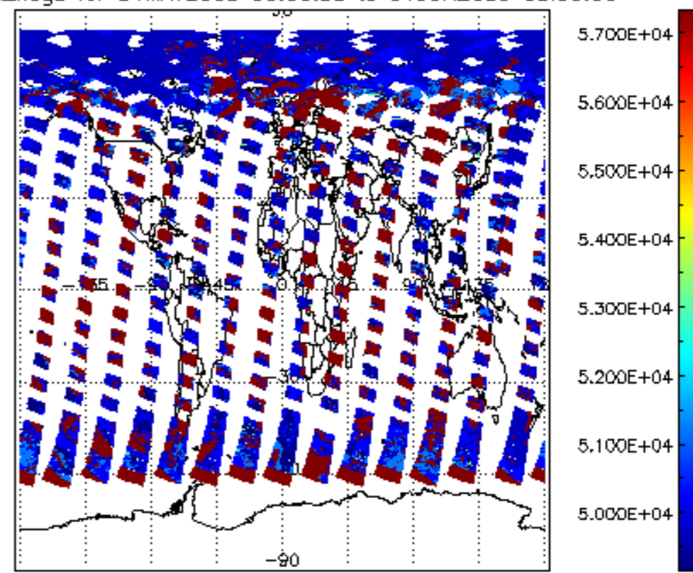
cloud_flags for 31MAY2009 00:00:00 to 01JUN2009 00:00:00
