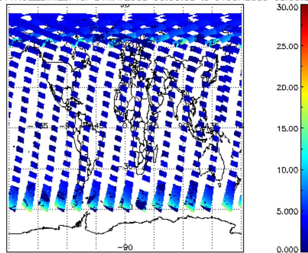
iCIOL2P_NADUV1NO2_amf_cl for 31MAY2009 00:00:00 to 01JUN2009 00:00:00
