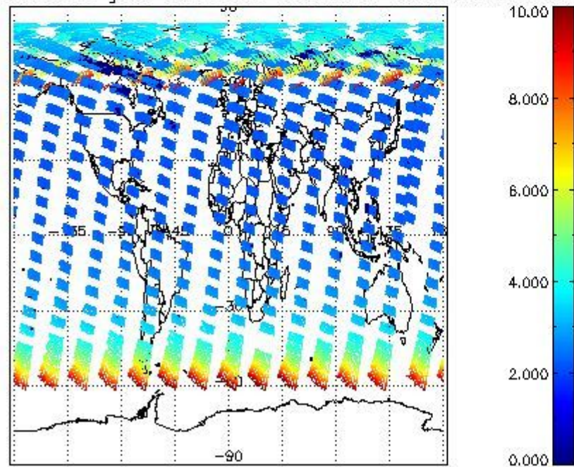
SCIOL2P_NADUV003_amf_gr for 31MAY2009 00:00:00 to 01JUN2009 00:00:00
