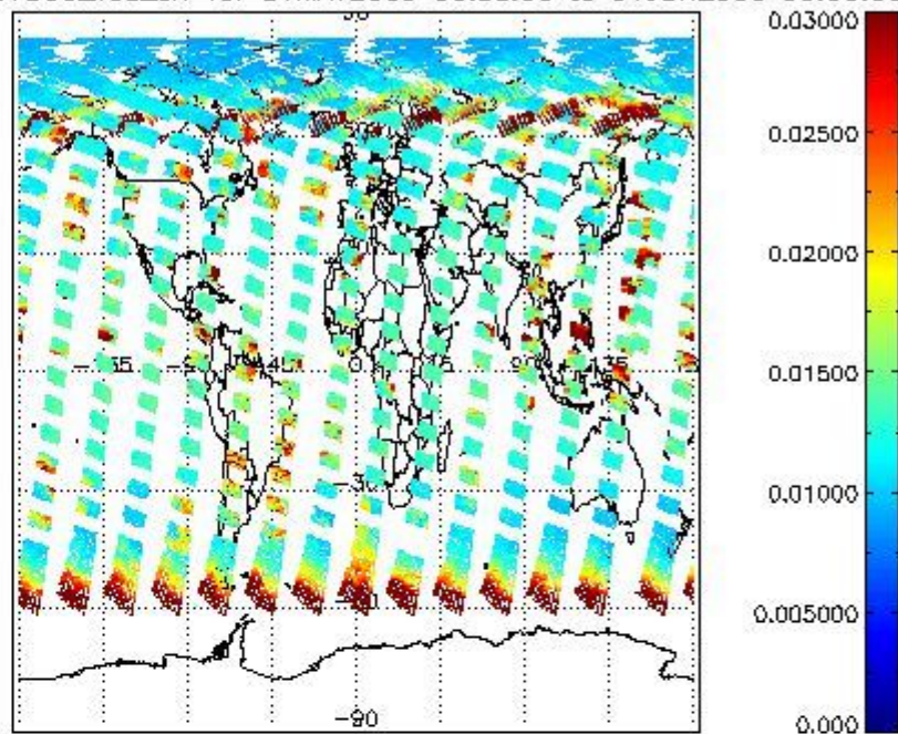
SCIOL2P_NADUV003_vcd_err for 31MAY2009 00:00:00 to 01JUN2009 00:00:00
