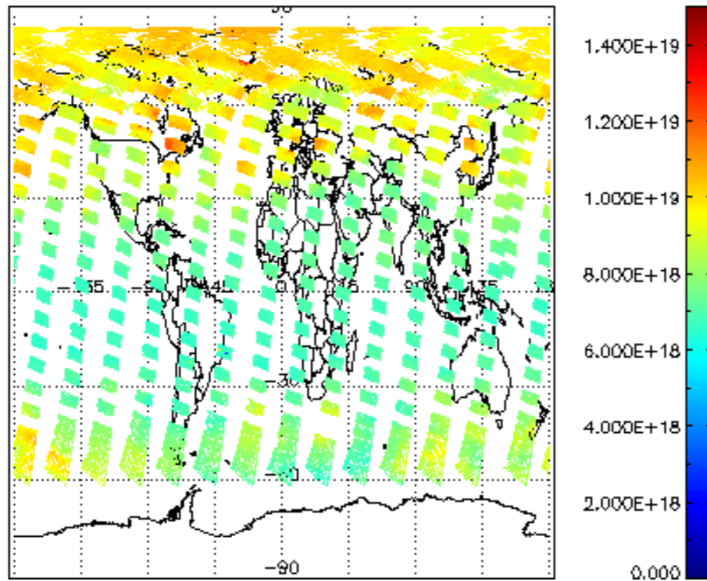
SCIOL2P_NADUV003_vcd for 31MAY2009 00:00:00 to 01JUN2009 00:00:00
