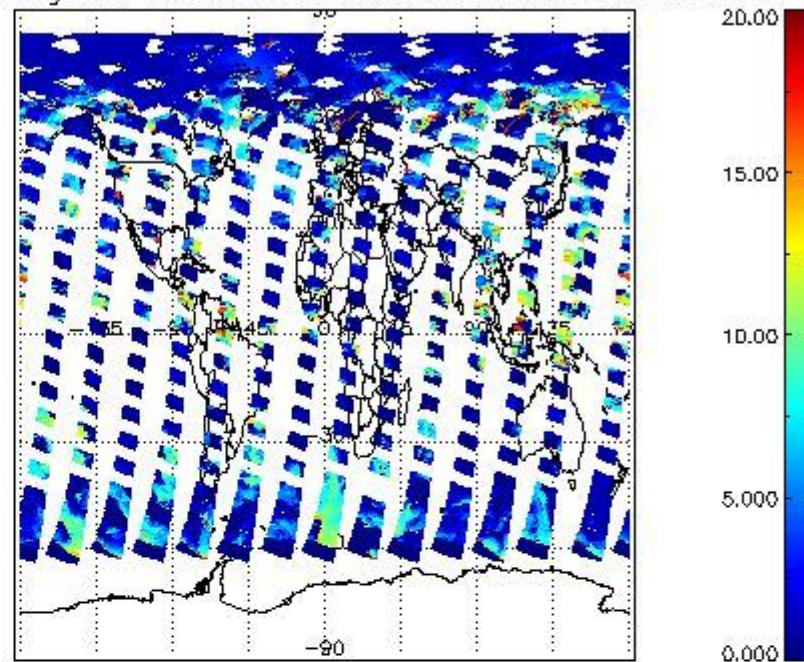
cL_top_height for 31MAY2009 00:00:00 to 01JUN2009 00:00:00
