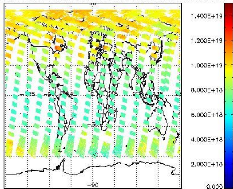
SCIOL2P_NADUV003_vcd for 31MAY2009 00:00:00 to 01JUN2009 00:00:00
