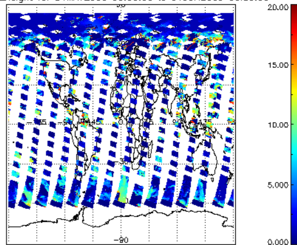
cl_top_height for 31MAY2009 00:00:00 to 01JUN2009 00:00:00
