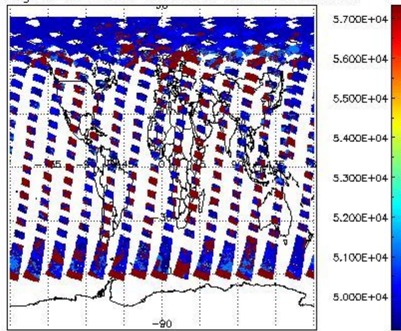
cloud_flags for 31MAY2009 00:00:00 to 01JUN2009 00:00:00
