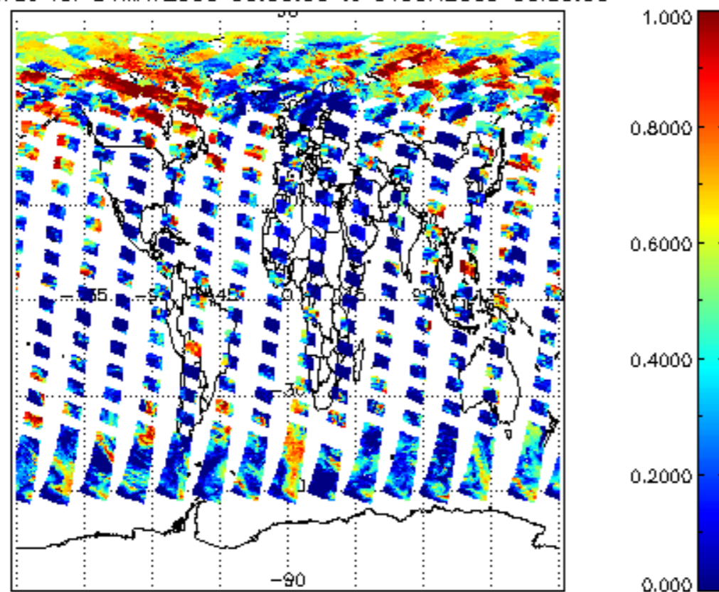
cl_frac for 31MAY2009 00:00:00 to 01JUN2009 00:00:00
