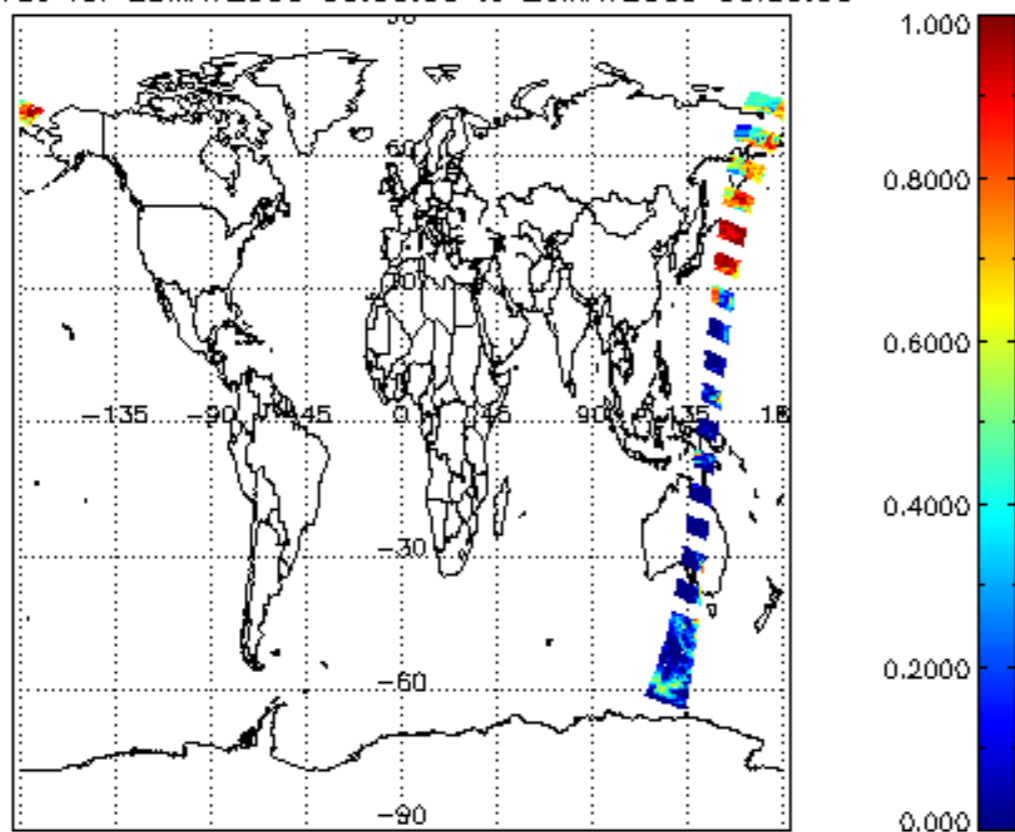
cl_frac for 25MAY2009 00:00:00 to 26MAY2009 00:00:00
