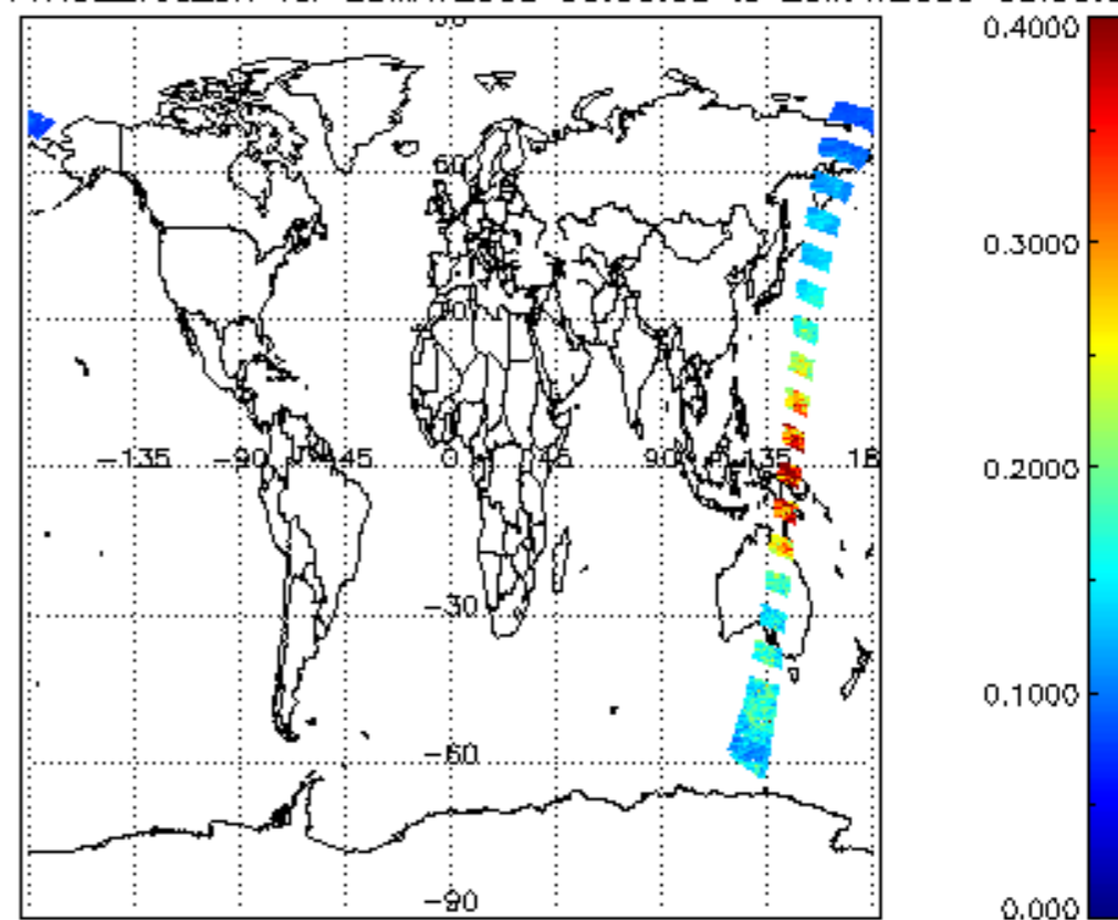
iCIOL2P_NADUV1NO2_vcd_err for 25MAY2009 00:00:00 to 26MAY2009 00:00:00
