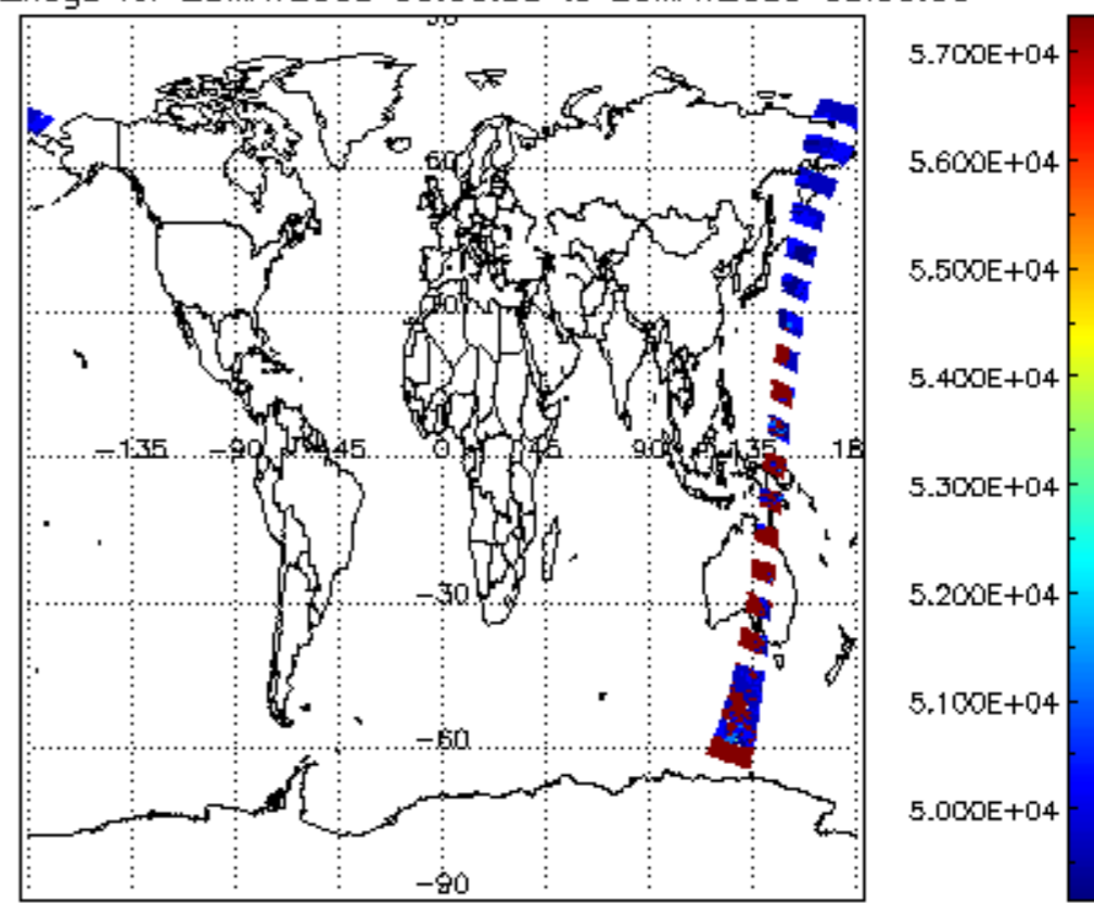
cloud_flags for 25MAY2009 00:00:00 to 26MAY2009 00:00:00
