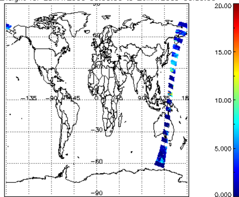
cl_top_height for 25MAY2009 00:00:00 to 26MAY2009 00:00:00
