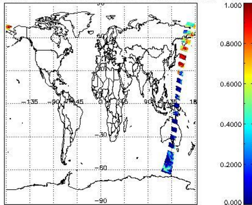
cL_frac for 25MAY2009 00:00:00 to 26MAY2009 00:00:00
