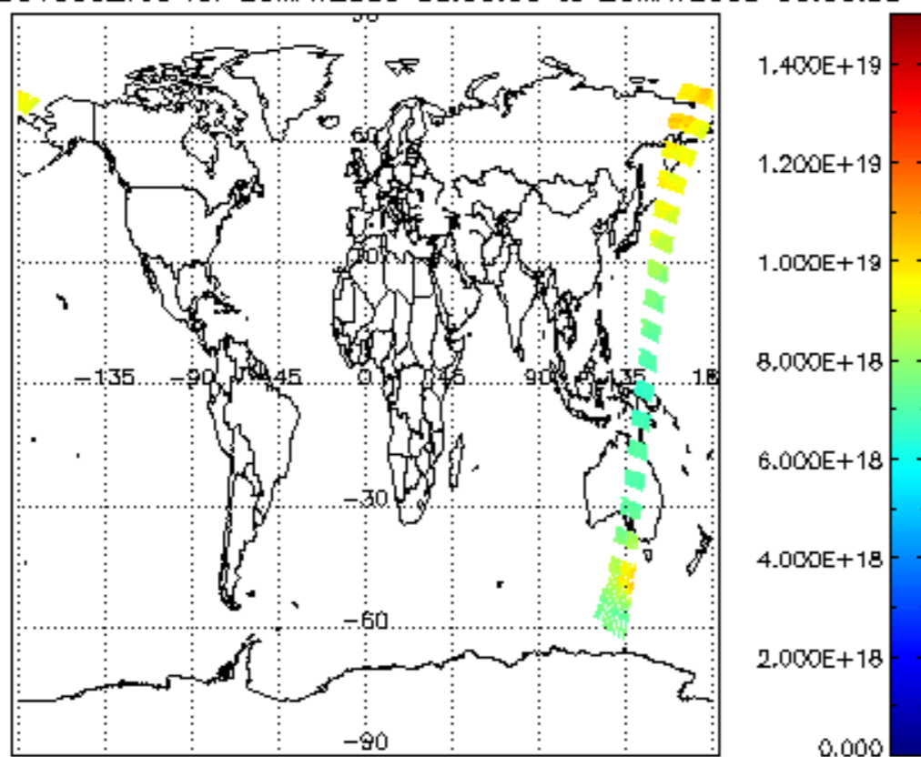
SCIOL2P_NADUV003_vcd for 25MAY2009 00:00:00 to 26MAY2009 00:00:00
