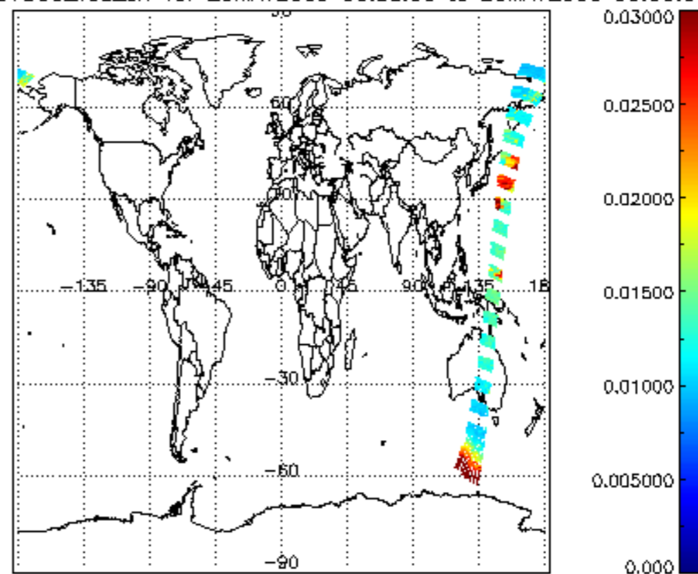
SCIOL2P_NADUV003_vcd_err for 25MAY2009 00:00:00 to 26MAY2009 00:00:00
