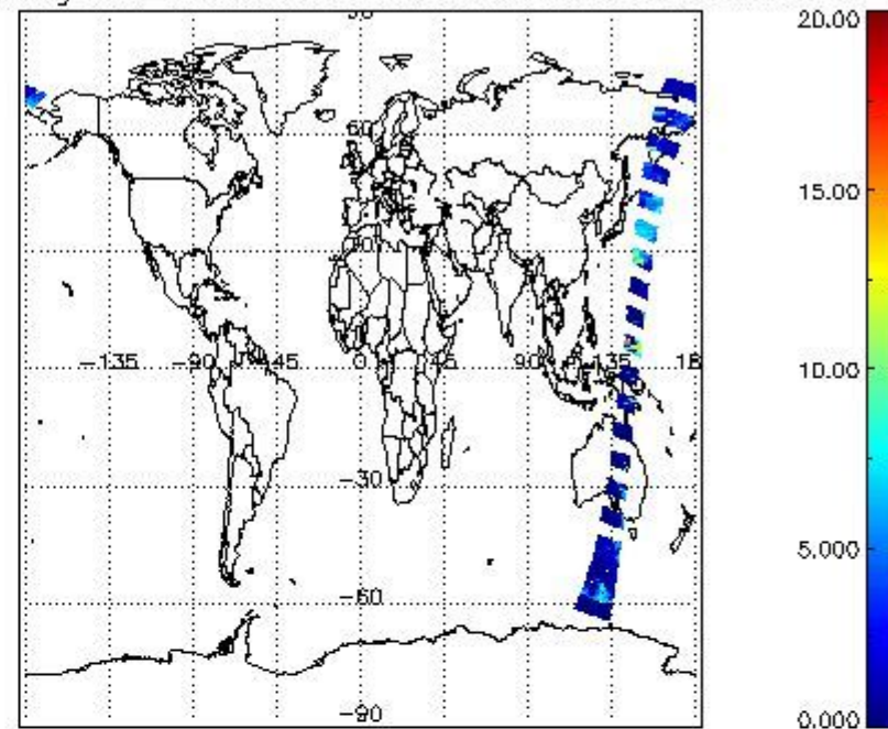
cL_top_height for 25MAY2009 00:00:00 to 26MAY2009 00:00:00
