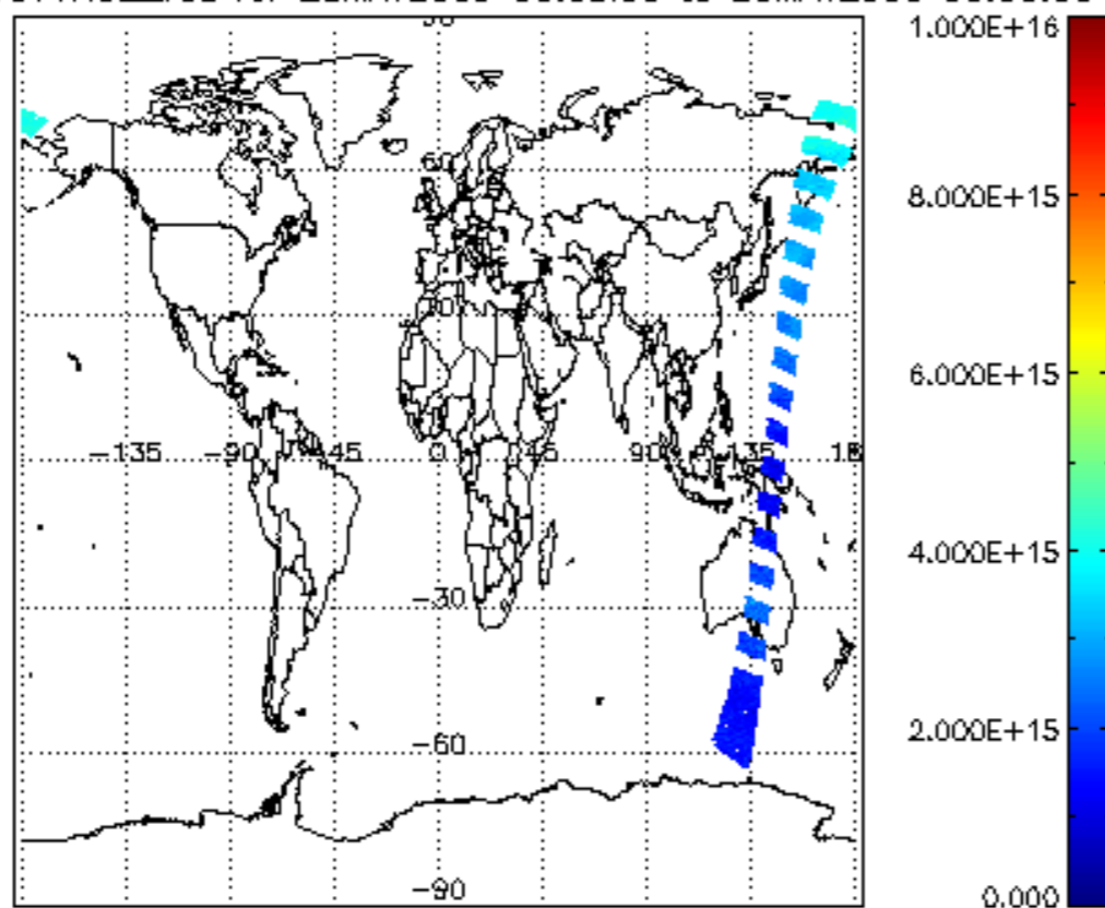
SCIOL2P_NADUV1NO2_vcd for 25MAY2009 00:00:00 to 26MAY2009 00:00:00
