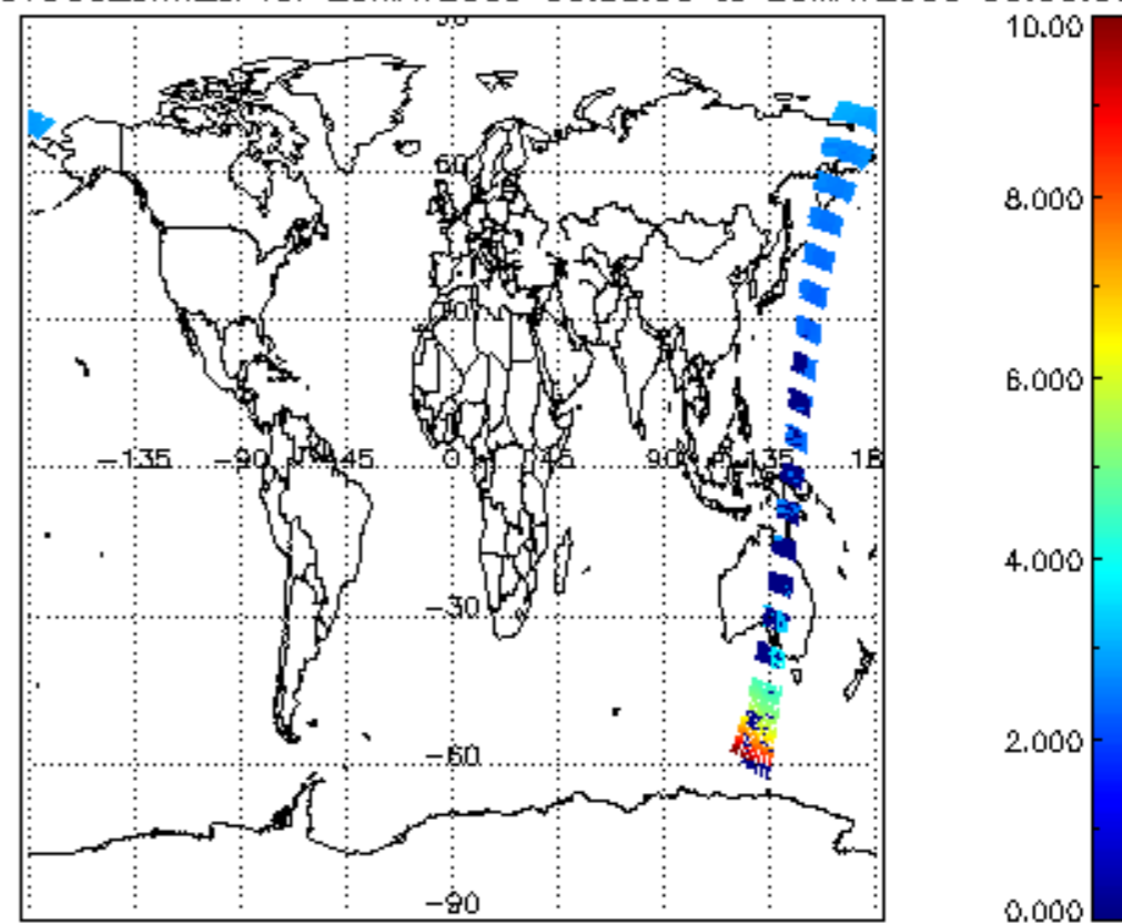
SCIOL2P_NADUV003_amf_cl for 25MAY2009 00:00:00 to 26MAY2009 00:00:00
