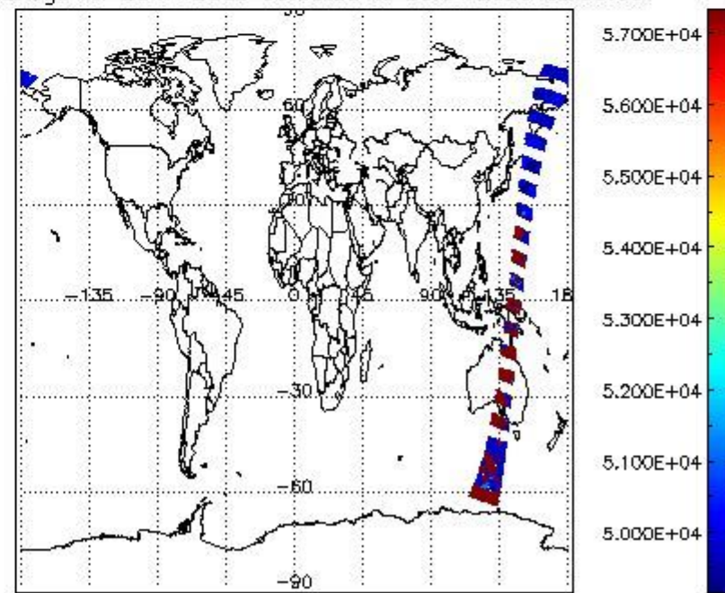
cloud_flags for 25MAY2009 00:00:00 to 26MAY2009 00:00:00
