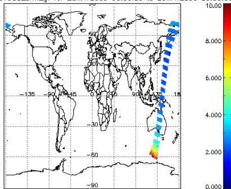
SCIOL2P_NADUV003_amf_gr for 25MAY2009 00:00:00 to 26MAY2009 00:00:00
