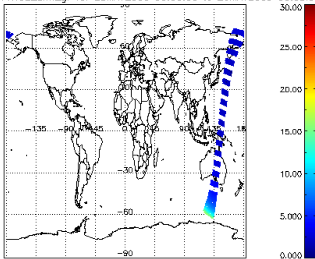
iCIOL2P_NADUV1NO2_amf_gr for 25MAY2009 00:00:00 to 26MAY2009 00:00:00
