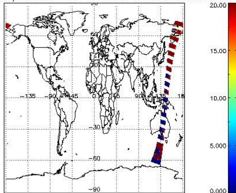
cL_opt_depth for 25MAY2009 00:00:00 to 26MAY2009 00:00:00
