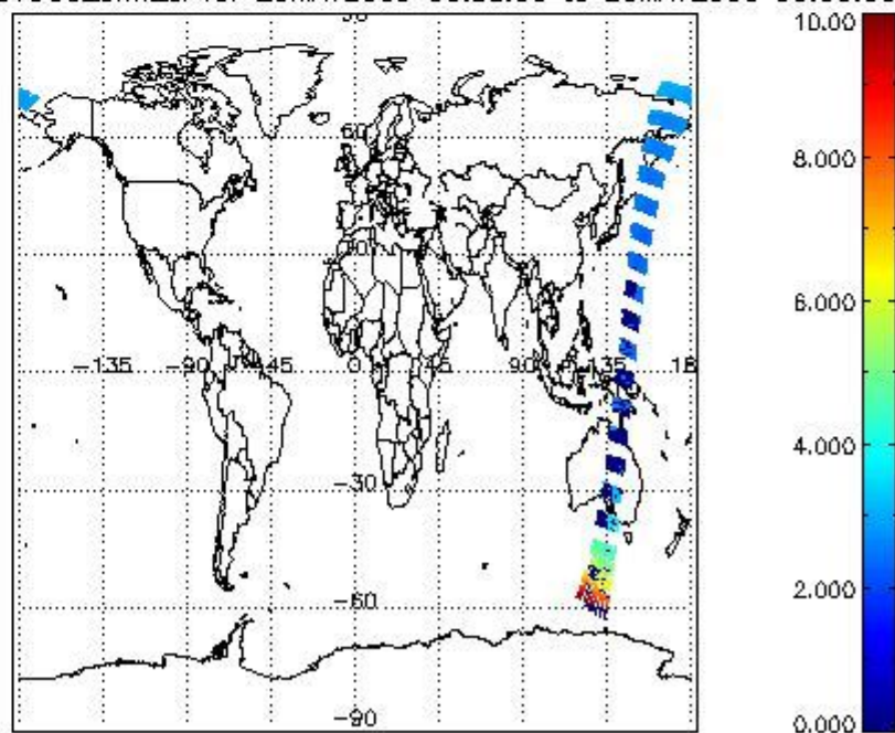
SCIOL2P_NADUV003_amf_cl for 25MAY2009 00:00:00 to 26MAY2009 00:00:00
