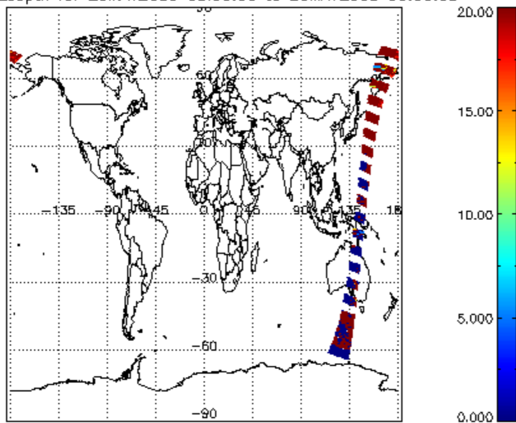
cl_opt_depth for 25MAY2009 00:00:00 to 26MAY2009 00:00:00
