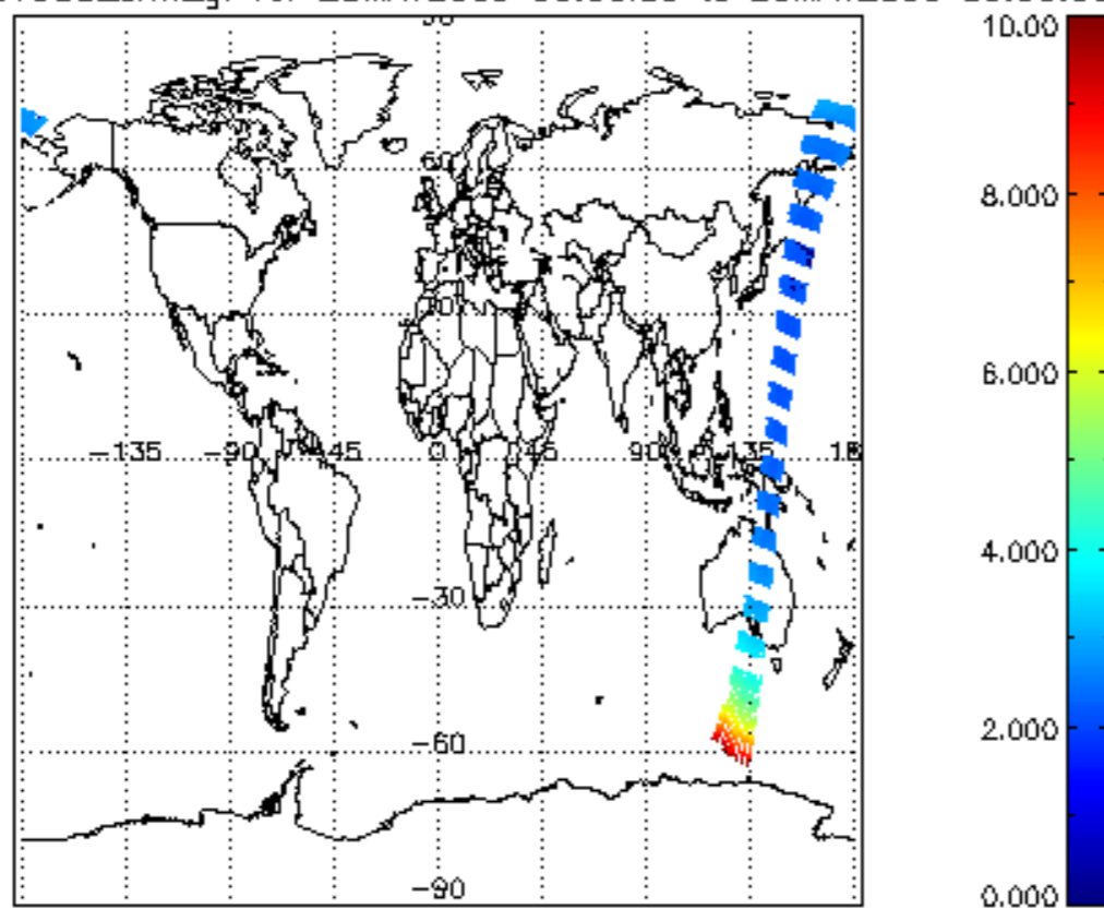
SCIOL2P_NADUV003_amf_gr for 25MAY2009 00:00:00 to 26MAY2009 00:00:00
