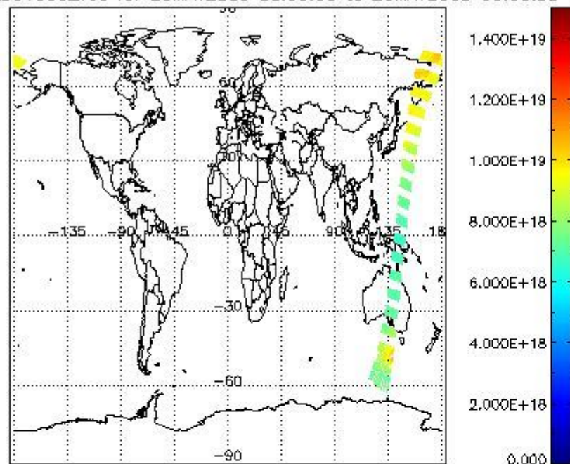
SCIOL2P_NADUV003_vcd for 25MAY2009 00:00:00 to 26MAY2009 00:00:00
