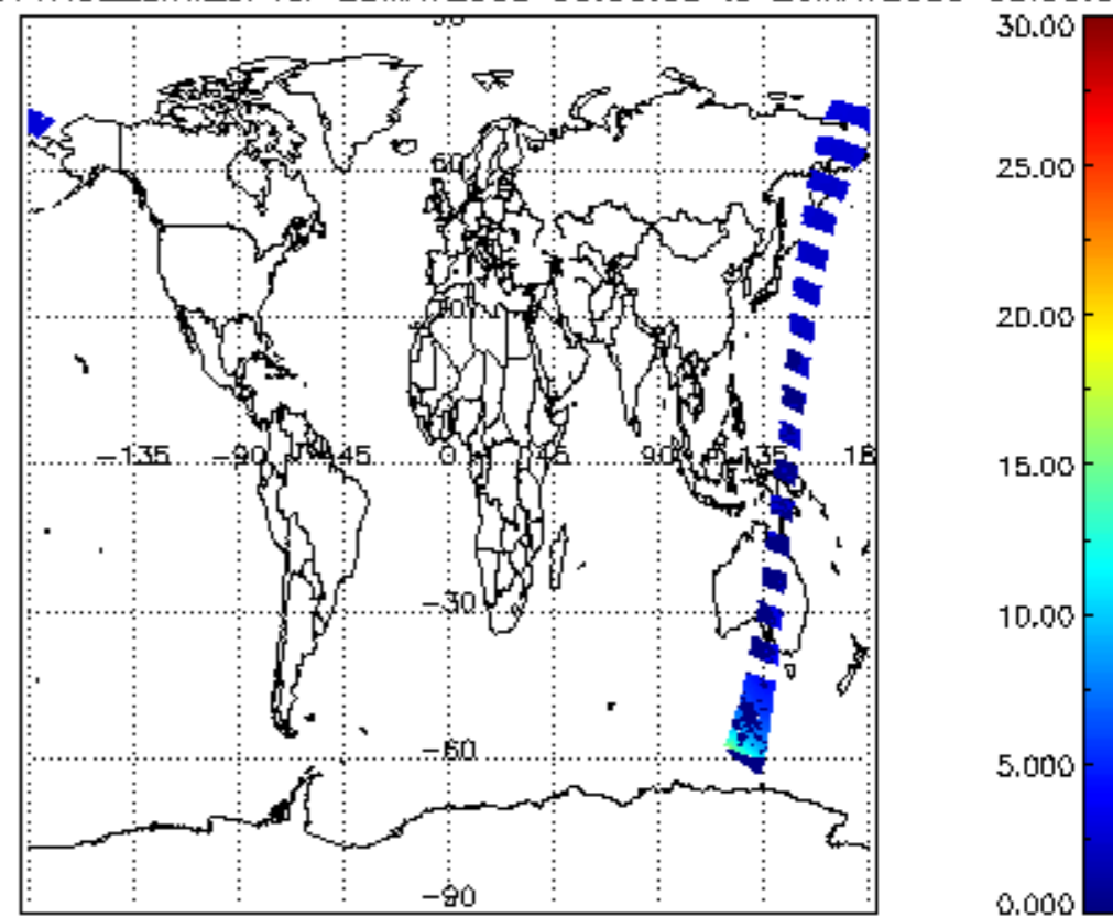
iCIOL2P_NADUV1NO2_amf_cl for 25MAY2009 00:00:00 to 26MAY2009 00:00:00
