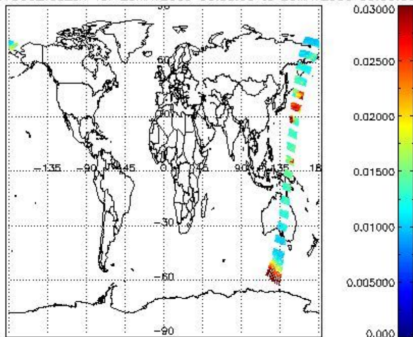
SCIOL2P_NADUV003_vcd_err for 25MAY2009 00:00:00 to 26MAY2009 00:00:00
