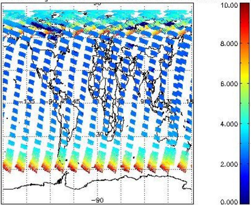
SCIOL2P_NADUV003_amf_gr for 22MAY2009 00:00:00 to 23MAY2009 00:00:00
