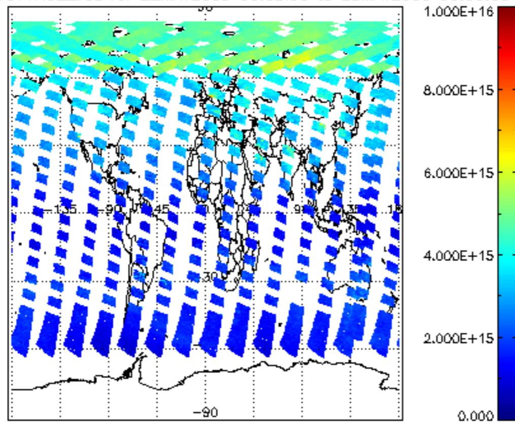
SCIOL2P_NADUV1NO2_vcd for 22MAY2009 00:00:00 to 23MAY2009 00:00:00
