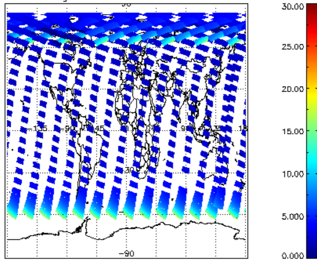
iCIOL2P_NADUV1NO2_amf_gr for 22MAY2009 00:00:00 to 23MAY2009 00:00:00
