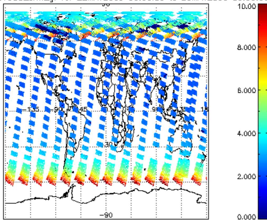
SCIOL2P_NADUV003_amf_gr for 22MAY2009 00:00:00 to 23MAY2009 00:00:00
