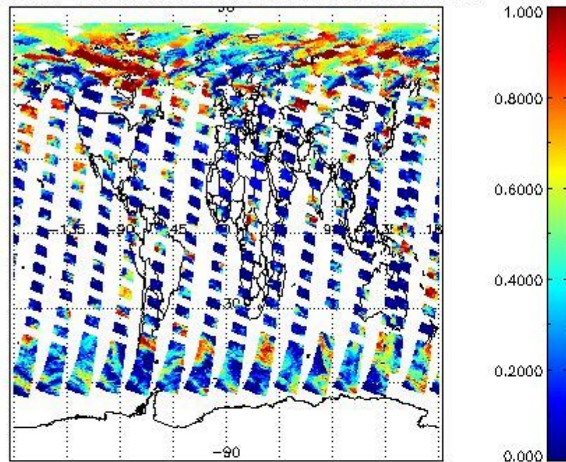
cL_frac for 22MAY2009 00:00:00 to 23MAY2009 00:00:00
