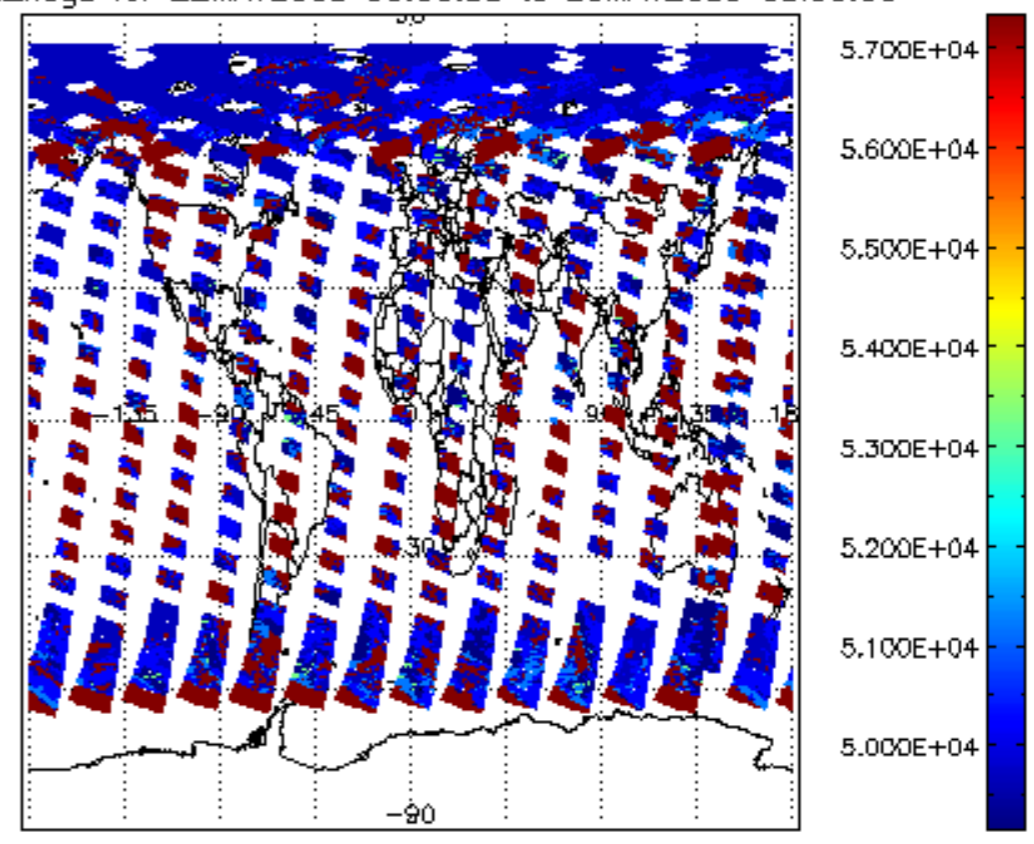
cloud_flags for 22MAY2009 00:00:00 to 23MAY2009 00:00:00
