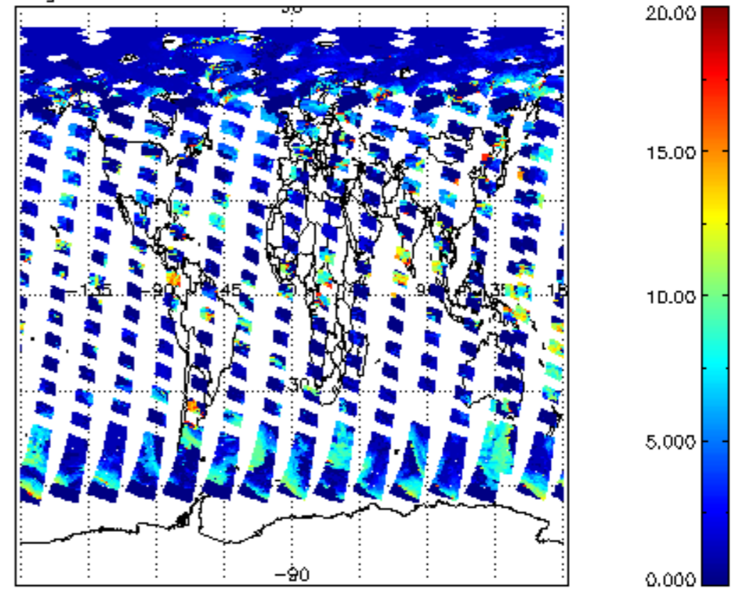
cl_top_height for 22MAY2009 00:00:00 to 23MAY2009 00:00:00
