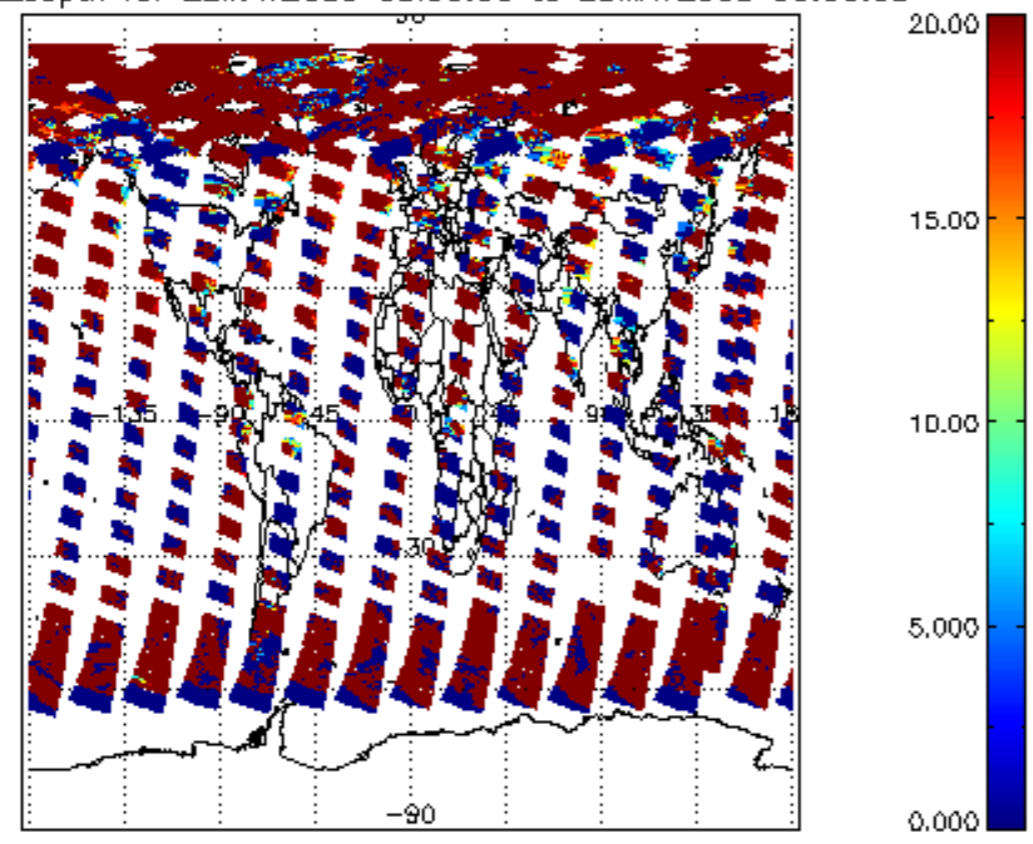
cl_opt_depth for 22MAY2009 00:00:00 to 23MAY2009 00:00:00
