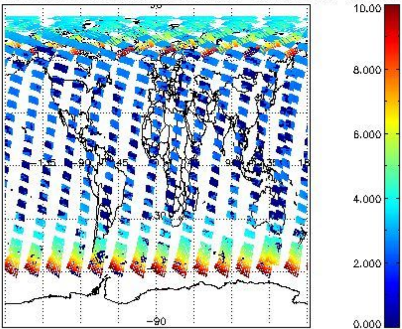
SCIOL2P_NADUV003_amf_cl for 22MAY2009 00:00:00 to 23MAY2009 00:00:00
