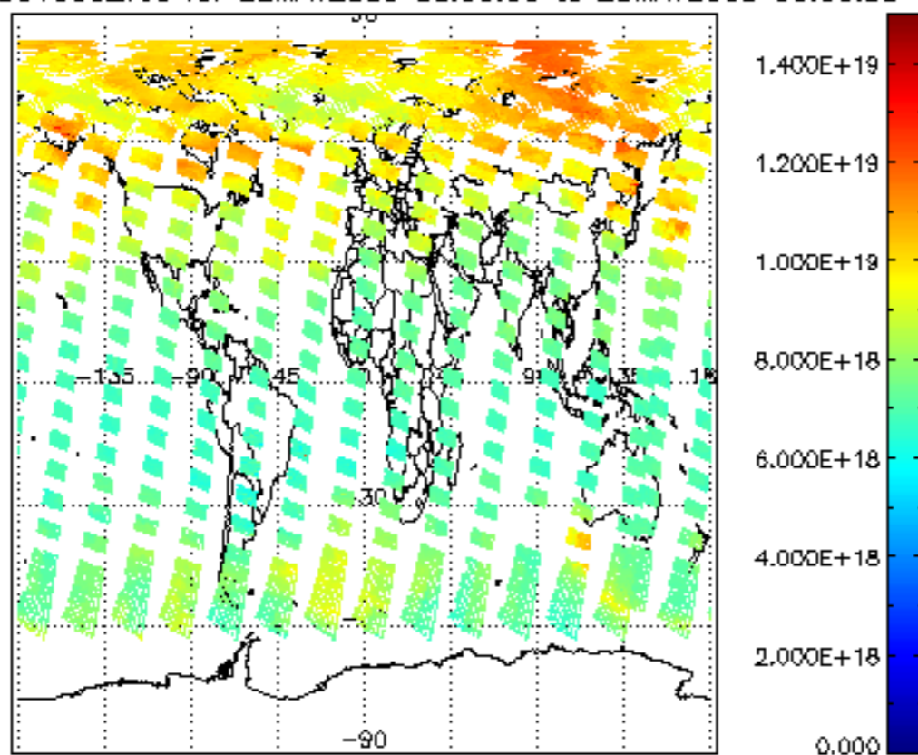
SCIOL2P_NADUV003_vcd for 22MAY2009 00:00:00 to 23MAY2009 00:00:00
