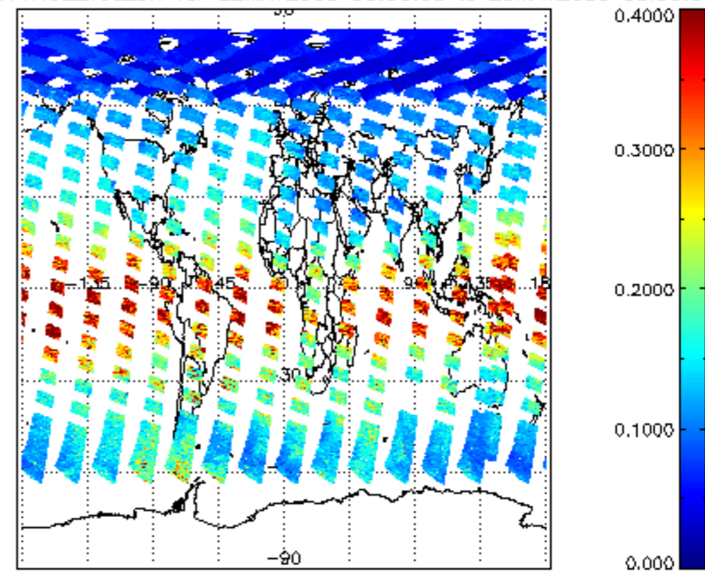
iCIOL2P_NADUV1NO2_vcd_err for 22MAY2009 00:00:00 to 23MAY2009 00:00:00
