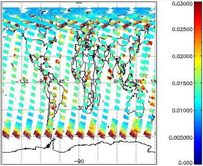
SCIOL2P_NADUV003_vcd_err for 22MAY2009 00:00:00 to 23MAY2009 00:00:00
