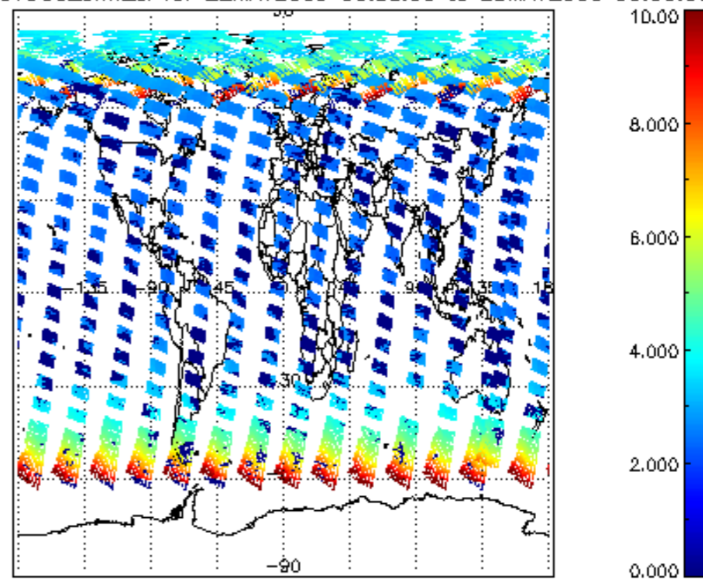
SCIOL2P_NADUV003_amf_cl for 22MAY2009 00:00:00 to 23MAY2009 00:00:00
