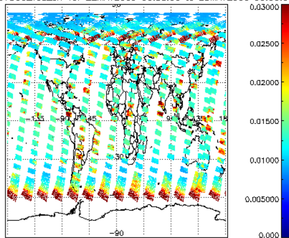
SCIOL2P_NADUV003_vcd_err for 22MAY2009 00:00:00 to 23MAY2009 00:00:00
