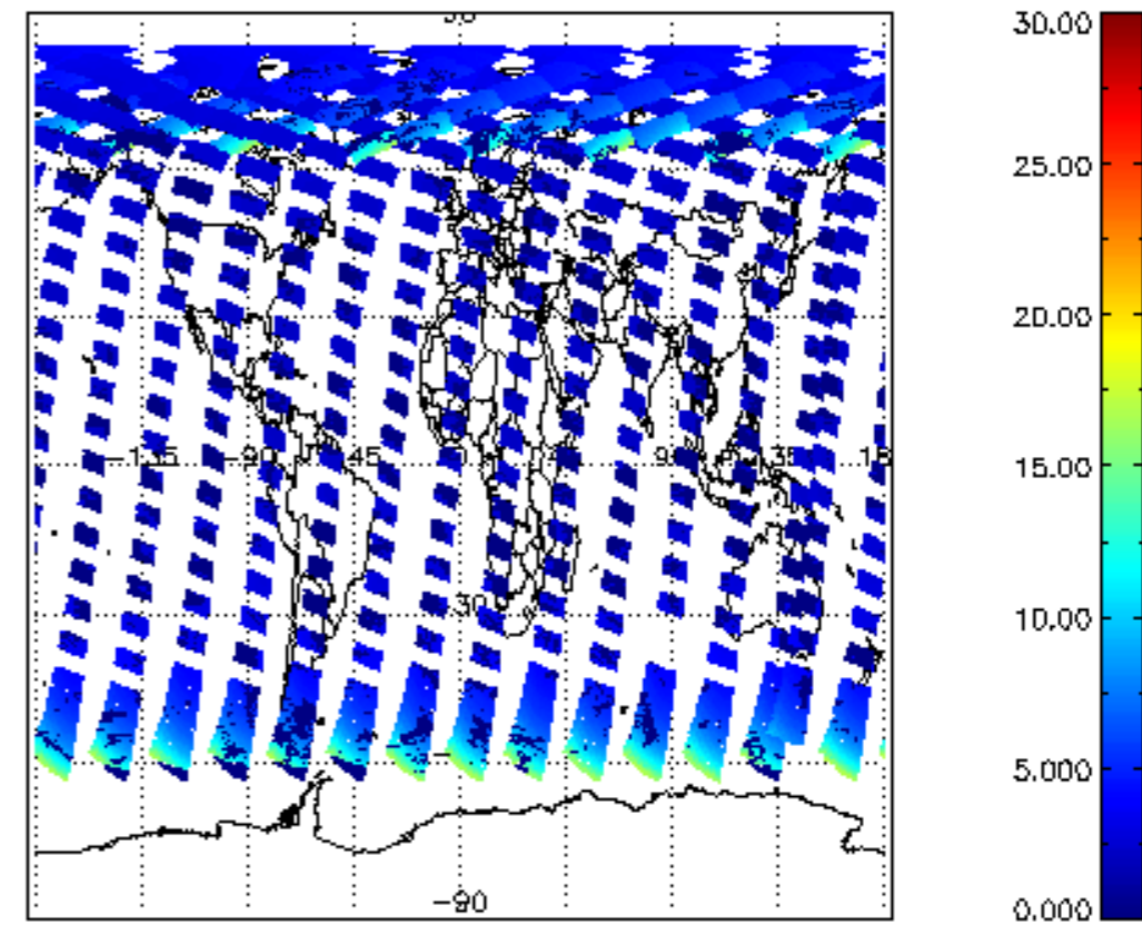
iCIOL2P_NADUV1NO2_amf_cl for 22MAY2009 00:00:00 to 23MAY2009 00:00:00
