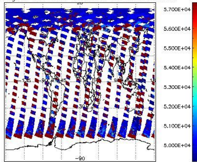
cloud_flags for 22MAY2009 00:00:00 to 23MAY2009 00:00:00
