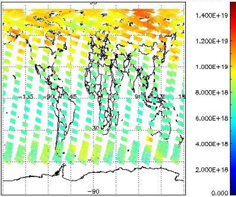
SCIOL2P_NADUV003_vcd for 22MAY2009 00:00:00 to 23MAY2009 00:00:00
