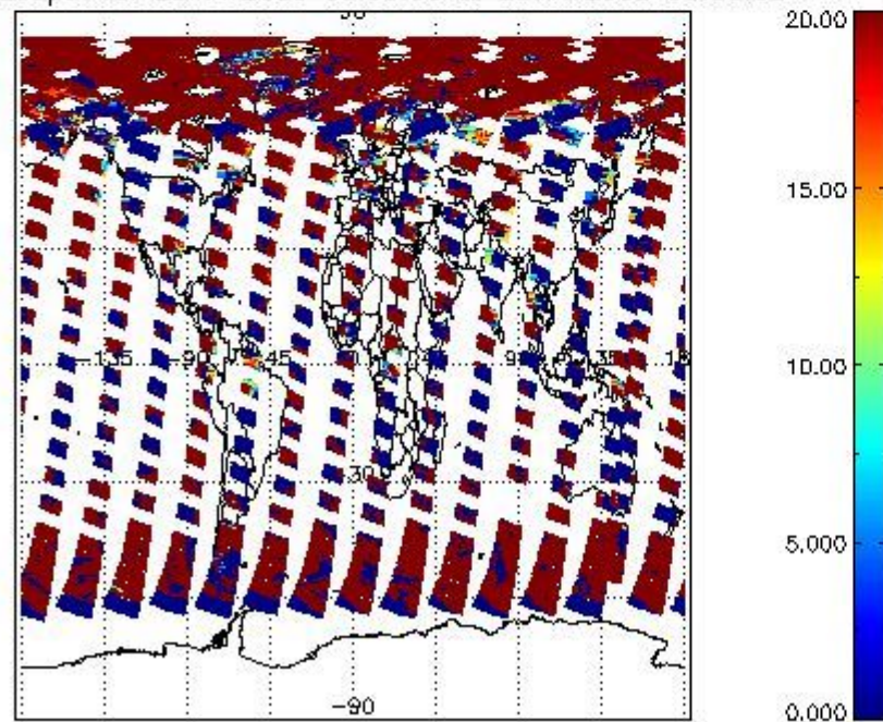
cL_opt_depth for 22MAY2009 00:00:00 to 23MAY2009 00:00:00
