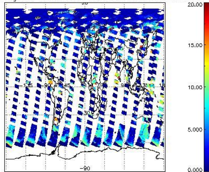
cL_top_height for 22MAY2009 00:00:00 to 23MAY2009 00:00:00
