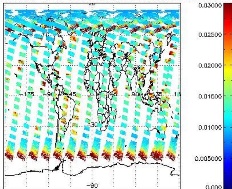
SCIOL2P_NADUV003_vcd_err for 19MAY2009 00:00:00 to 20MAY2009 00:00:00
