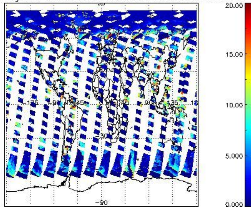
cL_top_height for 19MAY2009 00:00:00 to 20MAY2009 00:00:00
