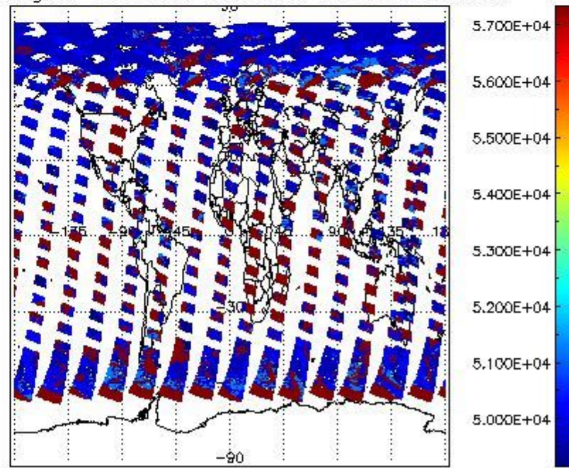
cloud_flags for 19MAY2009 00:00:00 to 20MAY2009 00:00:00
