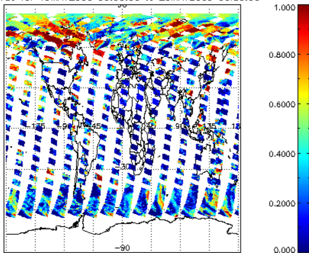
cl_frac for 19MAY2009 00:00:00 to 20MAY2009 00:00:00
