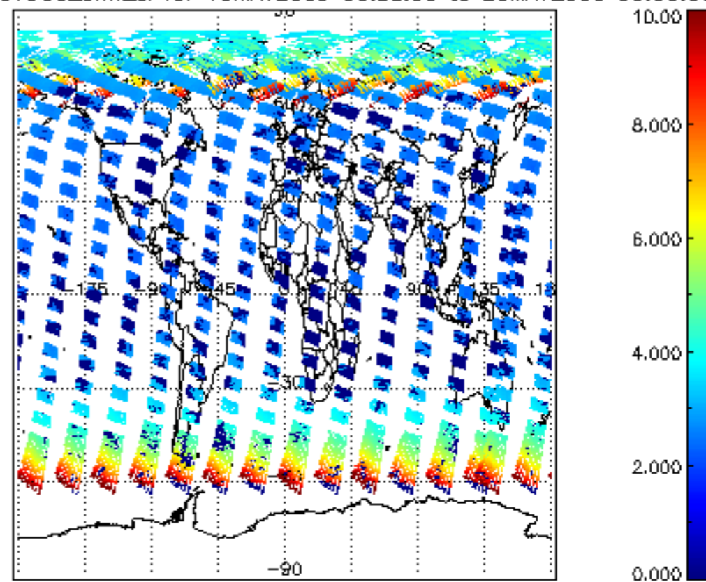
SCIOL2P_NADUV003_amf_cl for 19MAY2009 00:00:00 to 20MAY2009 00:00:00
