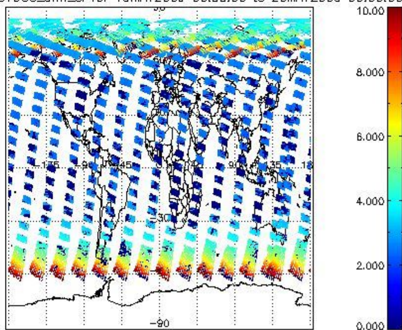
SCIOL2P_NADUV003_amf_cl for 19MAY2009 00:00:00 to 20MAY2009 00:00:00
