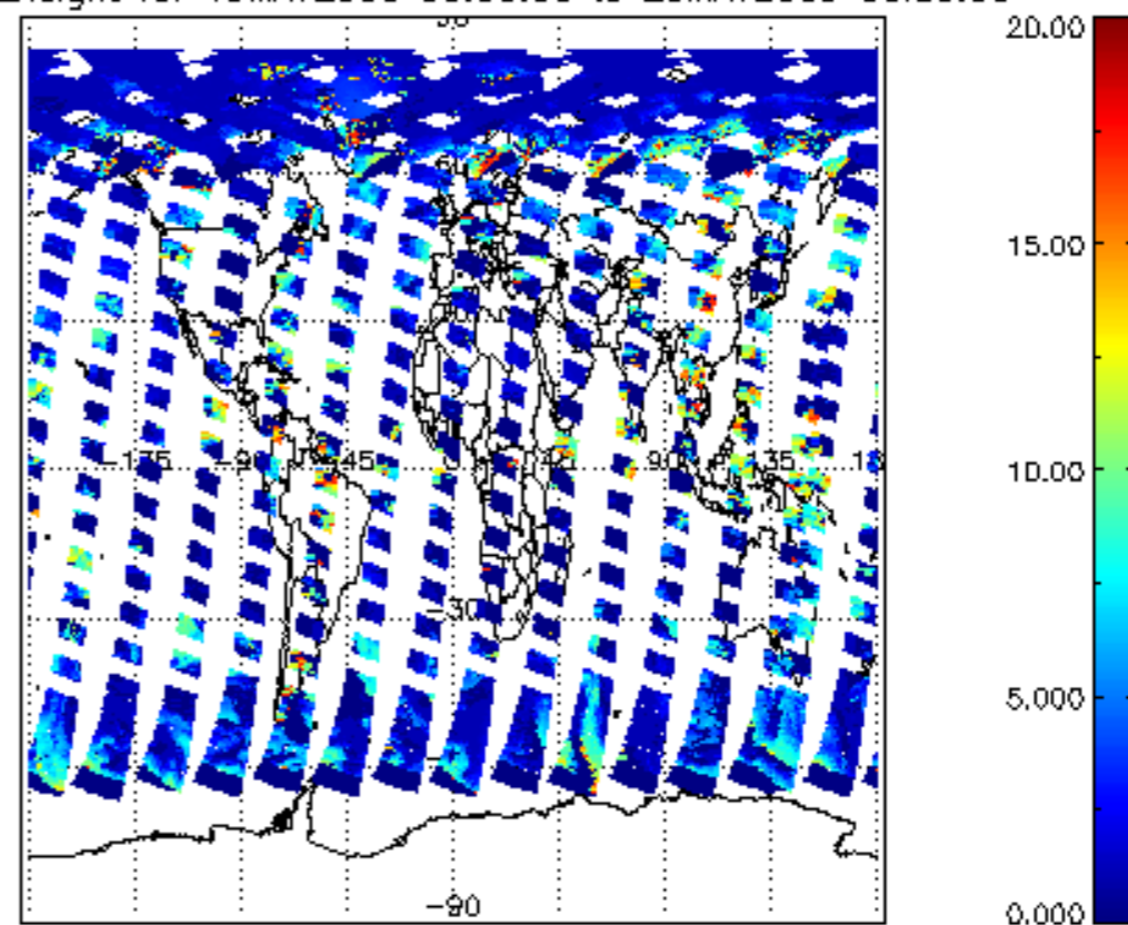
cl_top_height for 19MAY2009 00:00:00 to 20MAY2009 00:00:00
