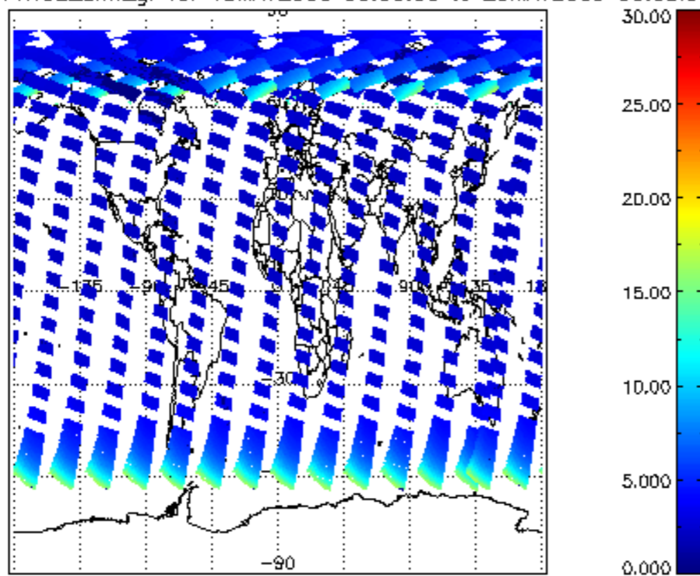
iCIOL2P_NADUV1NO2_amf_gr for 19MAY2009 00:00:00 to 20MAY2009 00:00:00
