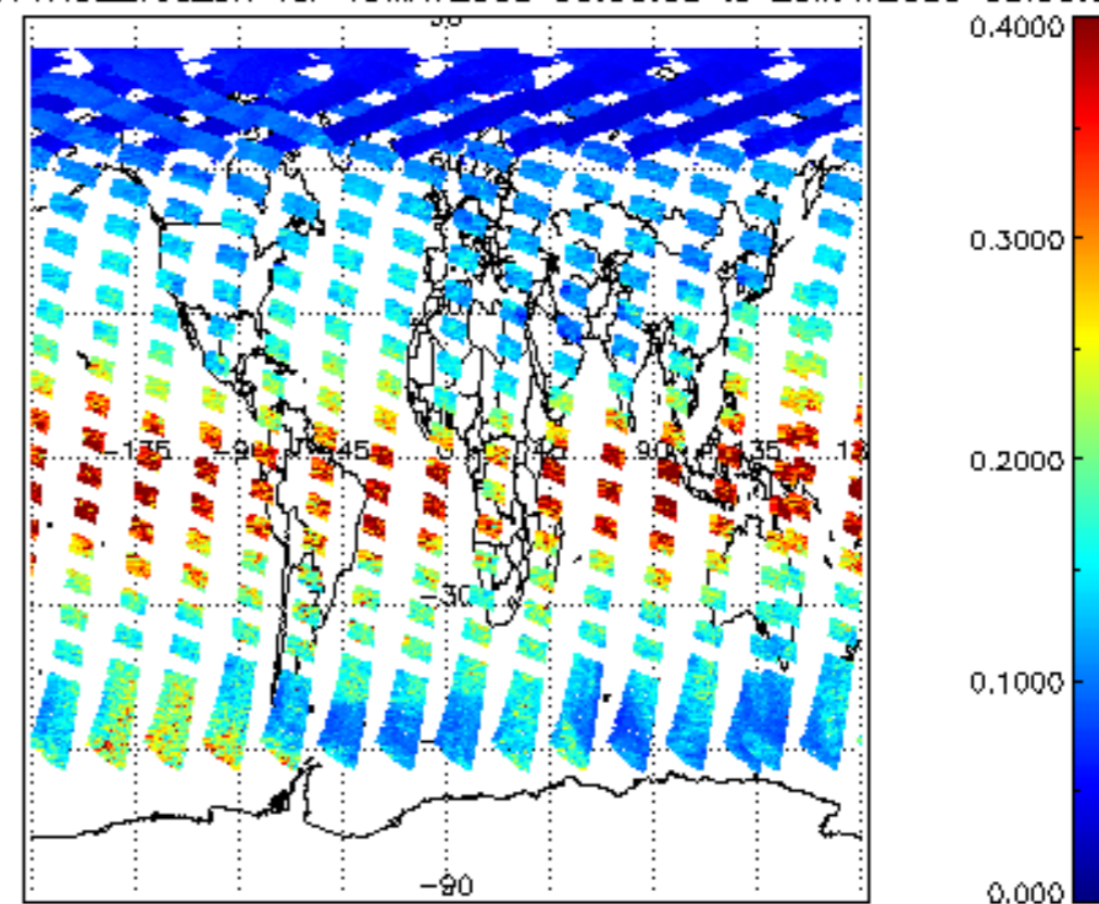
iCIOL2P_NADUV1NO2_vcd_err for 19MAY2009 00:00:00 to 20MAY2009 00:00:00
