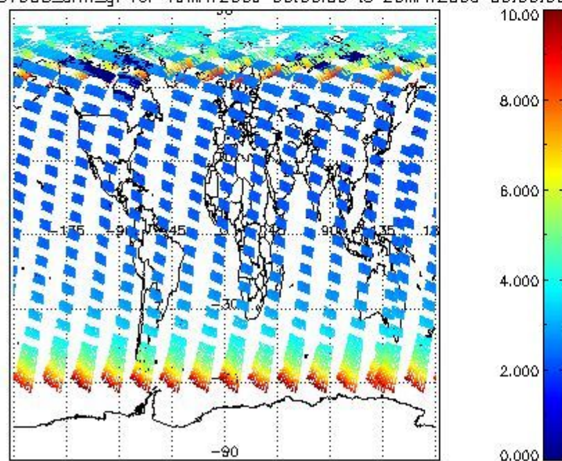
SCIOL2P_NADUV003_amf_gr for 19MAY2009 00:00:00 to 20MAY2009 00:00:00
