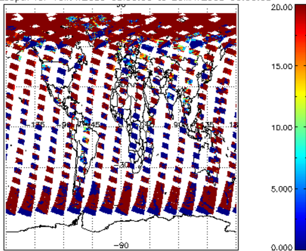
cl_opt_depth for 19MAY2009 00:00:00 to 20MAY2009 00:00:00
