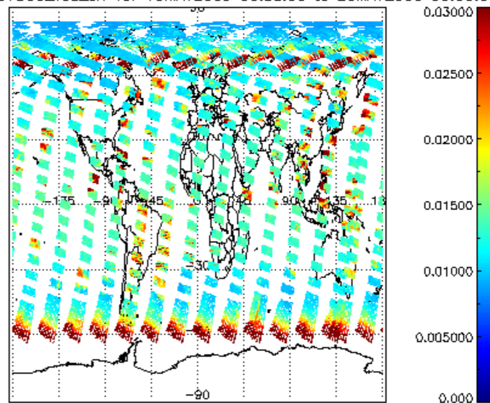
SCIOL2P_NADUV003_vcd_err for 19MAY2009 00:00:00 to 20MAY2009 00:00:00
