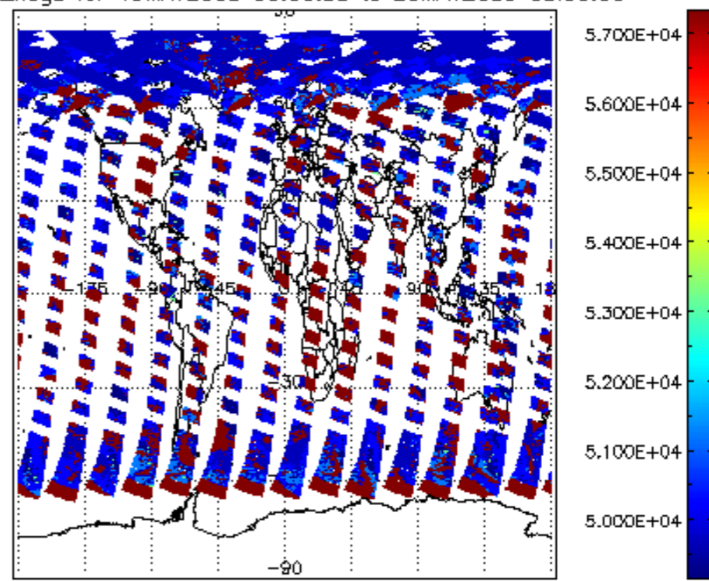
cloud_flags for 19MAY2009 00:00:00 to 20MAY2009 00:00:00
