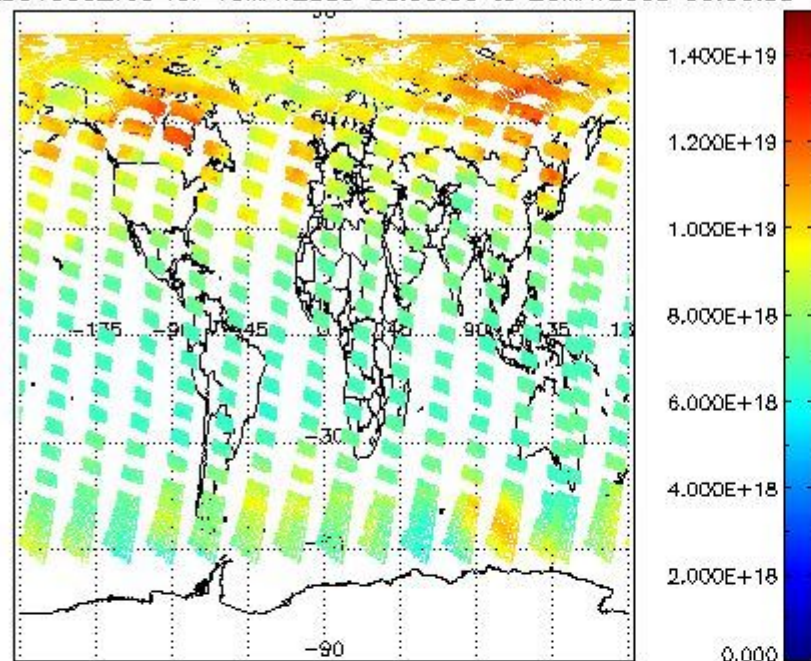
SCIOL2P_NADUV003_vcd for 19MAY2009 00:00:00 to 20MAY2009 00:00:00
