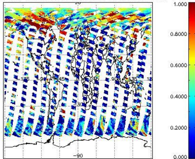
cL_frac for 19MAY2009 00:00:00 to 20MAY2009 00:00:00
