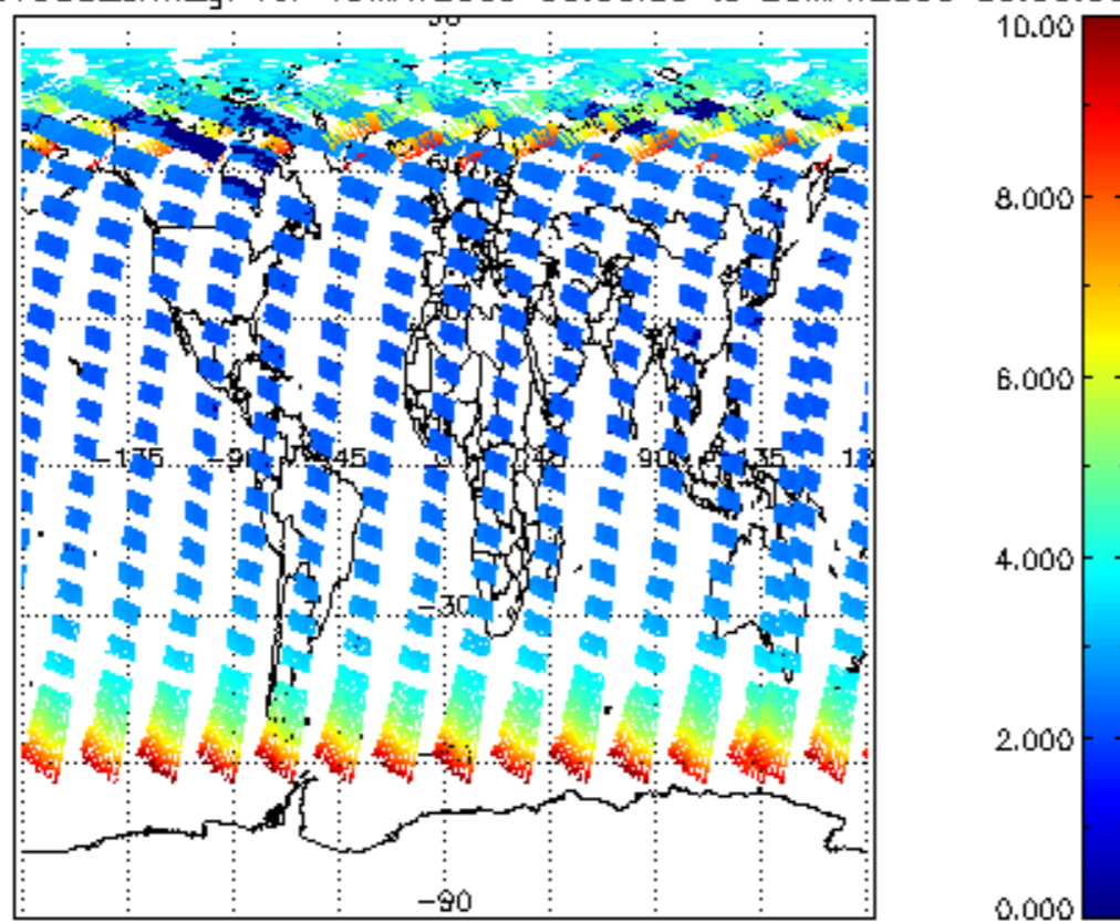
SCIOL2P_NADUV003_amf_gr for 19MAY2009 00:00:00 to 20MAY2009 00:00:00
