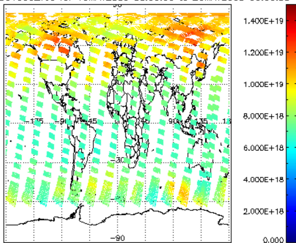
SCIOL2P_NADUV003_vcd for 19MAY2009 00:00:00 to 20MAY2009 00:00:00
