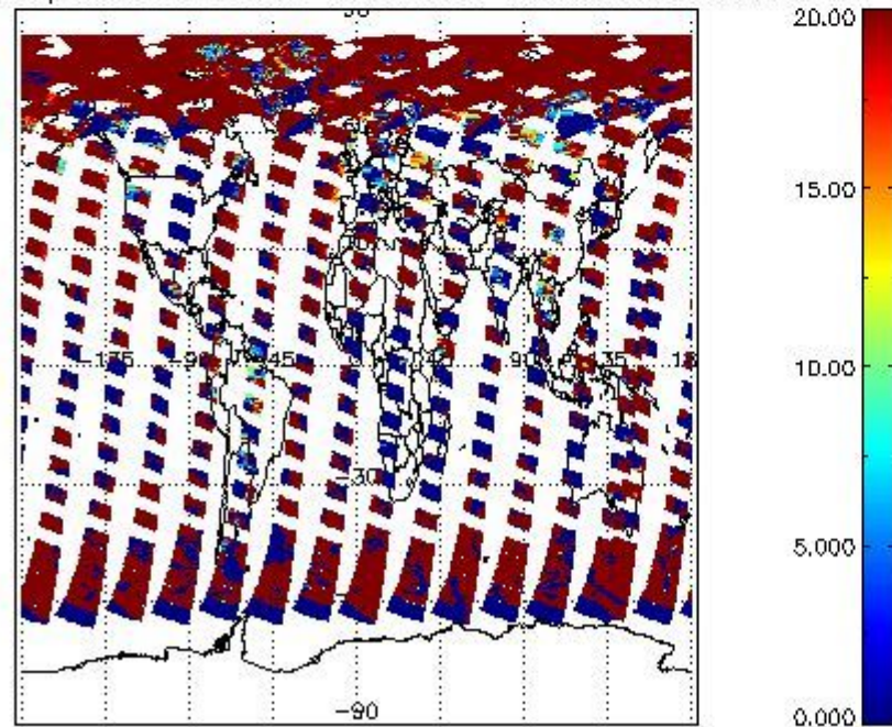
cL_opt_depth for 19MAY2009 00:00:00 to 20MAY2009 00:00:00
