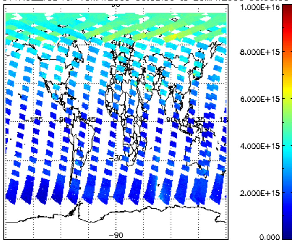
SCIOL2P_NADUV1NO2_vcd for 19MAY2009 00:00:00 to 20MAY2009 00:00:00
