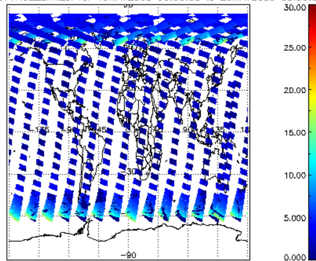
iCIOL2P_NADUV1NO2_amf_cl for 19MAY2009 00:00:00 to 20MAY2009 00:00:00
