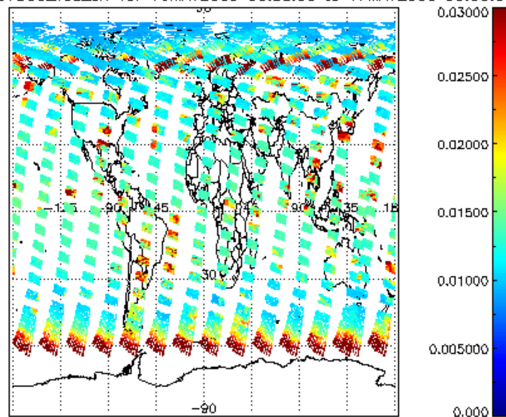
SCIOL2P_NADUV003_vcd_err for 16MAY2009 00:00:00 to 17MAY2009 00:00:00
