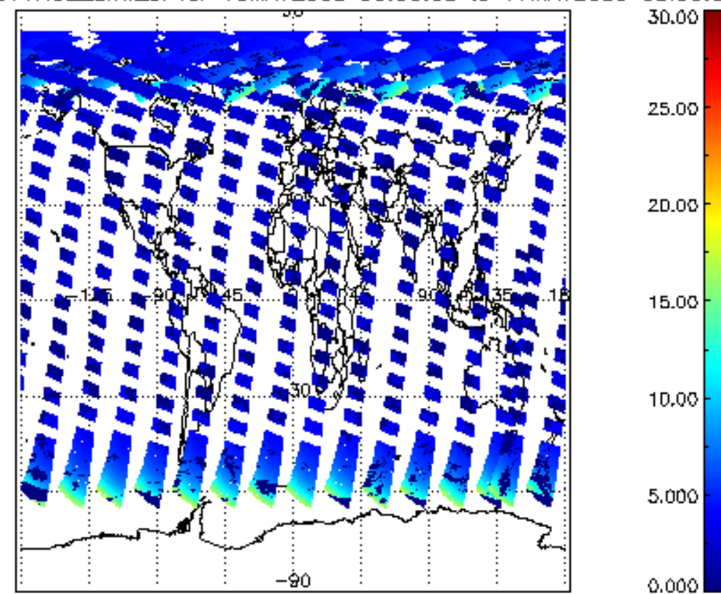
iCIOL2P_NADUV1NO2_amf_cl for 16MAY2009 00:00:00 to 17MAY2009 00:00:00
