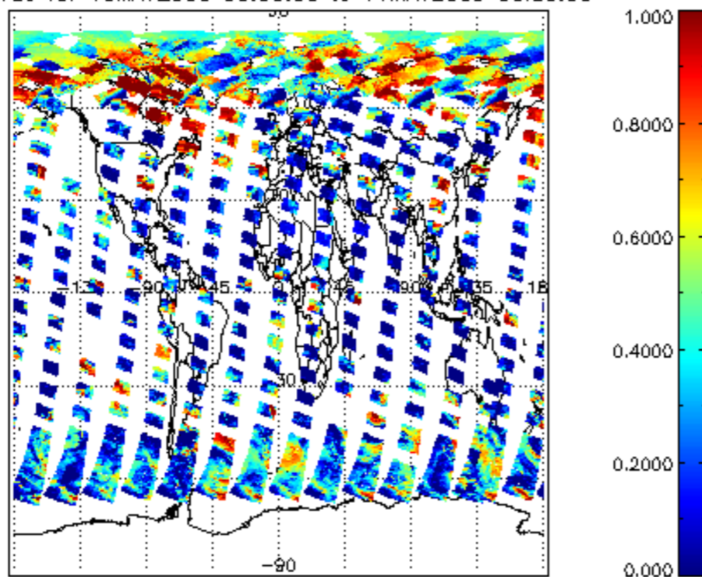
cl_frac for 10MAY2009 00:00:00 to 11MAY2009 00:00:00
