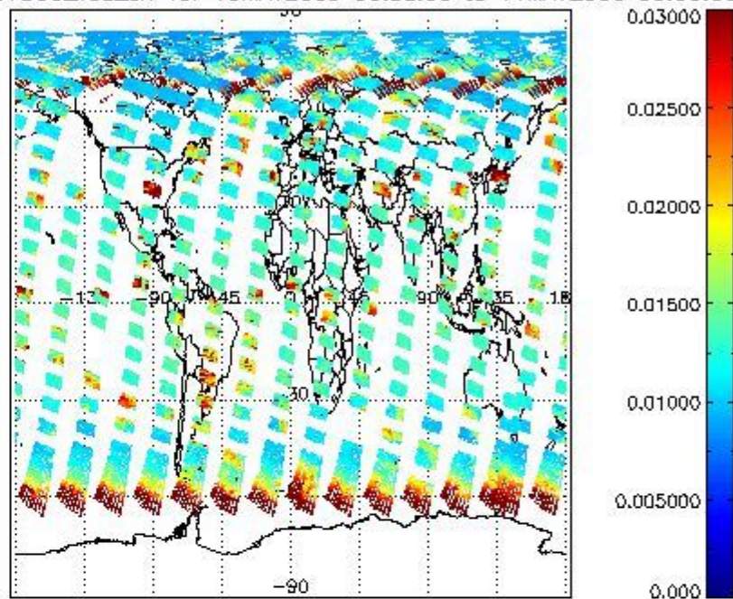
SCIOL2P_NADUV003_vcd_err for 10MAY2009 00:00:00 to 11MAY2009 00:00:00
