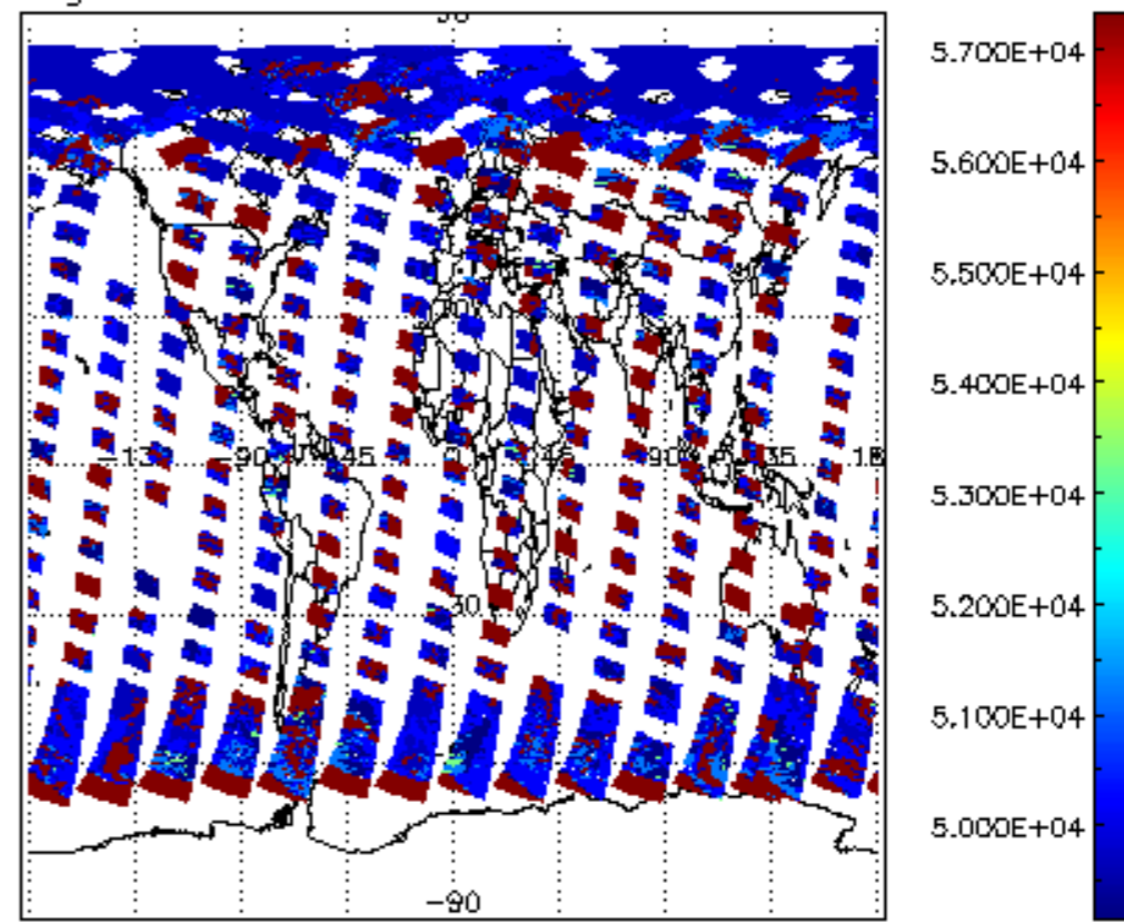
cloud_flags for 10MAY2009 00:00:00 to 11MAY2009 00:00:00
