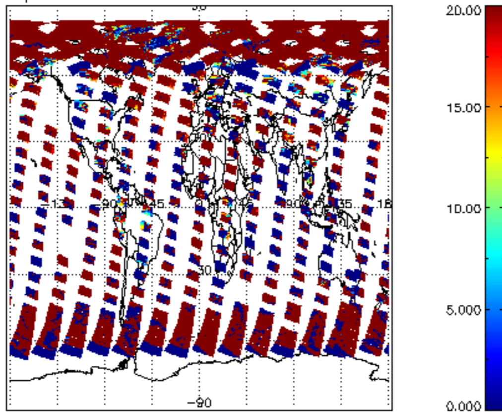
cl_opt_depth for 10MAY2009 00:00:00 to 11MAY2009 00:00:00
