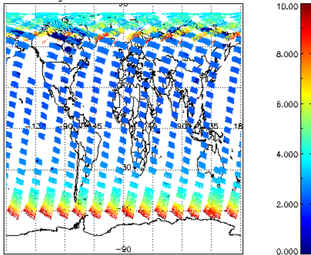
SCIOL2P_NADUV003_amf_gr for 10MAY2009 00:00:00 to 11MAY2009 00:00:00
