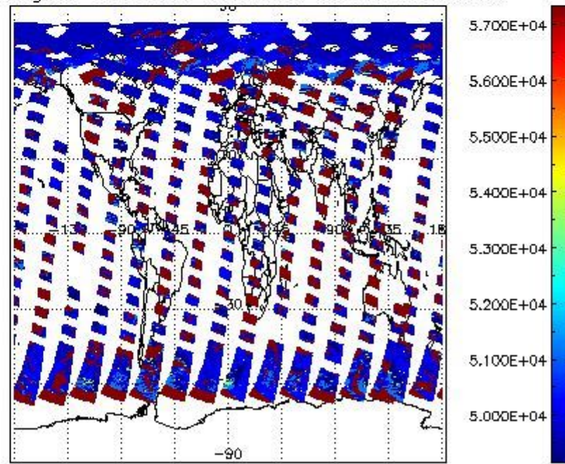
cloud_flags for 10MAY2009 00:00:00 to 11MAY2009 00:00:00
