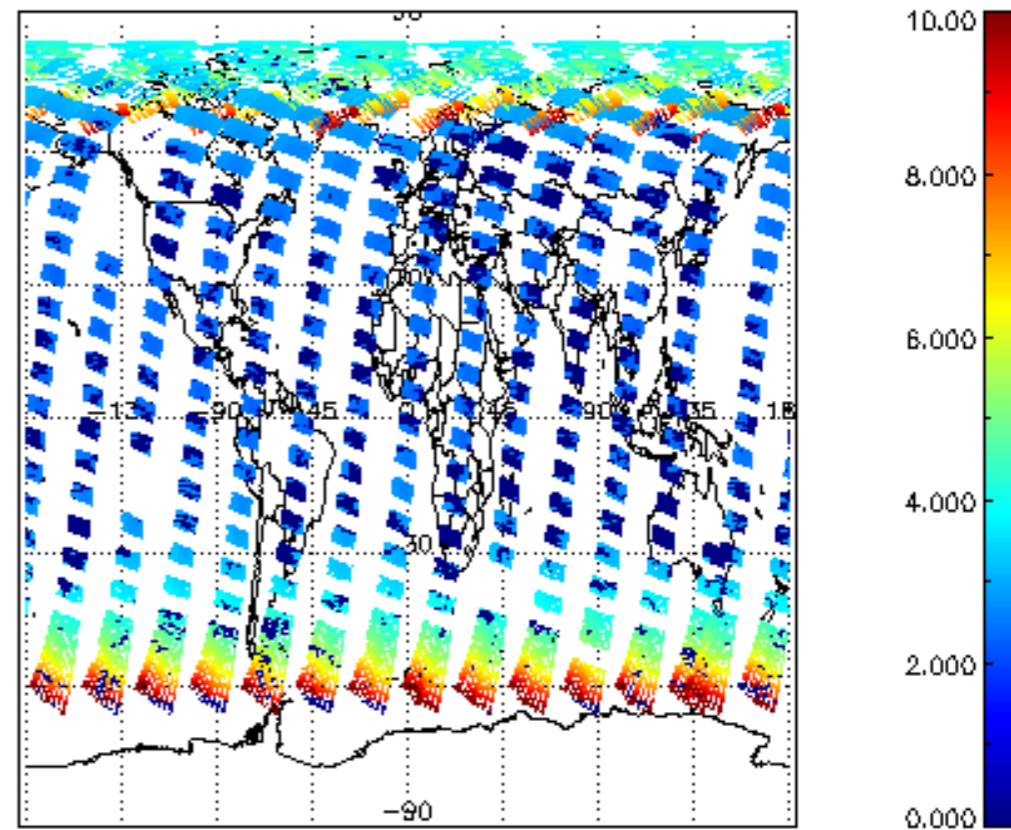
SCIOL2P_NADUV003_amf_cl for 10MAY2009 00:00:00 to 11MAY2009 00:00:00
