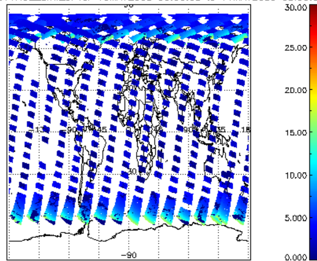
iCIOL2P_NADUV1NO2_amf_cl for 10MAY2009 00:00:00 to 11MAY2009 00:00:00
