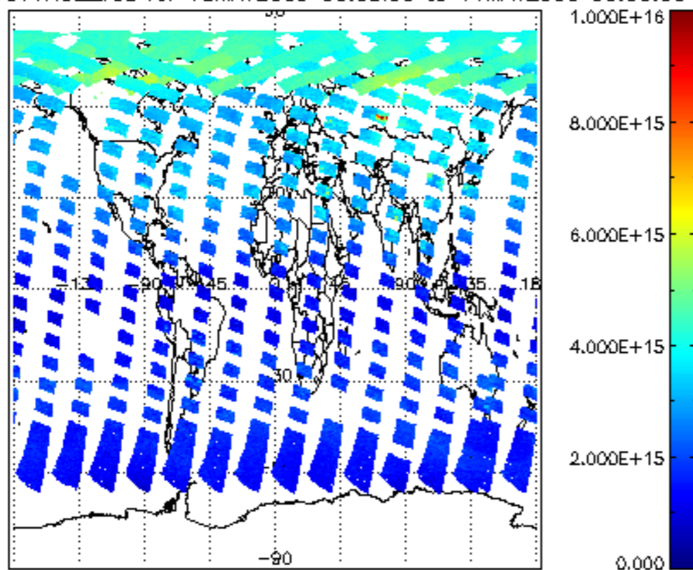
SCIOL2P_NADUV1NO2_vcd for 10MAY2009 00:00:00 to 11MAY2009 00:00:00
