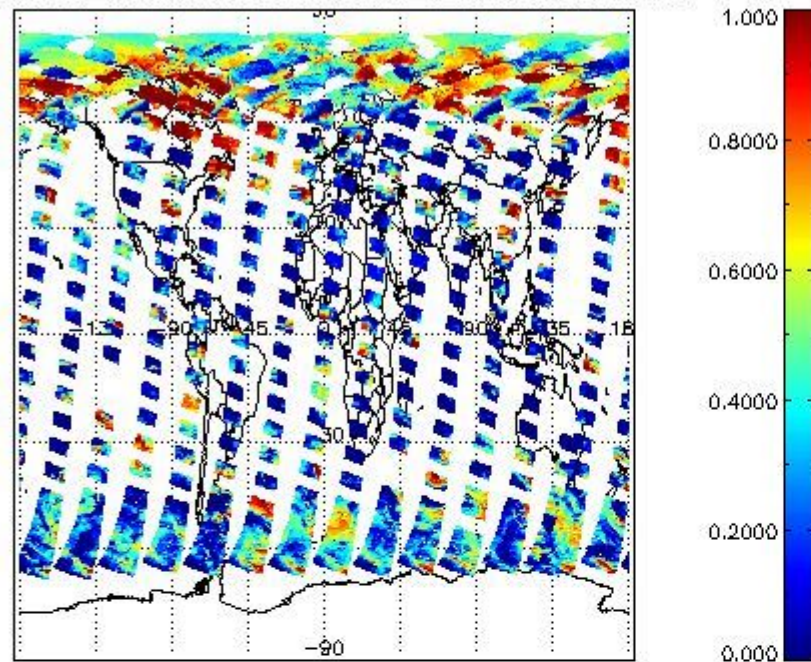
cL_frac for 10MAY2009 00:00:00 to 11MAY2009 00:00:00
