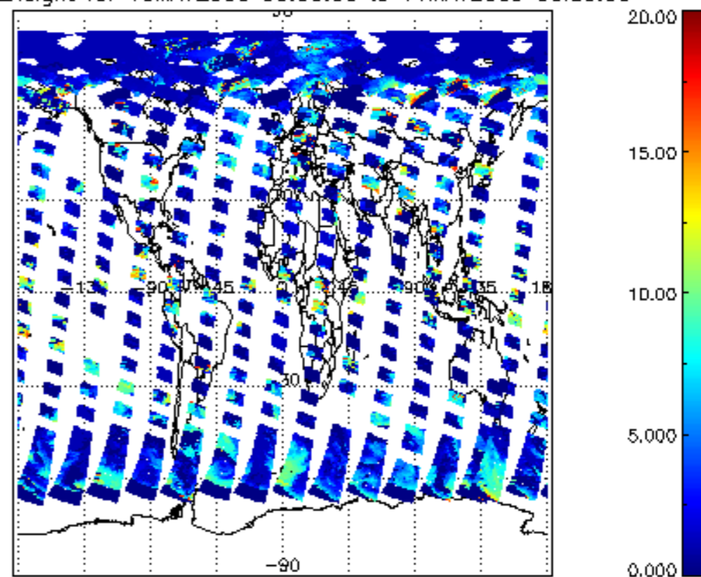
cl_top_height for 10MAY2009 00:00:00 to 11MAY2009 00:00:00
