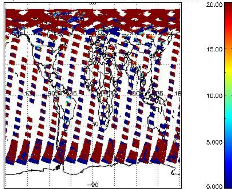
cL_opt_depth for 10MAY2009 00:00:00 to 11MAY2009 00:00:00
