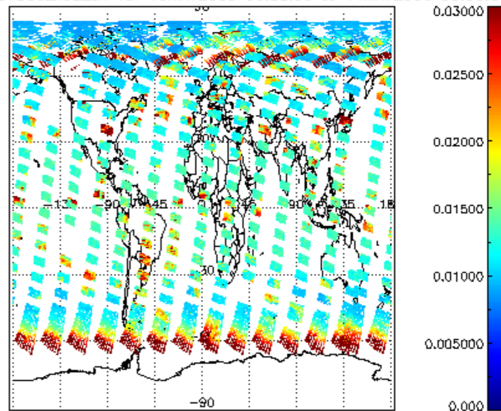
SCIOL2P_NADUV003_vcd_err for 10MAY2009 00:00:00 to 11MAY2009 00:00:00
