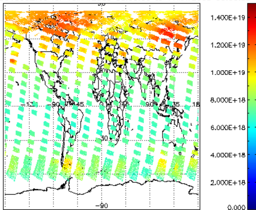
SCIOL2P_NADUV003_vcd for 10MAY2009 00:00:00 to 11MAY2009 00:00:00
