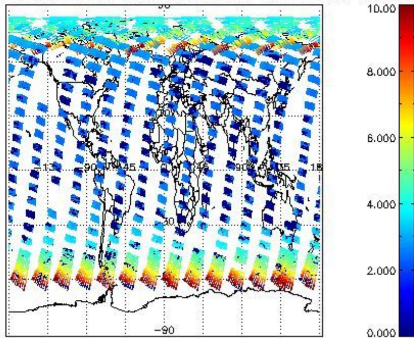
SCIOL2P_NADUV003_amf_cl for 10MAY2009 00:00:00 to 11MAY2009 00:00:00
