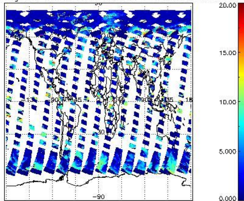
cL_top_height for 10MAY2009 00:00:00 to 11MAY2009 00:00:00
