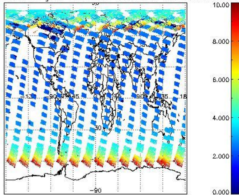
SCIOL2P_NADUV003_amf_gr for 10MAY2009 00:00:00 to 11MAY2009 00:00:00
