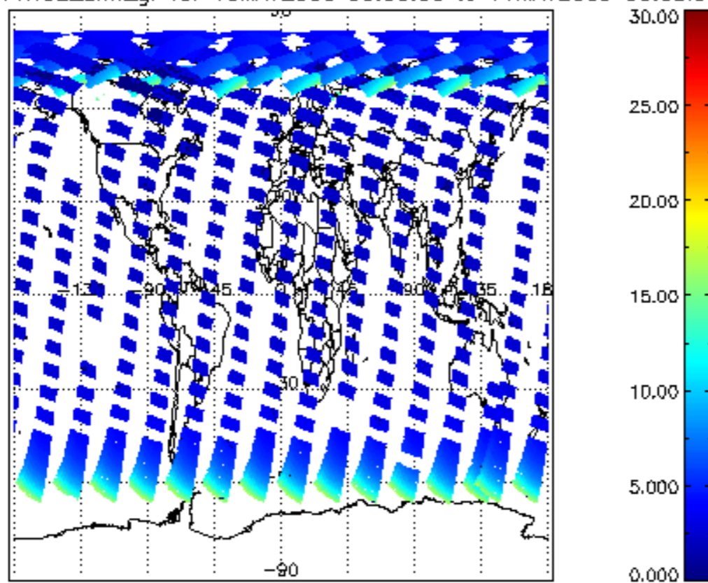
iCIOL2P_NADUV1NO2_amf_gr for 10MAY2009 00:00:00 to 11MAY2009 00:00:00
