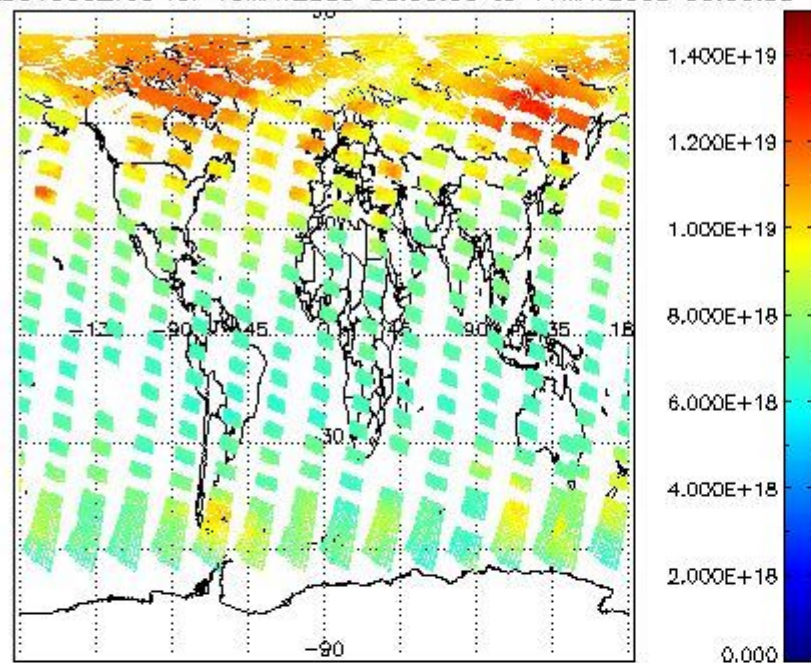
SCIOL2P_NADUV003_vcd for 10MAY2009 00:00:00 to 11MAY2009 00:00:00
