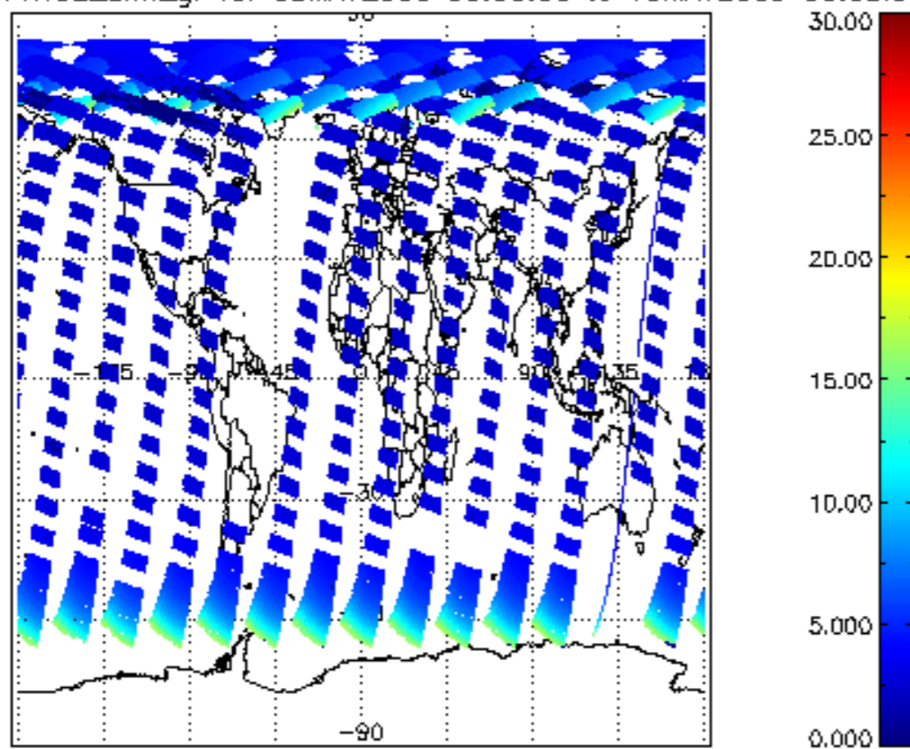
iCIOL2P_NADUV1NO2_amf_gr for 09MAY2009 00:00:00 to 10MAY2009 00:00:00
