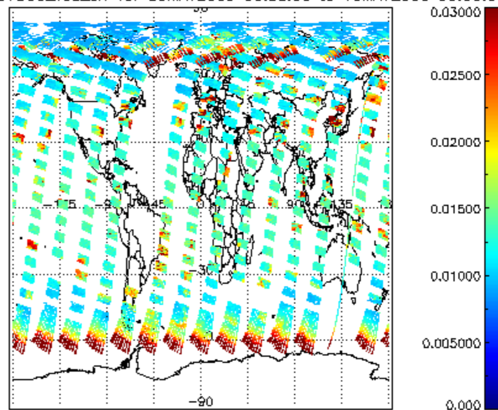
SCIOL2P_NADUV003_vcd_err for 09MAY2009 00:00:00 to 10MAY2009 00:00:00
