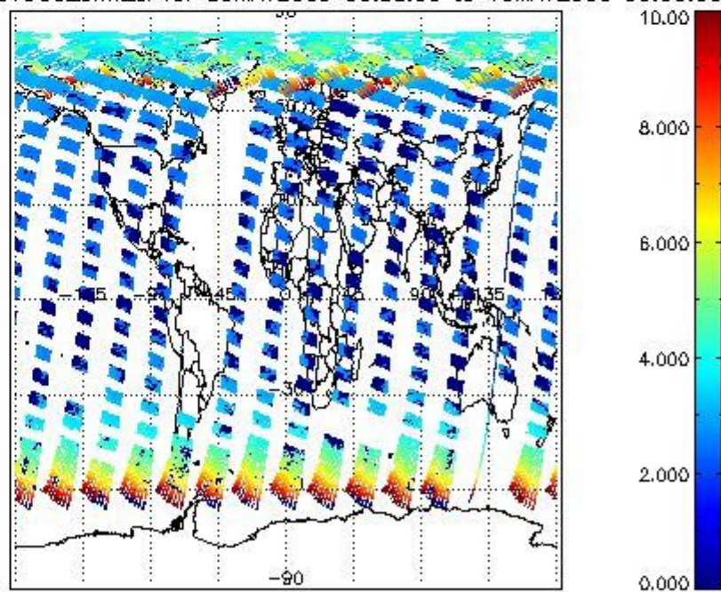
SCIOL2P_NADUV003_amf_cl for 09MAY2009 00:00:00 to 10MAY2009 00:00:00
