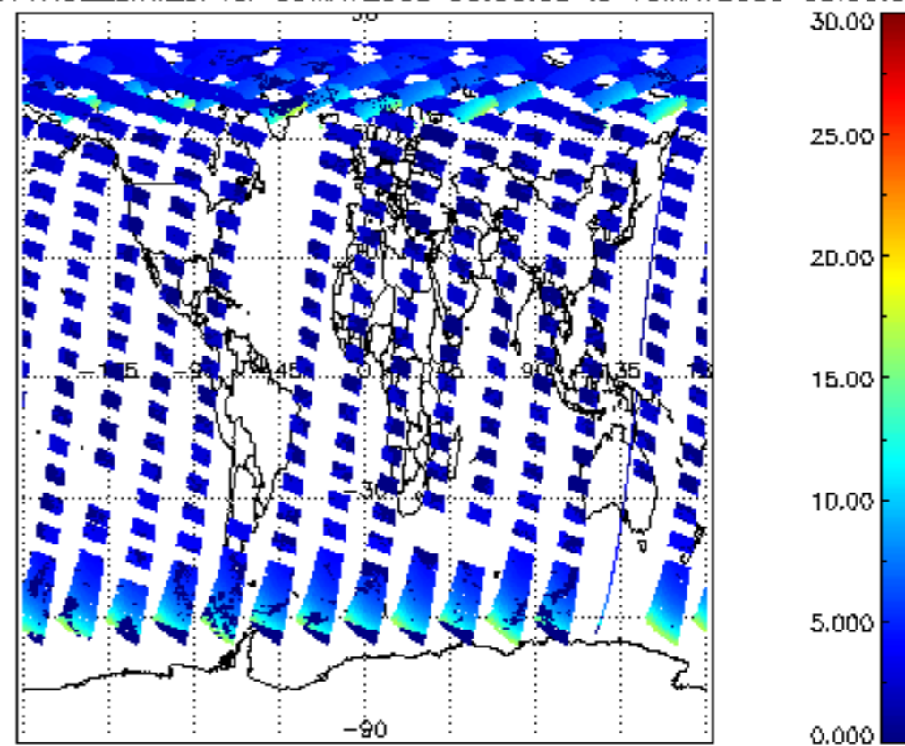
iCIOL2P_NADUV1NO2_amf_cl for 09MAY2009 00:00:00 to 10MAY2009 00:00:00
