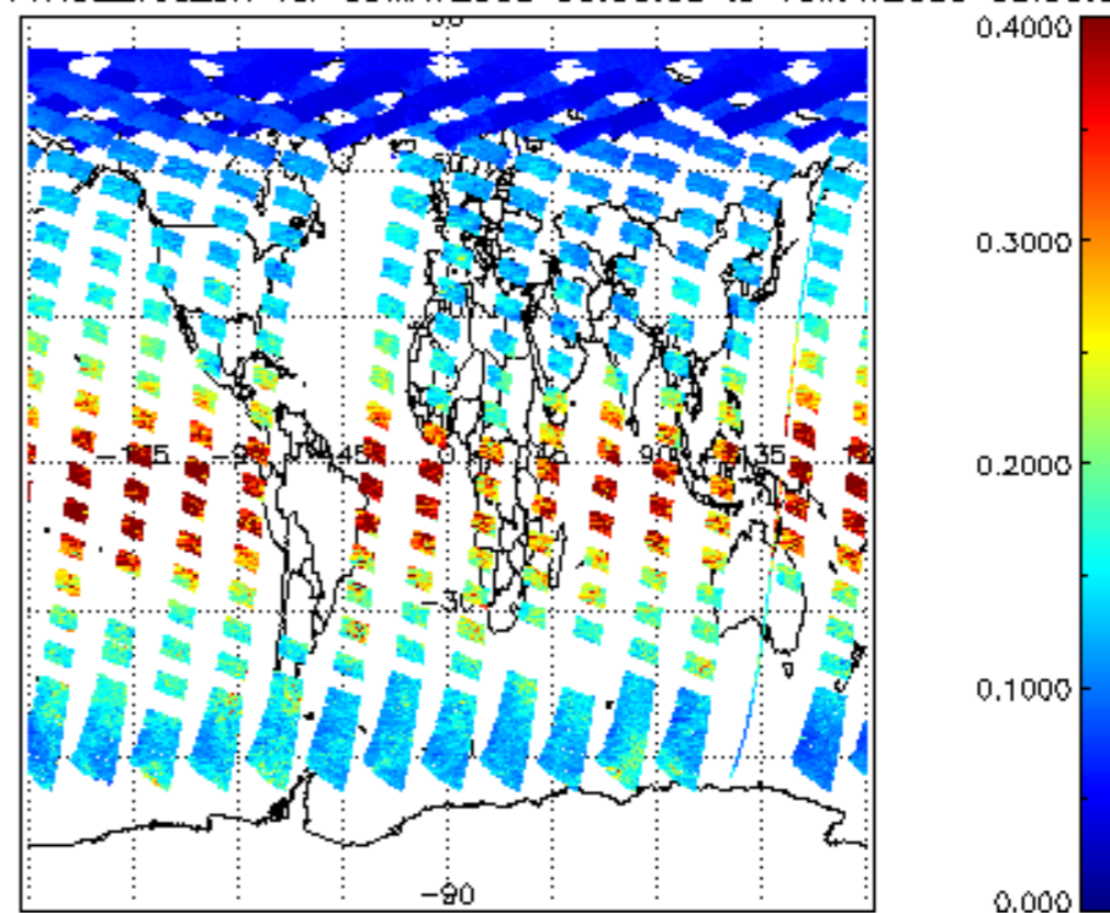
iCIOL2P_NADUV1NO2_vcd_err for 09MAY2009 00:00:00 to 10MAY2009 00:00:00
