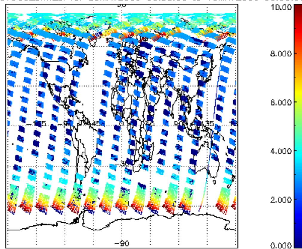
SCIOL2P_NADUV003_amf_cl for 09MAY2009 00:00:00 to 10MAY2009 00:00:00
