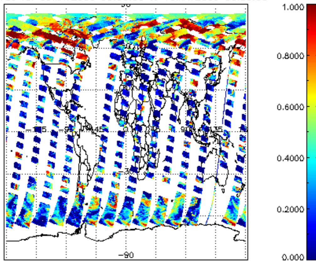
cL_frac for 09MAY2009 00:00:00 to 10MAY2009 00:00:00
