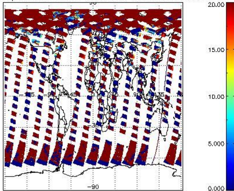
cL_opt_depth for 09MAY2009 00:00:00 to 10MAY2009 00:00:00
