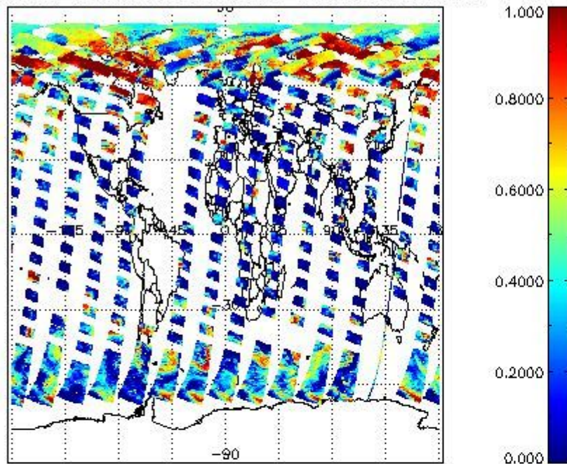
cL_frac for 09MAY2009 00:00:00 to 10MAY2009 00:00:00
