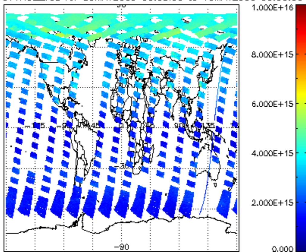
SCIOL2P_NADUV1NO2_vcd for 09MAY2009 00:00:00 to 10MAY2009 00:00:00
