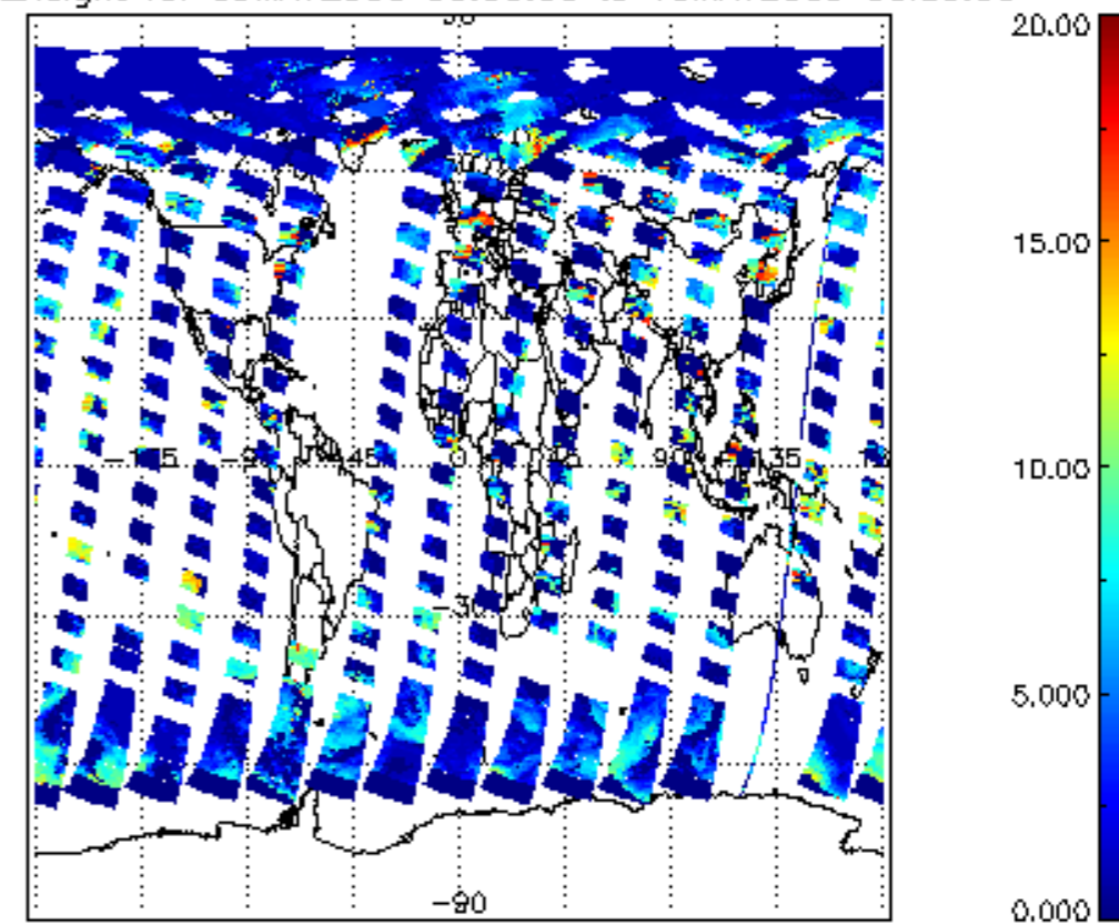
cL_top_height for 09MAY2009 00:00:00 to 10MAY2009 00:00:00
