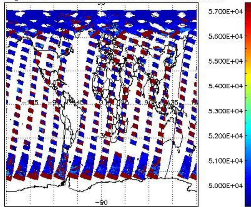
cloud_flags for 09MAY2009 00:00:00 to 10MAY2009 00:00:00
