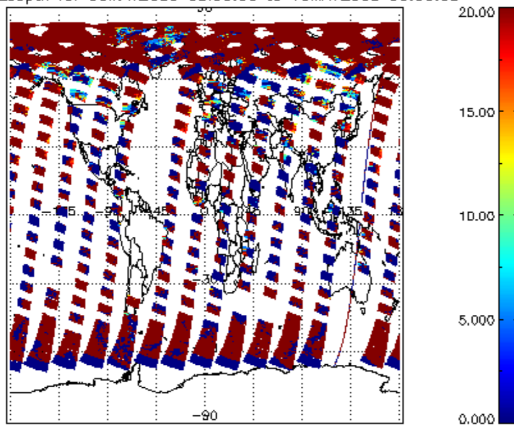
cL_opt_depth for 09MAY2009 00:00:00 to 10MAY2009 00:00:00
