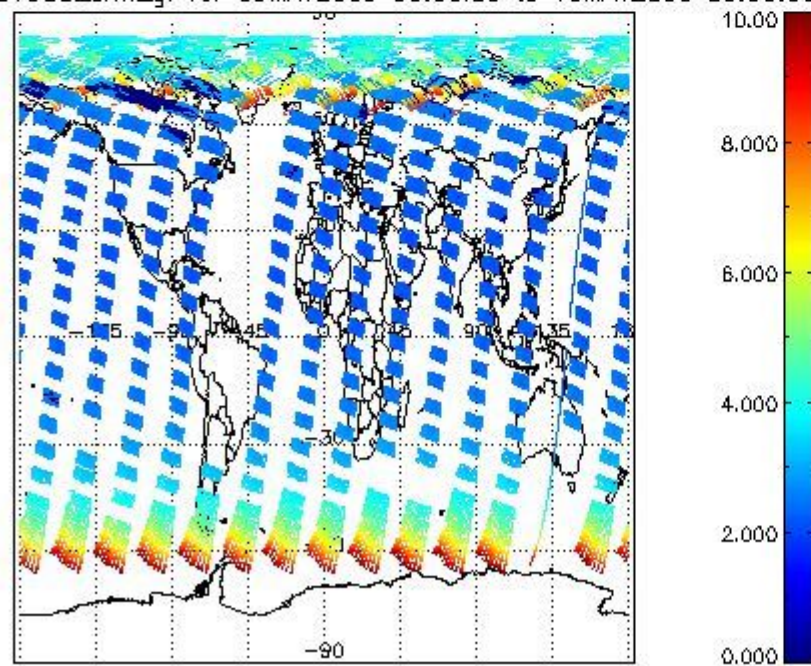
SCIOL2P_NADUV003_amf_gr for 09MAY2009 00:00:00 to 10MAY2009 00:00:00
