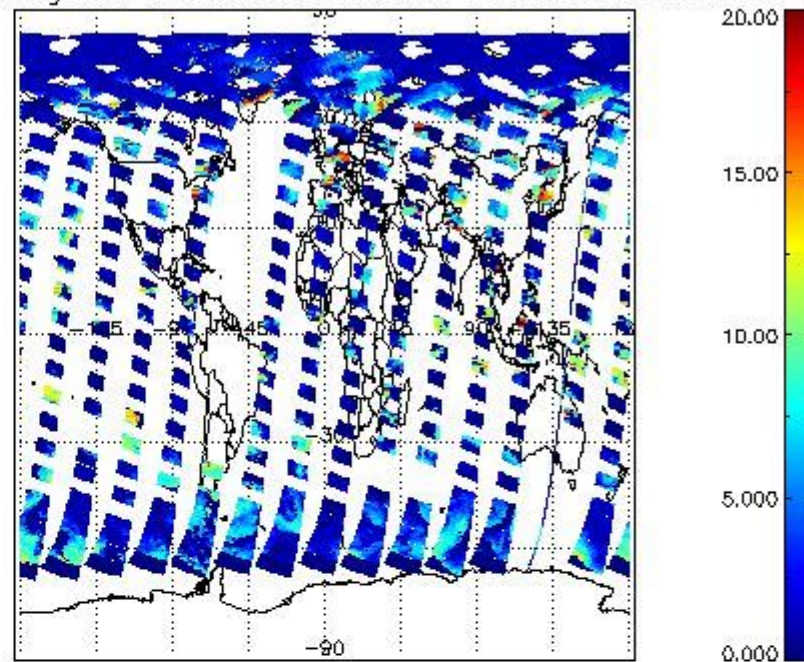
cL_top_height for 09MAY2009 00:00:00 to 10MAY2009 00:00:00
