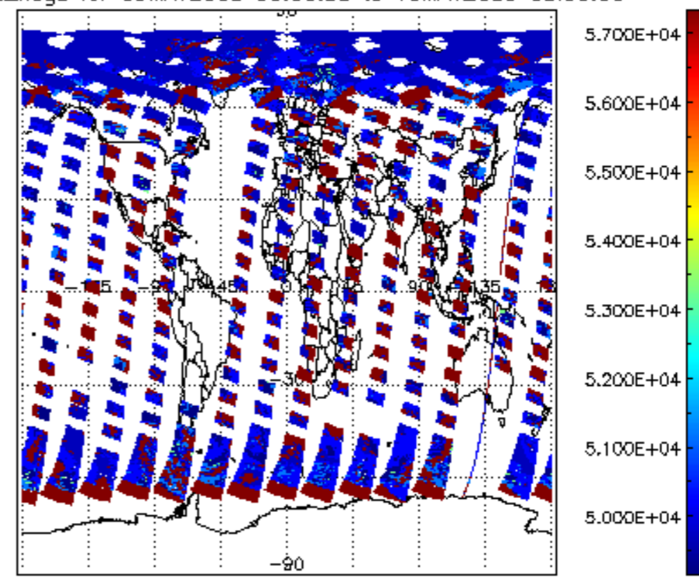
cloud_flags for 09MAY2009 00:00:00 to 10MAY2009 00:00:00
