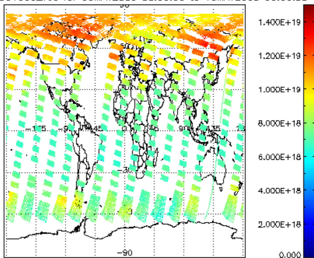
SCIOL2P_NADUV003_vcd for 09MAY2009 00:00:00 to 10MAY2009 00:00:00
