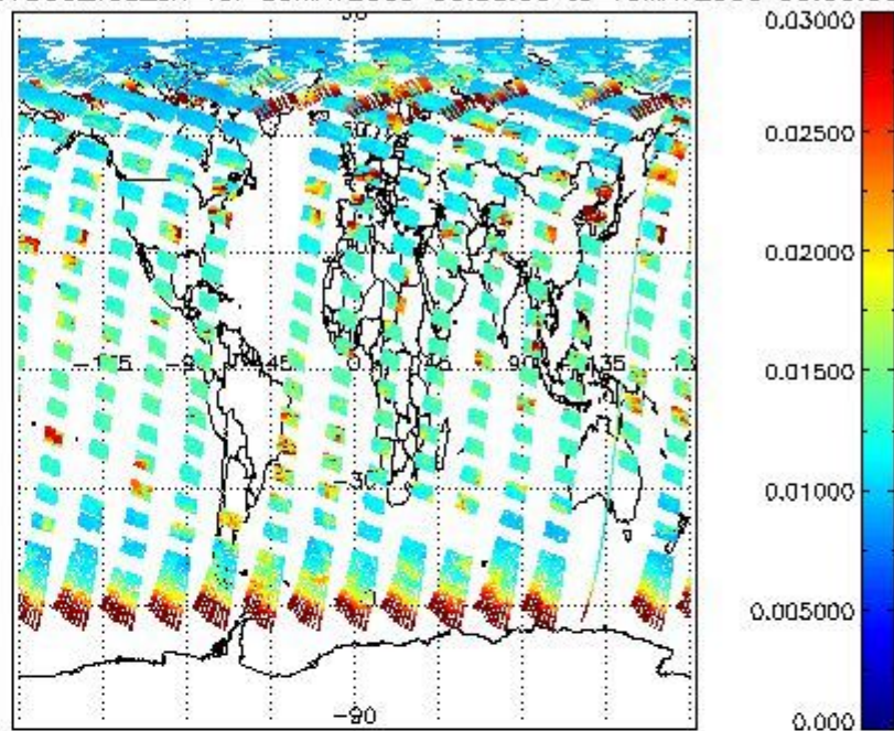
SCIOL2P_NADUV003_vcd_err for 09MAY2009 00:00:00 to 10MAY2009 00:00:00
