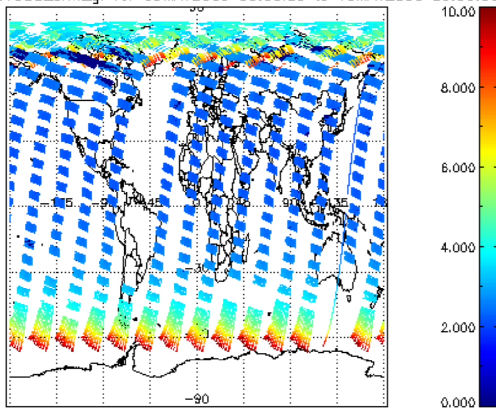
SCIOL2P_NADUV003_amf_gr for 09MAY2009 00:00:00 to 10MAY2009 00:00:00
