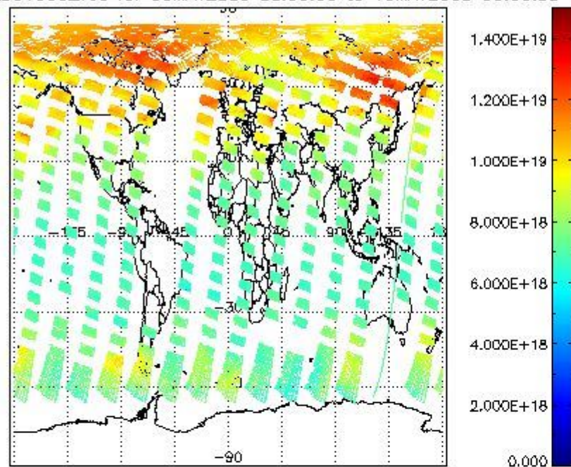
SCIOL2P_NADUV003_vcd for 09MAY2009 00:00:00 to 10MAY2009 00:00:00
