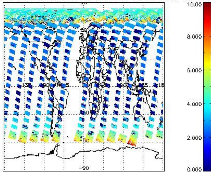
SCIOL2P_NADUV003_amf_cl for 04MAY2009 00:00:00 to 05MAY2009 00:00:00
