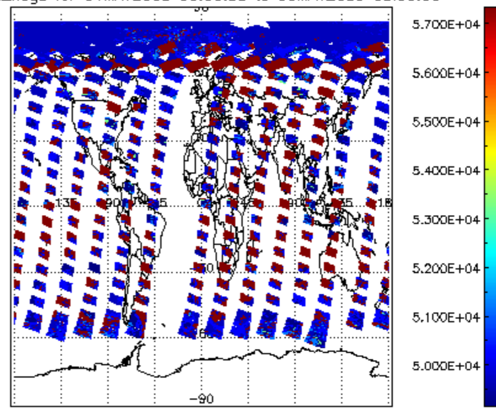
cloud_flags for 04MAY2009 00:00:00 to 05MAY2009 00:00:00
