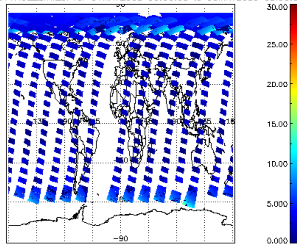
iCIOL2P_NADUV1NO2_amf_cl for 04MAY2009 00:00:00 to 05MAY2009 00:00:00
