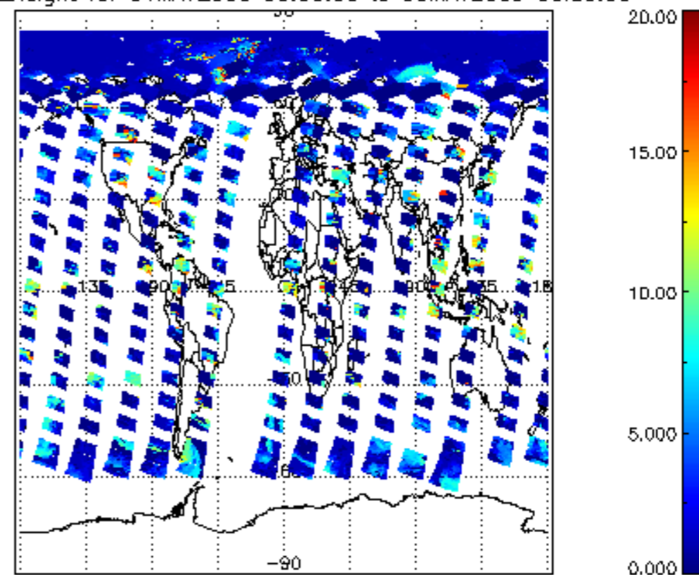
cl_top_height for 04MAY2009 00:00:00 to 05MAY2009 00:00:00
