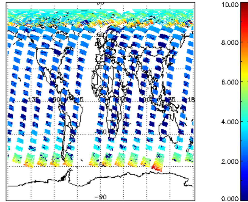
SCIOL2P_NADUV003_amf_cl for 04MAY2009 00:00:00 to 05MAY2009 00:00:00
