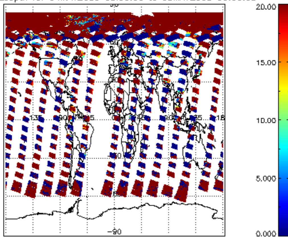
cl_opt_depth for 04MAY2009 00:00:00 to 05MAY2009 00:00:00
