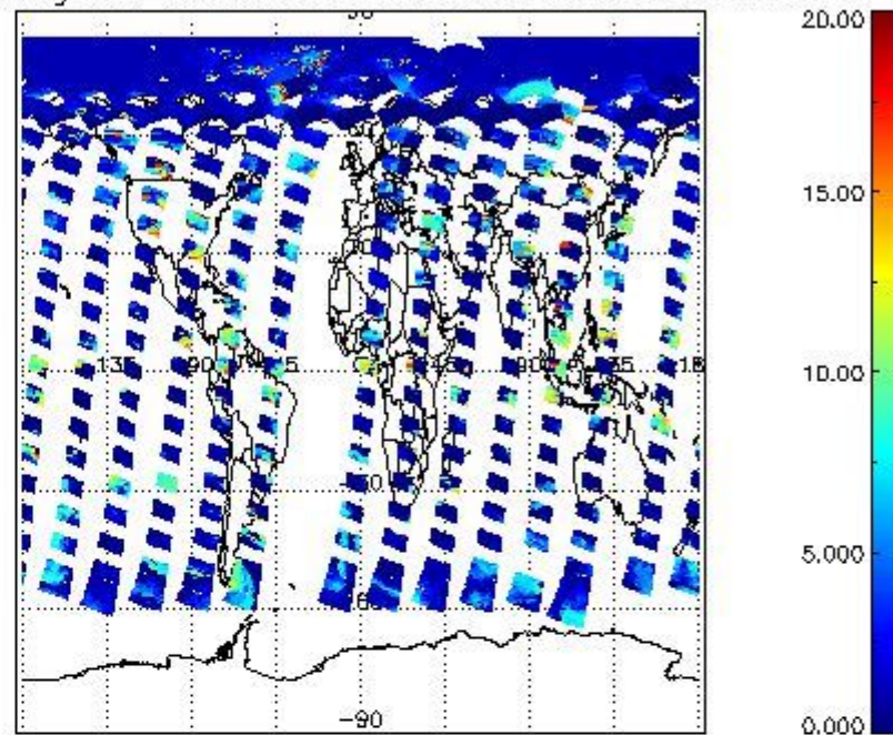
cL_top_height for 04MAY2009 00:00:00 to 05MAY2009 00:00:00
