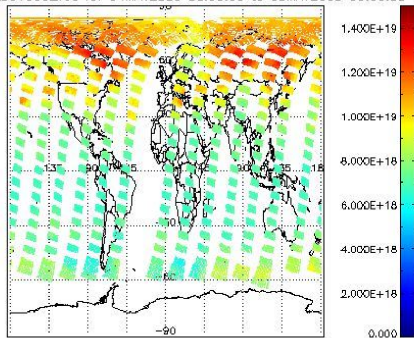
SCIOL2P_NADUV003_vcd for 04MAY2009 00:00:00 to 05MAY2009 00:00:00
