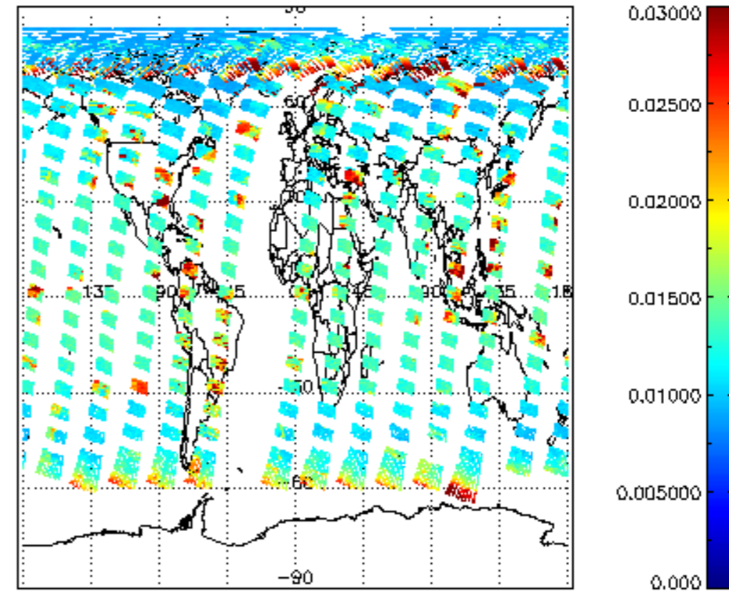
SCIOL2P_NADUV003_vcd_err for 04MAY2009 00:00:00 to 05MAY2009 00:00:00
