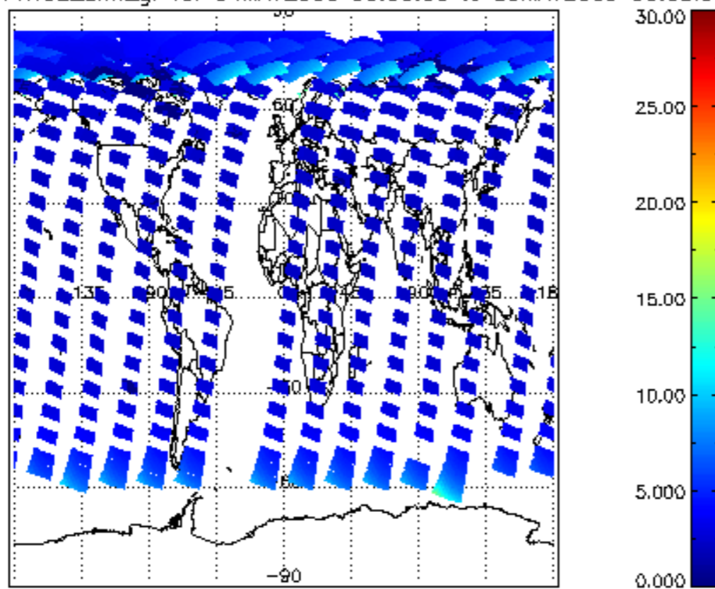
iCIOL2P_NADUV1NO2_amf_gr for 04MAY2009 00:00:00 to 05MAY2009 00:00:00
