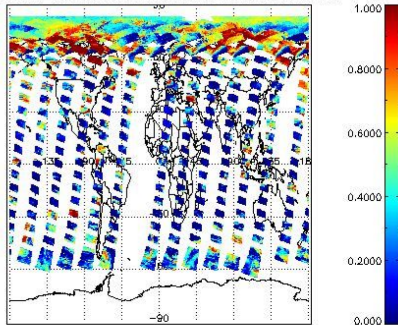
cL_frac for 04MAY2009 00:00:00 to 05MAY2009 00:00:00
