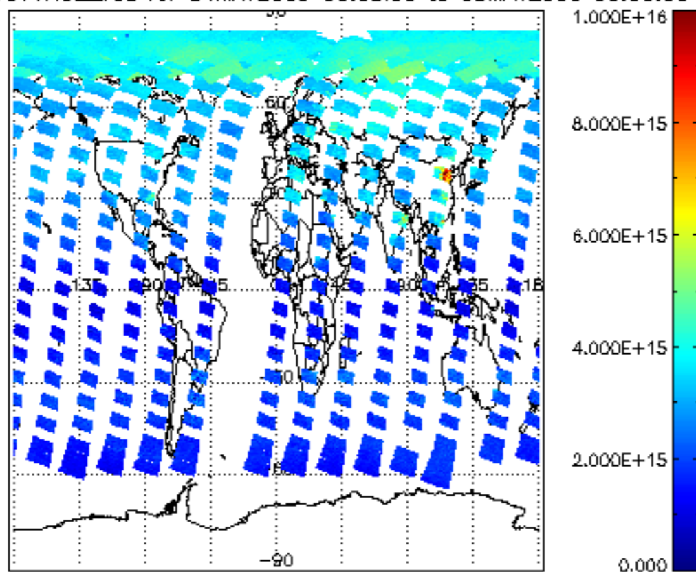
SCIOL2P_NADUV1NO2_vcd for 04MAY2009 00:00:00 to 05MAY2009 00:00:00
