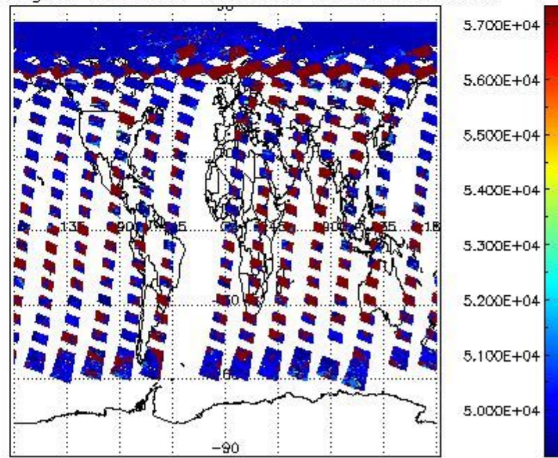
cloud_flags for 04MAY2009 00:00:00 to 05MAY2009 00:00:00
