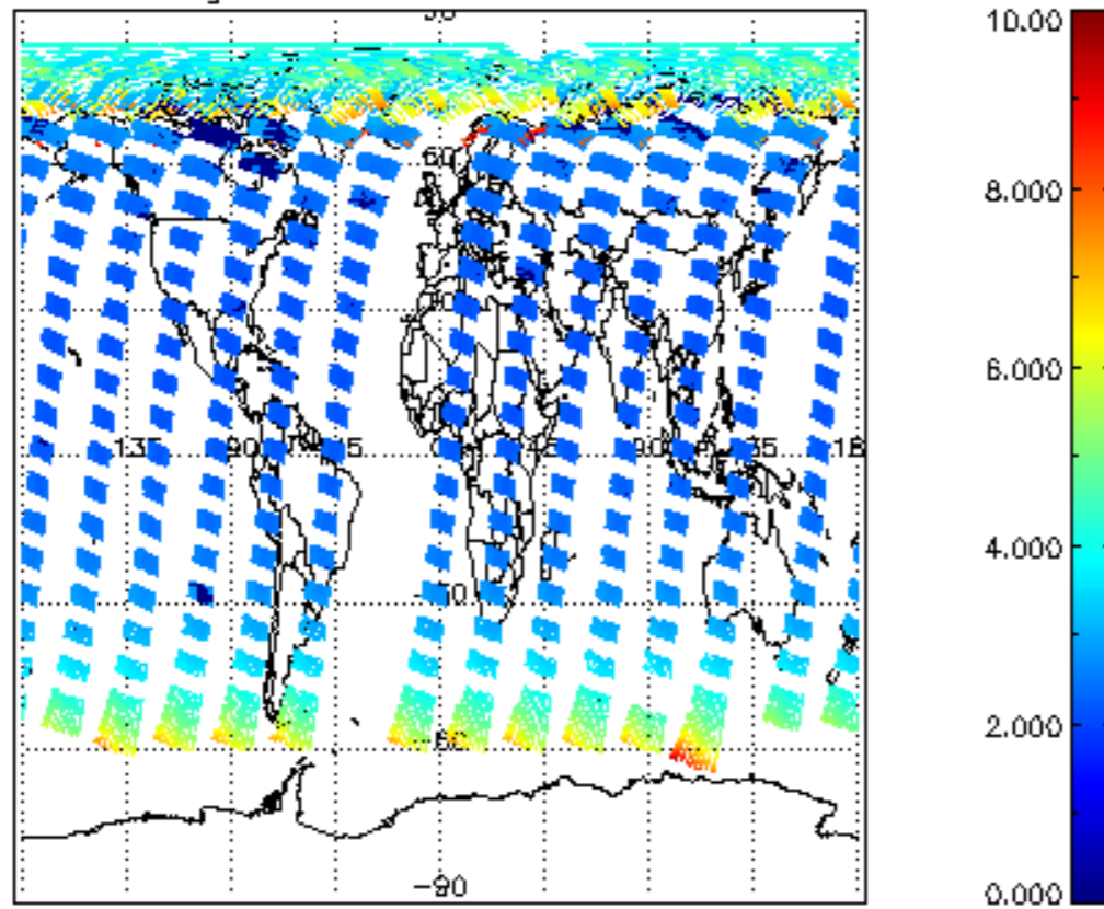
SCIOL2P_NADUV003_amf_gr for 04MAY2009 00:00:00 to 05MAY2009 00:00:00
