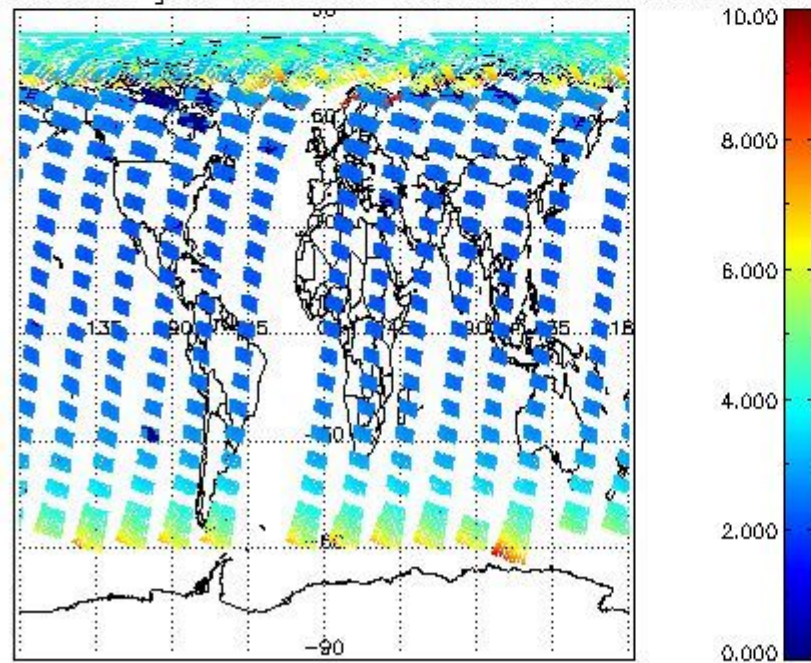
SCIOL2P_NADUV003_amf_gr for 04MAY2009 00:00:00 to 05MAY2009 00:00:00
