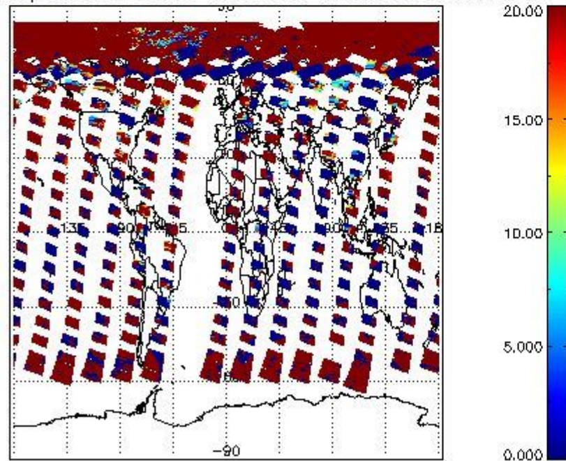
cL_opt_depth for 04MAY2009 00:00:00 to 05MAY2009 00:00:00
