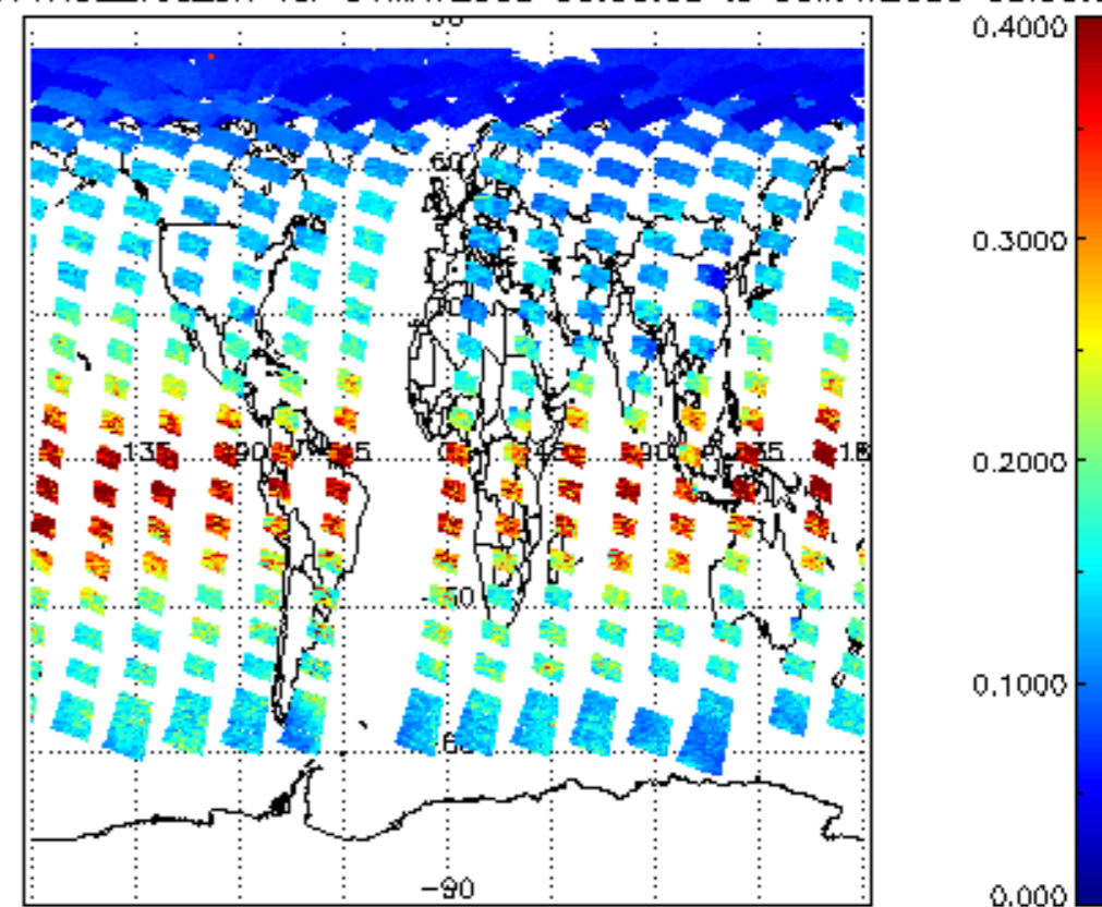
iCIOL2P_NADUV1NO2_vcd_err for 04MAY2009 00:00:00 to 05MAY2009 00:00:00
