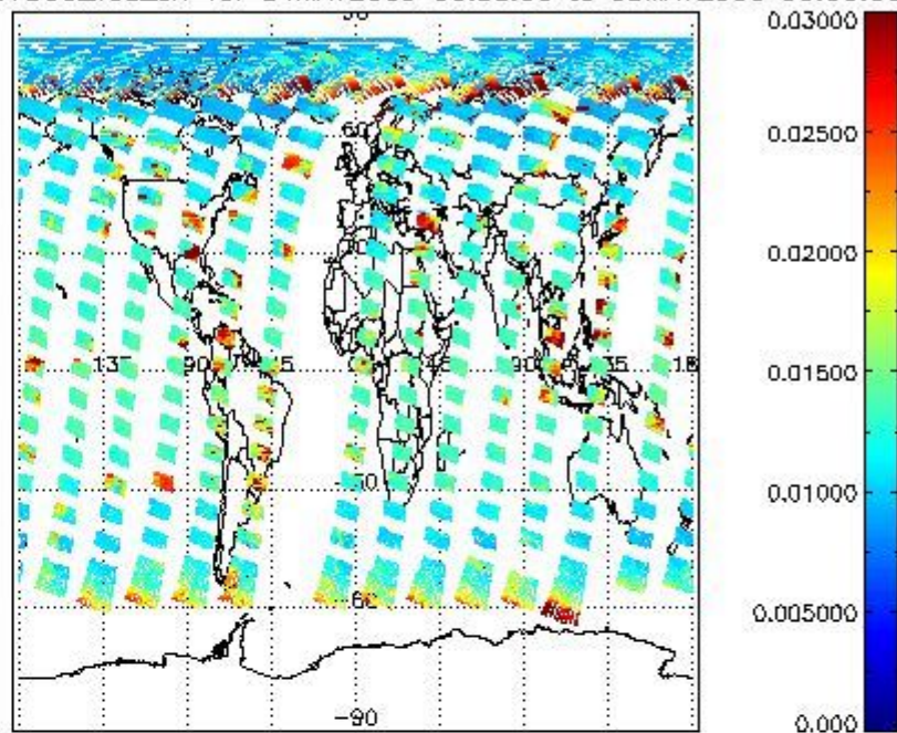
SCIOL2P_NADUV003_vcd_err for 04MAY2009 00:00:00 to 05MAY2009 00:00:00
