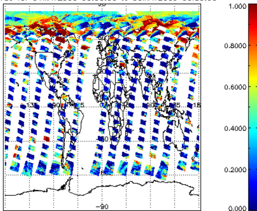
cl_frac for 04MAY2009 00:00:00 to 05MAY2009 00:00:00
