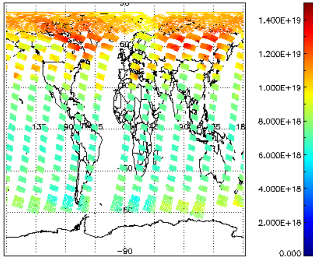
SCIOL2P_NADUV003_vcd for 04MAY2009 00:00:00 to 05MAY2009 00:00:00
