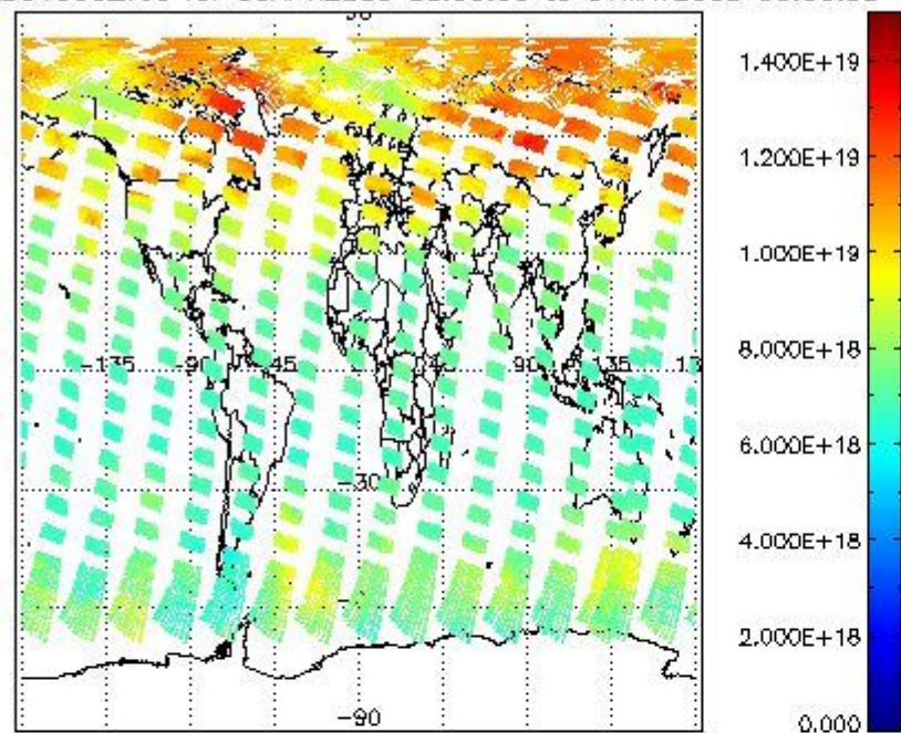
SCIOL2P_NADUV003_vcd for 30APR2009 00:00:00 to 01MAY2009 00:00:00
