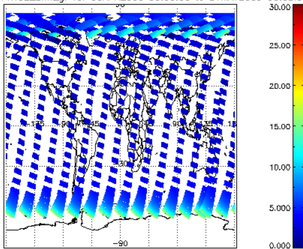
iCIOL2P_NADUV1NO2_amf_gr for 30APR2009 00:00:00 to 01MAY2009 00:00:00
