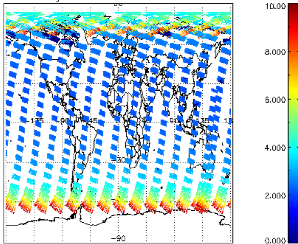
SCIOL2P_NADUV003_amf_gr for 30APR2009 00:00:00 to 01MAY2009 00:00:00
