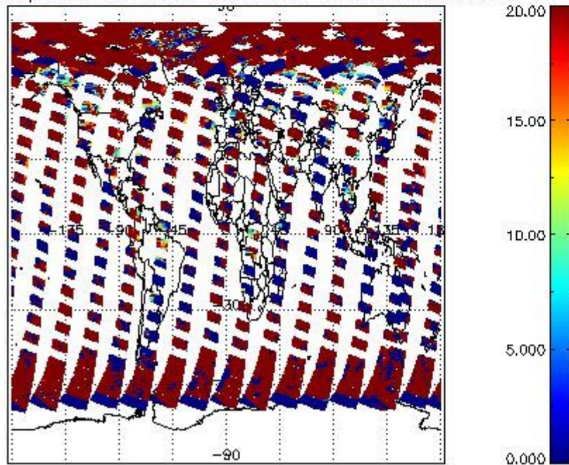
cL_opt_depth for 30APR2009 00:00:00 to 01MAY2009 00:00:00
