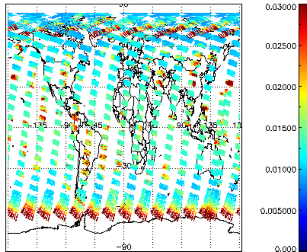
SCIOL2P_NADUV003_vcd_err for 30APR2009 00:00:00 to 01MAY2009 00:00:00
