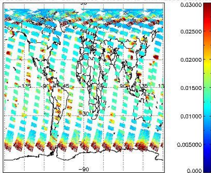
SCIOL2P_NADUV003_vcd_err for 30APR2009 00:00:00 to 01MAY2009 00:00:00
