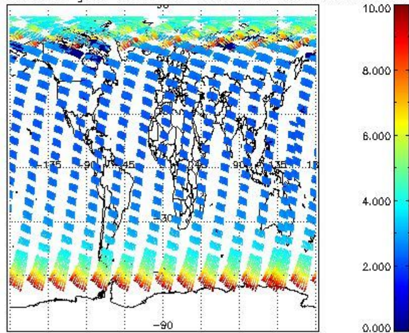
SCIOL2P_NADUV003_amf_gr for 30APR2009 00:00:00 to 01MAY2009 00:00:00
