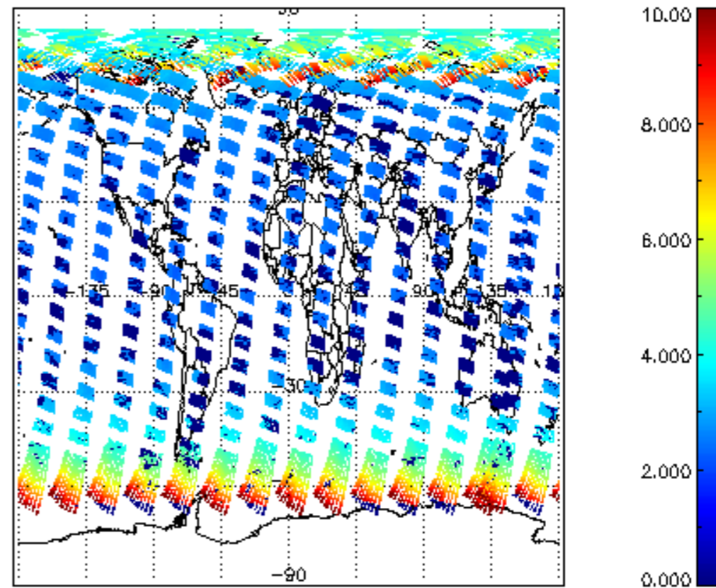
SCIOL2P_NADUV003_amf_cl for 30APR2009 00:00:00 to 01MAY2009 00:00:00
