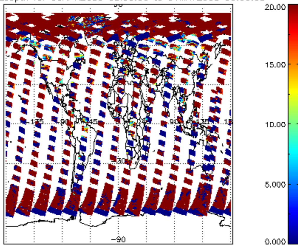
cl_opt_depth for 30APR2009 00:00:00 to 01MAY2009 00:00:00
