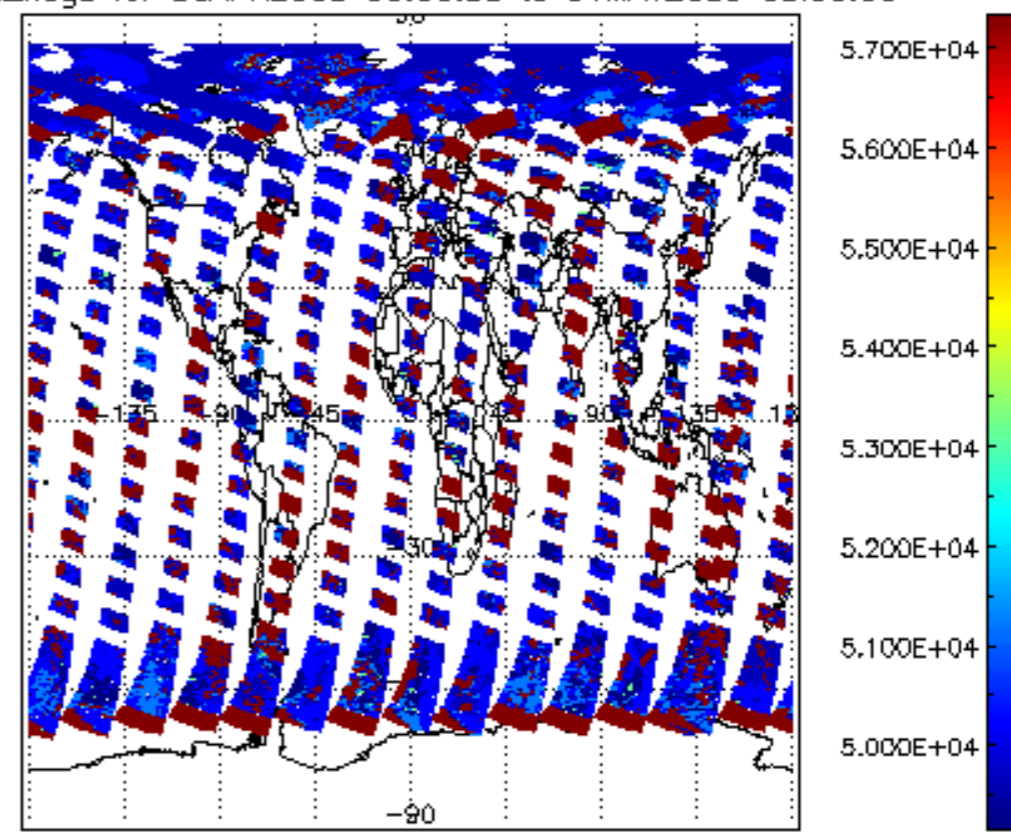
cloud_flags for 30APR2009 00:00:00 to 01MAY2009 00:00:00
