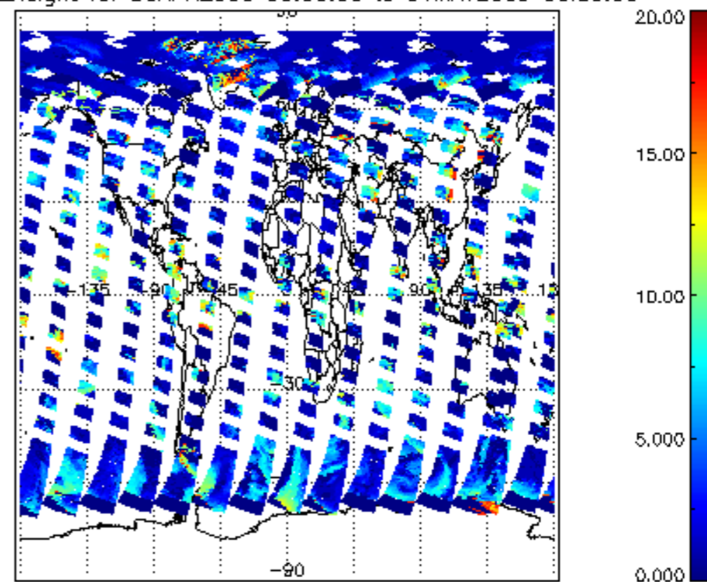
cl_top_height for 30APR2009 00:00:00 to 01MAY2009 00:00:00
