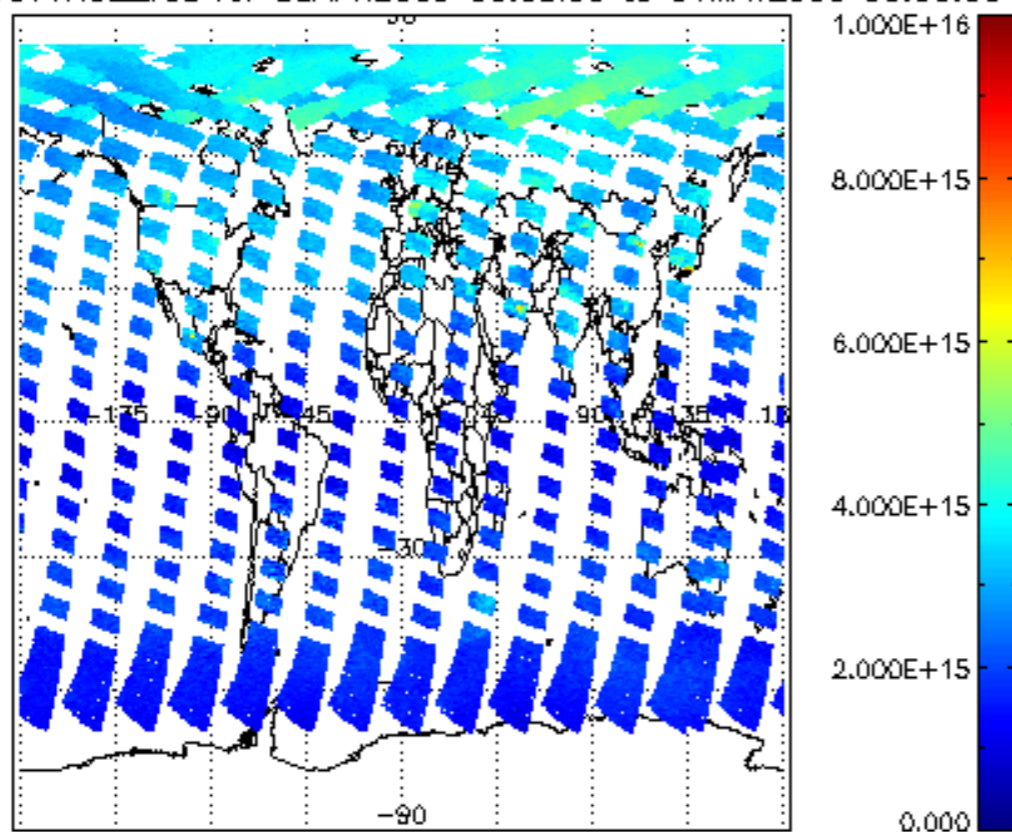
SCIOL2P_NADUV1NO2_vcd for 30APR2009 00:00:00 to 01MAY2009 00:00:00
