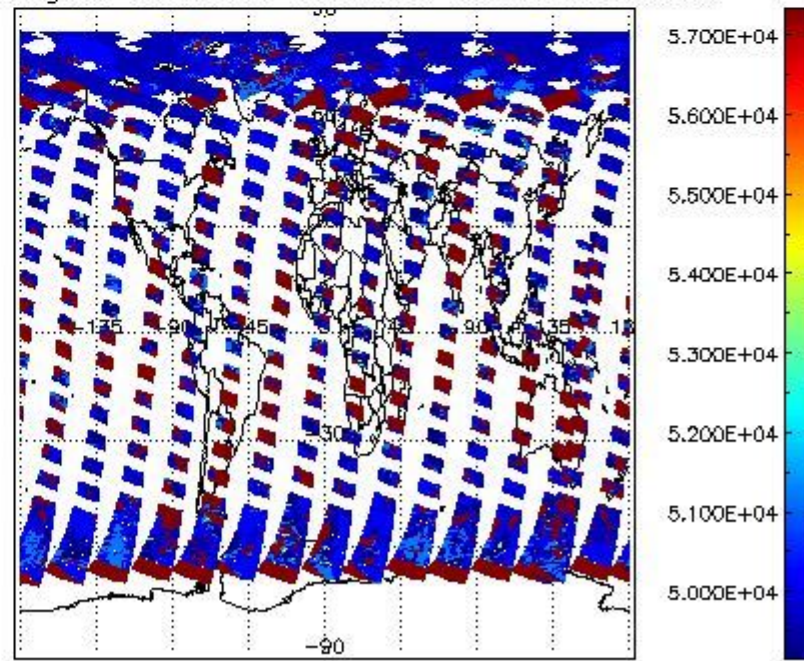
cloud_flags for 30APR2009 00:00:00 to 01MAY2009 00:00:00
