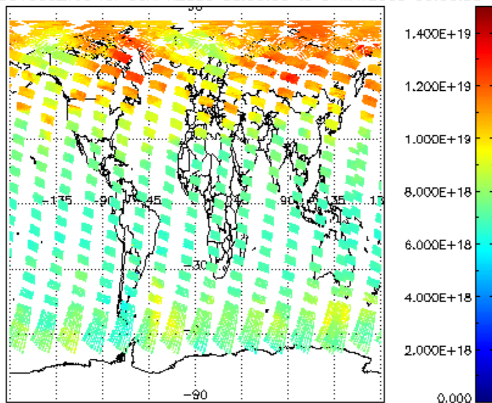
SCIOL2P_NADUV003_vcd for 30APR2009 00:00:00 to 01MAY2009 00:00:00
