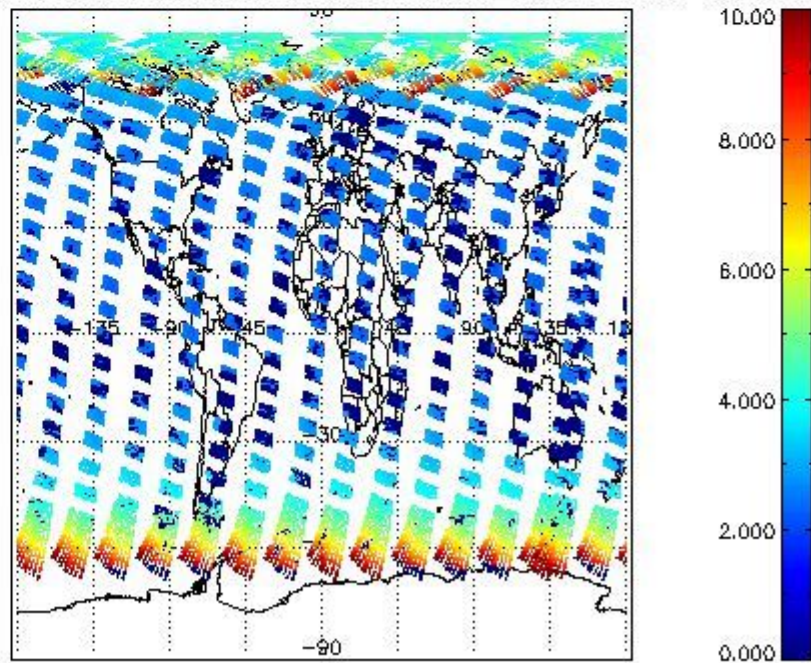
SCIOL2P_NADUV003_amf_sl for 30APR2009 00:00:00 to 01MAY2009 00:00:00
