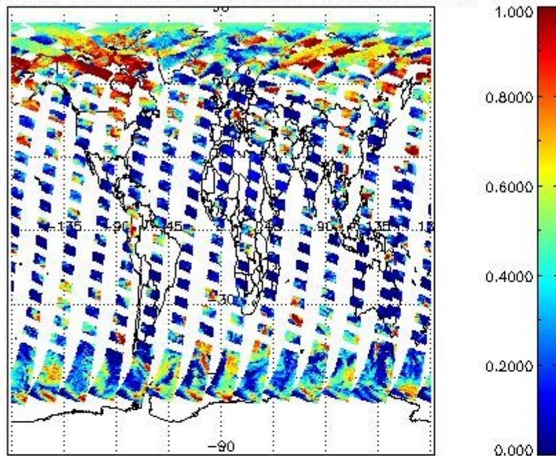
cL_frac for 30APR2009 00:00:00 to 01MAY2009 00:00:00
