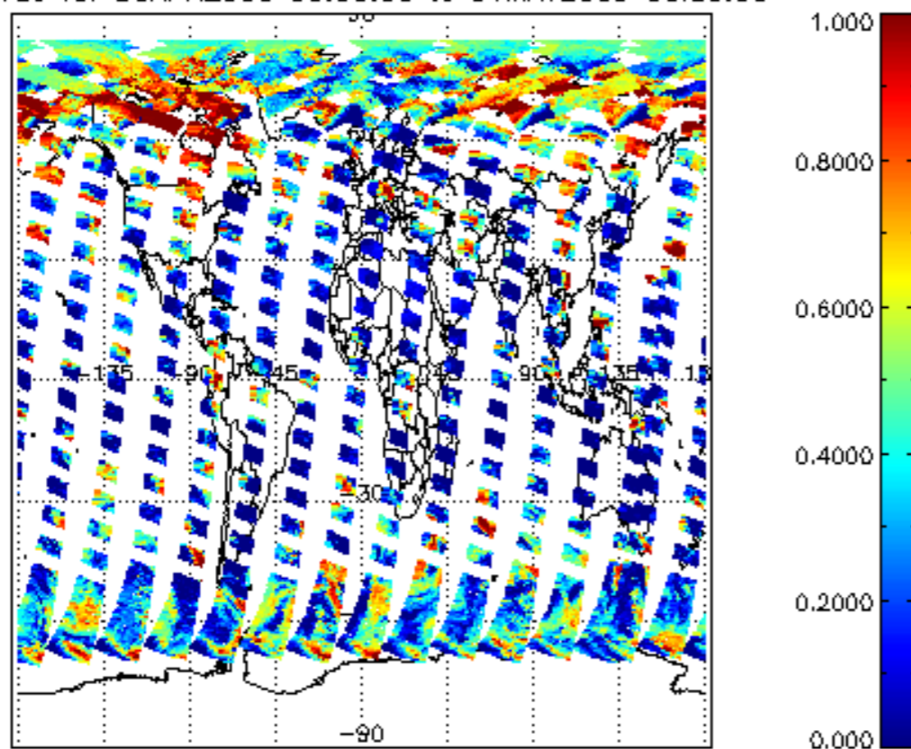
cl_frac for 30APR2009 00:00:00 to 01MAY2009 00:00:00
