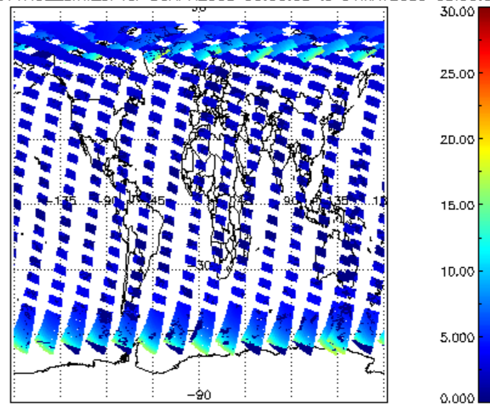
iCIOL2P_NADUV1NO2_amf_cl for 30APR2009 00:00:00 to 01MAY2009 00:00:00
