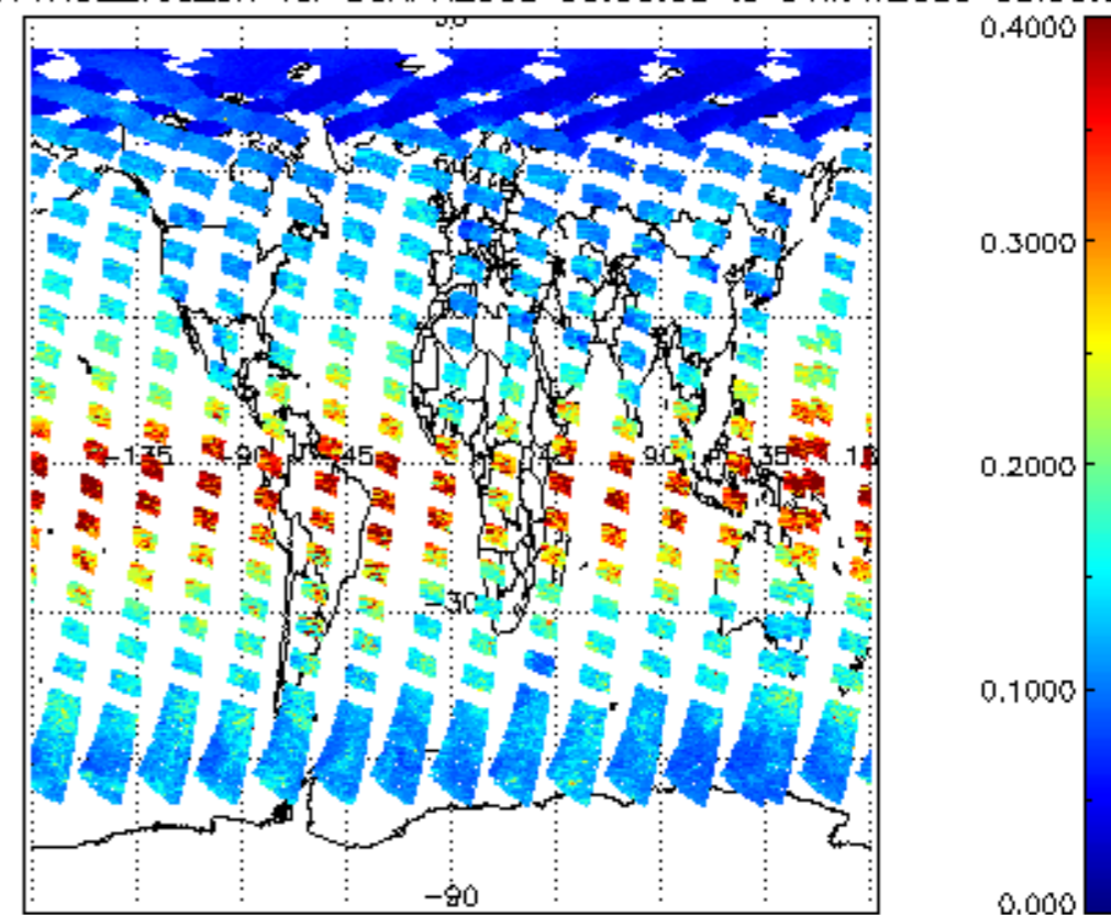
iCIOL2P_NADUV1NO2_vcd_err for 30APR2009 00:00:00 to 01MAY2009 00:00:00
