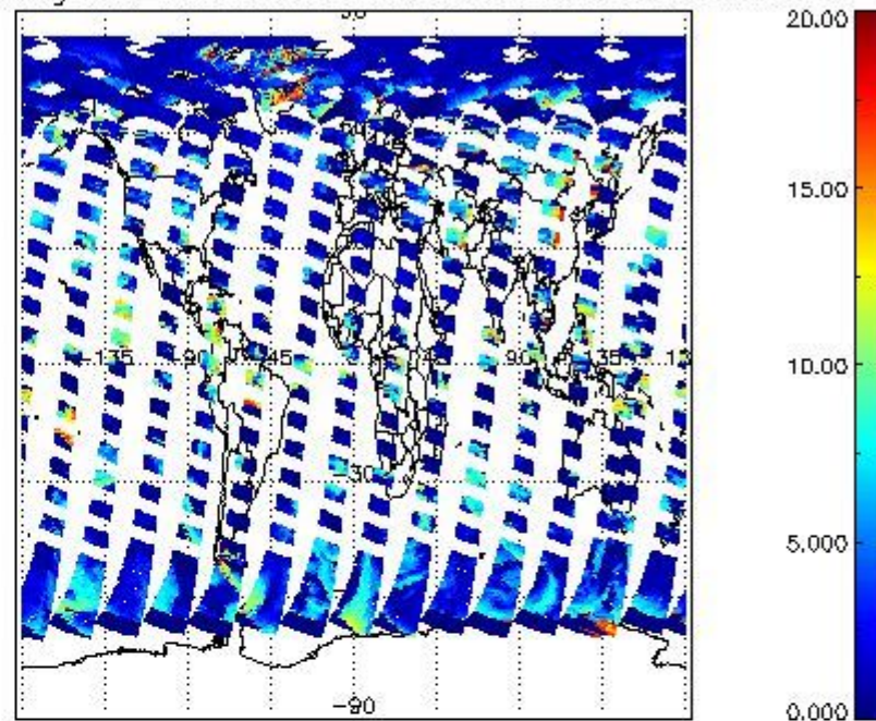
cL_top_height for 30APR2009 00:00:00 to 01MAY2009 00:00:00
