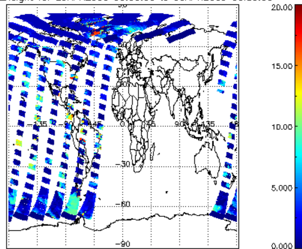
cl_top_height for 29APR2009 00:00:00 to 30APR2009 00:00:00
