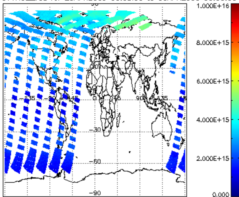
SCIOL2P_NADUV1NO2_vcd for 29APR2009 00:00:00 to 30APR2009 00:00:00
