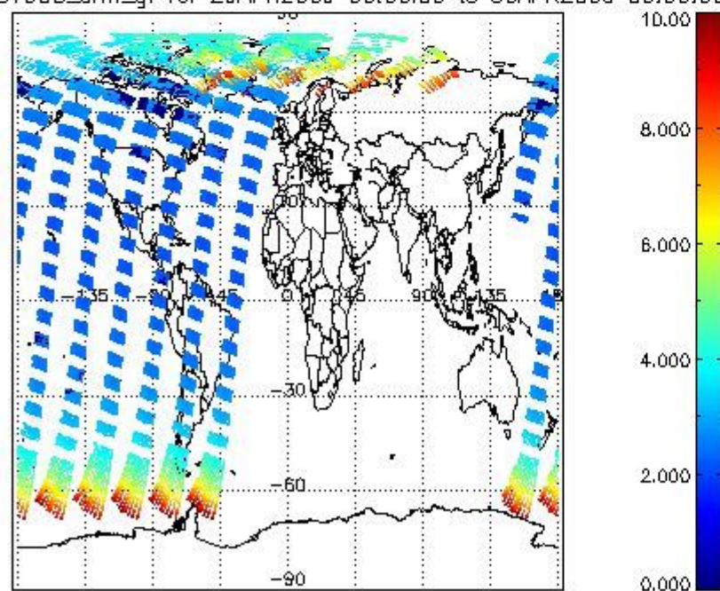
SCIOL2P_NADUV003_amf_gr for 29APR2009 00:00:00 to 30APR2009 00:00:00
