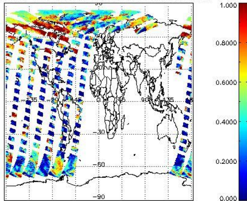
cL_frac for 29APR2009 00:00:00 to 30APR2009 00:00:00
