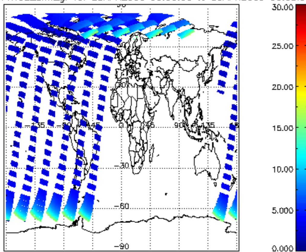
iCIOL2P_NADUV1NO2_amf_gr for 29APR2009 00:00:00 to 30APR2009 00:00:00
