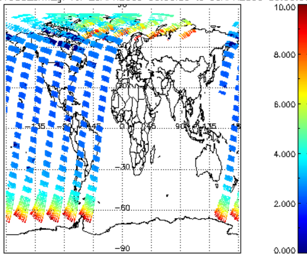
SCIOL2P_NADUV003_amf_gr for 29APR2009 00:00:00 to 30APR2009 00:00:00
