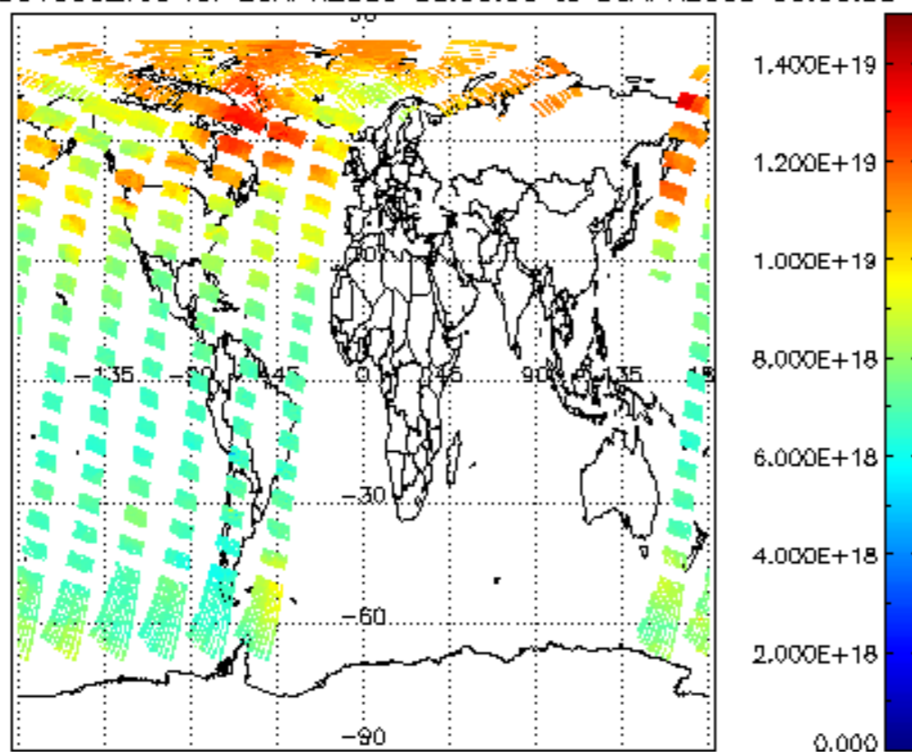
SCIOL2P_NADUV003_vcd for 29APR2009 00:00:00 to 30APR2009 00:00:00
