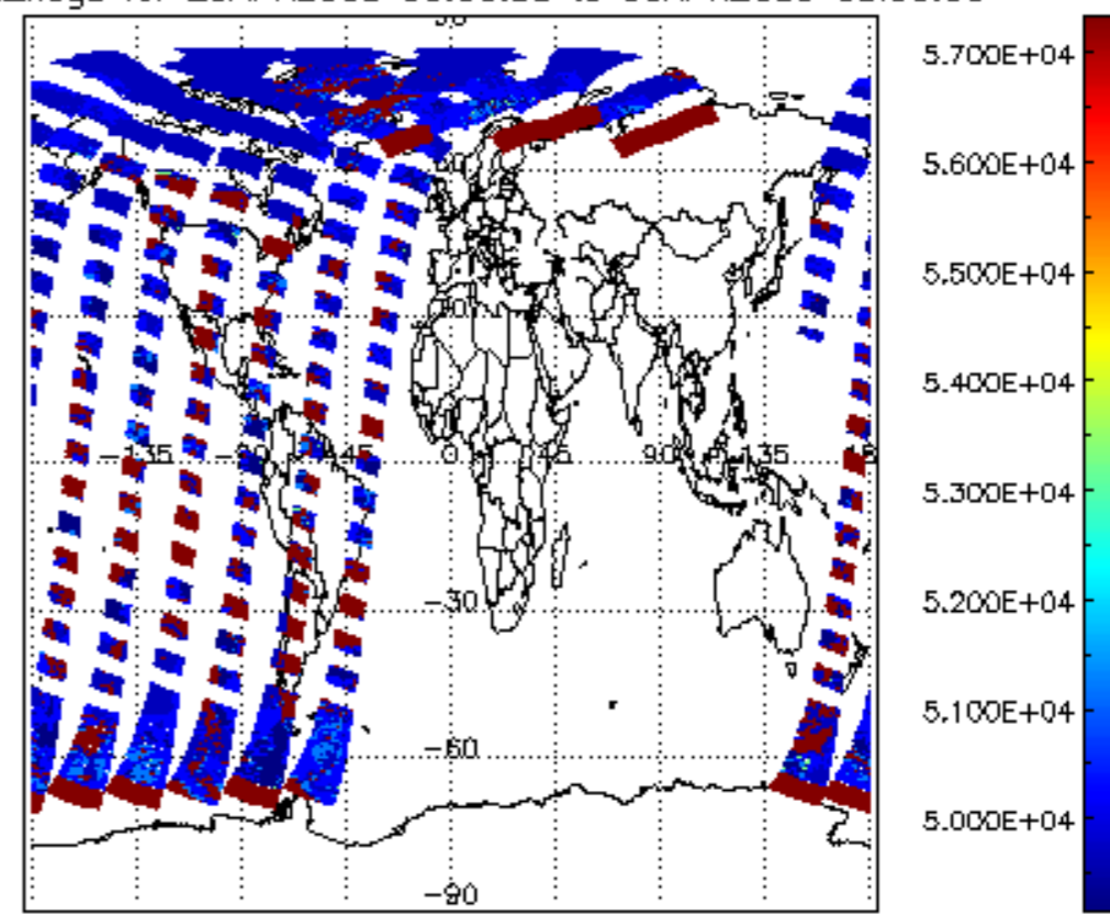
cloud_flags for 29APR2009 00:00:00 to 30APR2009 00:00:00
