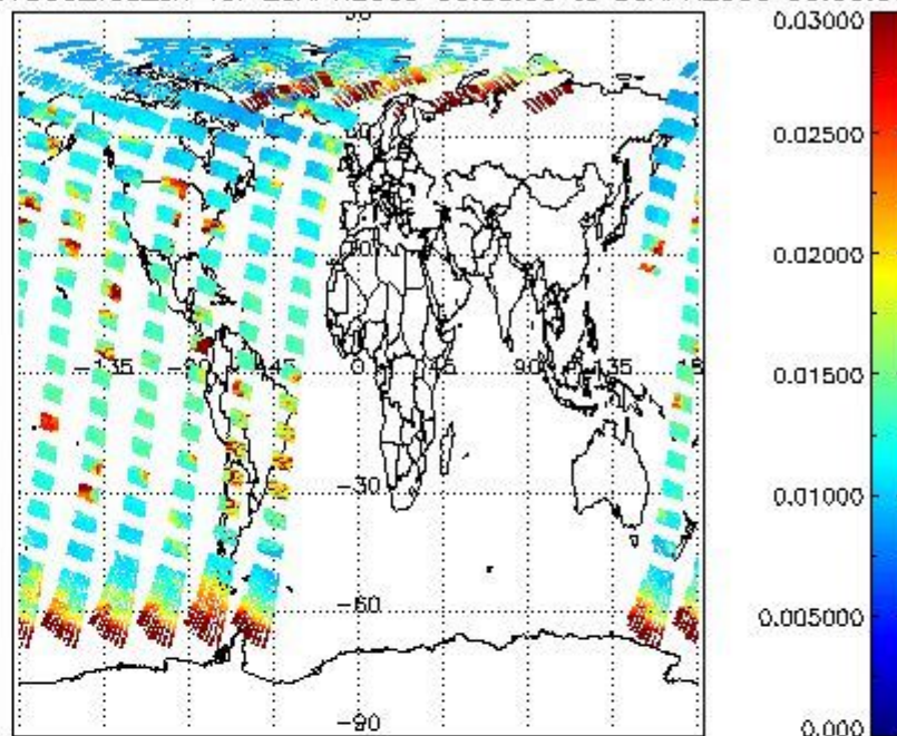
SCIOL2P_NADUV003_vcd_err for 29APR2009 00:00:00 to 30APR2009 00:00:00
