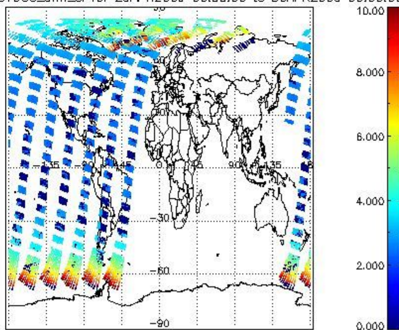
SCIOL2P_NADUV003_amf_cl for 29APR2009 00:00:00 to 30APR2009 00:00:00
