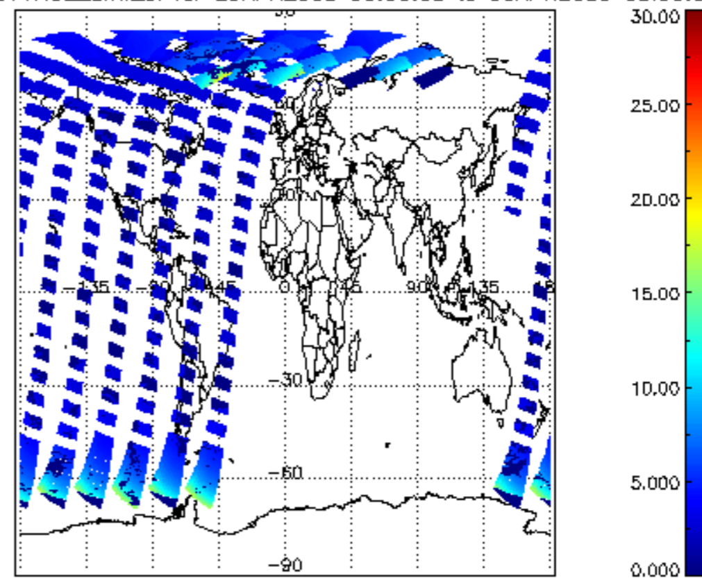
iCIOL2P_NADUV1NO2_amf_cl for 29APR2009 00:00:00 to 30APR2009 00:00:00
