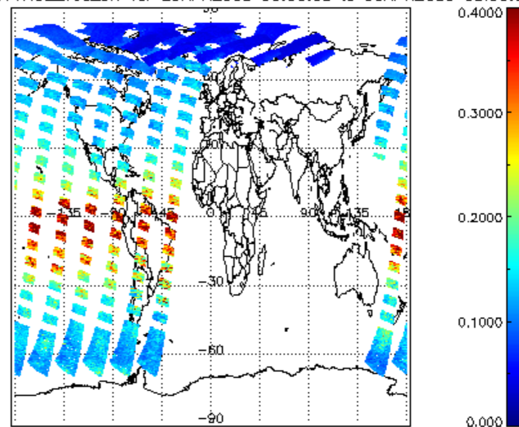
iCIOL2P_NADUV1NO2_vcd_err for 29APR2009 00:00:00 to 30APR2009 00:00:00
