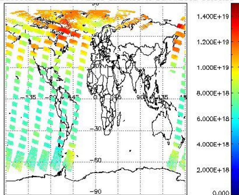
SCIOL2P_NADUV003_vcd for 29APR2009 00:00:00 to 30APR2009 00:00:00
