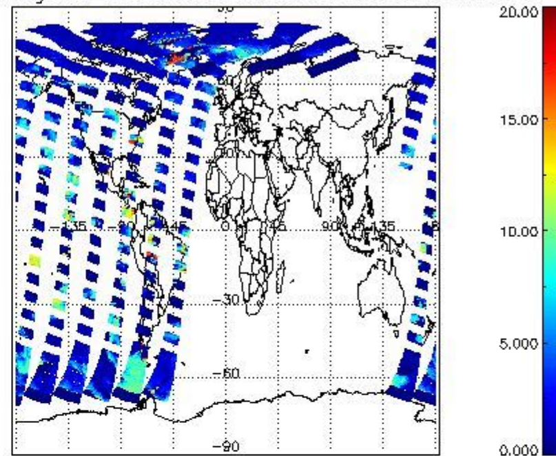
cL_top_height for 29APR2009 00:00:00 to 30APR2009 00:00:00
