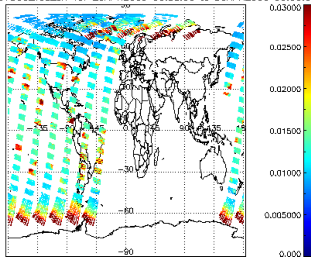
SCIOL2P_NADUV003_vcd_err for 29APR2009 00:00:00 to 30APR2009 00:00:00
