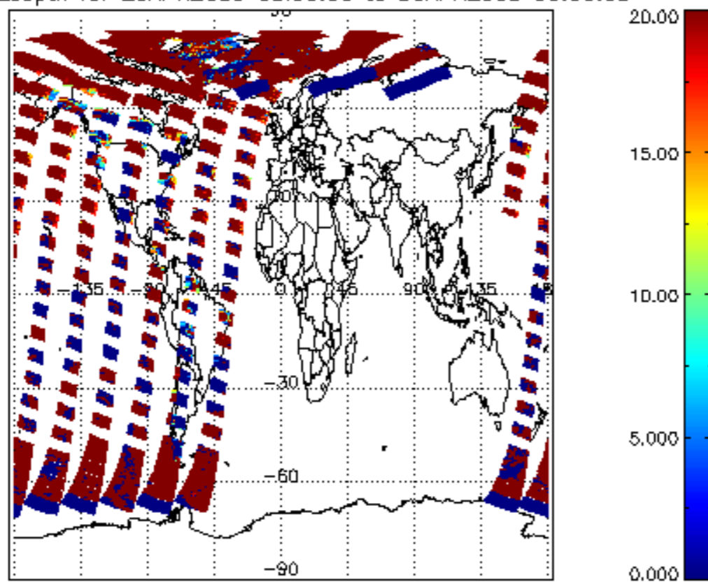
cl_opt_depth for 29APR2009 00:00:00 to 30APR2009 00:00:00
