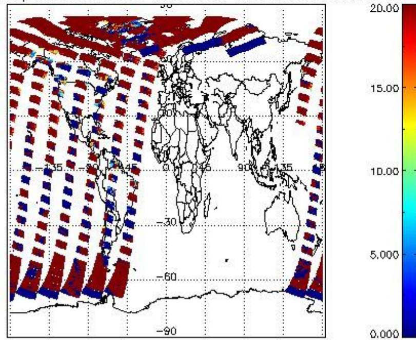
cL_opt_depth for 29APR2009 00:00:00 to 30APR2009 00:00:00
