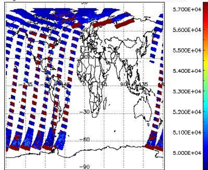
cloud_flags for 29APR2009 00:00:00 to 30APR2009 00:00:00
