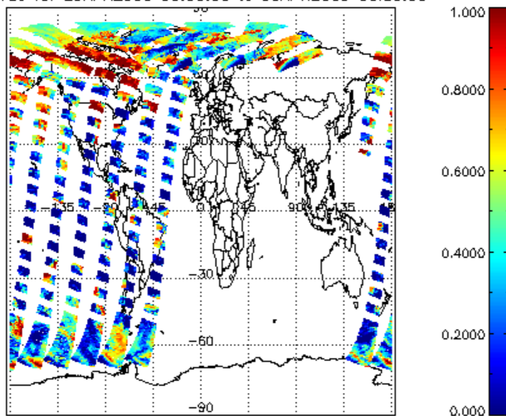
cl_frac for 29APR2009 00:00:00 to 30APR2009 00:00:00
