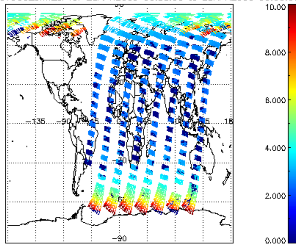
SCIOL2P_NADUV003_amf_cl for 28APR2009 00:00:00 to 29APR2009 00:00:00
