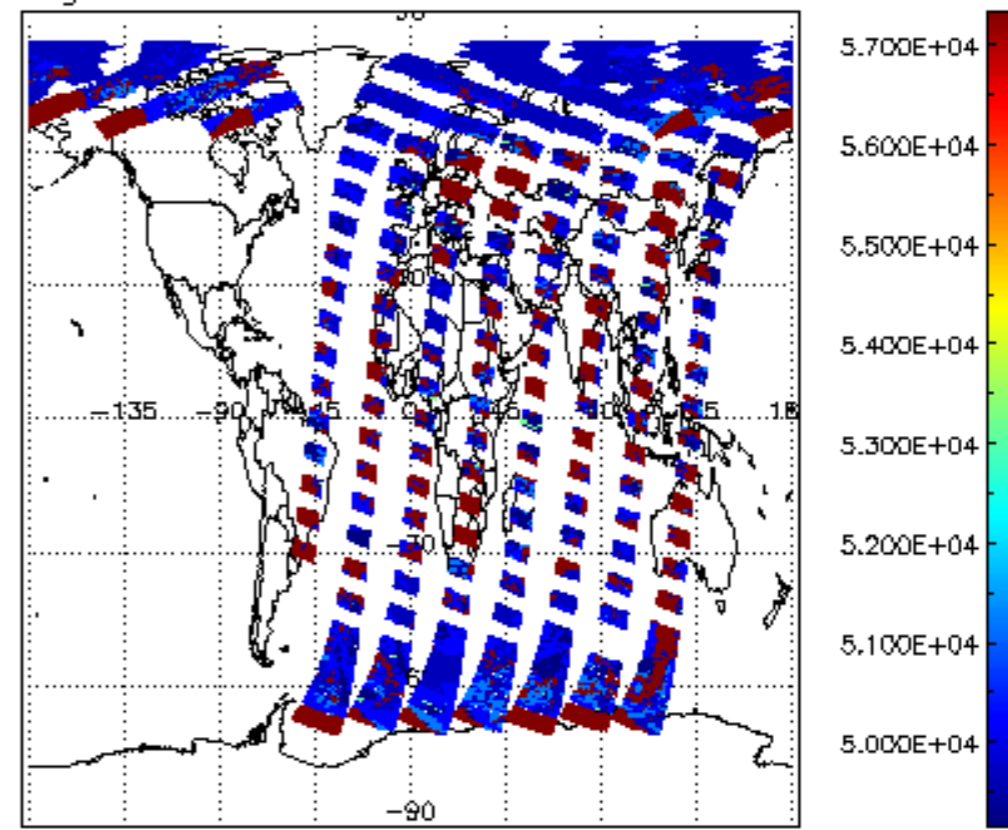
cloud_flags for 28APR2009 00:00:00 to 29APR2009 00:00:00
