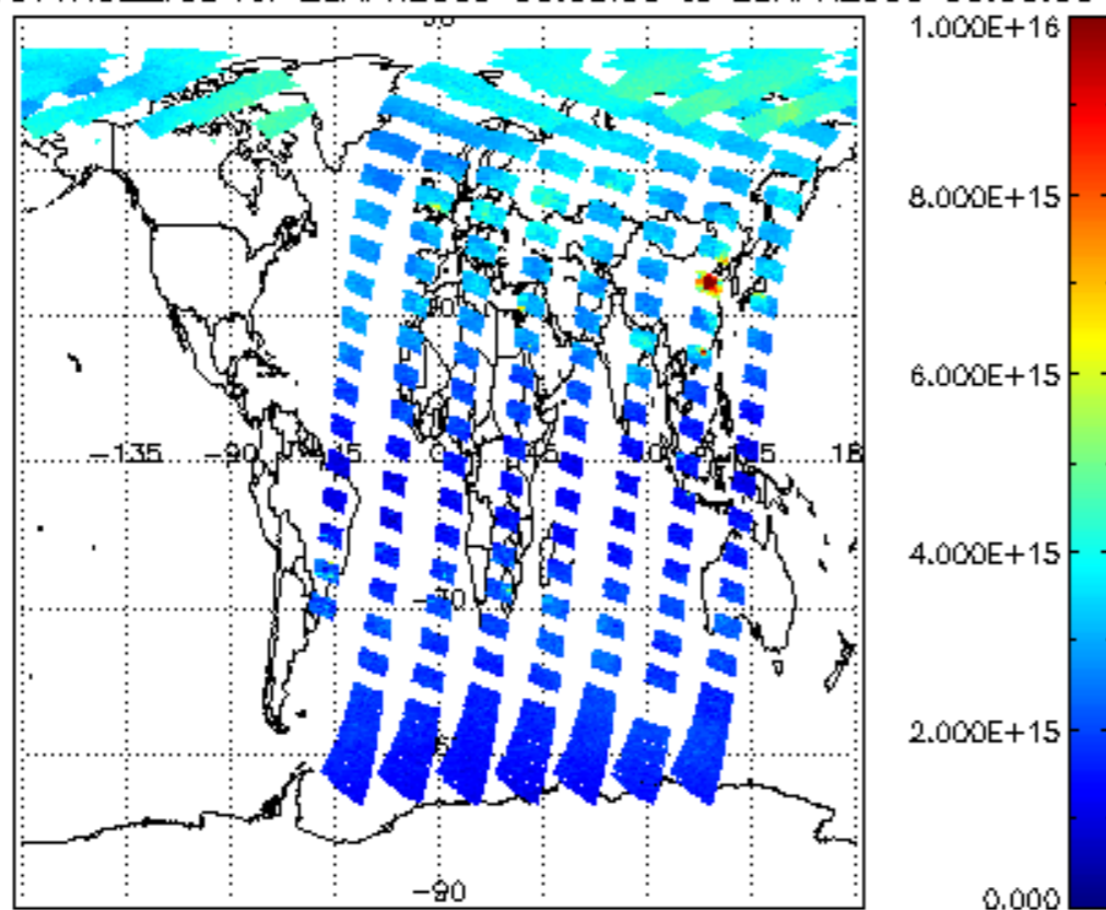
SCIOL2P_NADUV1NO2_vcd for 28APR2009 00:00:00 to 29APR2009 00:00:00
