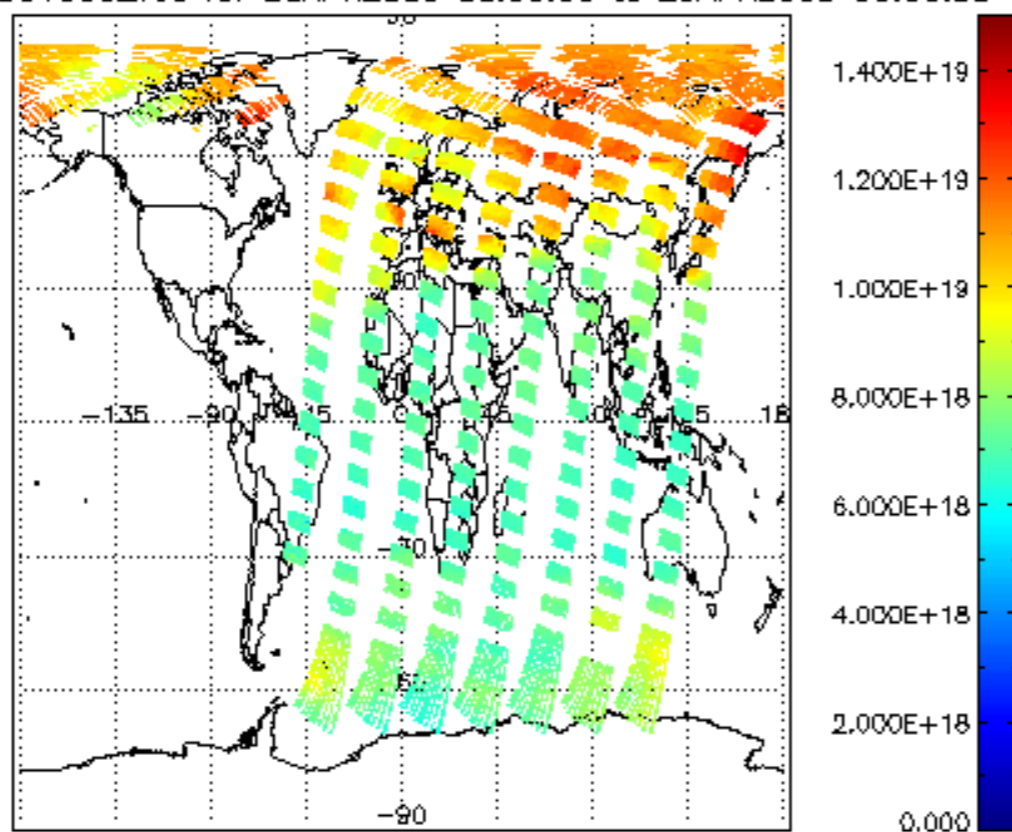
SCIOL2P_NADUV003_vcd for 28APR2009 00:00:00 to 29APR2009 00:00:00
