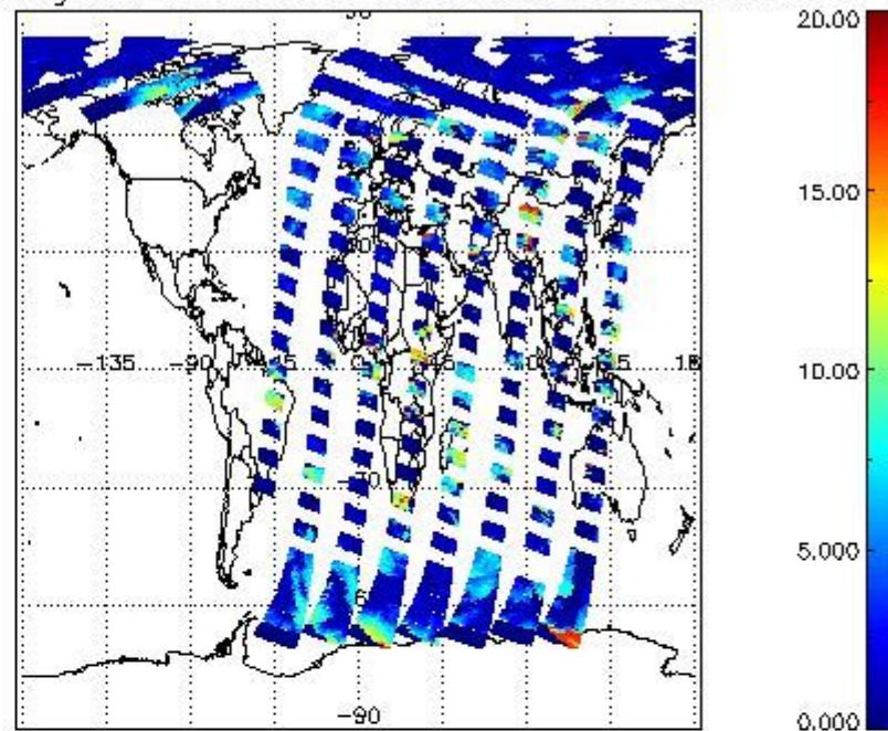
cL_top_height for 28APR2009 00:00:00 to 29APR2009 00:00:00
