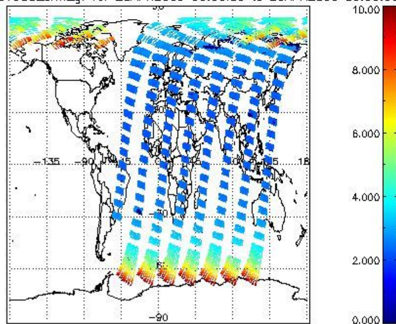
SCIOL2P_NADUV003_amf_gr for 28APR2009 00:00:00 to 29APR2009 00:00:00
