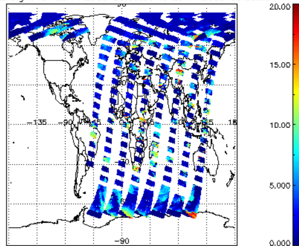
cl_top_height for 28APR2009 00:00:00 to 29APR2009 00:00:00
