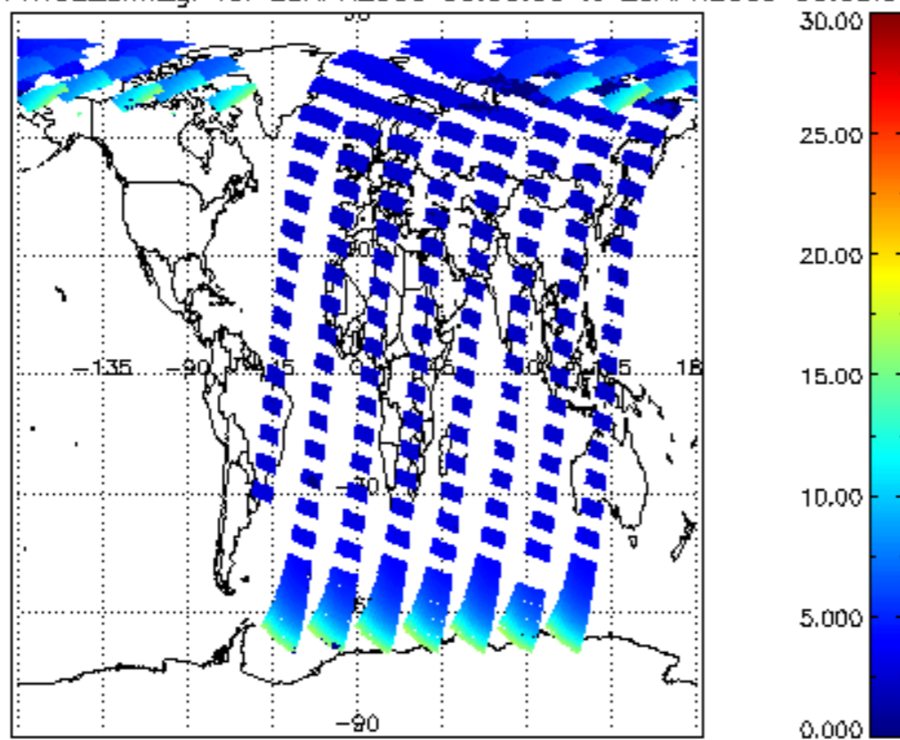
iCIOL2P_NADUV1NO2_amf_gr for 28APR2009 00:00:00 to 29APR2009 00:00:00
