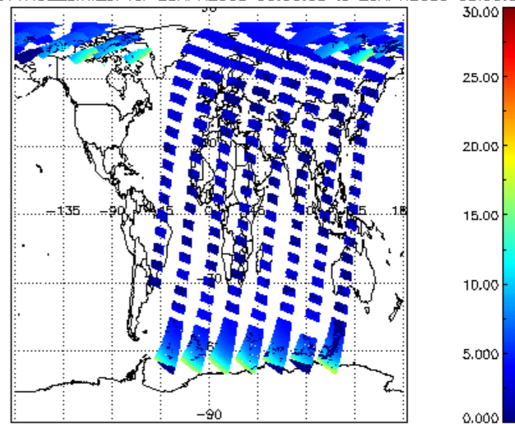
iCIOL2P_NADUV1NO2_amf_cl for 28APR2009 00:00:00 to 29APR2009 00:00:00
