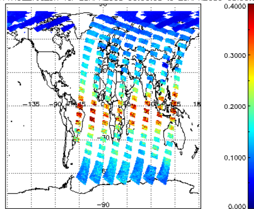
iCIOL2P_NADUV1NO2_vcd_err for 28APR2009 00:00:00 to 29APR2009 00:00:00
