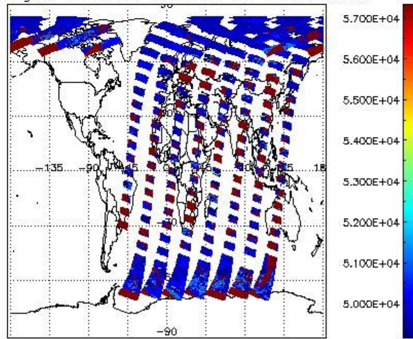
cloud_flags for 28APR2009 00:00:00 to 29APR2009 00:00:00
