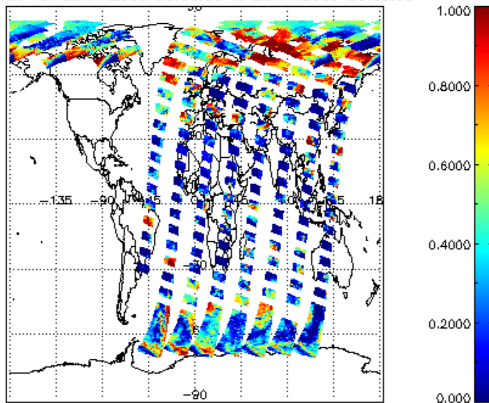
cl_frac for 28APR2009 00:00:00 to 29APR2009 00:00:00
