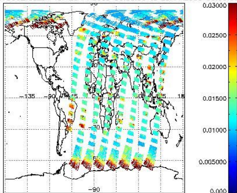
SCIOL2P_NADUV003_vcd_err for 28APR2009 00:00:00 to 29APR2009 00:00:00
