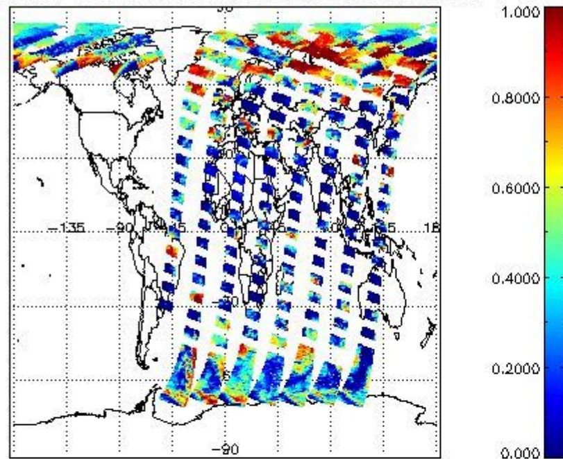
cL_frac for 28APR2009 00:00:00 to 29APR2009 00:00:00
