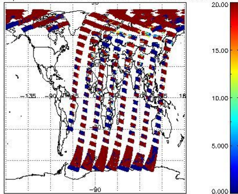
cL_opt_depth for 28APR2009 00:00:00 to 29APR2009 00:00:00
