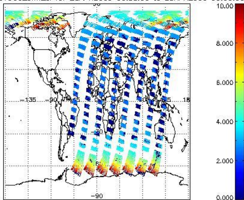
SCIOL2P_NADUV003_amf_cl for 28APR2009 00:00:00 to 29APR2009 00:00:00
