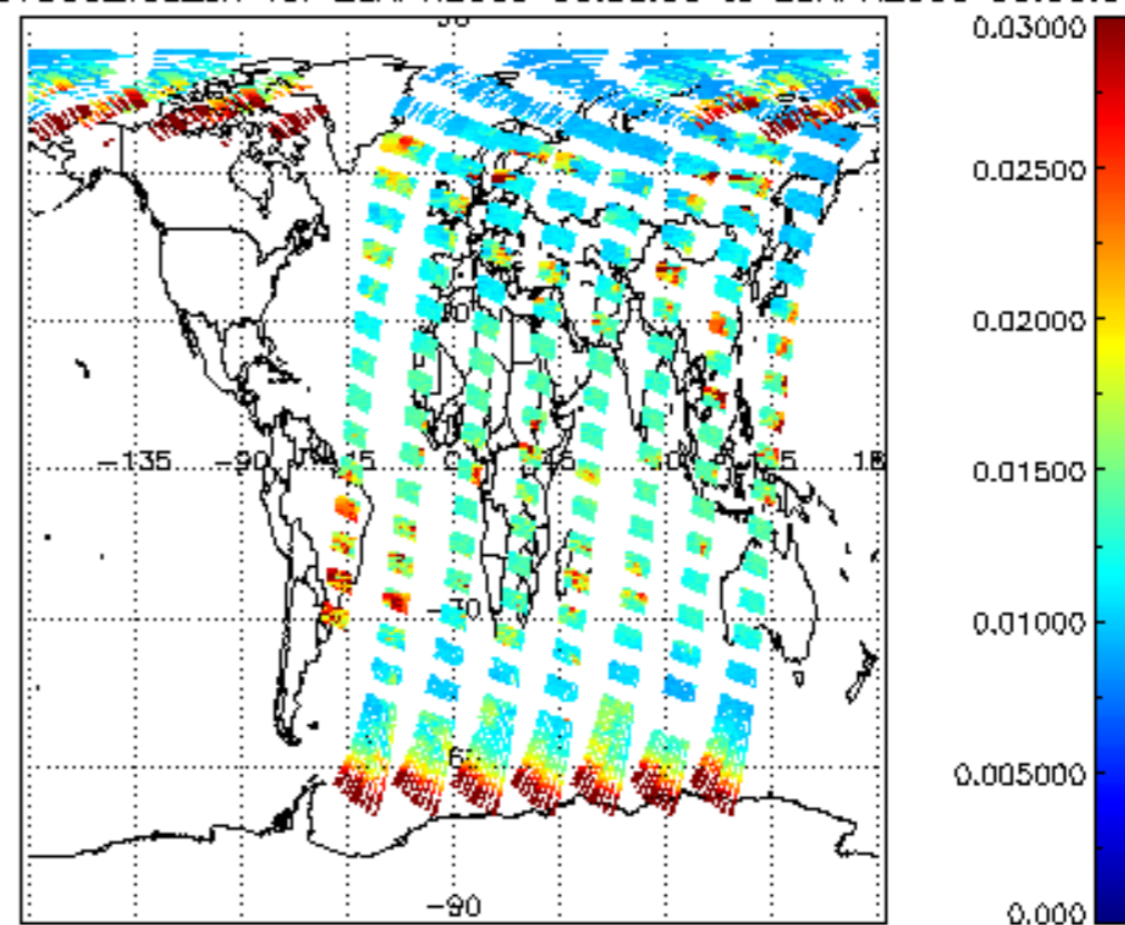
SCIOL2P_NADUV003_vcd_err for 28APR2009 00:00:00 to 29APR2009 00:00:00
