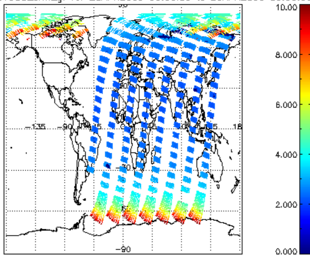
SCIOL2P_NADUV003_amf_gr for 28APR2009 00:00:00 to 29APR2009 00:00:00
