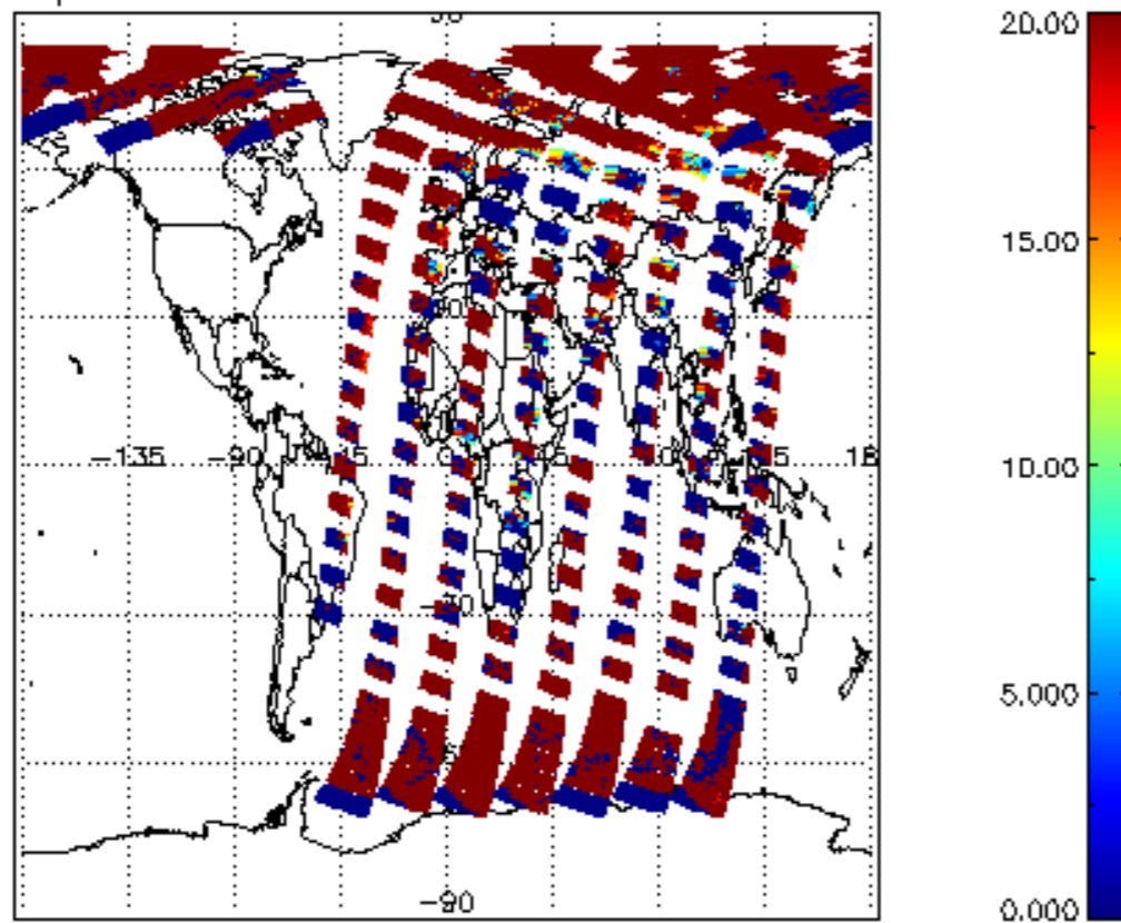
cl_opt_depth for 28APR2009 00:00:00 to 29APR2009 00:00:00
