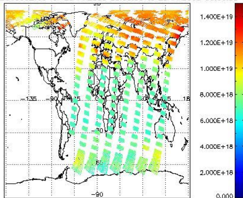
SCIOL2P_NADUV003_vcd for 28APR2009 00:00:00 to 29APR2009 00:00:00
