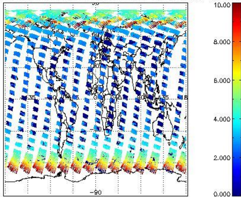
SCIOL2P_NADUV003_amf_cl for 25APR2009 00:00:00 to 26APR2009 00:00:00
