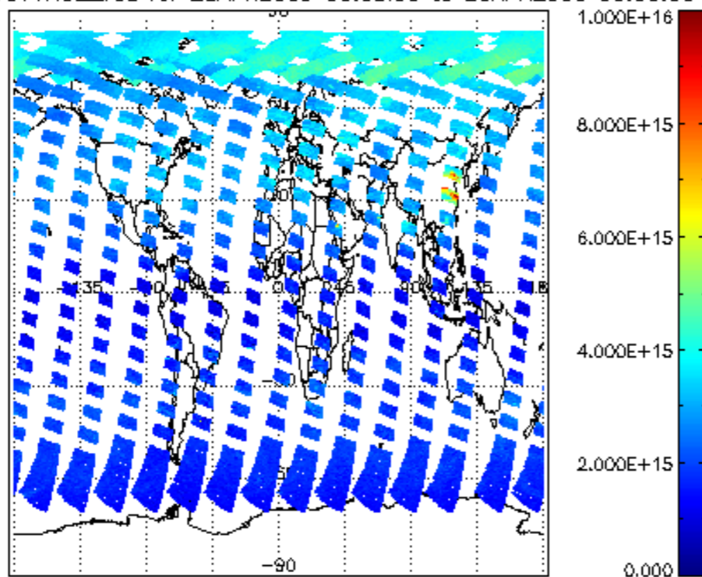
SCIOL2P_NADUV1NO2_vcd for 25APR2009 00:00:00 to 26APR2009 00:00:00
