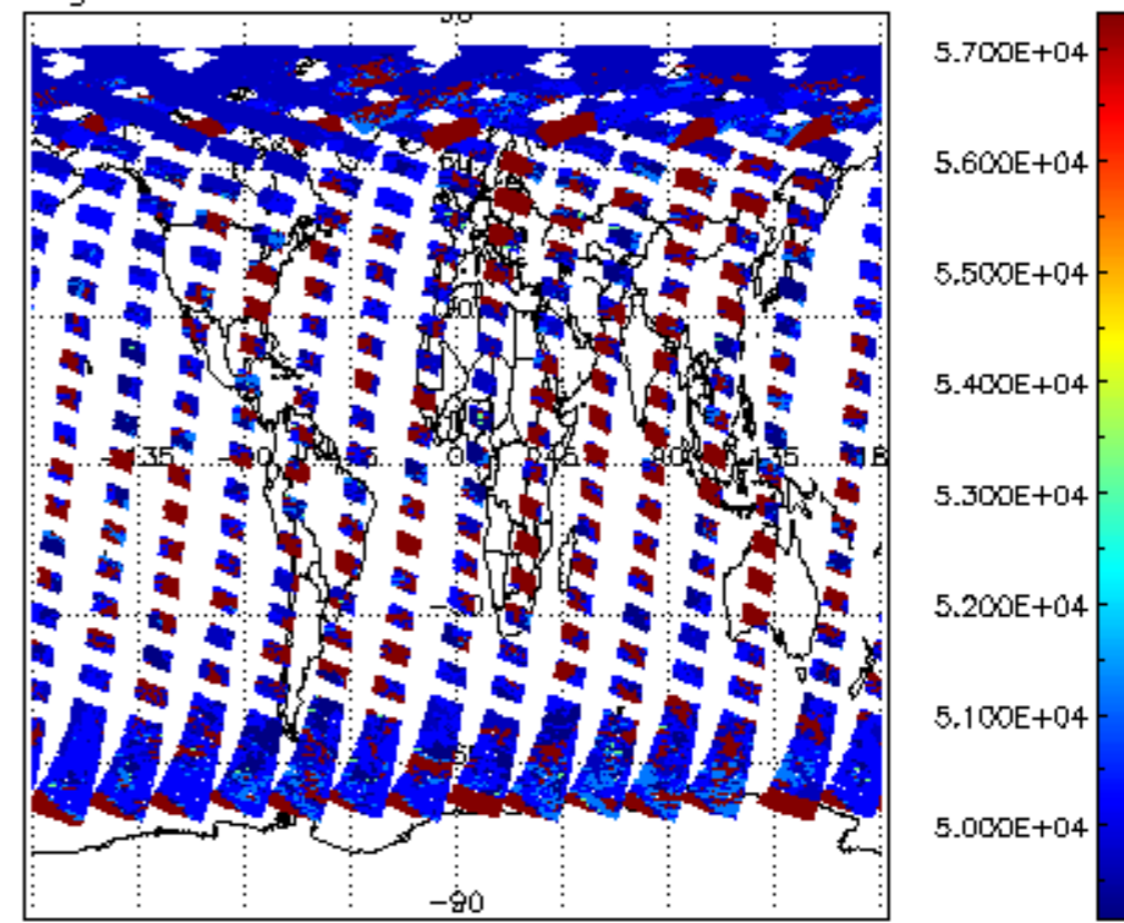
cloud_flags for 25APR2009 00:00:00 to 26APR2009 00:00:00
