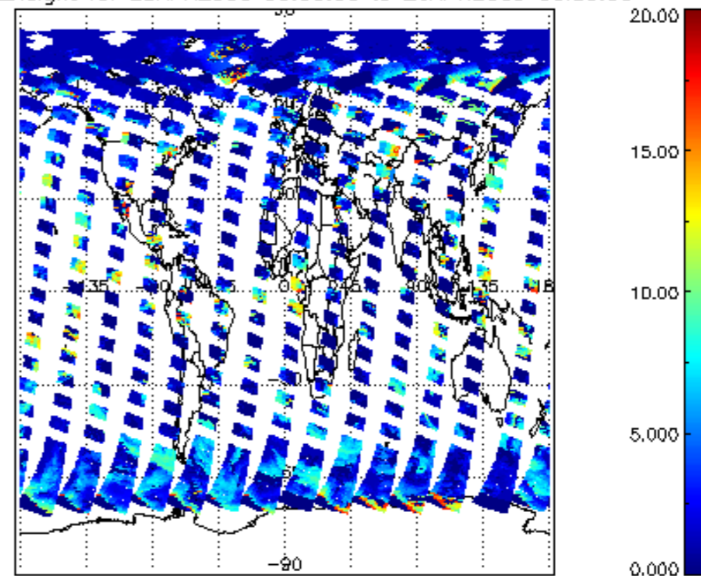
cl_top_height for 25APR2009 00:00:00 to 26APR2009 00:00:00
