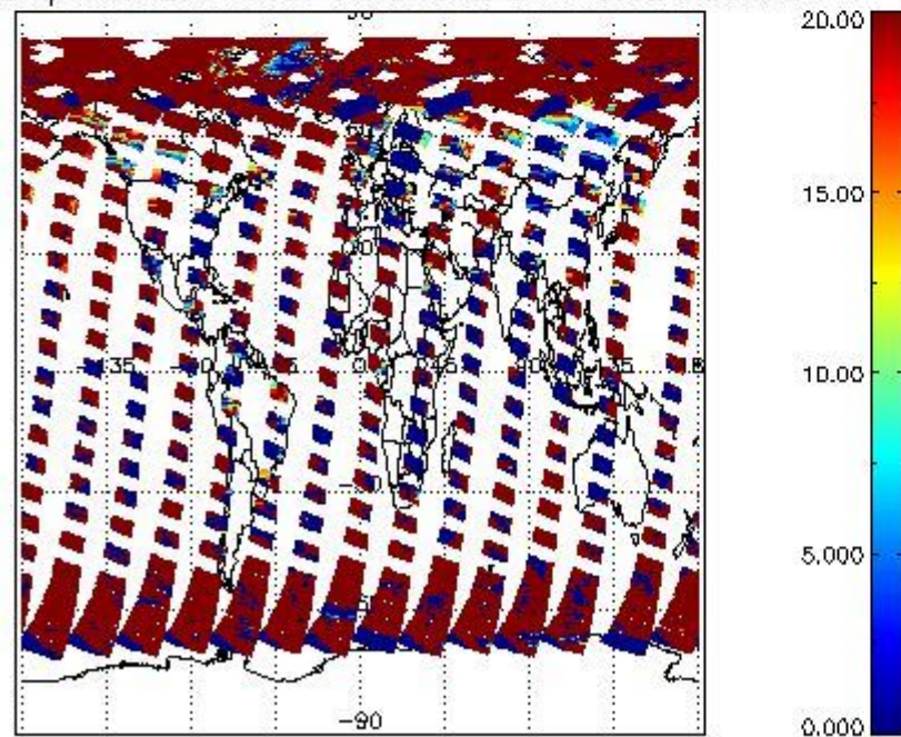
cLopt_depth for 25APR2009 00:00:00 to 26APR2009 00:00:00
