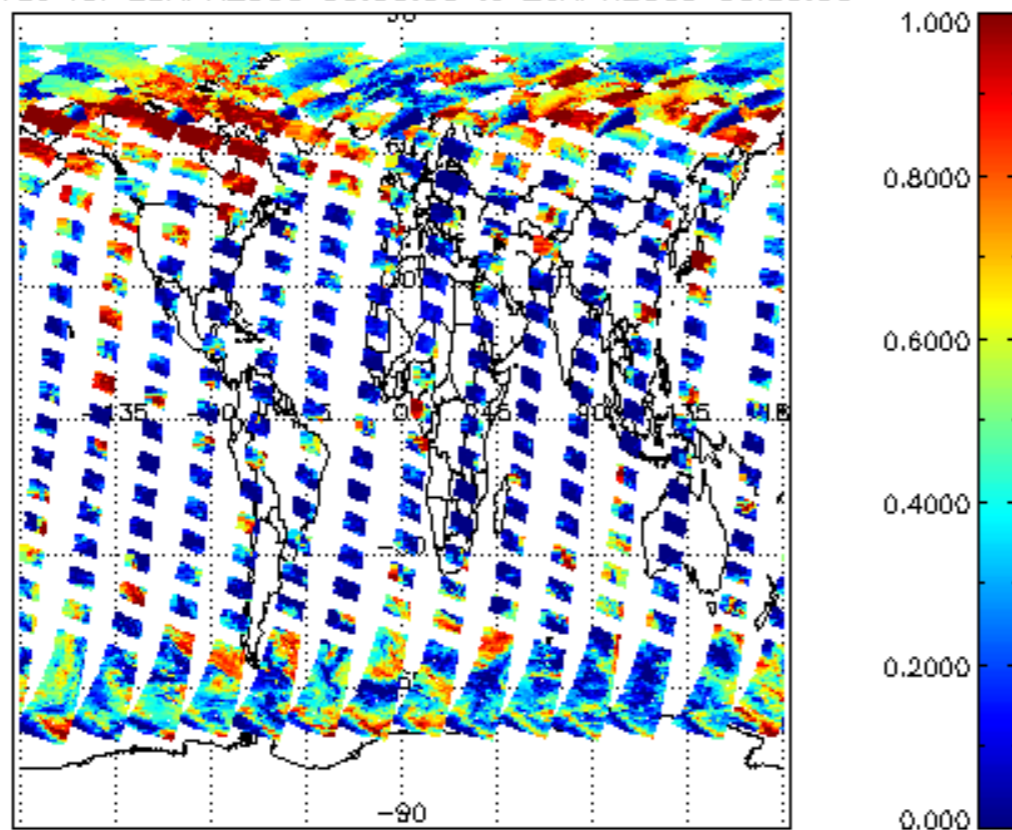
cl_frac for 25APR2009 00:00:00 to 26APR2009 00:00:00
