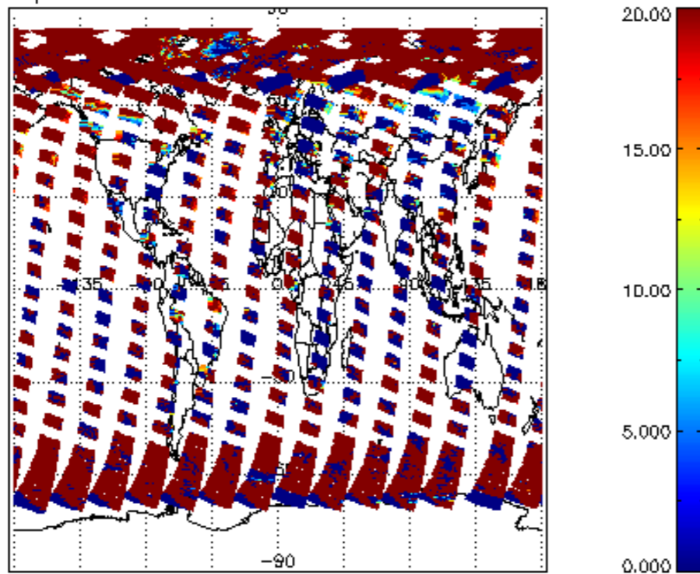
cl_opt_depth for 25APR2009 00:00:00 to 26APR2009 00:00:00
