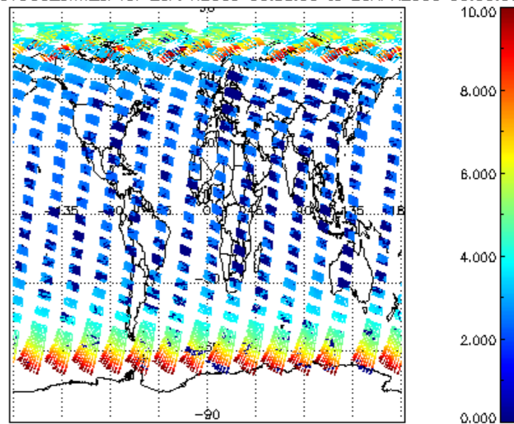
SCIOL2P_NADUV003_amf_cl for 25APR2009 00:00:00 to 26APR2009 00:00:00
