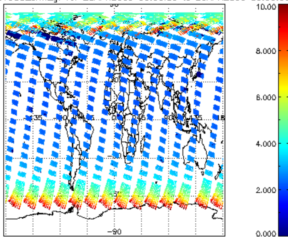
SCIOL2P_NADUV003_amf_gr for 25APR2009 00:00:00 to 26APR2009 00:00:00
