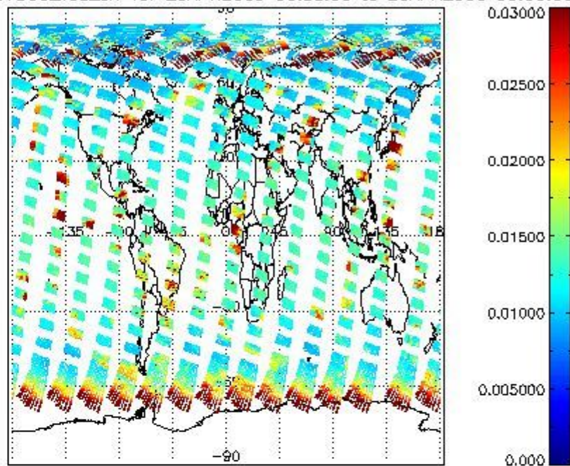
SCIOL2P_NADUV003_vcd_err for 25APR2009 00:00:00 to 26APR2009 00:00:00
