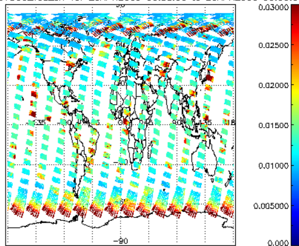
SCIOL2P_NADUV003_vcd_err for 25APR2009 00:00:00 to 26APR2009 00:00:00
