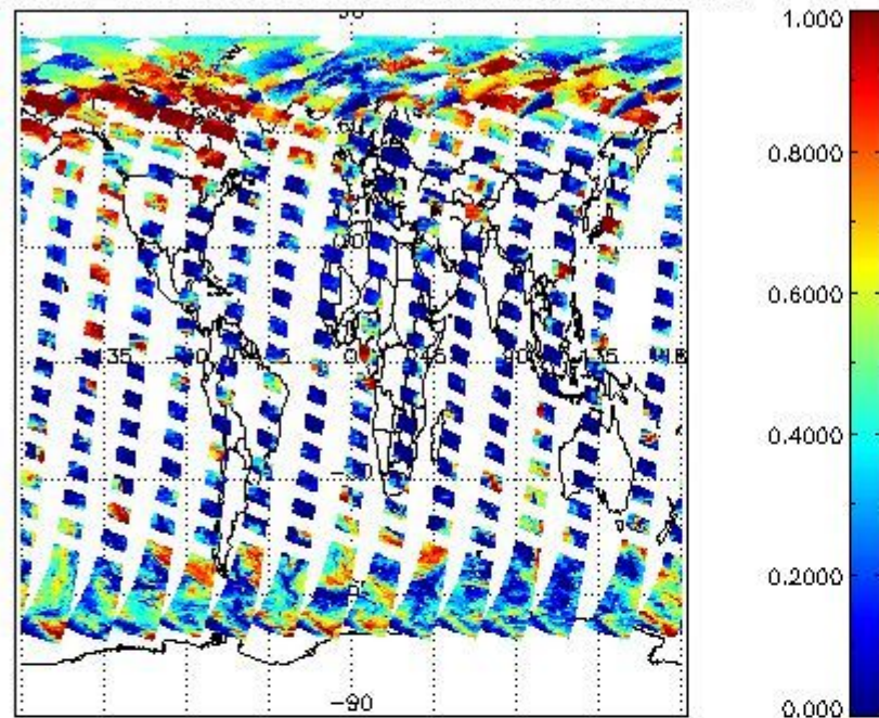
cLfrac for 25APR2009 00:00:00 to 26APR2009 00:00:00
