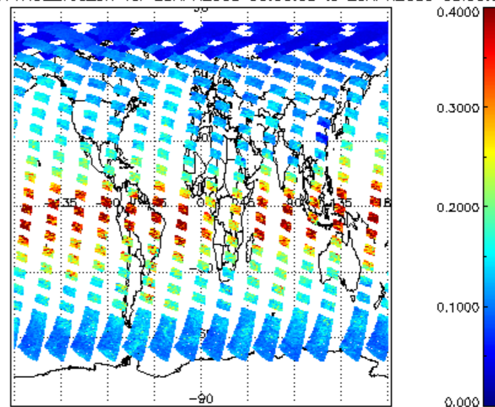
iCIOL2P_NADUV1NO2_vcd_err for 25APR2009 00:00:00 to 26APR2009 00:00:00
