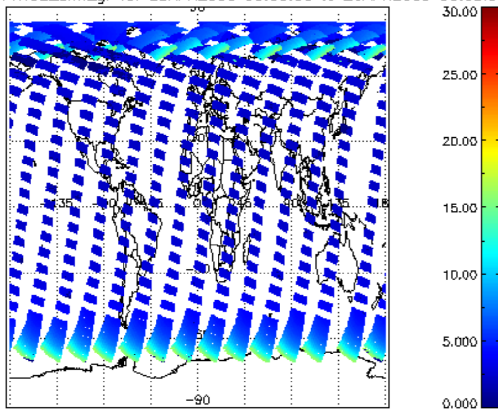
iCIOL2P_NADUV1NO2_amf_gr for 25APR2009 00:00:00 to 26APR2009 00:00:00
