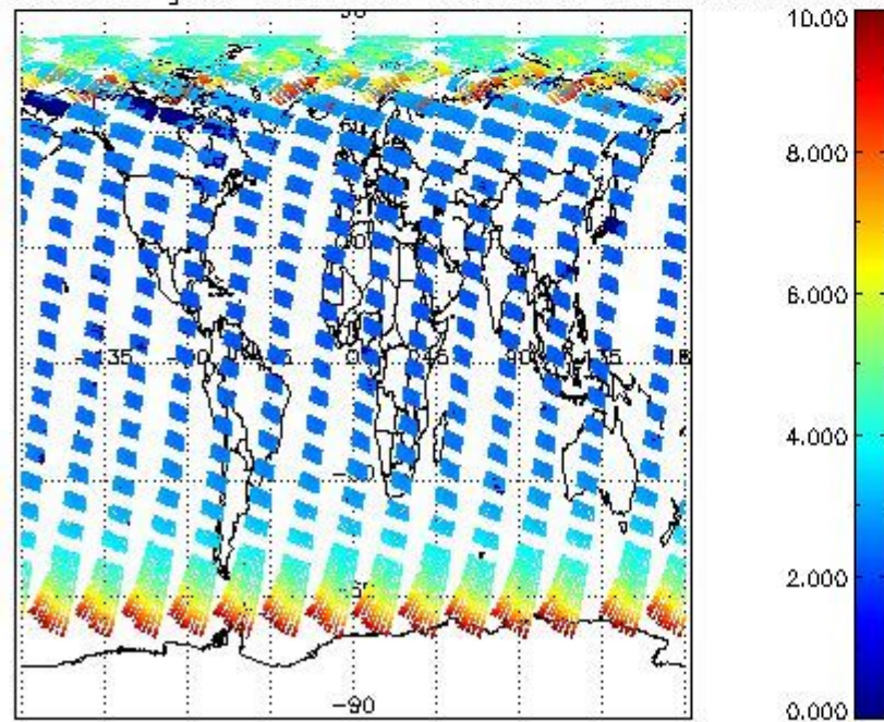
SCIOL2P_NADUV003_amf_gr for 25APR2009 00:00:00 to 26APR2009 00:00:00
