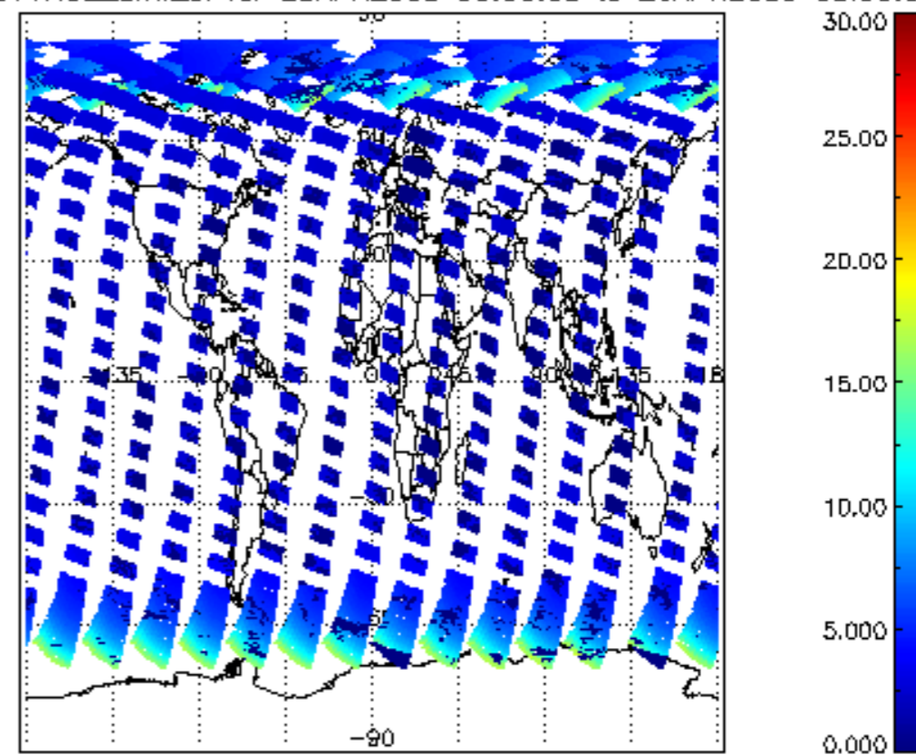
iCIOL2P_NADUV1NO2_amf_cl for 25APR2009 00:00:00 to 26APR2009 00:00:00
