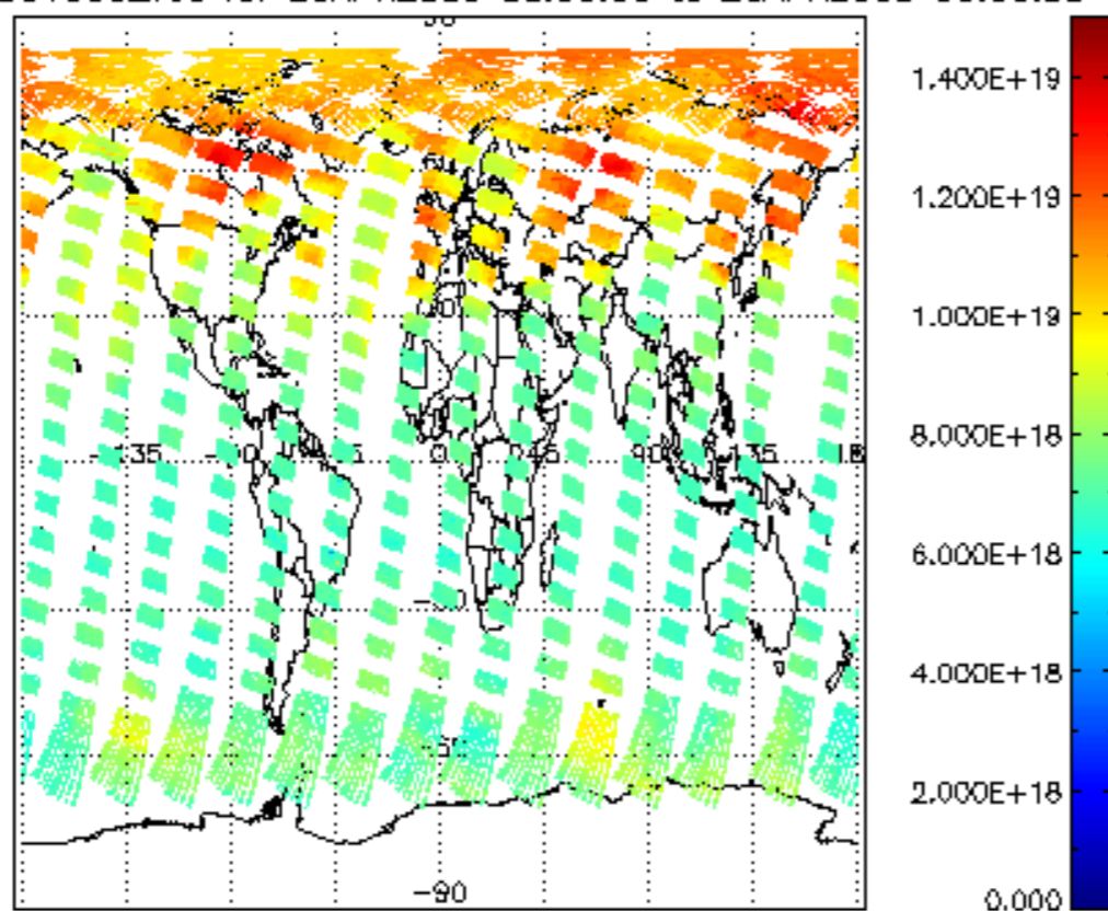
SCIOL2P_NADUV003_vcd for 25APR2009 00:00:00 to 26APR2009 00:00:00
