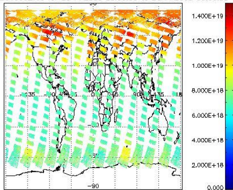
SCIOL2P_NADUV003_vcd for 25APR2009 00:00:00 to 26APR2009 00:00:00
