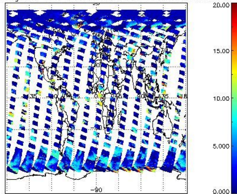
cL_top_height for 25APR2009 00:00:00 to 26APR2009 00:00:00
