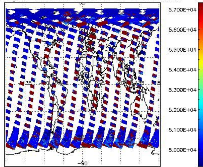
cloud_flags for 25APR2009 00:00:00 to 26APR2009 00:00:00
