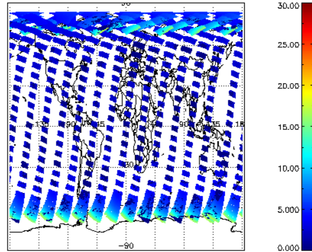
iCIOL2P_NADUV1NO2_amf_cl for 24APR2009 00:00:00 to 25APR2009 00:00:00
