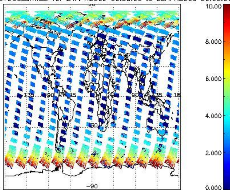
SCIOL2P_NADUV003_amf_cl for 24APR2009 00:00:00 to 25APR2009 00:00:00
