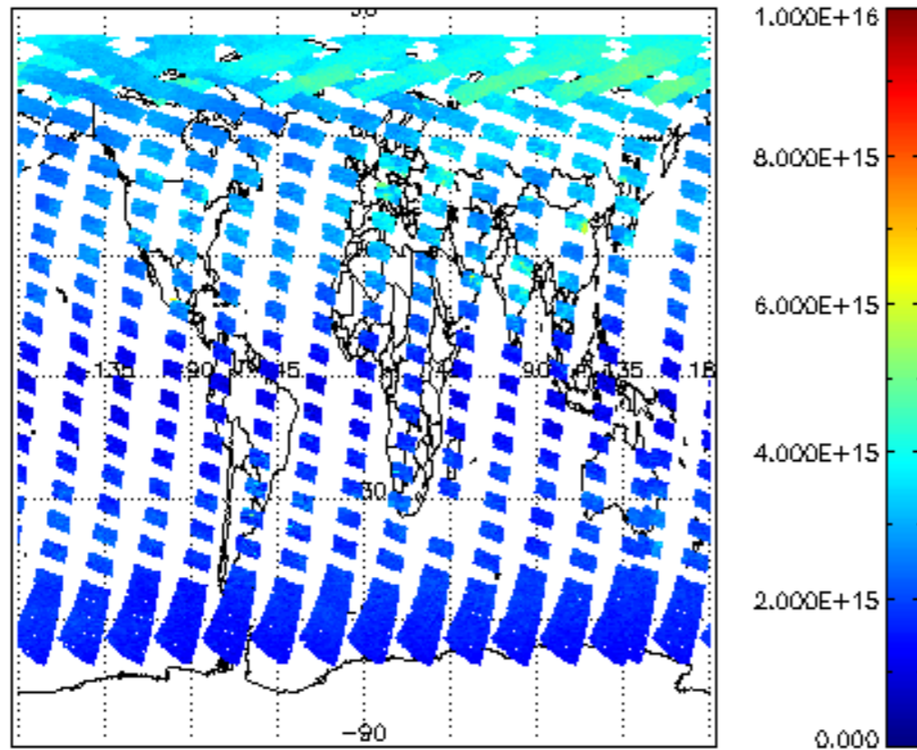
SCIOL2P_NADUV1NO2_vcd for 24APR2009 00:00:00 to 25APR2009 00:00:00
