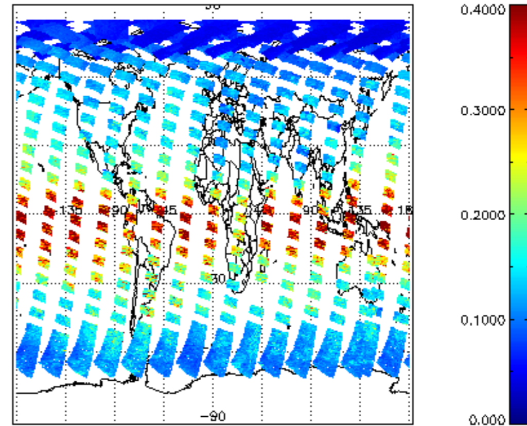
iCIOL2P_NADUV1NO2_vcd_err for 24APR2009 00:00:00 to 25APR2009 00:00:00
