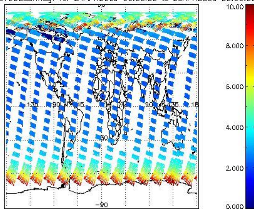
SCIOL2P_NADUV003_amf_gr for 24APR2009 00:00:00 to 25APR2009 00:00:00
