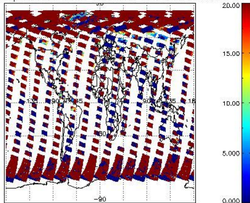
cL_opt_depth for 24APR2009 00:00:00 to 25APR2009 00:00:00
