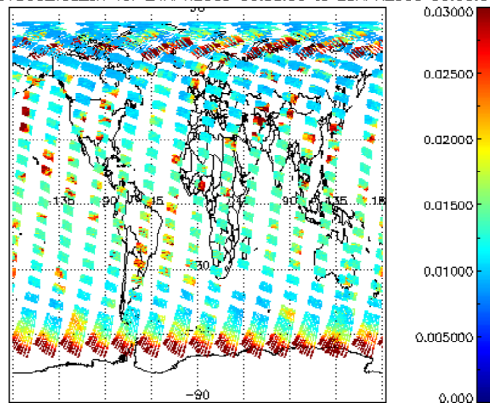
SCIOL2P_NADUV003_vcd_err for 24APR2009 00:00:00 to 25APR2009 00:00:00
