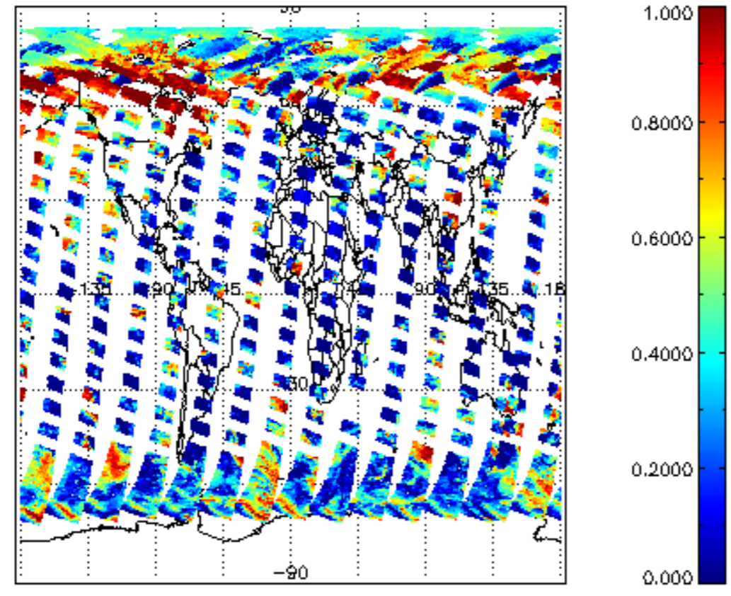
cL_frac for 24APR2009 00:00:00 to 25APR2009 00:00:00
