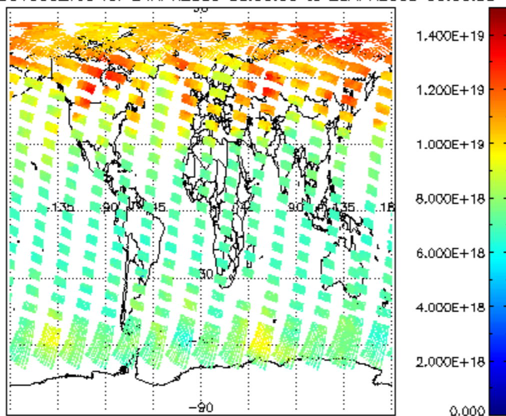
SCIOL2P_NADUV003_vcd for 24APR2009 00:00:00 to 25APR2009 00:00:00
