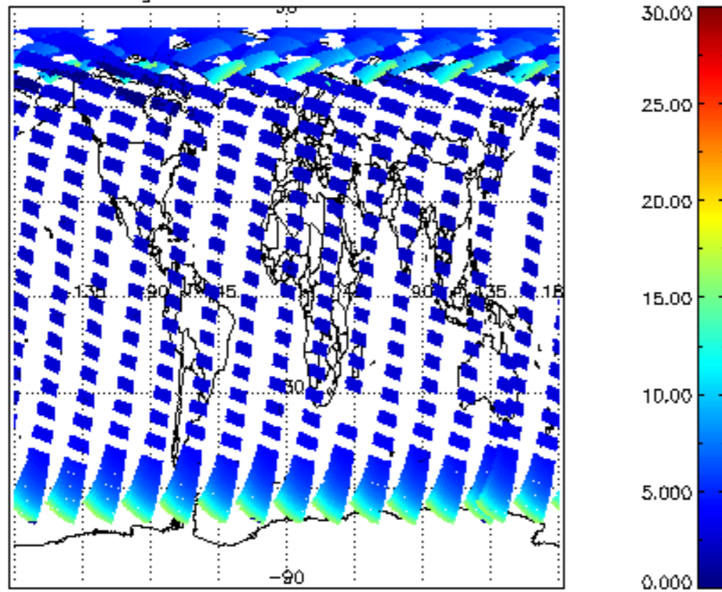
iCIOL2P_NADUV1NO2_amf_gr for 24APR2009 00:00:00 to 25APR2009 00:00:00
