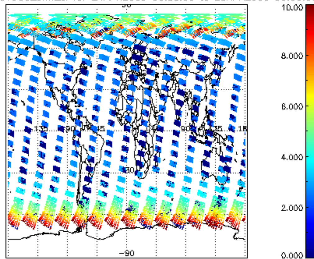
SCIOL2P_NADUV003_amf_cl for 24APR2009 00:00:00 to 25APR2009 00:00:00
