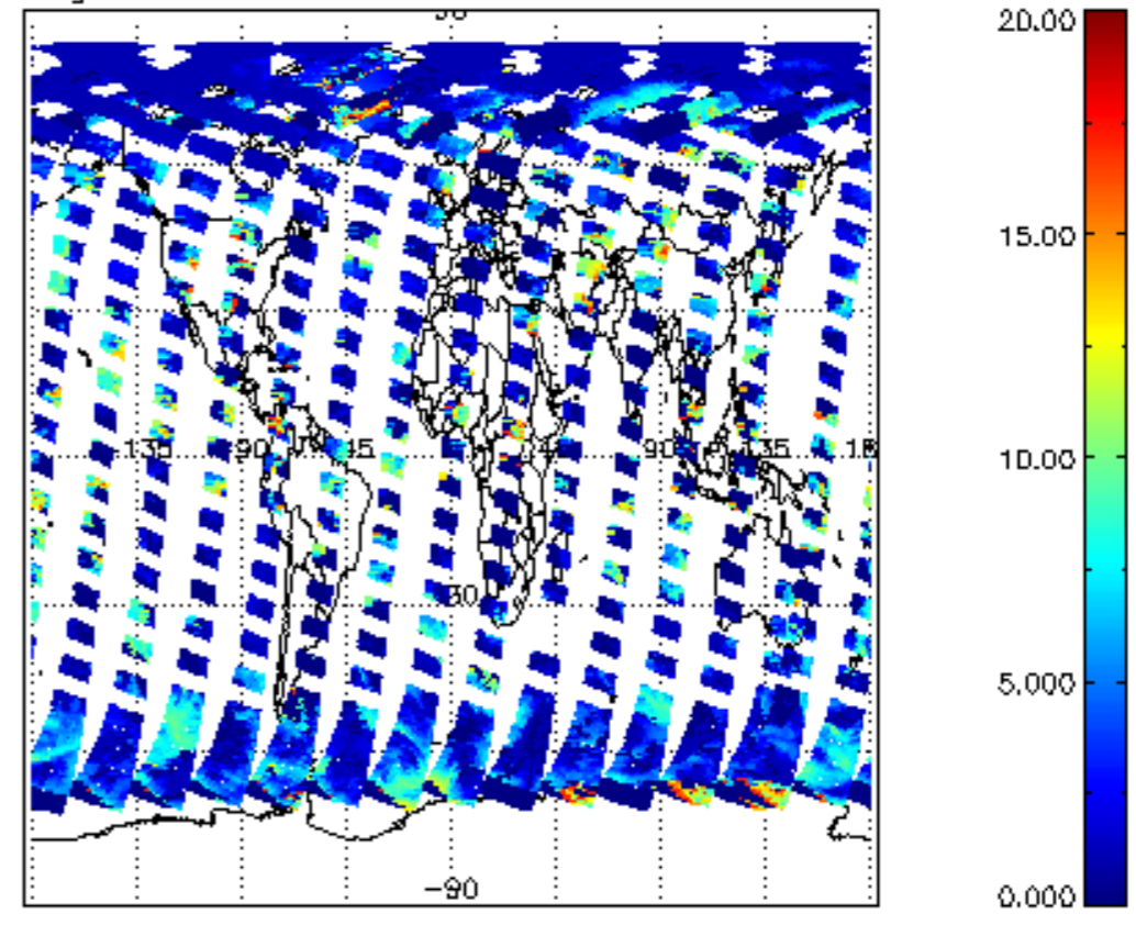
cL_top_height for 24APR2009 00:00:00 to 25APR2009 00:00:00
