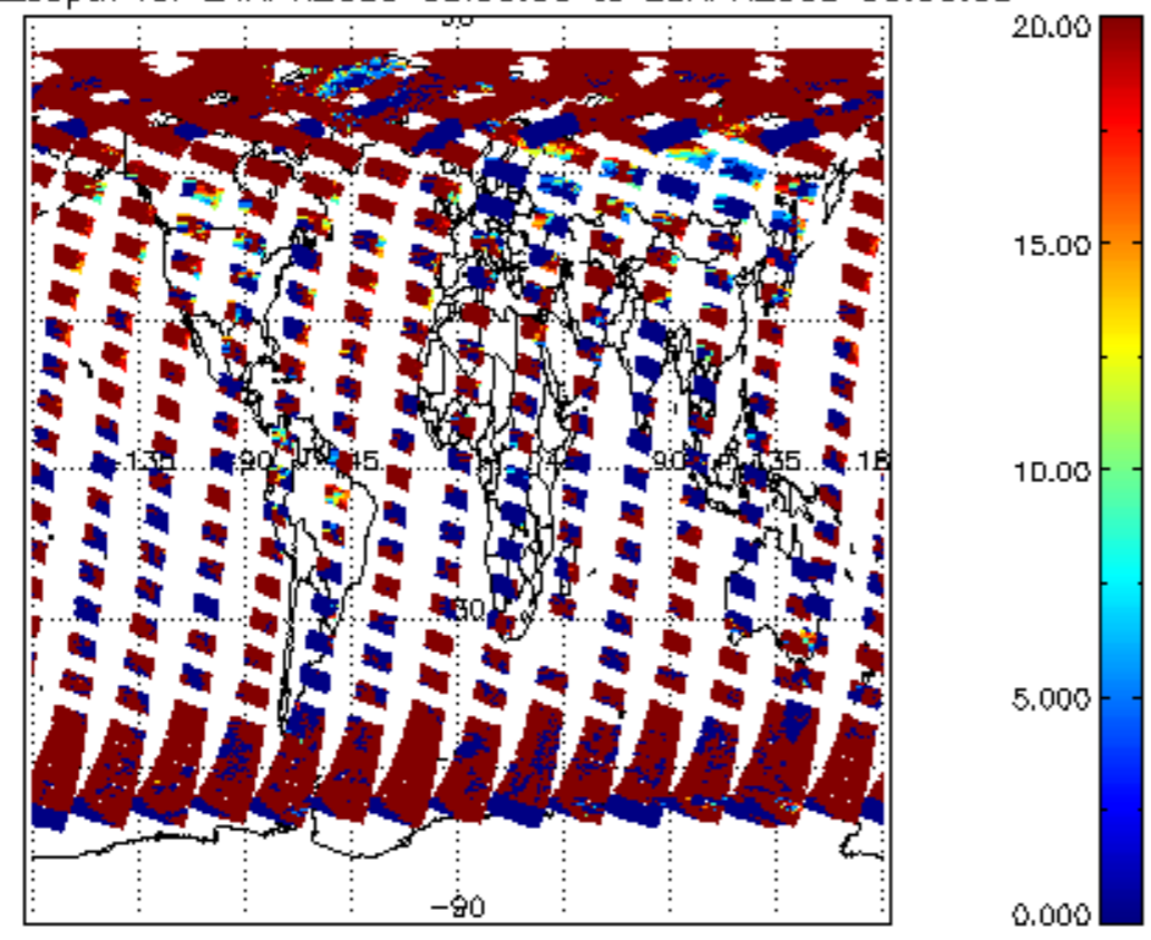
cL_opt_depth for 24APR2009 00:00:00 to 25APR2009 00:00:00
