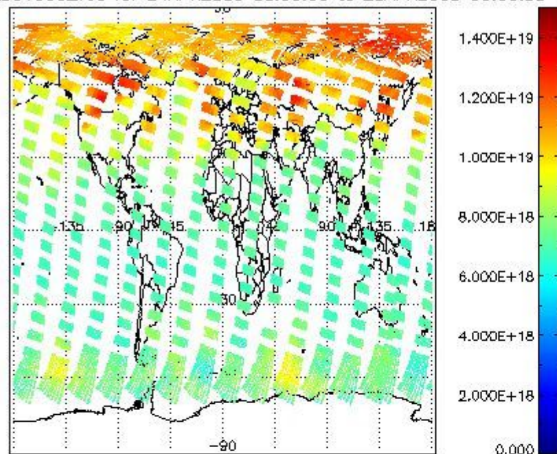
SCIOL2P_NADUV003_vcd for 24APR2009 00:00:00 to 25APR2009 00:00:00
