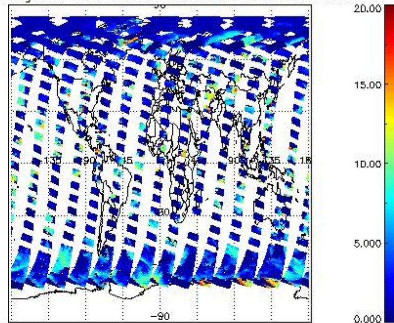
cL_top_height for 24APR2009 00:00:00 to 25APR2009 00:00:00
