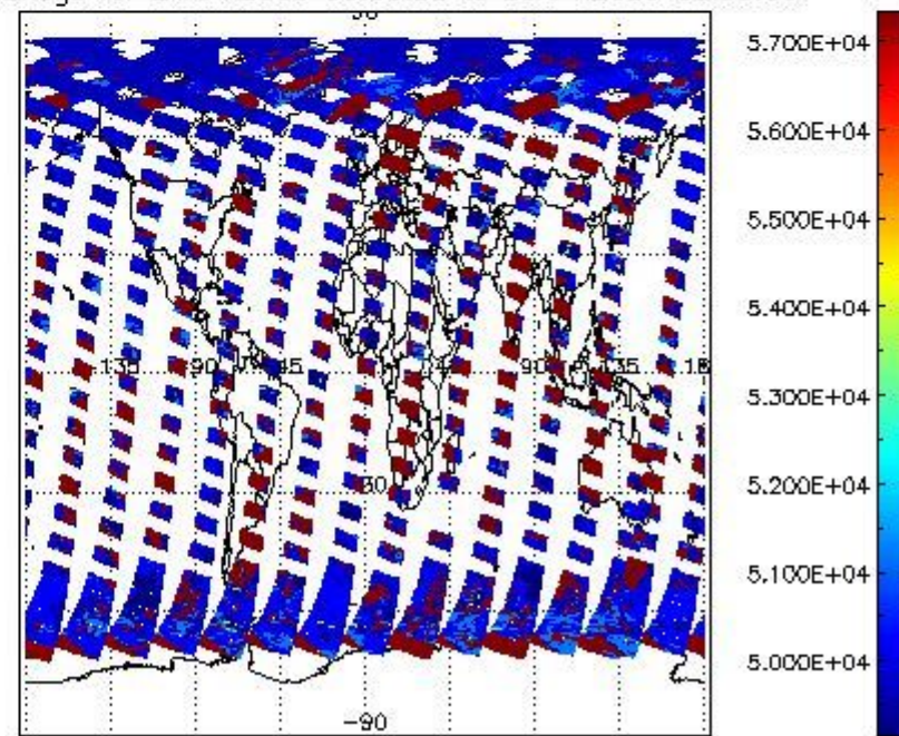
cloud_flags for 24APR2009 00:00:00 to 25APR2009 00:00:00
