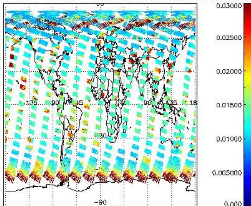
SCIOL2P_NADUV003_vcd_err for 24APR2009 00:00:00 to 25APR2009 00:00:00
