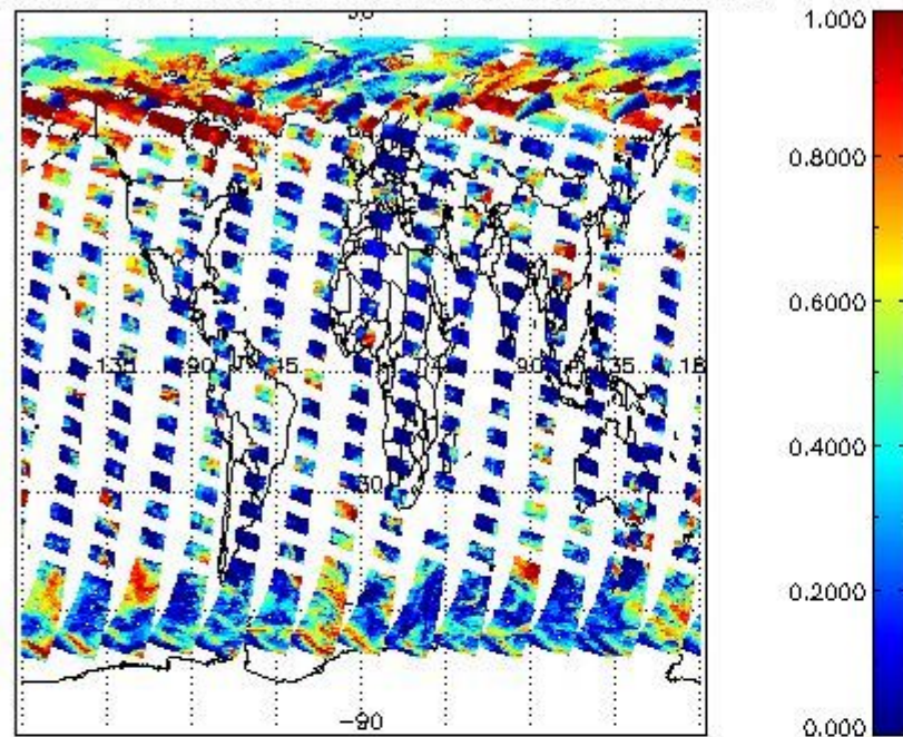
cL_frac for 24APR2009 00:00:00 to 25APR2009 00:00:00
