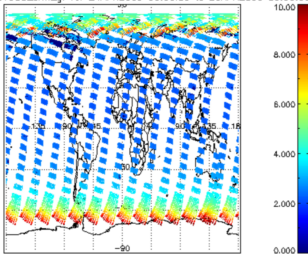
SCIOL2P_NADUV003_amf_gr for 24APR2009 00:00:00 to 25APR2009 00:00:00
