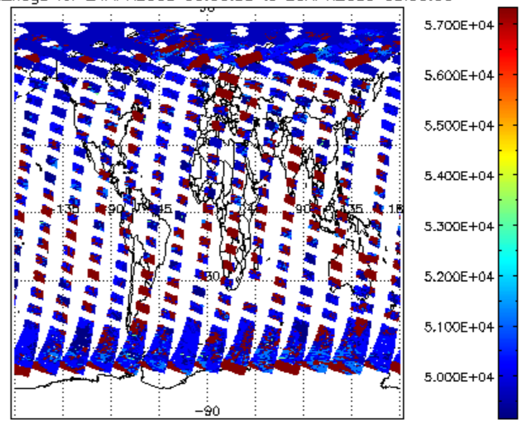
cloud_flags for 24APR2009 00:00:00 to 25APR2009 00:00:00
