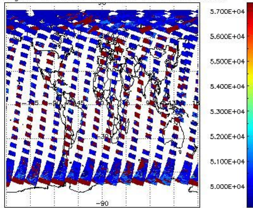
cloud_flags for 23APR2009 00:00:00 to 24APR2009 00:00:00
