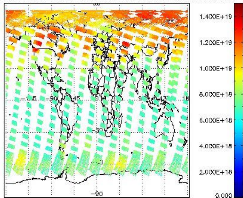
SCIOL2P_NADUV003_vcd for 23APR2009 00:00:00 to 24APR2009 00:00:00
