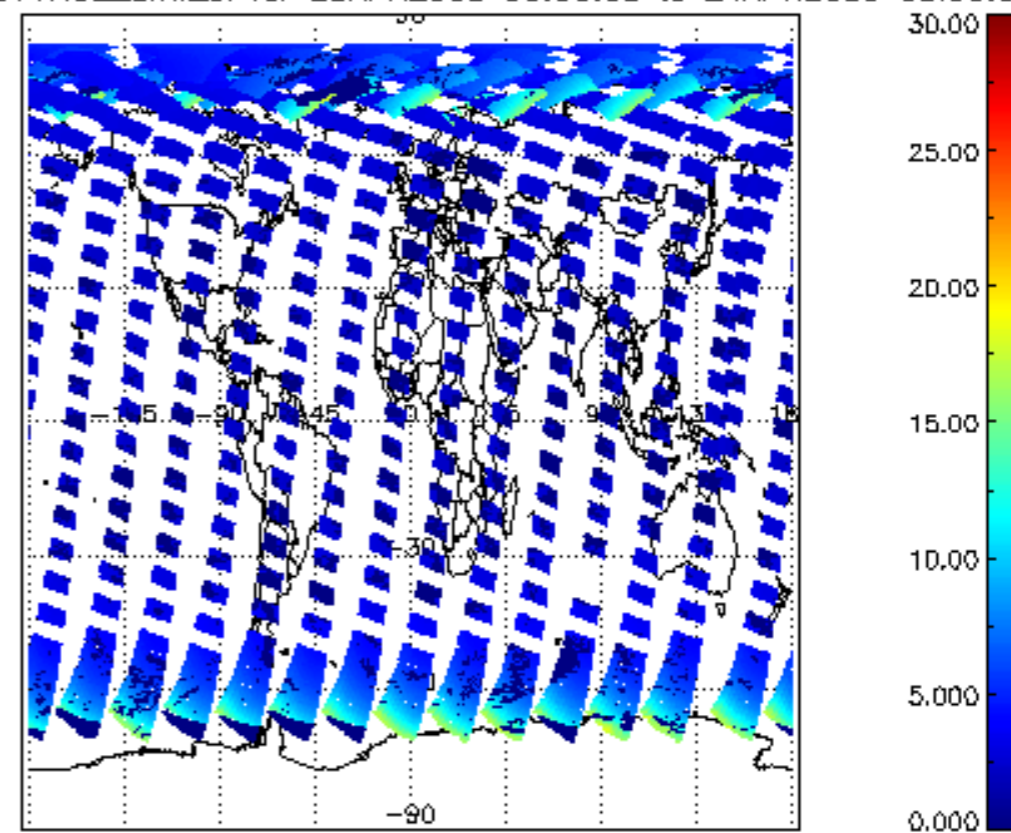
iCIOL2P_NADUV1NO2_amf_cl for 23APR2009 00:00:00 to 24APR2009 00:00:00
