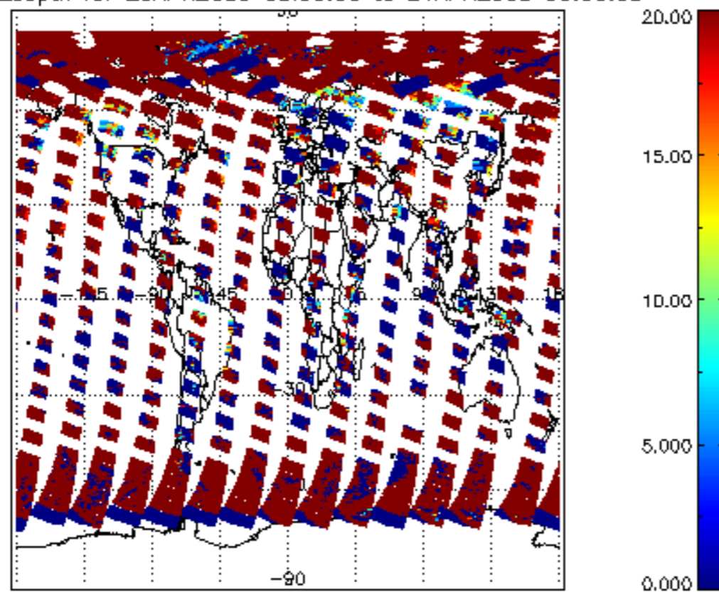
cl_opt_depth for 23APR2009 00:00:00 to 24APR2009 00:00:00
