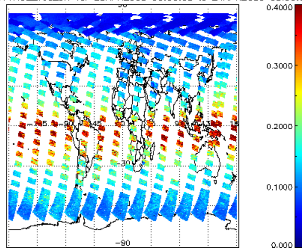
iCIOL2P_NADUV1NO2_vcd_err for 23APR2009 00:00:00 to 24APR2009 00:00:00
