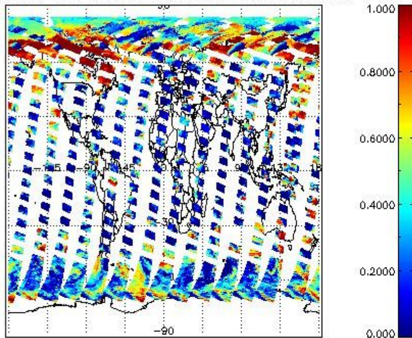
cL_frac for 23APR2009 00:00:00 to 24APR2009 00:00:00
