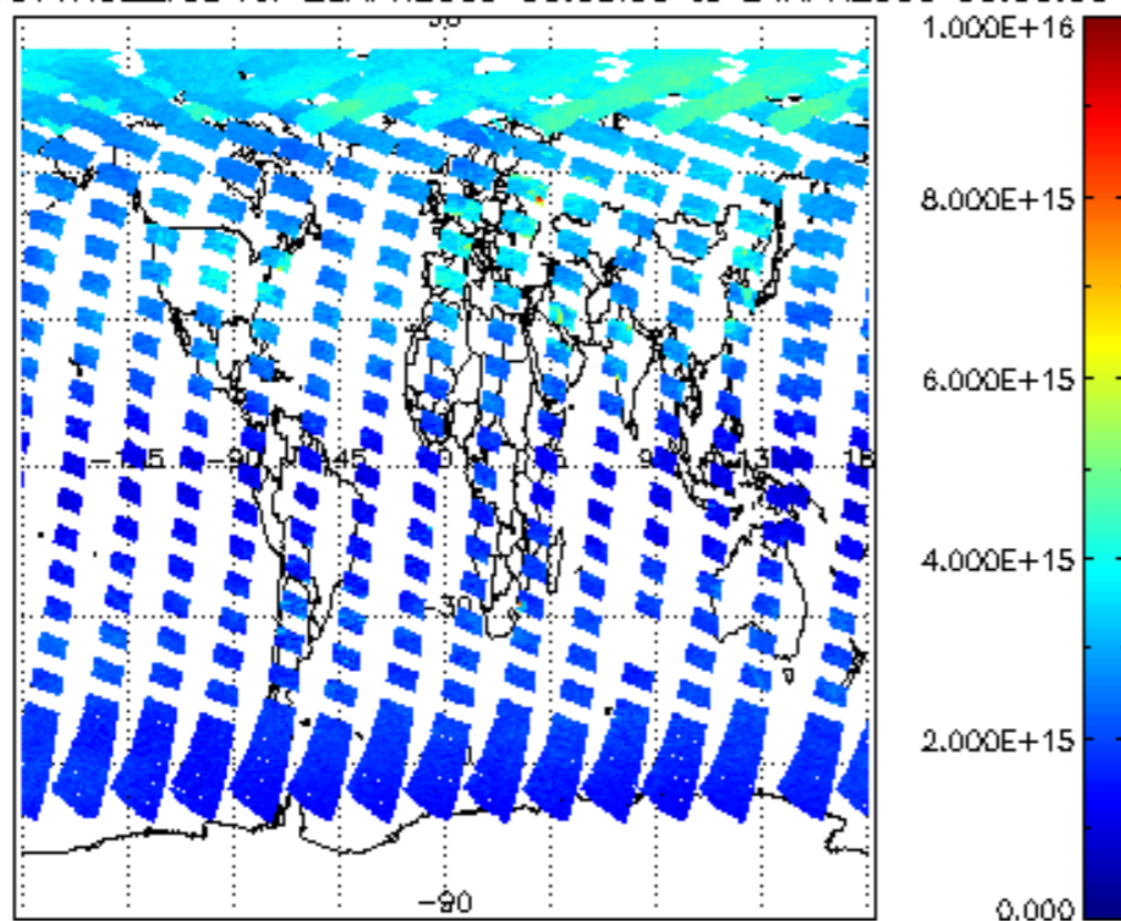
SCIOL2P_NADUV1NO2_vcd for 23APR2009 00:00:00 to 24APR2009 00:00:00
