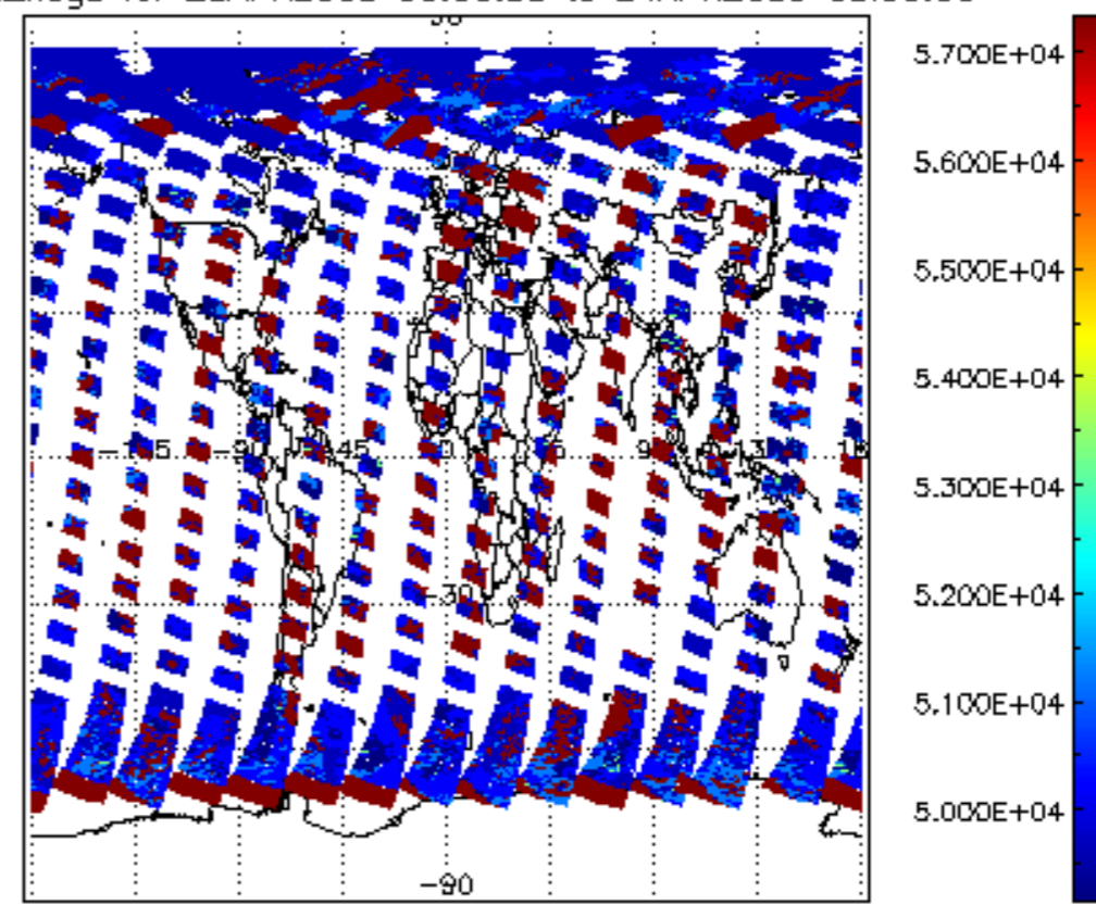
cloud_flags for 23APR2009 00:00:00 to 24APR2009 00:00:00
