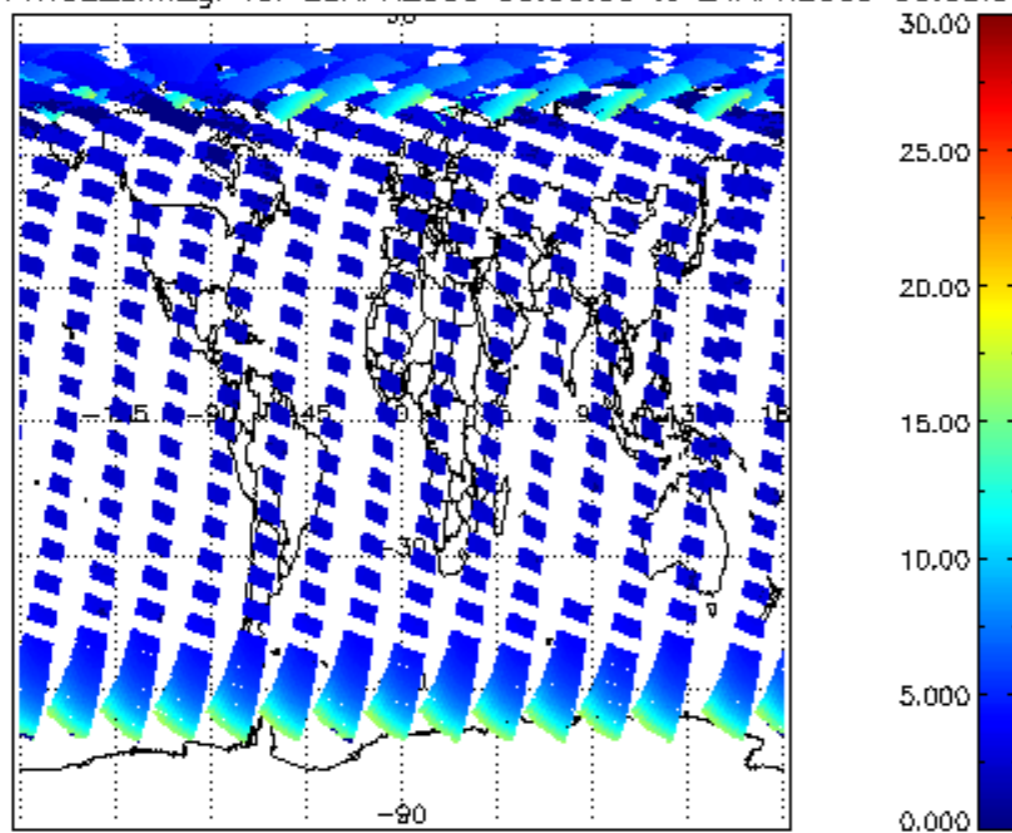
iCIOL2P_NADUV1NO2_amf_gr for 23APR2009 00:00:00 to 24APR2009 00:00:00
