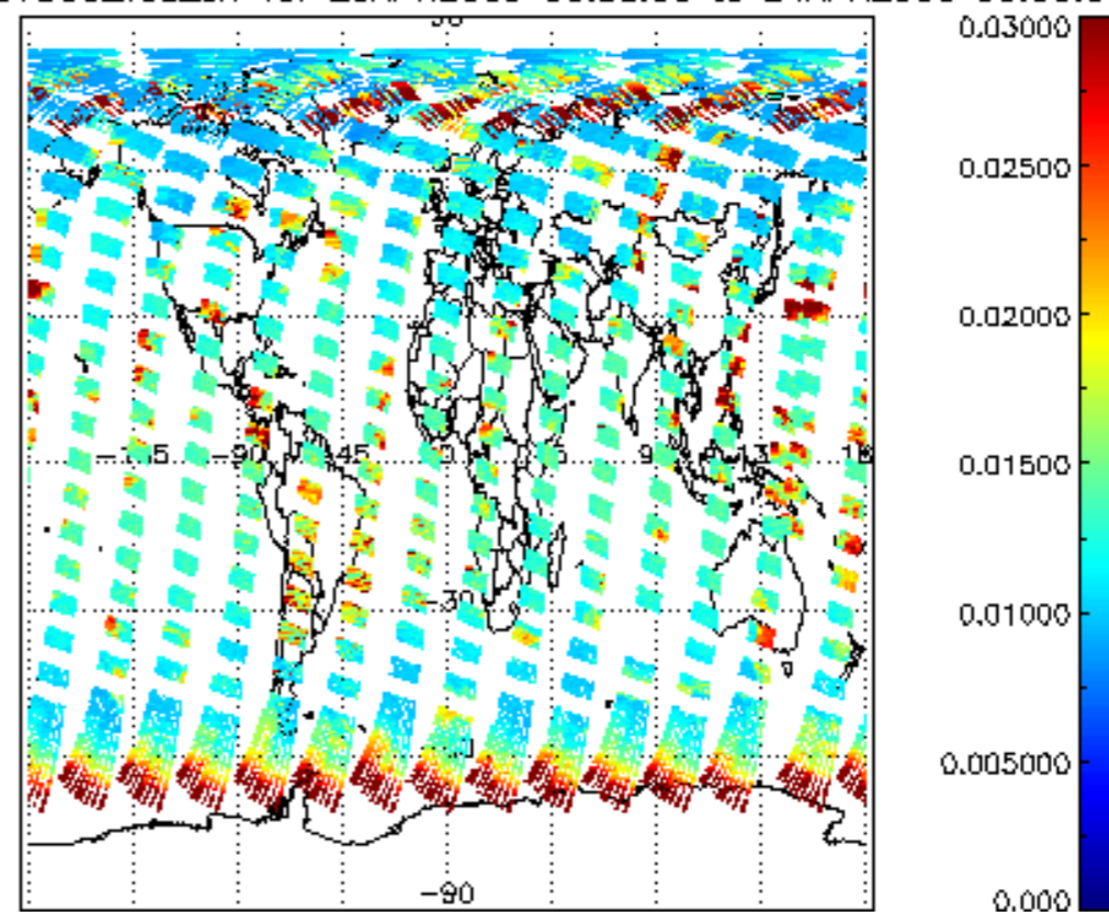
SCIOL2P_NADUV003_vcd_err for 23APR2009 00:00:00 to 24APR2009 00:00:00
