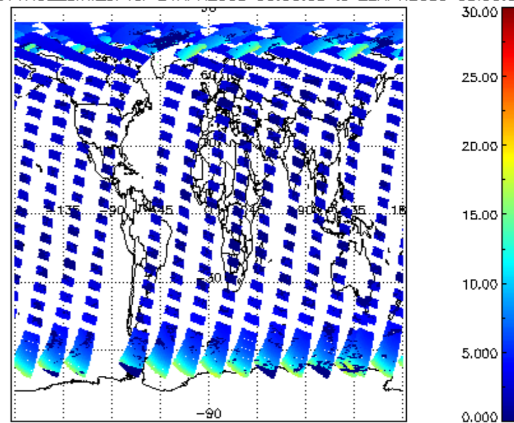
iCIOL2P_NADUV1NO2_amf_cl for 21APR2009 00:00:00 to 22APR2009 00:00:00
