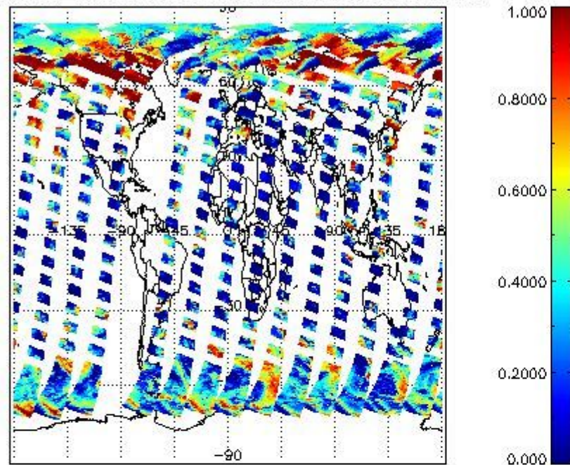
cL_frac for 21APR2009 00:00:00 to 22APR2009 00:00:00
