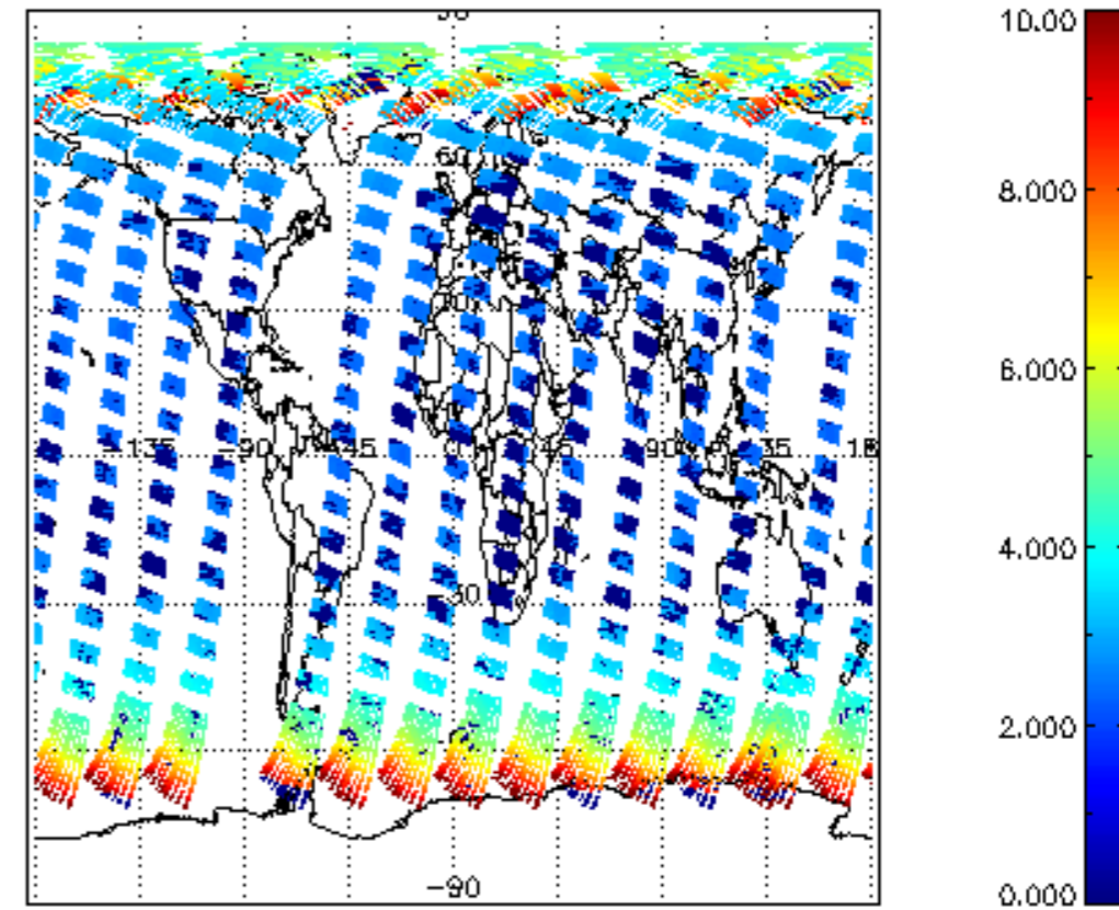
SCIOL2P_NADUV003_amf_cl for 21APR2009 00:00:00 to 22APR2009 00:00:00
