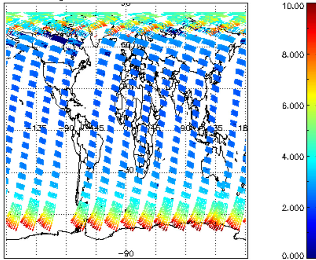
SCIOL2P_NADUV003_amf_gr for 21APR2009 00:00:00 to 22APR2009 00:00:00
