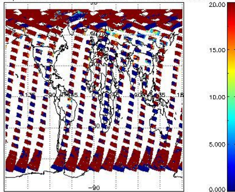
cL_opt_depth for 21APR2009 00:00:00 to 22APR2009 00:00:00
