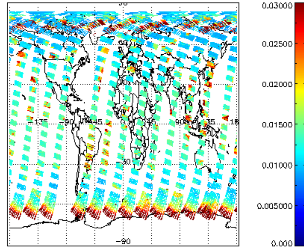
SCIOL2P_NADUV003_vcd_err for 21APR2009 00:00:00 to 22APR2009 00:00:00
