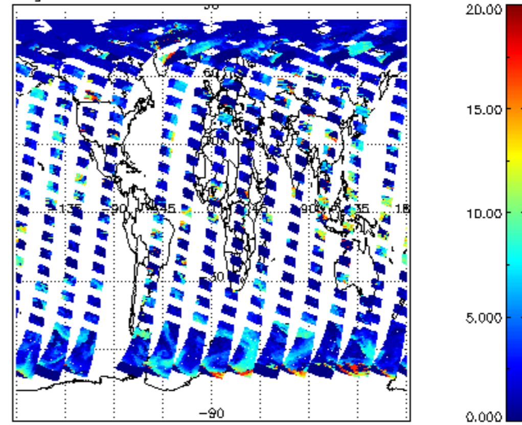
cl_top_height for 21APR2009 00:00:00 to 22APR2009 00:00:00
