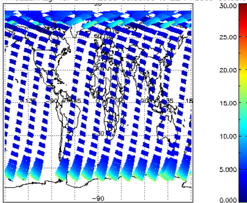
iCIOL2P_NADUV1NO2_amf_gr for 21APR2009 00:00:00 to 22APR2009 00:00:00
