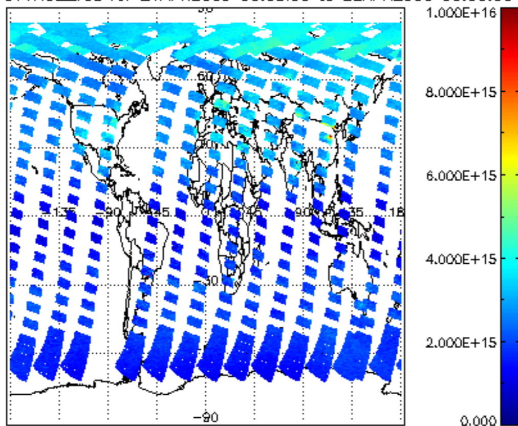
SCIOL2P_NADUV1NO2_vcd for 21APR2009 00:00:00 to 22APR2009 00:00:00
