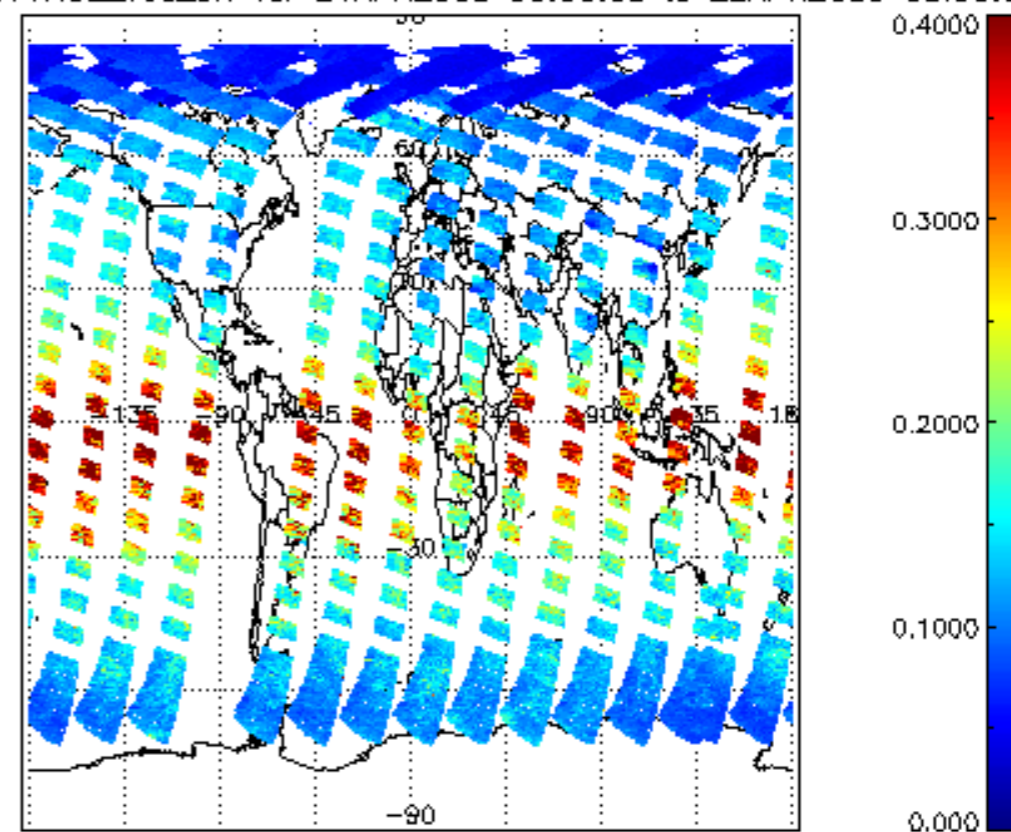
iCIOL2P_NADUV1NO2_vcd_err for 21APR2009 00:00:00 to 22APR2009 00:00:00
