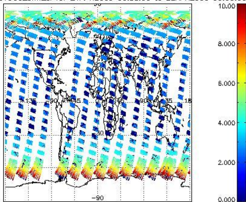
SCIOL2P_NADUV003_amf_cl for 21APR2009 00:00:00 to 22APR2009 00:00:00
