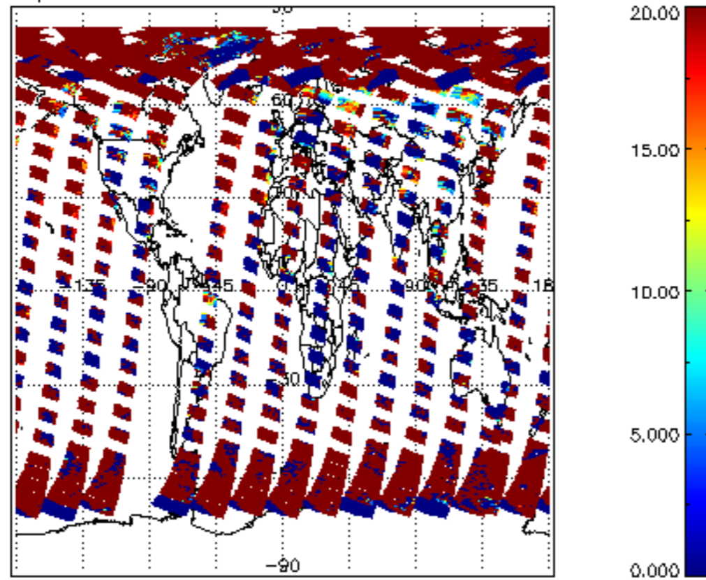
cl_opt_depth for 21APR2009 00:00:00 to 22APR2009 00:00:00
