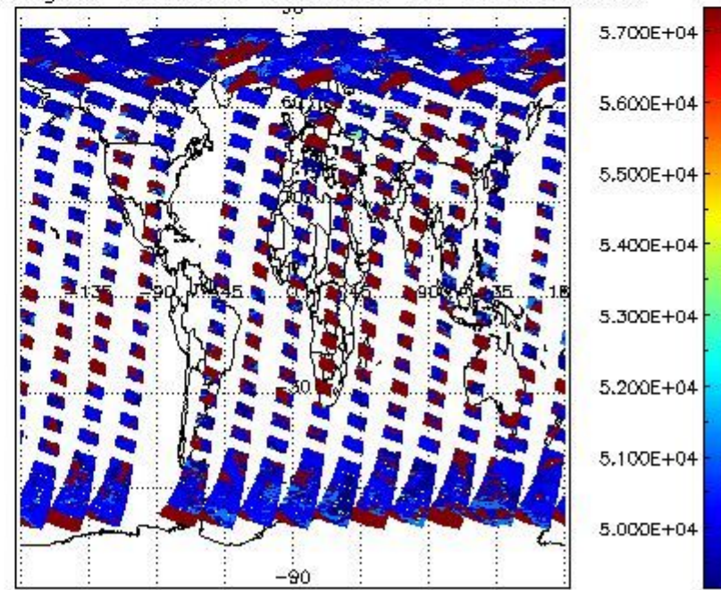
cloud_flags for 21APR2009 00:00:00 to 22APR2009 00:00:00
