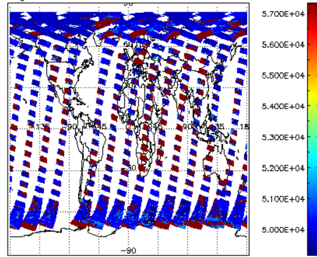
cloud_flags for 21APR2009 00:00:00 to 22APR2009 00:00:00
