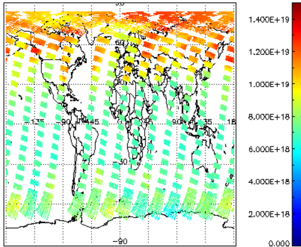
SCIOL2P_NADUV003_vcd for 21APR2009 00:00:00 to 22APR2009 00:00:00
