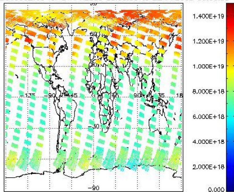
SCIOL2P_NADUV003_vcd for 21APR2009 00:00:00 to 22APR2009 00:00:00
