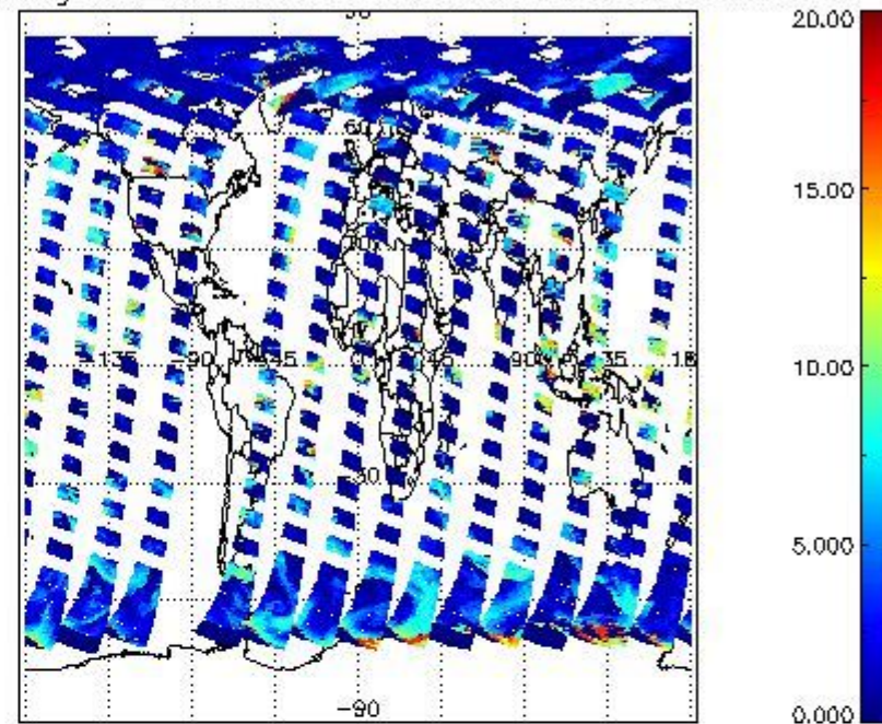
cL_top_height for 21APR2009 00:00:00 to 22APR2009 00:00:00
