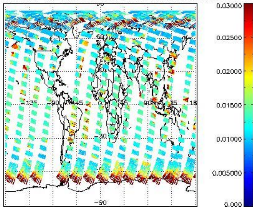
SCIOL2P_NADUV003_vcd_err for 21APR2009 00:00:00 to 22APR2009 00:00:00
