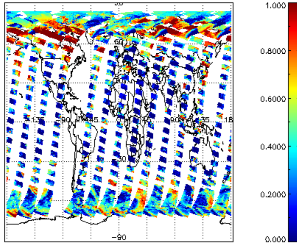
cl_frac for 21APR2009 00:00:00 to 22APR2009 00:00:00
