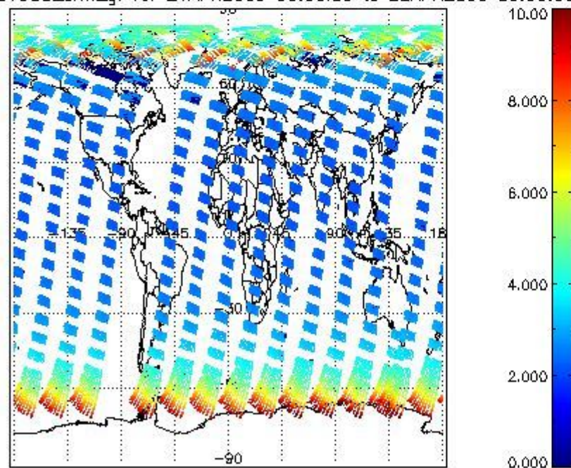
SCIOL2P_NADUV003_amf_gr for 21APR2009 00:00:00 to 22APR2009 00:00:00
