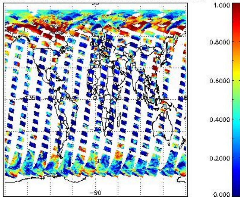
cL_frac for 19APR2009 00:00:00 to 20APR2009 00:00:00
