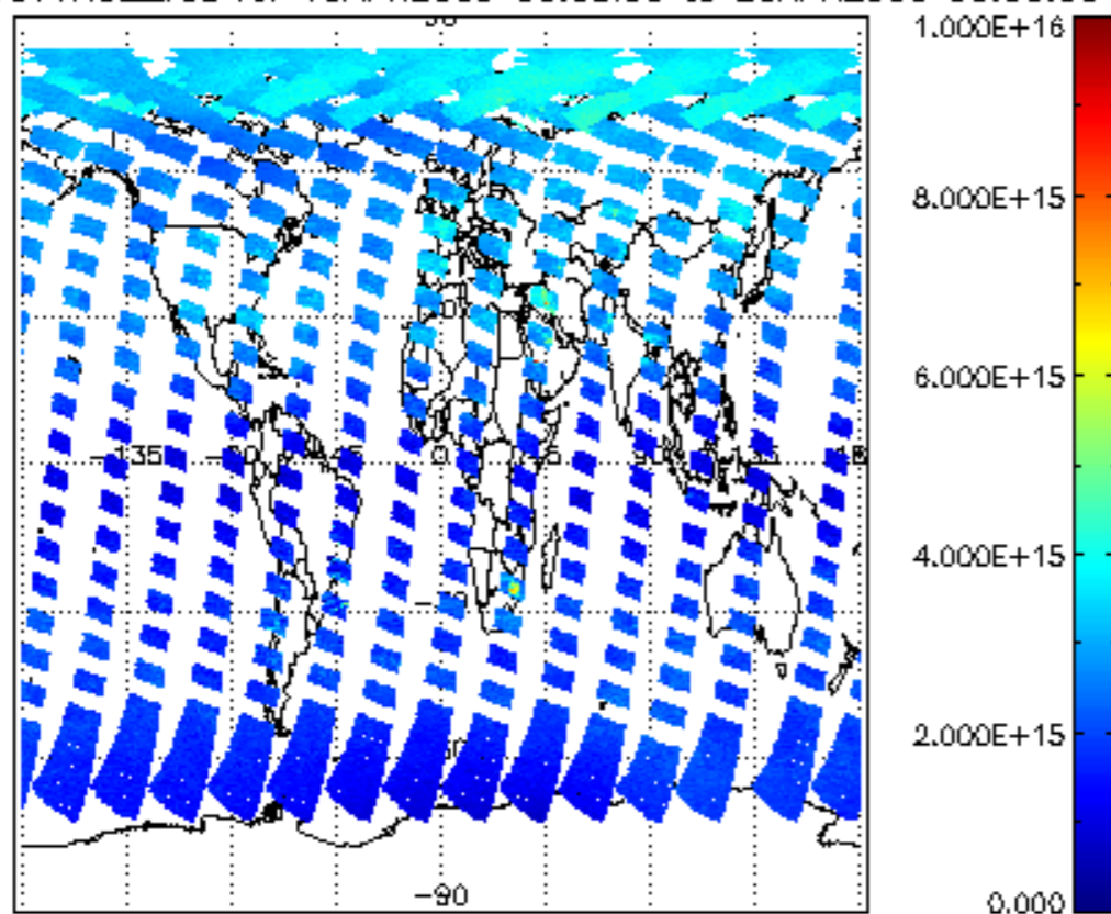
SCIOL2P_NADUV1NO2_vcd for 19APR2009 00:00:00 to 20APR2009 00:00:00
