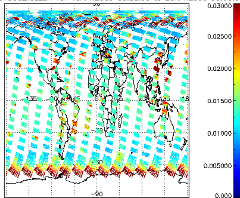
SCIOL2P_NADUV003_vcd_err for 19APR2009 00:00:00 to 20APR2009 00:00:00
