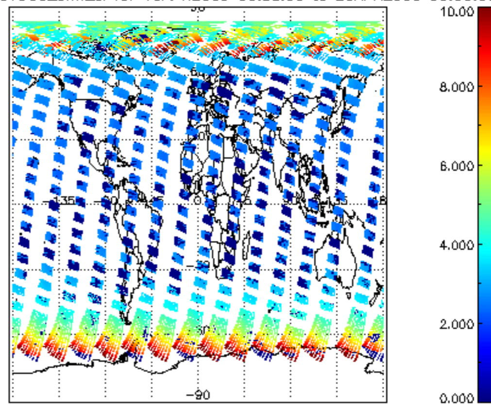
SCIOL2P_NADUV003_amf_cl for 19APR2009 00:00:00 to 20APR2009 00:00:00
