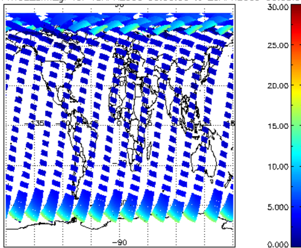
iCIOL2P_NADUV1NO2_amf_gr for 19APR2009 00:00:00 to 20APR2009 00:00:00
