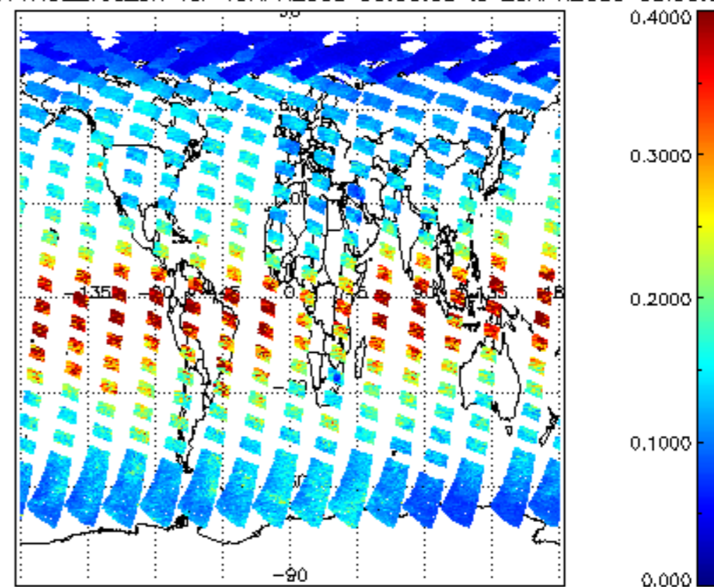
iCIOL2P_NADUV1NO2_vcd_err for 19APR2009 00:00:00 to 20APR2009 00:00:00
