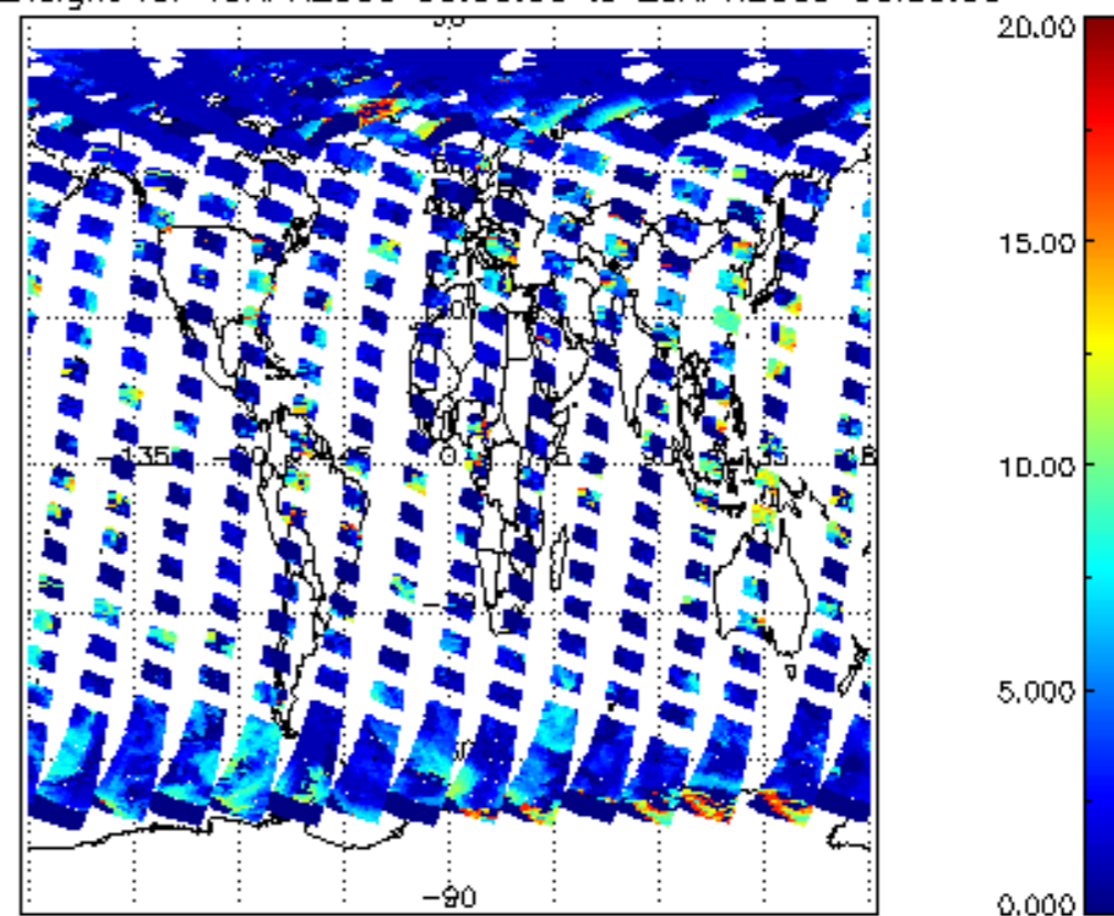
cl_top_height for 19APR2009 00:00:00 to 20APR2009 00:00:00
