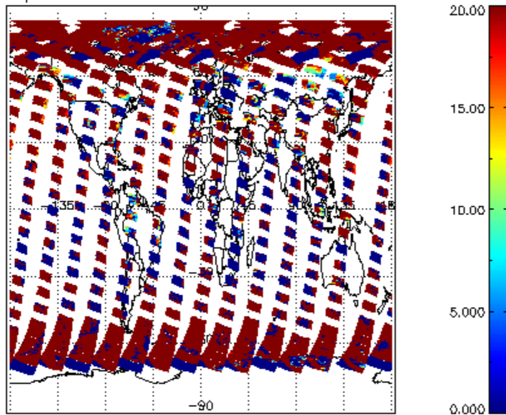
cl_opt_depth for 19APR2009 00:00:00 to 20APR2009 00:00:00
