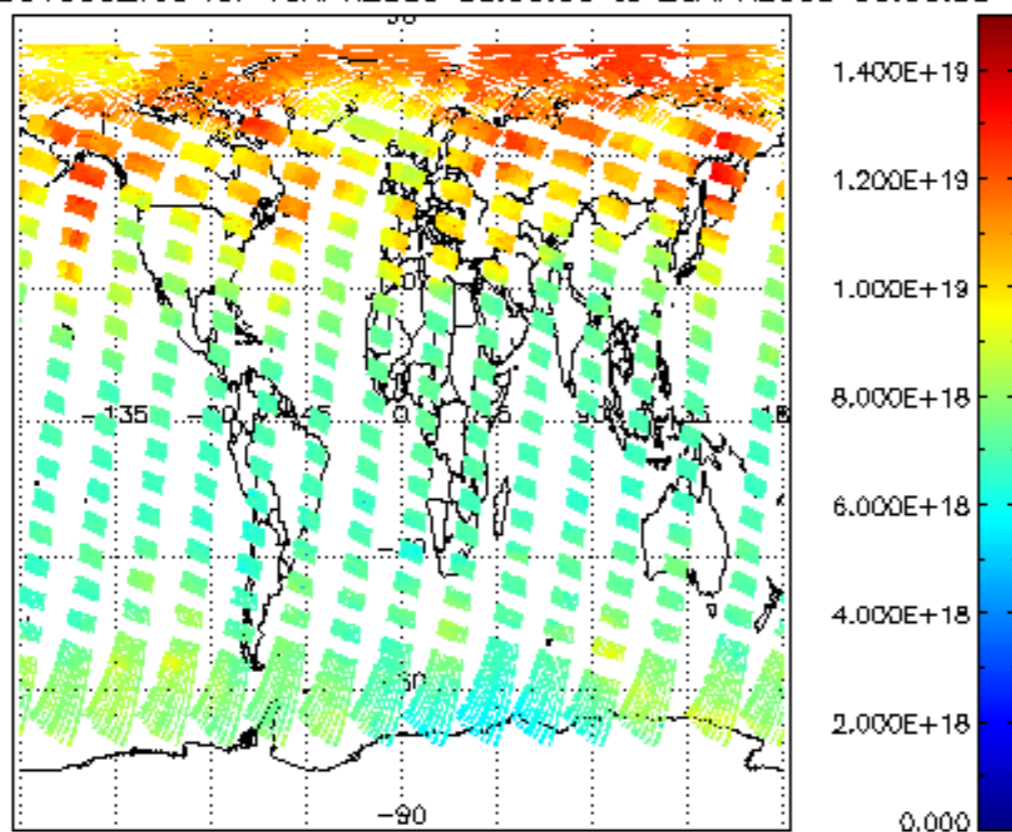
SCIOL2P_NADUV003_vcd for 19APR2009 00:00:00 to 20APR2009 00:00:00
