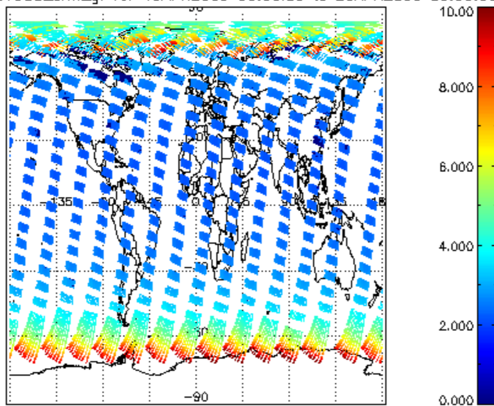
SCIOL2P_NADUV003_amf_gr for 19APR2009 00:00:00 to 20APR2009 00:00:00
