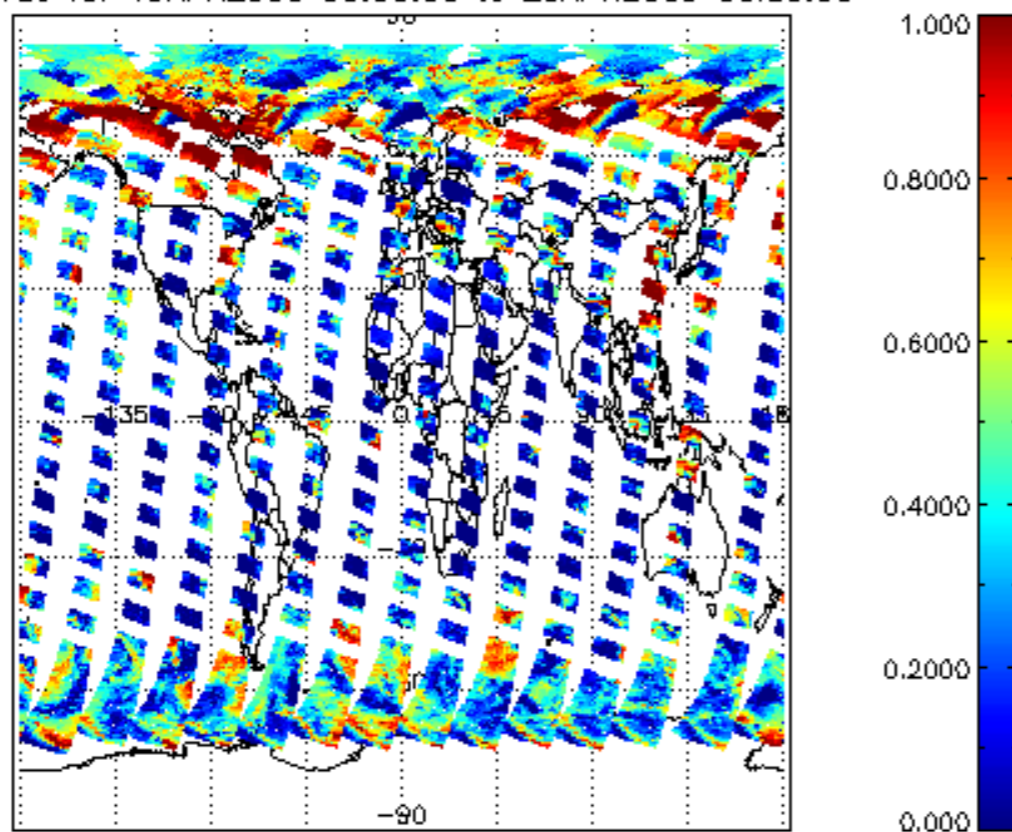
cl_frac for 19APR2009 00:00:00 to 20APR2009 00:00:00
