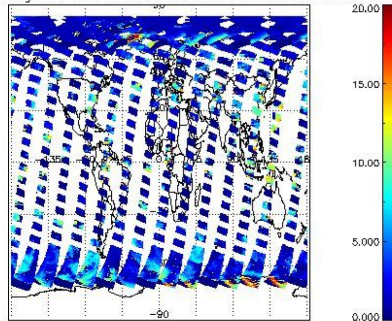
cL_top_height for 19APR2009 00:00:00 to 20APR2009 00:00:00
