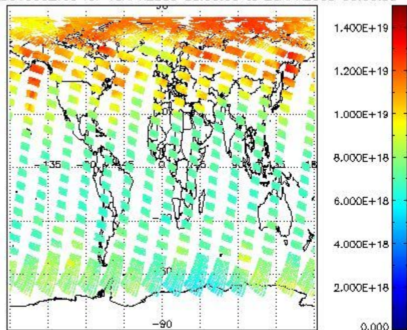
SCIOL2P_NADUV003_vcd for 19APR2009 00:00:00 to 20APR2009 00:00:00
