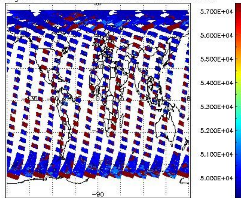
cloud_flags for 19APR2009 00:00:00 to 20APR2009 00:00:00
