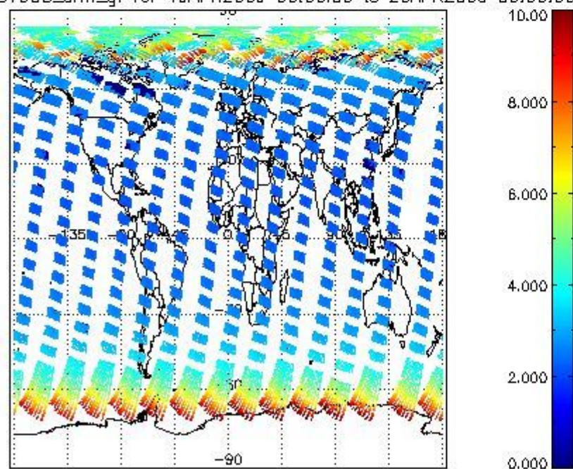
SCIOL2P_NADUV003_amf_gr for 19APR2009 00:00:00 to 20APR2009 00:00:00
