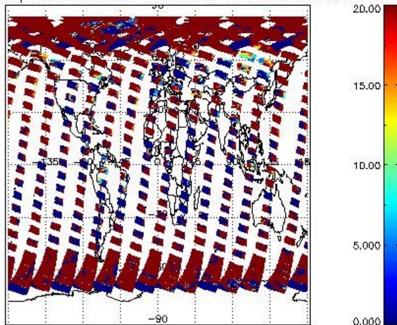
cL_opt_depth for 19APR2009 00:00:00 to 20APR2009 00:00:00
