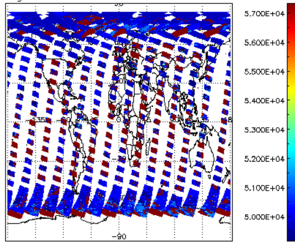
cloud_flags for 19APR2009 00:00:00 to 20APR2009 00:00:00
