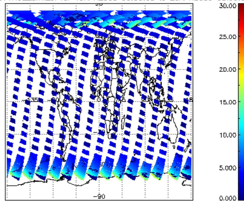
iCIOL2P_NADUV1NO2_amf_cl for 19APR2009 00:00:00 to 20APR2009 00:00:00
