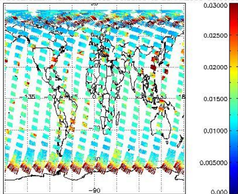
SCIOL2P_NADUV003_vcd_err for 19APR2009 00:00:00 to 20APR2009 00:00:00
