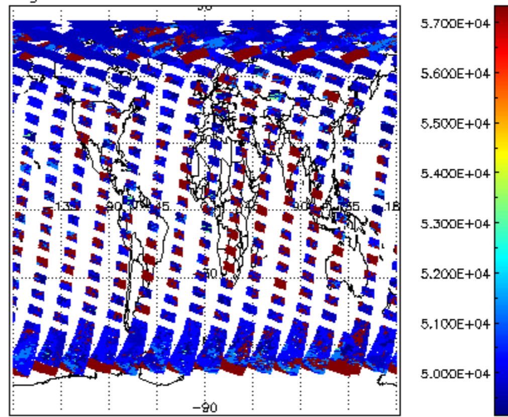
cloud_flags for 18APR2009 00:00:00 to 19APR2009 00:00:00
