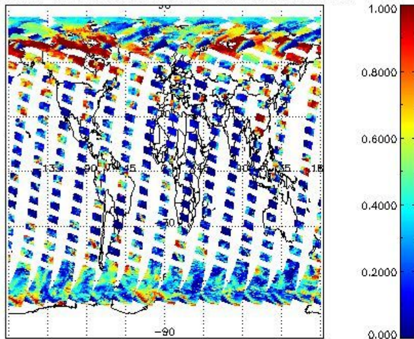
cL_frac for 18APR2009 00:00:00 to 19APR2009 00:00:00
