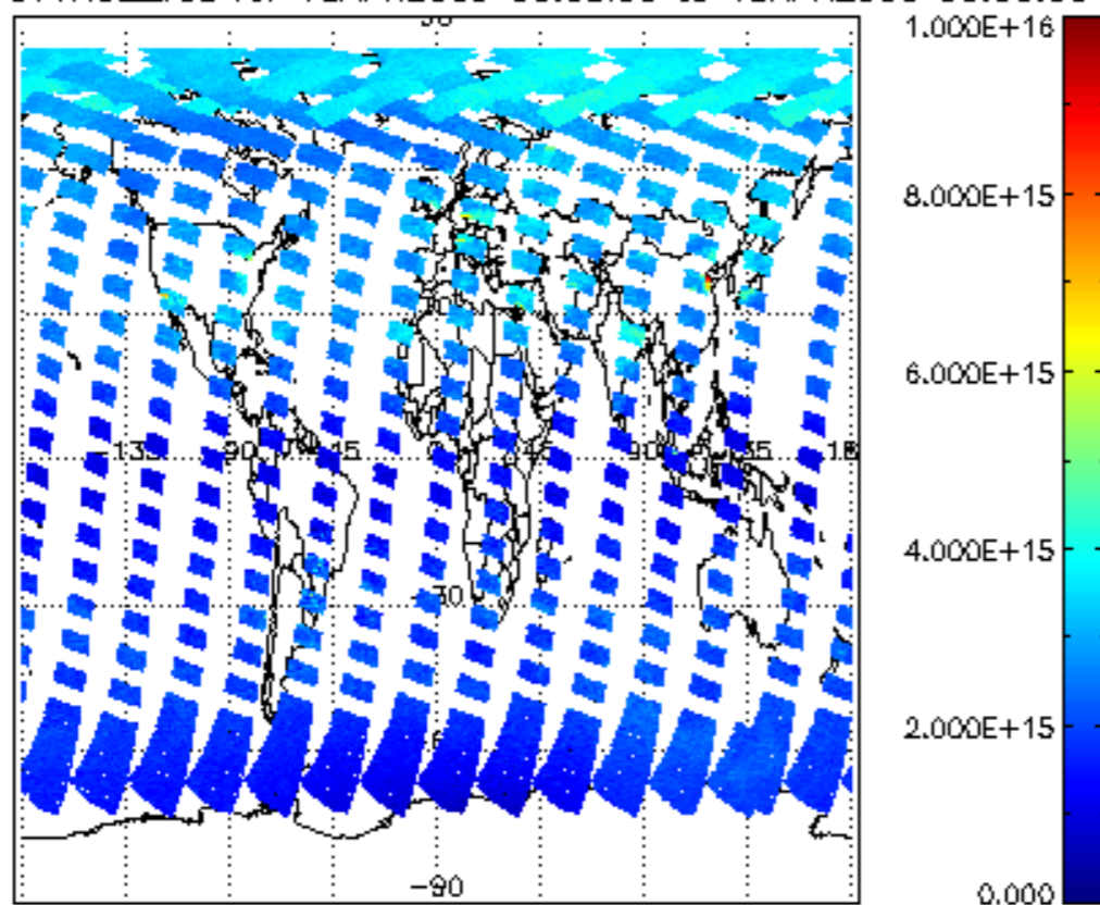
SCIOL2P_NADUV1NO2_vcd for 18APR2009 00:00:00 to 19APR2009 00:00:00
