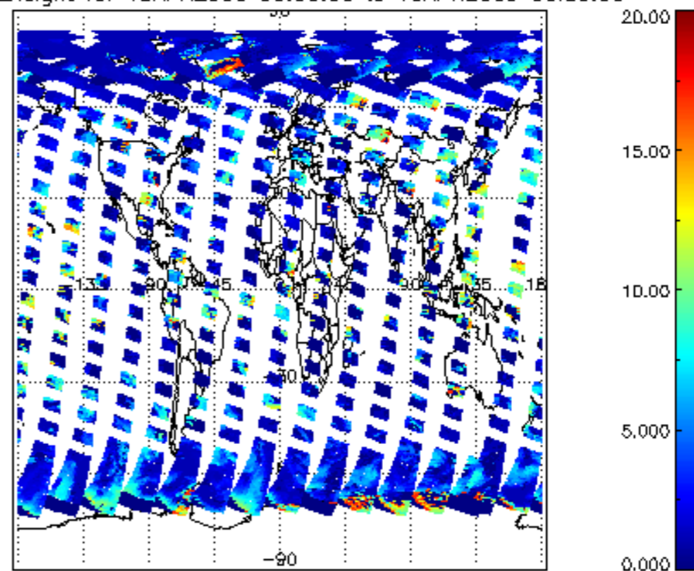
cl_top_height for 18APR2009 00:00:00 to 19APR2009 00:00:00
