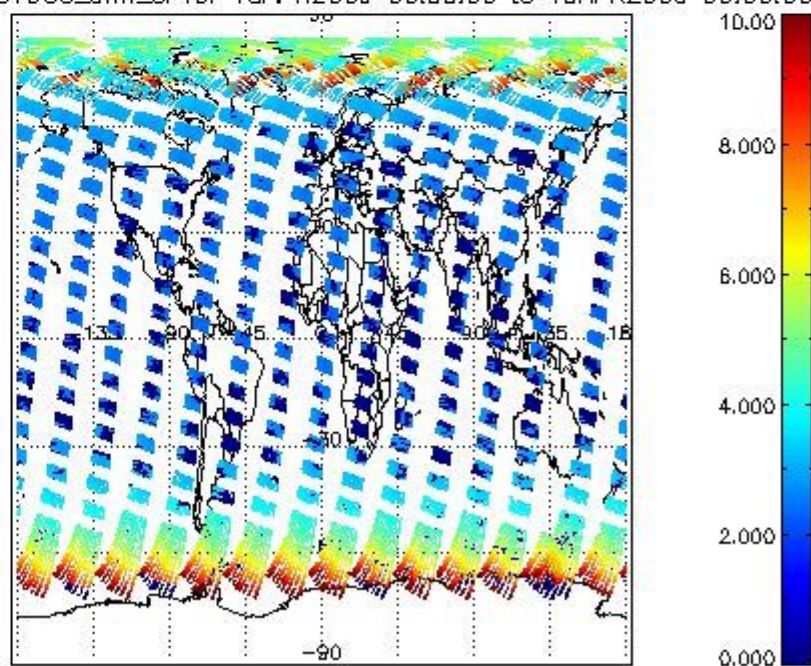
SCIOL2P_NADUV003_amf_cl for 18APR2009 00:00:00 to 19APR2009 00:00:00
