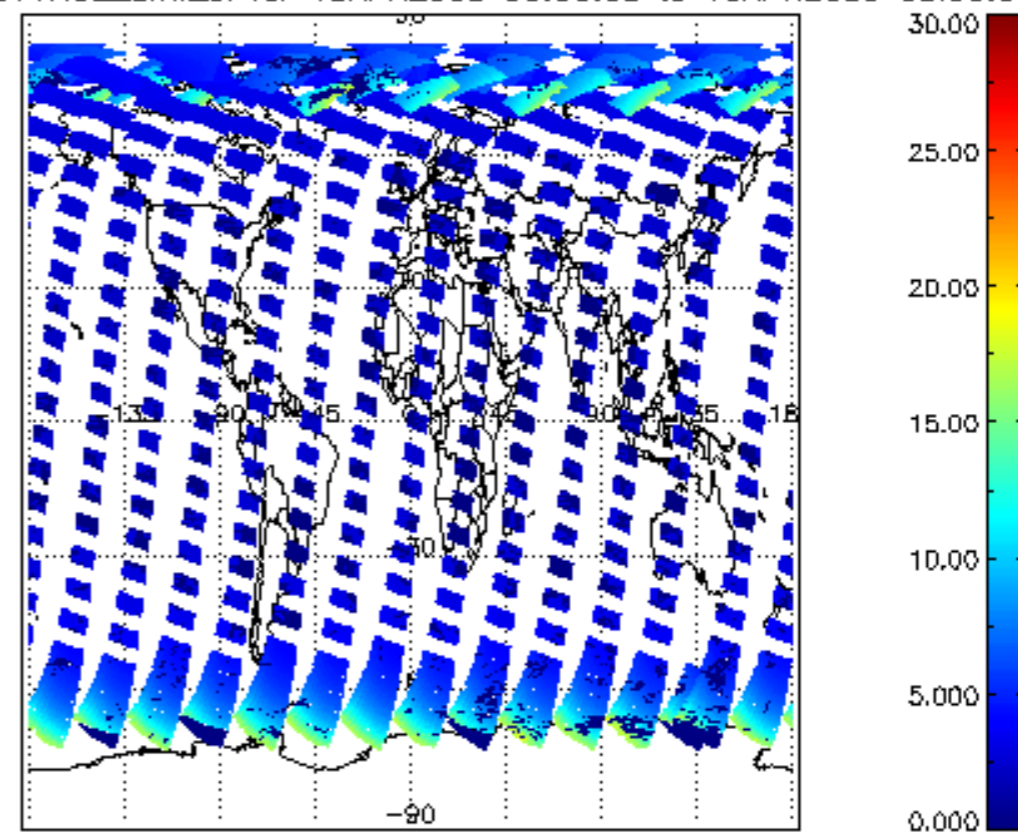
iCIOL2P_NADUV1NO2_amf_cl for 18APR2009 00:00:00 to 19APR2009 00:00:00
