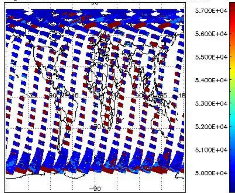
cloud_flags for 18APR2009 00:00:00 to 19APR2009 00:00:00
