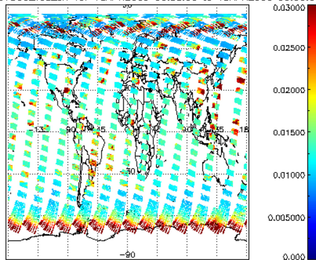
SCIOL2P_NADUV003_vcd_err for 18APR2009 00:00:00 to 19APR2009 00:00:00
