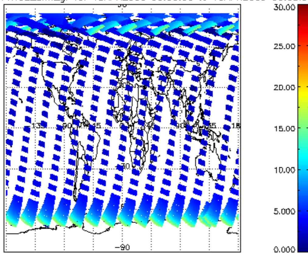
iCIOL2P_NADUV1NO2_amf_gr for 18APR2009 00:00:00 to 19APR2009 00:00:00
