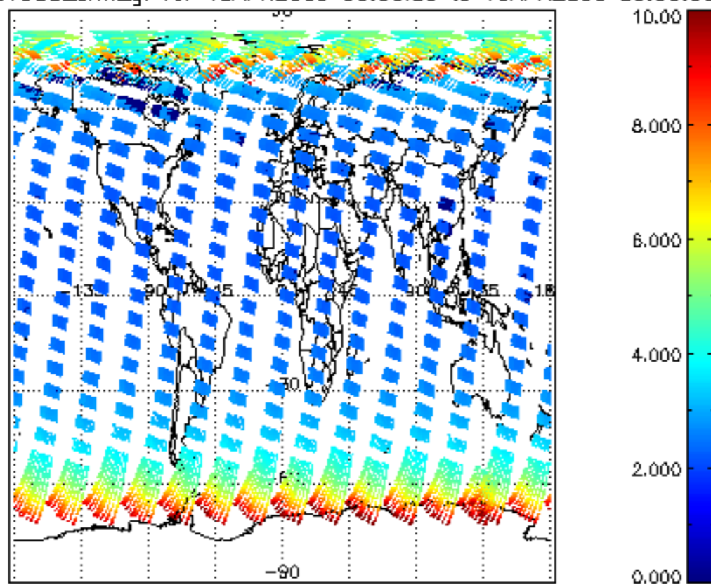
SCIOL2P_NADUV003_amf_gr for 18APR2009 00:00:00 to 19APR2009 00:00:00
