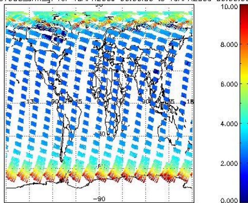
SCIOL2P_NADUV003_amf_gr for 18APR2009 00:00:00 to 19APR2009 00:00:00
