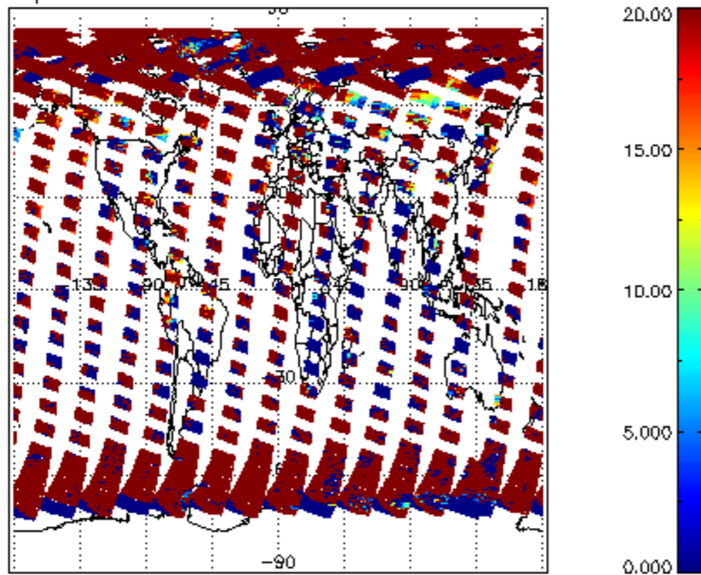
cl_opt_depth for 18APR2009 00:00:00 to 19APR2009 00:00:00
