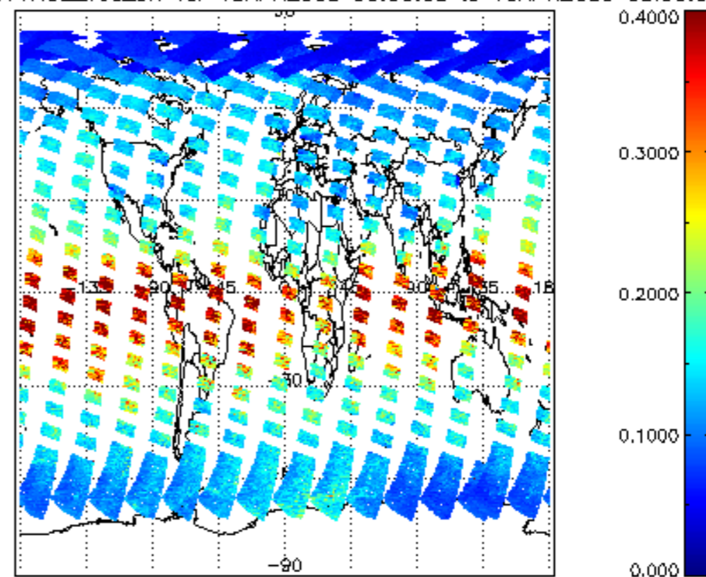
iCIOL2P_NADUV1NO2_vcd_err for 18APR2009 00:00:00 to 19APR2009 00:00:00
