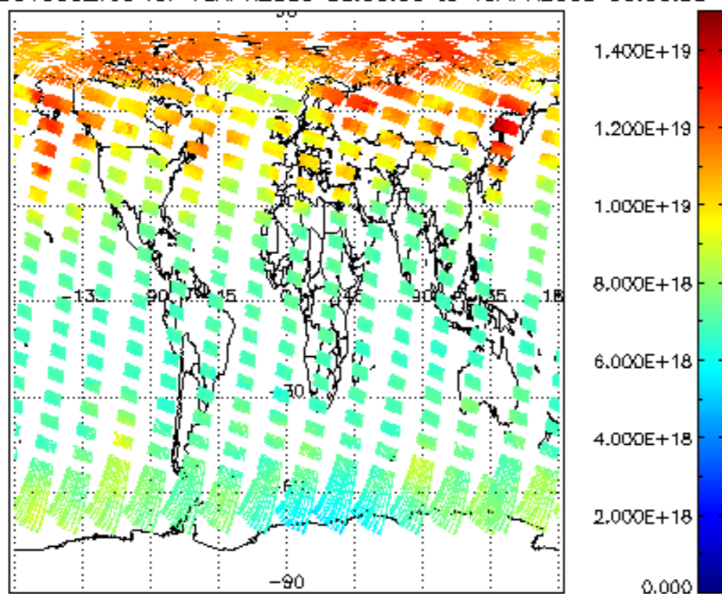
SCIOL2P_NADUV003_vcd for 18APR2009 00:00:00 to 19APR2009 00:00:00
