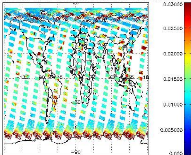
SCIOL2P_NADUV003_vcd_err for 18APR2009 00:00:00 to 19APR2009 00:00:00
