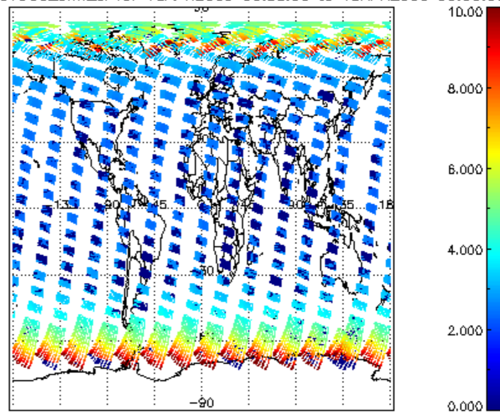
SCIOL2P_NADUV003_amf_cl for 18APR2009 00:00:00 to 19APR2009 00:00:00
