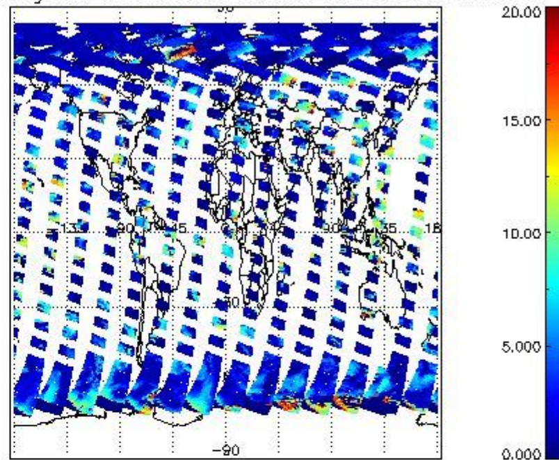
cL_top_height for 18APR2009 00:00:00 to 19APR2009 00:00:00
