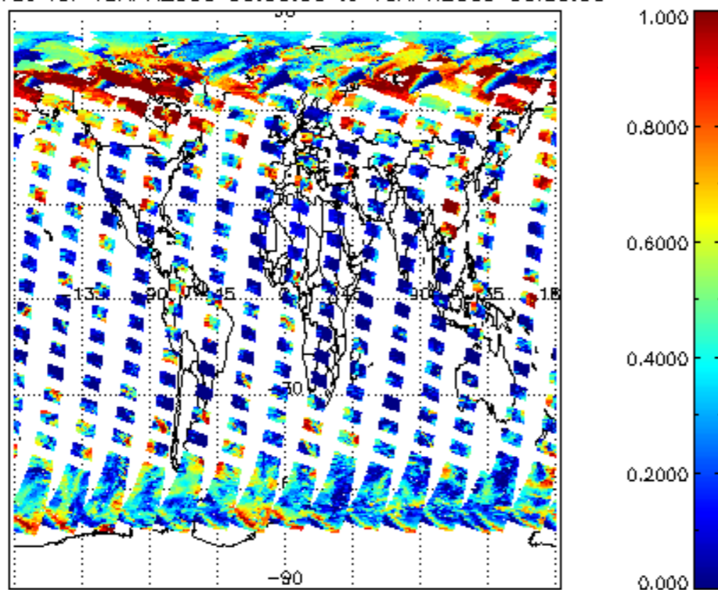
cl_frac for 18APR2009 00:00:00 to 19APR2009 00:00:00
