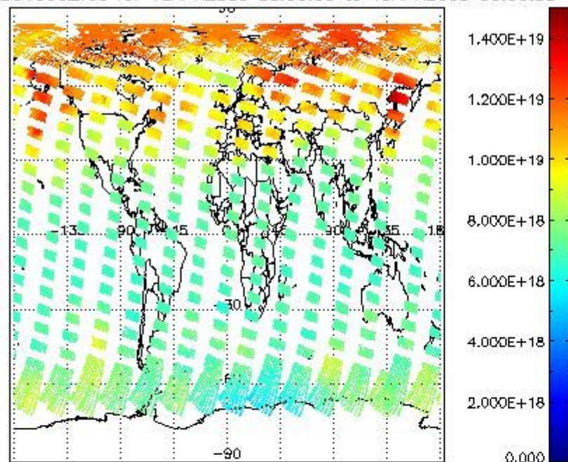
SCIOL2P_NADUV003_vcd for 18APR2009 00:00:00 to 19APR2009 00:00:00
