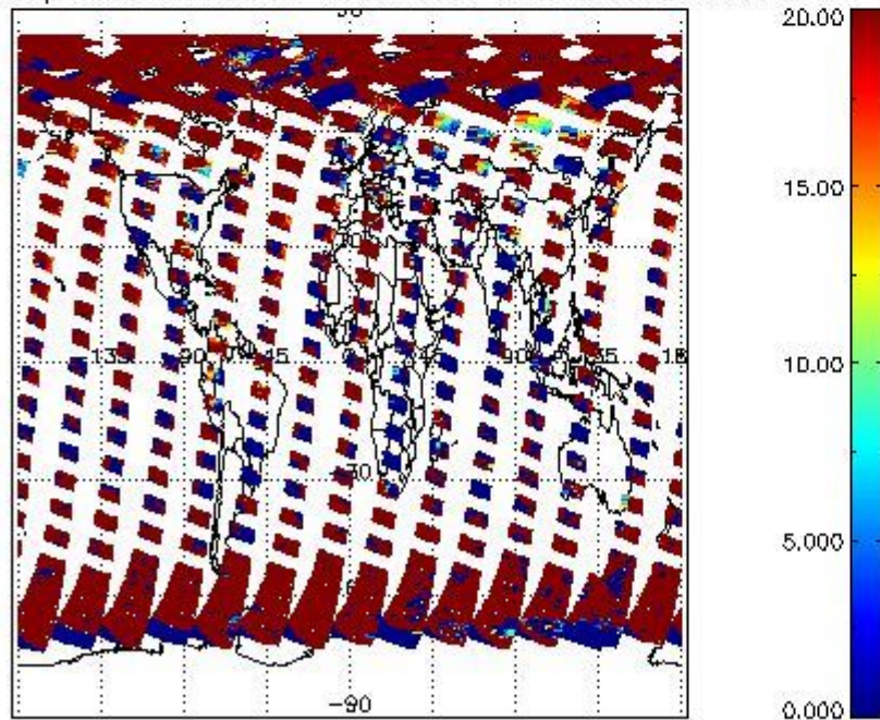
cL_opt_depth for 18APR2009 00:00:00 to 19APR2009 00:00:00
