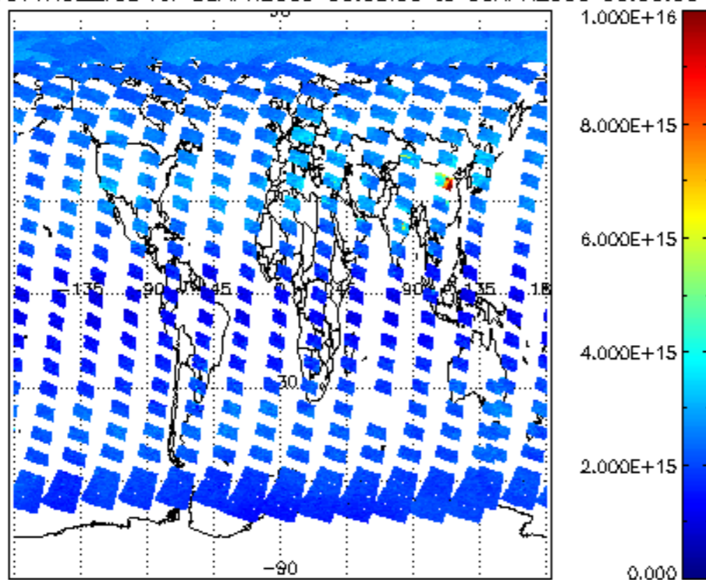
SCIOL2P_NADUV1NO2_vcd for 05APR2009 00:00:00 to 06APR2009 00:00:00
