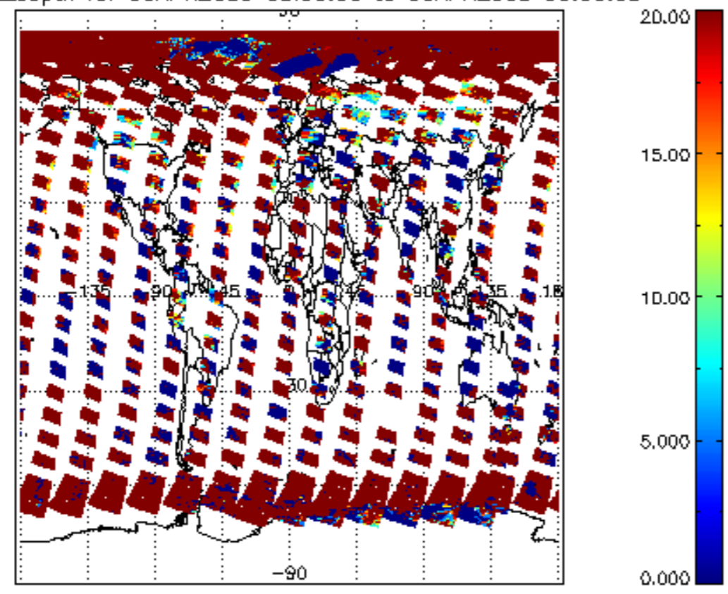
cl_opt_depth for 05APR2009 00:00:00 to 06APR2009 00:00:00
