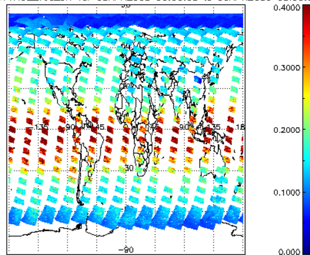
iCIOL2P_NADUV1NO2_vcd_err for 05APR2009 00:00:00 to 06APR2009 00:00:00
