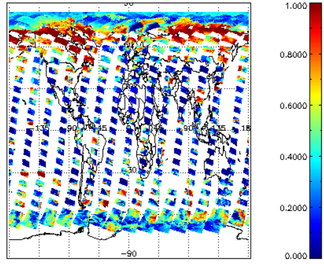
cl_frac for 05APR2009 00:00:00 to 06APR2009 00:00:00
