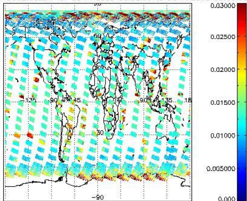
SCIOL2P_NADUV003_vcd for 05APR2009 00:00:00 to 06APR2009 00:00:00 SCIOL2P_NADUV003_vcd_err for 05APR2009 00:00:00 to 06APR2009 00:00:00
