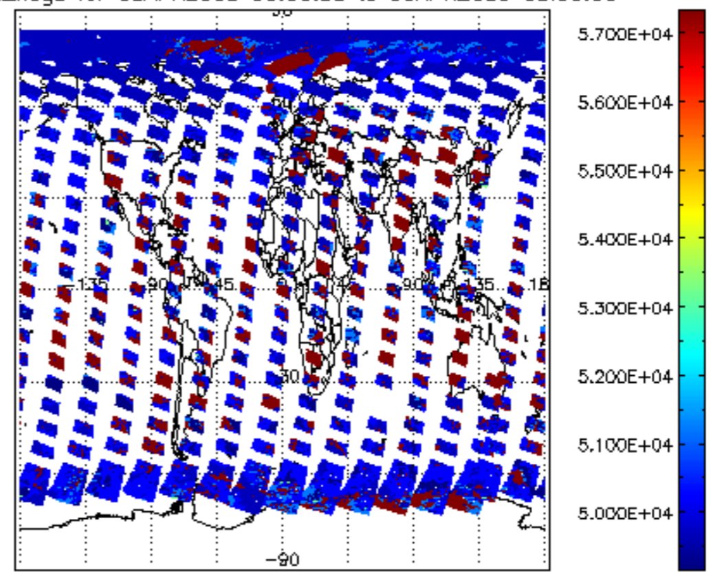
cloud_flags for 05APR2009 00:00:00 to 06APR2009 00:00:00
