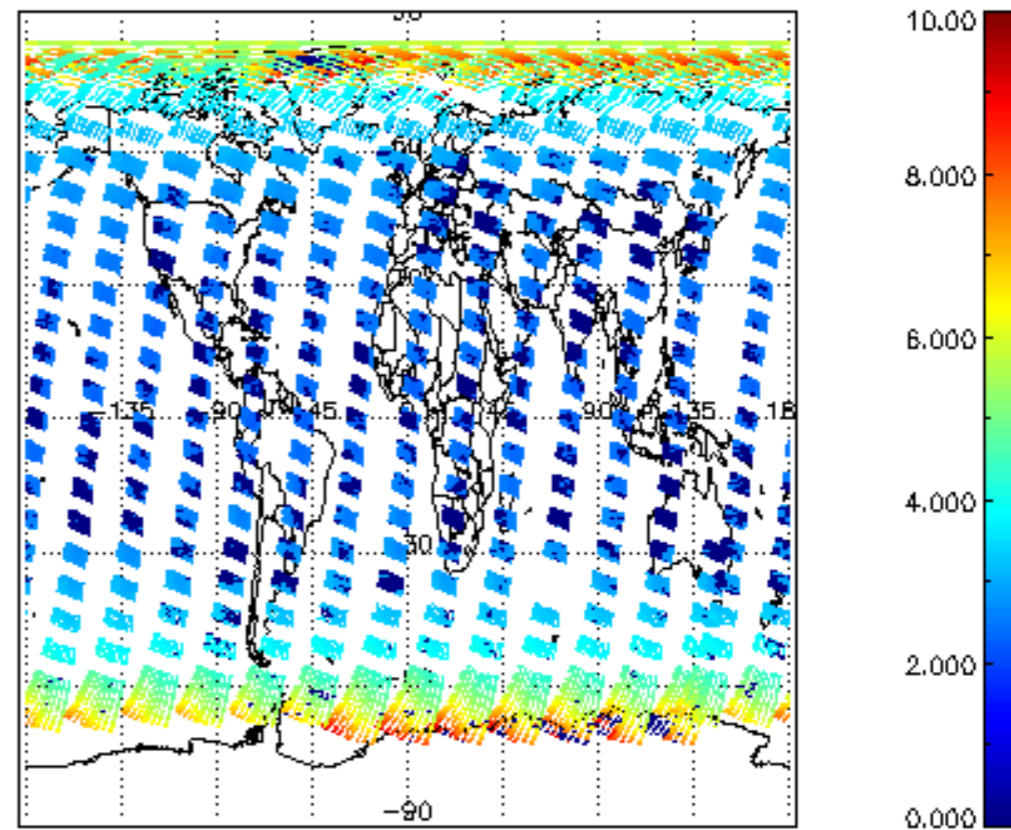
SCIOL2P_NADUV003_amf_cl for 05APR2009 00:00:00 to 06APR2009 00:00:00
