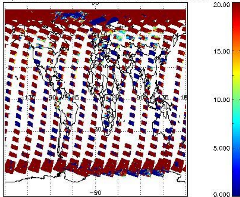
cLopt_depth for 05APR2009 00:00:00 to 06APR2009 00:00:00
