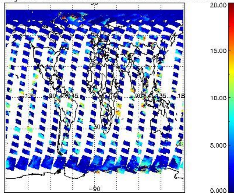
cL_top_height for 05APR2009 00:00:00 to 06APR2009 00:00:00
