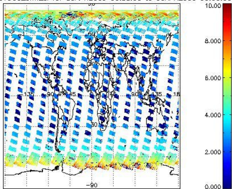
SCIOL2P_NADUV003_amf_gr for 05APR2009 00:00:00 to 06APR2009 00:00:00 SCIOL2P_NADUV003_amf_cl for 05APR2009 00:00:00 to 06APR2009 00:00:00
