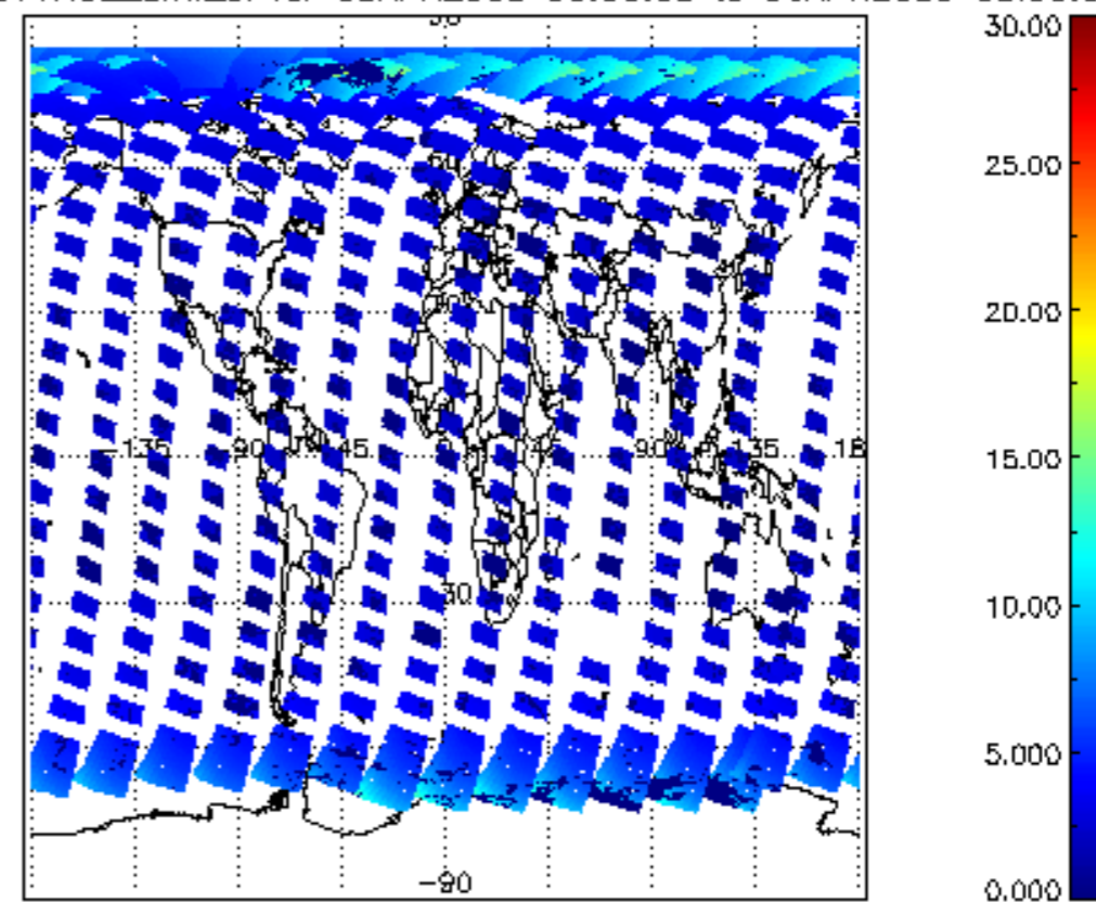
iCIOL2P_NADUV1NO2_amf_cl for 05APR2009 00:00:00 to 06APR2009 00:00:00
