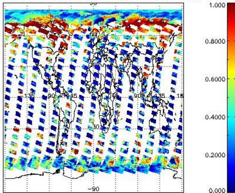
cLfrac for 05APR2009 00:00:00 to 06APR2009 00:00:00
