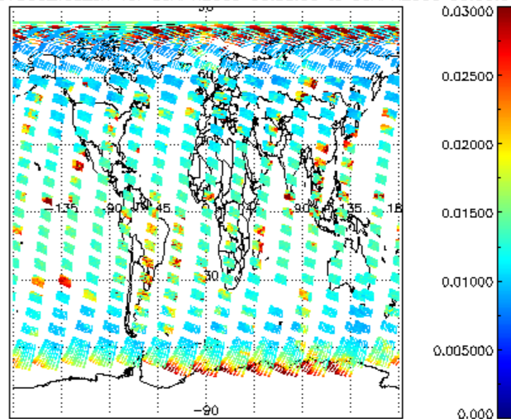
SCIOL2P_NADUV003_vcd_err for 05APR2009 00:00:00 to 06APR2009 00:00:00
