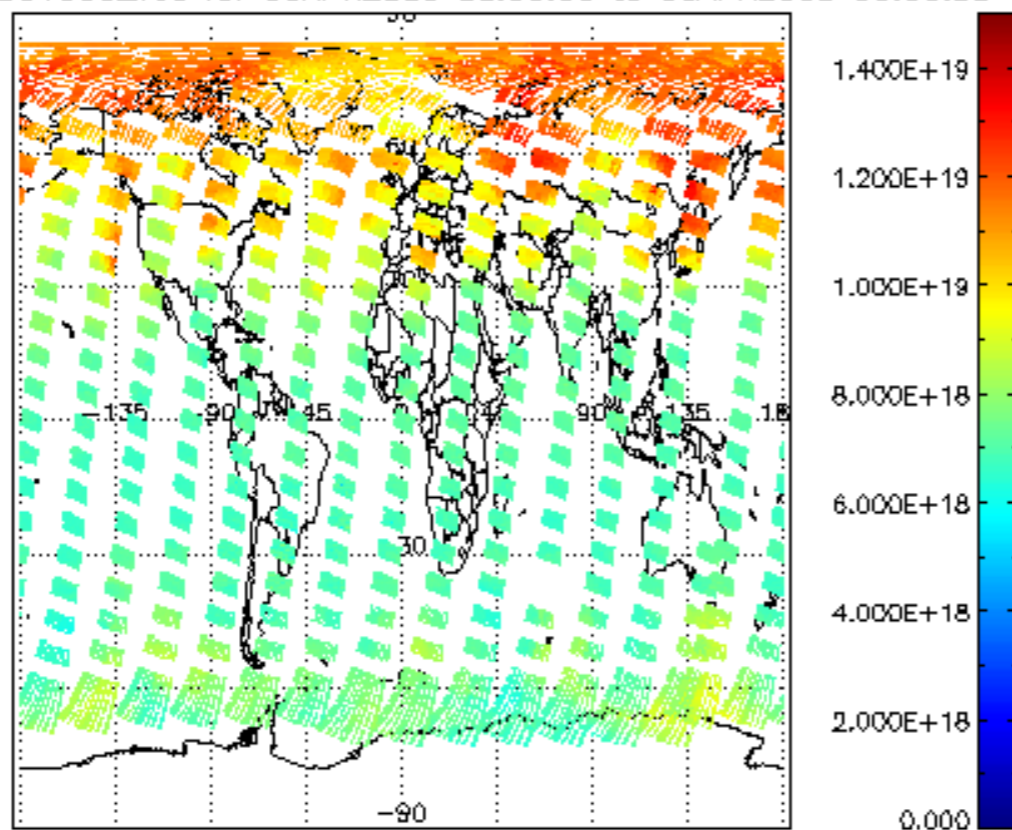
SCIOL2P_NADUV003_vcd for 05APR2009 00:00:00 to 06APR2009 00:00:00
