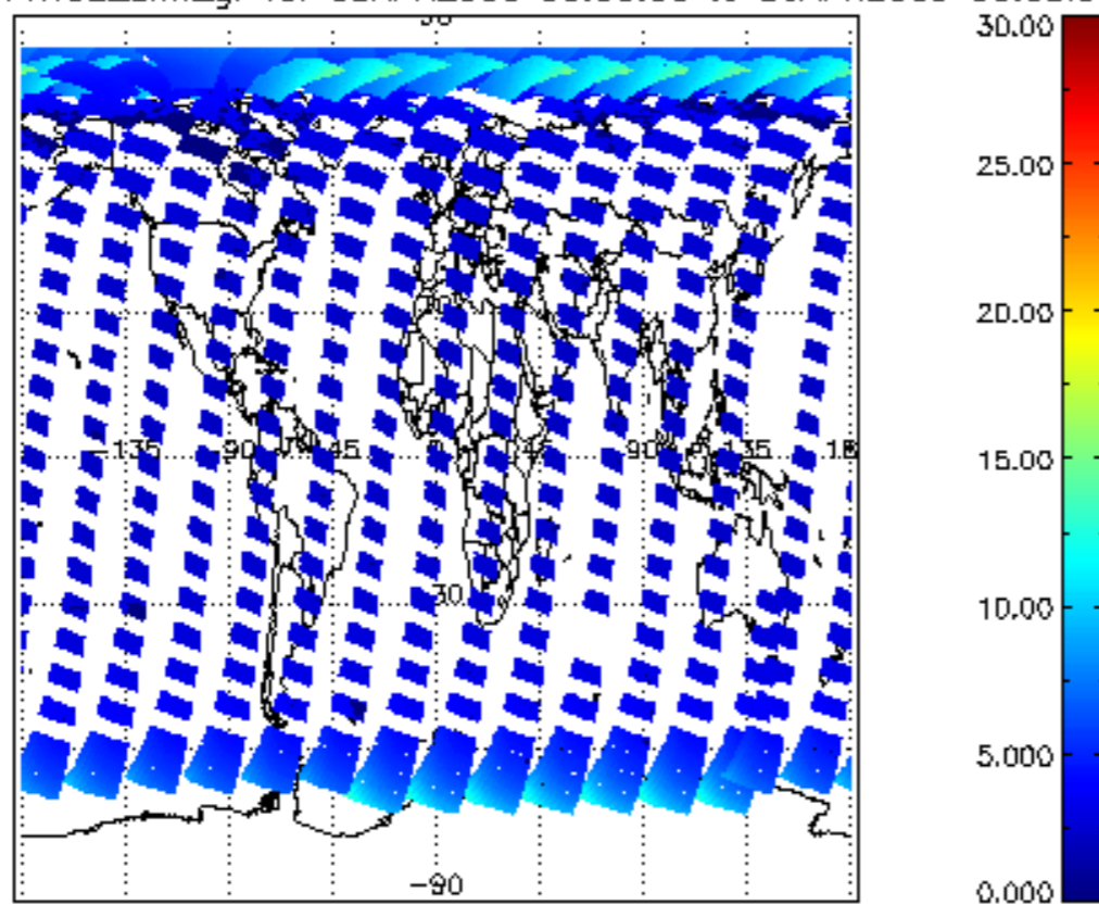
iCIOL2P_NADUV1NO2_amf_gr for 05APR2009 00:00:00 to 06APR2009 00:00:00
