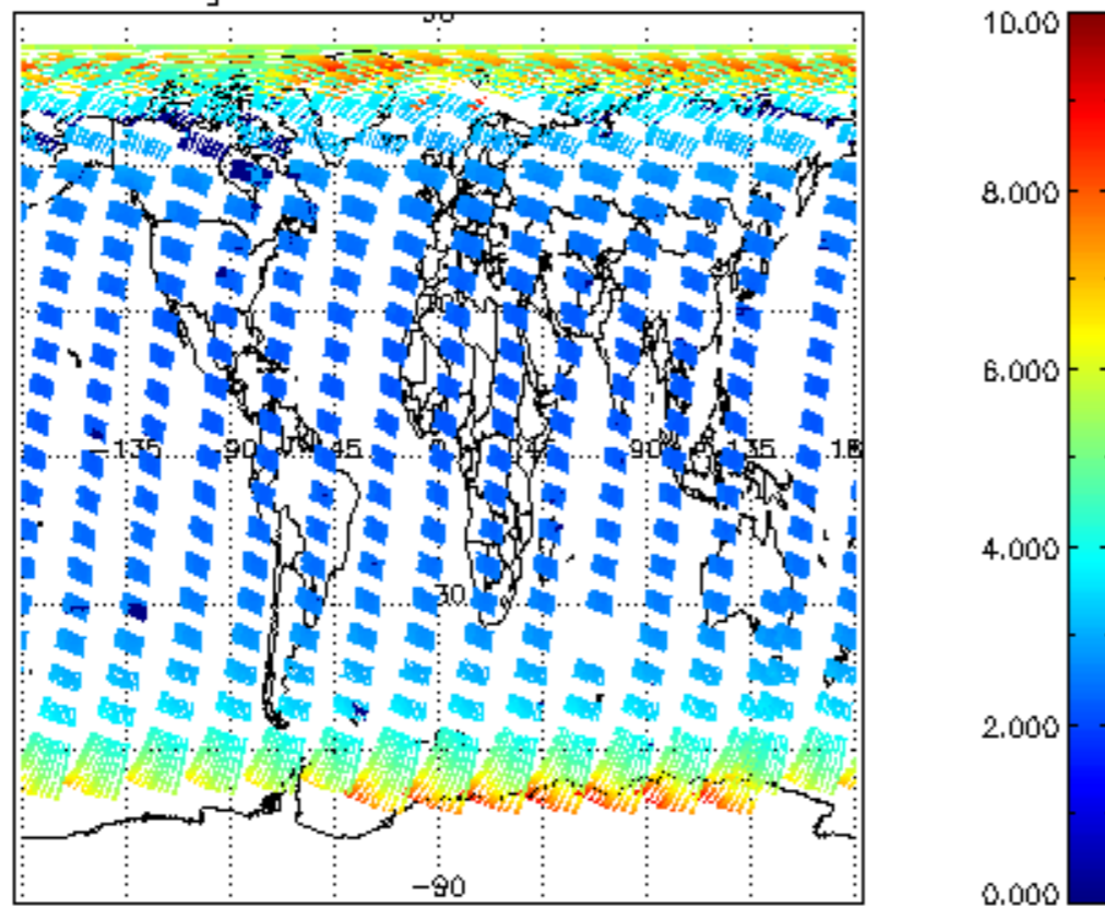
SCIOL2P_NADUV003_amf_gr for 05APR2009 00:00:00 to 06APR2009 00:00:00
