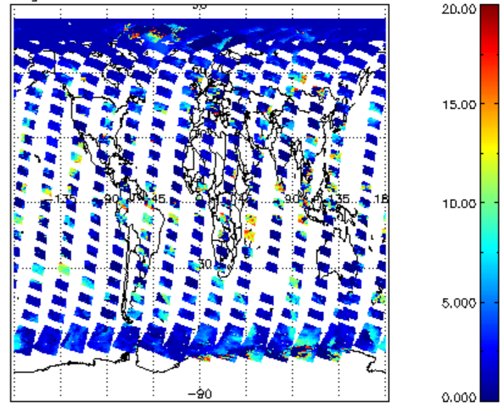
cl_top_height for 05APR2009 00:00:00 to 06APR2009 00:00:00
