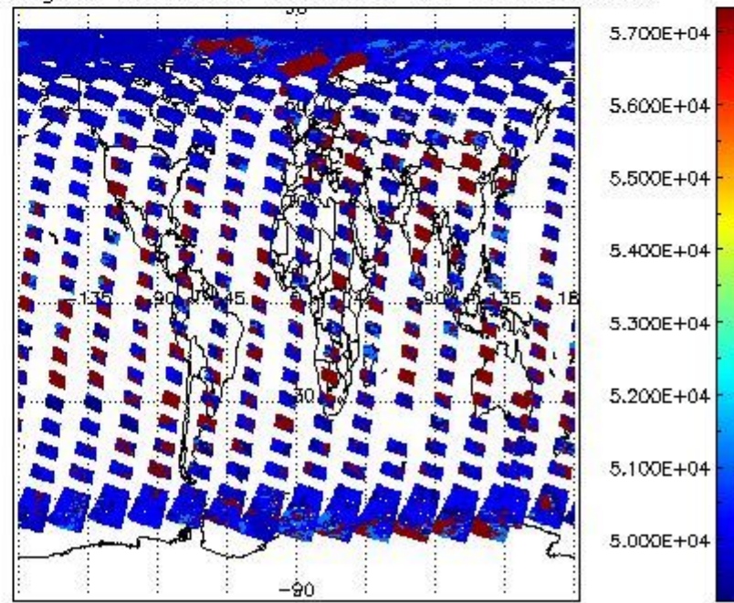
cloud_flags for 05APR2009 00:00:00 to 06APR2009 00:00:00
