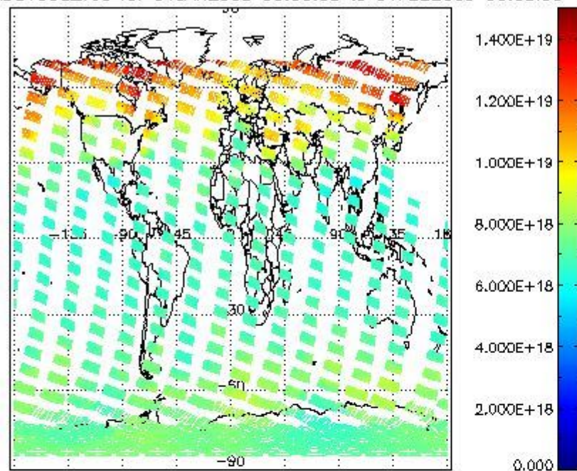
SCIOL2P_NADUV003_vcd for 31JAN2009 00:00:00 to 01FEB2009 00:00:00
