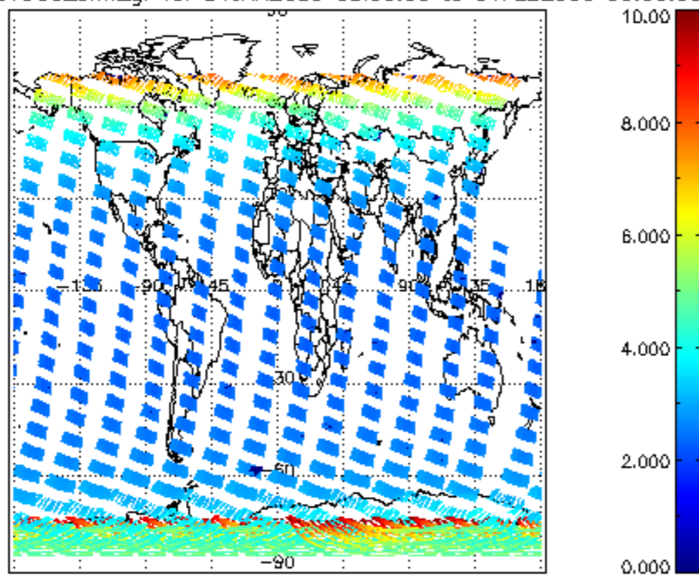
SCIOL2P_NADUV003_amf_gr for 31JAN2009 00:00:00 to 01FEB2009 00:00:00
