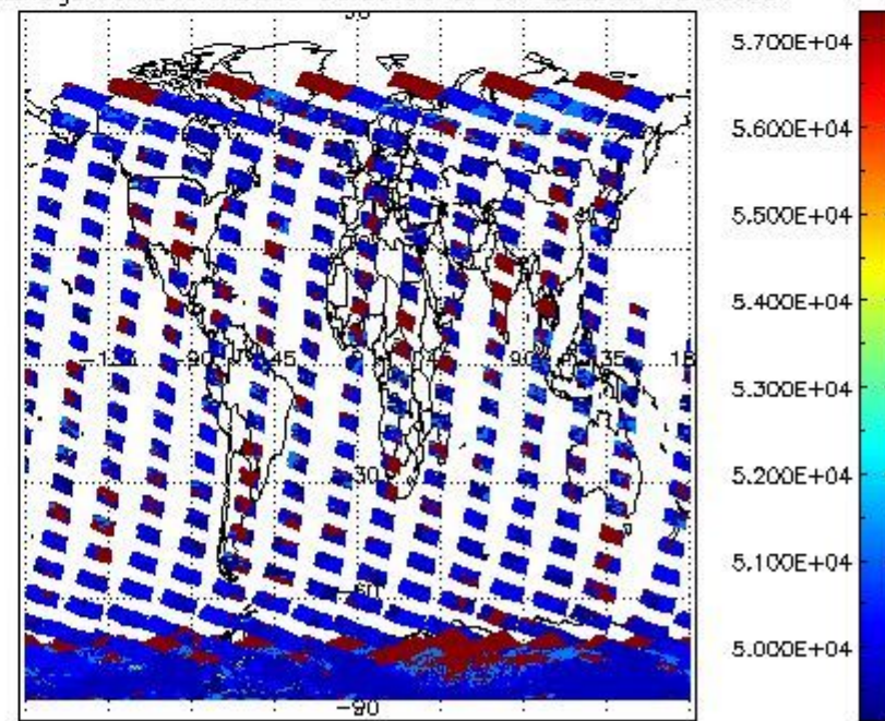
cloud_flags for 31JAN2009 00:00:00 to 01FEB2009 00:00:00
