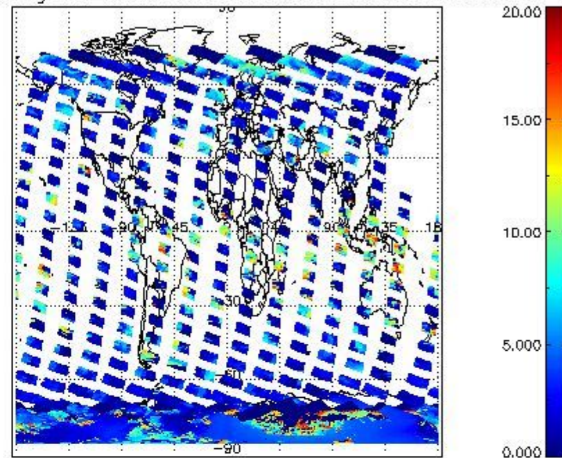
cL_top_height for 31JAN2009 00:00:00 to 01FEB2009 00:00:00
