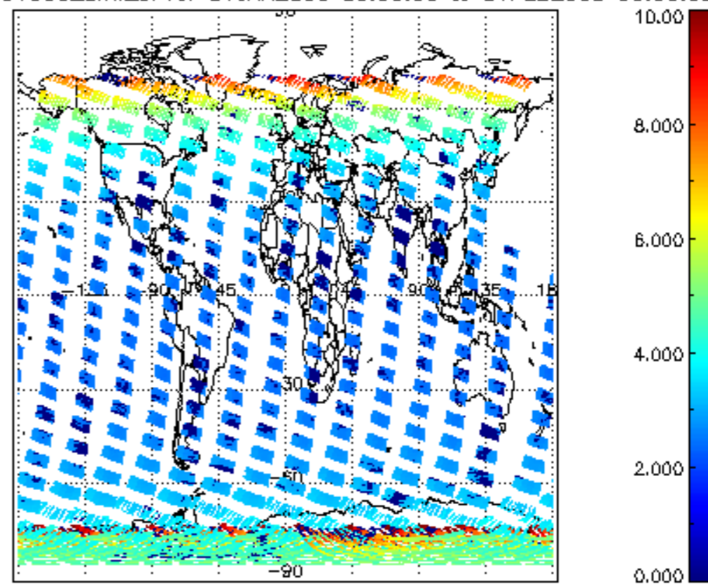
SCIOL2P_NADUV003_amf_cl for 31JAN2009 00:00:00 to 01FEB2009 00:00:00
