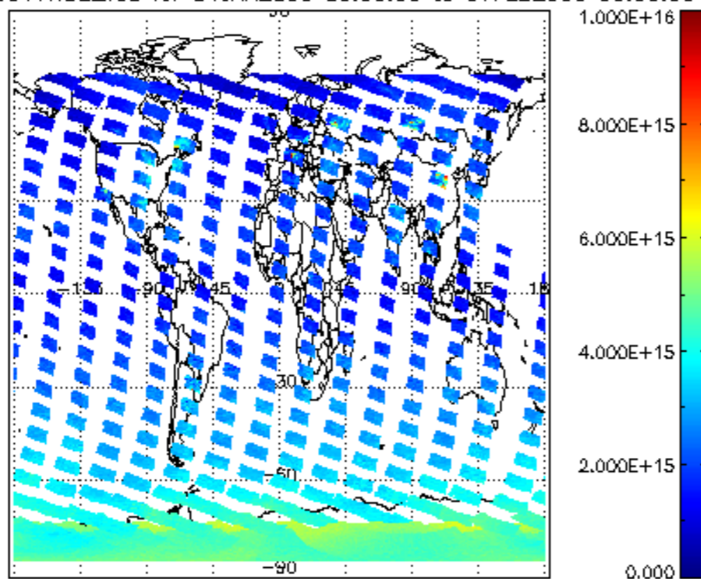
SCIOL2P_NADUV1NO2_vcd for 31JAN2009 00:00:00 to 01FEB2009 00:00:00
