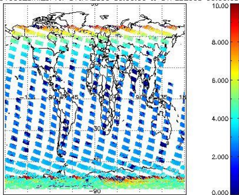
SCIOL2P_NADUV003_amf_cl for 31JAN2009 00:00:00 to 01FEB2009 00:00:00
