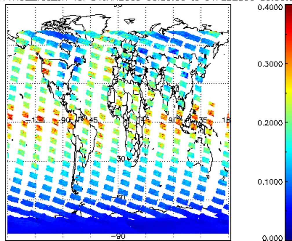
SCIOL2P_NADUV1NO2_vcd_err for 31JAN2009 00:00:00 to 01FEB2009 00:00:00
