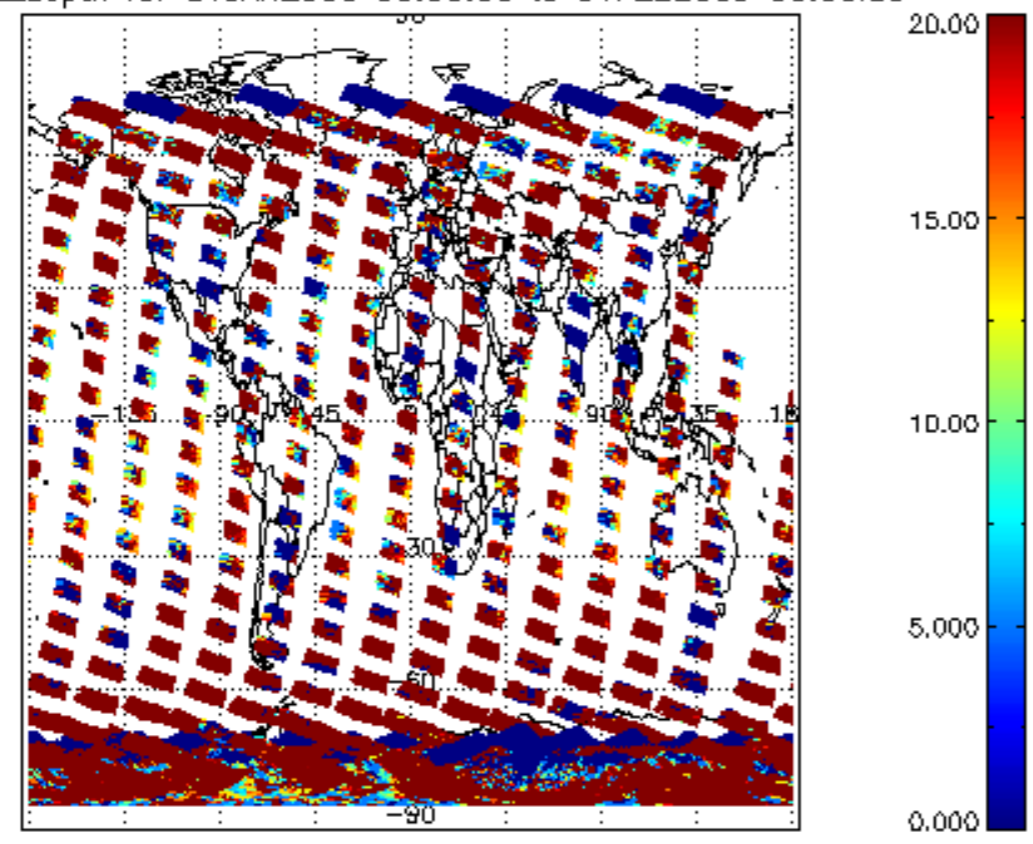
cl_opt_depth for 31JAN2009 00:00:00 to 01FEB2009 00:00:00
