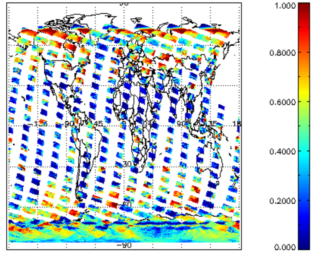
cl_frac for 31JAN2009 00:00:00 to 01FEB2009 00:00:00
