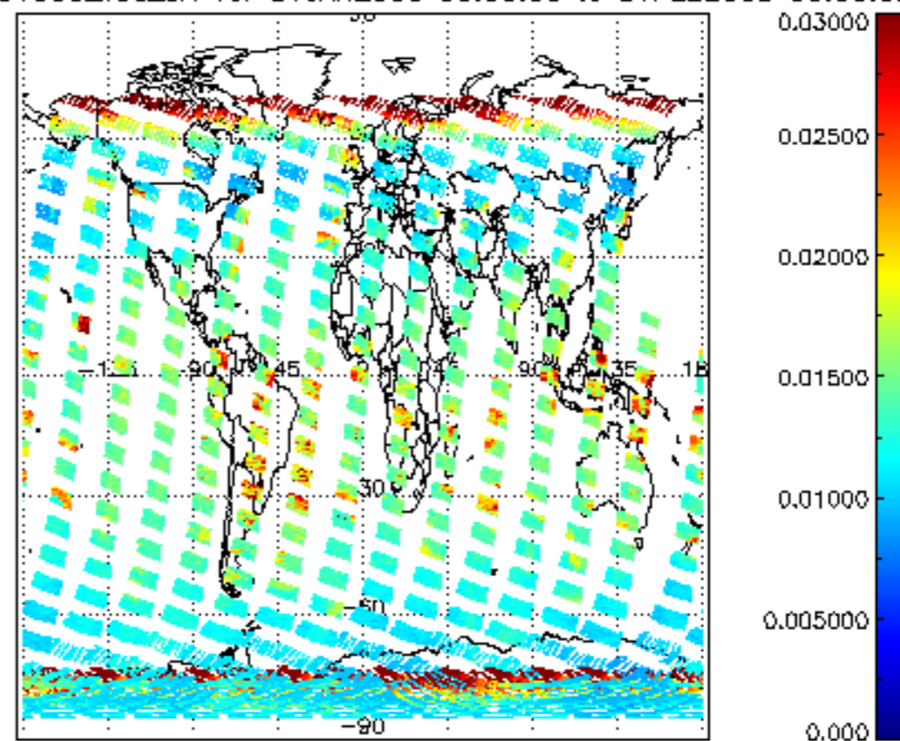
SCIOL2P_NADUV003_vcd_err for 31JAN2009 00:00:00 to 01FEB2009 00:00:00
