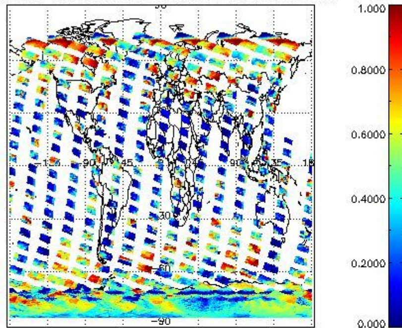
cL_frac for 31JAN2009 00:00:00 to 01FEB2009 00:00:00
