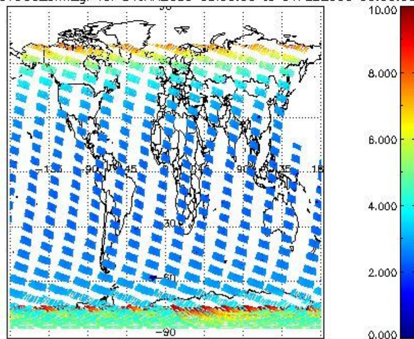
SCIOL2P_NADUV003_amf_gr for 31JAN2009 00:00:00 to 01FEB2009 00:00:00
