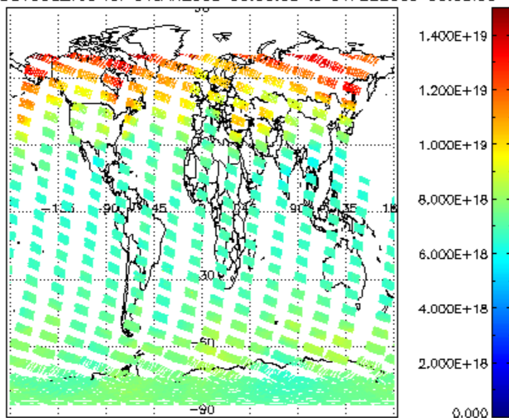
SCIOL2P_NADUV003_vcd for 31JAN2009 00:00:00 to 01FEB2009 00:00:00
