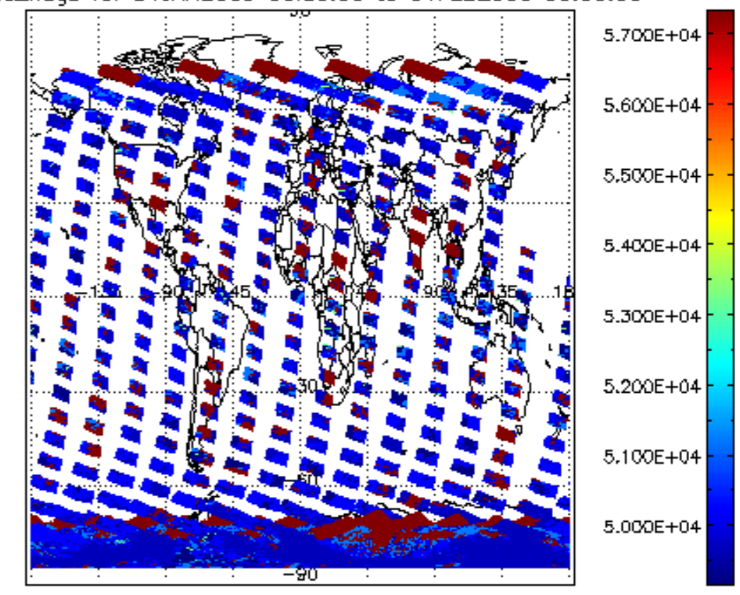
cloud_flags for 31JAN2009 00:00:00 to 01FEB2009 00:00:00
