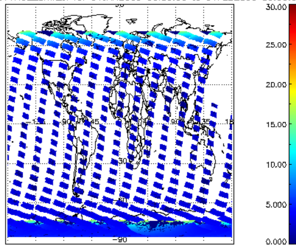
SCIOL2P_NADUV1NO2_amf_cl for 31JAN2009 00:00:00 to 01FEB2009 00:00:00
