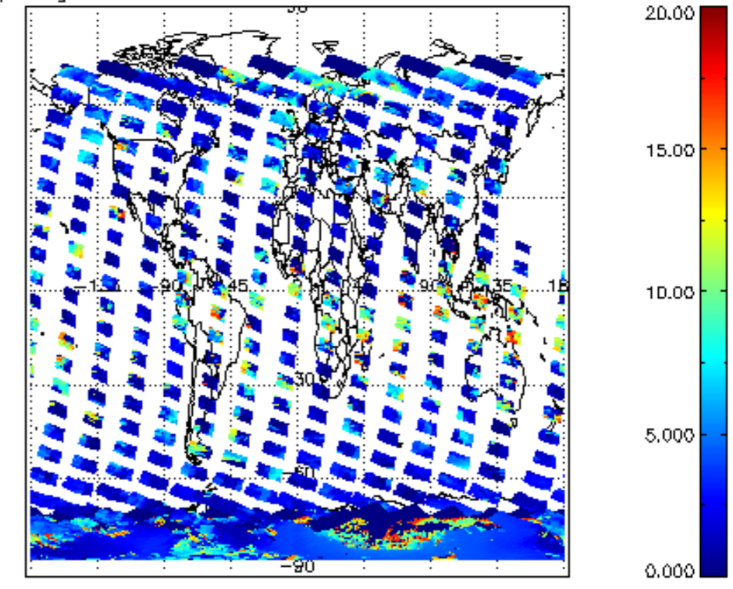
cl_top_height for 31JAN2009 00:00:00 to 01FEB2009 00:00:00
