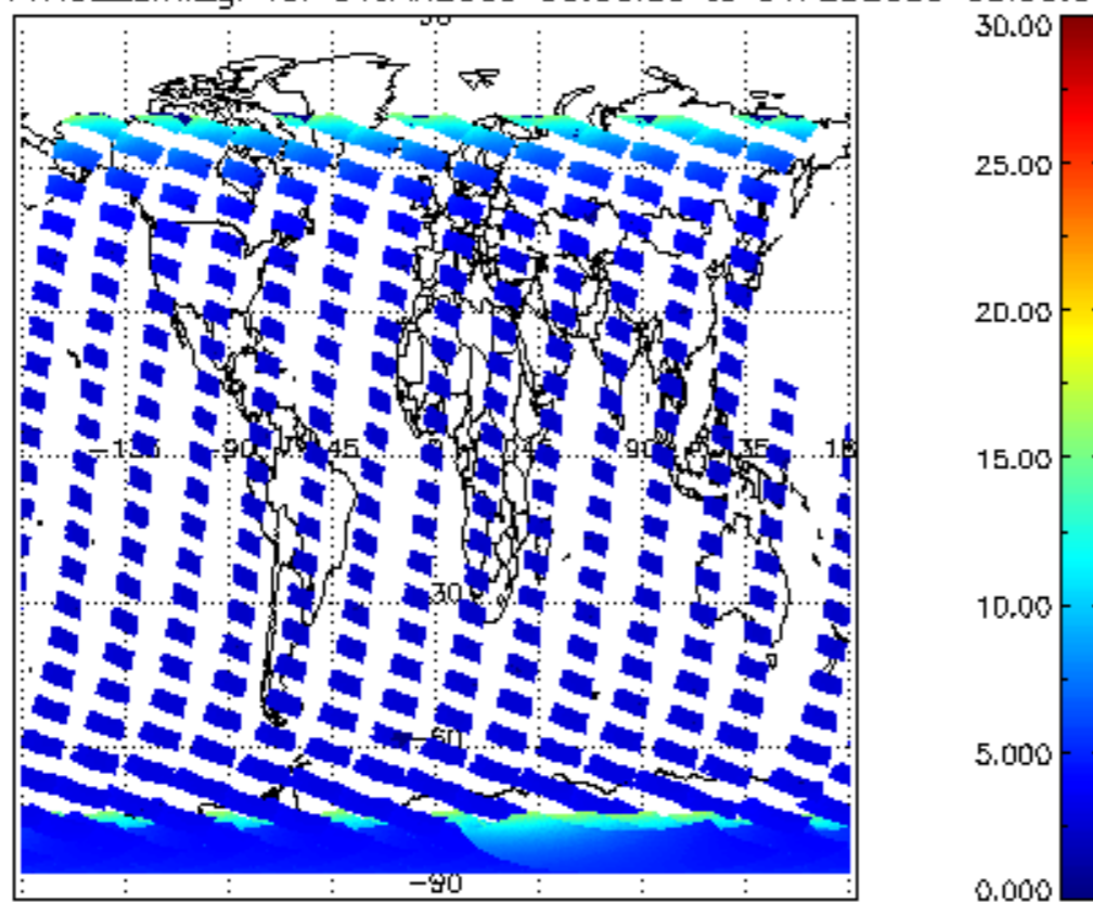
SCIOL2P_NADUV1NO2_amf_gr for 31JAN2009 00:00:00 to 01FEB2009 00:00:00
