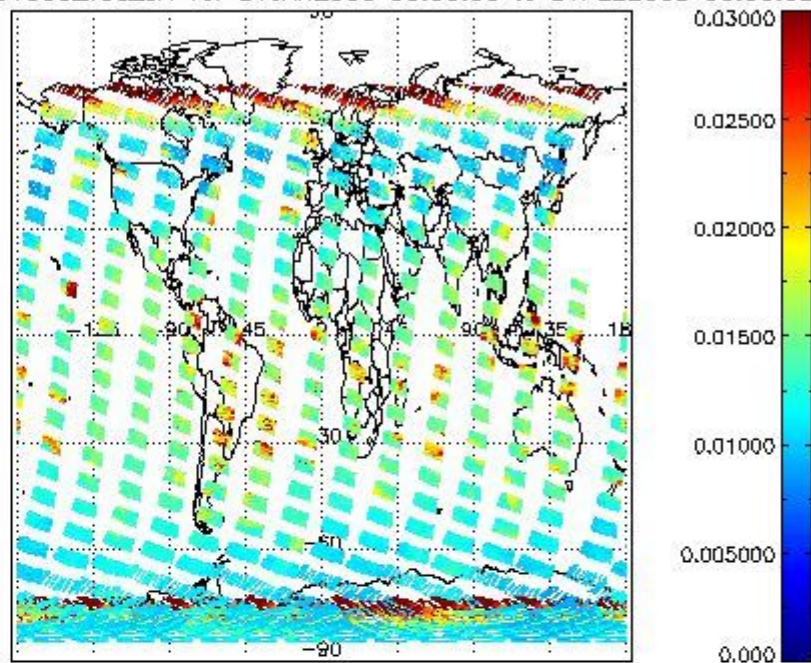
SCIOL2P_NADUV003_vcd_err for 31JAN2009 00:00:00 to 01FEB2009 00:00:00
