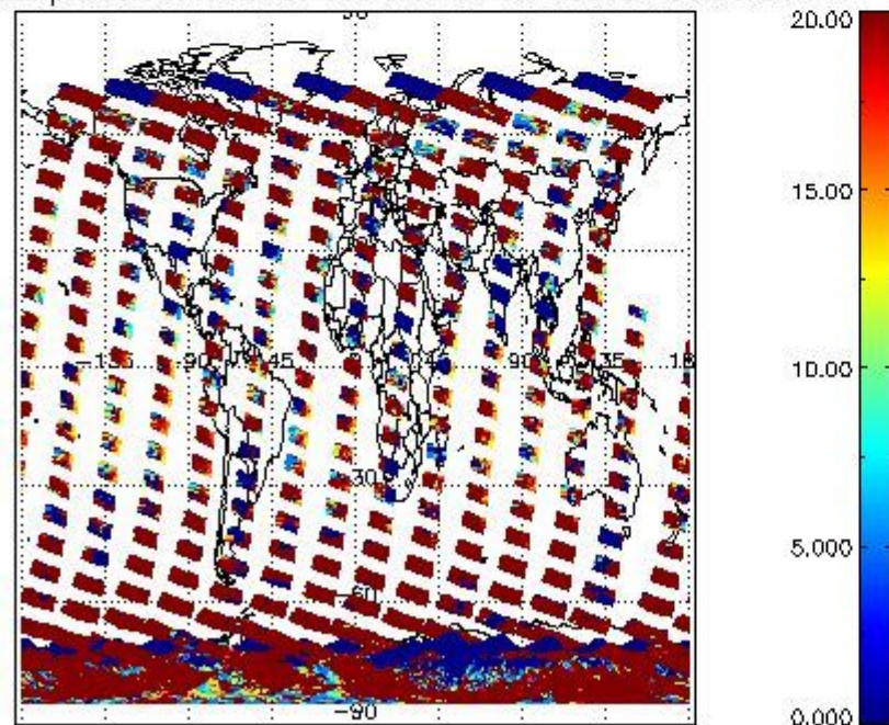
cL_opt_depth for 31JAN2009 00:00:00 to 01FEB2009 00:00:00
