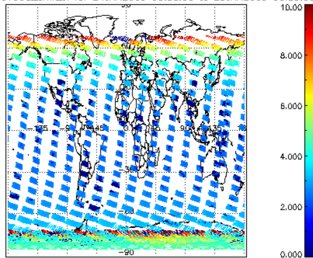
SCIOL2P_NADUV003_amf_cl for 24JAN2009 00:00:00 to 25JAN2009 00:00:00
