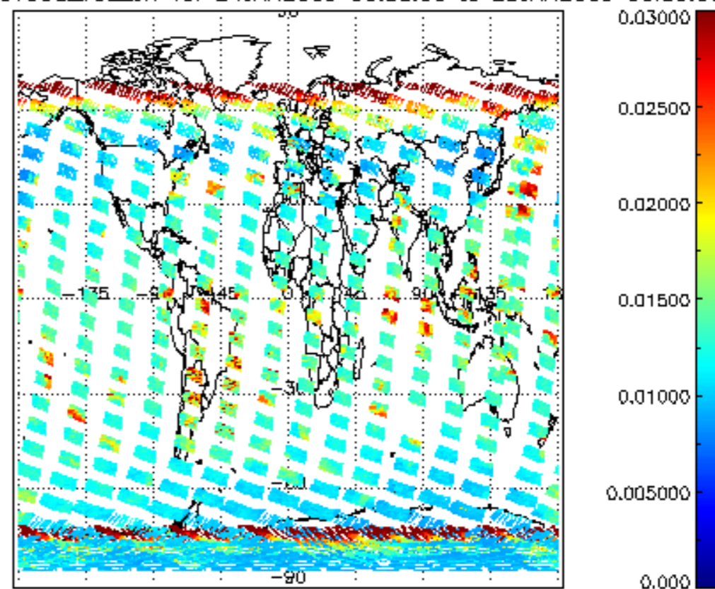
SCIOL2P_NADUV003_vcd_err for 24JAN2009 00:00:00 to 25JAN2009 00:00:00
