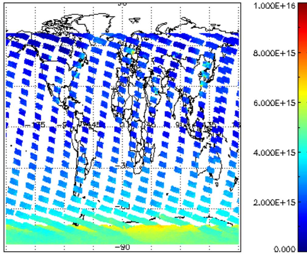
SCIOL2P_NADUV1NO2_vcd for 24JAN2009 00:00:00 to 25JAN2009 00:00:00
