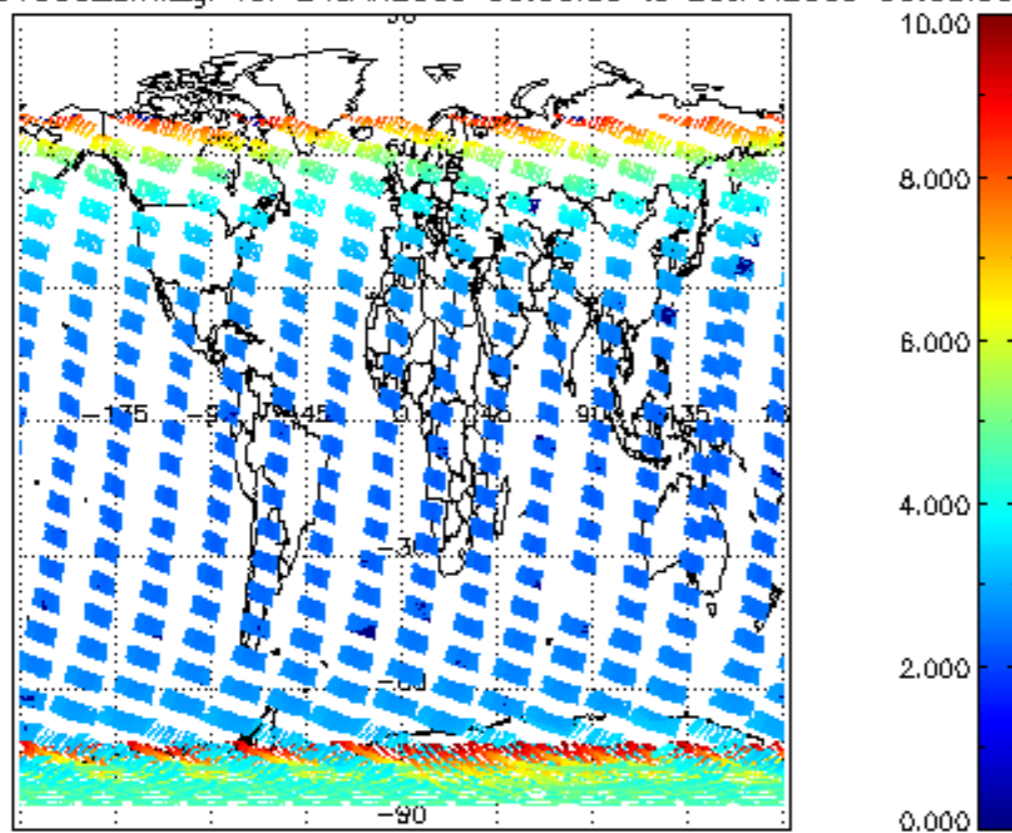
SCIOL2P_NADUV003_amf_gr for 24JAN2009 00:00:00 to 25JAN2009 00:00:00
