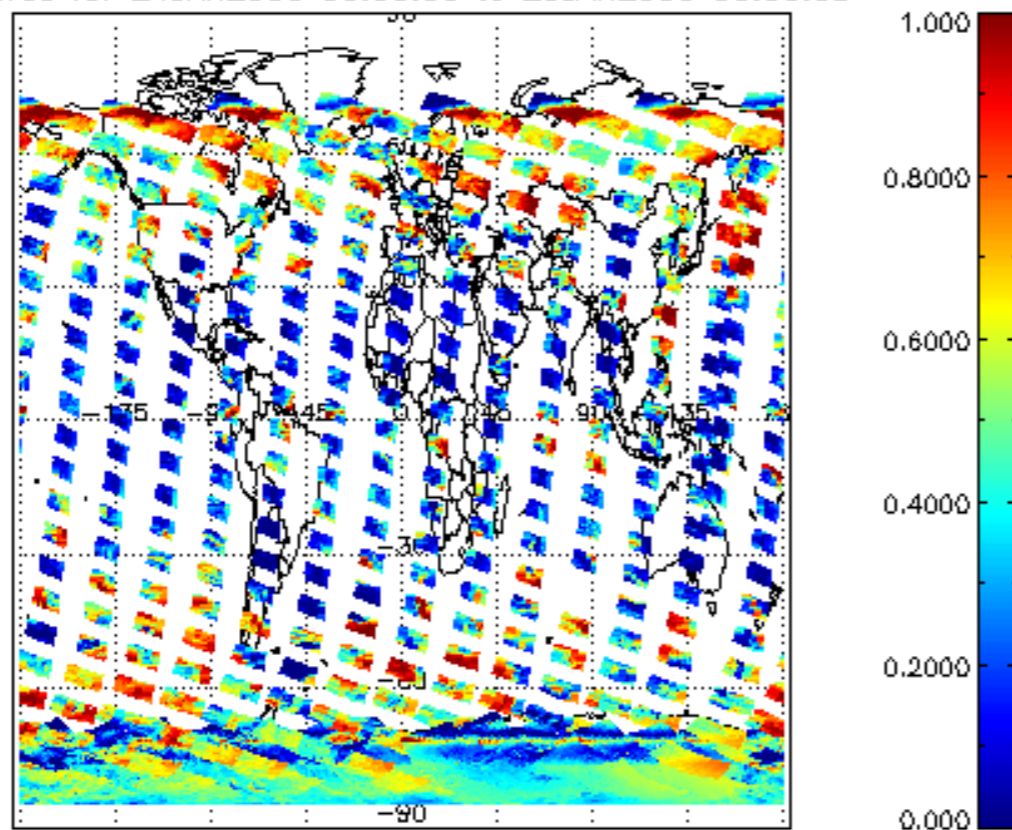
cL_frac for 24JAN2009 00:00:00 to 25JAN2009 00:00:00
