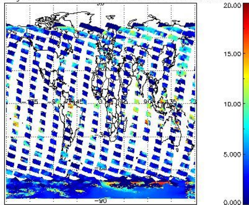
cL_top_height for 24JAN2009 00:00:00 to 25JAN2009 00:00:00
