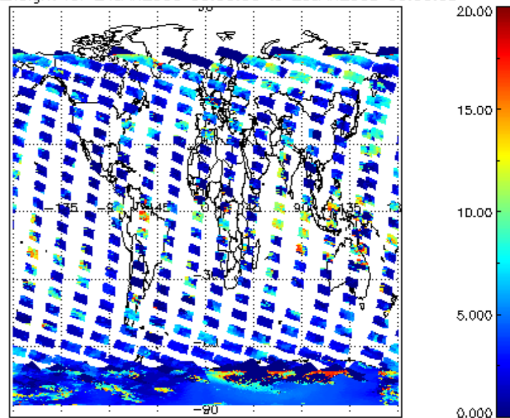
cL_top_height for 24JAN2009 00:00:00 to 25JAN2009 00:00:00
