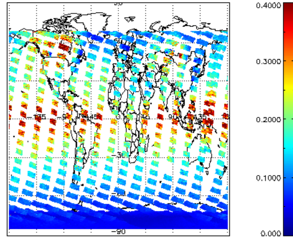
SCIOL2P_NADUV1NO2_vcd_err for 24JAN2009 00:00:00 to 25JAN2009 00:00:00
