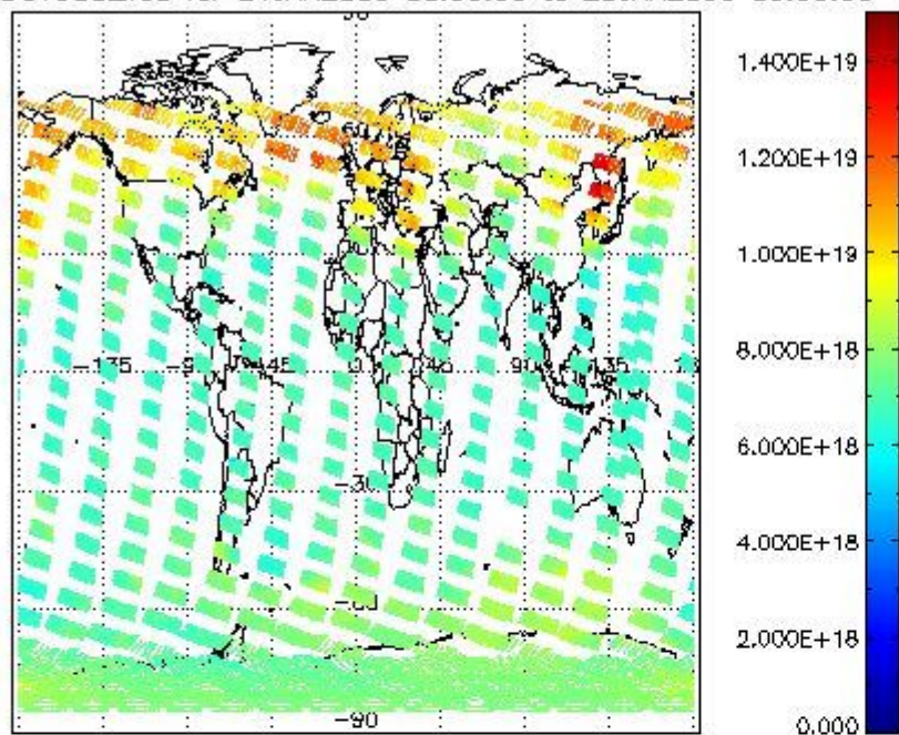
SCIOL2P_NADUV003_vcd for 24JAN2009 00:00:00 to 25JAN2009 00:00:00
