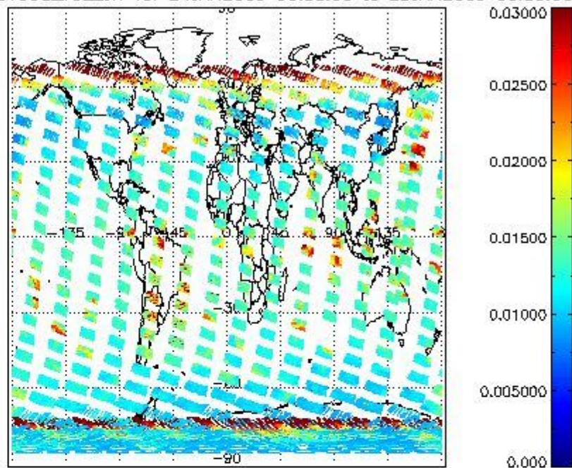
SCIOL2P_NADUV003_vcd_err for 24JAN2009 00:00:00 to 25JAN2009 00:00:00
