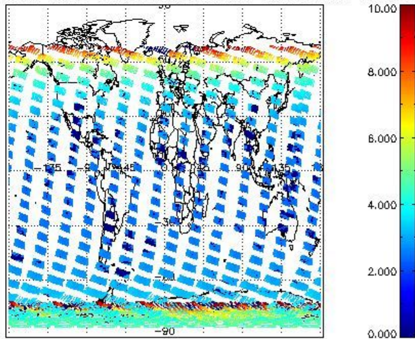
SCIOL2P_NADUV003_amf_cl for 24JAN2009 00:00:00 to 25JAN2009 00:00:00
