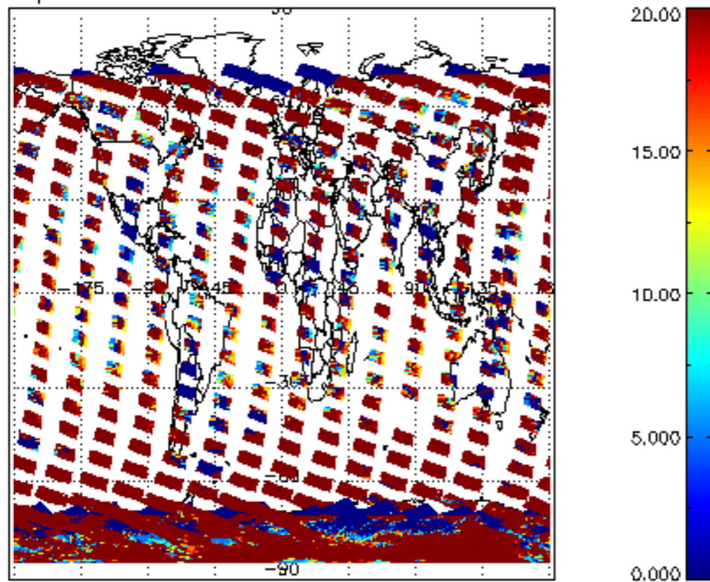
cLopt_depth for 24JAN2009 00:00:00 to 25JAN2009 00:00:00
