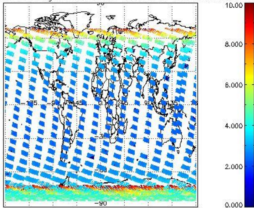
SCIOL2P_NADUV003_amf_gr for 24JAN2009 00:00:00 to 25JAN2009 00:00:00
