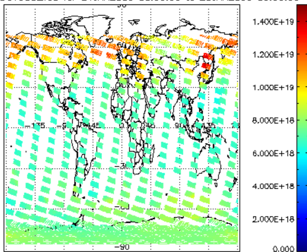
SCIOL2P_NADUV003_vcd for 24JAN2009 00:00:00 to 25JAN2009 00:00:00
