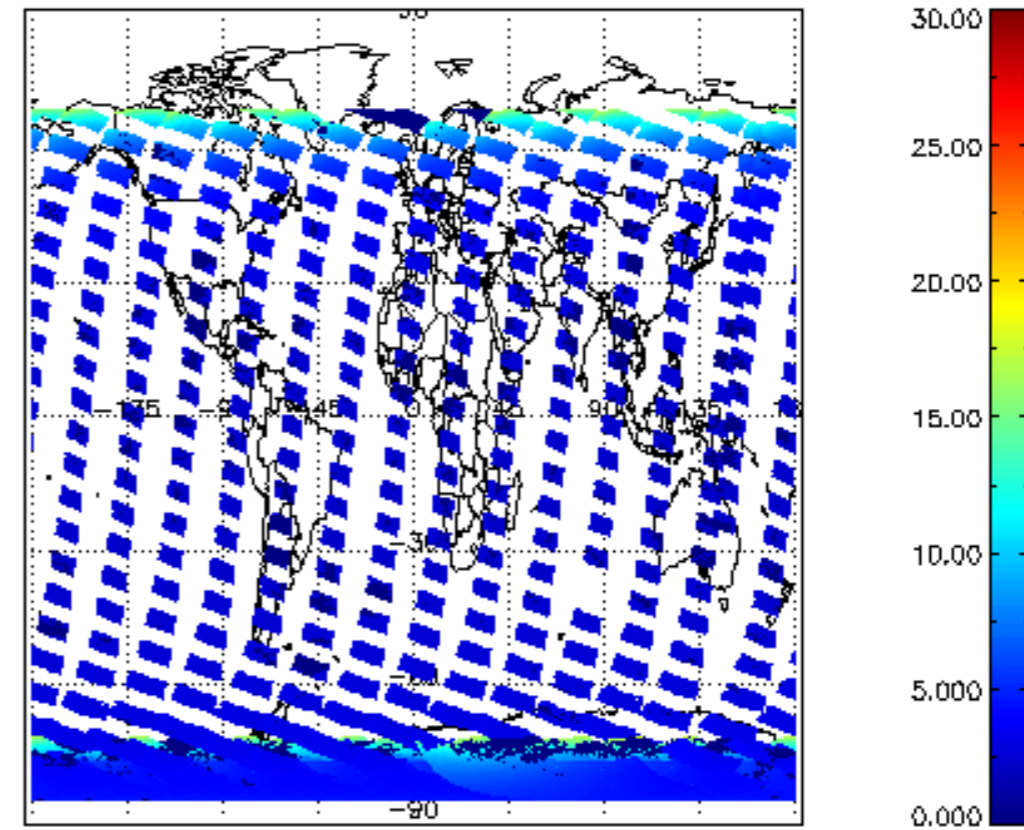
SCIOL2P_NADUV1NO2_amf_cl for 24JAN2009 00:00:00 to 25JAN2009 00:00:00
