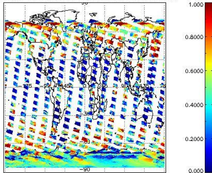
cL_frac for 24JAN2009 00:00:00 to 25JAN2009 00:00:00
