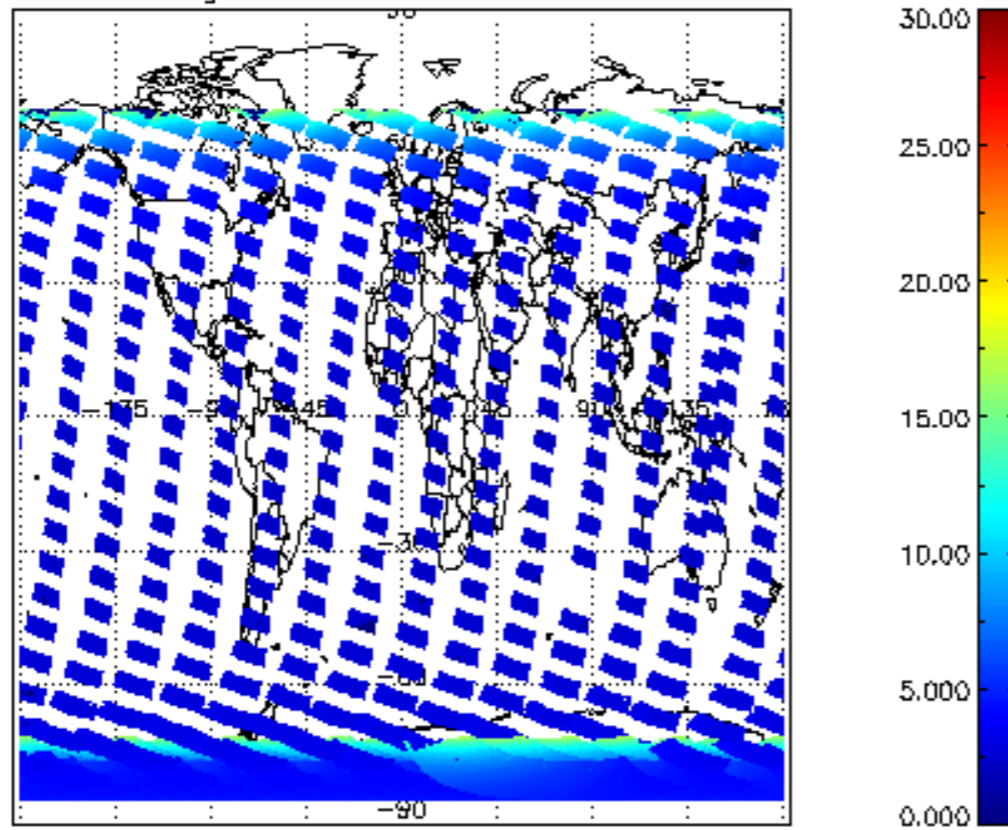
SCIOL2P_NADUV1NO2_amf_gr for 24JAN2009 00:00:00 to 25JAN2009 00:00:00
