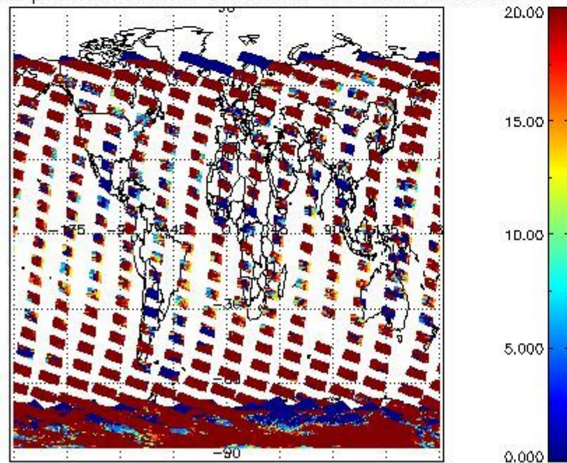
cLopt_depth for 24JAN2009 00:00:00 to 25JAN2009 00:00:00
