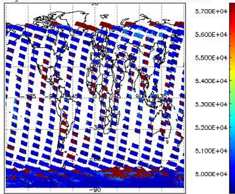
cloud_flags for 24JAN2009 00:00:00 to 25JAN2009 00:00:00
