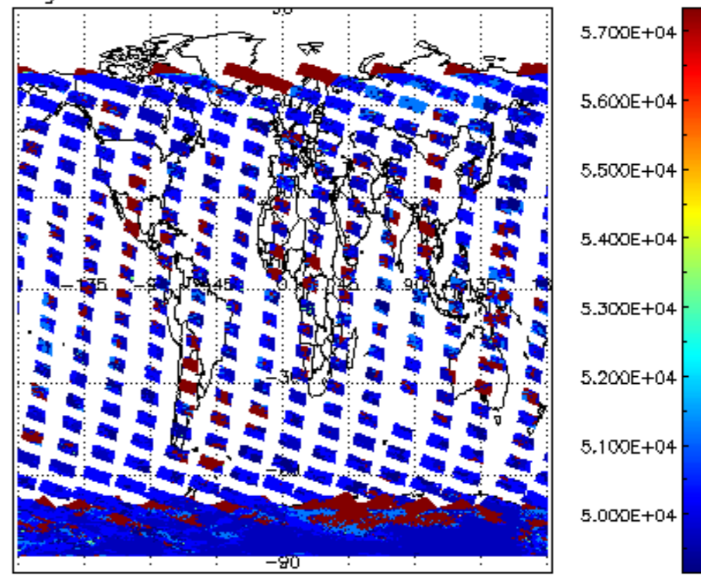
cloud_flags for 24JAN2009 00:00:00 to 25JAN2009 00:00:00
