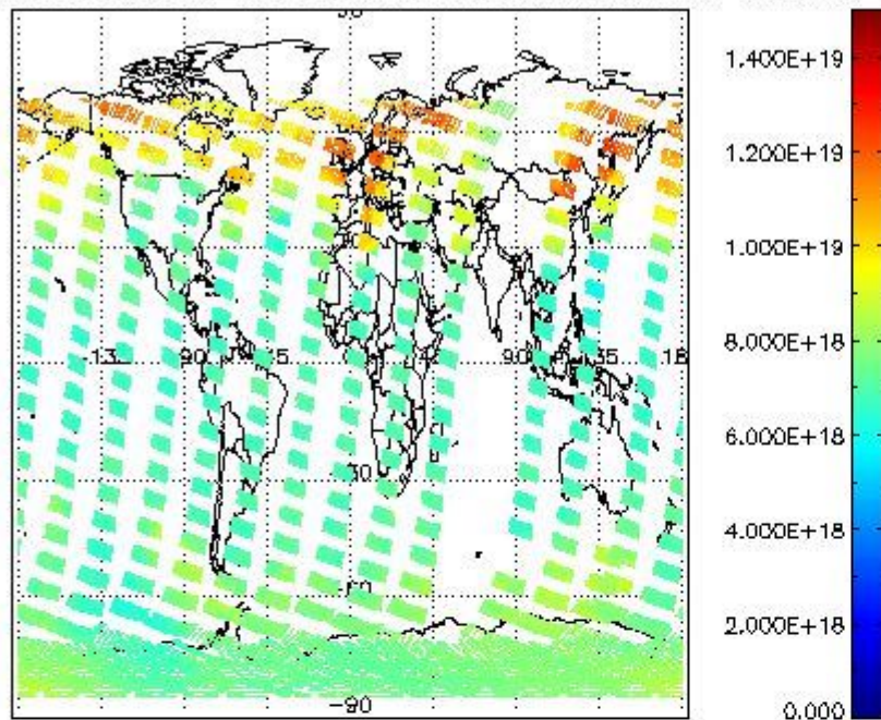
SCIOL2P_NADUV003_vcd for 22JAN2009 00:00:00 to 23JAN2009 00:00:00
