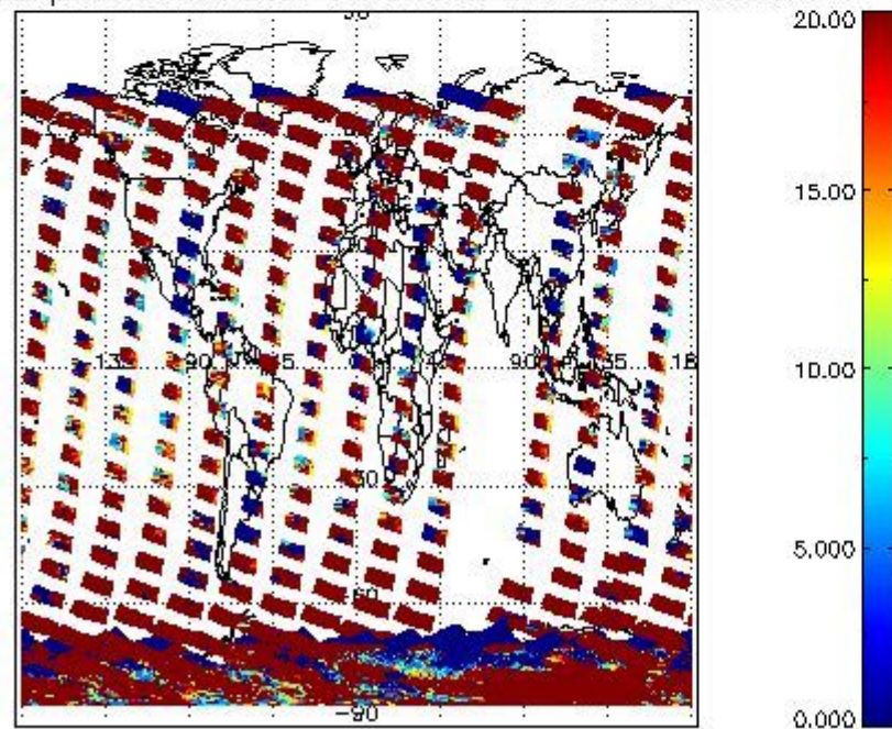
cLopt_depth for 22JAN2009 00:00:00 to 23JAN2009 00:00:00
