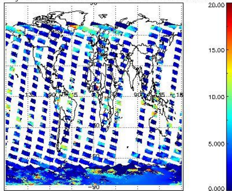
cL_top_height for 22JAN2009 00:00:00 to 23JAN2009 00:00:00
