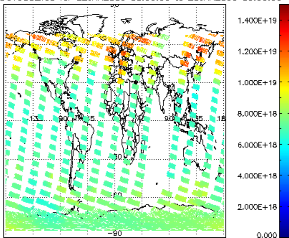
SCIOL2P_NADUV003_vcd for 22JAN2009 00:00:00 to 23JAN2009 00:00:00
