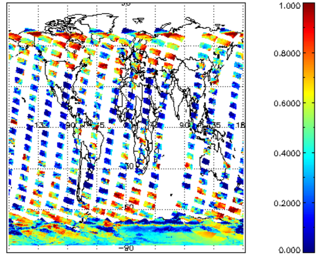
cL_frac for 22JAN2009 00:00:00 to 23JAN2009 00:00:00
