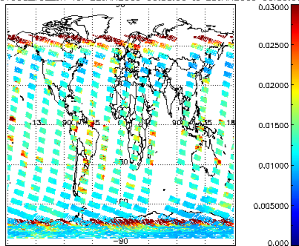
SCIOL2P_NADUV003_vcd_err for 22JAN2009 00:00:00 to 23JAN2009 00:00:00
