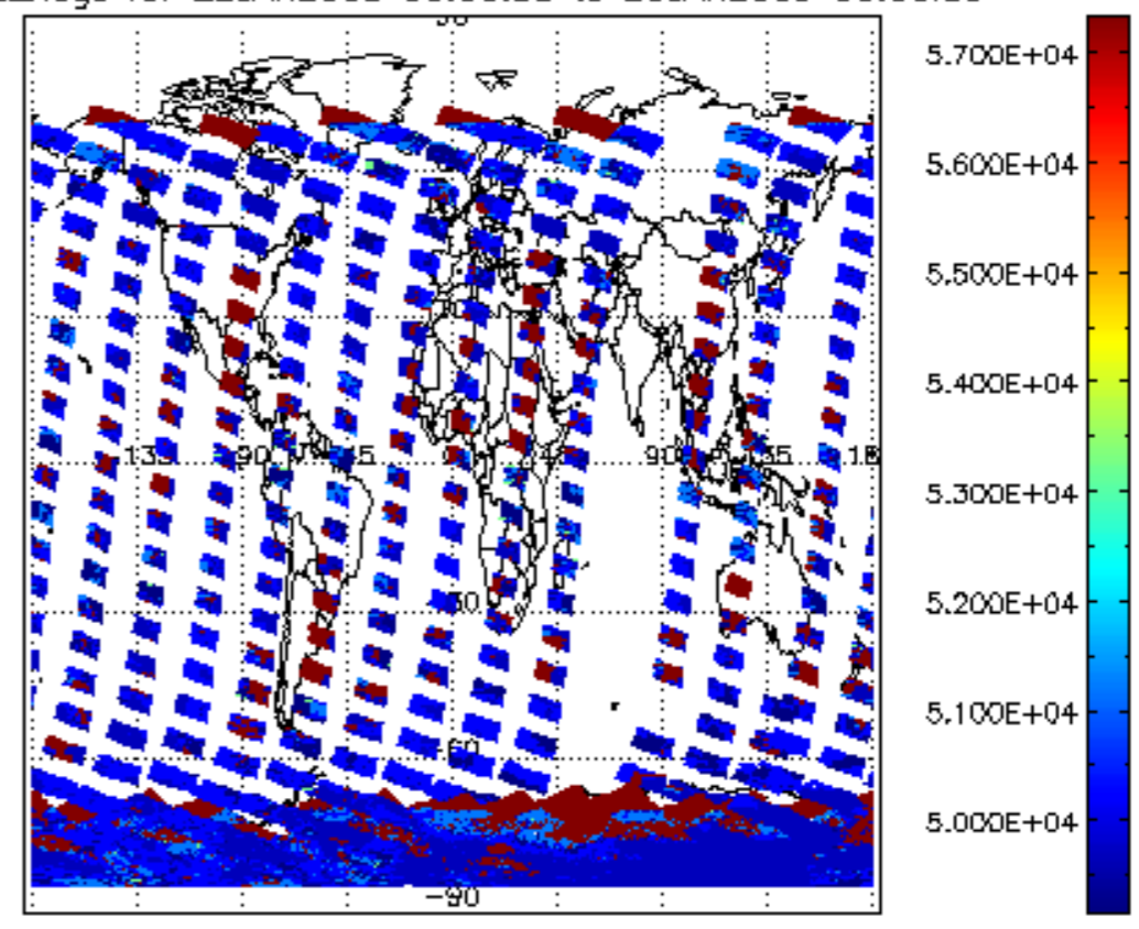
cloud_flags for 22JAN2009 00:00:00 to 23JAN2009 00:00:00
