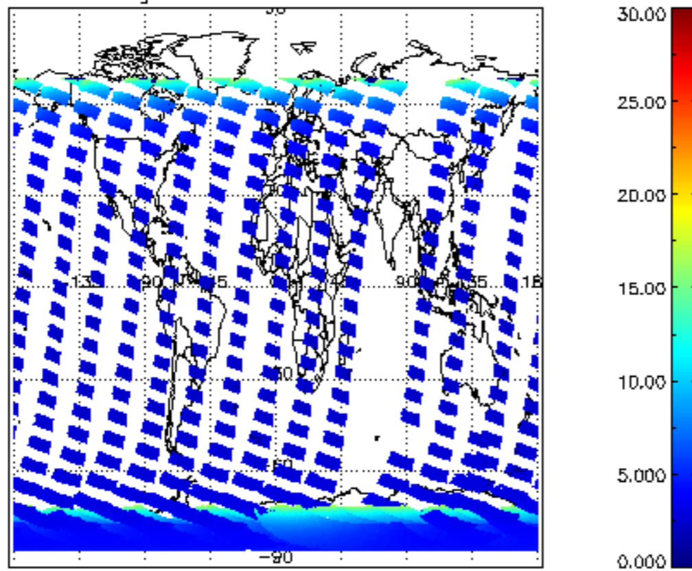
SCIOL2P_NADUV1NO2_amf_gr for 22JAN2009 00:00:00 to 23JAN2009 00:00:00
