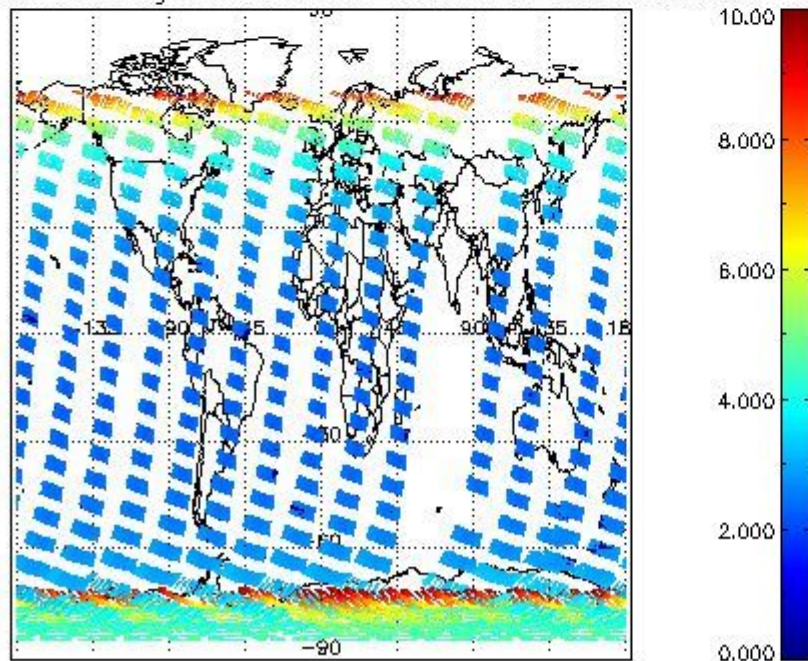
SCIOL2P_NADUV003_amf_gr for 22JAN2009 00:00:00 to 23JAN2009 00:00:00
