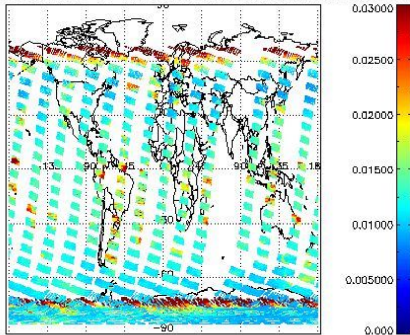
SCIOL2P_NADUV003_vcd_err for 22JAN2009 00:00:00 to 23JAN2009 00:00:00
