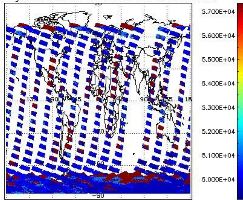
cloud_flags for 22JAN2009 00:00:00 to 23JAN2009 00:00:00
