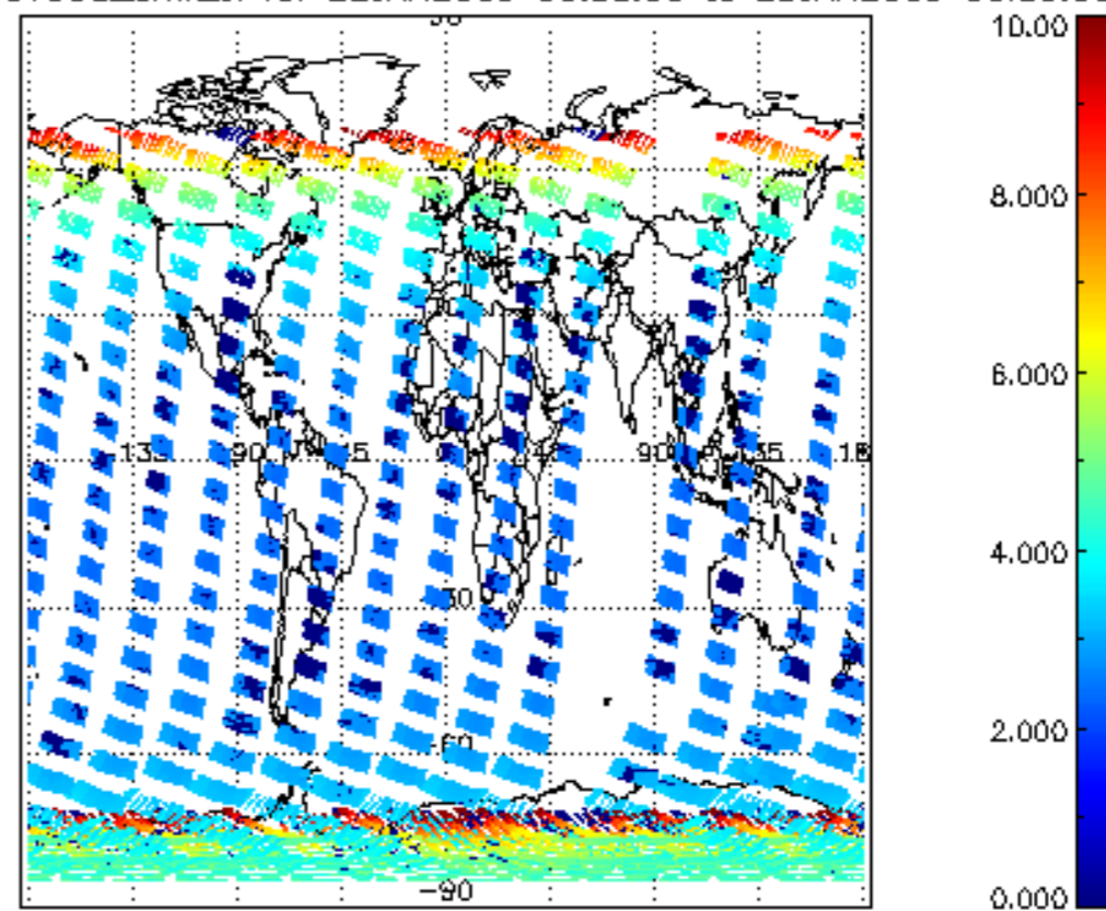
SCIOL2P_NADUV003_amf_cl for 22JAN2009 00:00:00 to 23JAN2009 00:00:00
