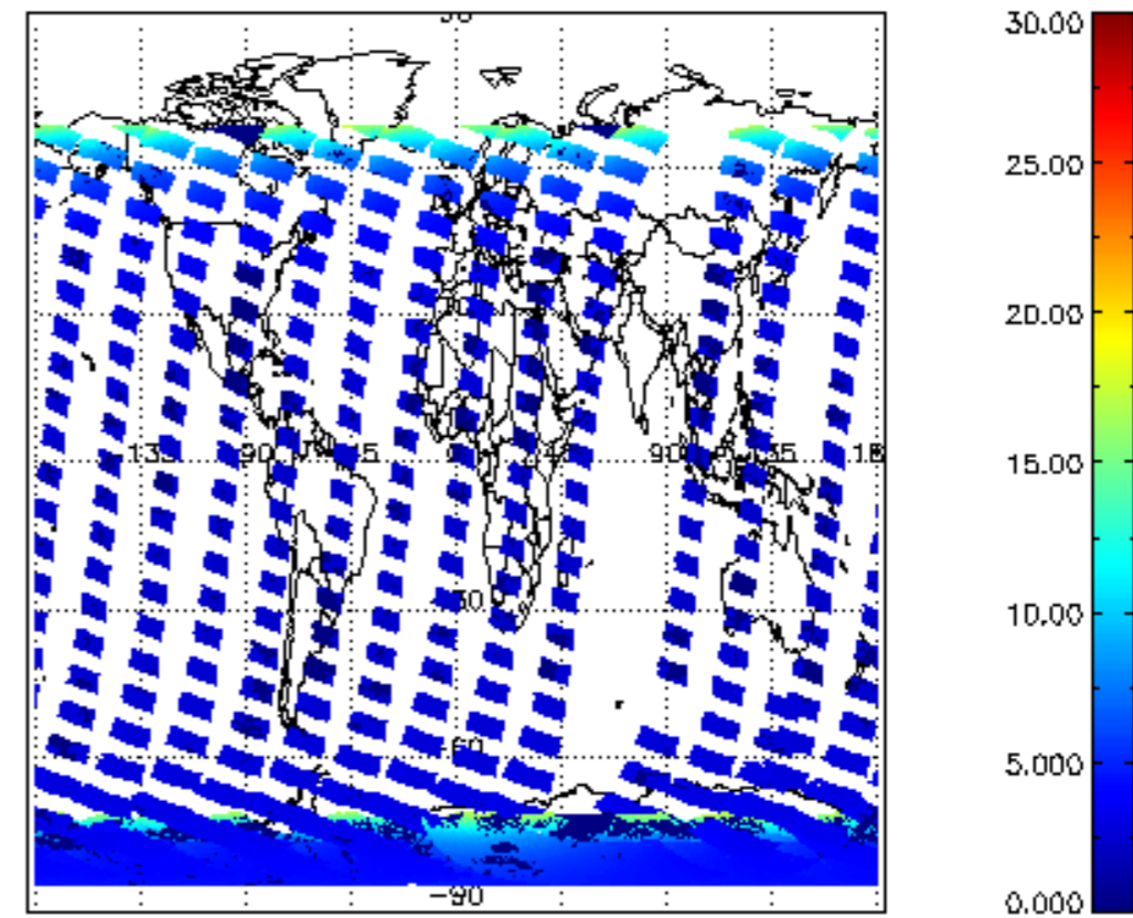
SCIOL2P_NADUV1NO2_amf_cl for 22JAN2009 00:00:00 to 23JAN2009 00:00:00
