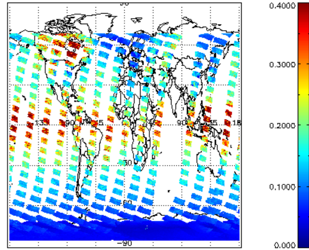
SCIOL2P_NADUV1NO2_vcd_err for 22JAN2009 00:00:00 to 23JAN2009 00:00:00
