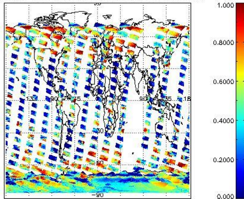
cL_frac for 22JAN2009 00:00:00 to 23JAN2009 00:00:00
