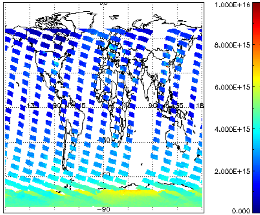
SCIOL2P_NADUV1NO2_vcd for 22JAN2009 00:00:00 to 23JAN2009 00:00:00
