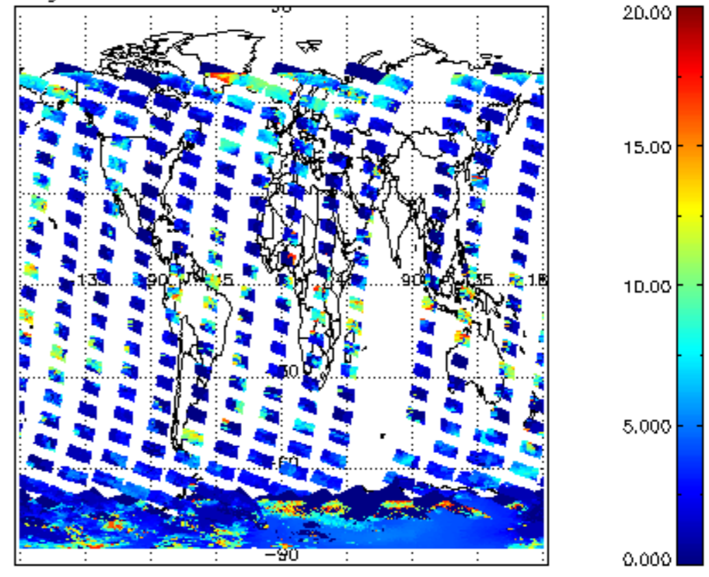
cL_top_height for 22JAN2009 00:00:00 to 23JAN2009 00:00:00
