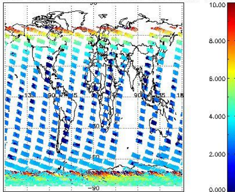
SCIOL2P_NADUV003_amf_cl for 22JAN2009 00:00:00 to 23JAN2009 00:00:00
