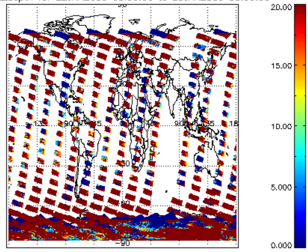
cLopt_depth for 22JAN2009 00:00:00 to 23JAN2009 00:00:00
