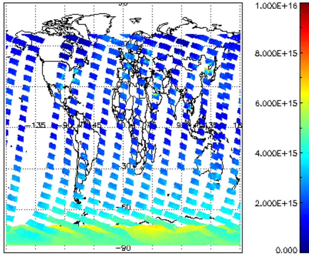
SCIOL2P_NADUV1NO2_vcd for 21JAN2009 00:00:00 to 22JAN2009 00:00:00
