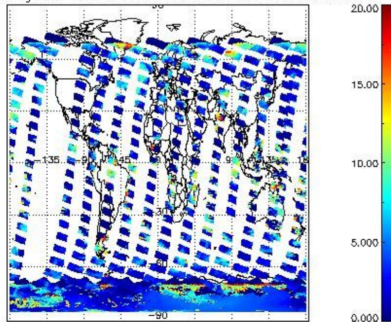
cL_top_height for 21JAN2009 00:00:00 to 22JAN2009 00:00:00
