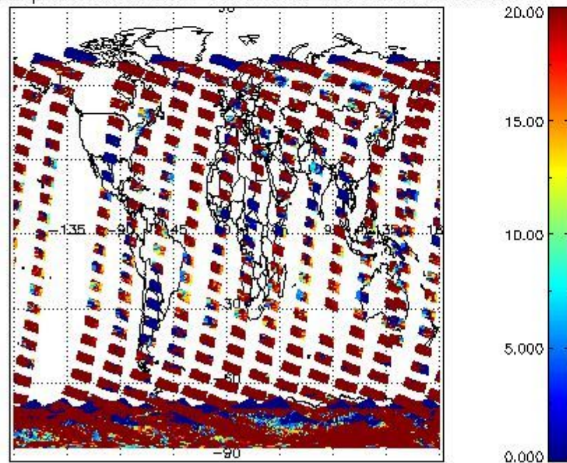
cLopt_depth for 21JAN2009 00:00:00 to 22JAN2009 00:00:00
