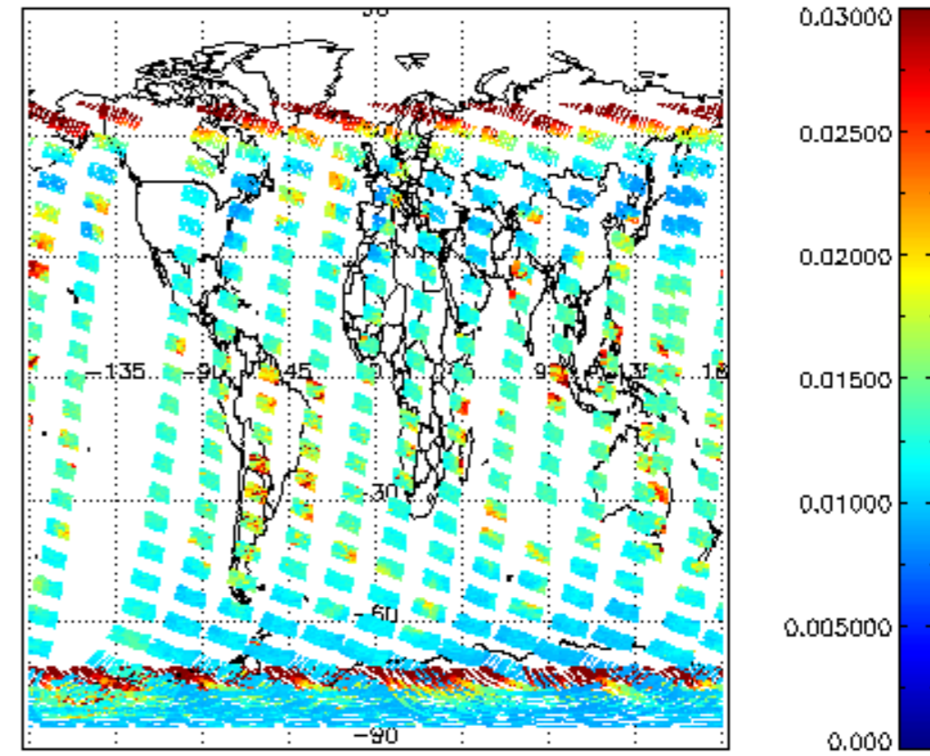
SCIOL2P_NADUV003_vcd_err for 21JAN2009 00:00:00 to 22JAN2009 00:00:00
