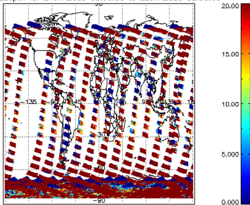
cLopt_depth for 21JAN2009 00:00:00 to 22JAN2009 00:00:00
