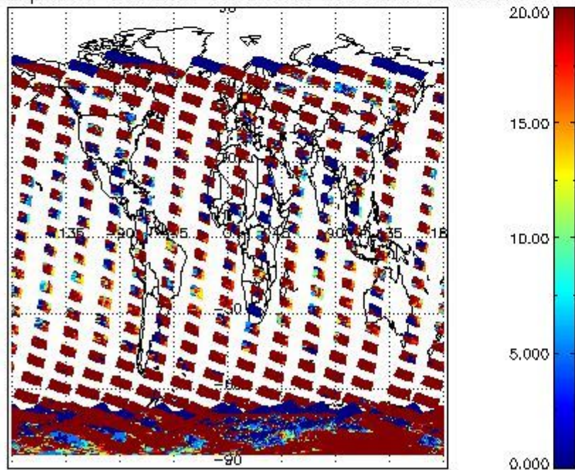
cLopt_depth for 19JAN2009 00:00:00 to 20JAN2009 00:00:00
