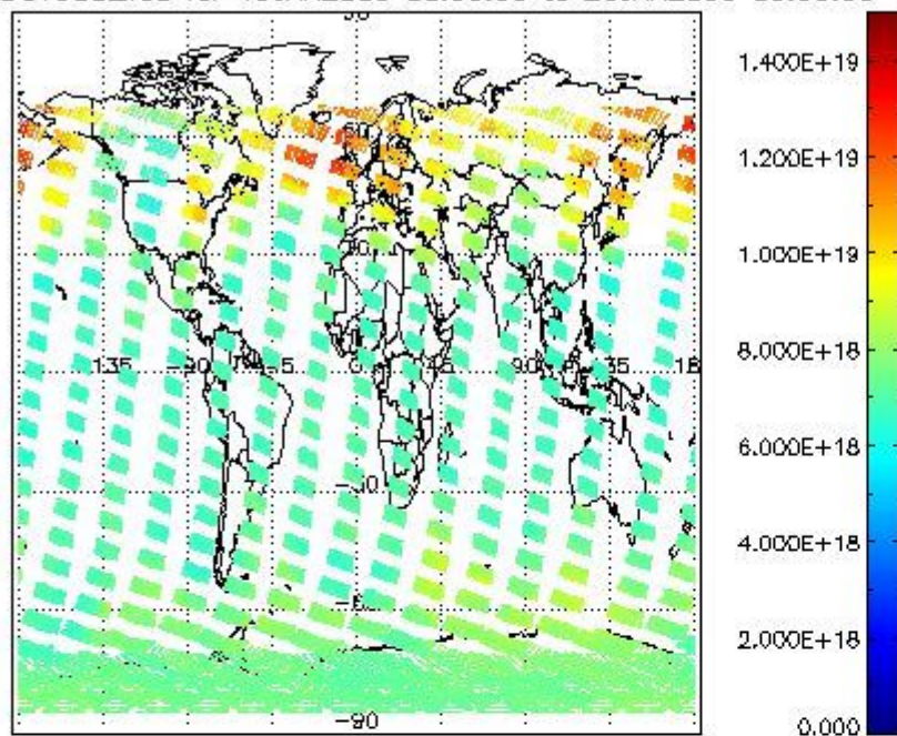
SCIOL2P_NADUV003_vcd for 19JAN2009 00:00:00 to 20JAN2009 00:00:00
