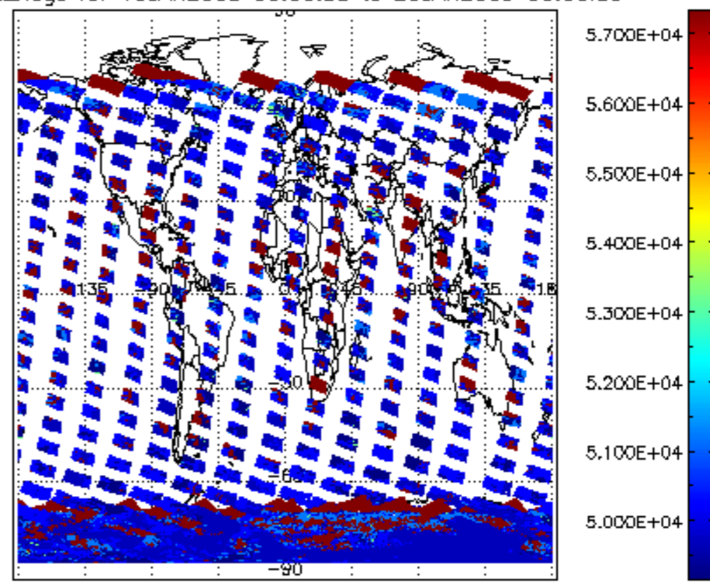
cloud_flags for 19JAN2009 00:00:00 to 20JAN2009 00:00:00
