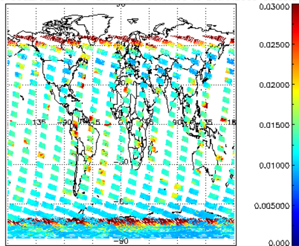
SCIOL2P_NADUV003_vcd_err for 19JAN2009 00:00:00 to 20JAN2009 00:00:00
