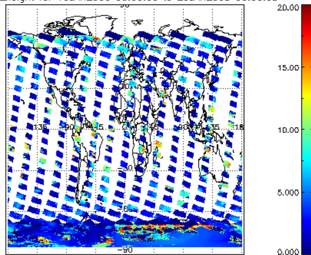
cL_top_height for 19JAN2009 00:00:00 to 20JAN2009 00:00:00
