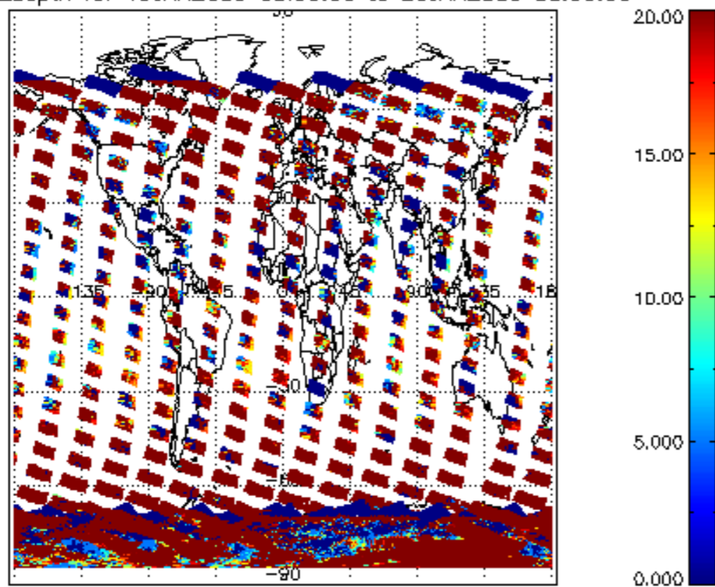
cLopt_depth for 19JAN2009 00:00:00 to 20JAN2009 00:00:00
