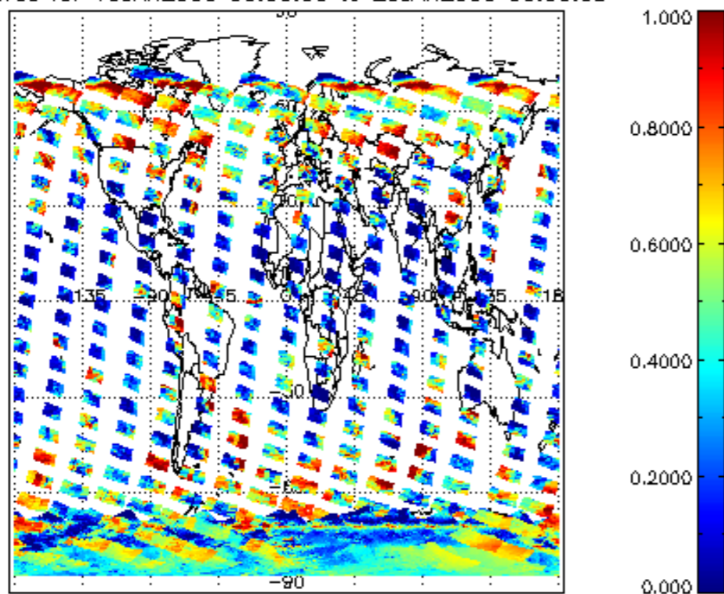
cL_frac for 19JAN2009 00:00:00 to 20JAN2009 00:00:00
