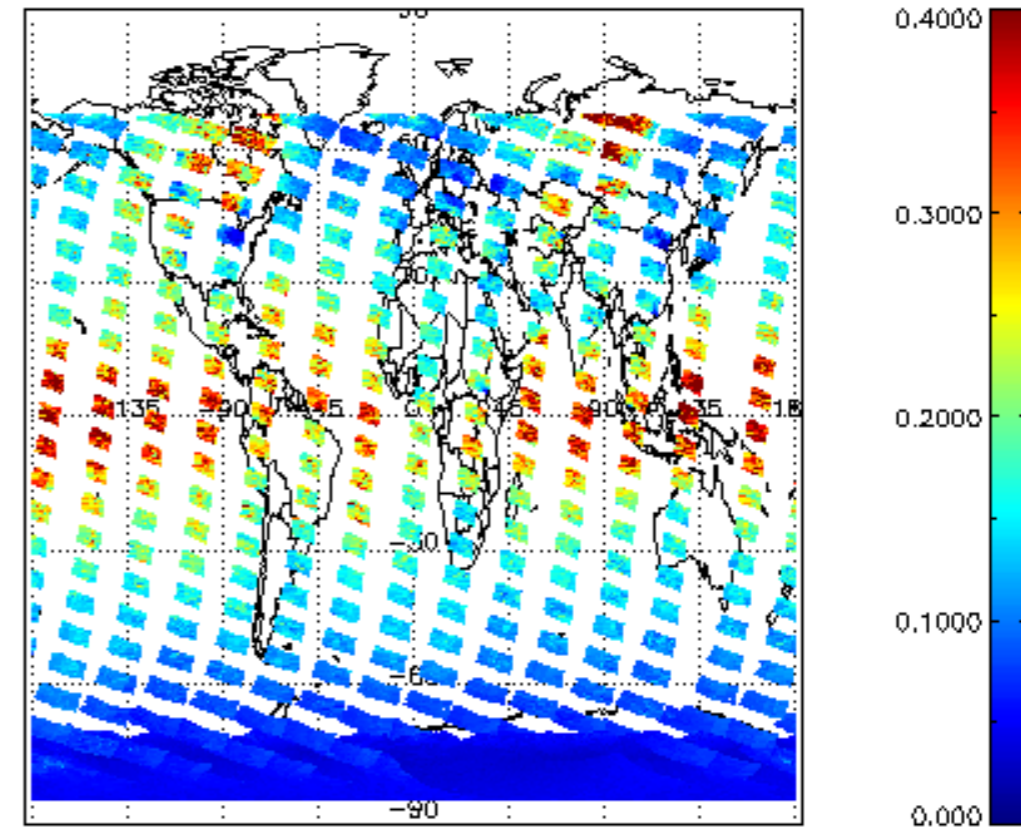
SCIOL2P_NADUV1NO2_vcd_err for 19JAN2009 00:00:00 to 20JAN2009 00:00:00
