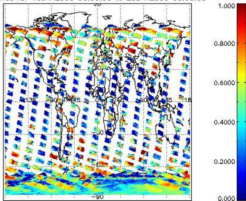
cL_frac for 19JAN2009 00:00:00 to 20JAN2009 00:00:00
