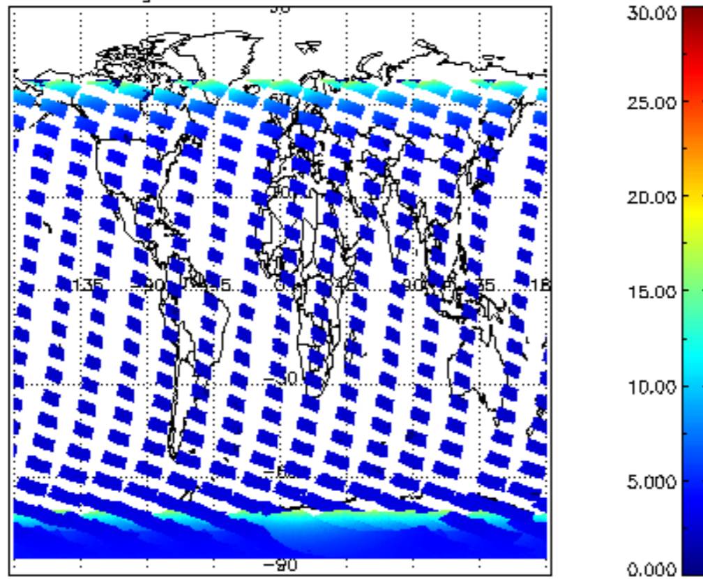
SCIOL2P_NADUV1NO2_amf_gr for 19JAN2009 00:00:00 to 20JAN2009 00:00:00
