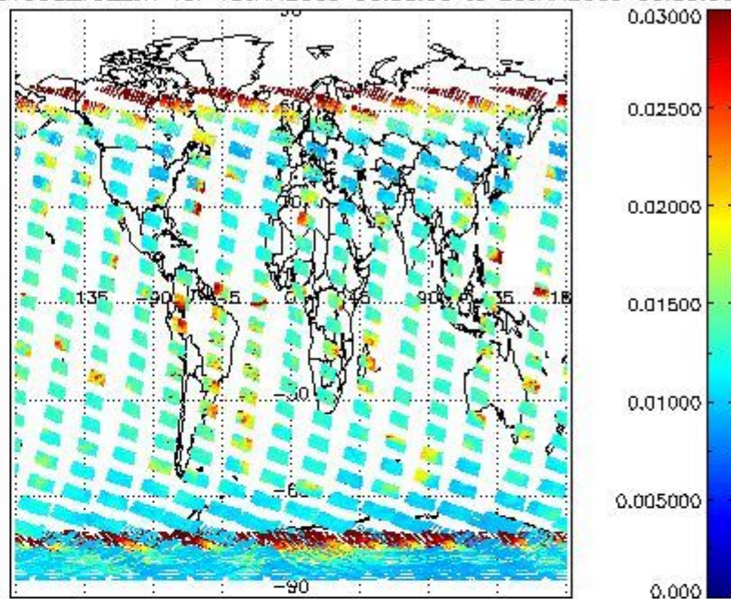
SCIOL2P_NADUV003_vcd_err for 19JAN2009 00:00:00 to 20JAN2009 00:00:00
