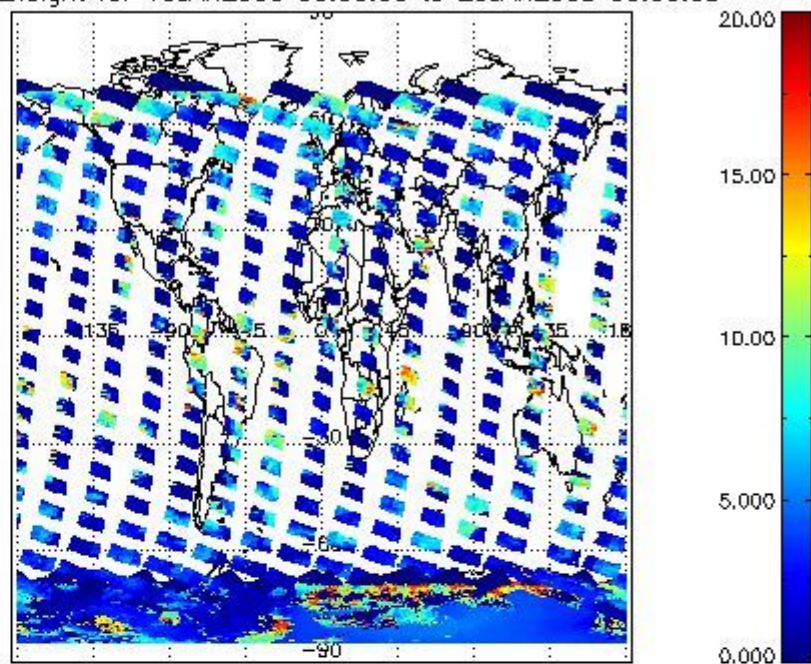
cL_top_height for 19JAN2009 00:00:00 to 20JAN2009 00:00:00
