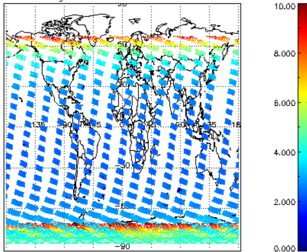
SCIOL2P_NADUV003_amf_gr for 19JAN2009 00:00:00 to 20JAN2009 00:00:00
