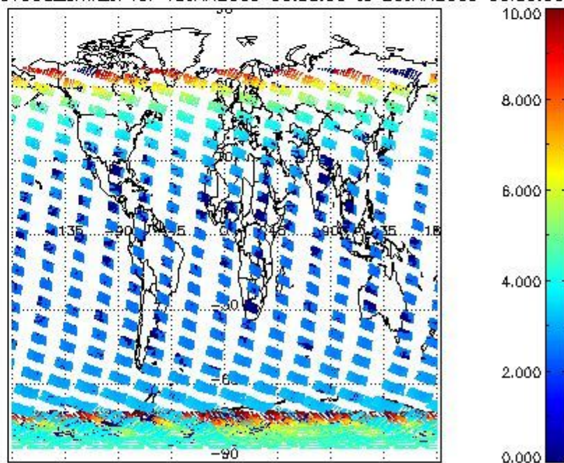
SCIOL2P_NADUV003_amf_cl for 19JAN2009 00:00:00 to 20JAN2009 00:00:00
