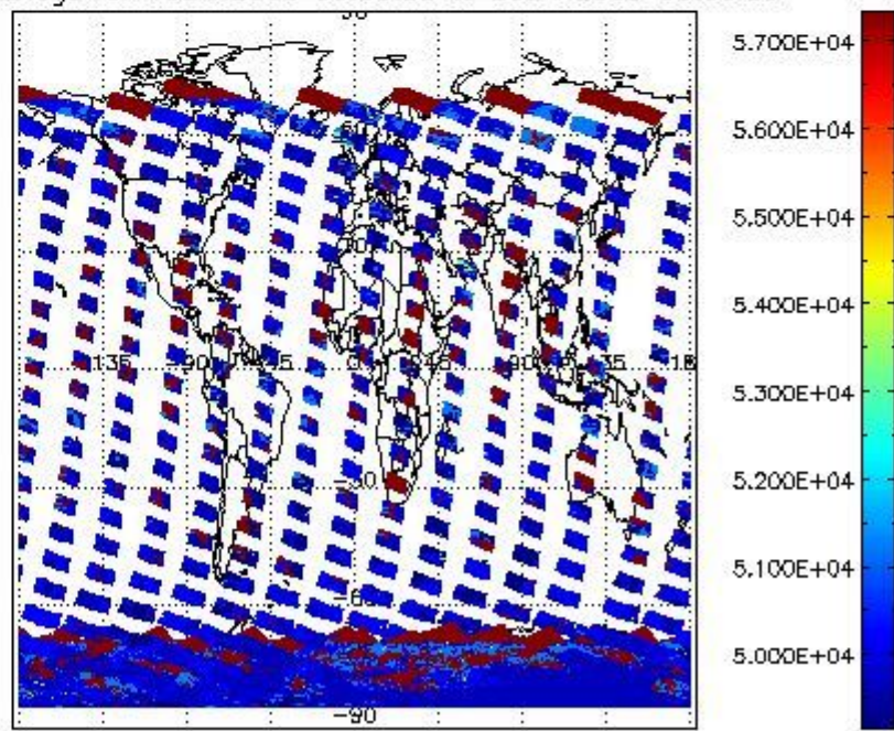
cloud_flags for 19JAN2009 00:00:00 to 20JAN2009 00:00:00
