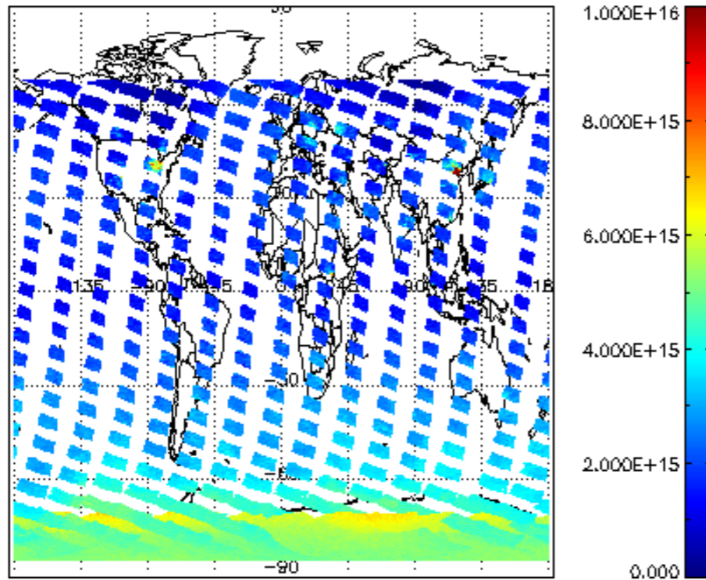
SCIOL2P_NADUV1NO2_vcd for 19JAN2009 00:00:00 to 20JAN2009 00:00:00
