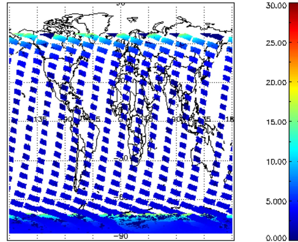
SCIOL2P_NADUV1NO2_amf_cl for 19JAN2009 00:00:00 to 20JAN2009 00:00:00
