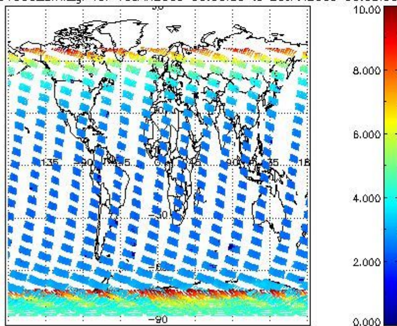
SCIOL2P_NADUV003_amf_gr for 19JAN2009 00:00:00 to 20JAN2009 00:00:00
