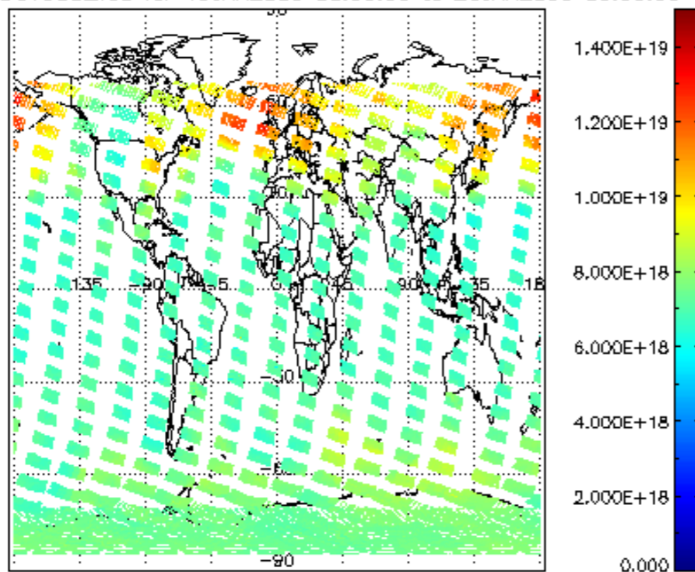
SCIOL2P_NADUV003_vcd for 19JAN2009 00:00:00 to 20JAN2009 00:00:00
