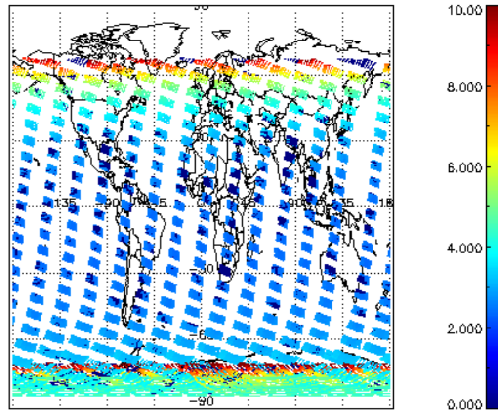
SCIOL2P_NADUV003_amf_cl for 19JAN2009 00:00:00 to 20JAN2009 00:00:00
