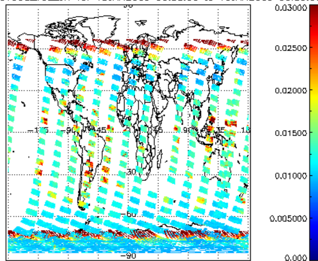
SCIOL2P_NADUV003_vcd_err for 15JAN2009 00:00:00 to 16JAN2009 00:00:00
