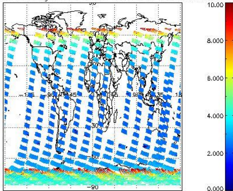
SCIOL2P_NADUV003_amf_gr for 15JAN2009 00:00:00 to 16JAN2009 00:00:00
