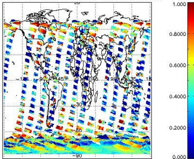
cL_frac for 15JAN2009 00:00:00 to 16JAN2009 00:00:00
