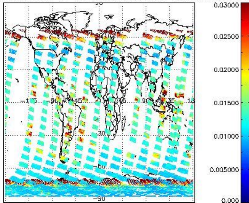
SCIOL2P_NADUV003_vcd_err for 15JAN2009 00:00:00 to 16JAN2009 00:00:00
