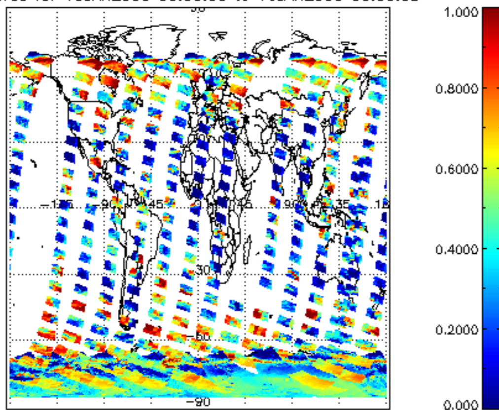
cL_frac for 15JAN2009 00:00:00 to 16JAN2009 00:00:00
