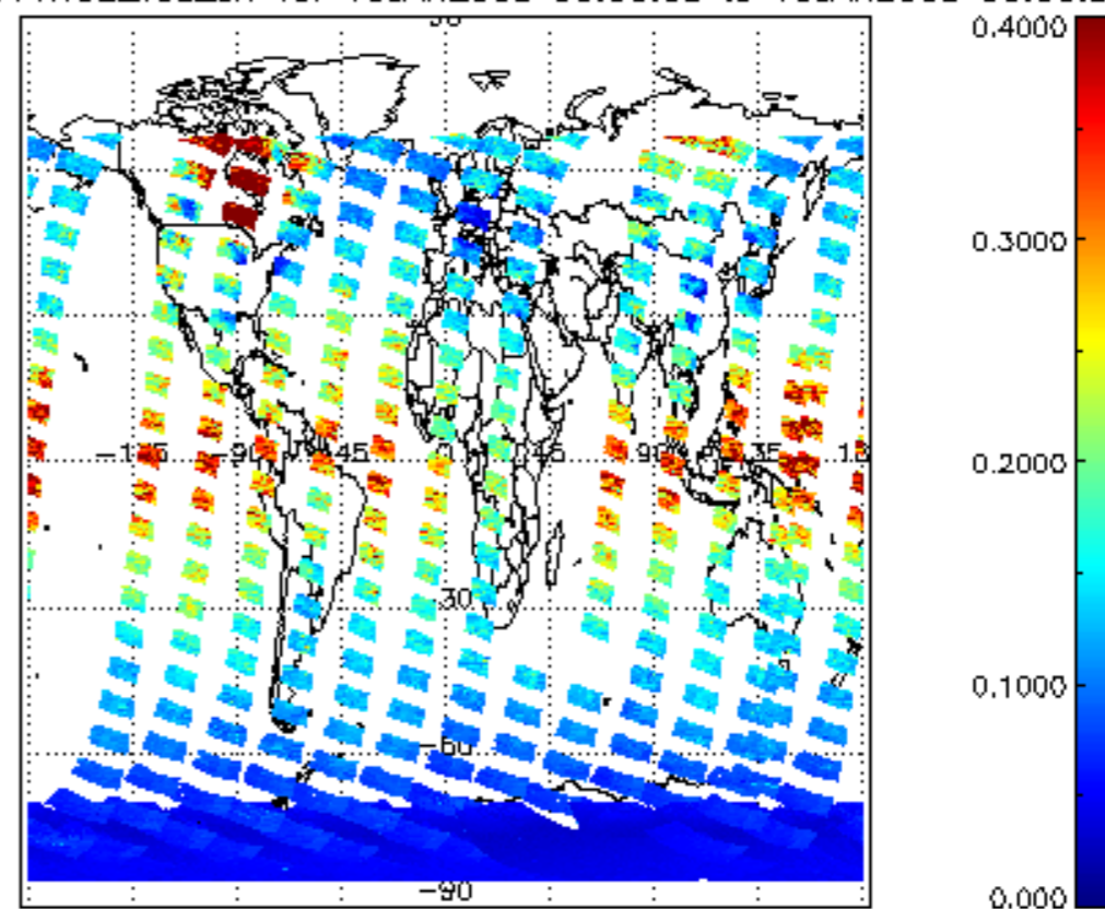
SCIOL2P_NADUV1NO2_vcd_err for 15JAN2009 00:00:00 to 16JAN2009 00:00:00
