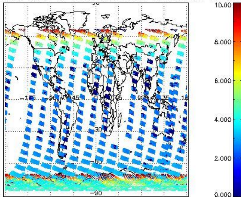
SCIOL2P_NADUV003_amf_cl for 15JAN2009 00:00:00 to 16JAN2009 00:00:00
