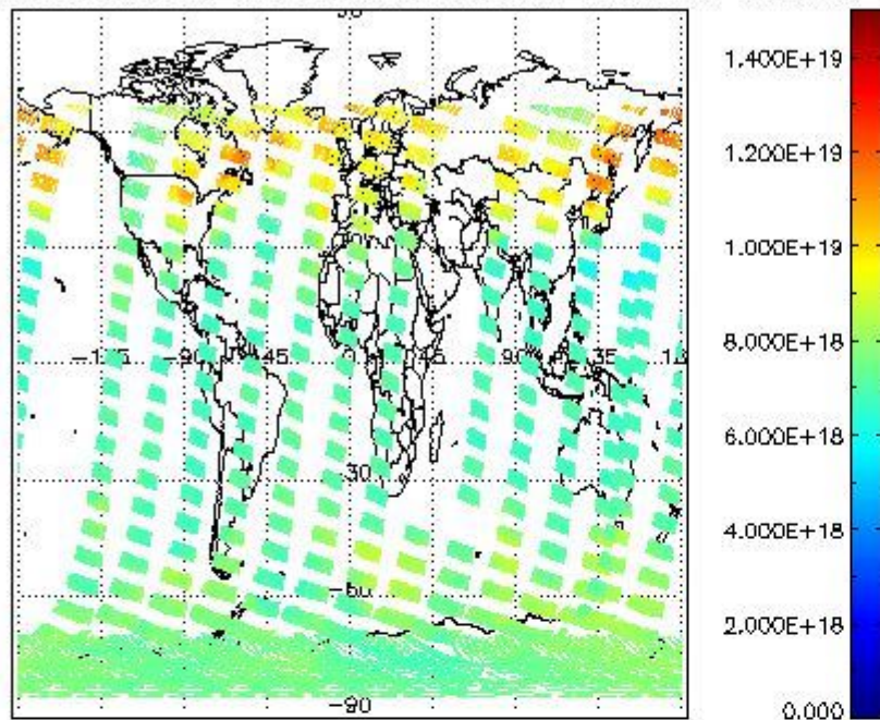
SCIOL2P_NADUV003_vcd for 15JAN2009 00:00:00 to 16JAN2009 00:00:00
