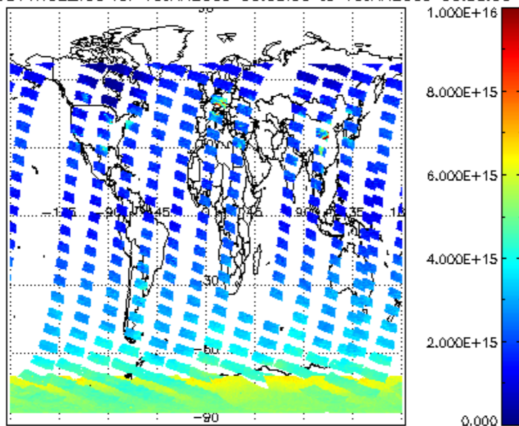
SCIOL2P_NADUV1NO2_vcd for 15JAN2009 00:00:00 to 16JAN2009 00:00:00
