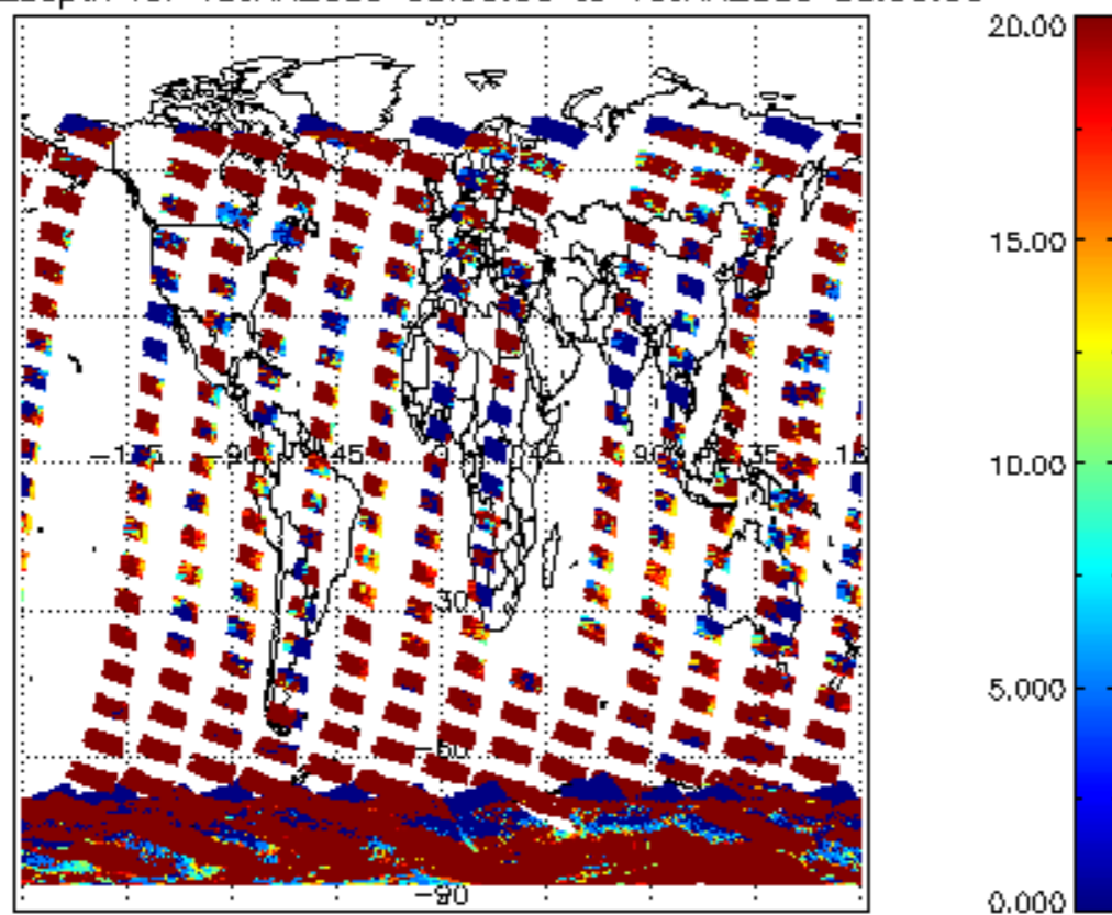
cLopt_depth for 15JAN2009 00:00:00 to 16JAN2009 00:00:00
