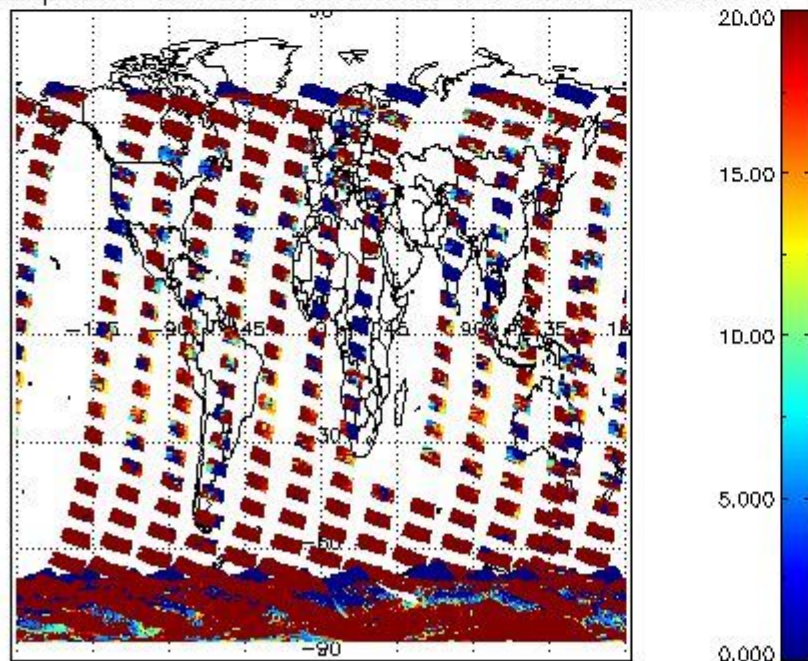
cLopt_depth for 15JAN2009 00:00:00 to 16JAN2009 00:00:00
