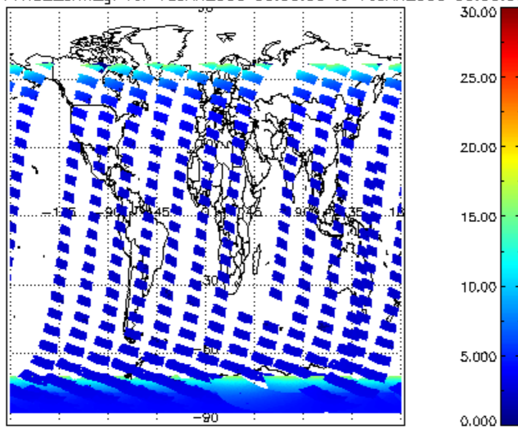
SCIOL2P_NADUV1NO2_amf_gr for 15JAN2009 00:00:00 to 16JAN2009 00:00:00
