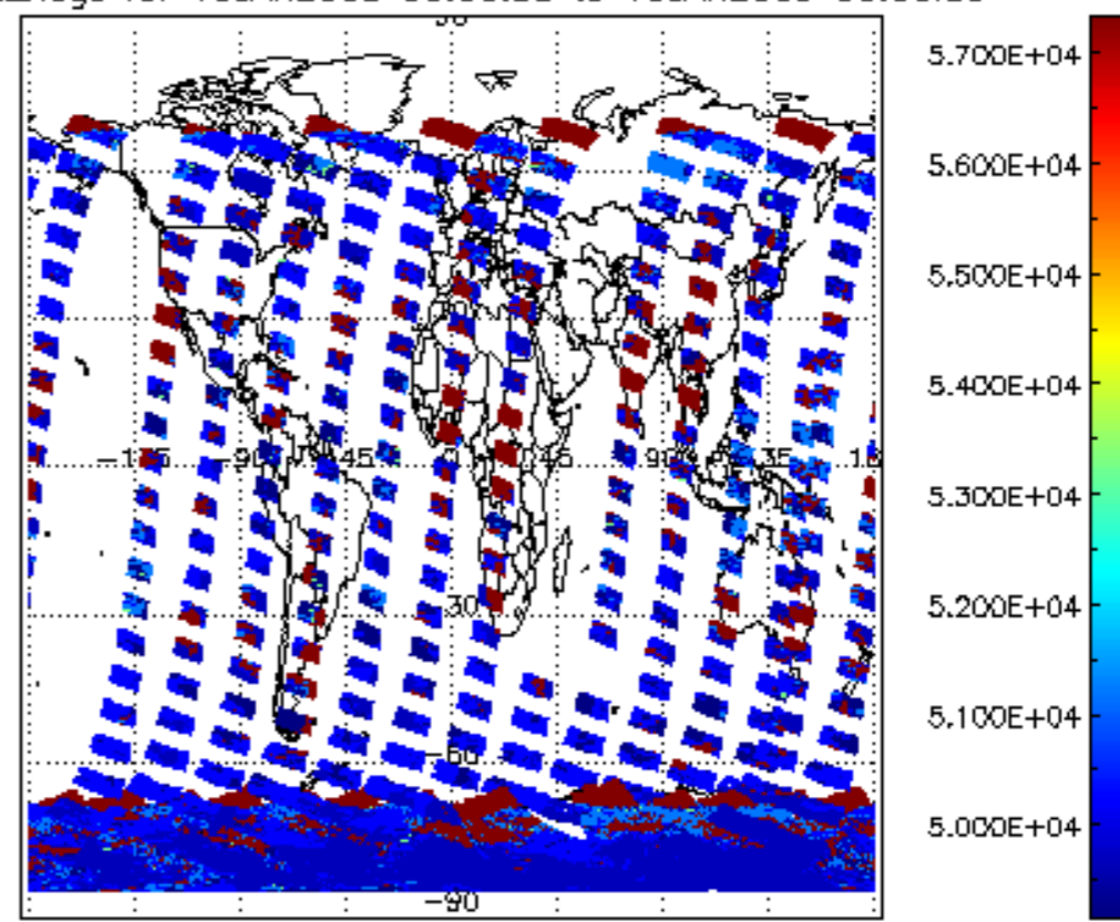
cloud_flags for 15JAN2009 00:00:00 to 16JAN2009 00:00:00
