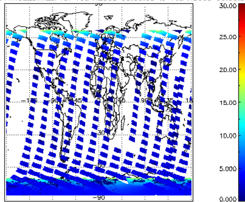
SCIOL2P_NADUV1NO2_amf_cl for 15JAN2009 00:00:00 to 16JAN2009 00:00:00
