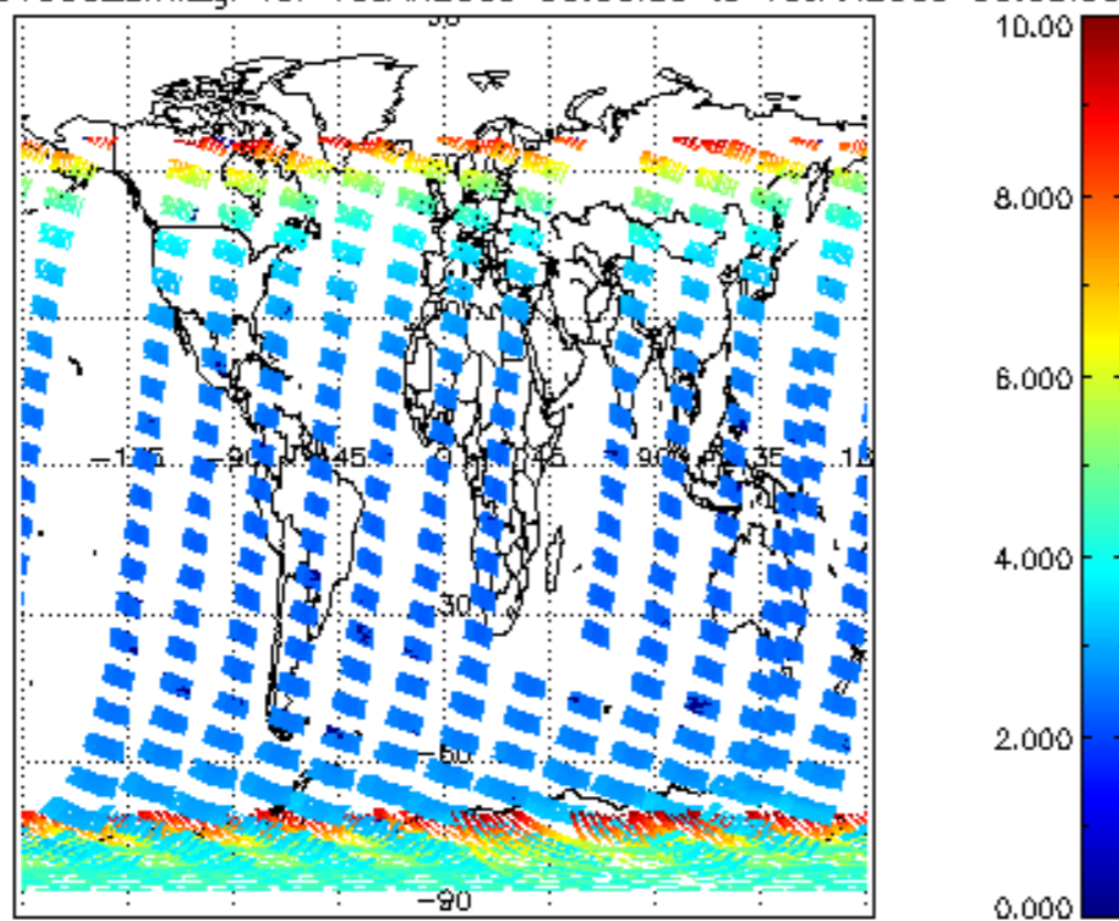
SCIOL2P_NADUV003_amf_gr for 15JAN2009 00:00:00 to 16JAN2009 00:00:00
