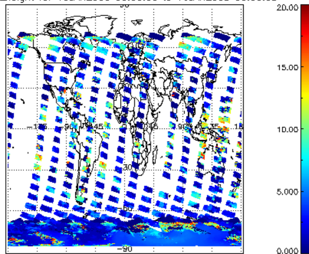
cL_top_height for 15JAN2009 00:00:00 to 16JAN2009 00:00:00
