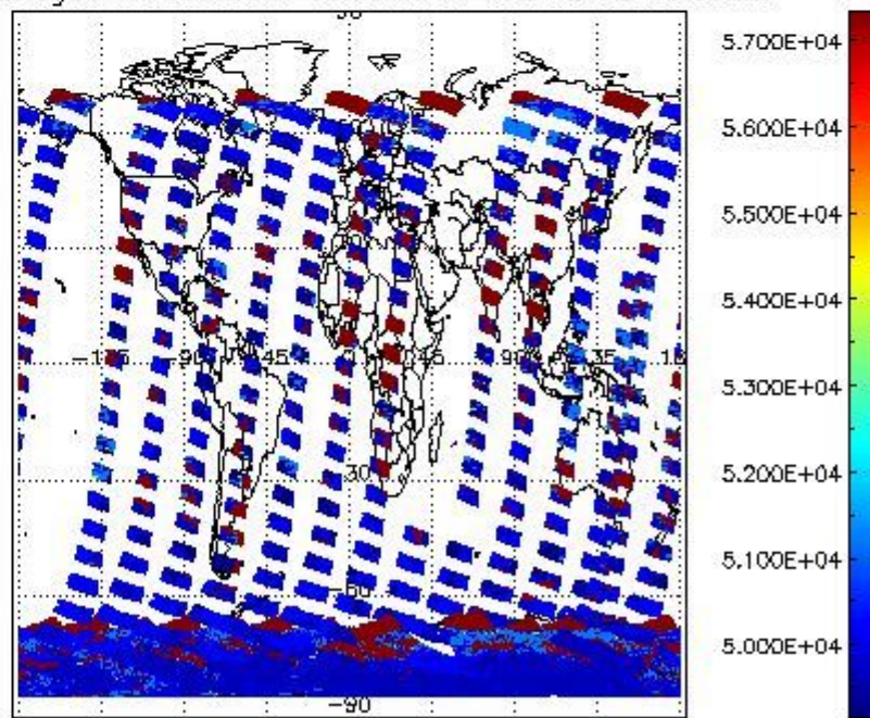
cloud_flags for 15JAN2009 00:00:00 to 16JAN2009 00:00:00
