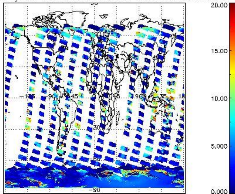
cL_top_height for 15JAN2009 00:00:00 to 16JAN2009 00:00:00
