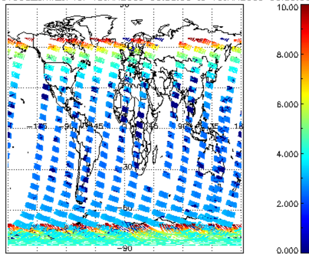
SCIOL2P_NADUV003_amf_cl for 15JAN2009 00:00:00 to 16JAN2009 00:00:00
