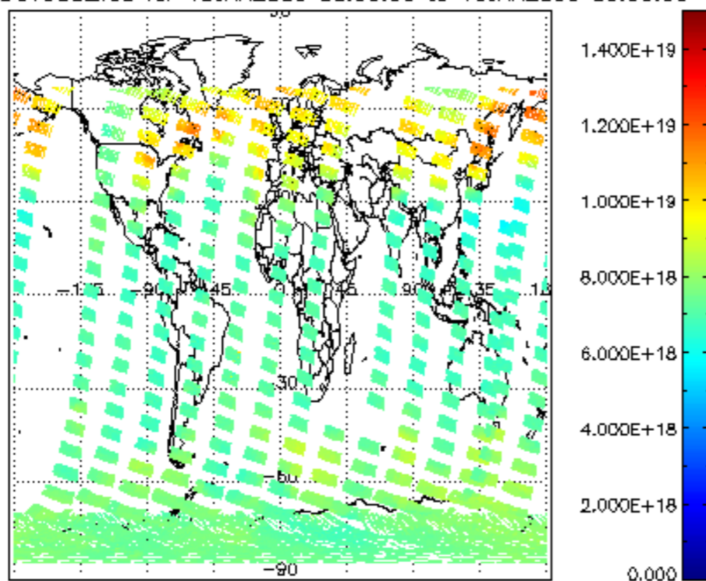
SCIOL2P_NADUV003_vcd for 15JAN2009 00:00:00 to 16JAN2009 00:00:00
