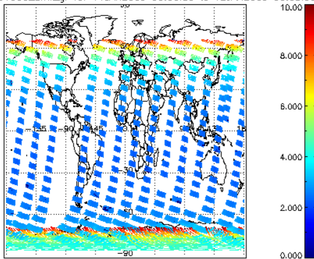
SCIOL2P_NADUV003_amf_gr for 11JAN2009 00:00:00 to 12JAN2009 00:00:00
