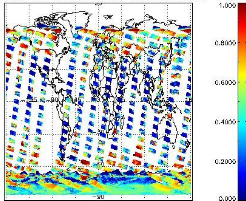
cL_frac for 11JAN2009 00:00:00 to 12JAN2009 00:00:00
