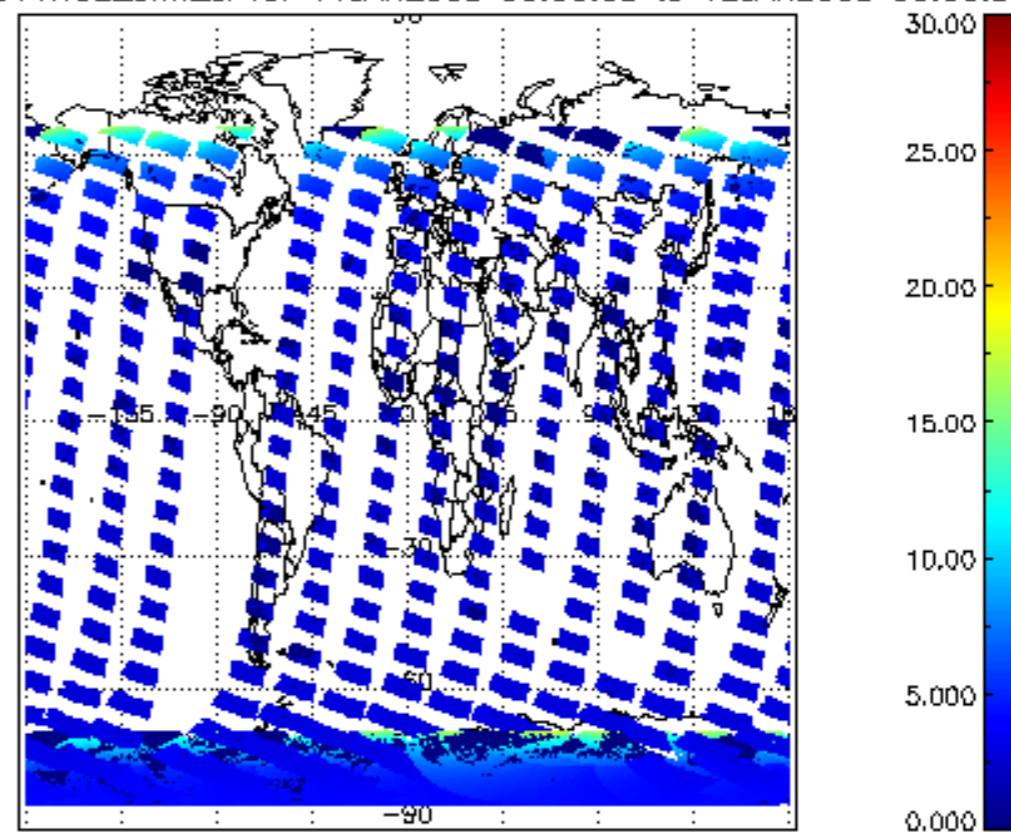
SCIOL2P_NADUV1NO2_amf_cl for 11JAN2009 00:00:00 to 12JAN2009 00:00:00
