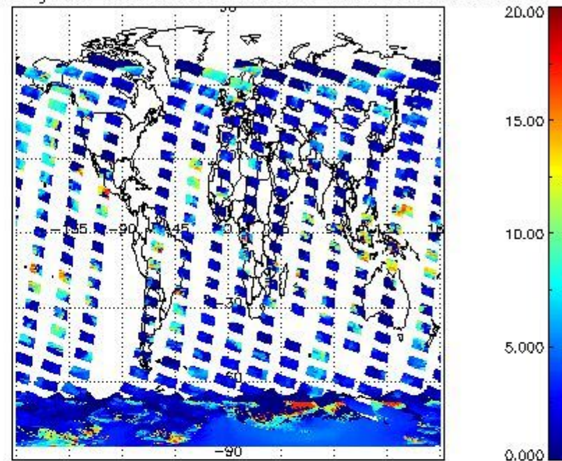
cL_top_height for 11JAN2009 00:00:00 to 12JAN2009 00:00:00
