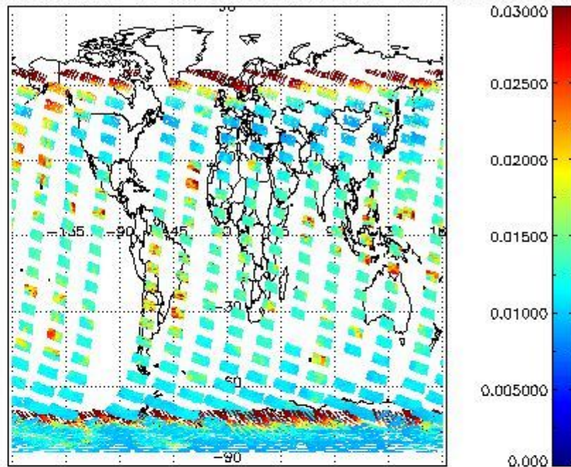
SCIOL2P_NADUV003_vcd_err for 11JAN2009 00:00:00 to 12JAN2009 00:00:00
