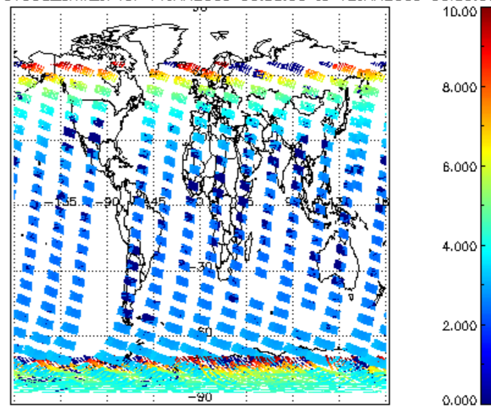
SCIOL2P_NADUV003_amf_cl for 11JAN2009 00:00:00 to 12JAN2009 00:00:00
