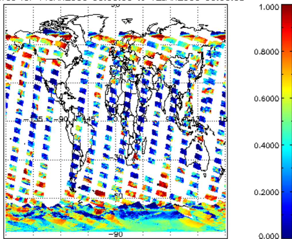
cL_frac for 11JAN2009 00:00:00 to 12JAN2009 00:00:00
