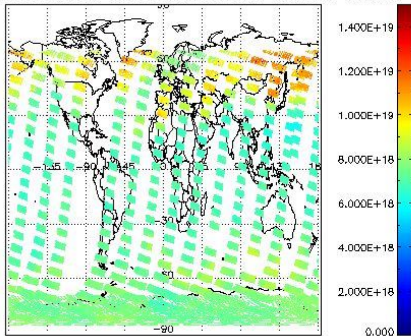
SCIOL2P_NADUV003_vcd for 11JAN2009 00:00:00 to 12JAN2009 00:00:00
