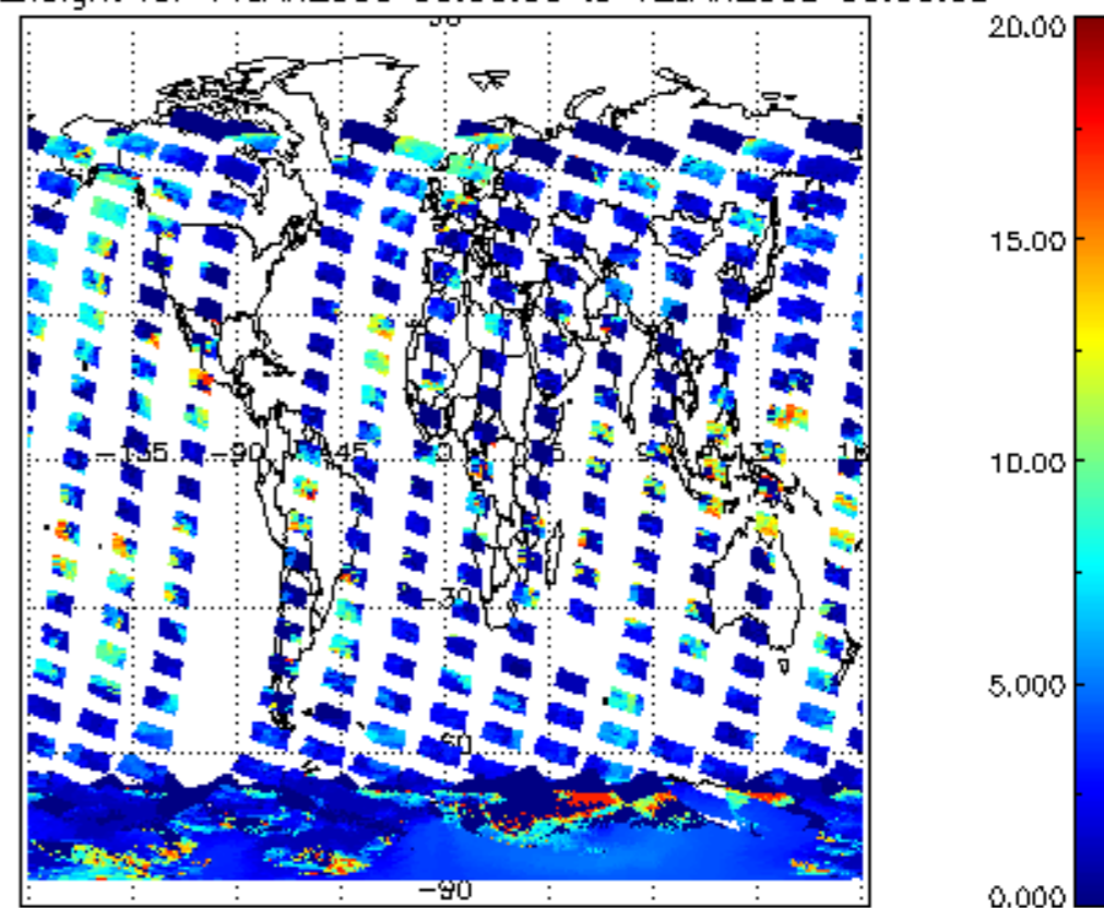
cL_top_height for 11JAN2009 00:00:00 to 12JAN2009 00:00:00
