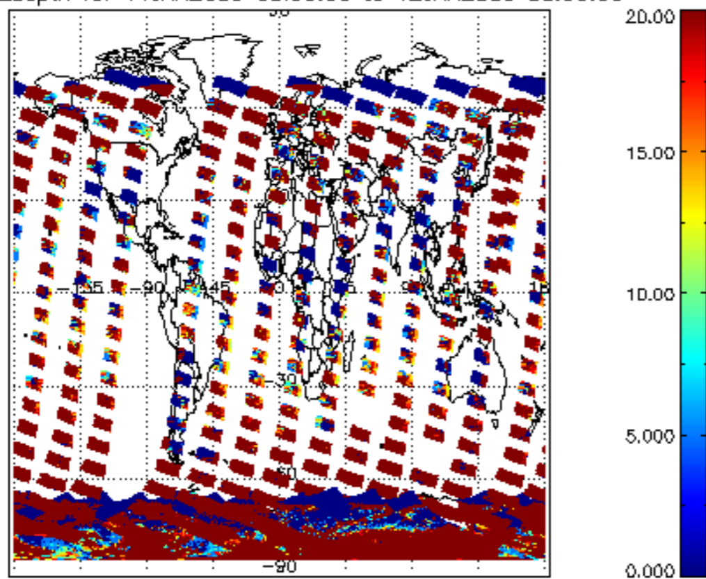
cLopt_depth for 11JAN2009 00:00:00 to 12JAN2009 00:00:00
