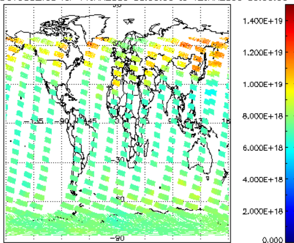
SCIOL2P_NADUV003_vcd for 11JAN2009 00:00:00 to 12JAN2009 00:00:00
