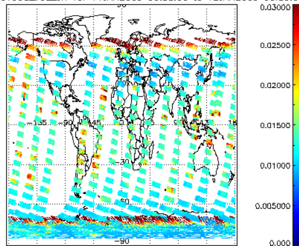
SCIOL2P_NADUV003_vcd_err for 11JAN2009 00:00:00 to 12JAN2009 00:00:00
