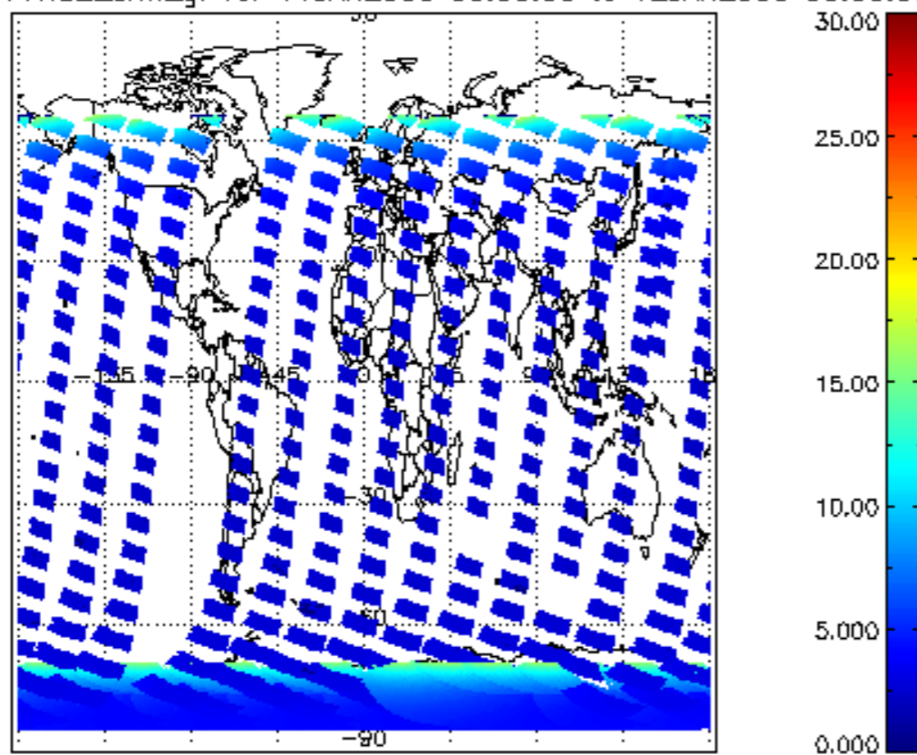
SCIOL2P_NADUV1NO2_amf_gr for 11JAN2009 00:00:00 to 12JAN2009 00:00:00
