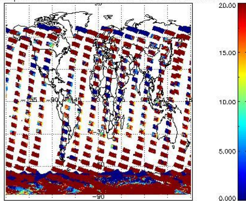
cLopt_depth for 11JAN2009 00:00:00 to 12JAN2009 00:00:00
