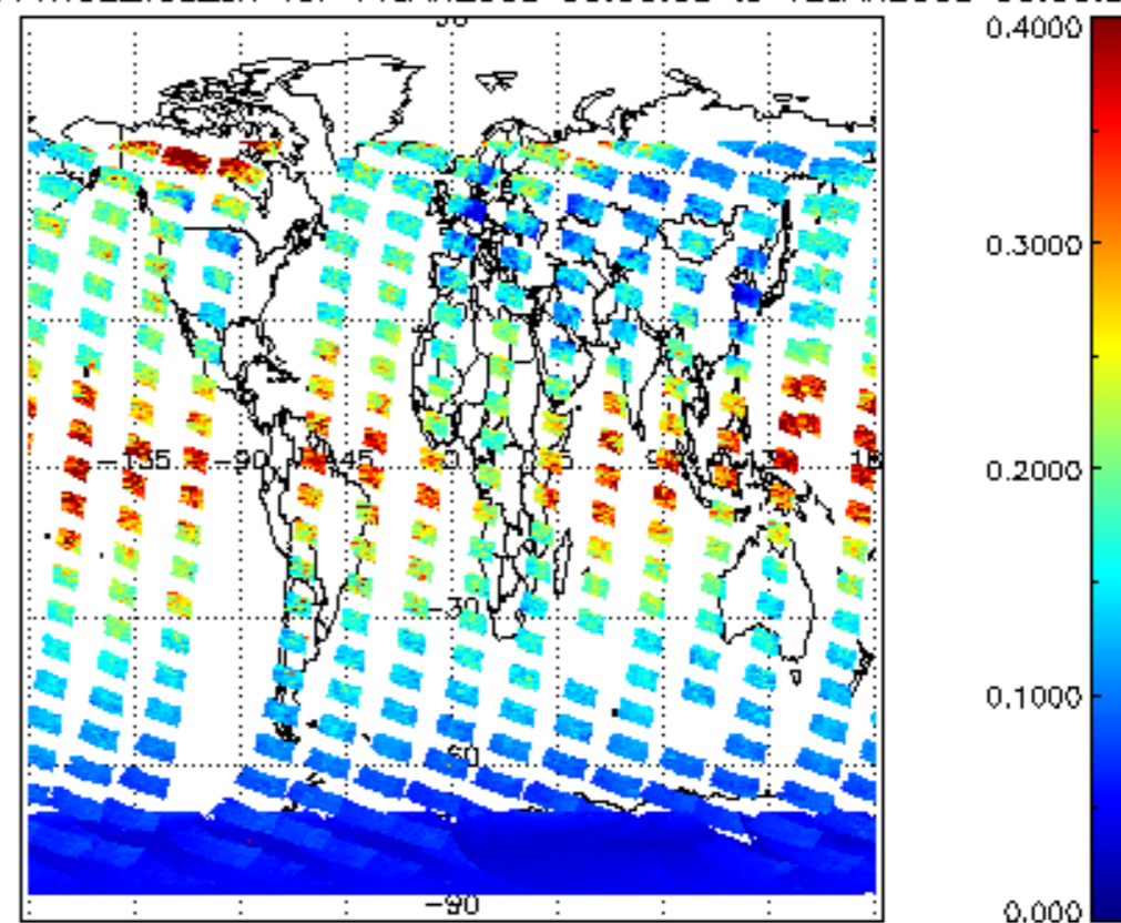
SCIOL2P_NADUV1NO2_vcd_err for 11JAN2009 00:00:00 to 12JAN2009 00:00:00
