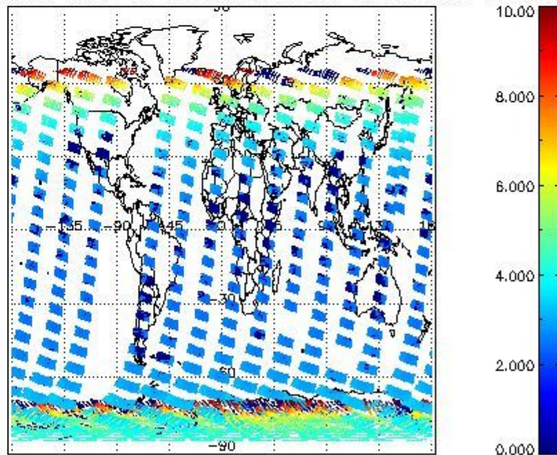
SCIOL2P_NADUV003_amf_cl for 11JAN2009 00:00:00 to 12JAN2009 00:00:00
