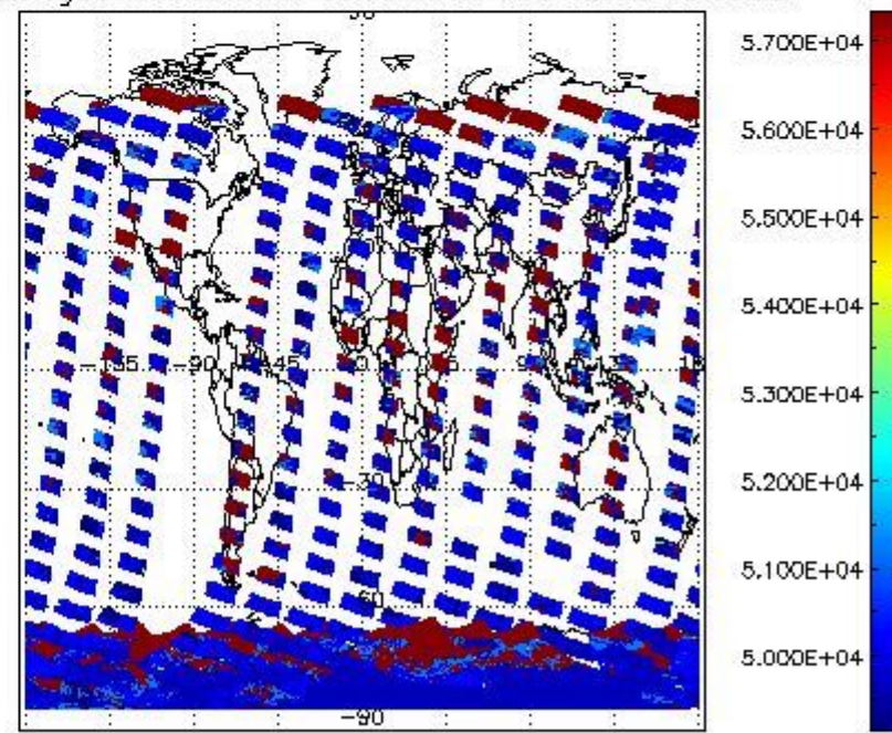
cloud_flags for 11JAN2009 00:00:00 to 12JAN2009 00:00:00
