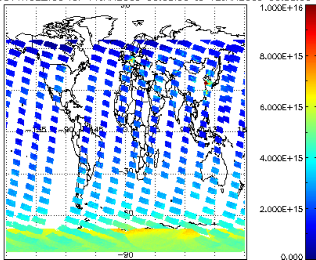
SCIOL2P_NADUV1NO2_vcd for 11JAN2009 00:00:00 to 12JAN2009 00:00:00
