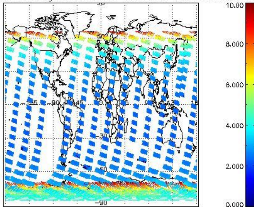
SCIOL2P_NADUV003_amf_gr for 11JAN2009 00:00:00 to 12JAN2009 00:00:00
