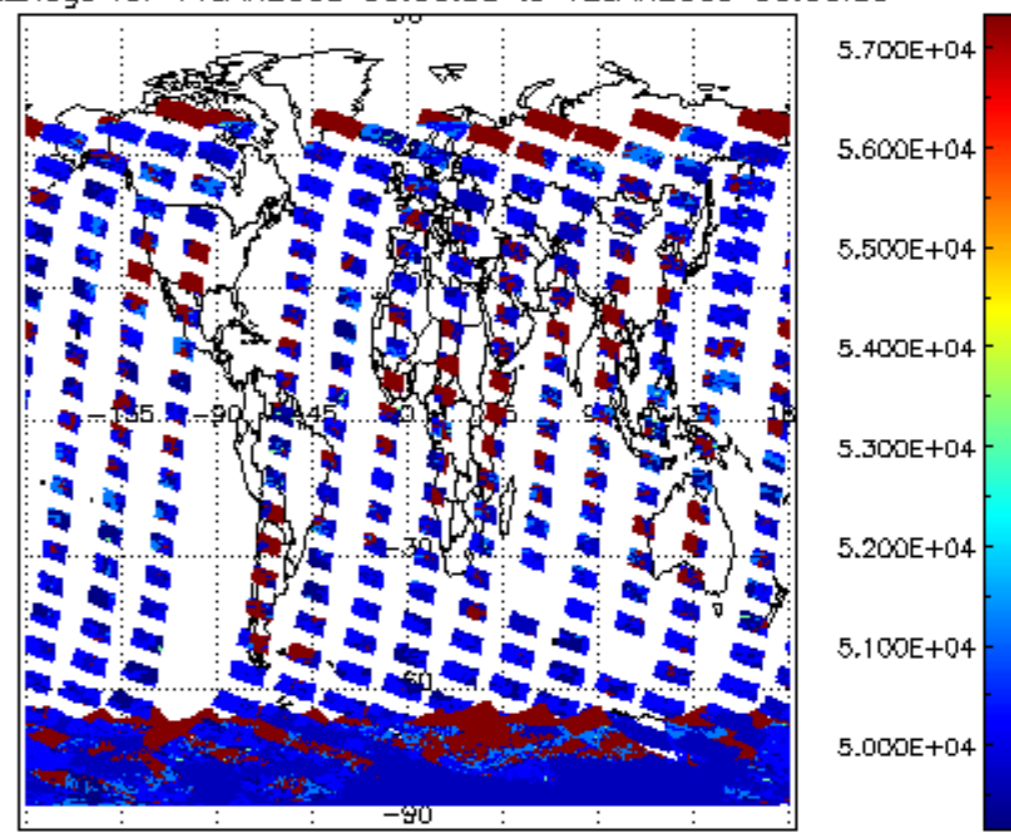
cloud_flags for 11JAN2009 00:00:00 to 12JAN2009 00:00:00
