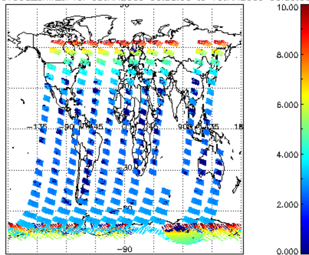
SCIOL2P_NADUV003_amf_cl for 09JAN2009 00:00:00 to 10JAN2009 00:00:00
