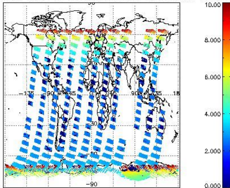
SCIOL2P_NADUV003_amf_cl for 09JAN2009 00:00:00 to 10JAN2009 00:00:00
