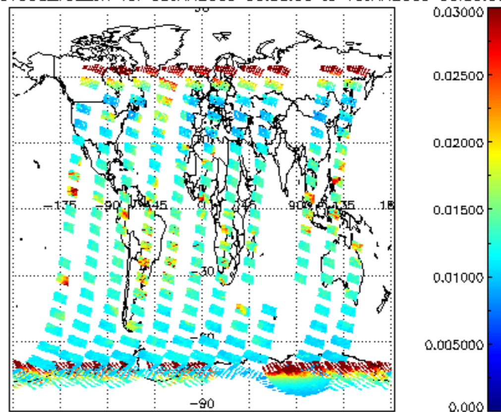
SCIOL2P_NADUV003_vcd_err for 09JAN2009 00:00:00 to 10JAN2009 00:00:00
