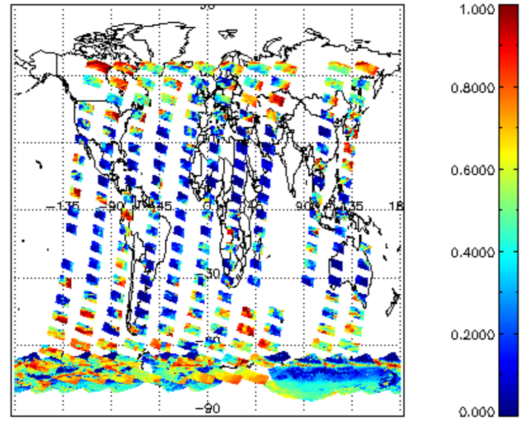
cL_frac for 09JAN2009 00:00:00 to 10JAN2009 00:00:00
