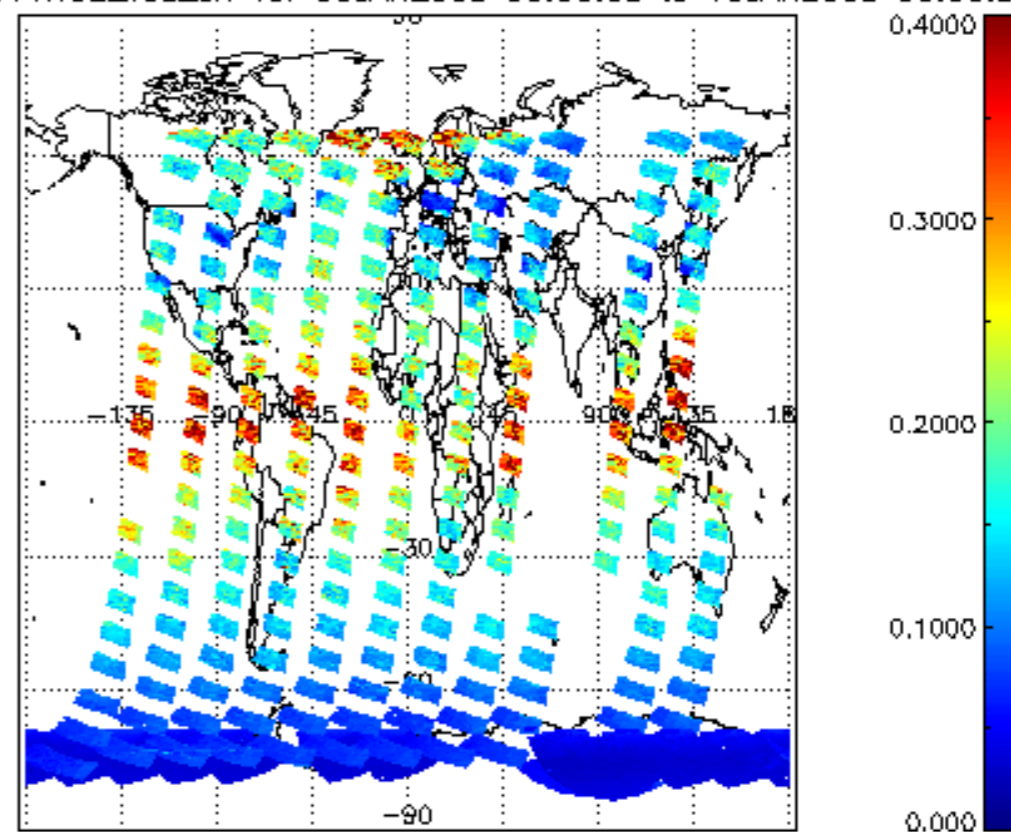
SCIOL2P_NADUV1NO2_vcd_err for 09JAN2009 00:00:00 to 10JAN2009 00:00:00
