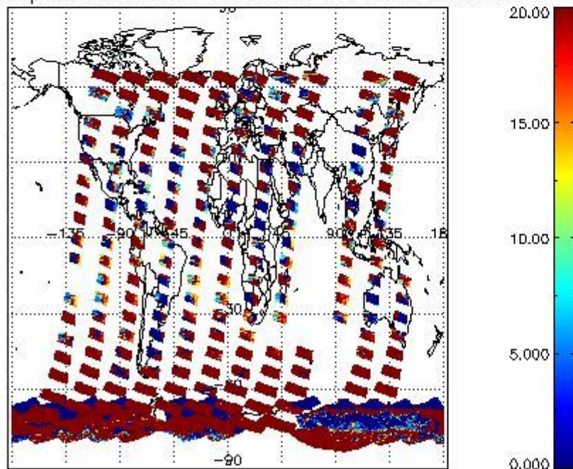
cLopt_depth for 09JAN2009 00:00:00 to 10JAN2009 00:00:00
