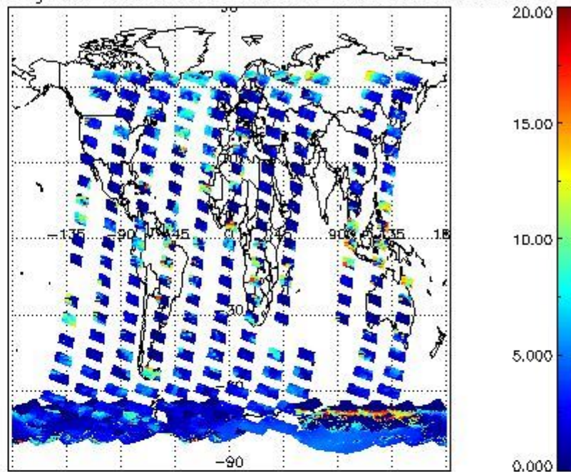
cL_top_height for 09JAN2009 00:00:00 to 10JAN2009 00:00:00
