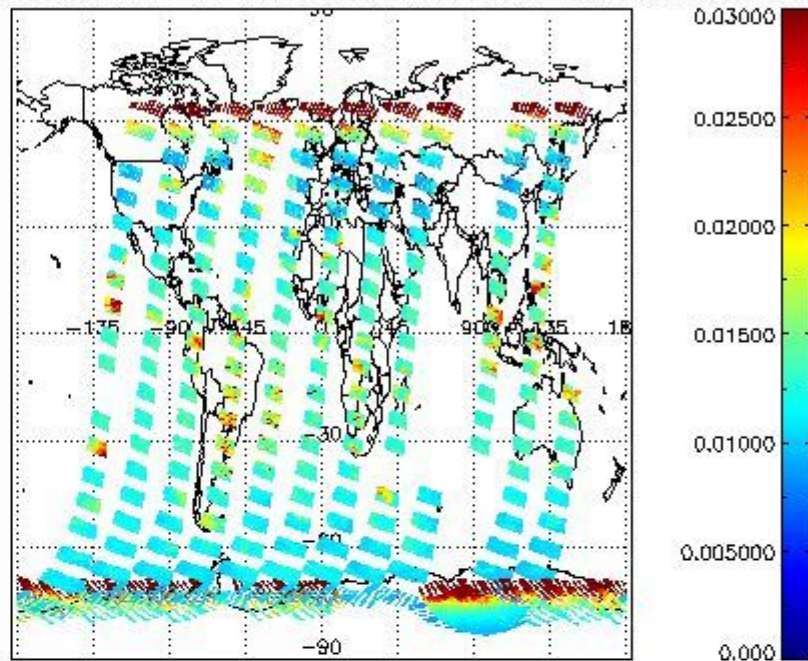
SCIOL2P_NADUV003_vcd_err for 09JAN2009 00:00:00 to 10JAN2009 00:00:00
