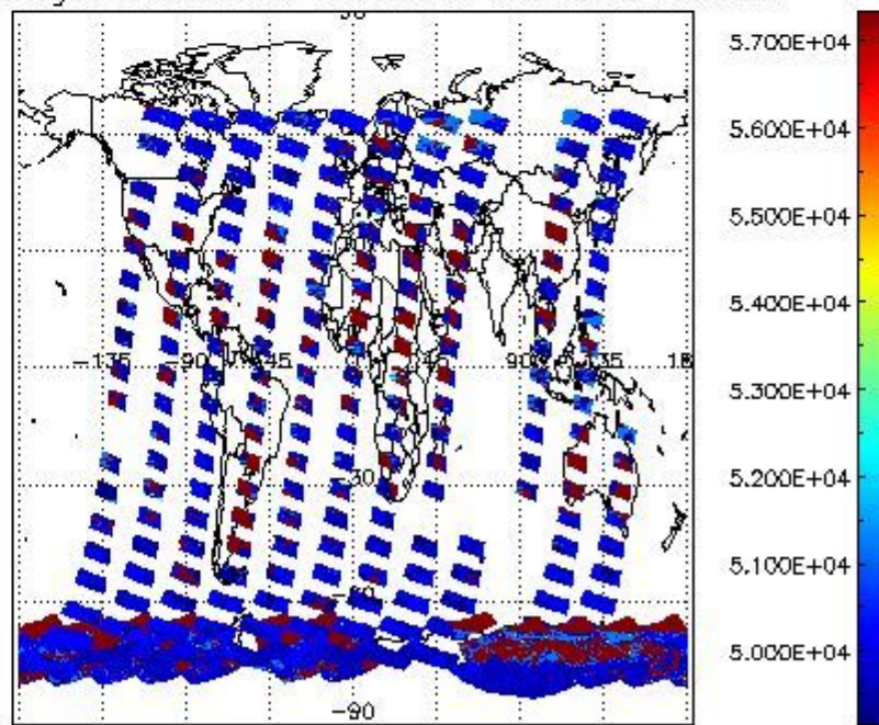
cloud_flags for 09JAN2009 00:00:00 to 10JAN2009 00:00:00
