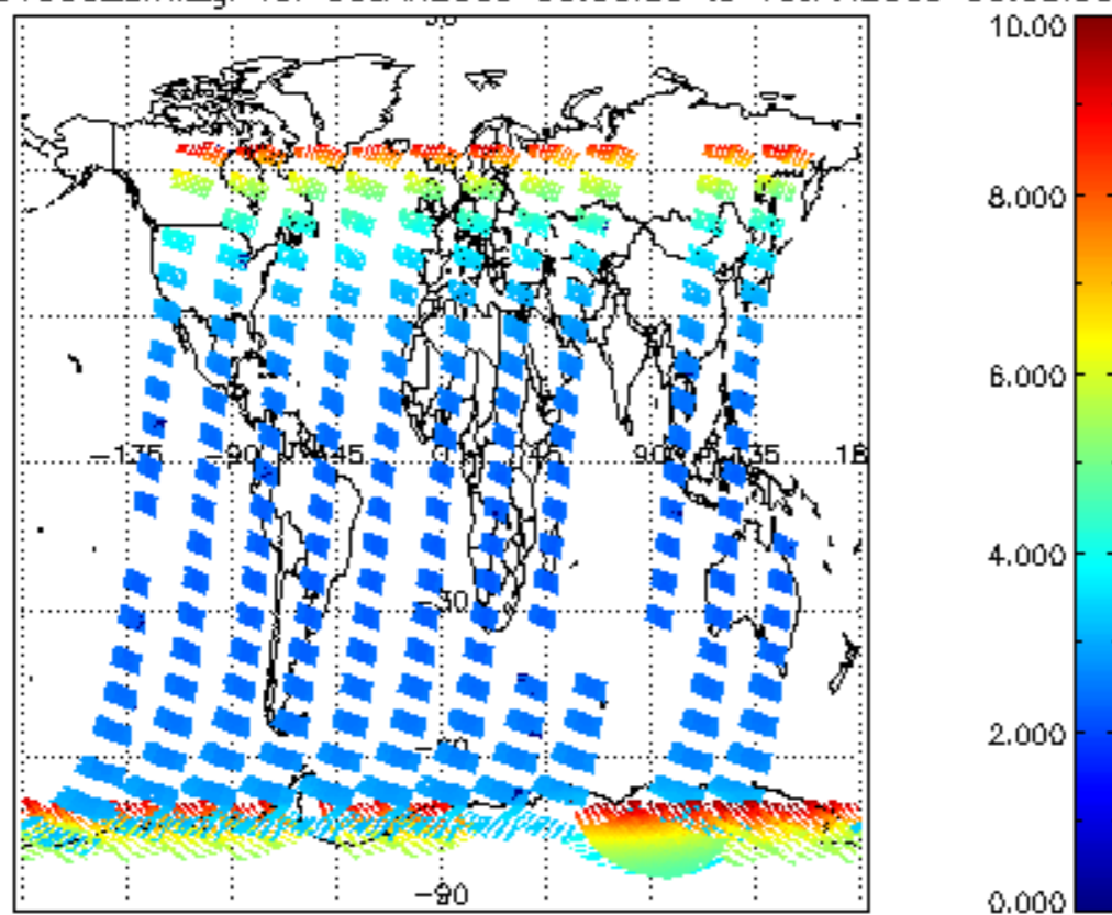
SCIOL2P_NADUV003_amf_gr for 09JAN2009 00:00:00 to 10JAN2009 00:00:00
