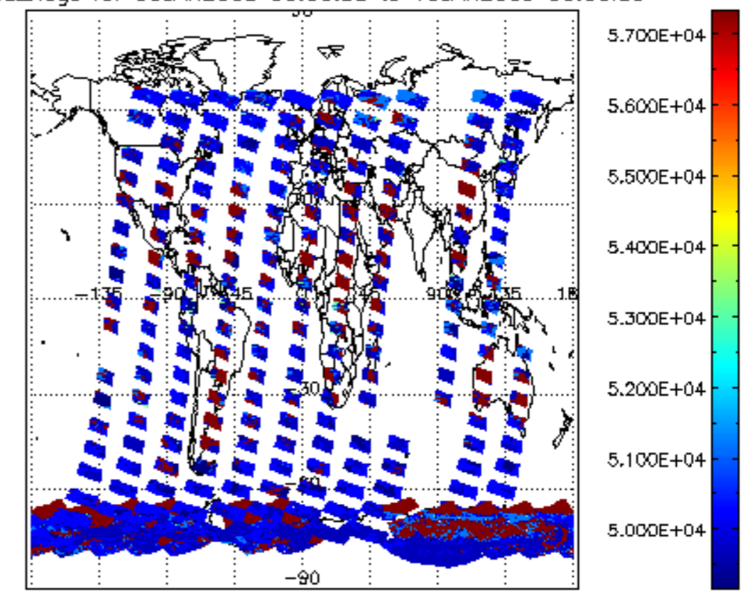
cloud_flags for 09JAN2009 00:00:00 to 10JAN2009 00:00:00
