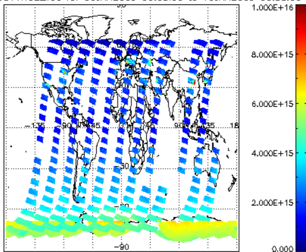
SCIOL2P_NADUV1NO2_vcd for 09JAN2009 00:00:00 to 10JAN2009 00:00:00
