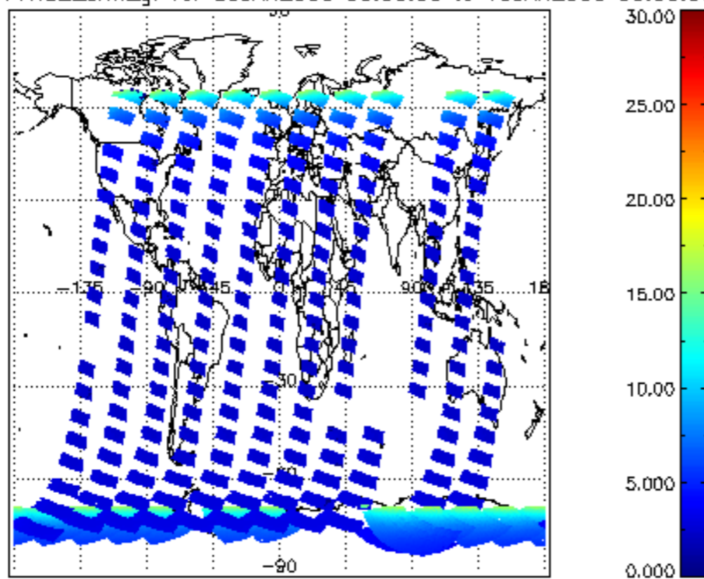
SCIOL2P_NADUV1NO2_amf_gr for 09JAN2009 00:00:00 to 10JAN2009 00:00:00
