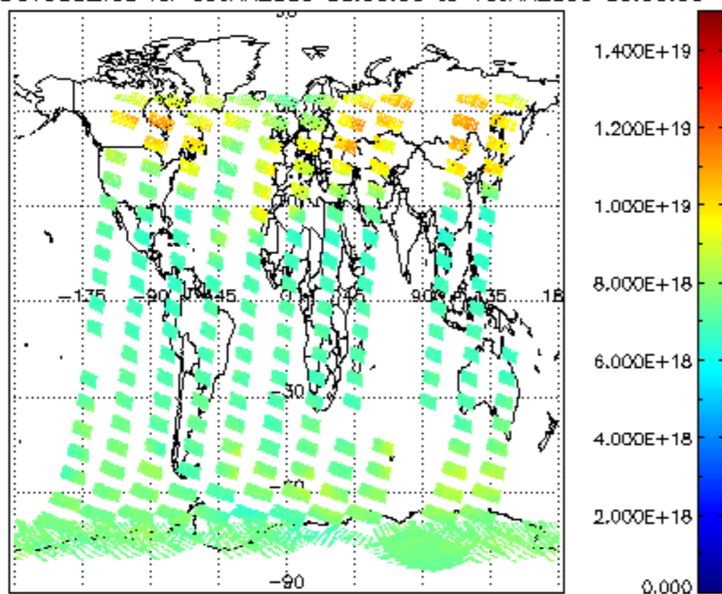
SCIOL2P_NADUV003_vcd for 09JAN2009 00:00:00 to 10JAN2009 00:00:00
