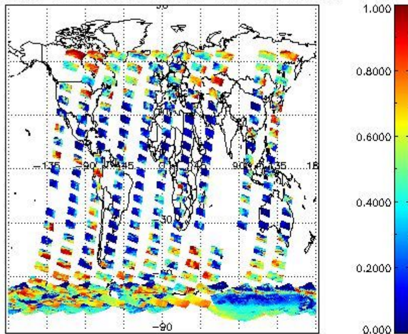
cL_frac for 09JAN2009 00:00:00 to 10JAN2009 00:00:00
