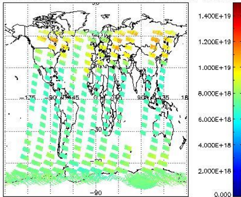
SCIOL2P_NADUV003_vcd for 09JAN2009 00:00:00 to 10JAN2009 00:00:00
