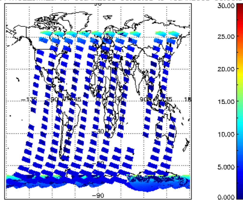
SCIOL2P_NADUV1NO2_amf_cl for 09JAN2009 00:00:00 to 10JAN2009 00:00:00
