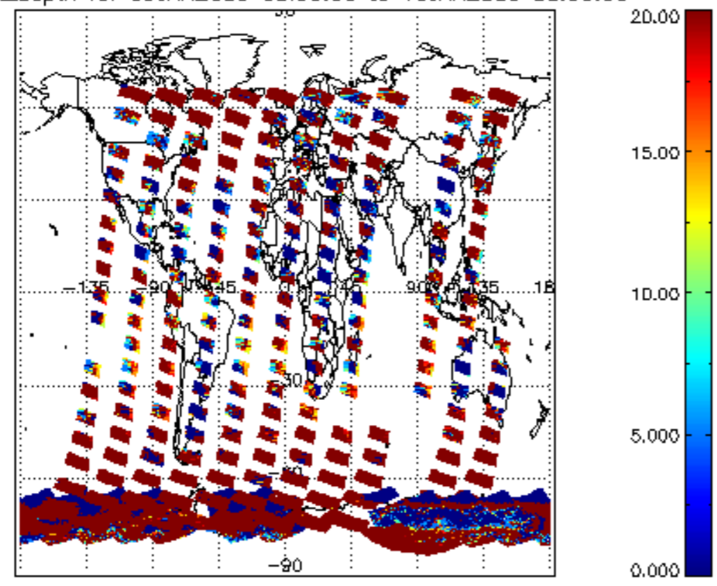
cLopt_depth for 09JAN2009 00:00:00 to 10JAN2009 00:00:00
