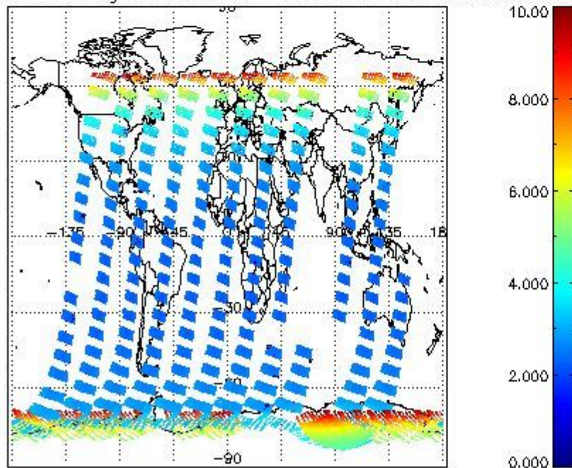
SCIOL2P_NADUV003_amf_gr for 09JAN2009 00:00:00 to 10JAN2009 00:00:00
