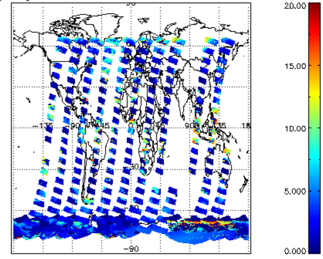
cL_top_height for 09JAN2009 00:00:00 to 10JAN2009 00:00:00
