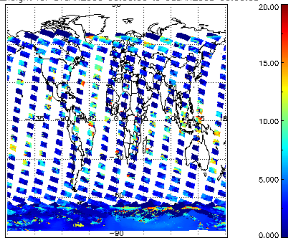
cL_top_height for 07JAN2009 00:00:00 to 08JAN2009 00:00:00
