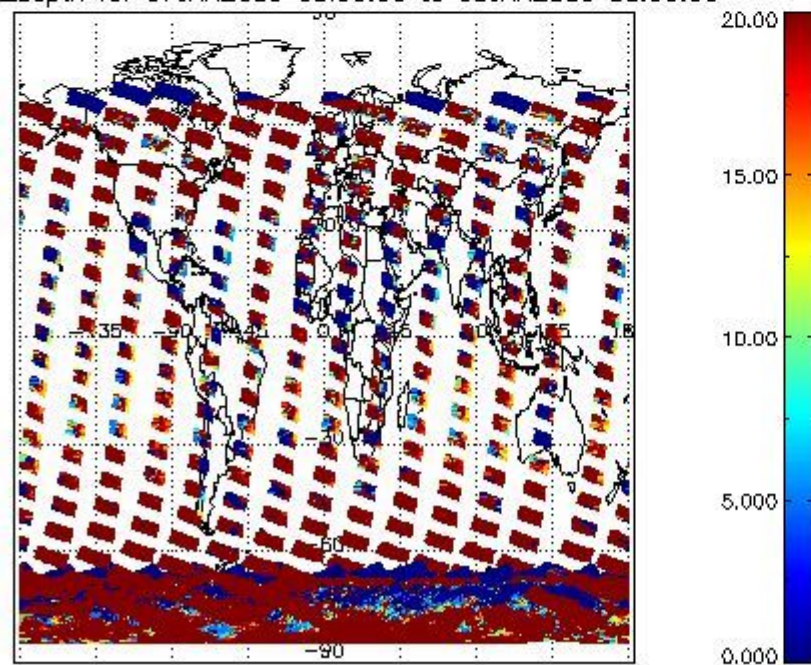
cLopt_depth for 07JAN2009 00:00:00 to 08JAN2009 00:00:00
