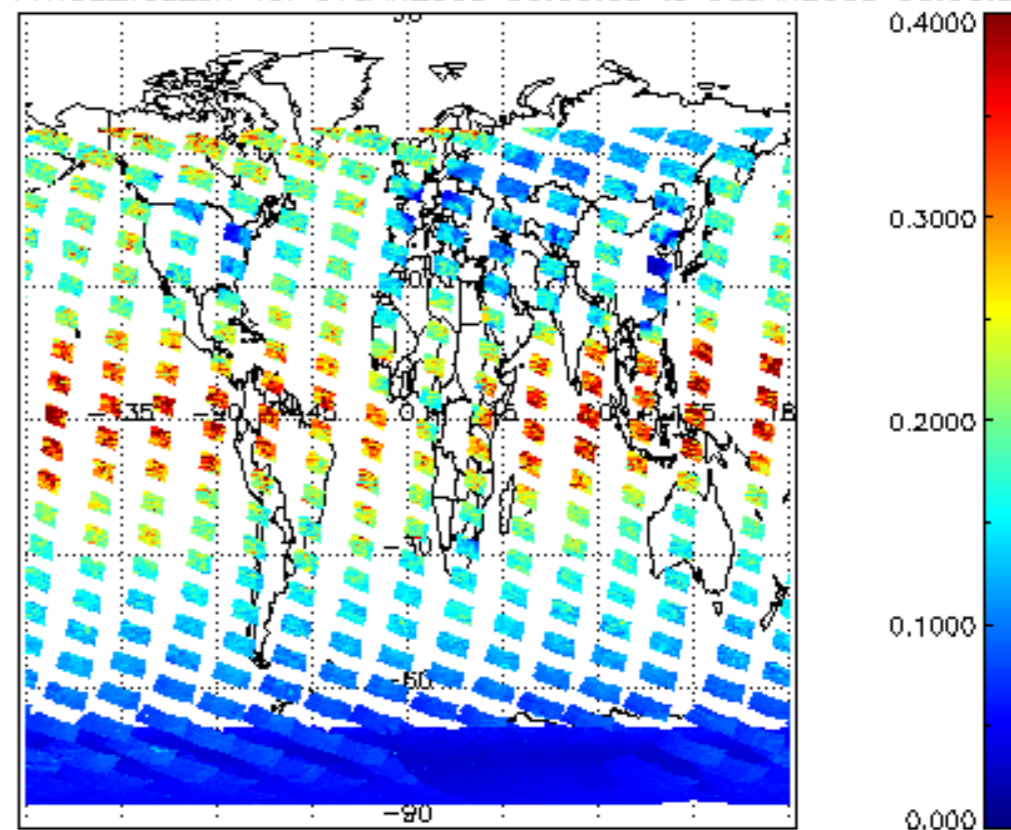
SCIOL2P_NADUV1NO2_vcd_err for 07JAN2009 00:00:00 to 08JAN2009 00:00:00
