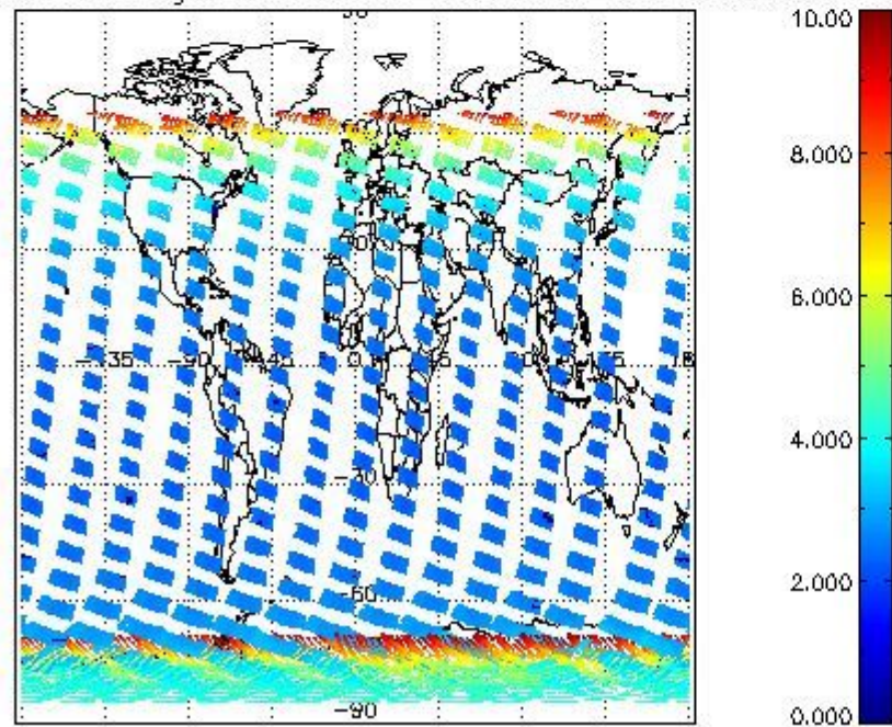
SCIOL2P_NADUV003_amf_gr for 07JAN2009 00:00:00 to 08JAN2009 00:00:00
