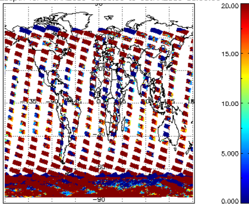
cLopt_depth for 07JAN2009 00:00:00 to 08JAN2009 00:00:00
