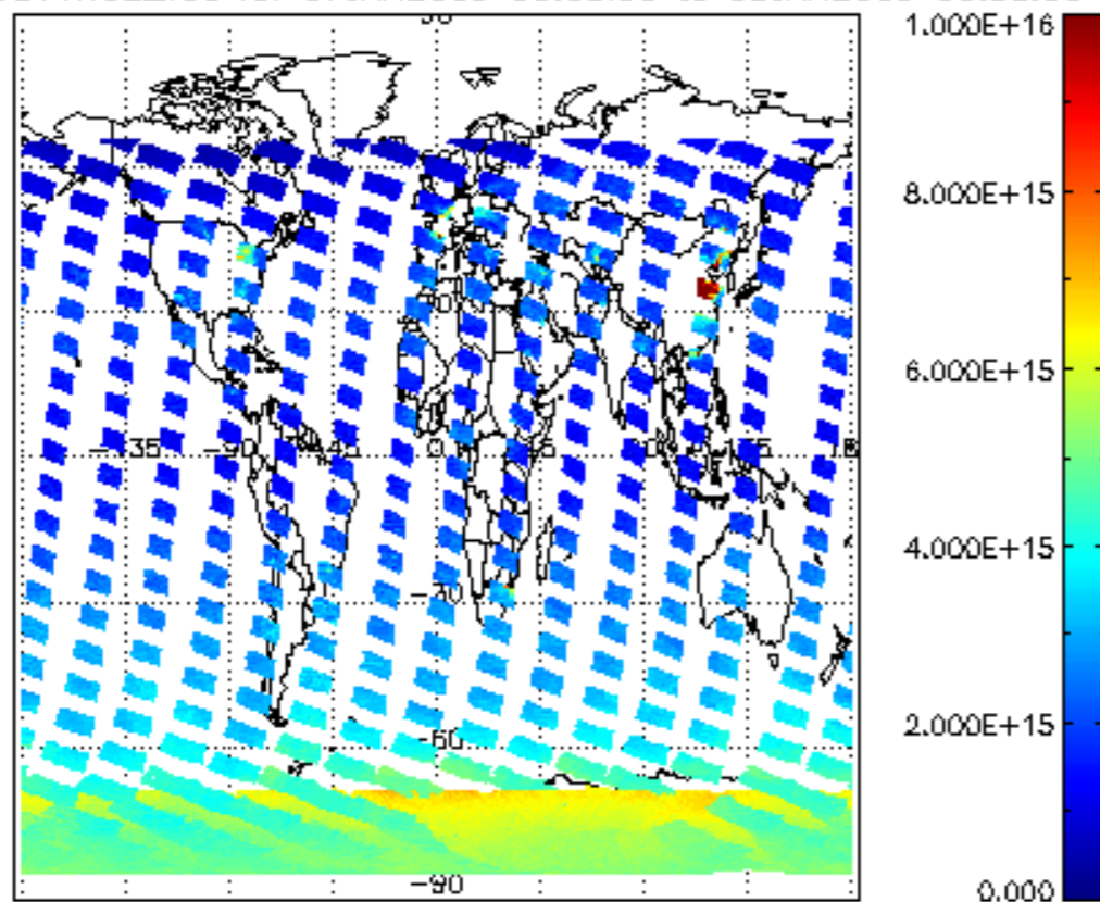
SCIOL2P_NADUV1NO2_vcd for 07JAN2009 00:00:00 to 08JAN2009 00:00:00
