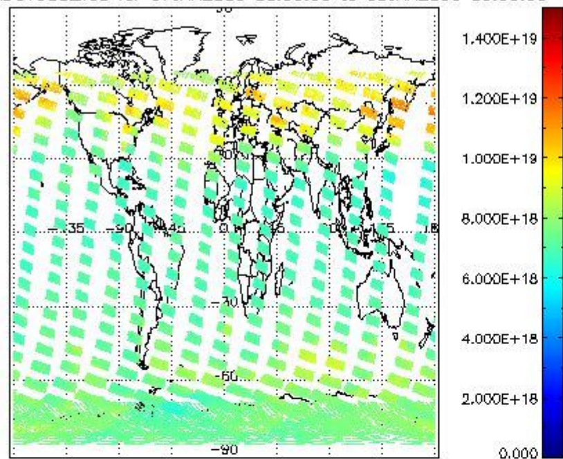
SCIOL2P_NADUV003_vcd for 07JAN2009 00:00:00 to 08JAN2009 00:00:00
