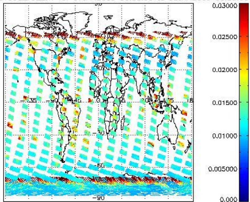
SCIOL2P_NADUV003_vcd_err for 07JAN2009 00:00:00 to 08JAN2009 00:00:00
