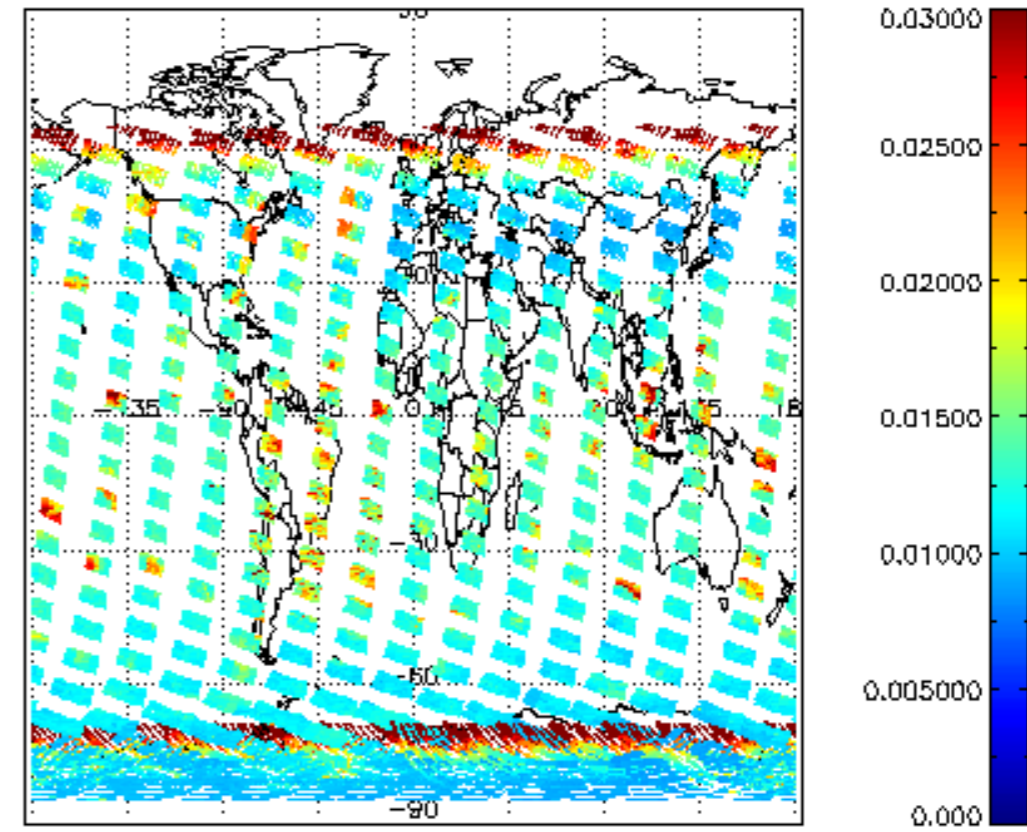
SCIOL2P_NADUV003_vcd_err for 07JAN2009 00:00:00 to 08JAN2009 00:00:00
