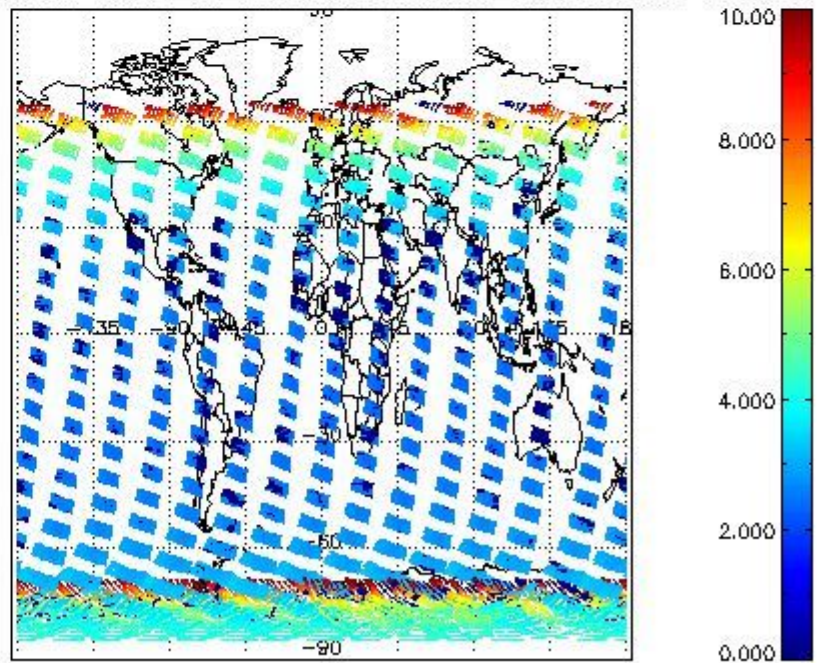
SCIOL2P_NADUV003_amf_cl for 07JAN2009 00:00:00 to 08JAN2009 00:00:00
