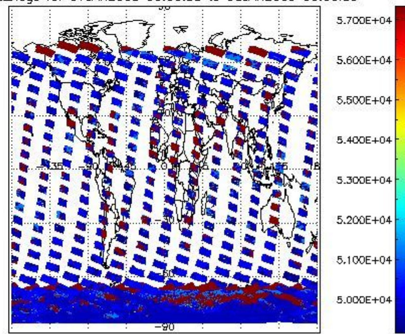
cloud_flags for 07JAN2009 00:00:00 to 08JAN2009 00:00:00
