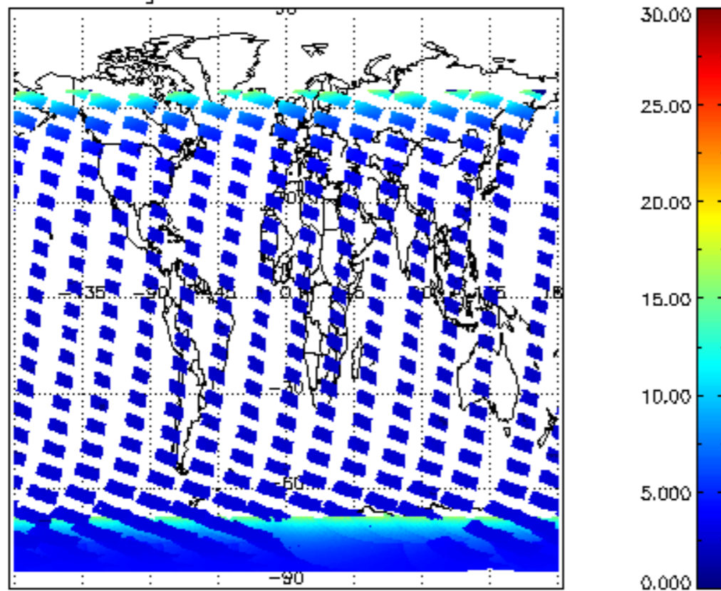
SCIOL2P_NADUV1NO2_amf_gr for 07JAN2009 00:00:00 to 08JAN2009 00:00:00
