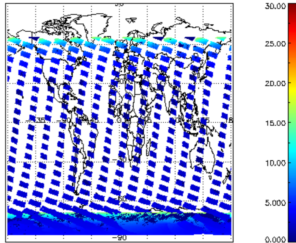
SCIOL2P_NADUV1NO2_amf_cl for 07JAN2009 00:00:00 to 08JAN2009 00:00:00
