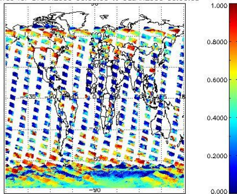
cL_frac for 07JAN2009 00:00:00 to 08JAN2009 00:00:00
