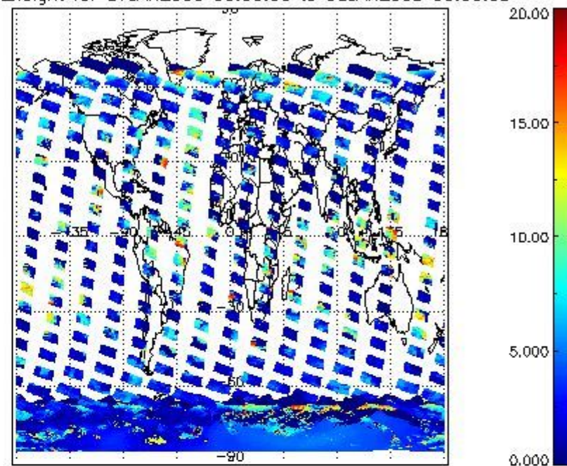
cL_top_height for 07JAN2009 00:00:00 to 08JAN2009 00:00:00
