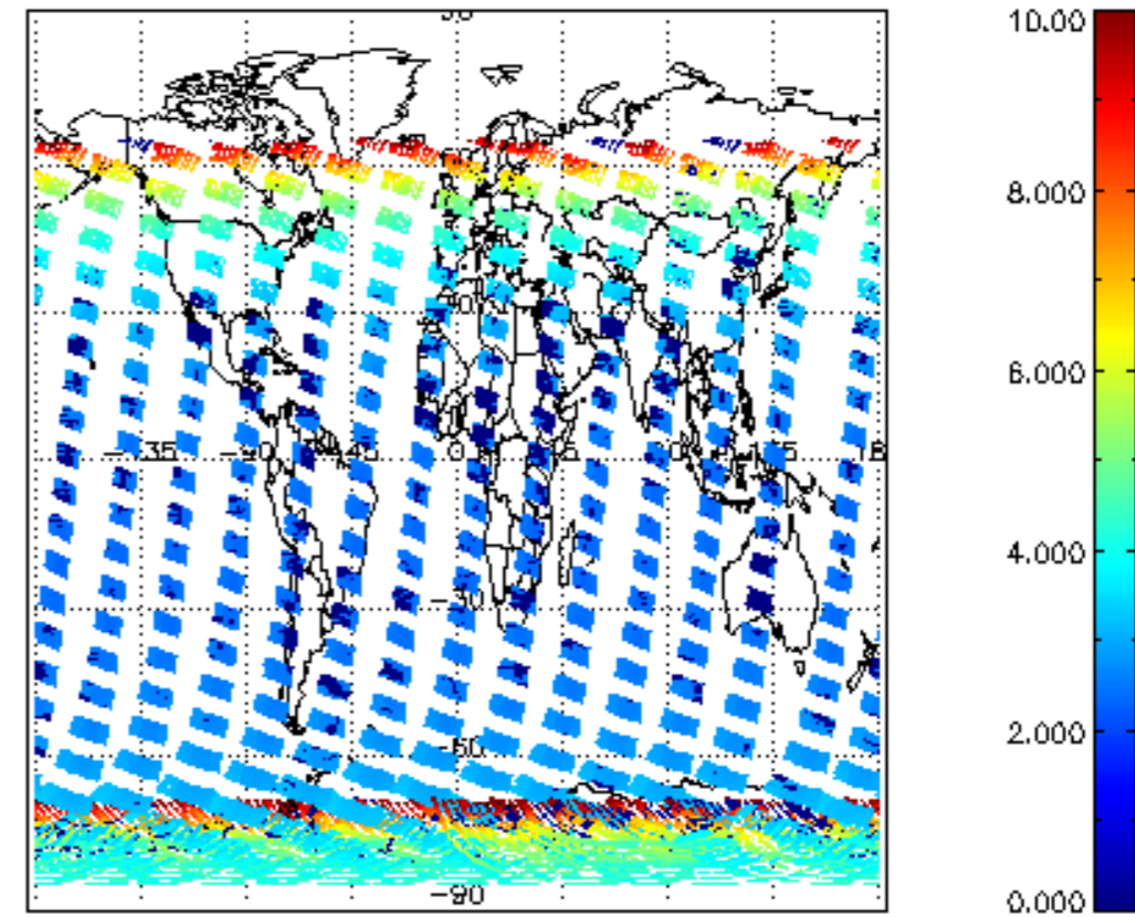
SCIOL2P_NADUV003_amf_cl for 07JAN2009 00:00:00 to 08JAN2009 00:00:00
