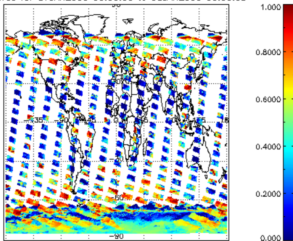
cL_frac for 07JAN2009 00:00:00 to 08JAN2009 00:00:00
