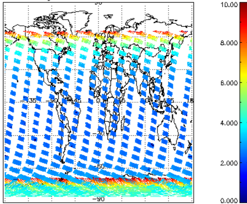
SCIOL2P_NADUV003_amf_gr for 07JAN2009 00:00:00 to 08JAN2009 00:00:00
