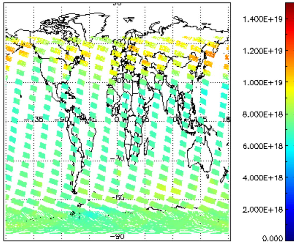
SCIOL2P_NADUV003_vcd for 07JAN2009 00:00:00 to 08JAN2009 00:00:00
