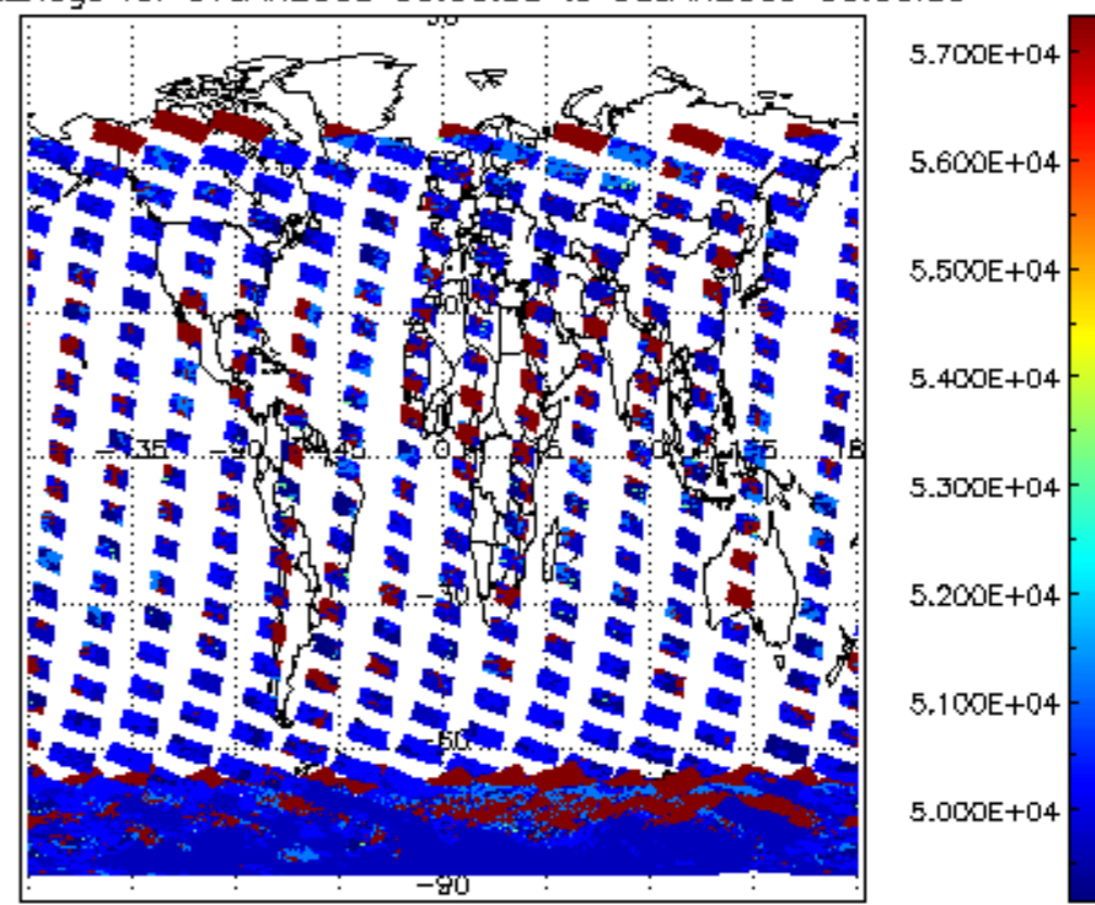
cloud_flags for 07JAN2009 00:00:00 to 08JAN2009 00:00:00
