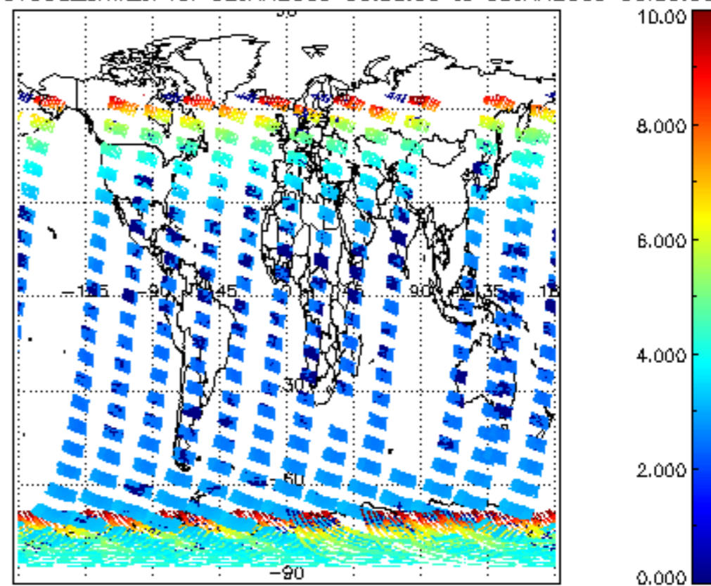
SCIOL2P_NADUV003_amf_cl for 02JAN2009 00:00:00 to 03JAN2009 00:00:00
