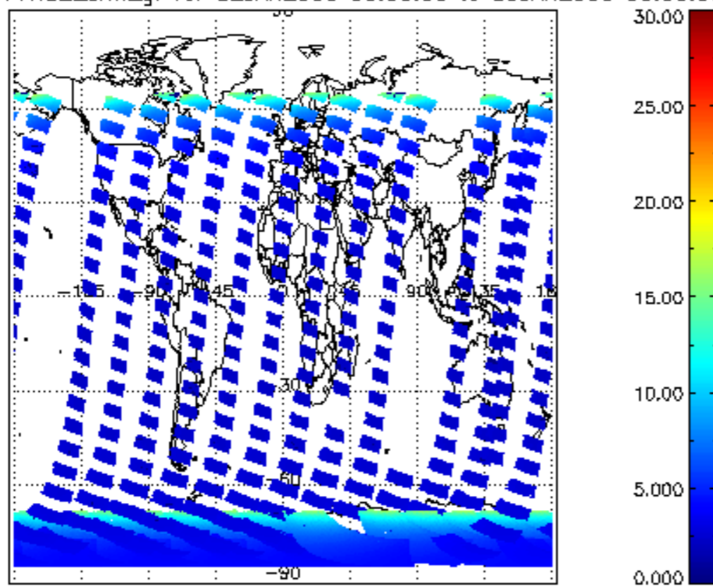
SCIOL2P_NADUV1NO2_amf_gr for 02JAN2009 00:00:00 to 03JAN2009 00:00:00
