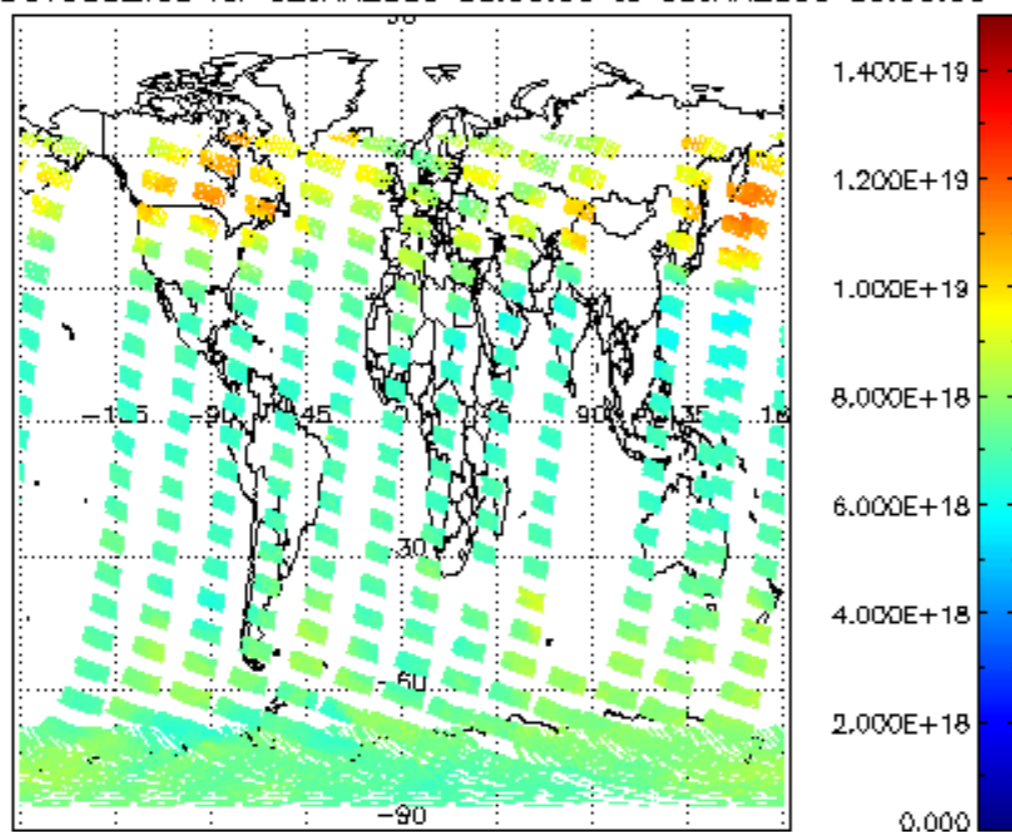
SCIOL2P_NADUV003_vcd for 02JAN2009 00:00:00 to 03JAN2009 00:00:00
