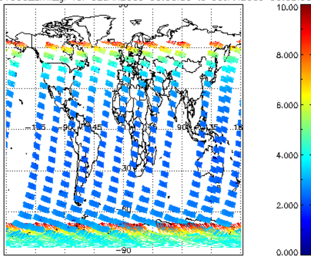
SCIOL2P_NADUV003_amf_gr for 02JAN2009 00:00:00 to 03JAN2009 00:00:00
