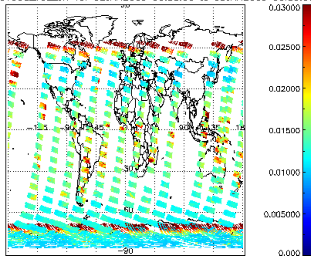
SCIOL2P_NADUV003_vcd_err for 02JAN2009 00:00:00 to 03JAN2009 00:00:00
