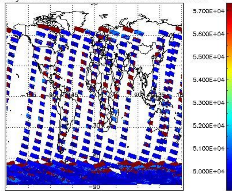
cloud_flags for 02JAN2009 00:00:00 to 03JAN2009 00:00:00
