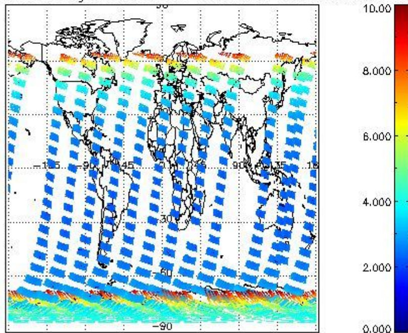
SCIOL2P_NADUV003_amf_gr for 02JAN2009 00:00:00 to 03JAN2009 00:00:00
