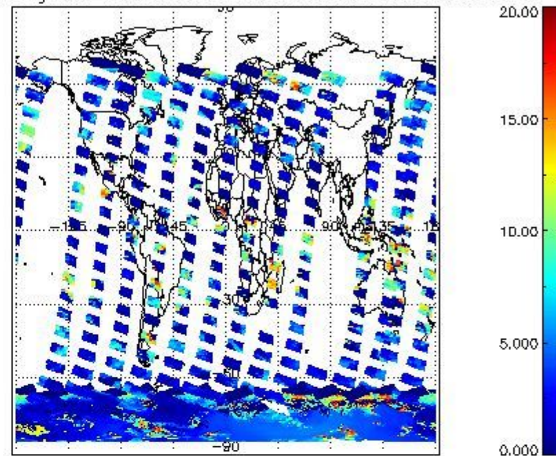
cL_top_height for 02JAN2009 00:00:00 to 03JAN2009 00:00:00
