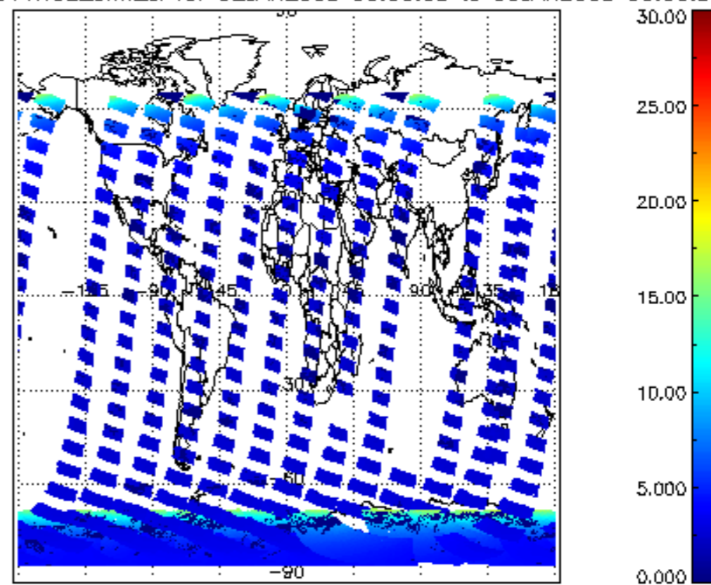
SCIOL2P_NADUV1NO2_amf_cl for 02JAN2009 00:00:00 to 03JAN2009 00:00:00
