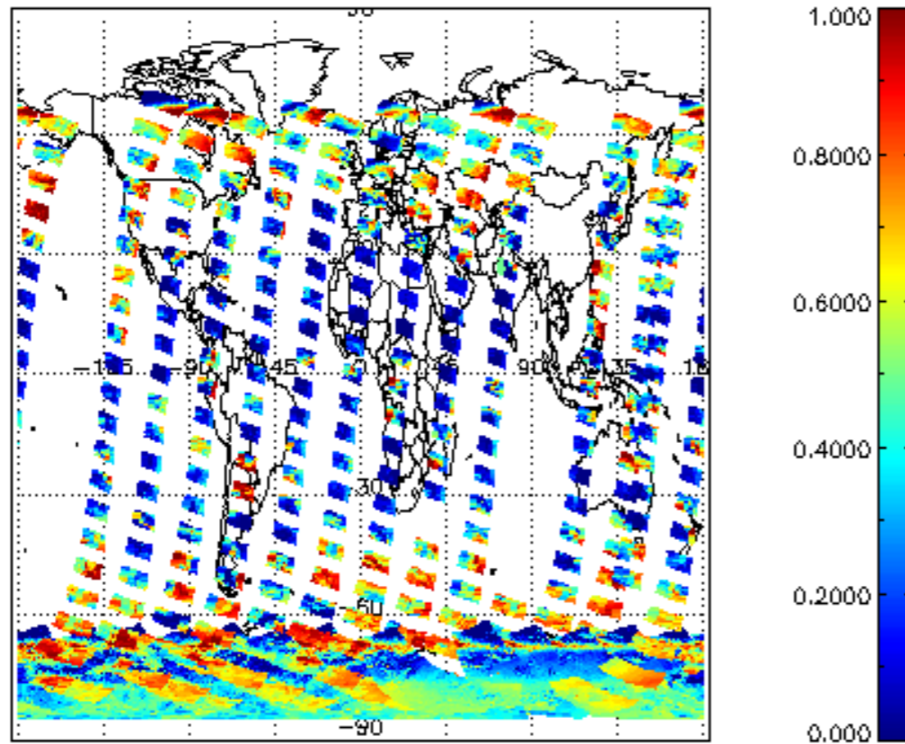
cL_frac for 02JAN2009 00:00:00 to 03JAN2009 00:00:00
