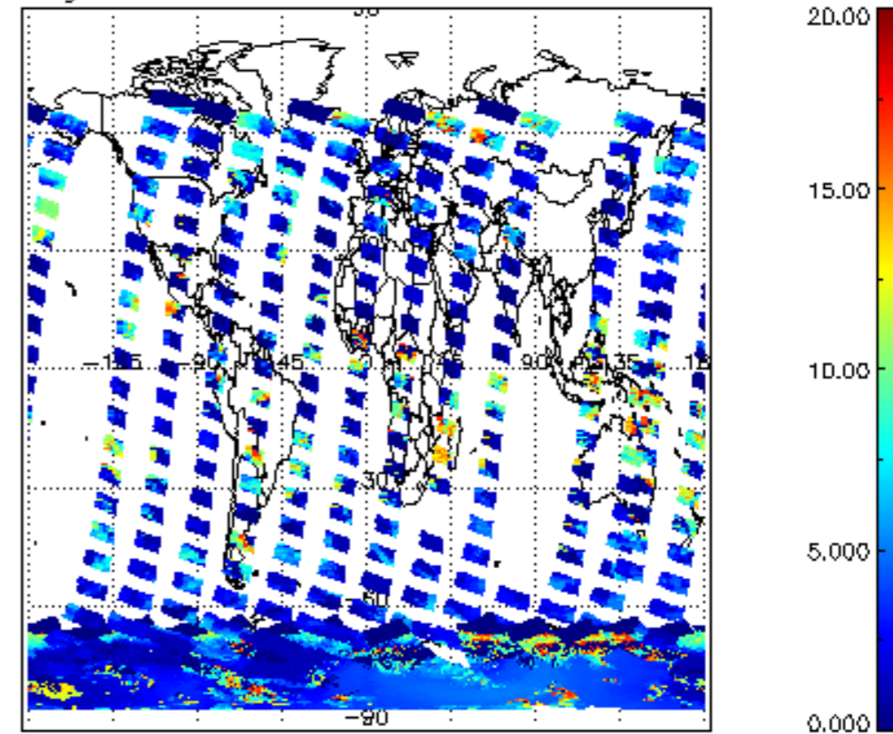
cL_top_height for 02JAN2009 00:00:00 to 03JAN2009 00:00:00
