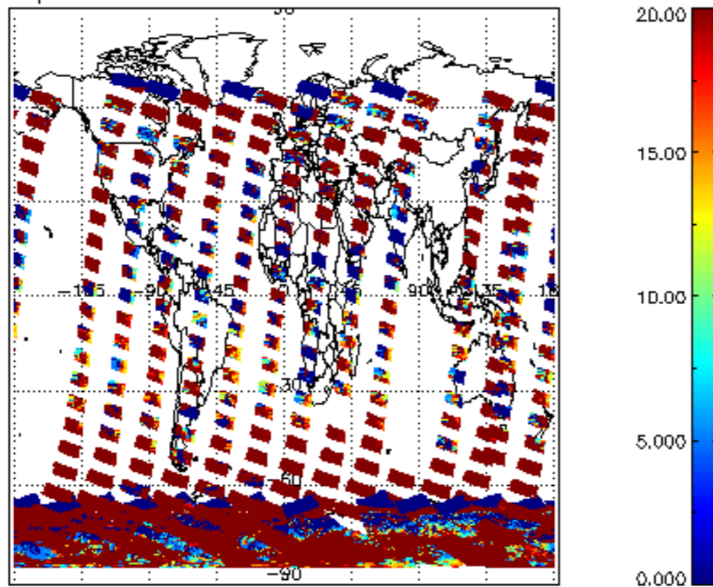
cL_opt_depth for 02JAN2009 00:00:00 to 03JAN2009 00:00:00
