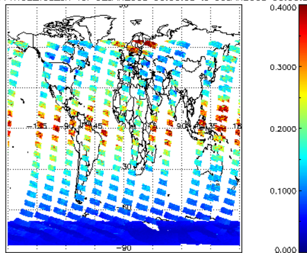
SCIOL2P_NADUV1NO2_vcd_err for 02JAN2009 00:00:00 to 03JAN2009 00:00:00
