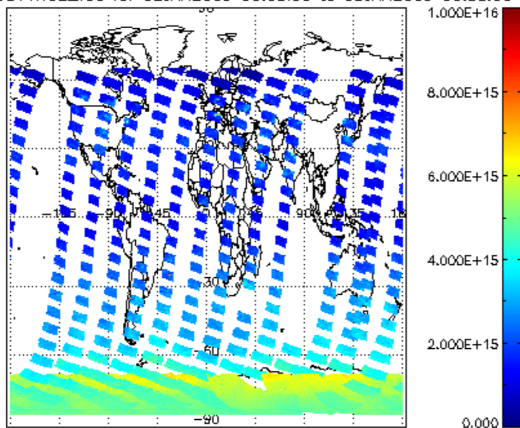
SCIOL2P_NADUV1NO2_vcd for 02JAN2009 00:00:00 to 03JAN2009 00:00:00
