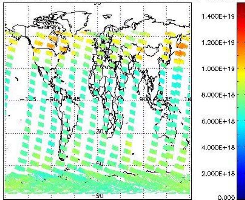
SCIOL2P_NADUV003_vcd for 02JAN2009 00:00:00 to 03JAN2009 00:00:00
