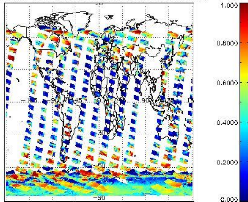
cL_frac for 02JAN2009 00:00:00 to 03JAN2009 00:00:00
