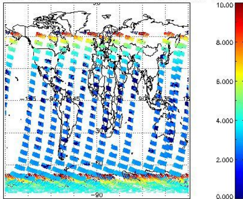
SCIOL2P_NADUV003_amf_cl for 02JAN2009 00:00:00 to 03JAN2009 00:00:00
