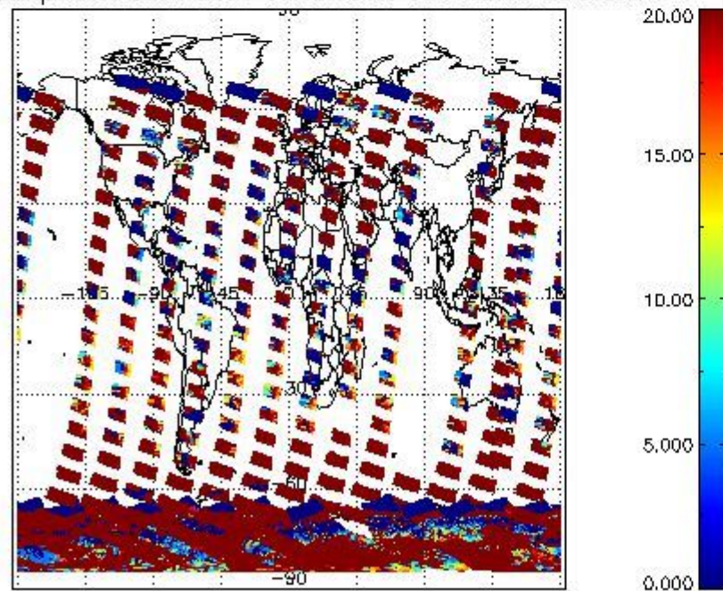
cLopt_depth for 02JAN2009 00:00:00 to 03JAN2009 00:00:00
