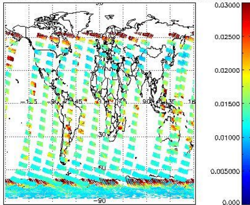
SCIOL2P_NADUV003_vcd_err for 02JAN2009 00:00:00 to 03JAN2009 00:00:00
