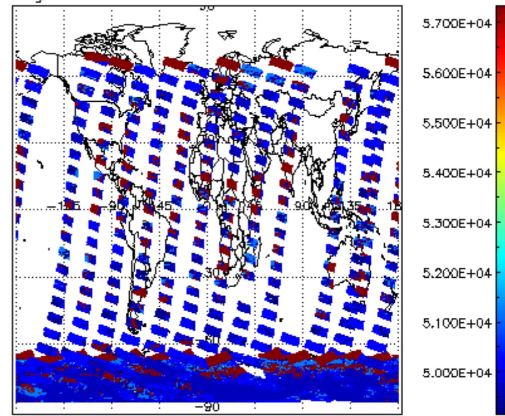
cloud_flags for 02JAN2009 00:00:00 to 03JAN2009 00:00:00
