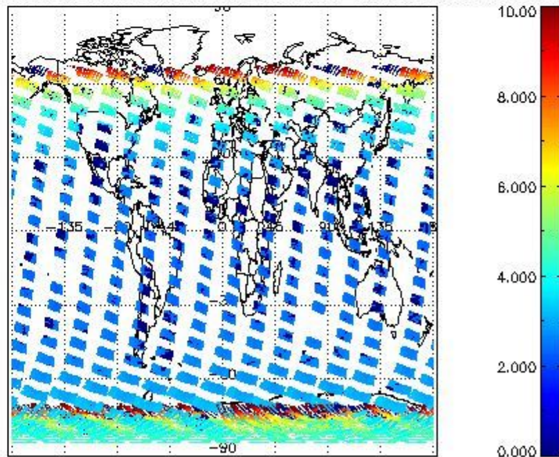
SCIOL2P_NADUV003_amf_cl for 24NOV2008 00:00:00 to 25NOV2008 00:00:00
