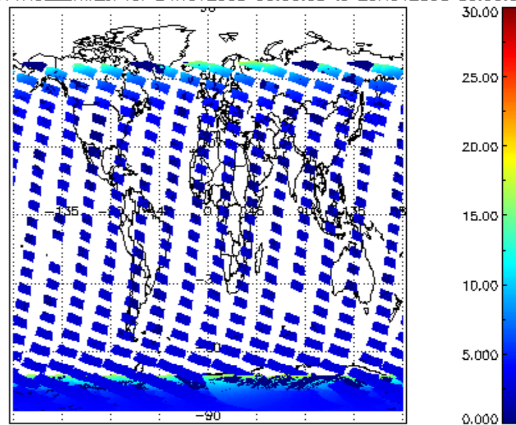
SCIOL2P_NADUV1NO2_amf_cl for 24NOV2008 00:00:00 to 25NOV2008 00:00:00
