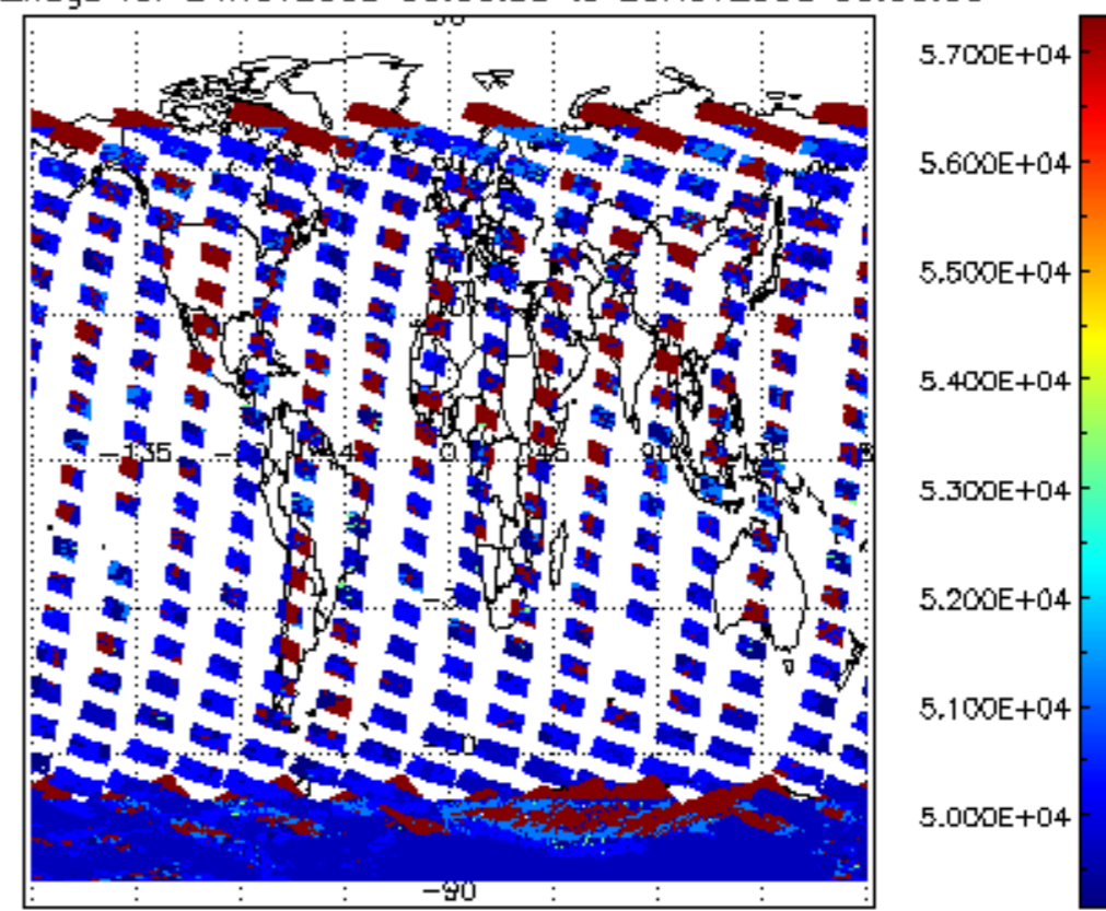
cloud_flags for 24NOV2008 00:00:00 to 25NOV2008 00:00:00
