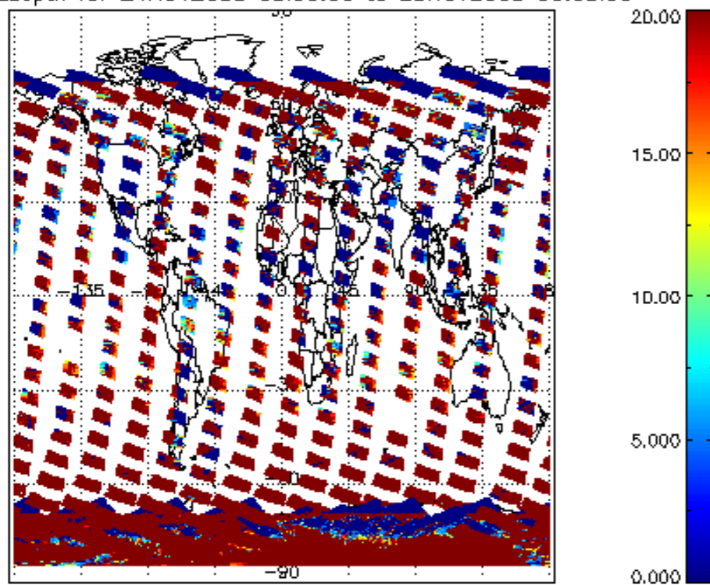
cL_opt_depth for 24NOV2008 00:00:00 to 25NOV2008 00:00:00
