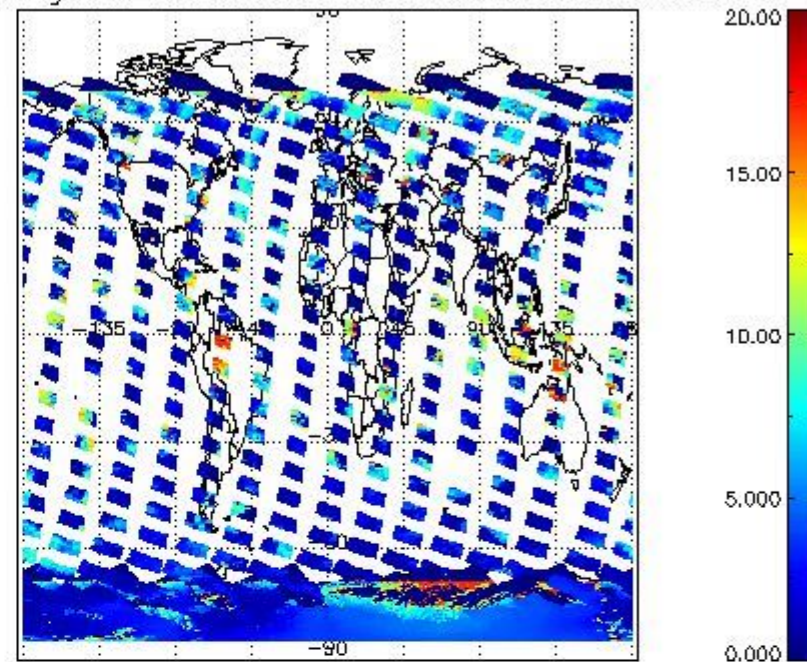
cL_top_height for 24NOV2008 00:00:00 to 25NOV2008 00:00:00
