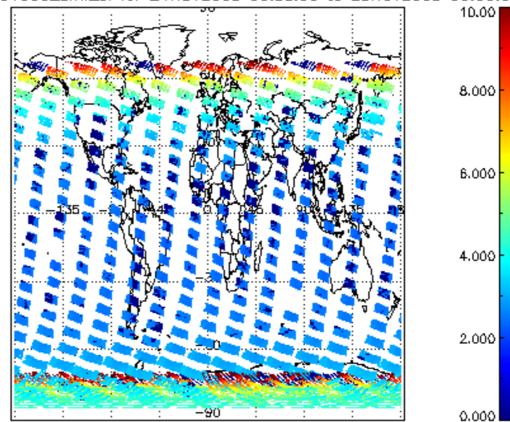
SCIOL2P_NADUV003_amf_cl for 24NOV2008 00:00:00 to 25NOV2008 00:00:00
