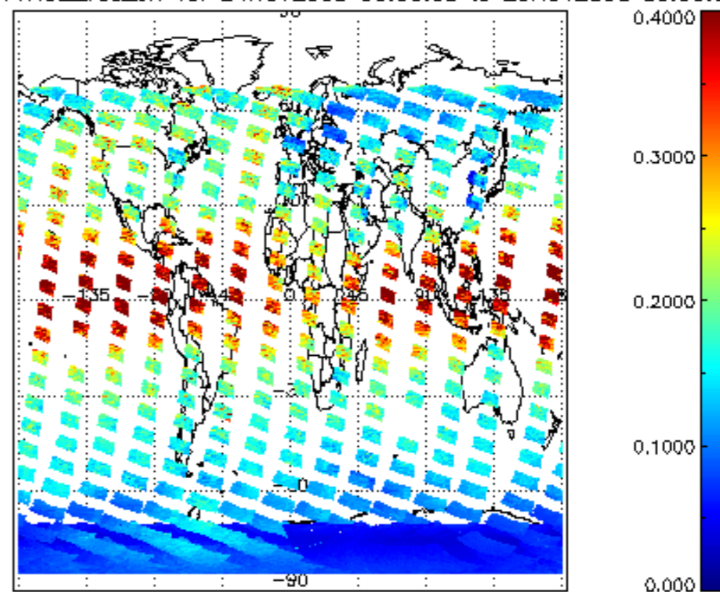
SCIOL2P_NADUV1NO2_vcd_err for 24NOV2008 00:00:00 to 25NOV2008 00:00:00
