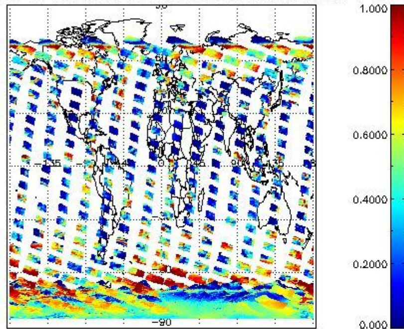
cLfrac for 24NOV2008 00:00:00 to 25NOV2008 00:00:00
