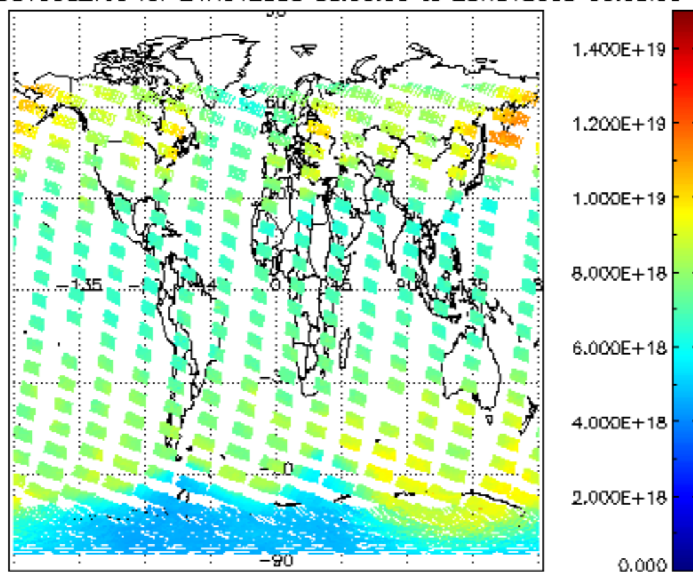
SCIOL2P_NADUV003_vcd for 24NOV2008 00:00:00 to 25NOV2008 00:00:00
