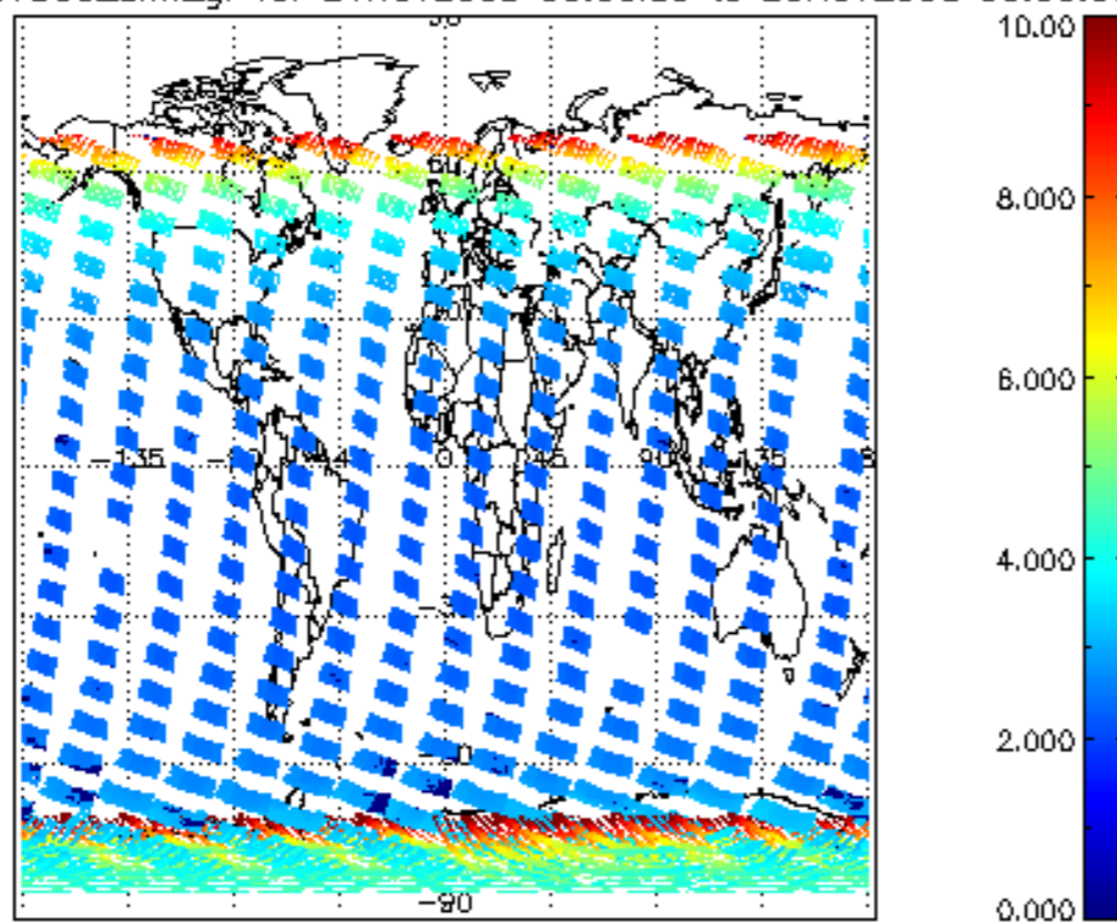
SCIOL2P_NADUV003_amf_gr for 24NOV2008 00:00:00 to 25NOV2008 00:00:00
