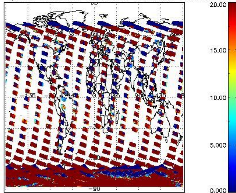
cLopt_depth for 24NOV2008 00:00:00 to 25NOV2008 00:00:00
