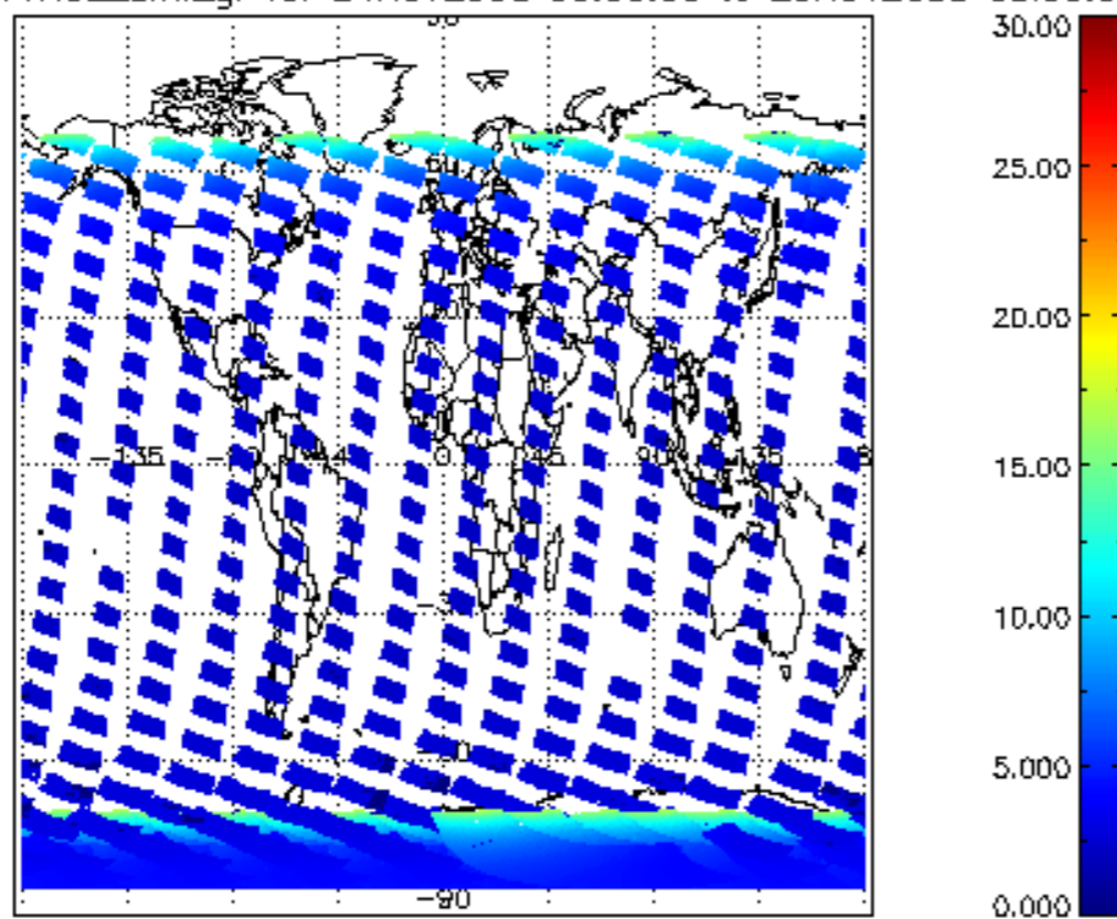
SCIOL2P_NADUV1NO2_amf_gr for 24NOV2008 00:00:00 to 25NOV2008 00:00:00
