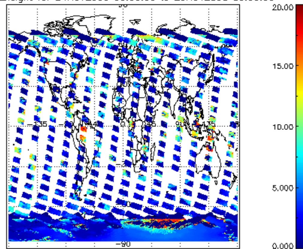
cL_top_height for 24NOV2008 00:00:00 to 25NOV2008 00:00:00
