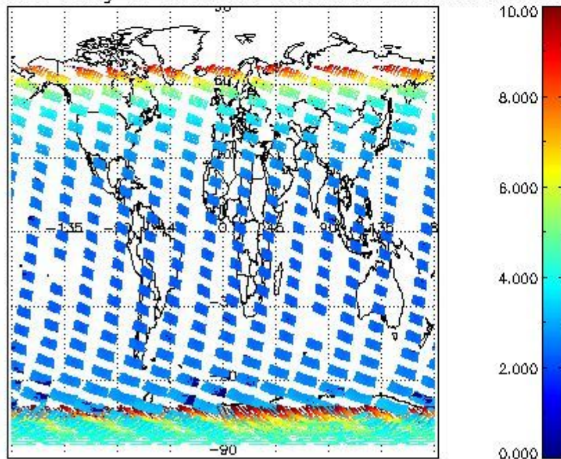
SCIOL2P_NADUV003_amf_gr for 24NOV2008 00:00:00 to 25NOV2008 00:00:00
