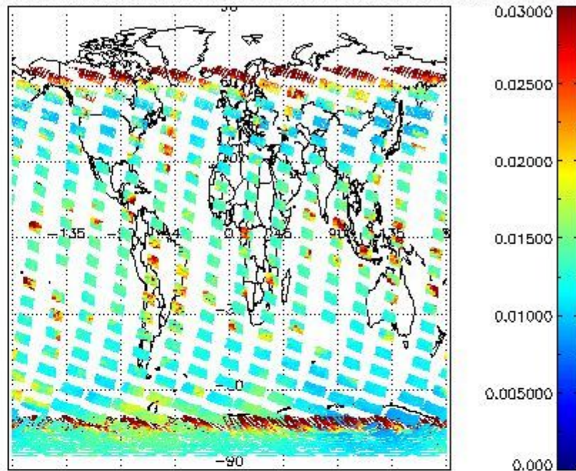
SCIOL2P_NADUV003_vcd_err for 24NOV2008 00:00:00 to 25NOV2008 00:00:00
