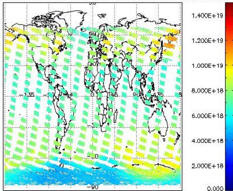
SCIOL2P_NADUV003_vcd for 24NOV2008 00:00:00 to 25NOV2008 00:00:00
