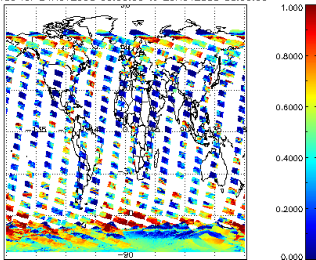
cLfrac for 24NOV2008 00:00:00 to 25NOV2008 00:00:00
