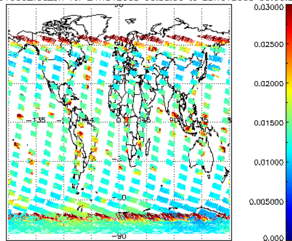
SCIOL2P_NADUV003_vcd_err for 24NOV2008 00:00:00 to 25NOV2008 00:00:00
