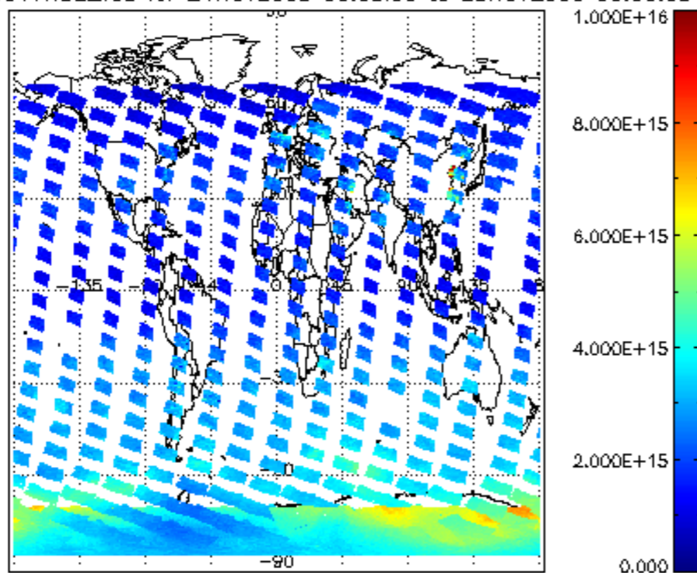
SCIOL2P_NADUV1NO2_vcd for 24NOV2008 00:00:00 to 25NOV2008 00:00:00
