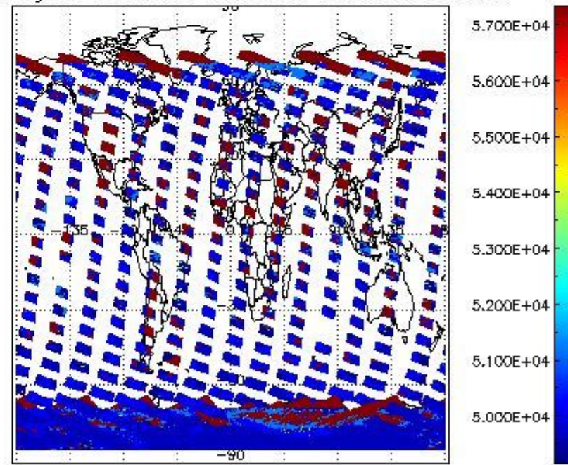
cloud_flags for 24NOV2008 00:00:00 to 25NOV2008 00:00:00
