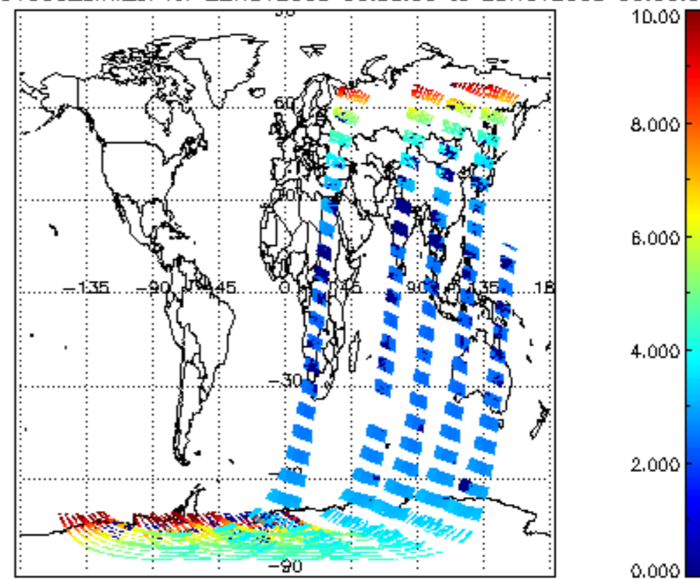
SCIOL2P_NADUV003_amf_cl for 22NOV2008 00:00:00 to 23NOV2008 00:00:00
