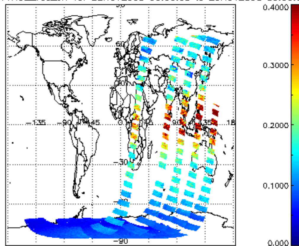
SCIOL2P_NADUV1NO2_vcd_err for 22NOV2008 00:00:00 to 23NOV2008 00:00:00
