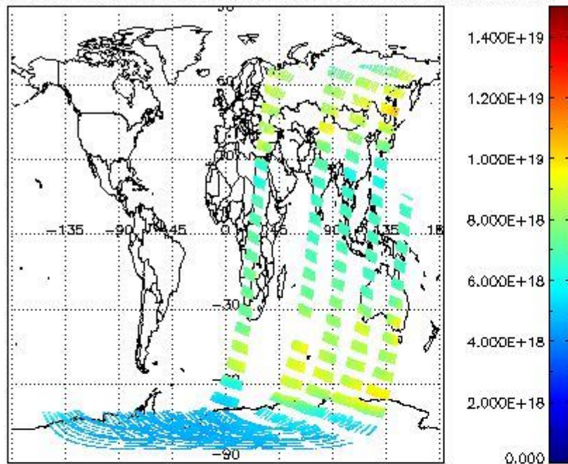
SCIOL2P_NADUV003_vcd for 22NOV2008 00:00:00 to 23NOV2008 00:00:00
