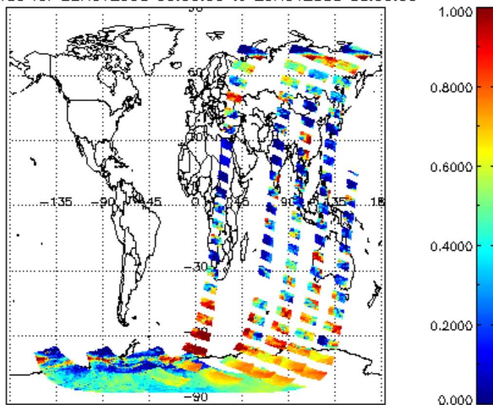
cLfrac for 22NOV2008 00:00:00 to 23NOV2008 00:00:00
