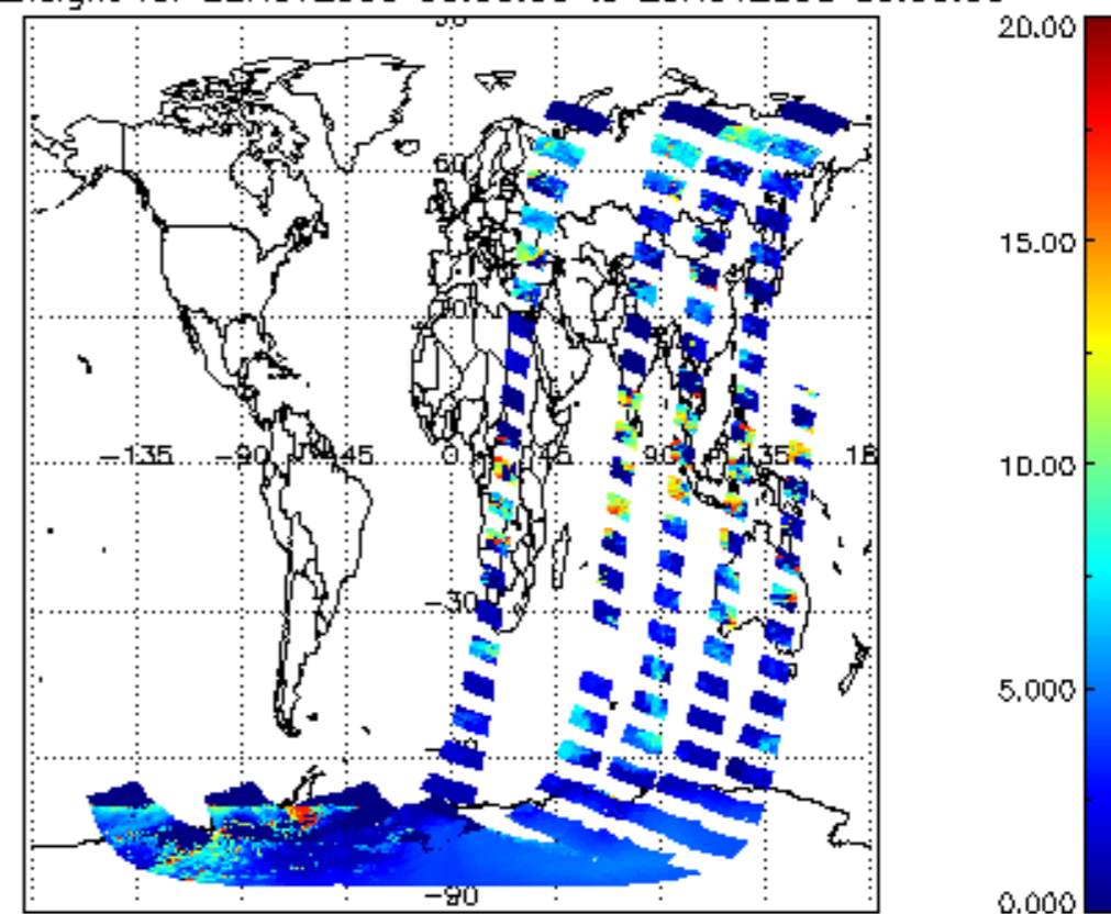
cl_top_height for 22NOV2008 00:00:00 to 23NOV2008 00:00:00
