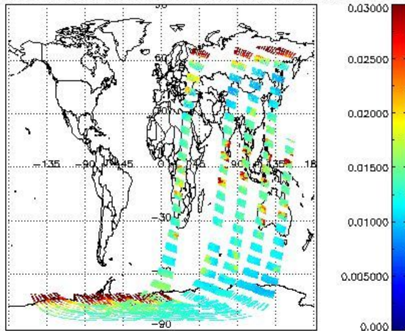
SCIOL2P_NADUV003_vcd_err for 22NOV2008 00:00:00 to 23NOV2008 00:00:00
