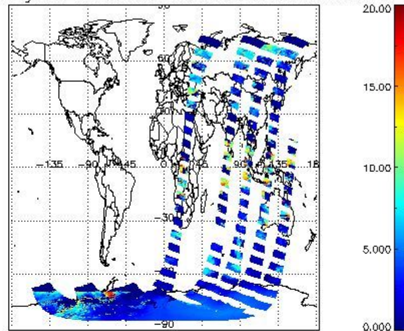
cL_top_height for 22NOV2008 00:00:00 to 23NOV2008 00:00:00
