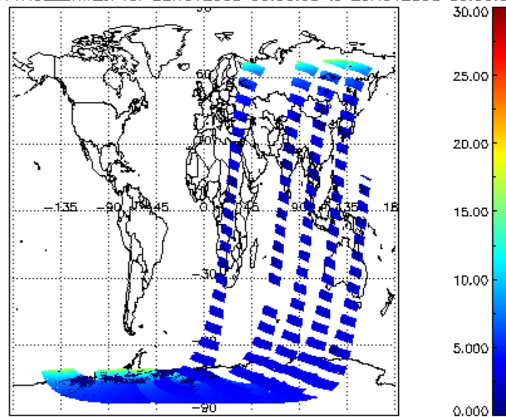
SCIOL2P_NADUV1NO2_amf_cl for 22NOV2008 00:00:00 to 23NOV2008 00:00:00
