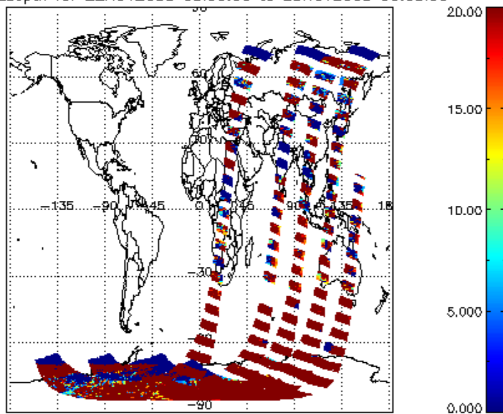
cl_opt_depth for 22NOV2008 00:00:00 to 23NOV2008 00:00:00
