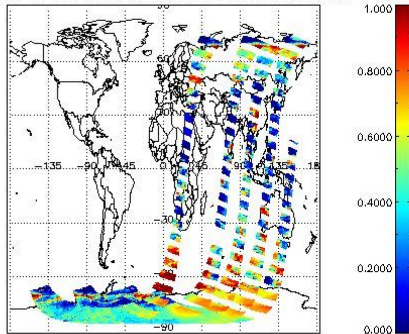
cLfrac for 22NOV2008 00:00:00 to 23NOV2008 00:00:00
