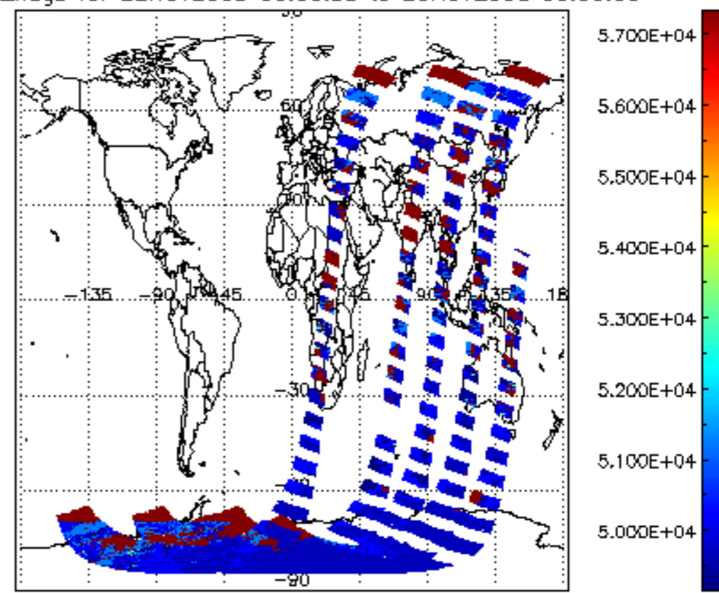
cloud_flags for 22NOV2008 00:00:00 to 23NOV2008 00:00:00
