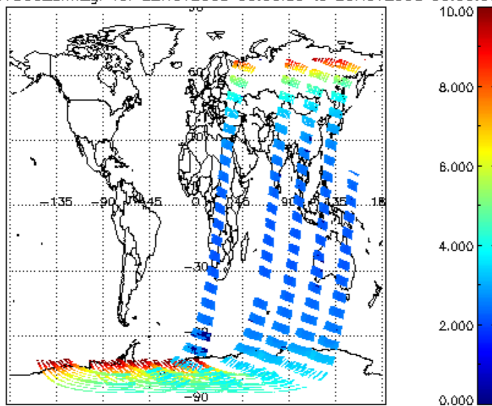
SCIOL2P_NADUV003_amf_gr for 22NOV2008 00:00:00 to 23NOV2008 00:00:00
