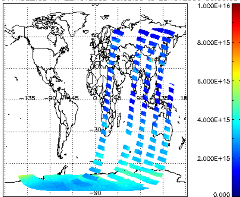
SCIOL2P_NADUV1NO2_vcd for 22NOV2008 00:00:00 to 23NOV2008 00:00:00
