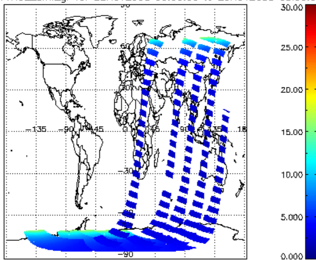
SCIOL2P_NADUV1NO2_amf_gr for 22NOV2008 00:00:00 to 23NOV2008 00:00:00
