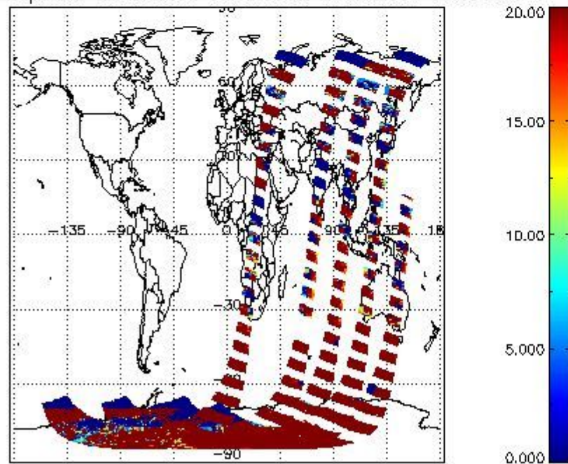
cLopt_depth for 22NOV2008 00:00:00 to 23NOV2008 00:00:00
