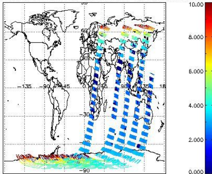
SCIOL2P_NADUV003_amf_cl for 22NOV2008 00:00:00 to 23NOV2008 00:00:00
