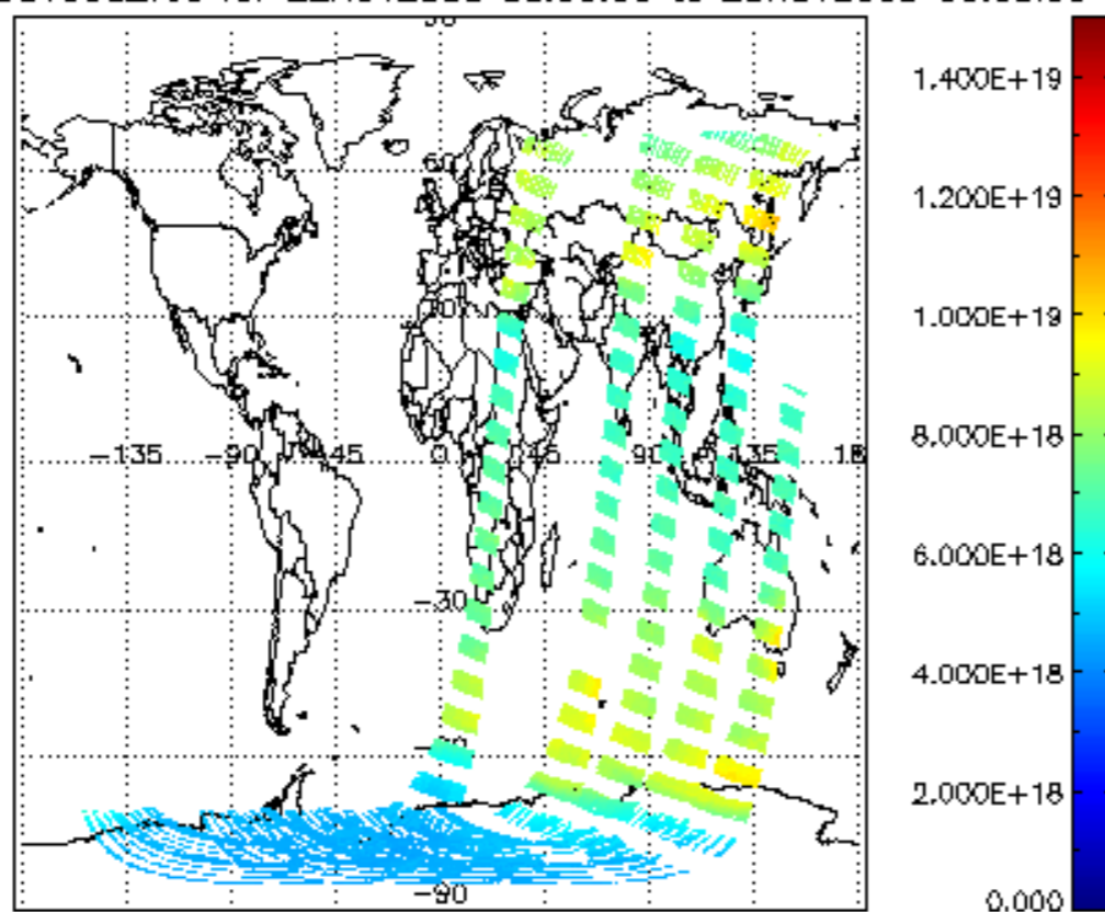
SCIOL2P_NADUV003_vcd for 22NOV2008 00:00:00 to 23NOV2008 00:00:00
