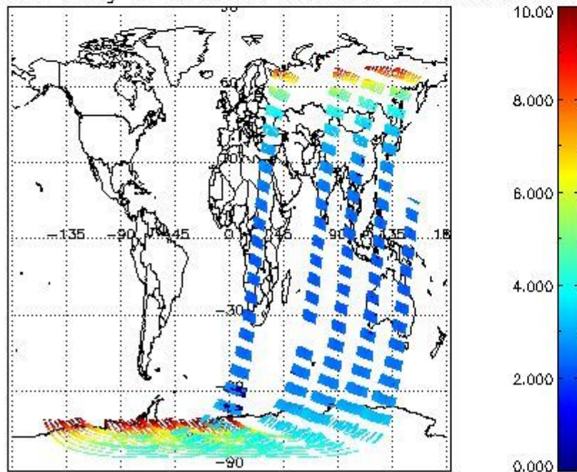
SCIOL2P_NADUV003_amf_gr for 22NOV2008 00:00:00 to 23NOV2008 00:00:00
