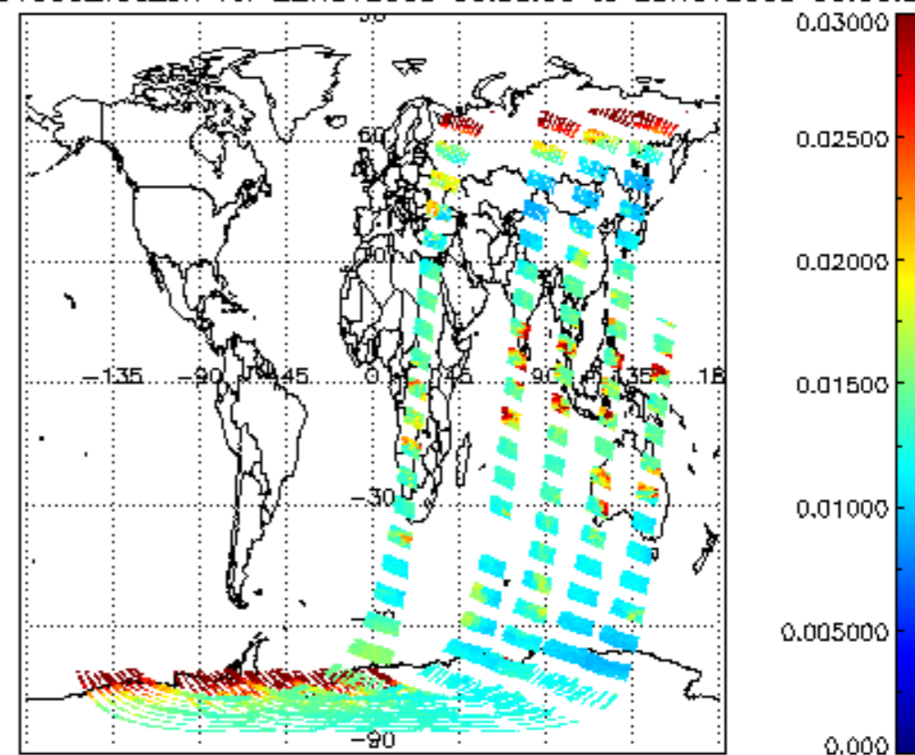
SCIOL2P_NADUV003_vcd_err for 22NOV2008 00:00:00 to 23NOV2008 00:00:00
