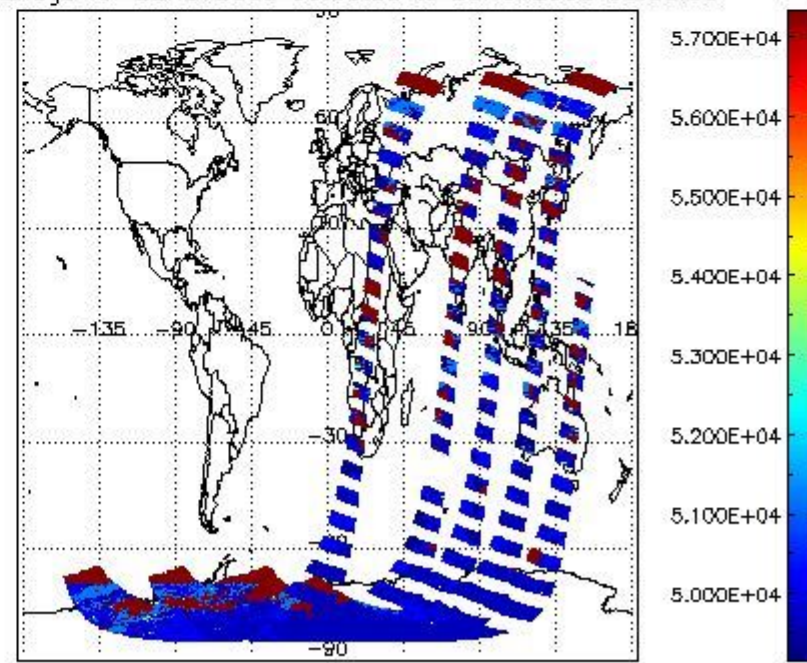
cloud_flags for 22NOV2008 00:00:00 to 23NOV2008 00:00:00
