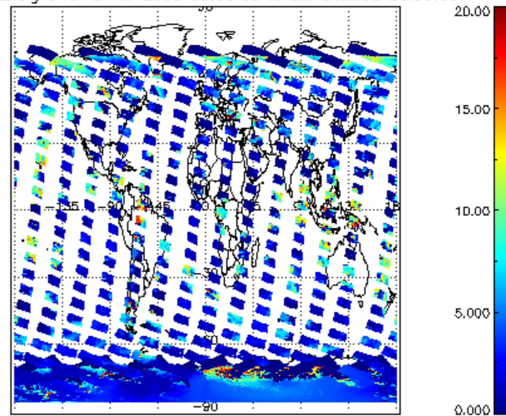
cL_top_height for 21NOV2008 00:00:00 to 22NOV2008 00:00:00
