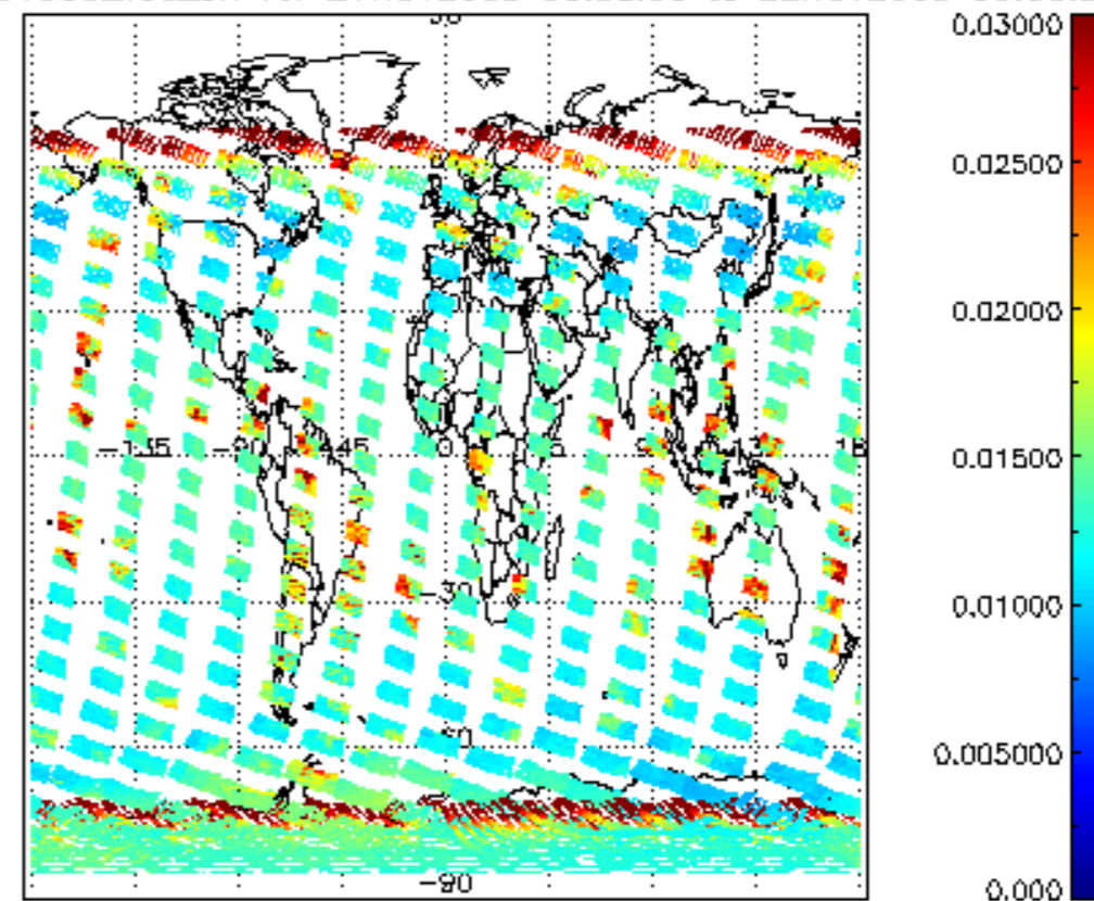
SCIOL2P_NADUV003_vcd_err for 21NOV2008 00:00:00 to 22NOV2008 00:00:00
