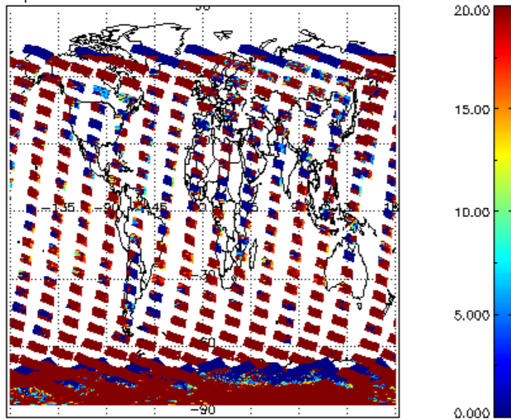
cL_opt_depth for 21NOV2008 00:00:00 to 22NOV2008 00:00:00
