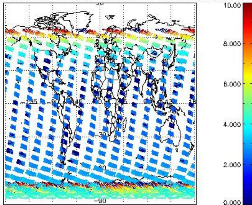
SCIOL2P_NADUV003_amf_cl for 21NOV2008 00:00:00 to 22NOV2008 00:00:00
