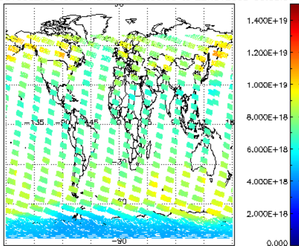
SCIOL2P_NADUV003_vcd for 21NOV2008 00:00:00 to 22NOV2008 00:00:00
