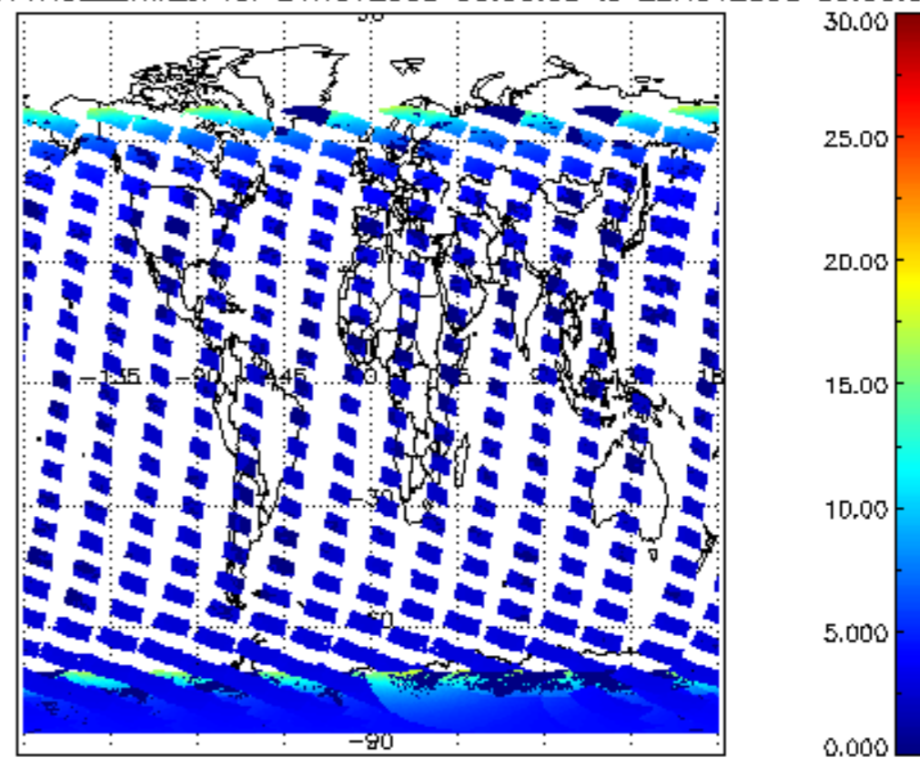
SCIOL2P_NADUV1NO2_amf_cl for 21NOV2008 00:00:00 to 22NOV2008 00:00:00
