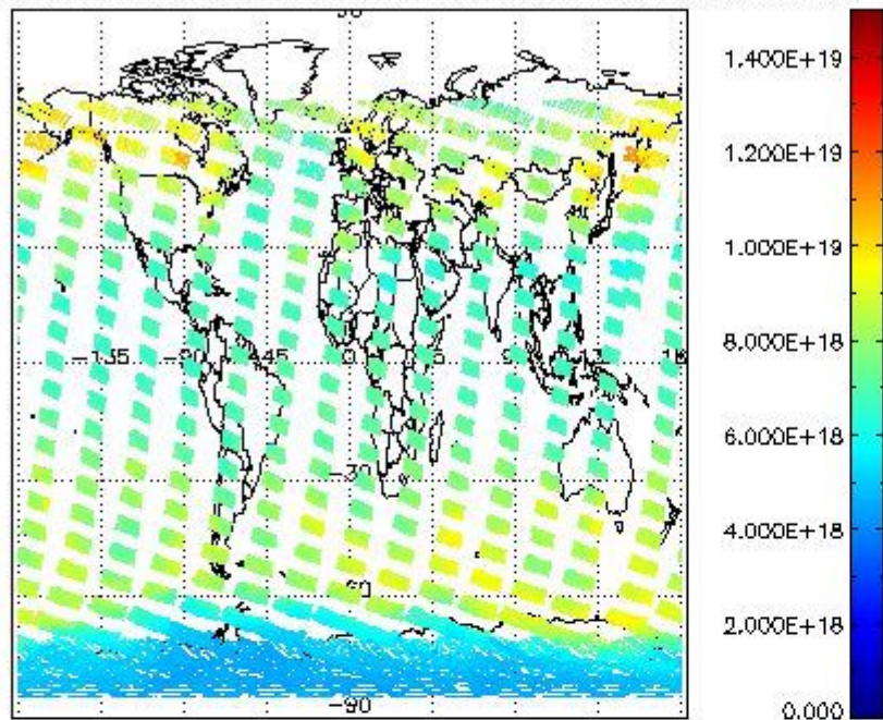
SCIOL2P_NADUV003_vcd for 21NOV2008 00:00:00 to 22NOV2008 00:00:00
