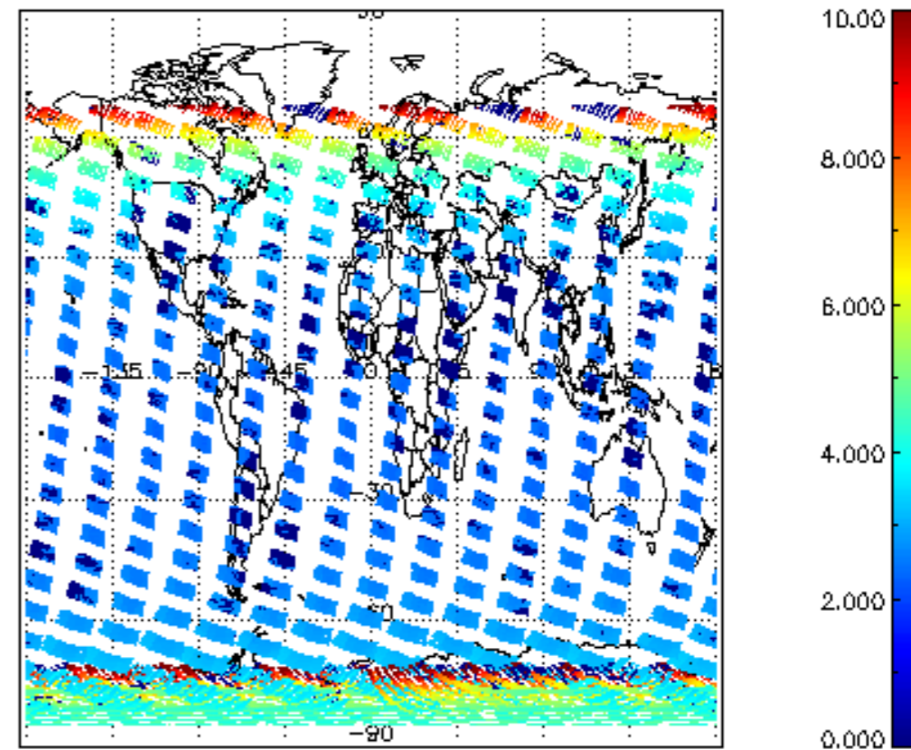
SCIOL2P_NADUV003_amf_cl for 21NOV2008 00:00:00 to 22NOV2008 00:00:00
