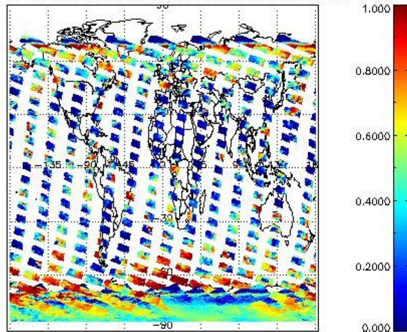
cLfrac for 21NOV2008 00:00:00 to 22NOV2008 00:00:00
