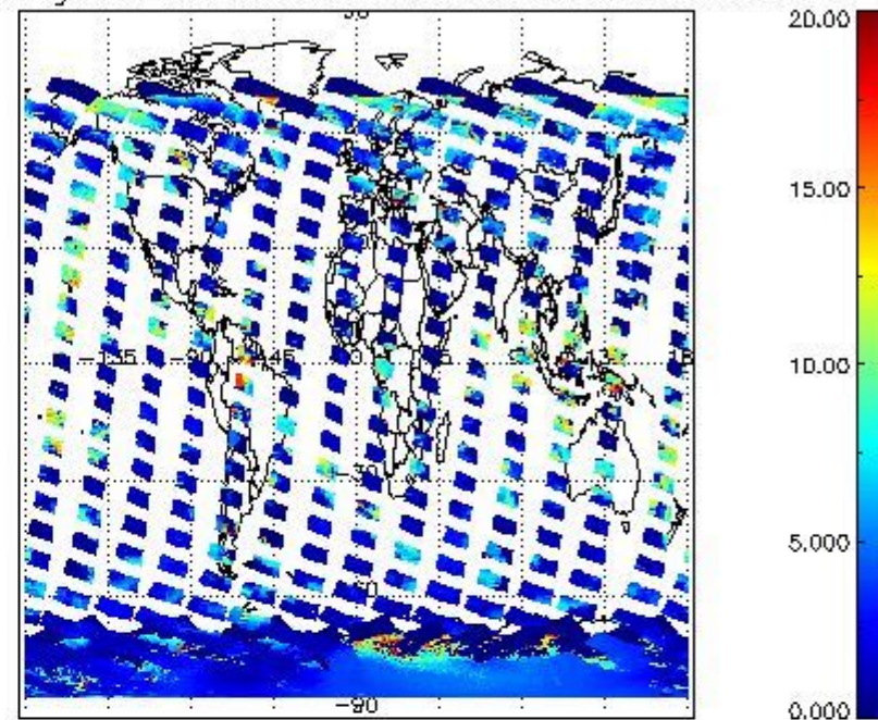
cL_top_height for 21NOV2008 00:00:00 to 22NOV2008 00:00:00
