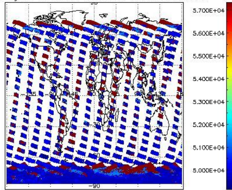
cloud_flags for 21NOV2008 00:00:00 to 22NOV2008 00:00:00
