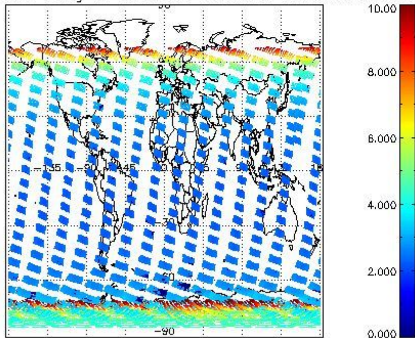
SCIOL2P_NADUV003_amf_gr for 21NOV2008 00:00:00 to 22NOV2008 00:00:00
