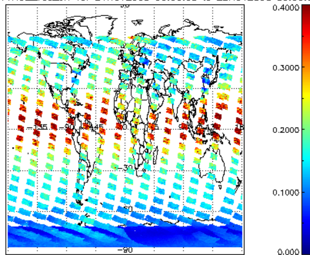
SCIOL2P_NADUV1NO2_vcd_err for 21NOV2008 00:00:00 to 22NOV2008 00:00:00
