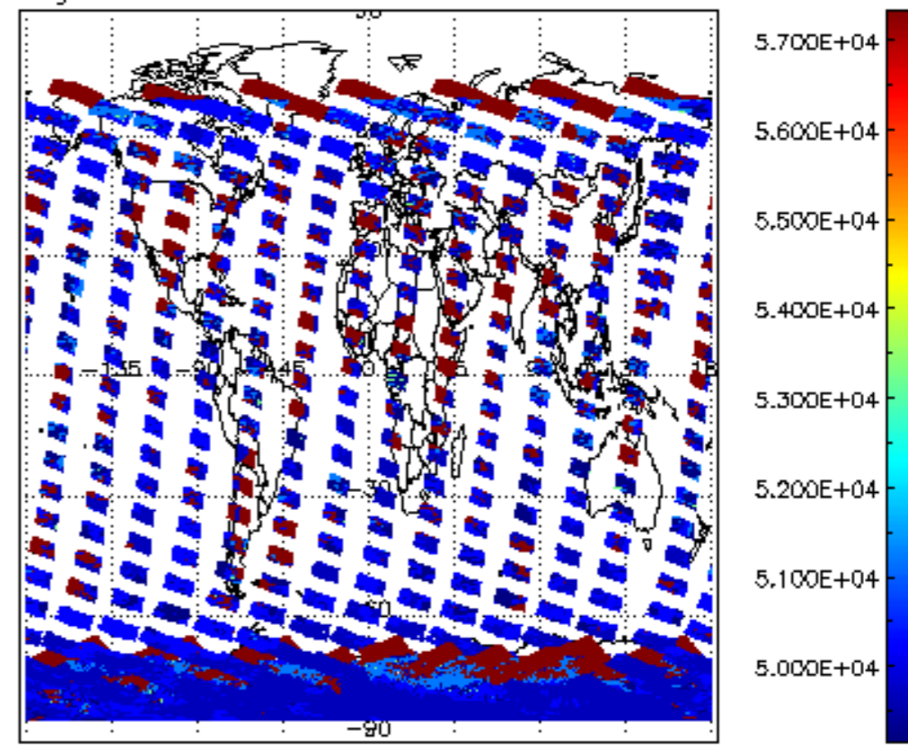
cloud_flags for 21NOV2008 00:00:00 to 22NOV2008 00:00:00
