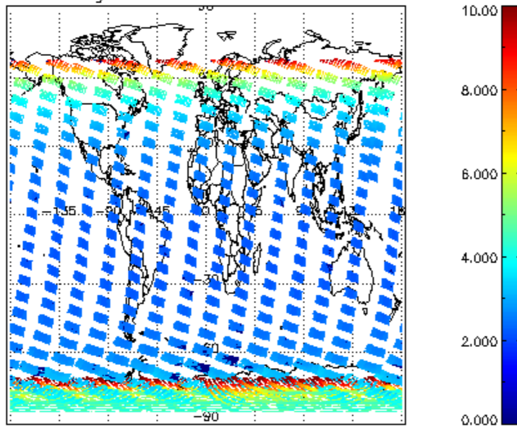
SCIOL2P_NADUV003_amf_gr for 21NOV2008 00:00:00 to 22NOV2008 00:00:00
