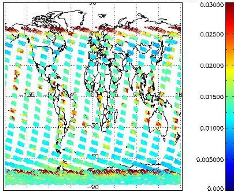
SCIOL2P_NADUV003_vcd_err for 21NOV2008 00:00:00 to 22NOV2008 00:00:00
