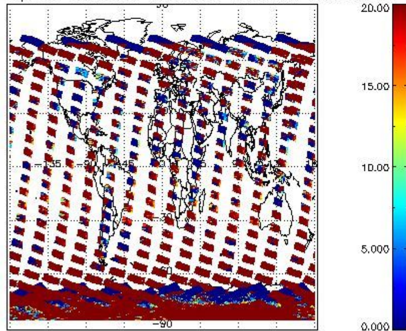
cLopt_depth for 21NOV2008 00:00:00 to 22NOV2008 00:00:00
