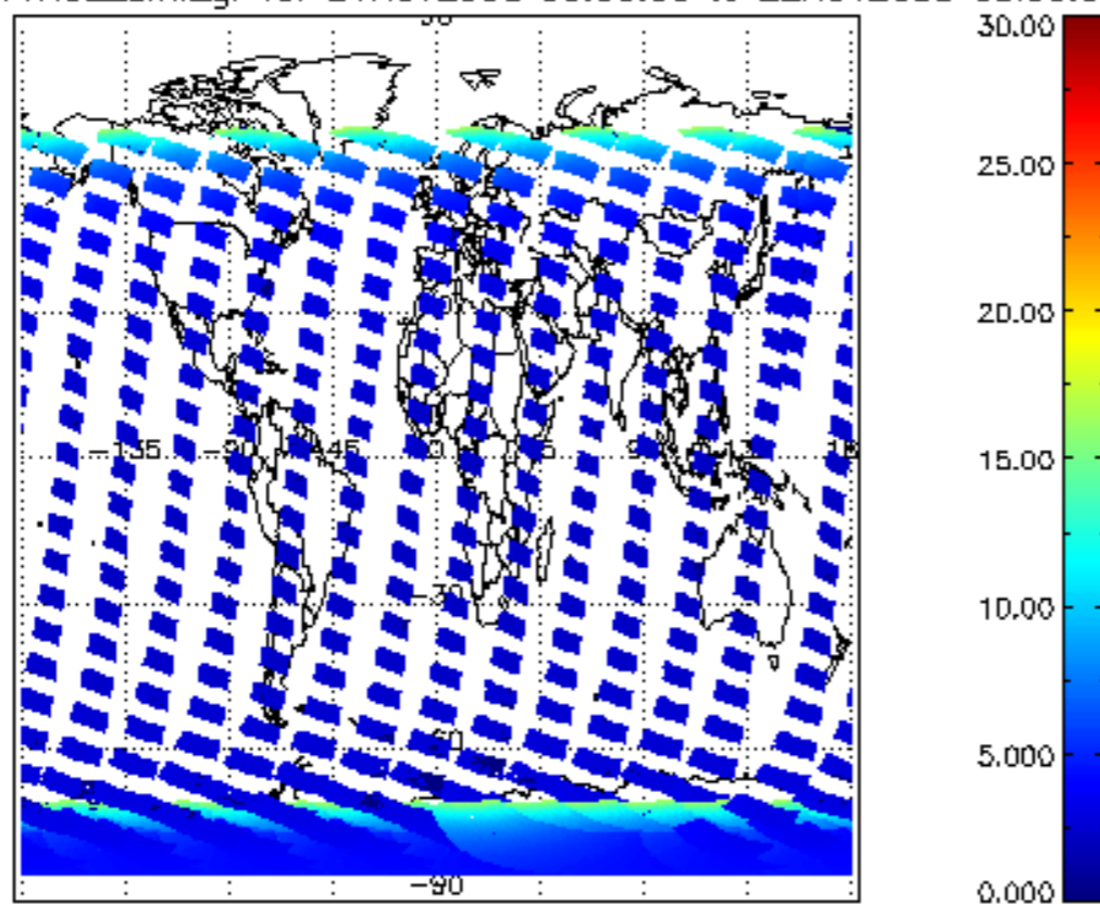
SCIOL2P_NADUV1NO2_amf_gr for 21NOV2008 00:00:00 to 22NOV2008 00:00:00
