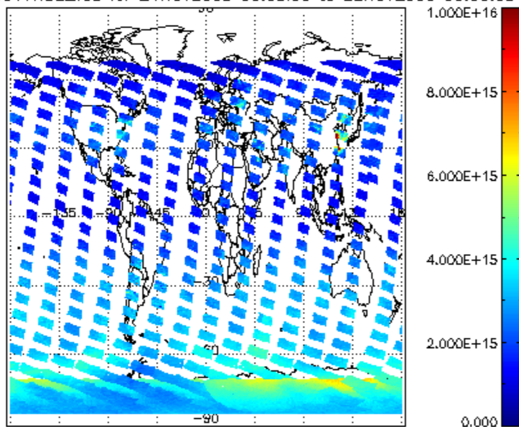
SCIOL2P_NADUV1NO2_vcd for 21NOV2008 00:00:00 to 22NOV2008 00:00:00
