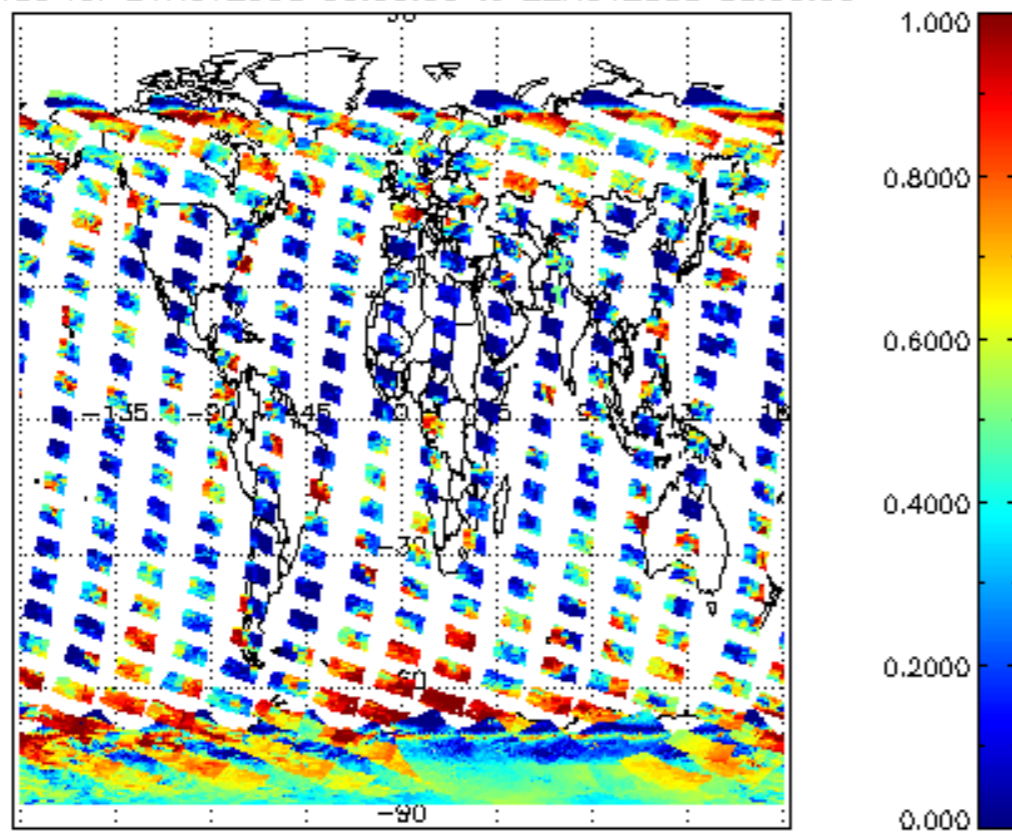
cLfrac for 21NOV2008 00:00:00 to 22NOV2008 00:00:00
