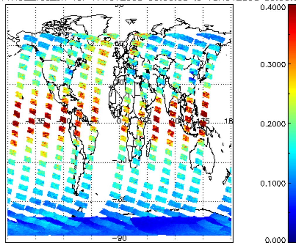
SCIOL2P_NADUV1NO2_vcd_err for 17NOV2008 00:00:00 to 18NOV2008 00:00:00
