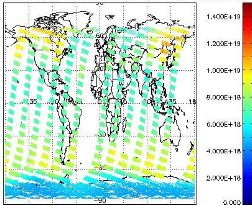
SCIOL2P_NADUV003_vcd for 17NOV2008 00:00:00 to 18NOV2008 00:00:00
