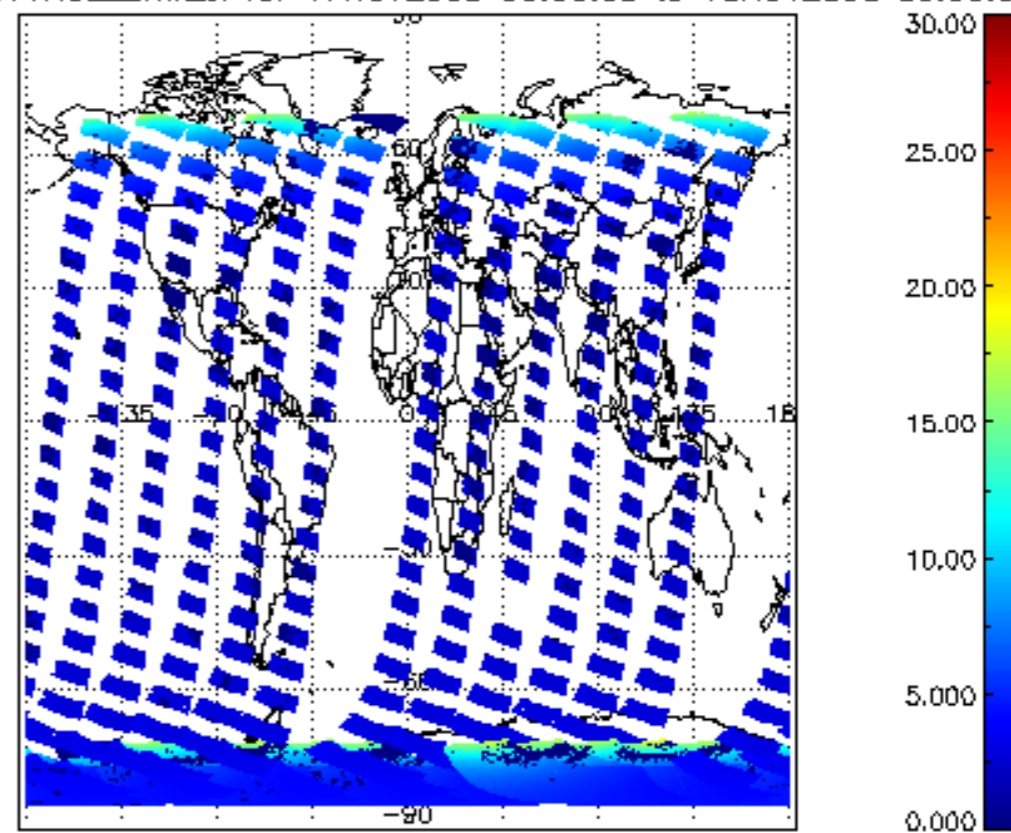
SCIOL2P_NADUV1NO2_amf_cl for 17NOV2008 00:00:00 to 18NOV2008 00:00:00
