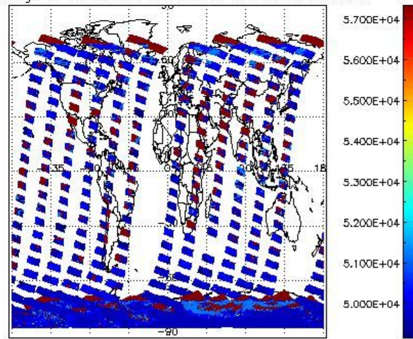
cloud_flags for 17NOV2008 00:00:00 to 18NOV2008 00:00:00
