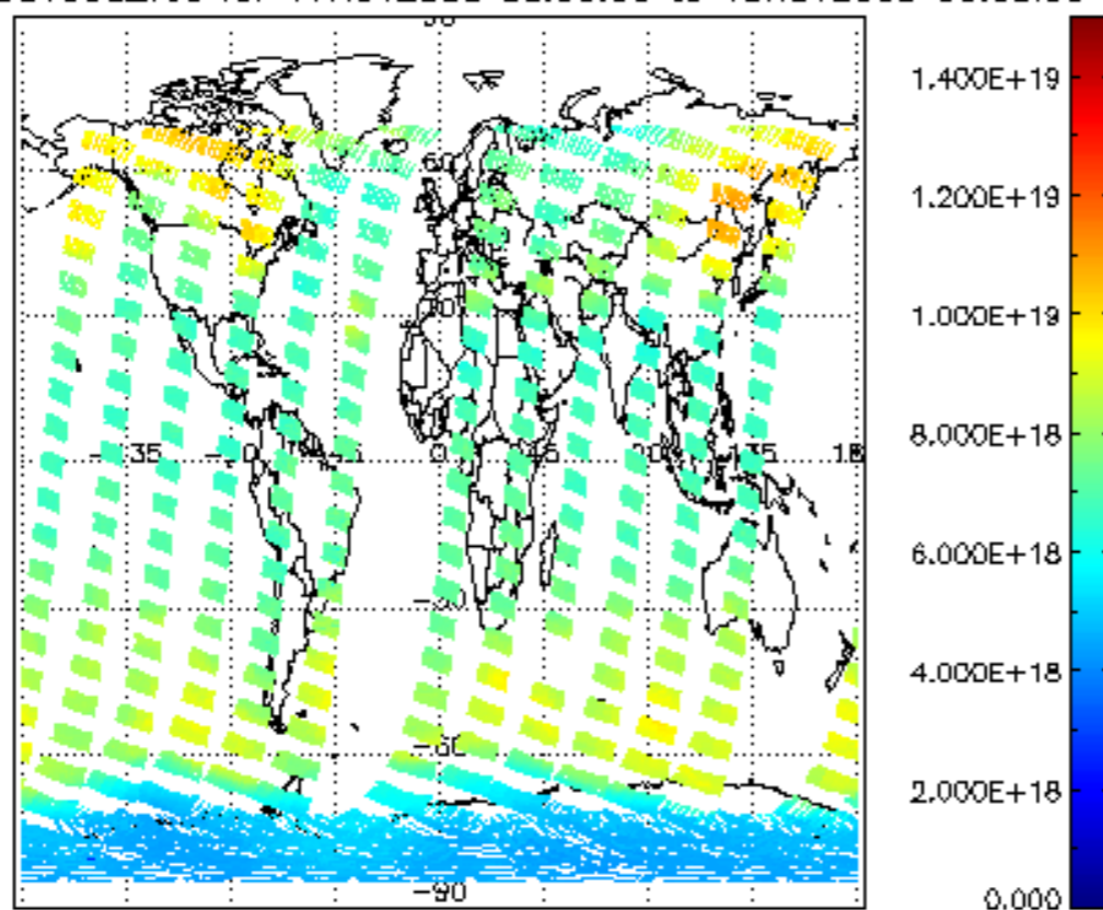
SCIOL2P_NADUV003_vcd for 17NOV2008 00:00:00 to 18NOV2008 00:00:00
