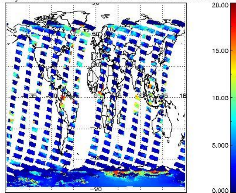
cL_top_height for 17NOV2008 00:00:00 to 18NOV2008 00:00:00
