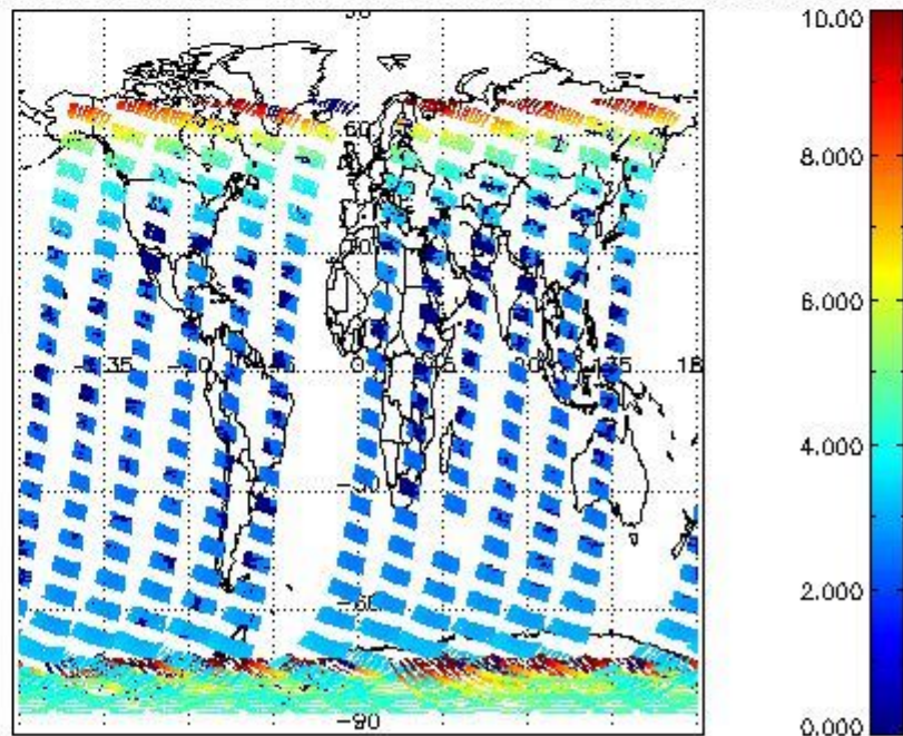
SCIOL2P_NADUV003_amf_cl for 17NOV2008 00:00:00 to 18NOV2008 00:00:00
