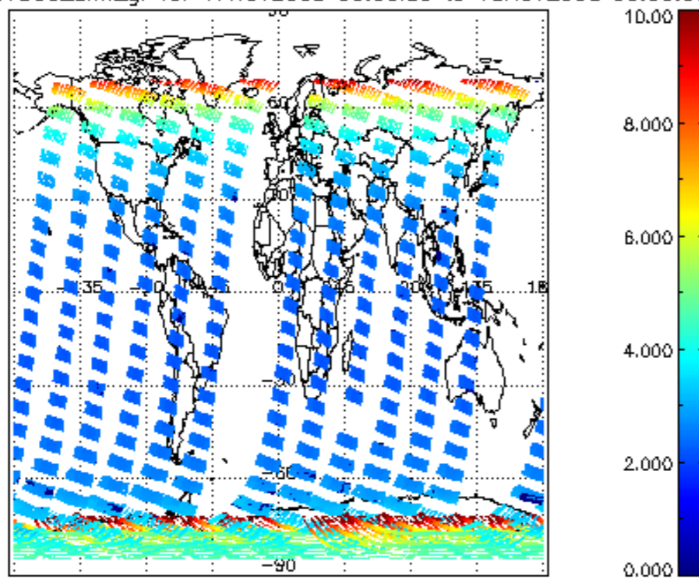
SCIOL2P_NADUV003_amf_gr for 17NOV2008 00:00:00 to 18NOV2008 00:00:00
