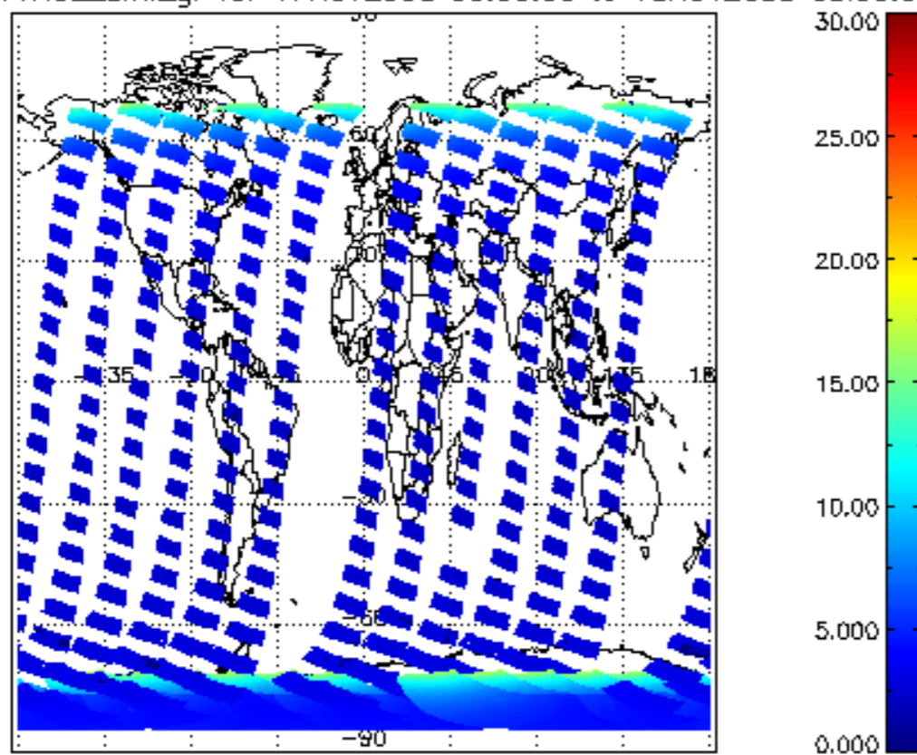
SCIOL2P_NADUV1NO2_amf_gr for 17NOV2008 00:00:00 to 18NOV2008 00:00:00
