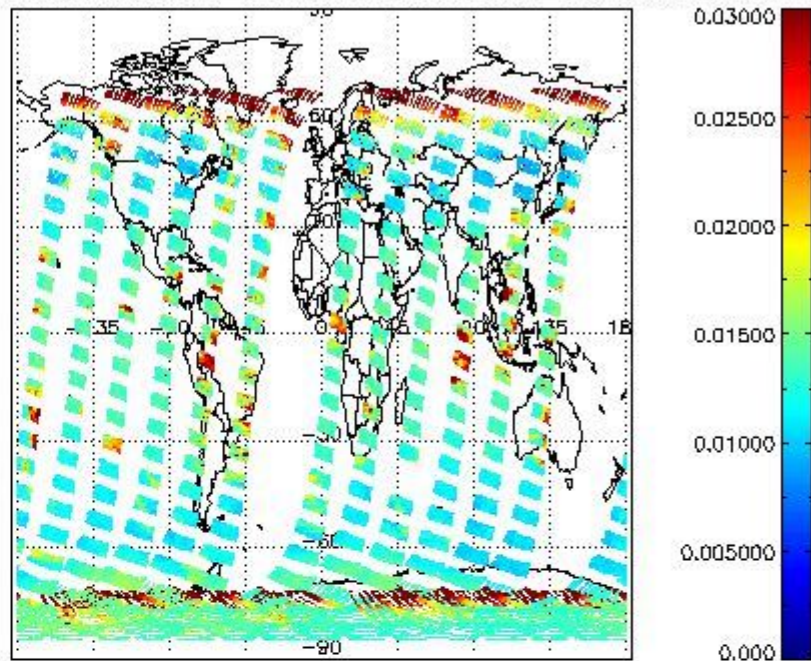
SCIOL2P_NADUV003_vcd_err for 17NOV2008 00:00:00 to 18NOV2008 00:00:00
