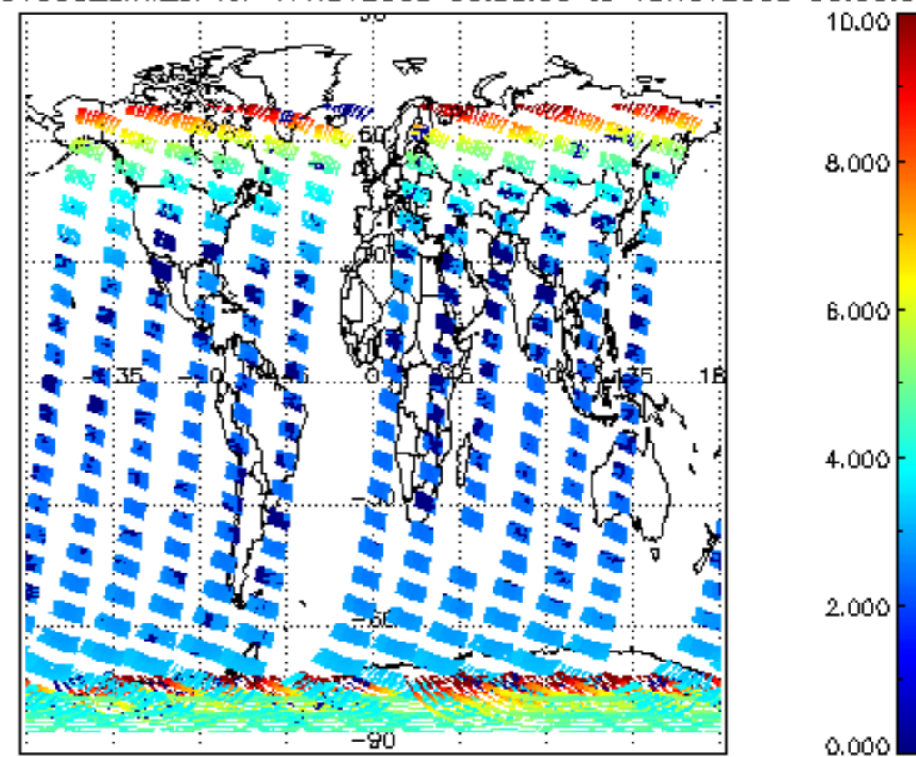
SCIOL2P_NADUV003_amf_cl for 17NOV2008 00:00:00 to 18NOV2008 00:00:00
