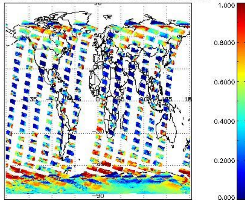
cLfrac for 17NOV2008 00:00:00 to 18NOV2008 00:00:00
