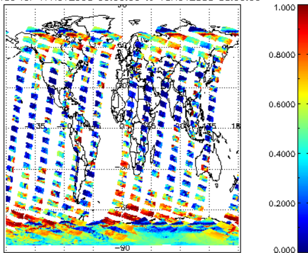
cLfrac for 17NOV2008 00:00:00 to 18NOV2008 00:00:00
