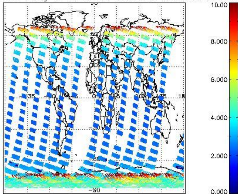
SCIOL2P_NADUV003_amf_gr for 17NOV2008 00:00:00 to 18NOV2008 00:00:00
