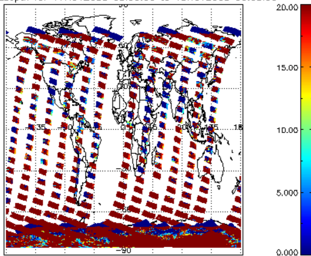
cL_opt_depth for 17NOV2008 00:00:00 to 18NOV2008 00:00:00
