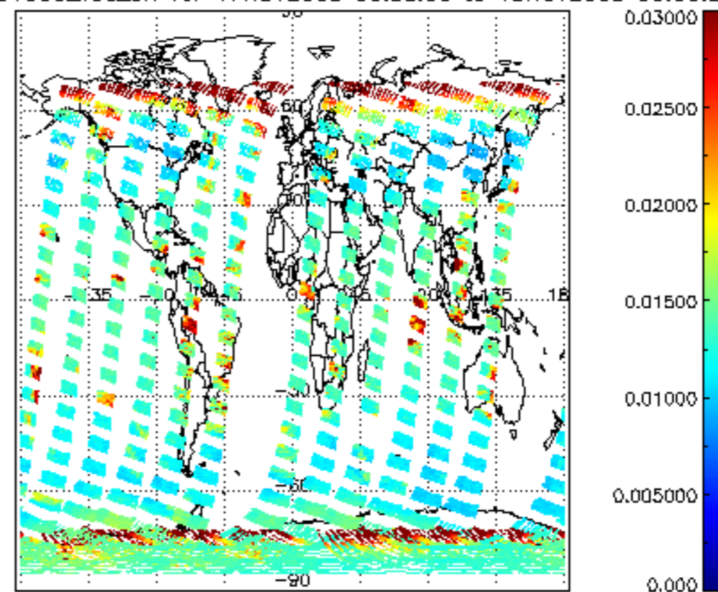
SCIOL2P_NADUV003_vcd_err for 17NOV2008 00:00:00 to 18NOV2008 00:00:00
