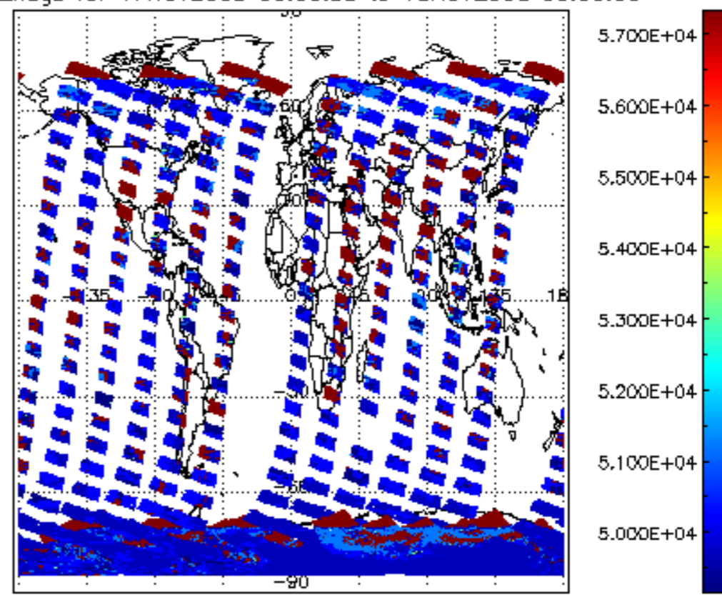
cloud_flags for 17NOV2008 00:00:00 to 18NOV2008 00:00:00
