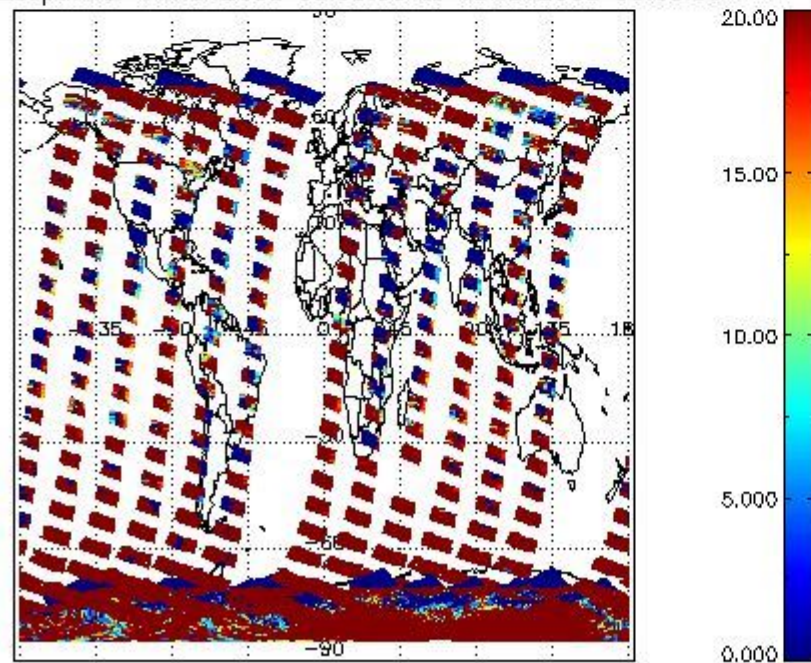
cLopt_depth for 17NOV2008 00:00:00 to 18NOV2008 00:00:00
