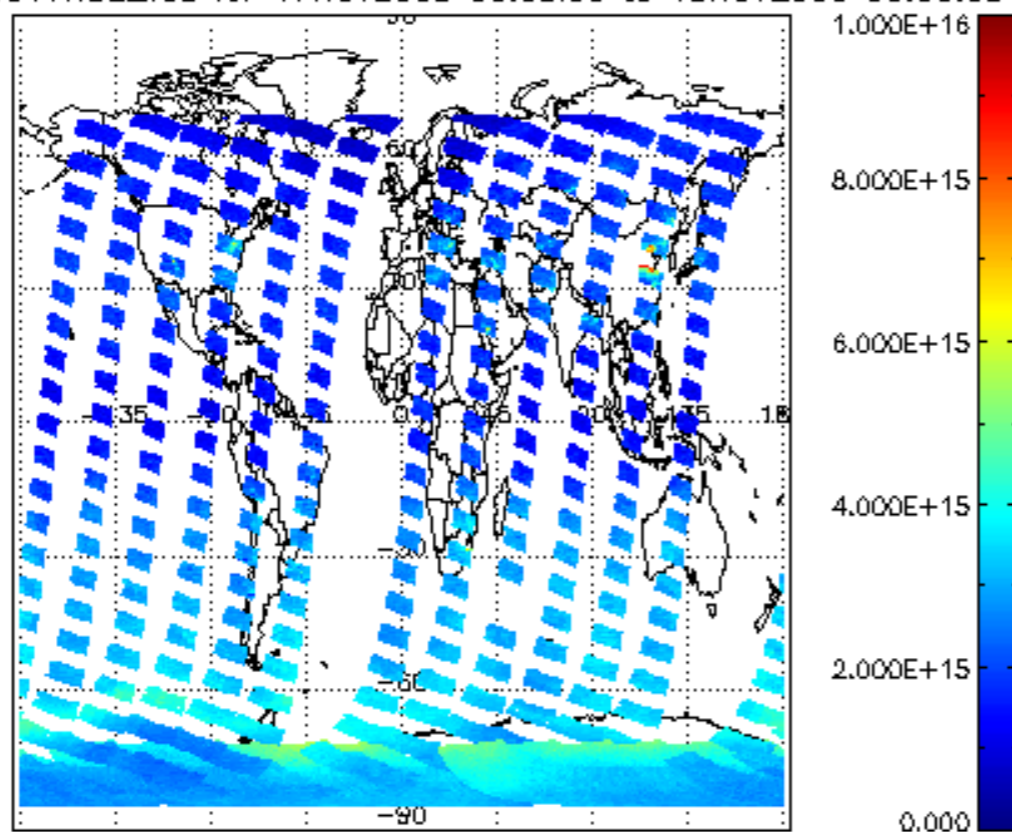
SCIOL2P_NADUV1NO2_vcd for 17NOV2008 00:00:00 to 18NOV2008 00:00:00
