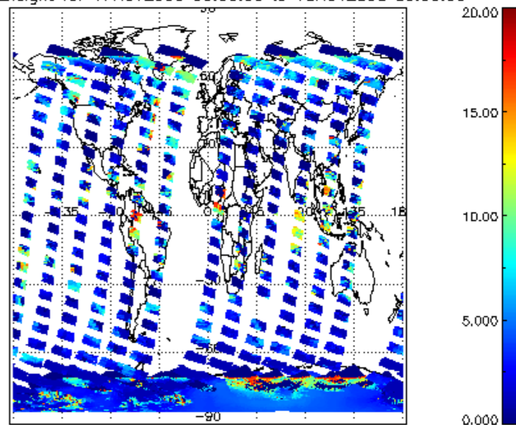
cL_top_height for 17NOV2008 00:00:00 to 18NOV2008 00:00:00
