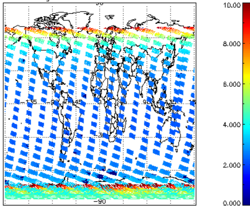
SCIOL2P_NADUV003_amf_gr for 15NOV2008 00:00:00 to 16NOV2008 00:00:00
