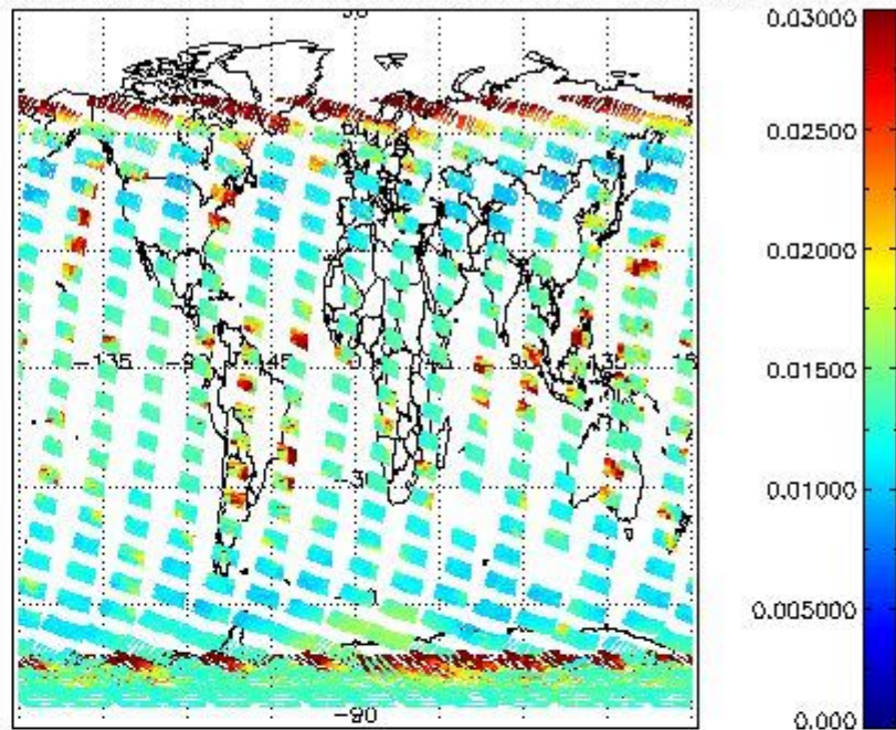
SCIOL2P_NADUV003_vcd_err for 15NOV2008 00:00:00 to 16NOV2008 00:00:00
