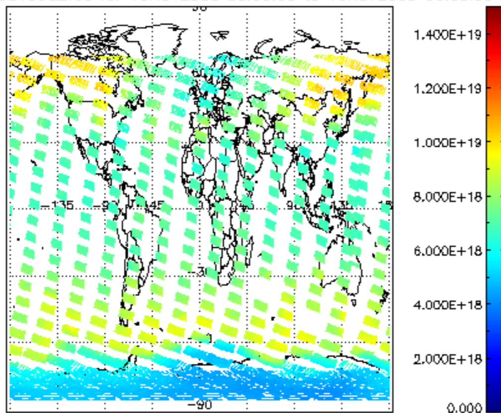
SCIOL2P_NADUV003_vcd for 15NOV2008 00:00:00 to 16NOV2008 00:00:00
