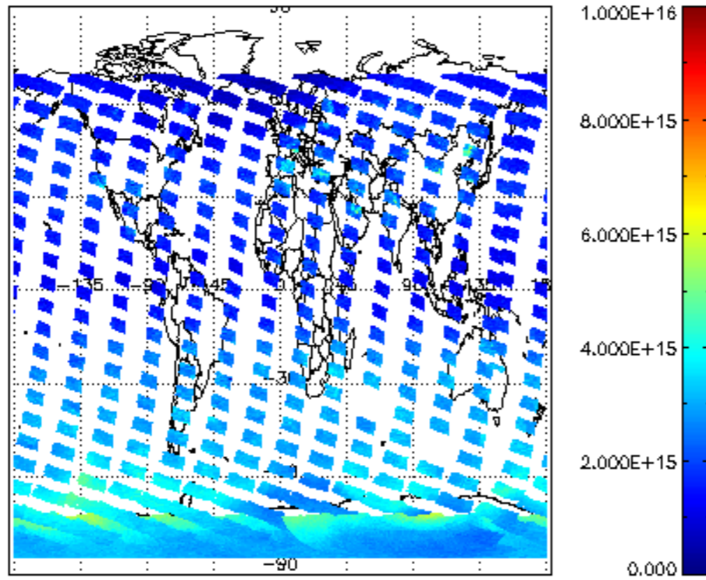
SCIOL2P_NADUV1NO2_vcd for 15NOV2008 00:00:00 to 16NOV2008 00:00:00
