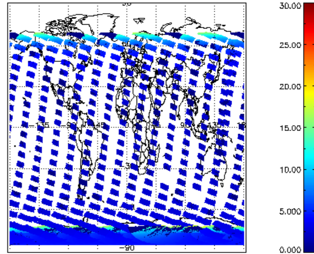
SCIOL2P_NADUV1NO2_amf_cl for 15NOV2008 00:00:00 to 16NOV2008 00:00:00
