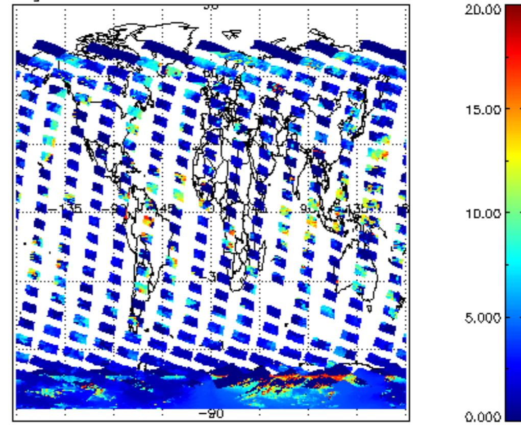
cL_top_height for 15NOV2008 00:00:00 to 16NOV2008 00:00:00
