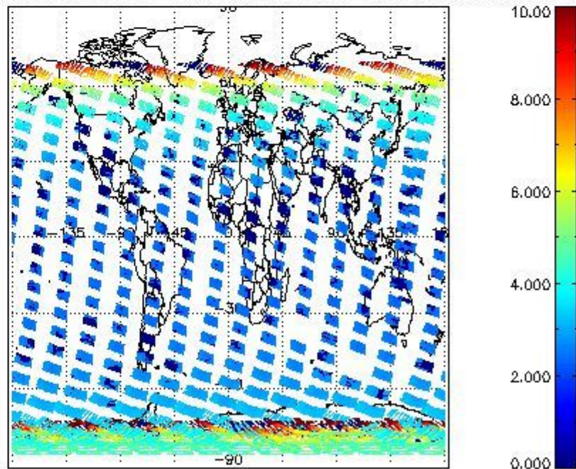
SCIOL2P_NADUV003_amf_cl for 15NOV2008 00:00:00 to 16NOV2008 00:00:00
