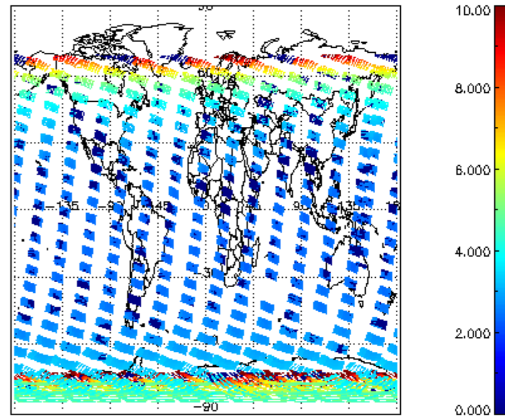
SCIOL2P_NADUV003_amf_cl for 15NOV2008 00:00:00 to 16NOV2008 00:00:00
