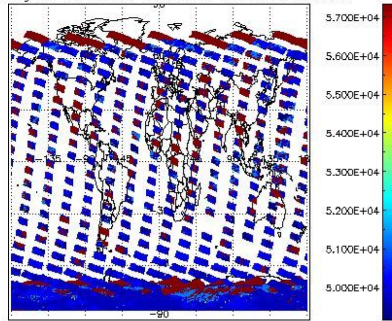
cloud_flags for 15NOV2008 00:00:00 to 16NOV2008 00:00:00
