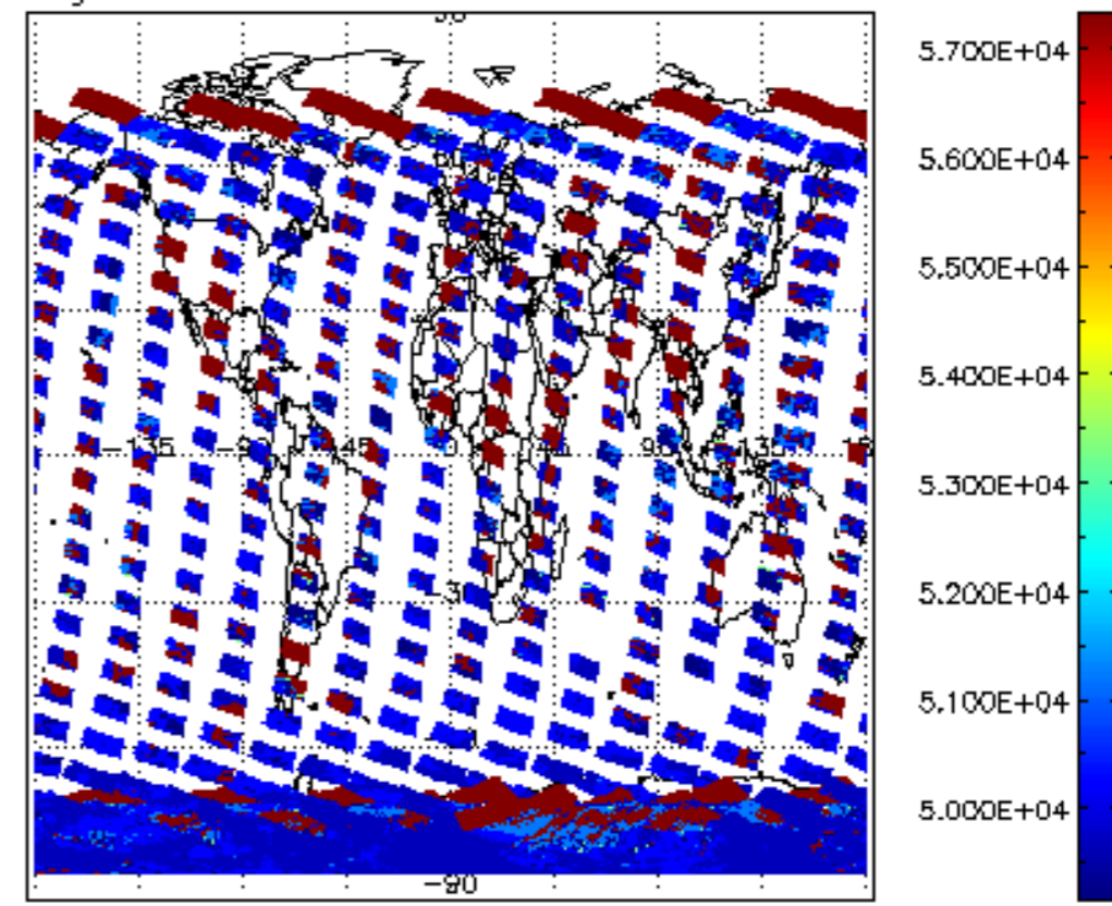
cloud_flags for 15NOV2008 00:00:00 to 16NOV2008 00:00:00
