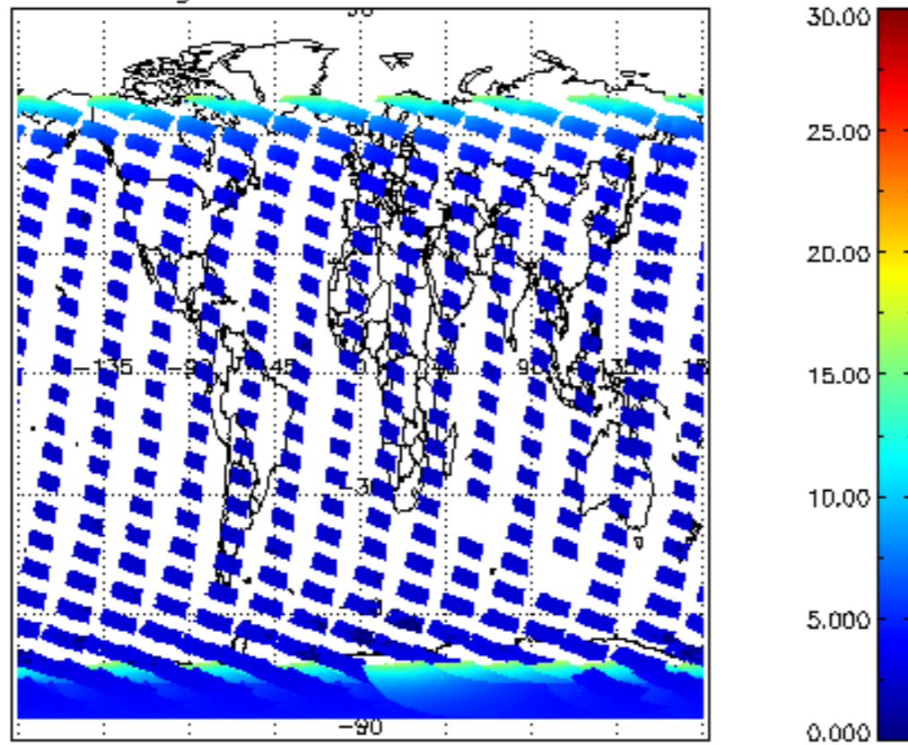
SCIOL2P_NADUV1NO2_amf_gr for 15NOV2008 00:00:00 to 16NOV2008 00:00:00
