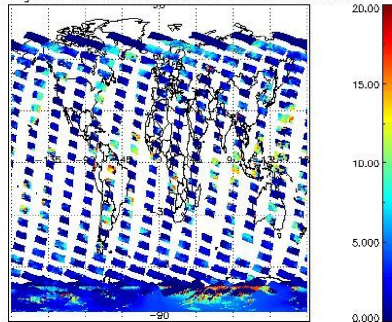
cL_top_height for 15NOV2008 00:00:00 to 16NOV2008 00:00:00
