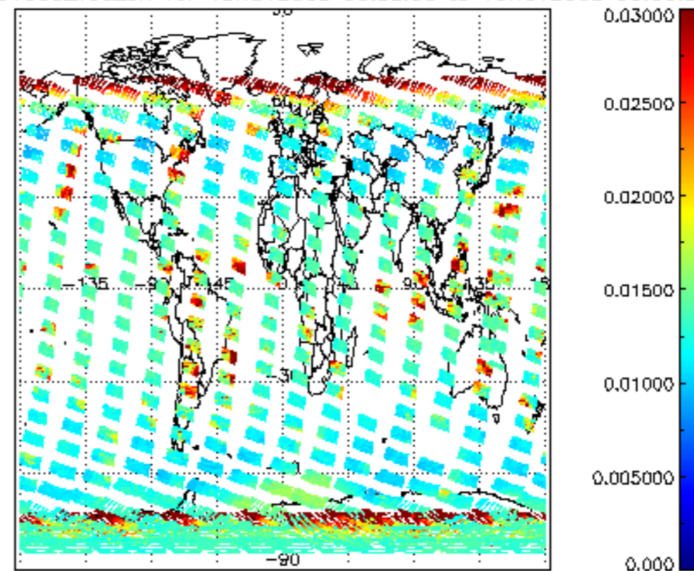
SCIOL2P_NADUV003_vcd_err for 15NOV2008 00:00:00 to 16NOV2008 00:00:00
