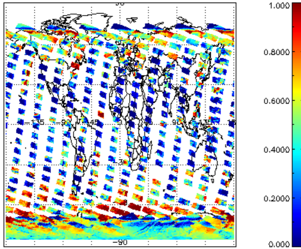
cLfrac for 15NOV2008 00:00:00 to 16NOV2008 00:00:00
