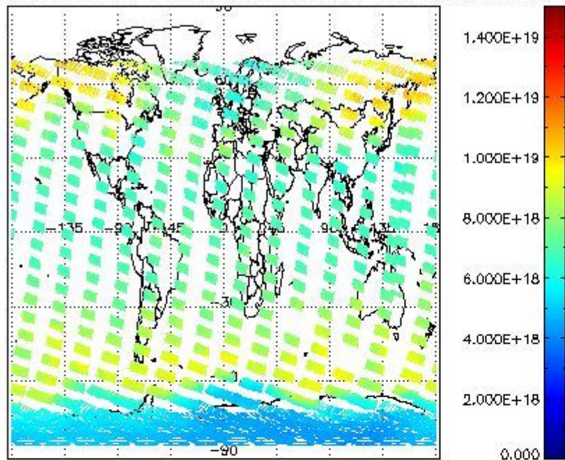
SCIOL2P_NADUV003_vcd for 15NOV2008 00:00:00 to 16NOV2008 00:00:00
