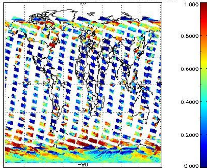
cLfrac for 15NOV2008 00:00:00 to 16NOV2008 00:00:00
