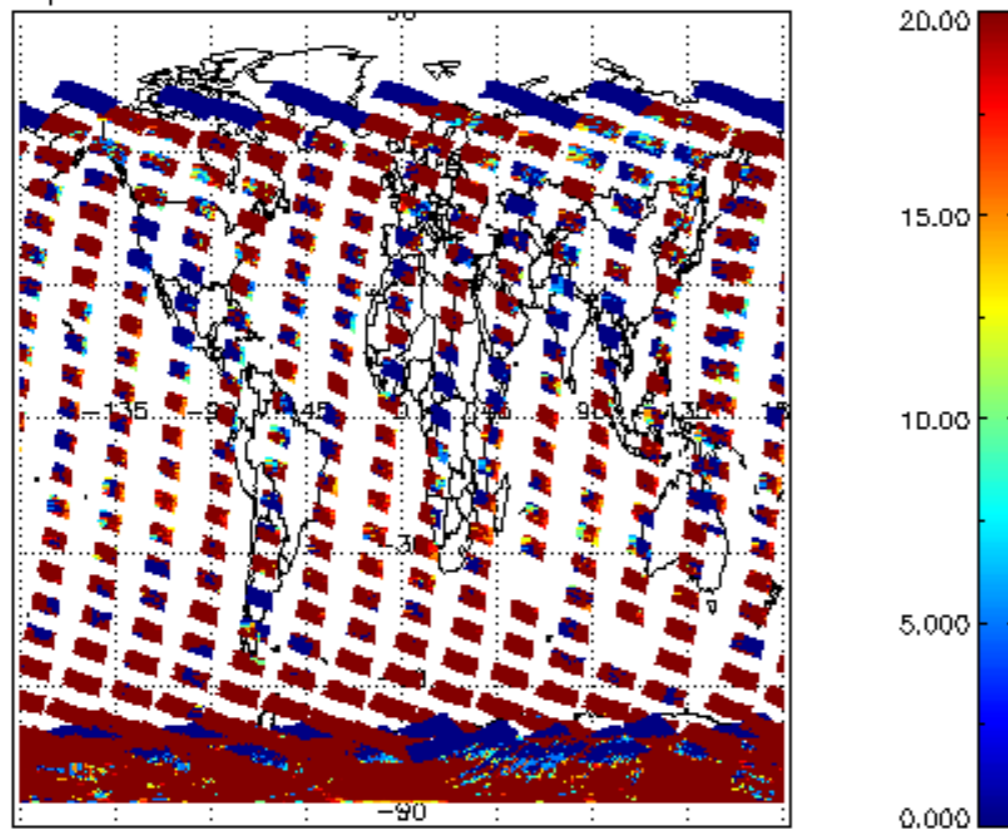
cL_opt_depth for 15NOV2008 00:00:00 to 16NOV2008 00:00:00
