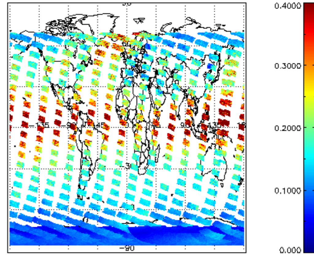
SCIOL2P_NADUV1NO2_vcd_err for 15NOV2008 00:00:00 to 16NOV2008 00:00:00
