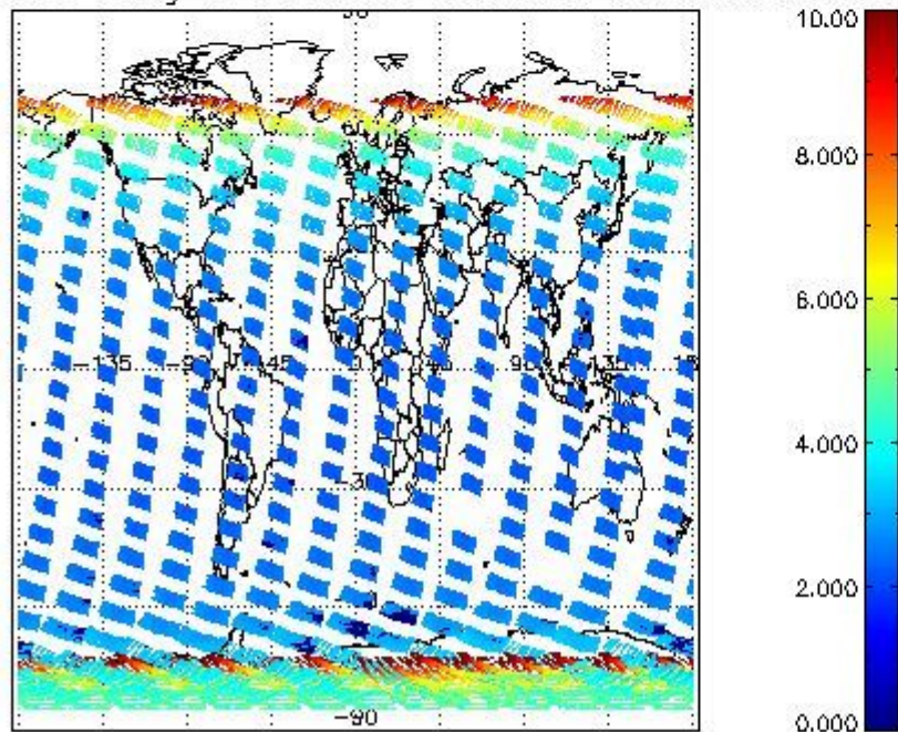
SCIOL2P_NADUV003_amf_gr for 15NOV2008 00:00:00 to 16NOV2008 00:00:00
