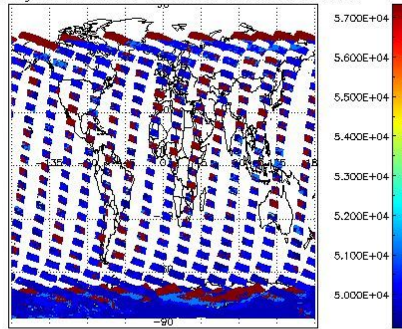
cloud_flags for 14NOV2008 00:00:00 to 15NOV2008 00:00:00
