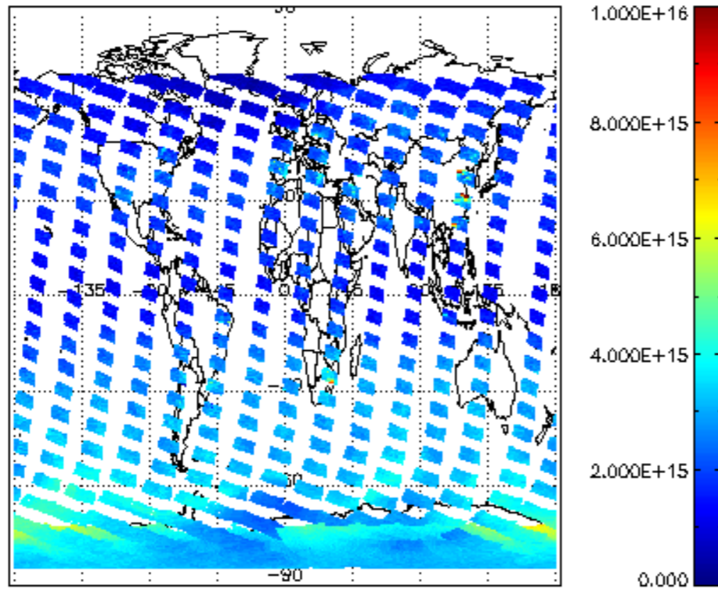
SCIOL2P_NADUV1NO2_vcd for 14NOV2008 00:00:00 to 15NOV2008 00:00:00
