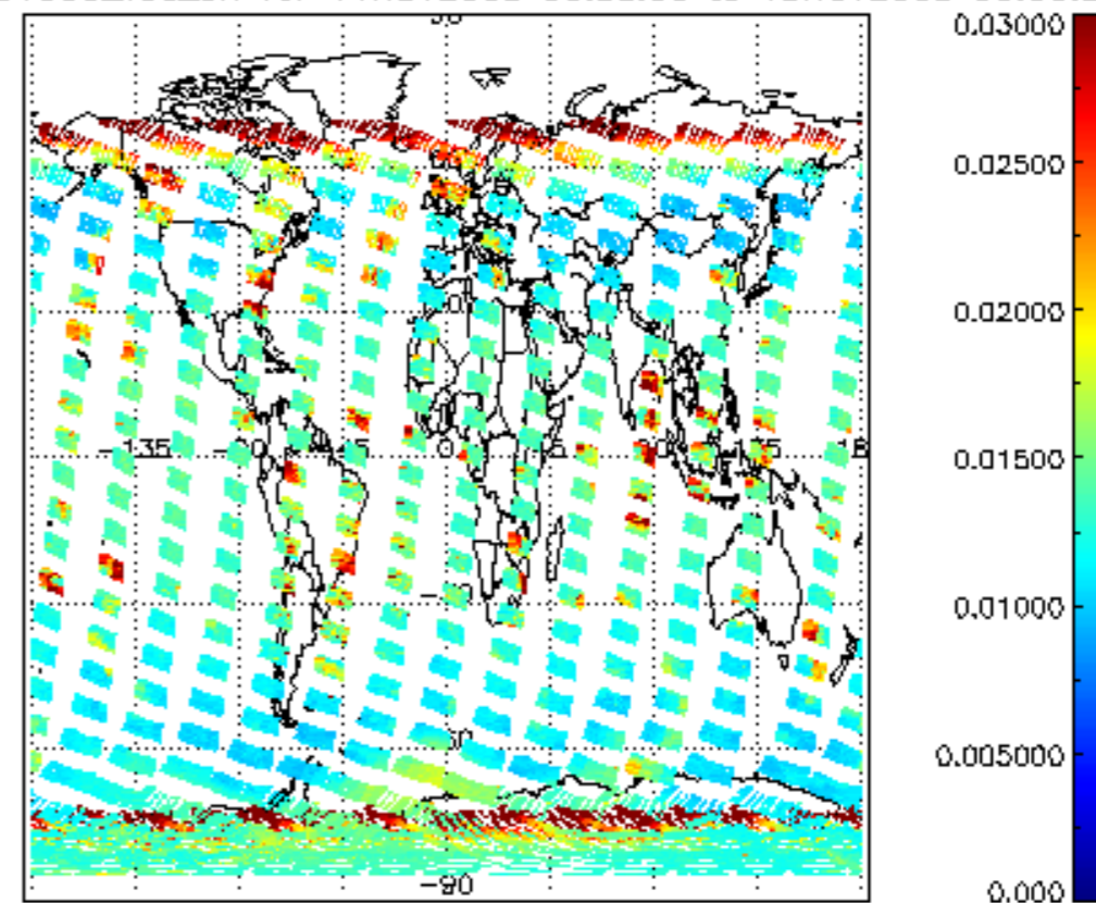
SCIOL2P_NADUV003_vcd_err for 14NOV2008 00:00:00 to 15NOV2008 00:00:00
