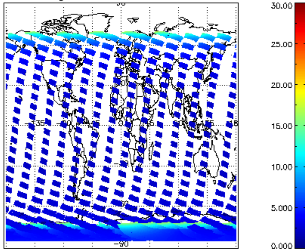
SCIOL2P_NADUV1NO2_amf_gr for 14NOV2008 00:00:00 to 15NOV2008 00:00:00
