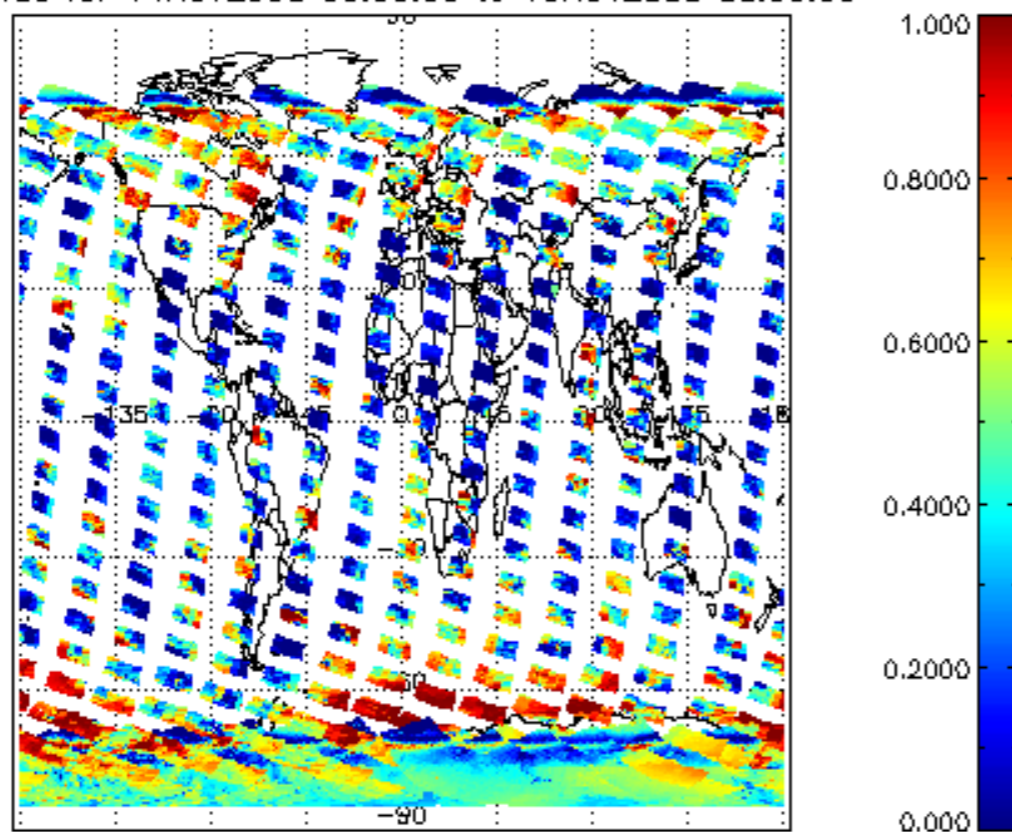
cLfrac for 14NOV2008 00:00:00 to 15NOV2008 00:00:00
