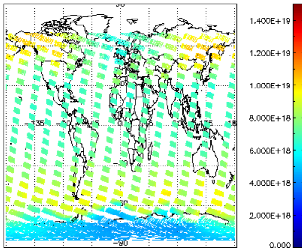
SCIOL2P_NADUV003_vcd for 14NOV2008 00:00:00 to 15NOV2008 00:00:00
