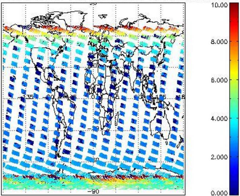
SCIOL2P_NADUV003_amf_cl for 14NOV2008 00:00:00 to 15NOV2008 00:00:00
