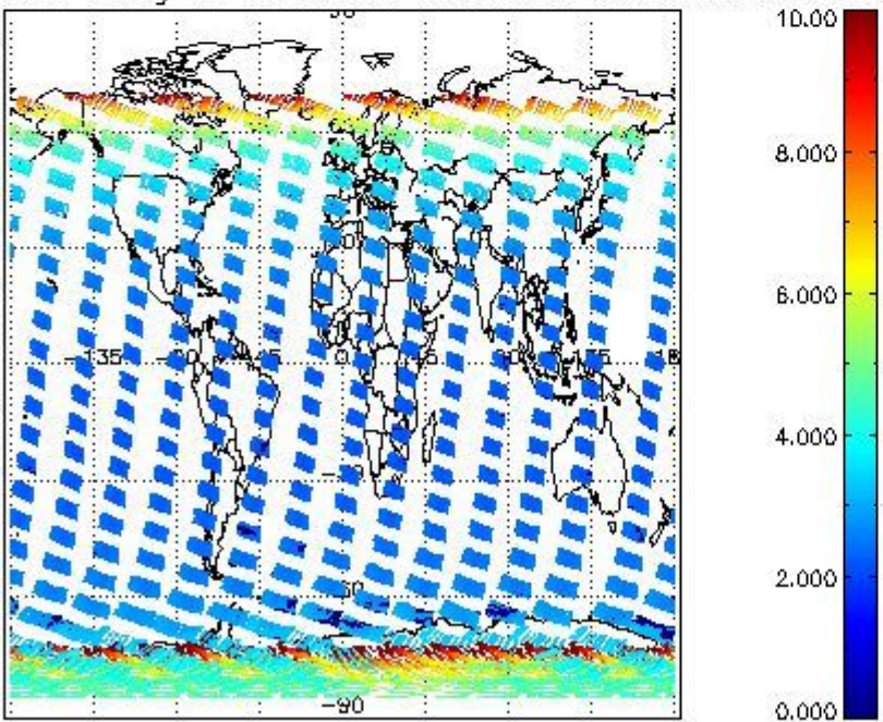
SCIOL2P_NADUV003_amf_gr for 14NOV2008 00:00:00 to 15NOV2008 00:00:00
