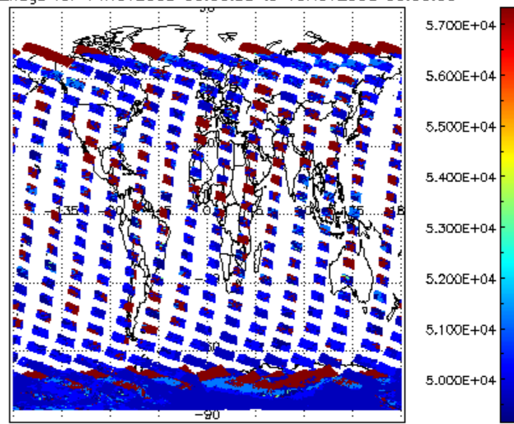
cloud_flags for 14NOV2008 00:00:00 to 15NOV2008 00:00:00
