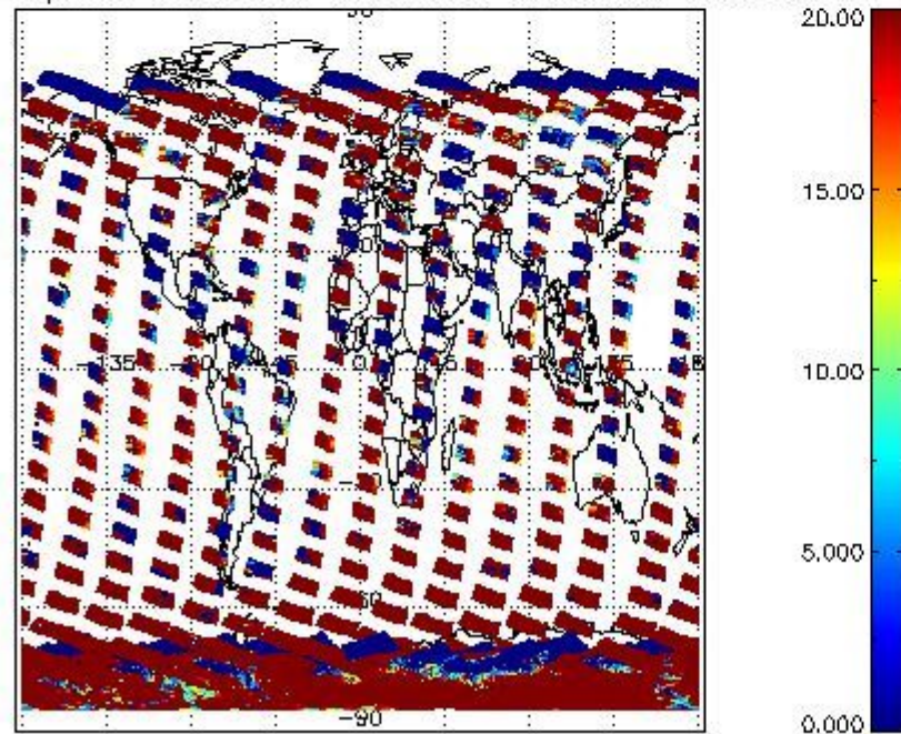
cLopt_depth for 14NOV2008 00:00:00 to 15NOV2008 00:00:00
