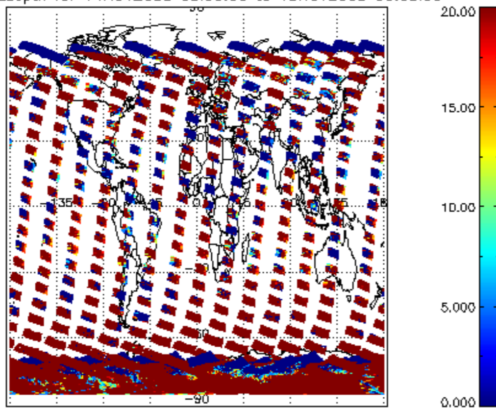
cL_opt_depth for 14NOV2008 00:00:00 to 15NOV2008 00:00:00
