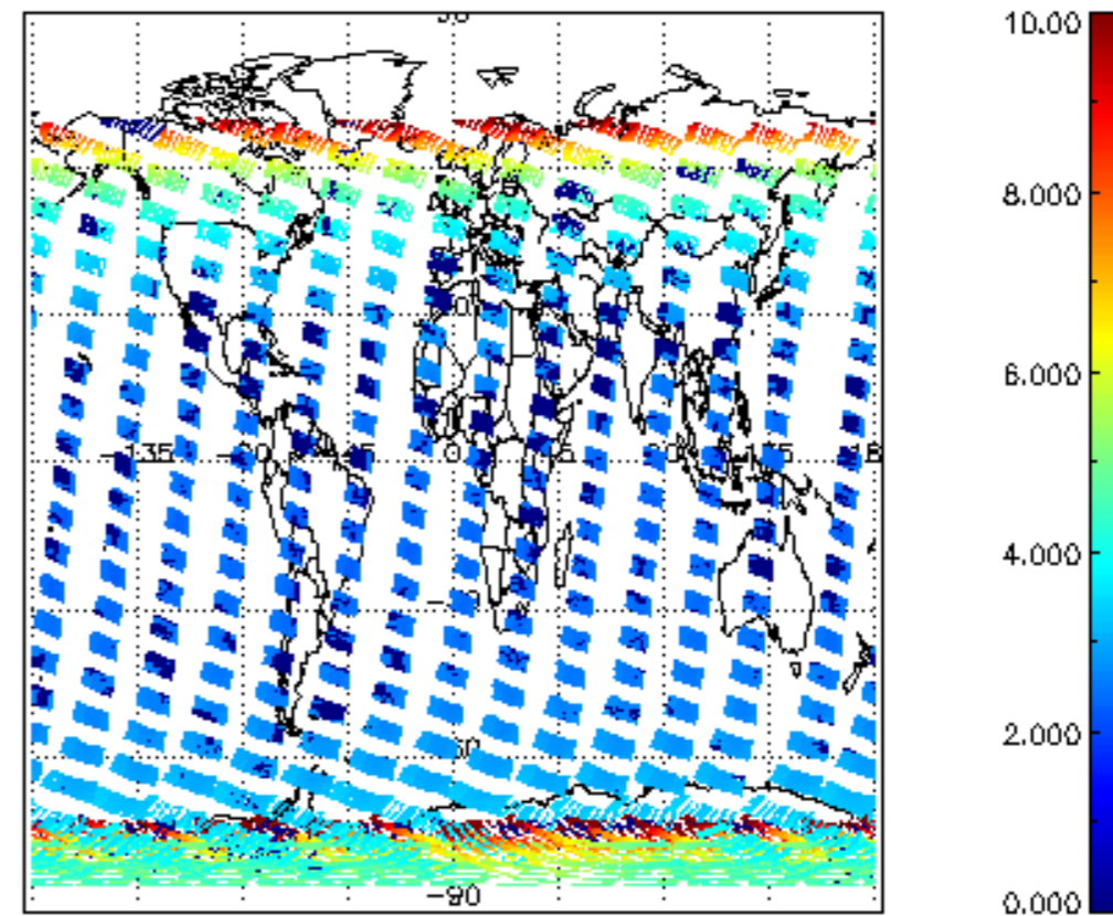
SCIOL2P_NADUV003_amf_cl for 14NOV2008 00:00:00 to 15NOV2008 00:00:00
