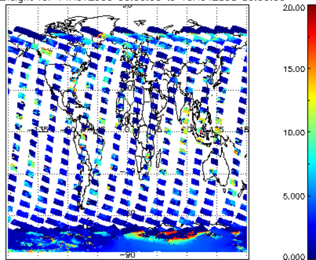
cL_top_height for 14NOV2008 00:00:00 to 15NOV2008 00:00:00
