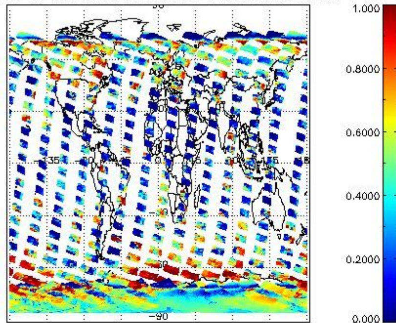
cLfrac for 14NOV2008 00:00:00 to 15NOV2008 00:00:00
