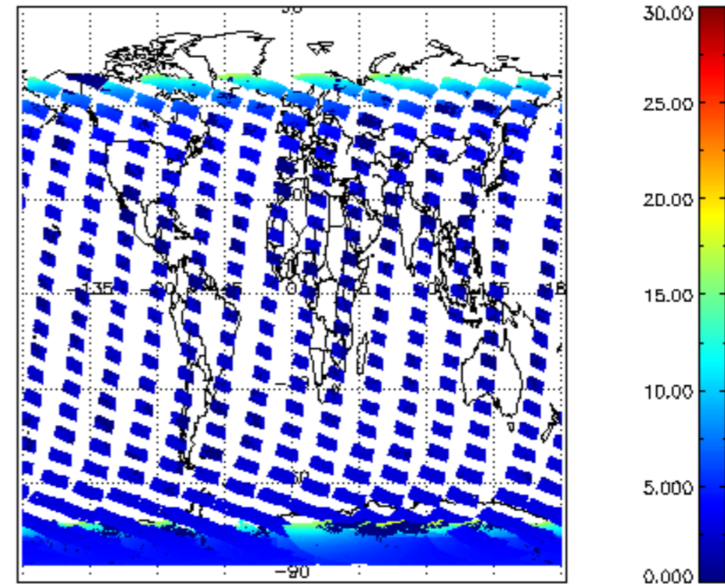
SCIOL2P_NADUV1NO2_amf_cl for 14NOV2008 00:00:00 to 15NOV2008 00:00:00
