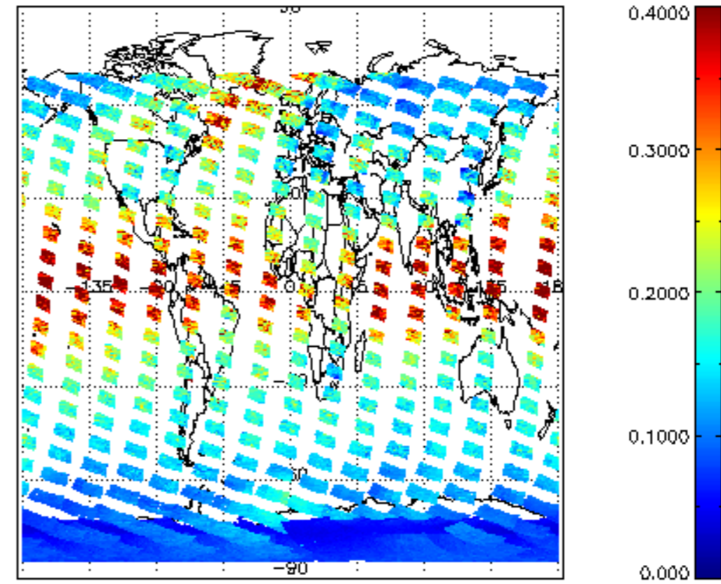
SCIOL2P_NADUV1NO2_vcd_err for 14NOV2008 00:00:00 to 15NOV2008 00:00:00
