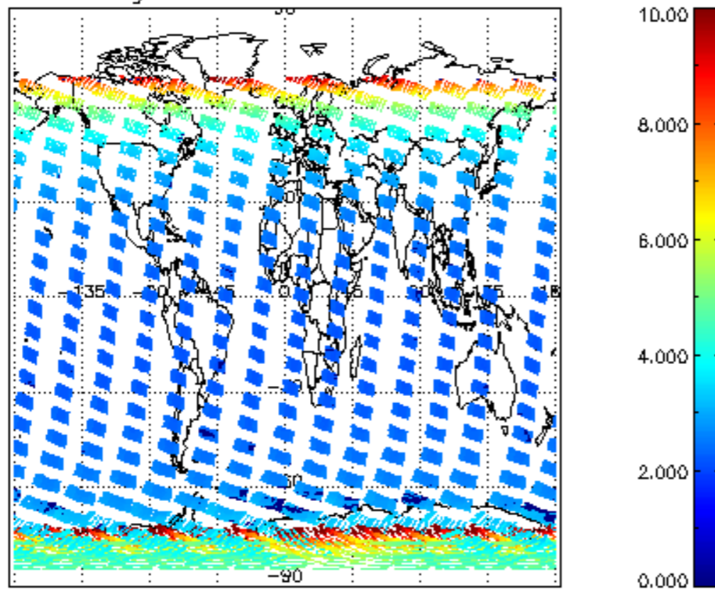
SCIOL2P_NADUV003_amf_gr for 14NOV2008 00:00:00 to 15NOV2008 00:00:00
