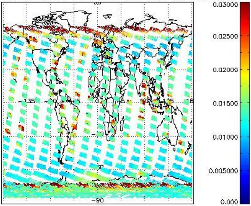
SCIOL2P_NADUV003_vcd_err for 14NOV2008 00:00:00 to 15NOV2008 00:00:00
