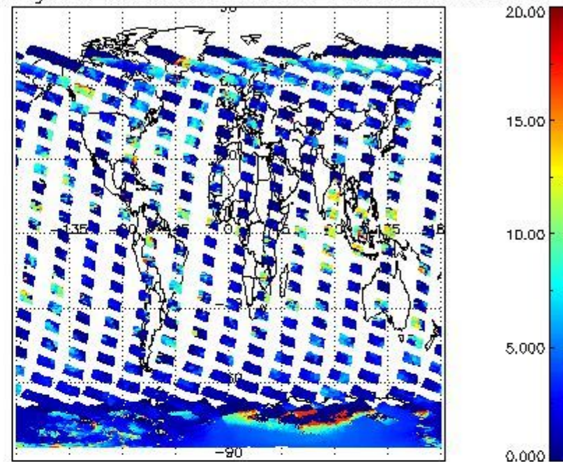
cL_top_height for 14NOV2008 00:00:00 to 15NOV2008 00:00:00
