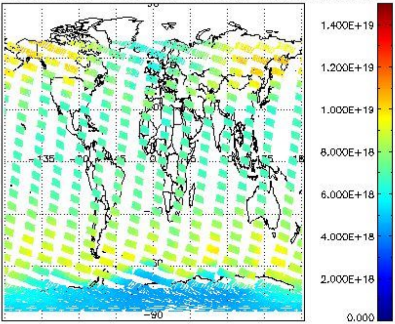
SCIOL2P_NADUV003_vcd for 14NOV2008 00:00:00 to 15NOV2008 00:00:00
