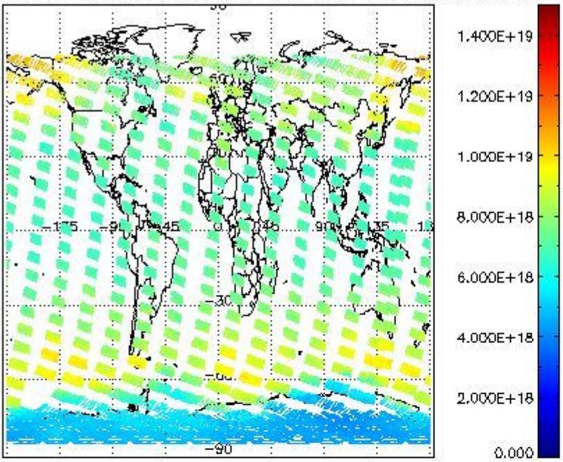
SCIOL2P_NADUV003_vcd for 09NOV2008 00:00:00 to 10NOV2008 00:00:00
