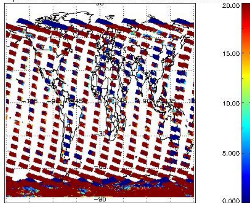
cLopt_depth for 09NOV2008 00:00:00 to 10NOV2008 00:00:00
