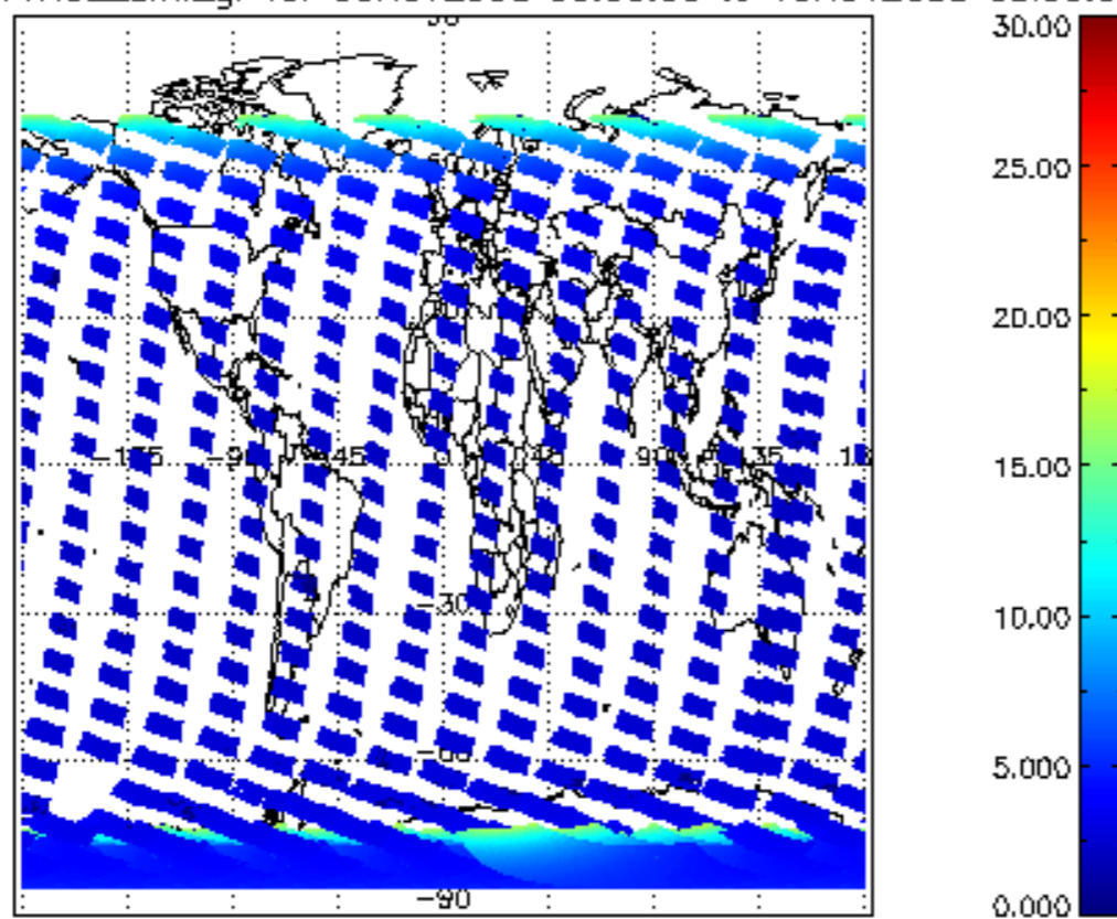
SCIOL2P_NADUV1NO2_amf_gr for 09NOV2008 00:00:00 to 10NOV2008 00:00:00
