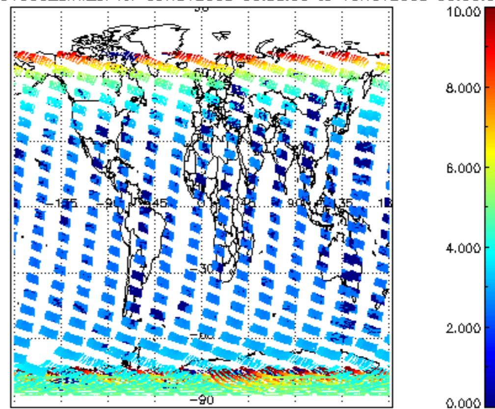
SCIOL2P_NADUV003_amf_cl for 09NOV2008 00:00:00 to 10NOV2008 00:00:00
