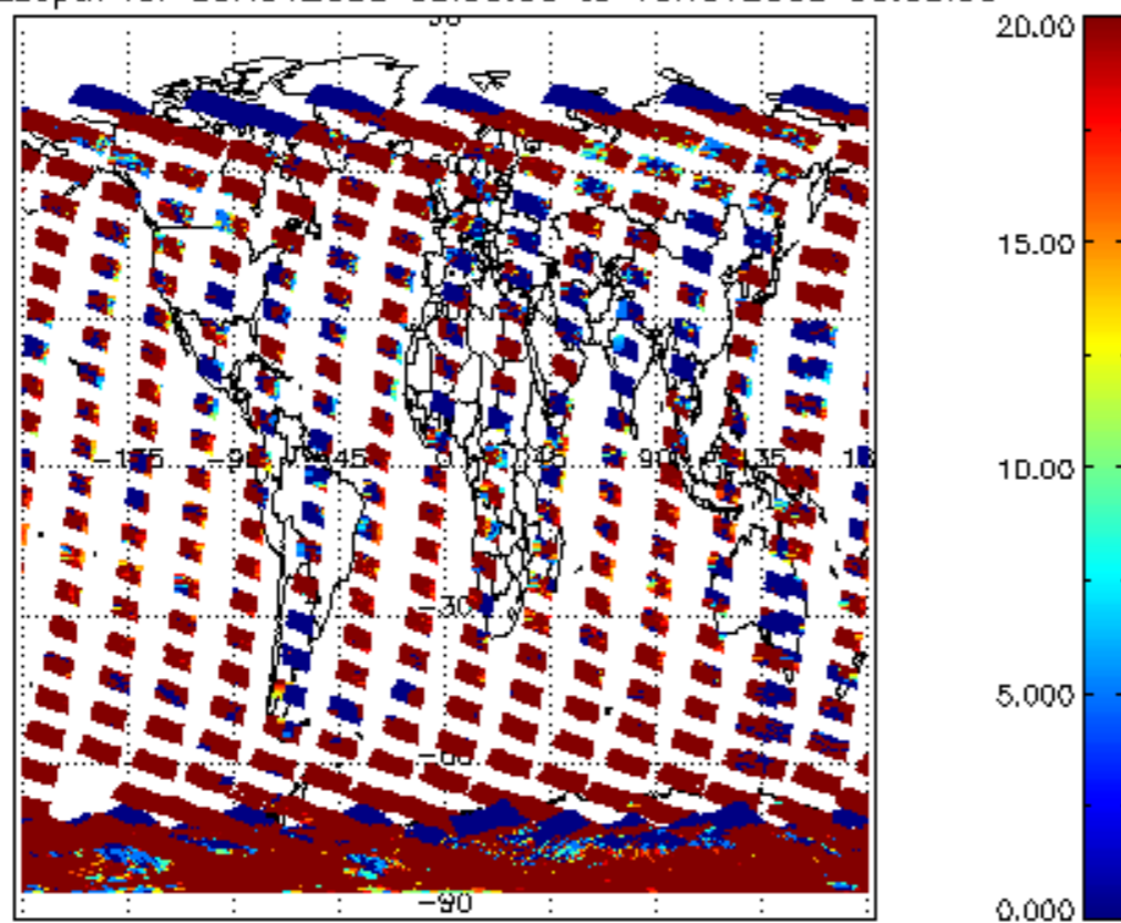
cL_opt_depth for 09NOV2008 00:00:00 to 10NOV2008 00:00:00
