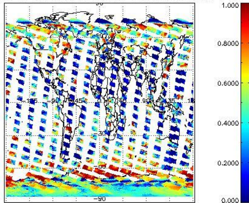
cLfrac for 09NOV2008 00:00:00 to 10NOV2008 00:00:00
