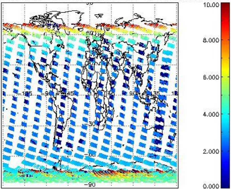
SCIOL2P_NADUV003_amf_cl for 09NOV2008 00:00:00 to 10NOV2008 00:00:00
