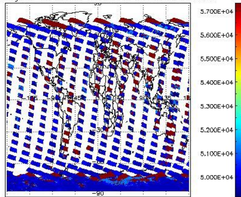
cloud_flags for 09NOV2008 00:00:00 to 10NOV2008 00:00:00
