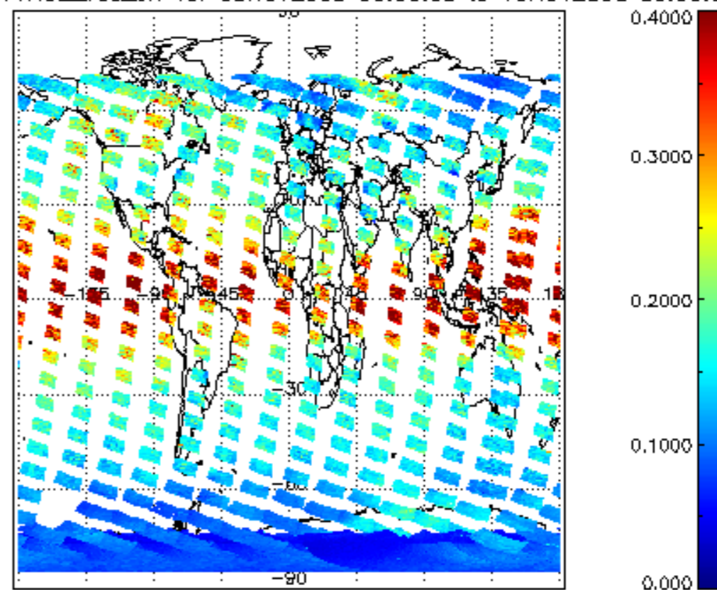
SCIOL2P_NADUV1NO2_vcd_err for 09NOV2008 00:00:00 to 10NOV2008 00:00:00
