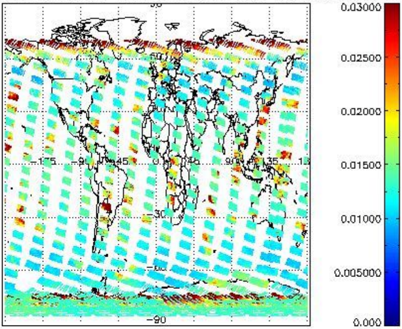
SCIOL2P_NADUV003_vcd_err for 09NOV2008 00:00:00 to 10NOV2008 00:00:00
