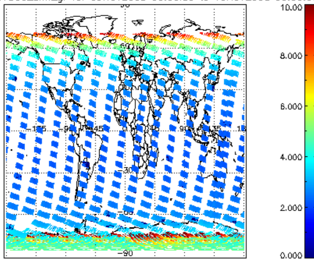
SCIOL2P_NADUV003_amf_gr for 09NOV2008 00:00:00 to 10NOV2008 00:00:00
