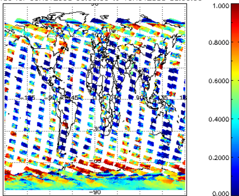
cLfrac for 09NOV2008 00:00:00 to 10NOV2008 00:00:00
