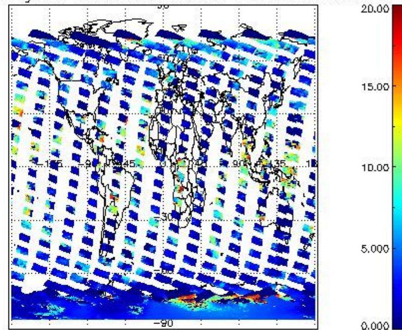
cL_top_height for 09NOV2008 00:00:00 to 10NOV2008 00:00:00
