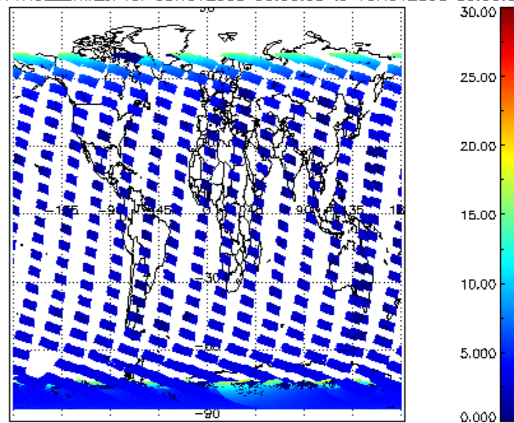
SCIOL2P_NADUV1NO2_amf_cl for 09NOV2008 00:00:00 to 10NOV2008 00:00:00
