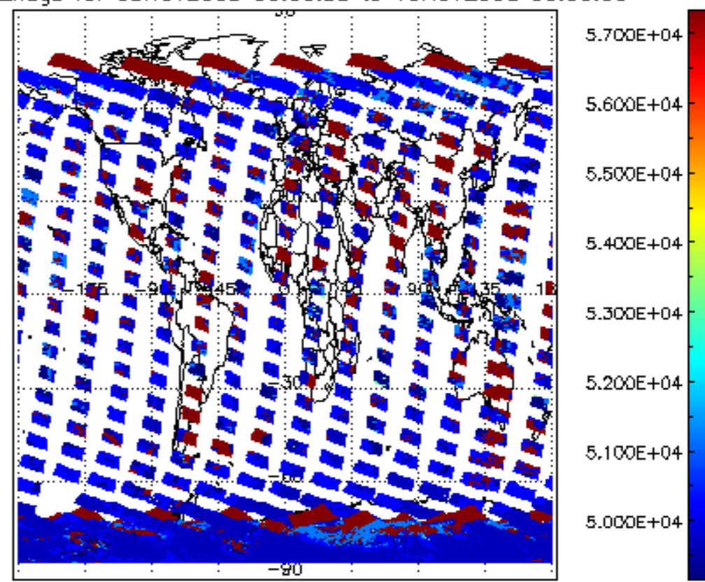
cloud_flags for 09NOV2008 00:00:00 to 10NOV2008 00:00:00
