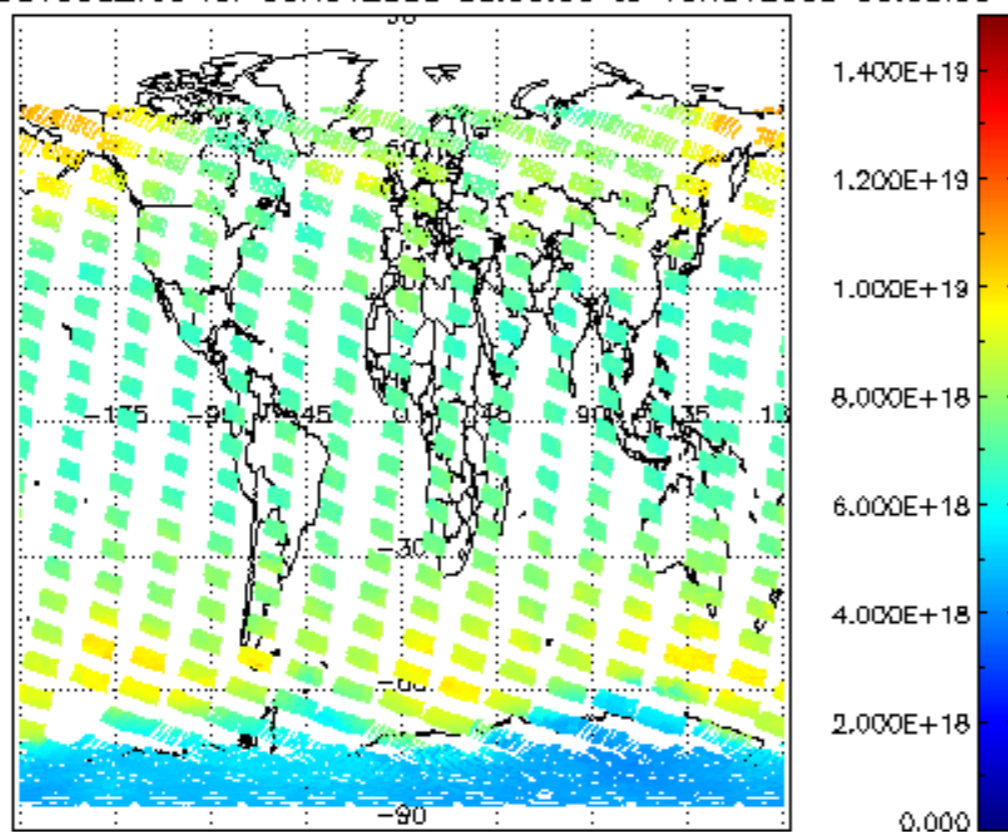
SCIOL2P_NADUV003_vcd for 09NOV2008 00:00:00 to 10NOV2008 00:00:00
