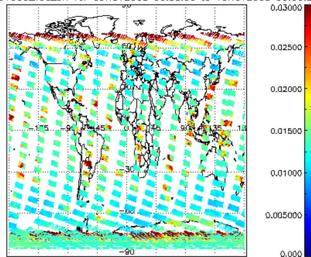
SCIOL2P_NADUV003_vcd_err for 09NOV2008 00:00:00 to 10NOV2008 00:00:00
