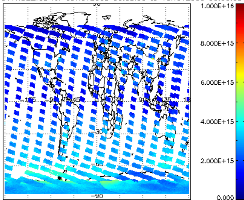
SCIOL2P_NADUV1NO2_vcd for 09NOV2008 00:00:00 to 10NOV2008 00:00:00
