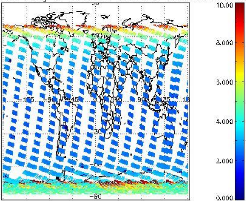
SCIOL2P_NADUV003_amf_gr for 09NOV2008 00:00:00 to 10NOV2008 00:00:00
