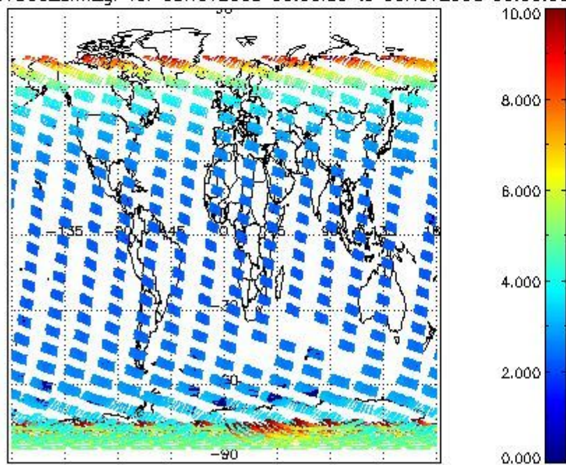
SCIOL2P_NADUV003_amf_gr for 05NOV2008 00:00:00 to 06NOV2008 00:00:00
