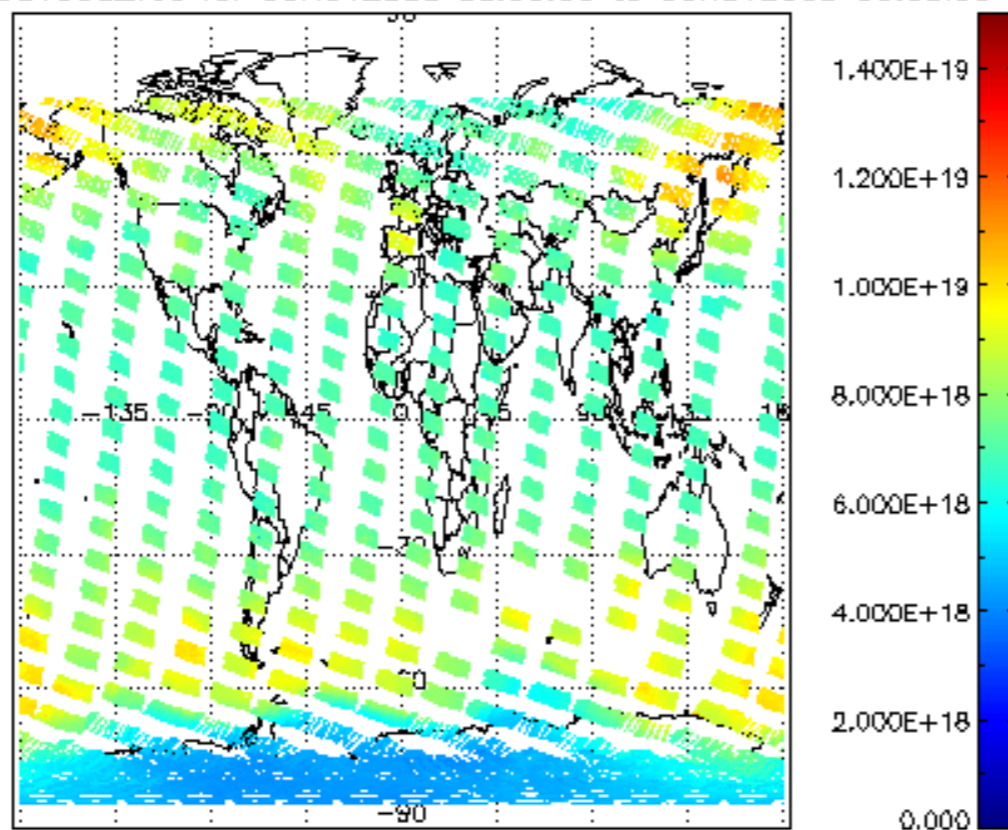
SCIOL2P_NADUV003_vcd for 05NOV2008 00:00:00 to 06NOV2008 00:00:00
