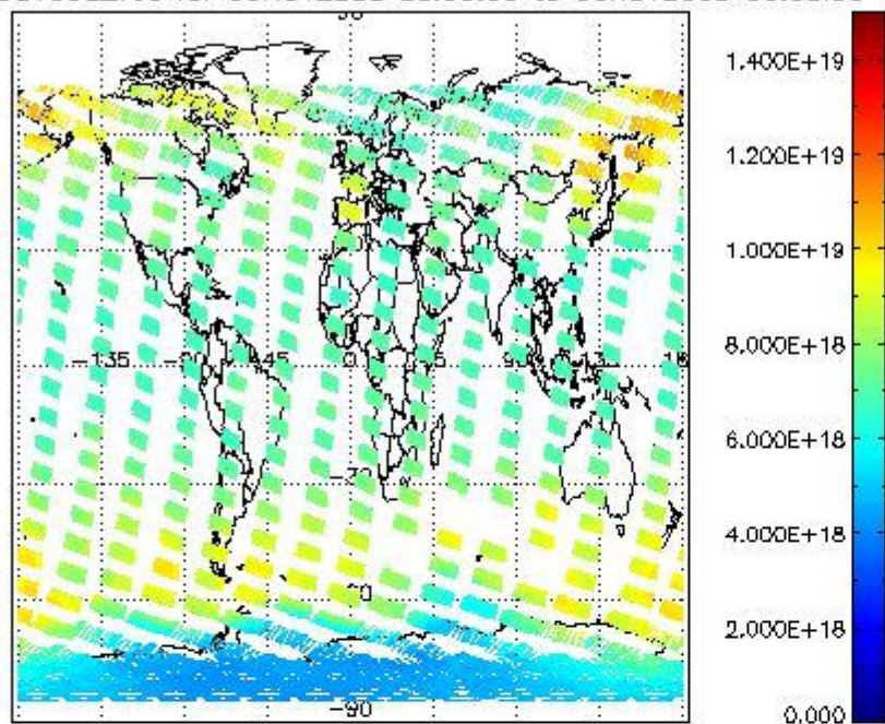
SCIOL2P_NADUV003_vcd for 05NOV2008 00:00:00 to 06NOV2008 00:00:00
