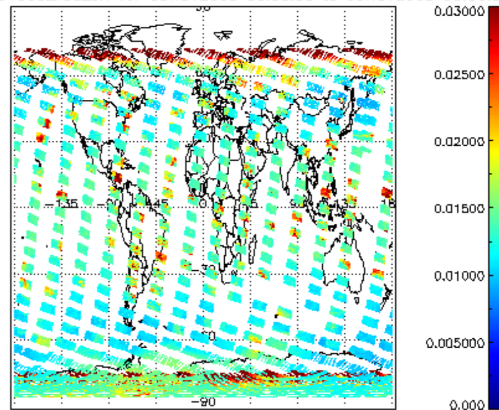
SCIOL2P_NADUV003_vcd_err for 05NOV2008 00:00:00 to 06NOV2008 00:00:00
