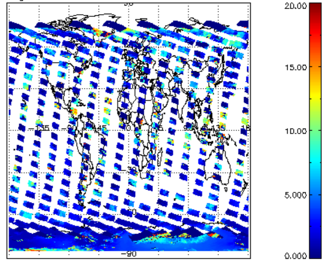
cL_top_height for 05NOV2008 00:00:00 to 06NOV2008 00:00:00
