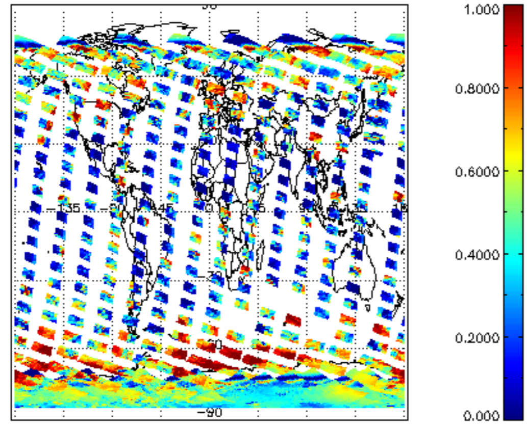
cLfrac for 05NOV2008 00:00:00 to 06NOV2008 00:00:00
