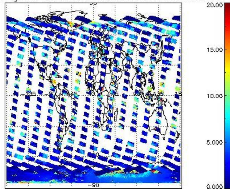
cL_top_height for 05NOV2008 00:00:00 to 06NOV2008 00:00:00
