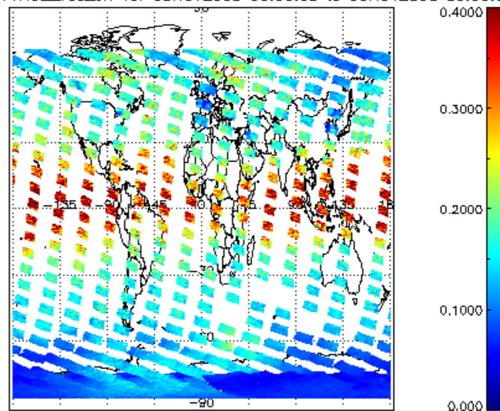
SCIOL2P_NADUV1NO2_vcd_err for 05NOV2008 00:00:00 to 06NOV2008 00:00:00
