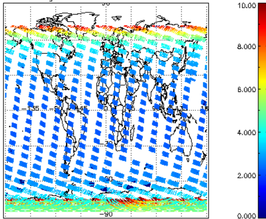
SCIOL2P_NADUV003_amf_gr for 05NOV2008 00:00:00 to 06NOV2008 00:00:00
