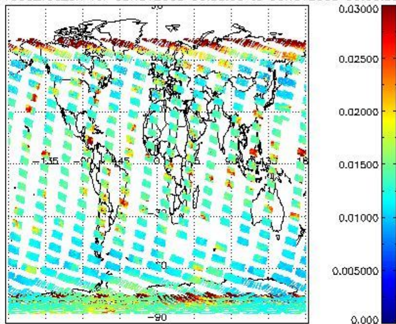
SCIOL2P_NADUV003_vcd_err for 05NOV2008 00:00:00 to 06NOV2008 00:00:00
