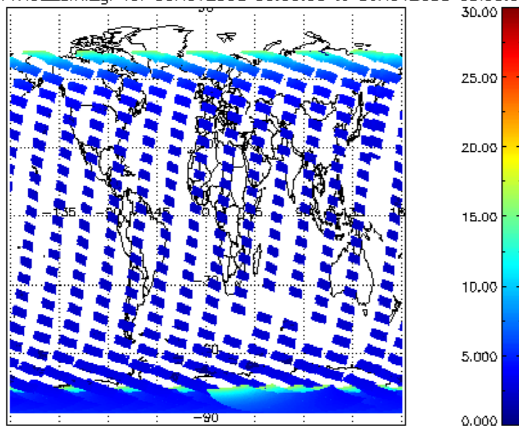
SCIOL2P_NADUV1NO2_amf_gr for 05NOV2008 00:00:00 to 06NOV2008 00:00:00
