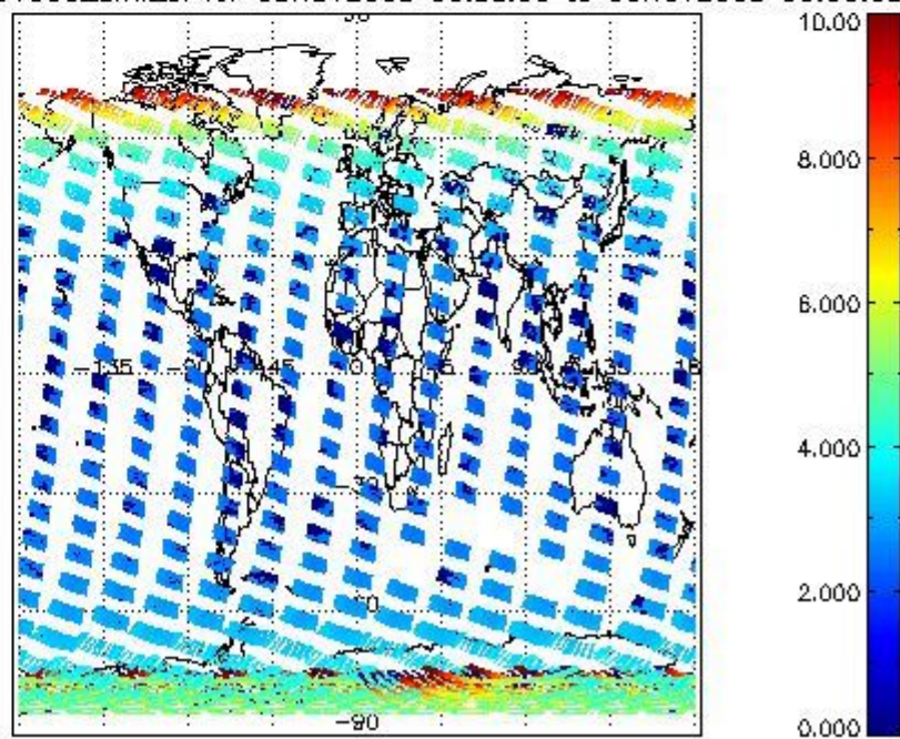
SCIOL2P_NADUV003_amf_cl for 05NOV2008 00:00:00 to 06NOV2008 00:00:00
