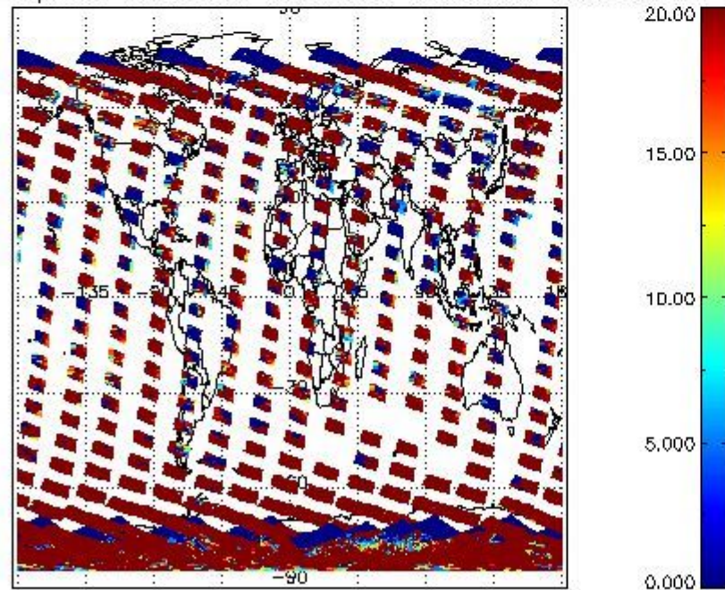
cLopt_depth for 05NOV2008 00:00:00 to 06NOV2008 00:00:00
