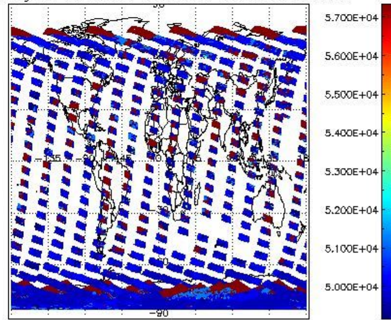
cloud_flags for 05NOV2008 00:00:00 to 06NOV2008 00:00:00
