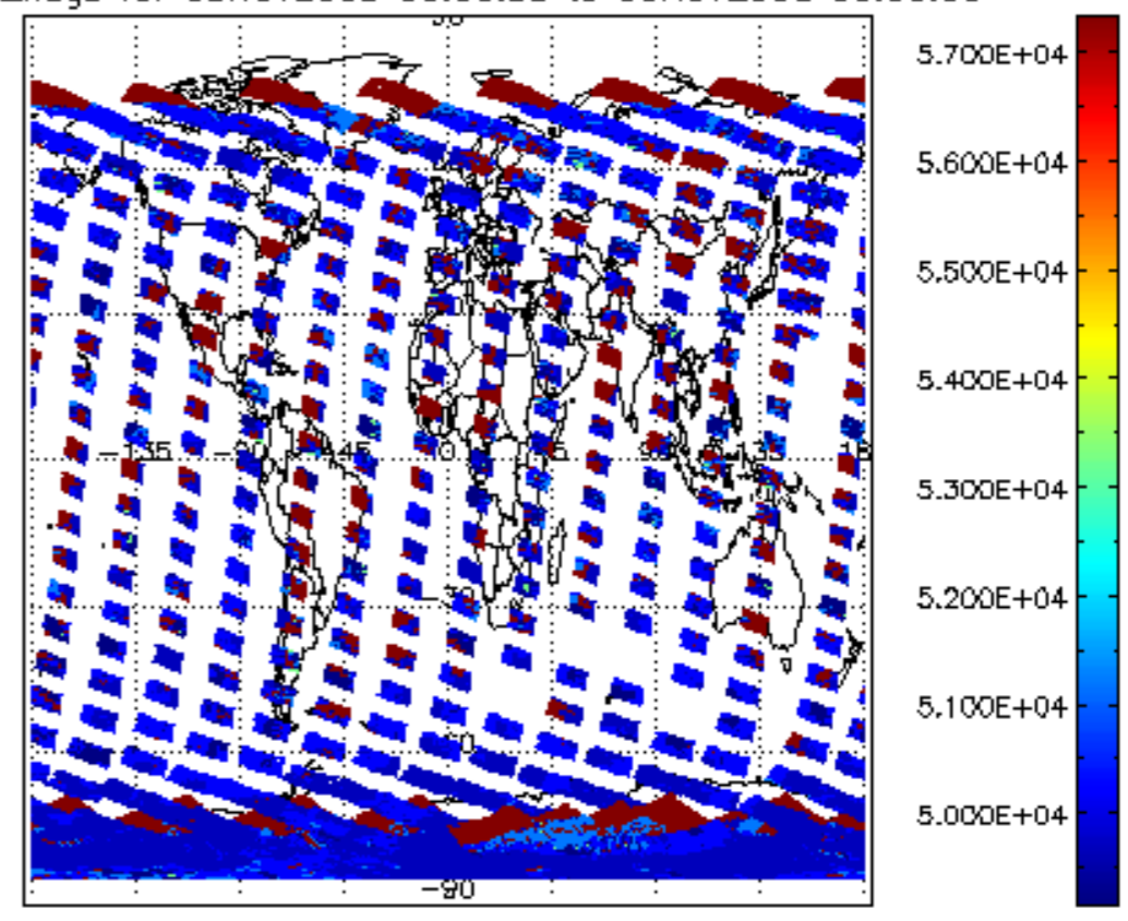
cloud_flags for 05NOV2008 00:00:00 to 06NOV2008 00:00:00
