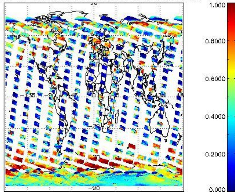
cLfrac for 05NOV2008 00:00:00 to 06NOV2008 00:00:00
