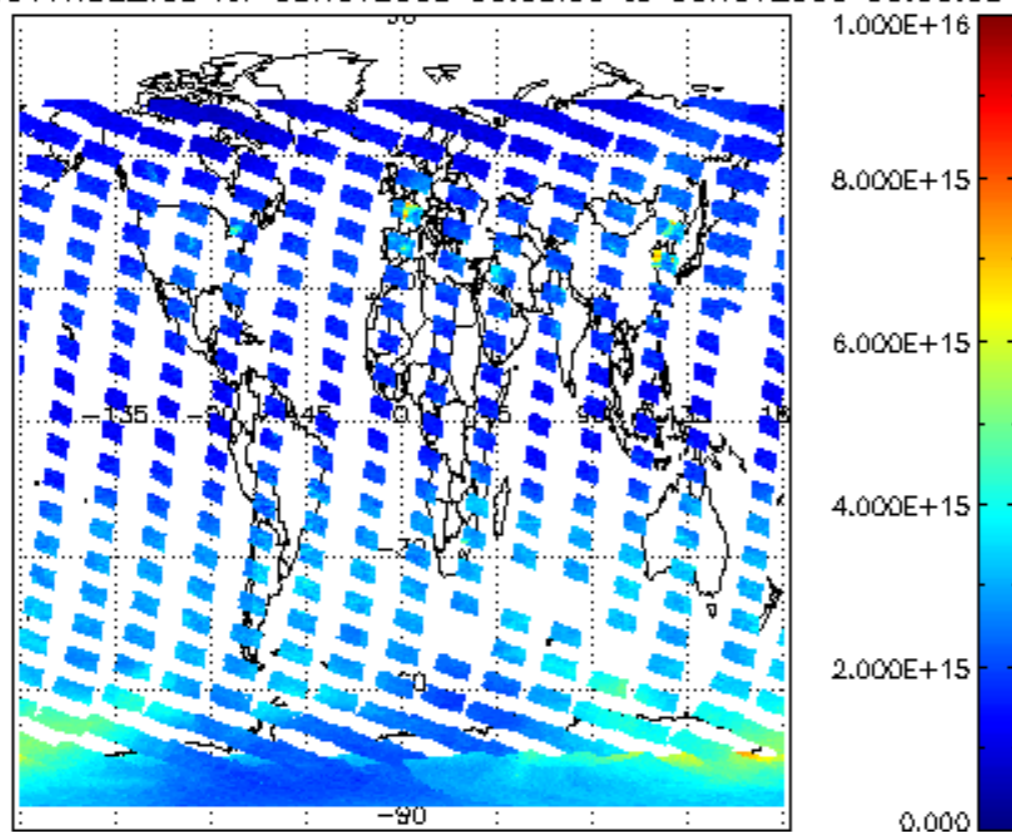
SCIOL2P_NADUV1NO2_vcd for 05NOV2008 00:00:00 to 06NOV2008 00:00:00
