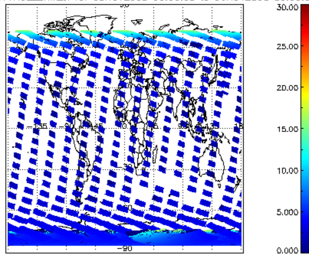
SCIOL2P_NADUV1NO2_amf_cl for 05NOV2008 00:00:00 to 06NOV2008 00:00:00
