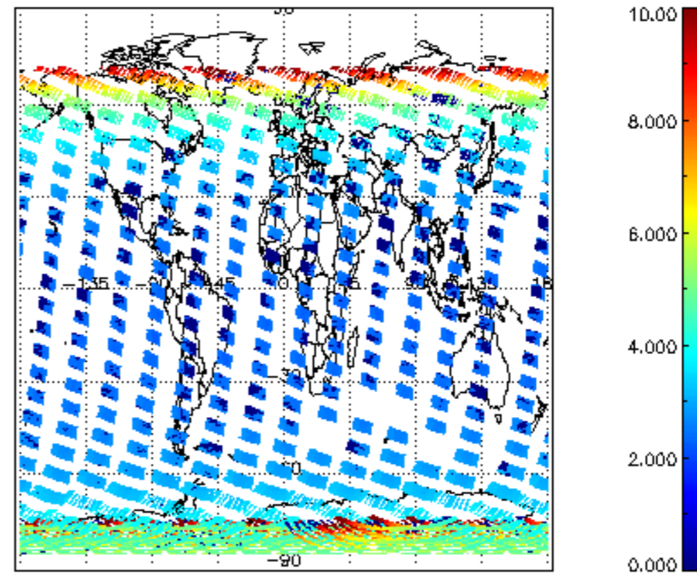
SCIOL2P_NADUV003_amf_cl for 05NOV2008 00:00:00 to 06NOV2008 00:00:00
