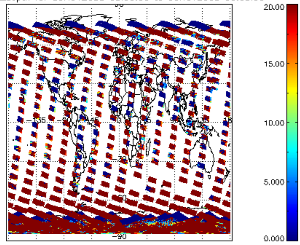
cL_opt_depth for 05NOV2008 00:00:00 to 06NOV2008 00:00:00
