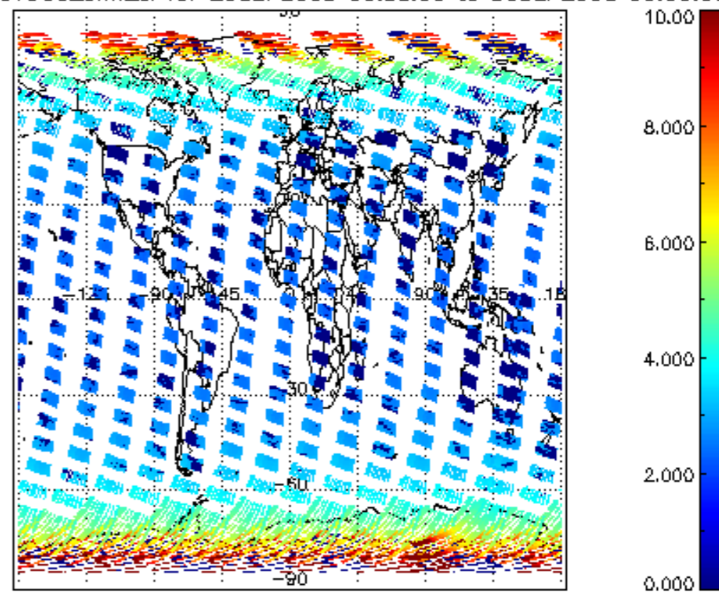
SCIOL2P_NADUV003_amf_cl for 29SEP2008 00:00:00 to 30SEP2008 00:00:00
