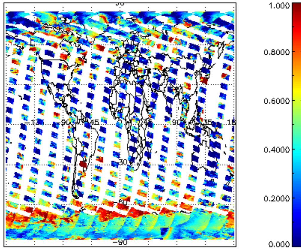
cl_frac for 29SEP2008 00:00:00 to 30SEP2008 00:00:00
