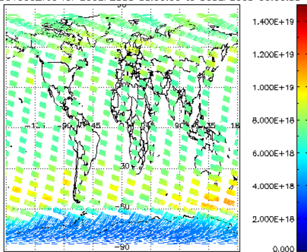
SCIOL2P_NADUV003_vcd for 29SEP2008 00:00:00 to 30SEP2008 00:00:00
