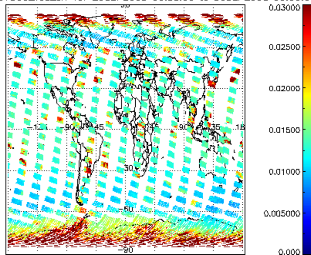
SCIOL2P_NADUV003_vcd_err for 29SEP2008 00:00:00 to 30SEP2008 00:00:00
