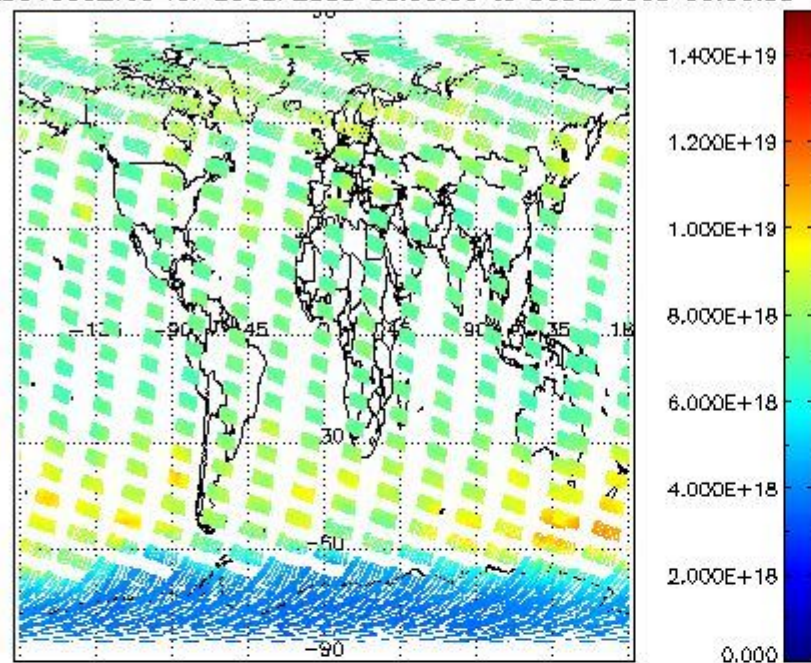
SCIOL2P_NADUV003_vcd for 29SEP2008 00:00:00 to 30SEP2008 00:00:00
