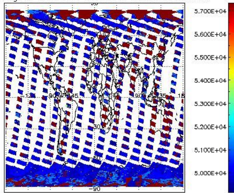
cloud_flags for 29SEP2008 00:00:00 to 30SEP2008 00:00:00
