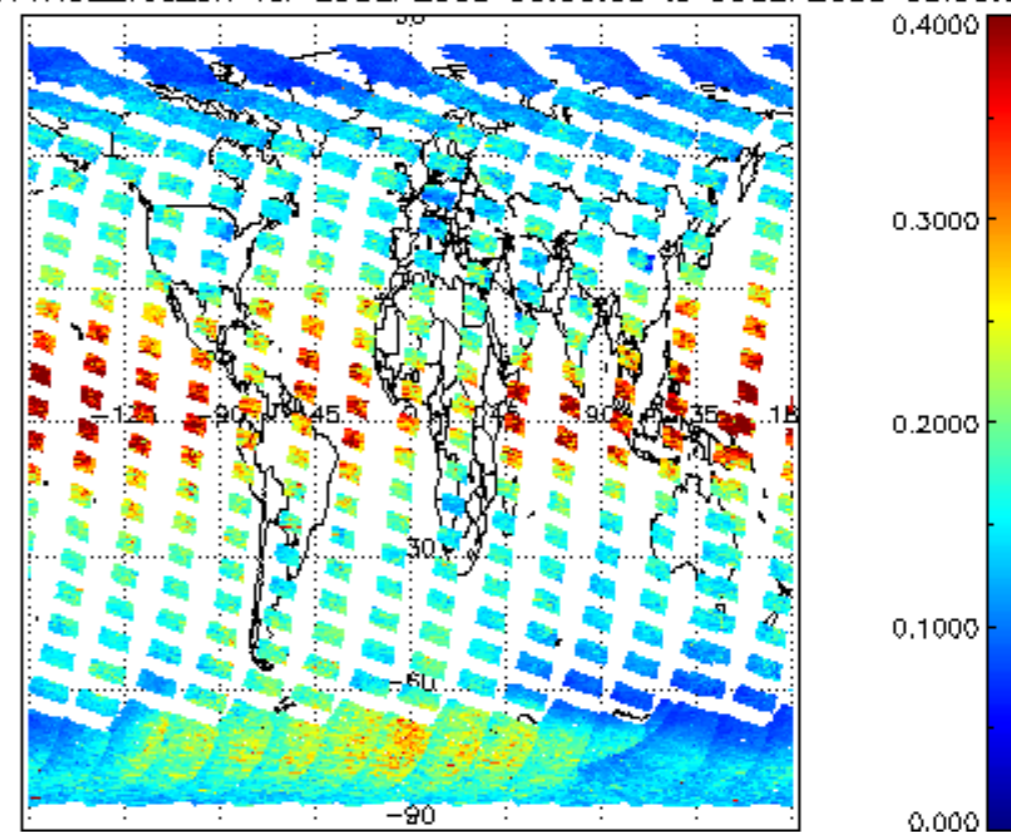
iCIOL2P_NADUV1NO2_vcd_err for 29SEP2008 00:00:00 to 30SEP2008 00:00:00
