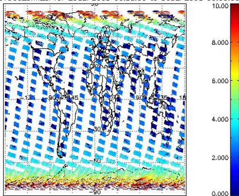
SCIOL2P_NADUV003_amf_cl for 29SEP2008 00:00:00 to 30SEP2008 00:00:00
