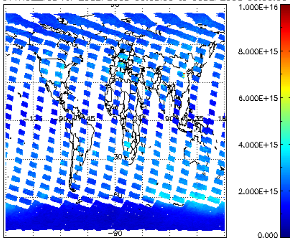
SCIOL2P_NADUV1NO2_vcd for 29SEP2008 00:00:00 to 30SEP2008 00:00:00
