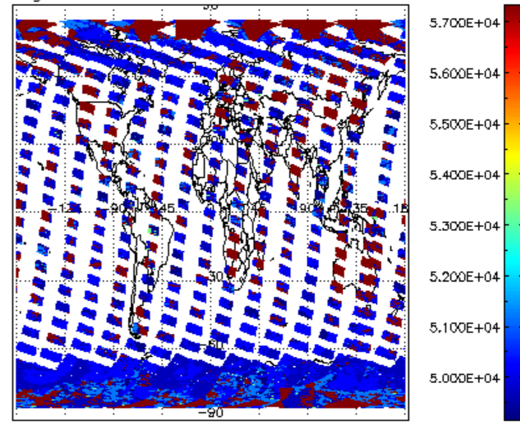
cloud_flags for 29SEP2008 00:00:00 to 30SEP2008 00:00:00
