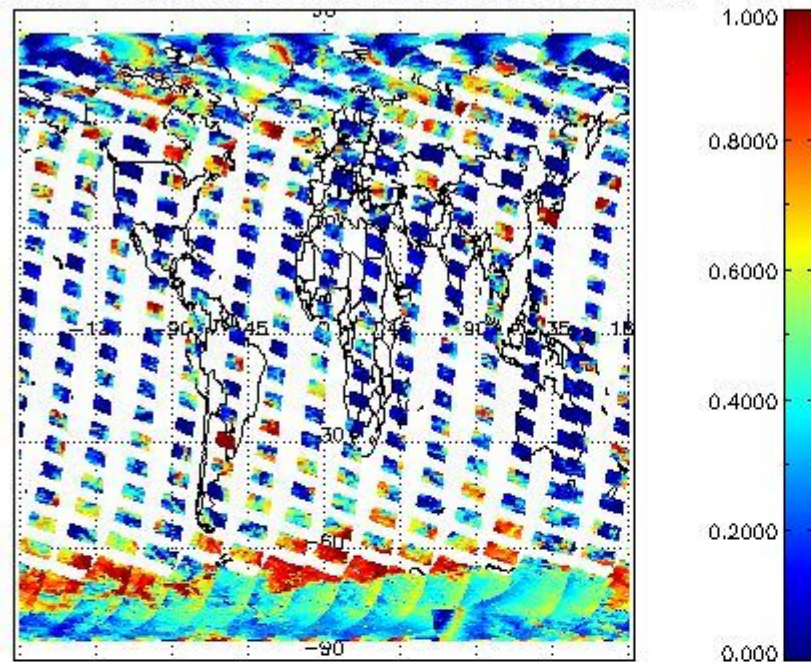
cL_frac for 29SEP2008 00:00:00 to 30SEP2008 00:00:00
