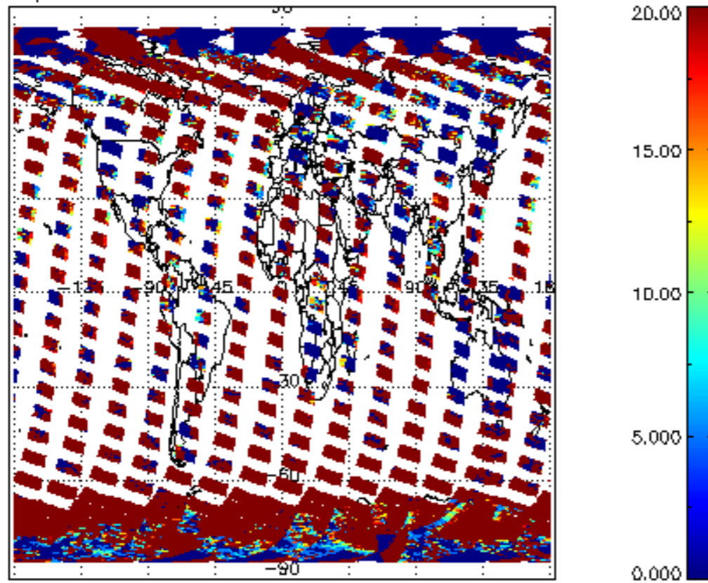
cl_opt_depth for 29SEP2008 00:00:00 to 30SEP2008 00:00:00
