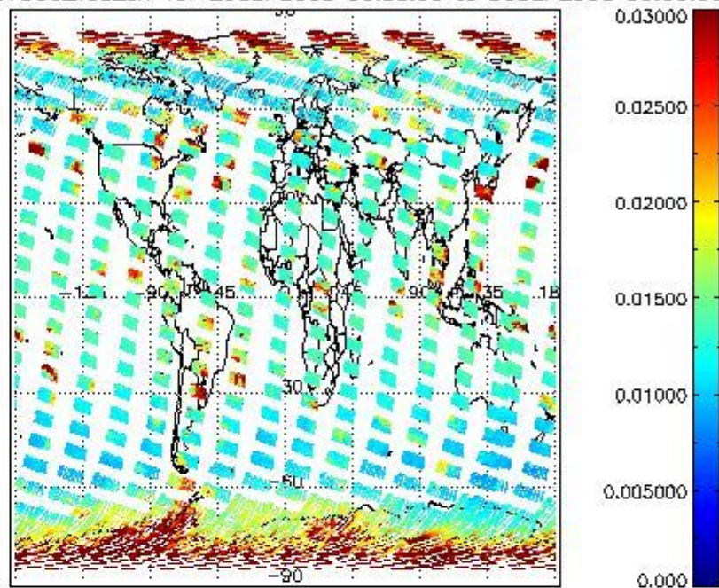
SCIOL2P_NADUV003_vcd_err for 29SEP2008 00:00:00 to 30SEP2008 00:00:00
