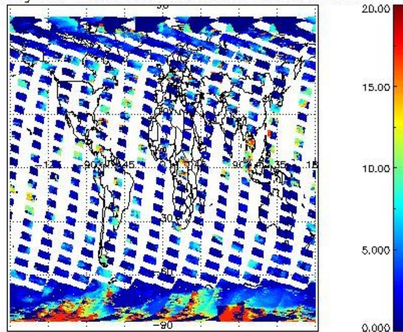
cL_top_height for 29SEP2008 00:00:00 to 30SEP2008 00:00:00
