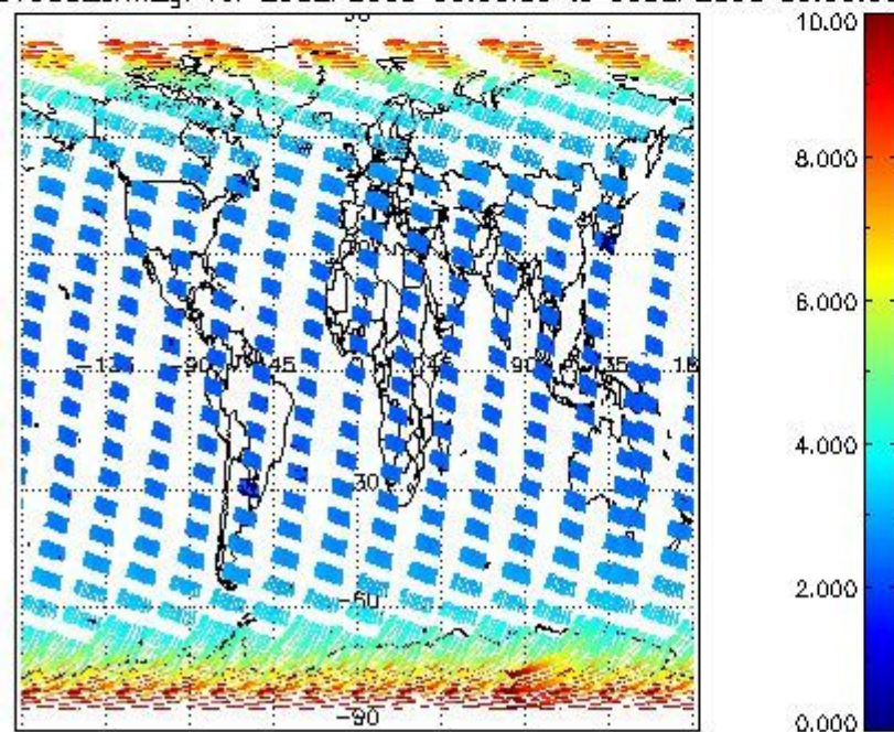
SCIOL2P_NADUV003_amf_gr for 29SEP2008 00:00:00 to 30SEP2008 00:00:00
