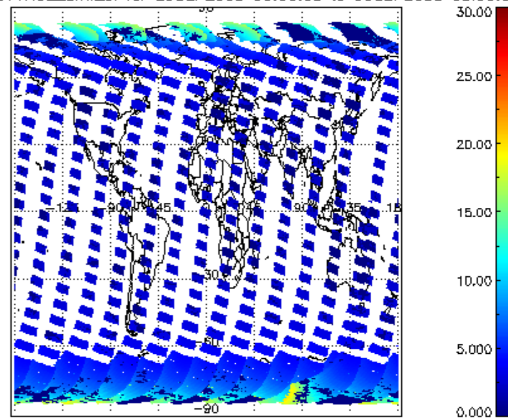
iCIOL2P_NADUV1NO2_amf_cl for 29SEP2008 00:00:00 to 30SEP2008 00:00:00
