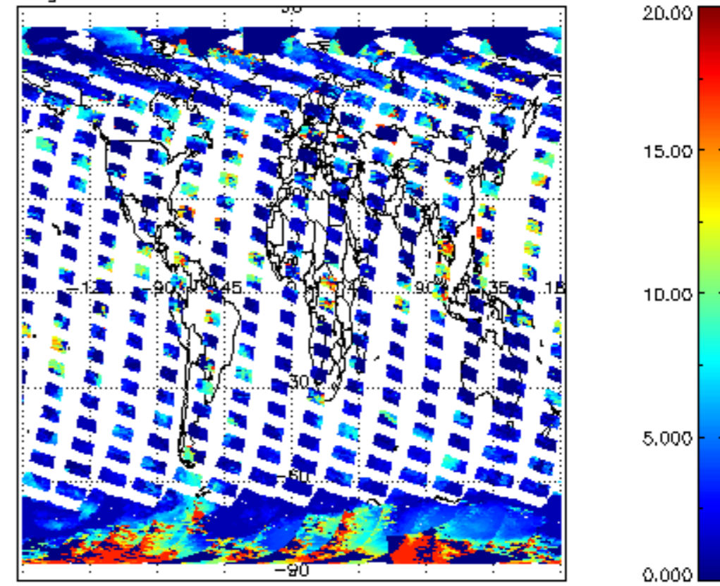
cl_top_height for 29SEP2008 00:00:00 to 30SEP2008 00:00:00
