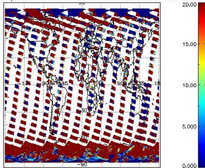
cL_opt_depth for 29SEP2008 00:00:00 to 30SEP2008 00:00:00
