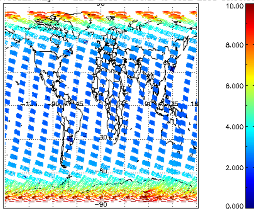
SCIOL2P_NADUV003_amf_gr for 29SEP2008 00:00:00 to 30SEP2008 00:00:00
