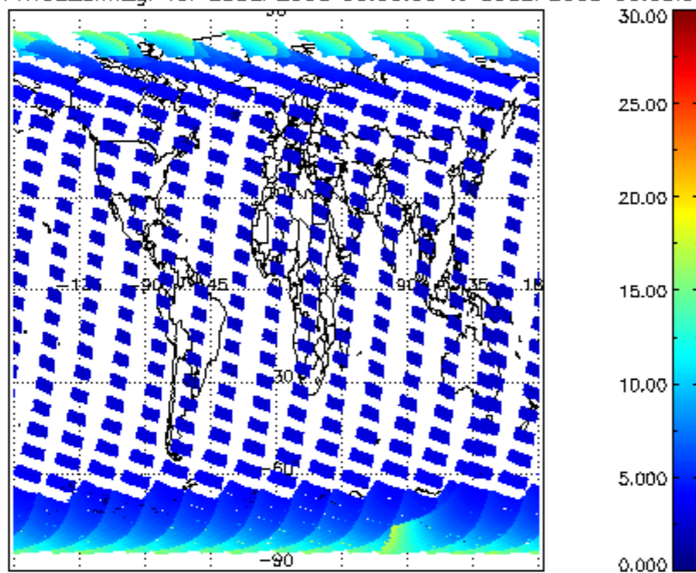
iCIOL2P_NADUV1NO2_amf_gr for 29SEP2008 00:00:00 to 30SEP2008 00:00:00
