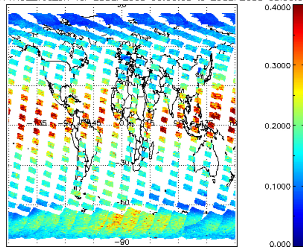
iCIOL2P_NADUV1NO2_vcd_err for 28SEP2008 00:00:00 to 29SEP2008 00:00:00
