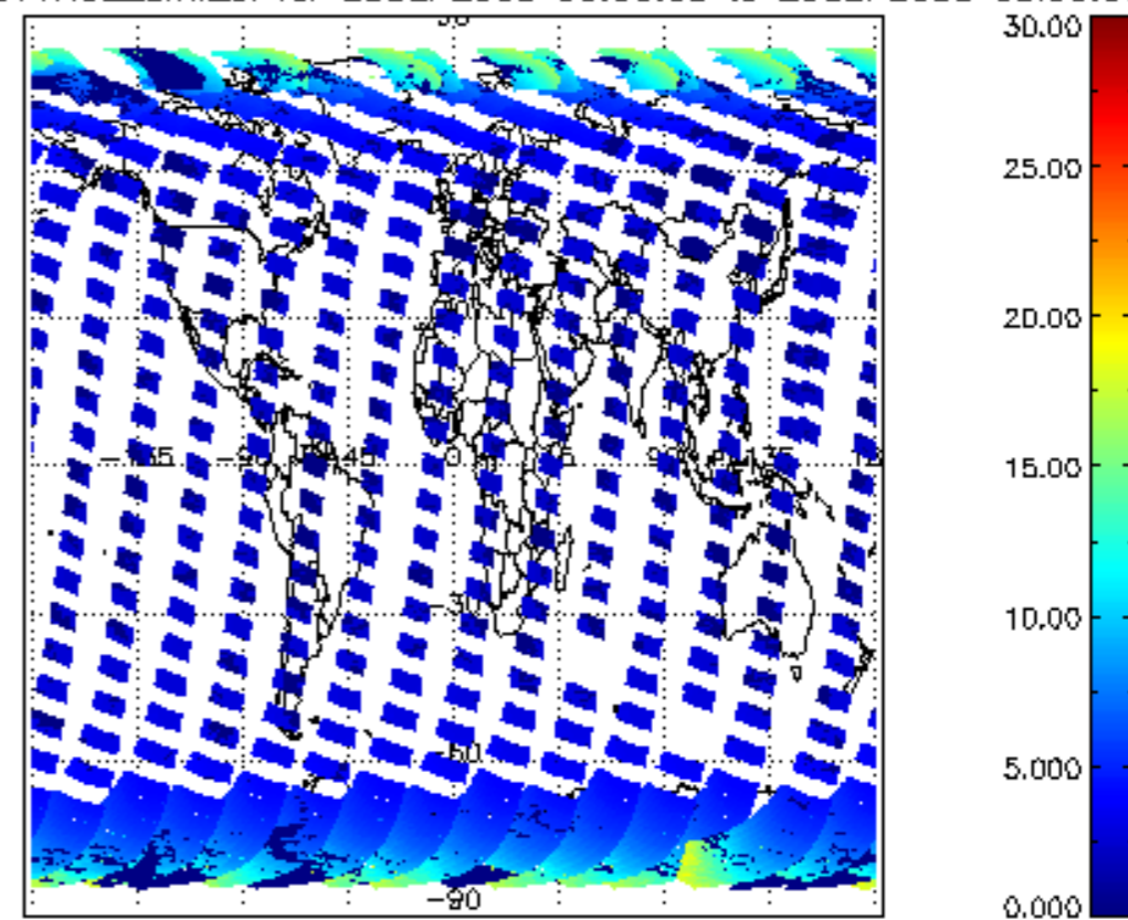
iCIOL2P_NADUV1NO2_amf_cl for 28SEP2008 00:00:00 to 29SEP2008 00:00:00
