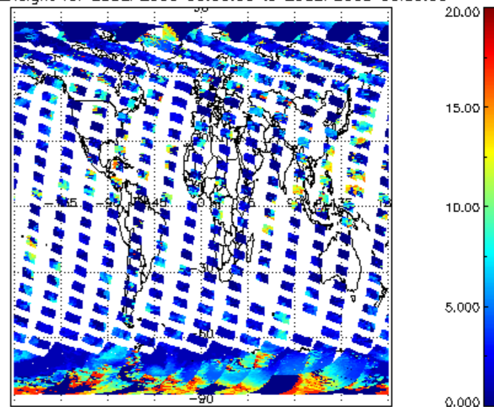
cl_top_height for 28SEP2008 00:00:00 to 29SEP2008 00:00:00
