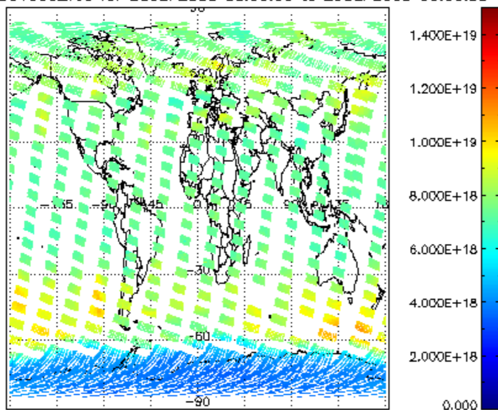
SCIOL2P_NADUV003_vcd for 28SEP2008 00:00:00 to 29SEP2008 00:00:00
