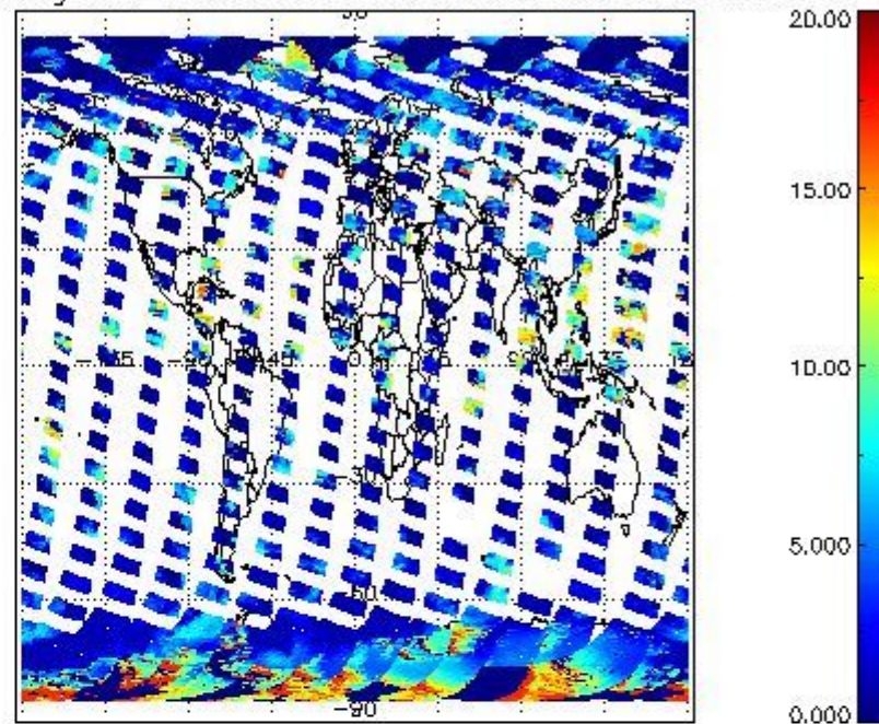
cL_top_height for 28SEP2008 00:00:00 to 29SEP2008 00:00:00
