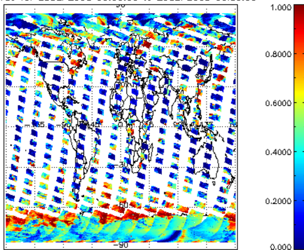
cl_frac for 28SEP2008 00:00:00 to 29SEP2008 00:00:00
