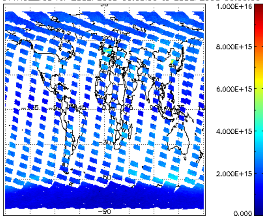
SCIOL2P_NADUV1NO2_vcd for 28SEP2008 00:00:00 to 29SEP2008 00:00:00
