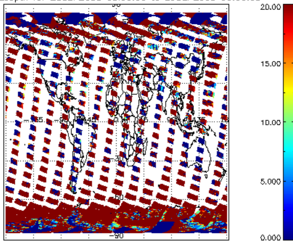
cl_opt_depth for 28SEP2008 00:00:00 to 29SEP2008 00:00:00
