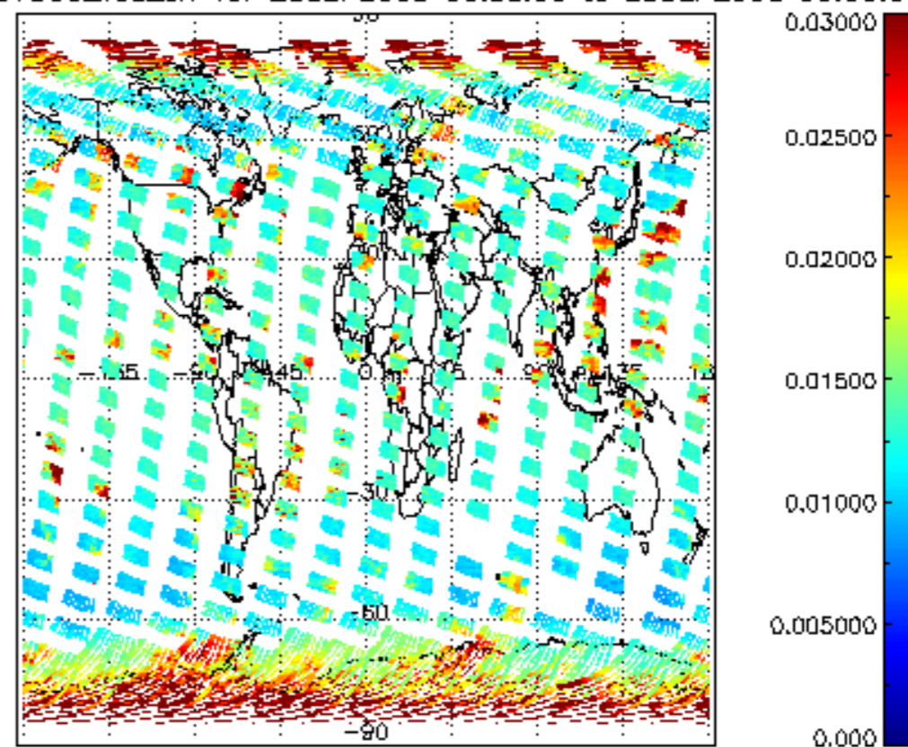
SCIOL2P_NADUV003_vcd_err for 28SEP2008 00:00:00 to 29SEP2008 00:00:00
