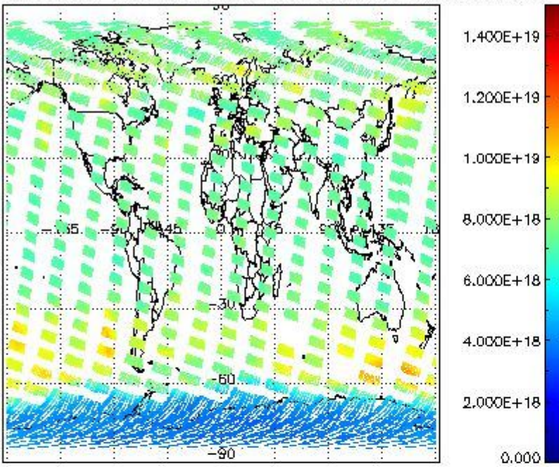
SCIOL2P_NADUV003_vcd for 28SEP2008 00:00:00 to 29SEP2008 00:00:00
