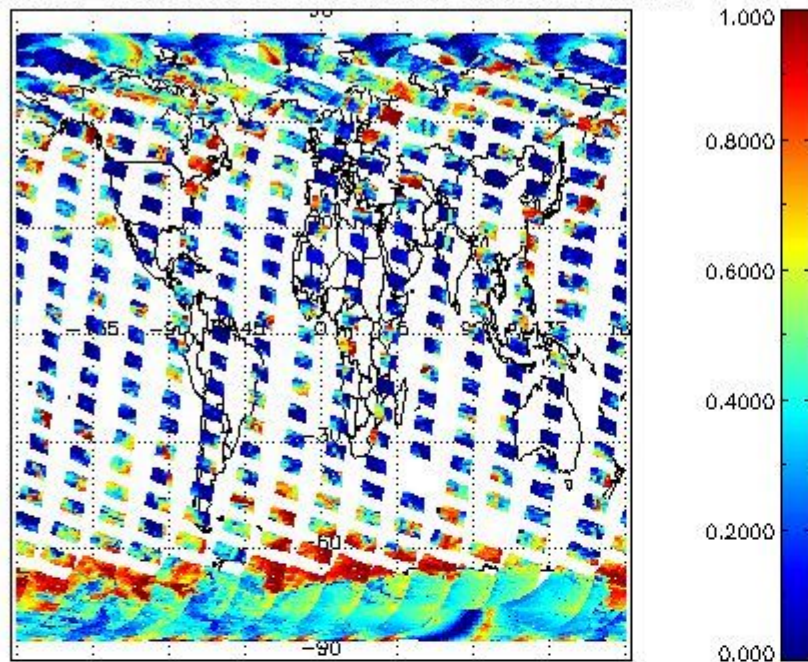
cL_frac for 28SEP2008 00:00:00 to 29SEP2008 00:00:00
