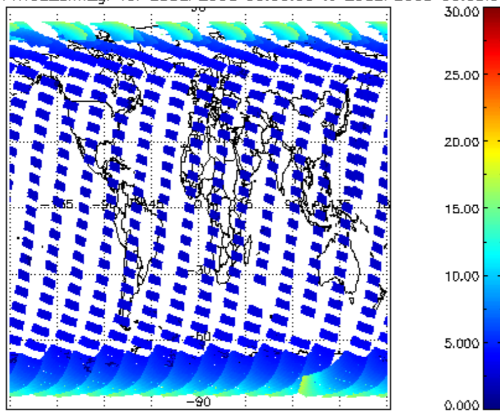
iCIOL2P_NADUV1NO2_amf_gr for 28SEP2008 00:00:00 to 29SEP2008 00:00:00
