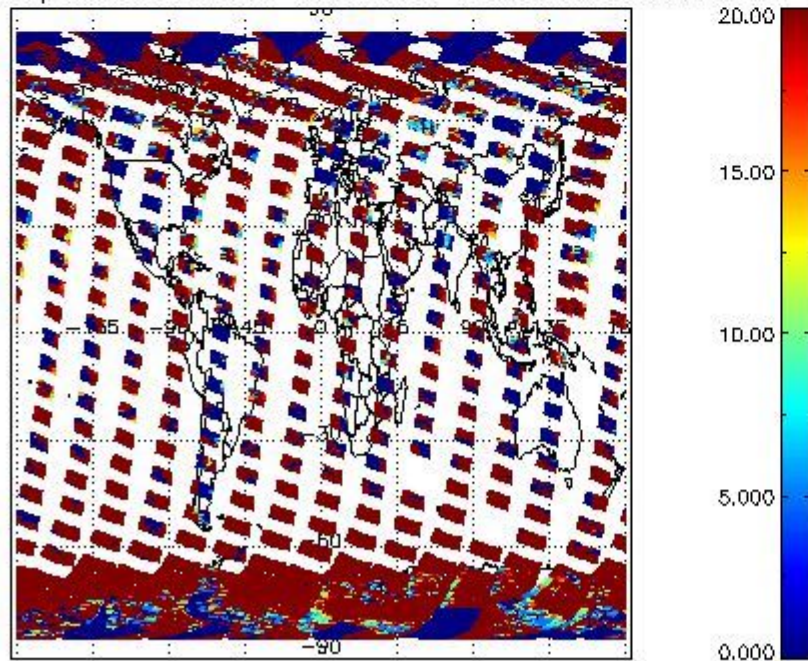
cL_opt_depth for 28SEP2008 00:00:00 to 29SEP2008 00:00:00
