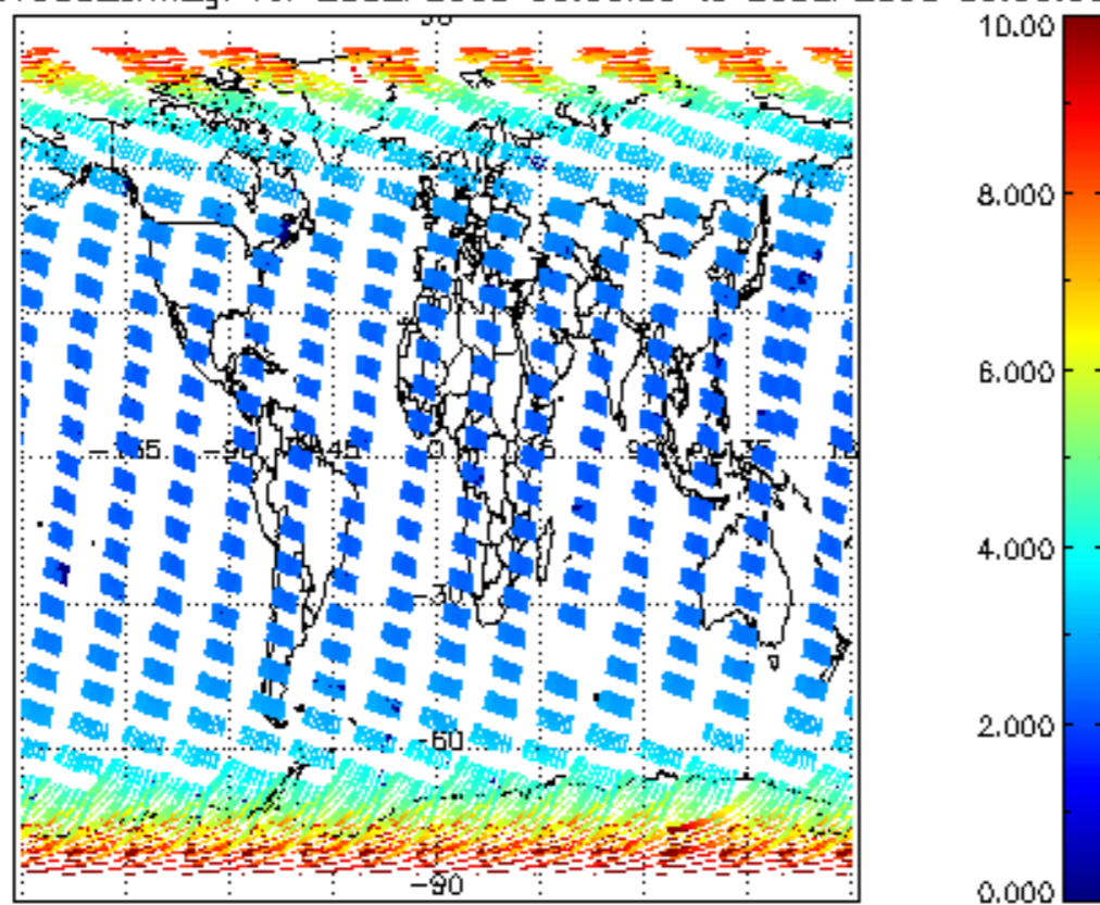
SCIOL2P_NADUV003_amf_gr for 28SEP2008 00:00:00 to 29SEP2008 00:00:00
