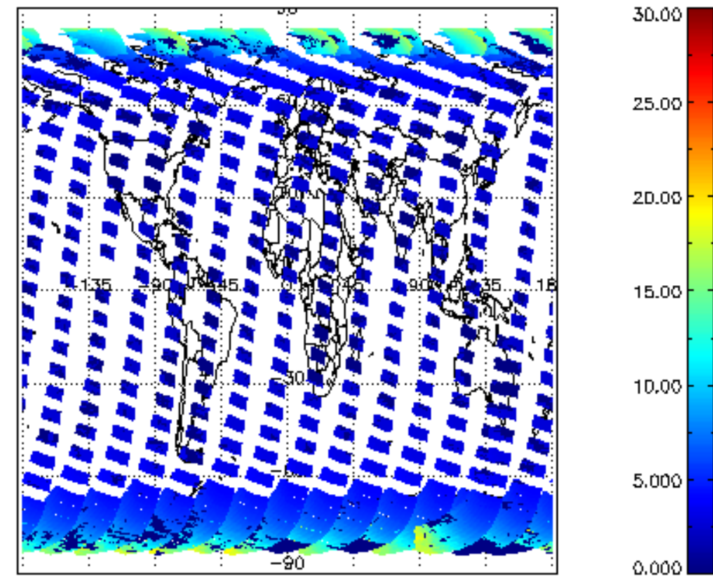
iCIOL2P_NADUV1NO2_amf_cl for 26SEP2008 00:00:00 to 27SEP2008 00:00:00
