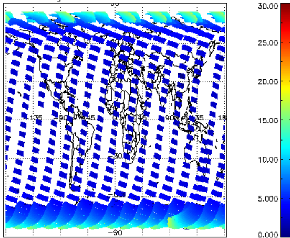
iCIOL2P_NADUV1NO2_amf_gr for 26SEP2008 00:00:00 to 27SEP2008 00:00:00
