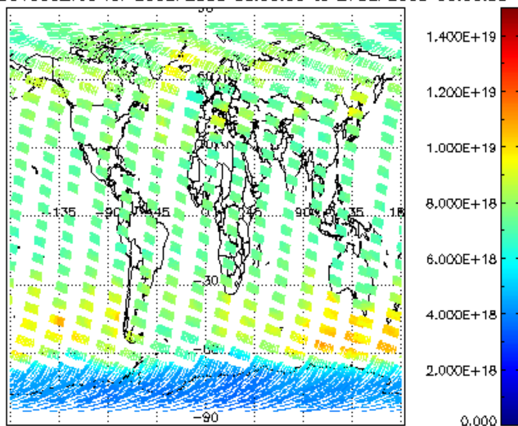
SCIOL2P_NADUV003_vcd for 26SEP2008 00:00:00 to 27SEP2008 00:00:00
