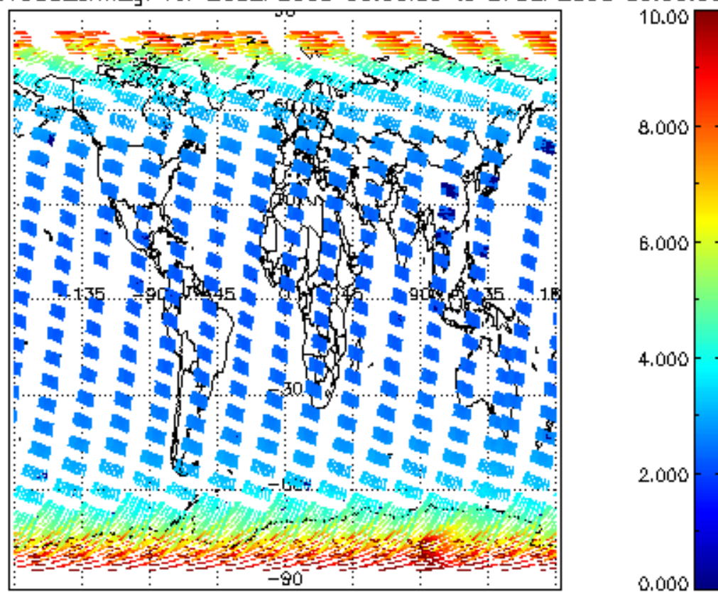
SCIOL2P_NADUV003_amf_gr for 26SEP2008 00:00:00 to 27SEP2008 00:00:00
