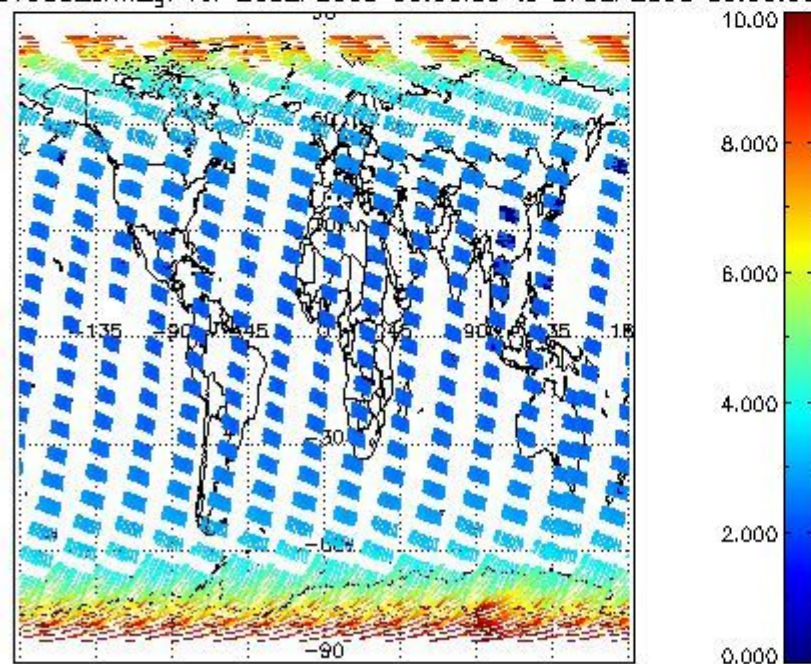
SCIOL2P_NADUV003_amf_gr for 26SEP2008 00:00:00 to 27SEP2008 00:00:00
