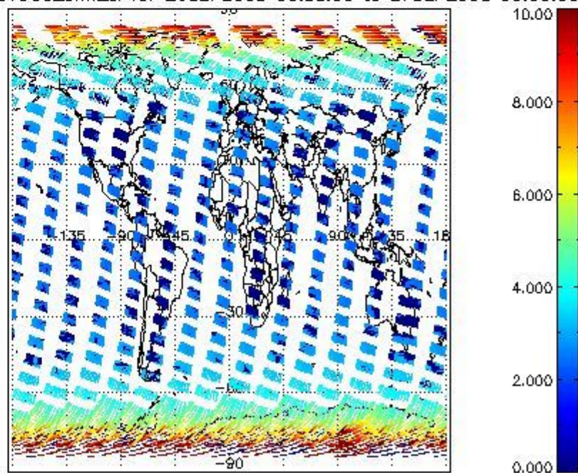
SCIOL2P_NADUV003_amf_cl for 26SEP2008 00:00:00 to 27SEP2008 00:00:00
