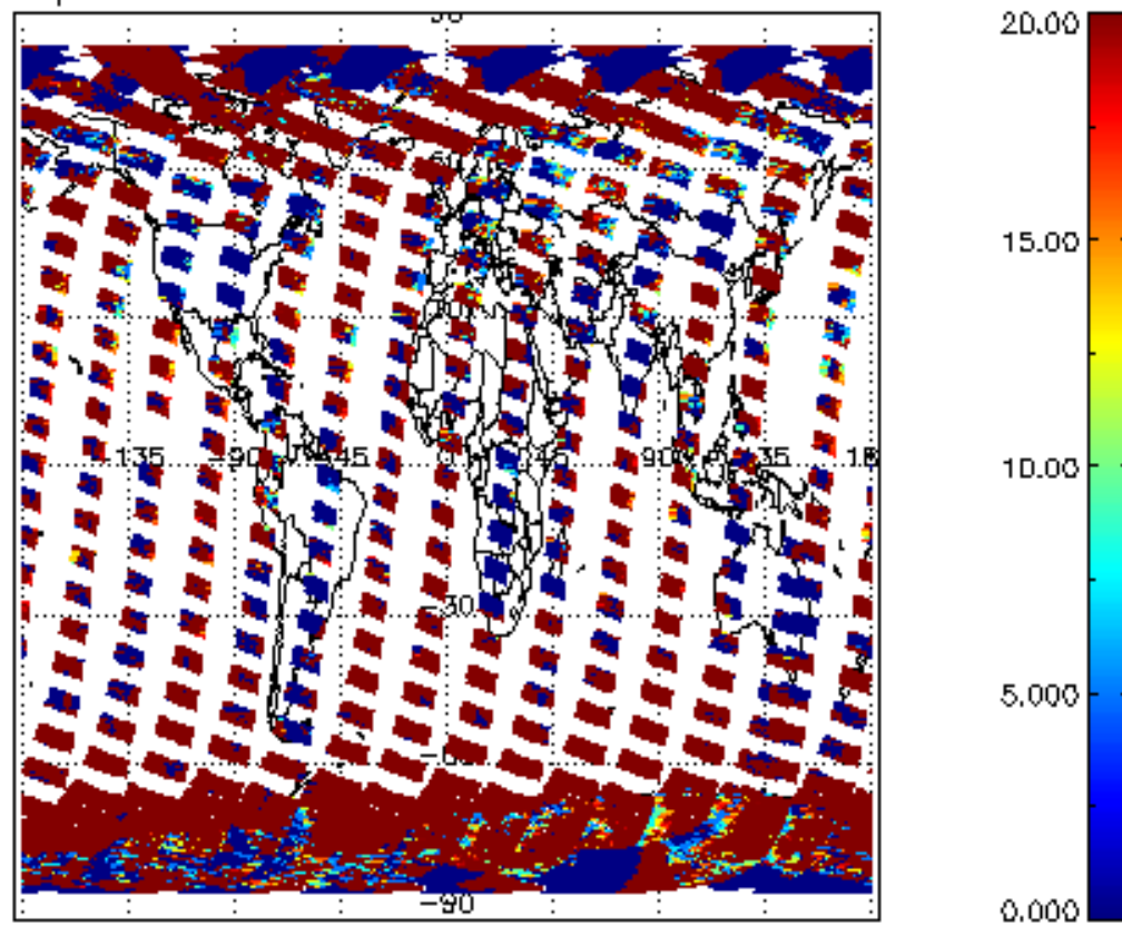
cl_opt_depth for 26SEP2008 00:00:00 to 27SEP2008 00:00:00
