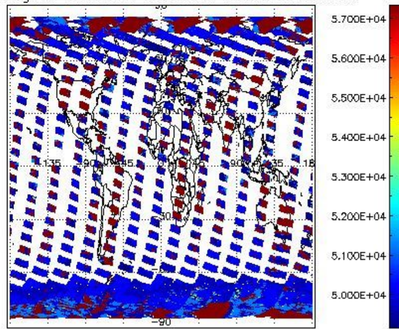
cloud_flags for 26SEP2008 00:00:00 to 27SEP2008 00:00:00
