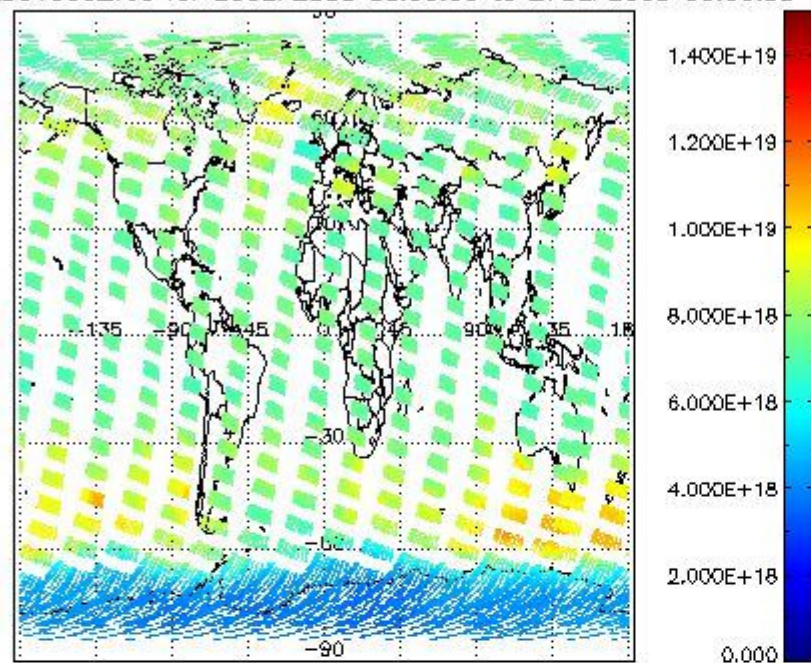
SCIOL2P_NADUV003_vcd for 26SEP2008 00:00:00 to 27SEP2008 00:00:00
