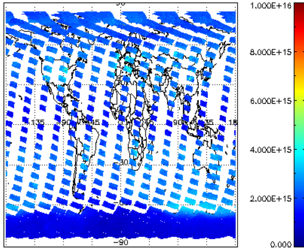
SCIOL2P_NADUV1NO2_vcd for 26SEP2008 00:00:00 to 27SEP2008 00:00:00
