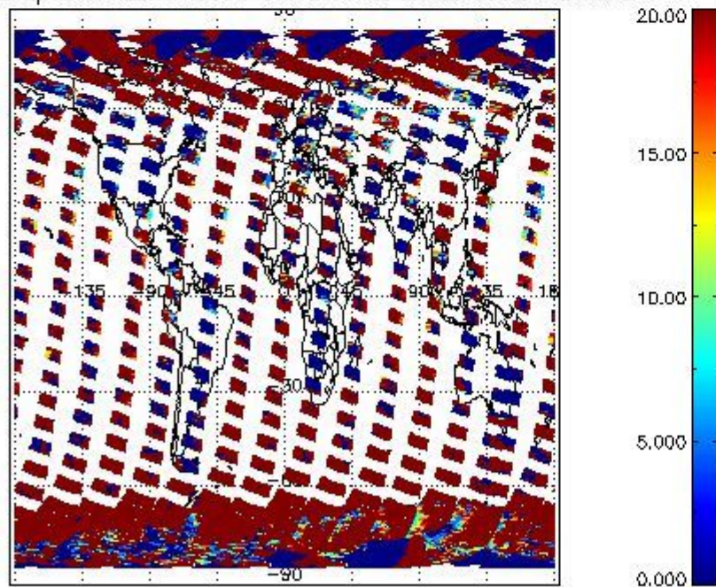
cL_opt_depth for 26SEP2008 00:00:00 to 27SEP2008 00:00:00
