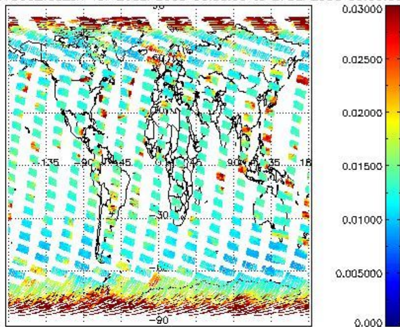
SCIOL2P_NADUV003_vcd_err for 26SEP2008 00:00:00 to 27SEP2008 00:00:00
