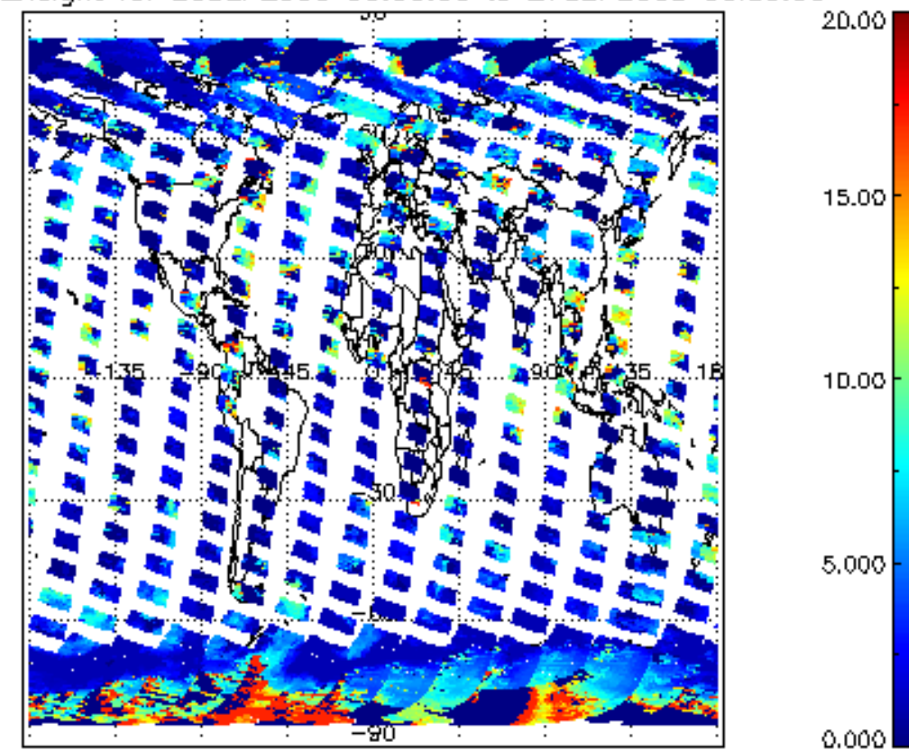
cl_top_height for 26SEP2008 00:00:00 to 27SEP2008 00:00:00
