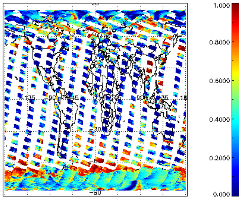
cl_frac for 26SEP2008 00:00:00 to 27SEP2008 00:00:00
