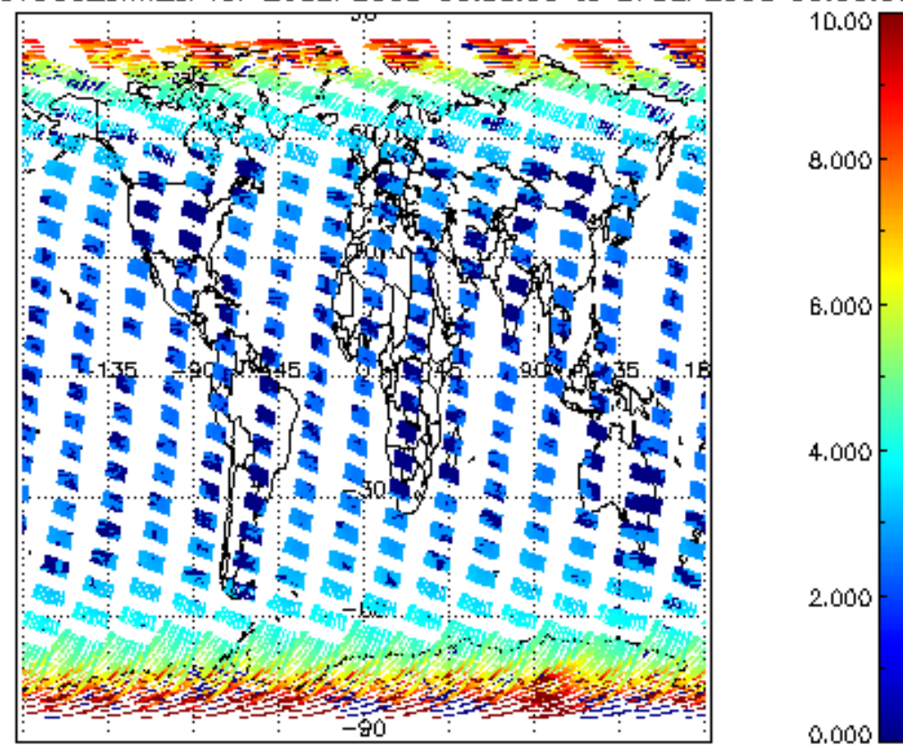
SCIOL2P_NADUV003_amf_cl for 26SEP2008 00:00:00 to 27SEP2008 00:00:00
