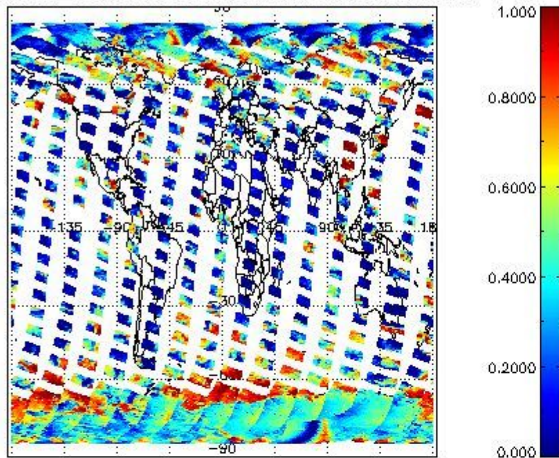
cL_frac for 26SEP2008 00:00:00 to 27SEP2008 00:00:00
