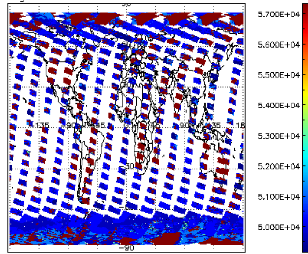
cloud_flags for 26SEP2008 00:00:00 to 27SEP2008 00:00:00
