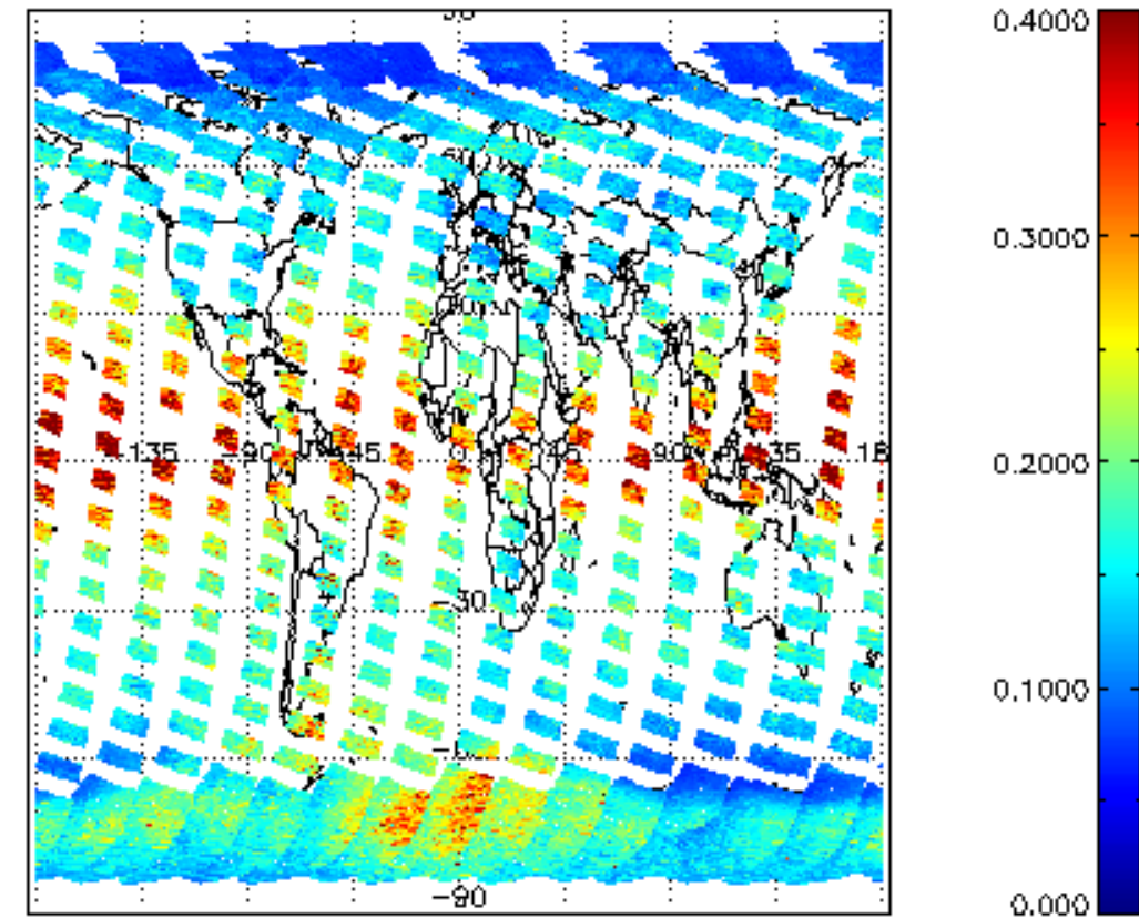
iCIOL2P_NADUV1NO2_vcd_err for 26SEP2008 00:00:00 to 27SEP2008 00:00:00
