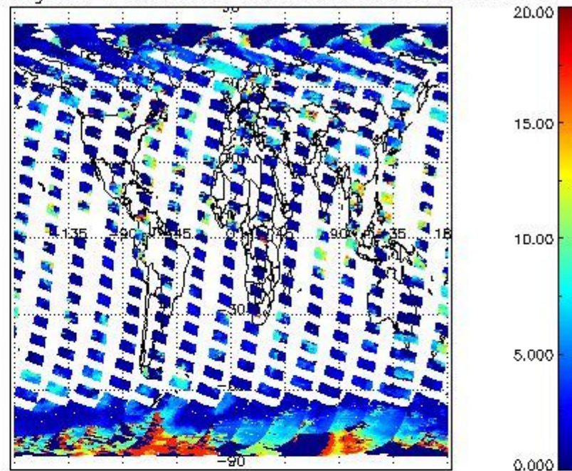
cL_top_height for 26SEP2008 00:00:00 to 27SEP2008 00:00:00
