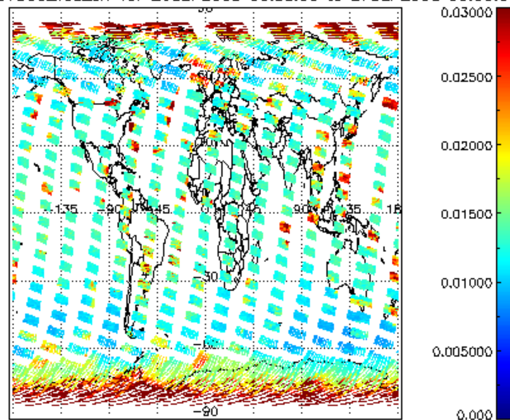
SCIOL2P_NADUV003_vcd_err for 26SEP2008 00:00:00 to 27SEP2008 00:00:00
