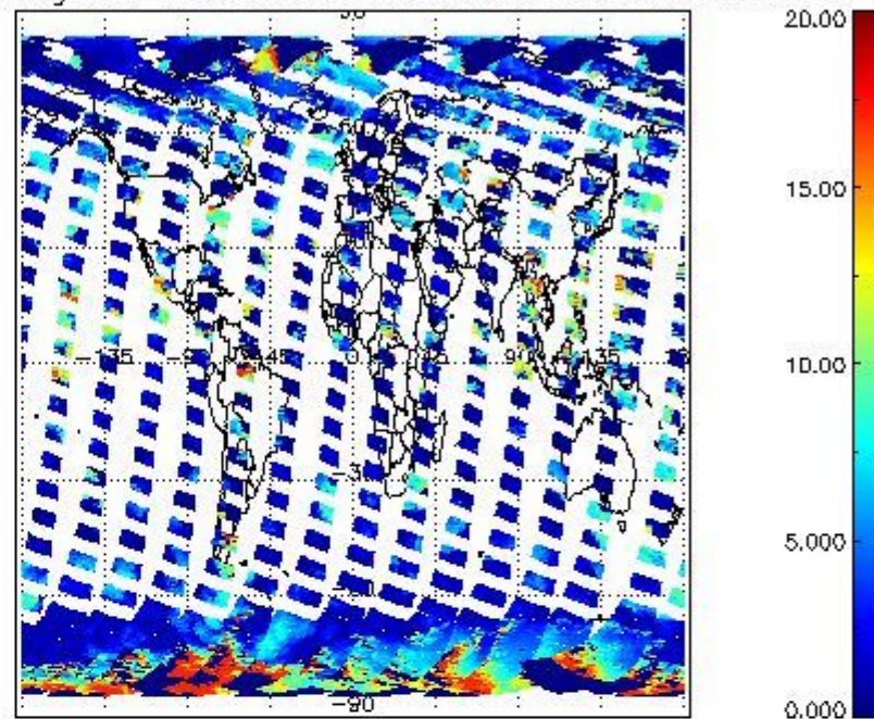
cL_top_height for 25SEP2008 00:00:00 to 26SEP2008 00:00:00
