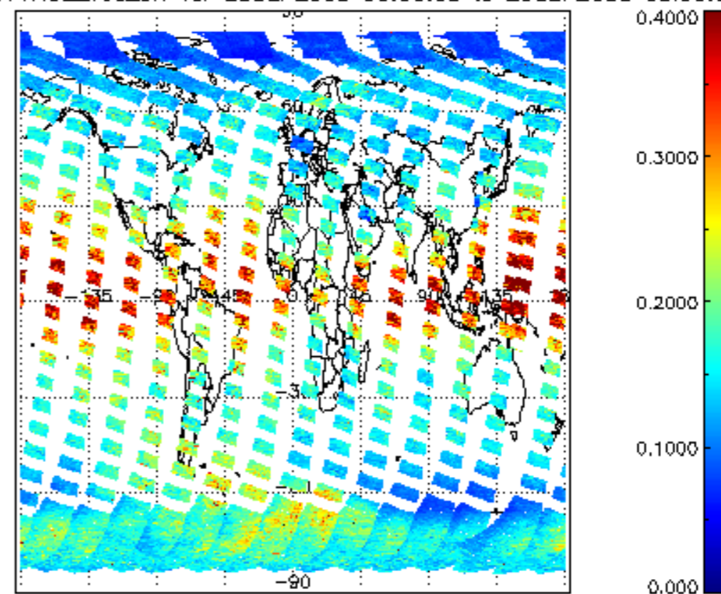
iCIOL2P_NADUV1NO2_vcd_err for 25SEP2008 00:00:00 to 26SEP2008 00:00:00
