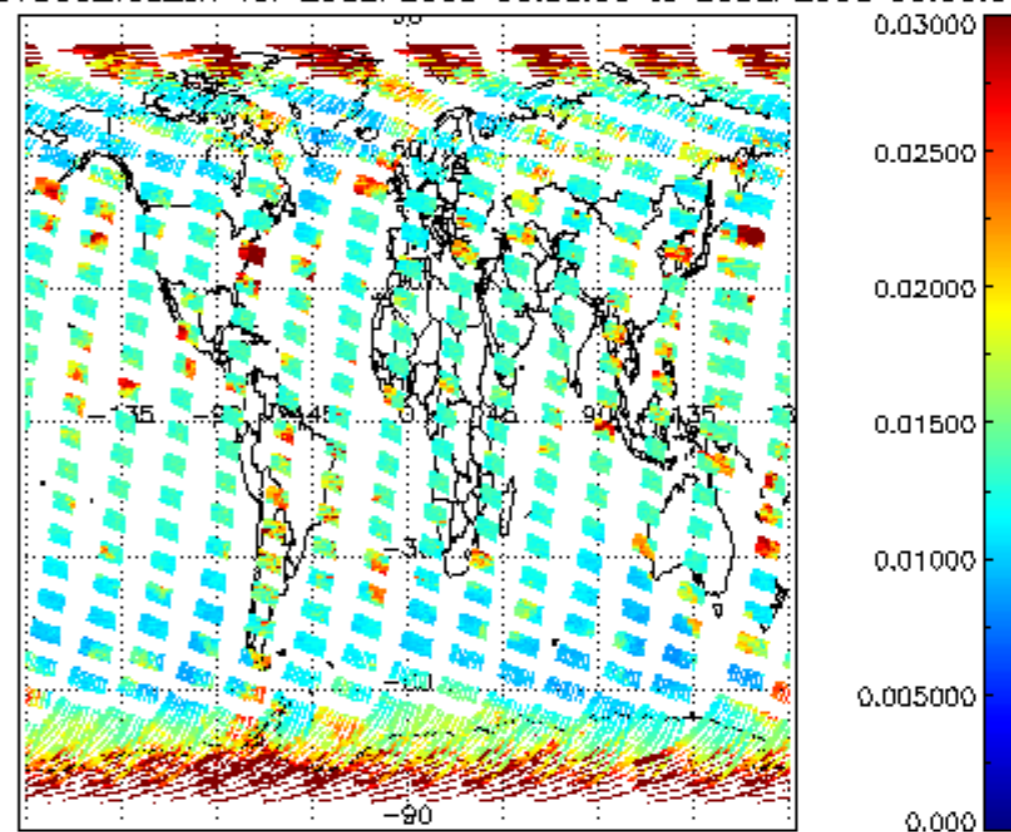
SCIOL2P_NADUV003_vcd_err for 25SEP2008 00:00:00 to 26SEP2008 00:00:00
