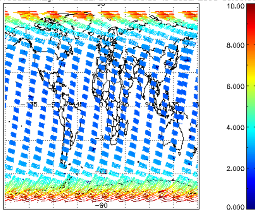
SCIOL2P_NADUV003_amf_gr for 25SEP2008 00:00:00 to 26SEP2008 00:00:00
