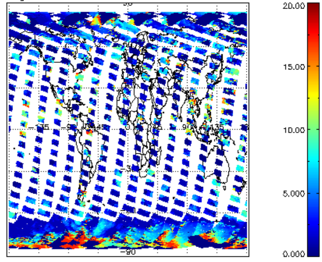
cl_top_height for 25SEP2008 00:00:00 to 26SEP2008 00:00:00
