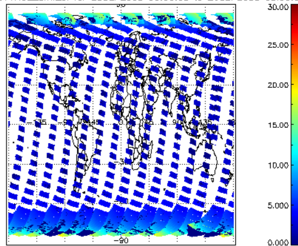
iCIOL2P_NADUV1NO2_amf_cl for 25SEP2008 00:00:00 to 26SEP2008 00:00:00
