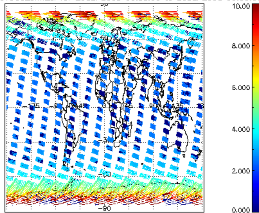
SCIOL2P_NADUV003_amf_cl for 25SEP2008 00:00:00 to 26SEP2008 00:00:00
