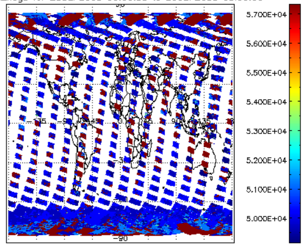
cloud_flags for 25SEP2008 00:00:00 to 26SEP2008 00:00:00
