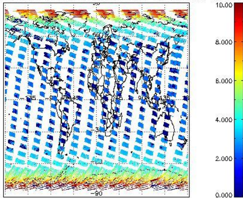
SCIOL2P_NADUV003_amf_cl for 25SEP2008 00:00:00 to 26SEP2008 00:00:00
