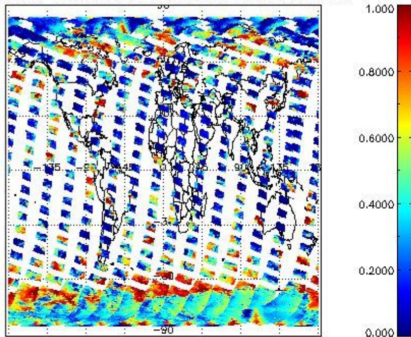
cL_frac for 25SEP2008 00:00:00 to 26SEP2008 00:00:00
