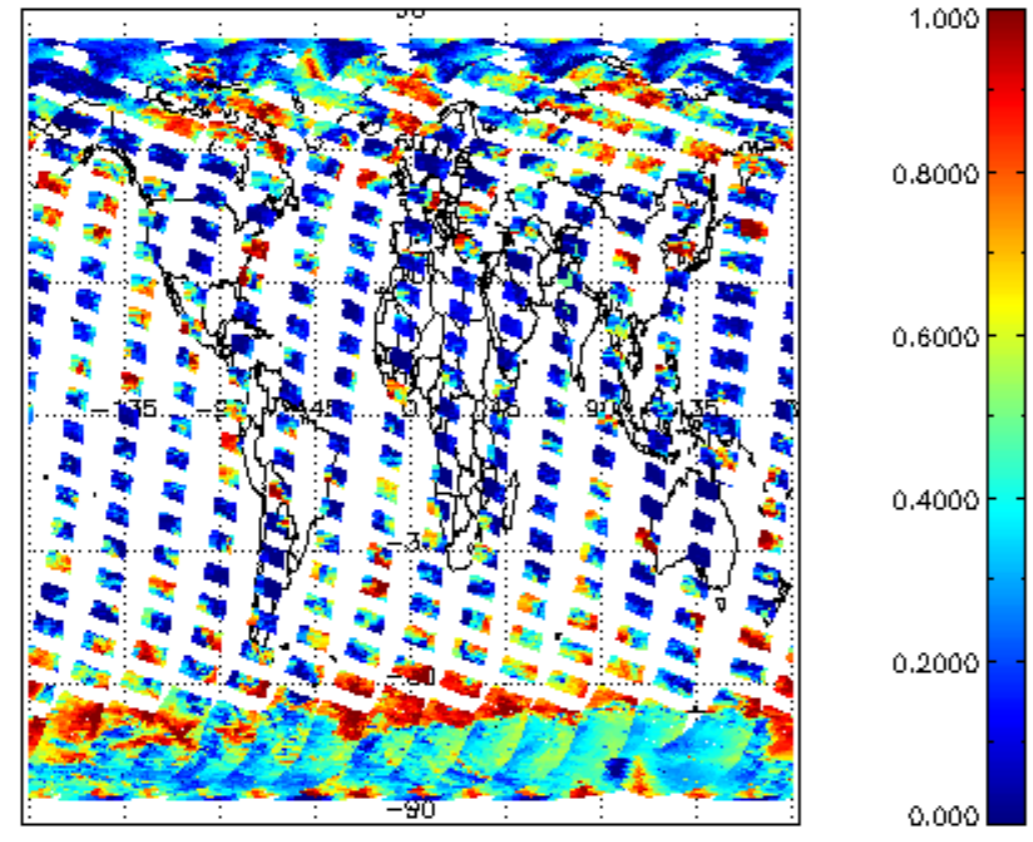
cl_frac for 25SEP2008 00:00:00 to 26SEP2008 00:00:00
