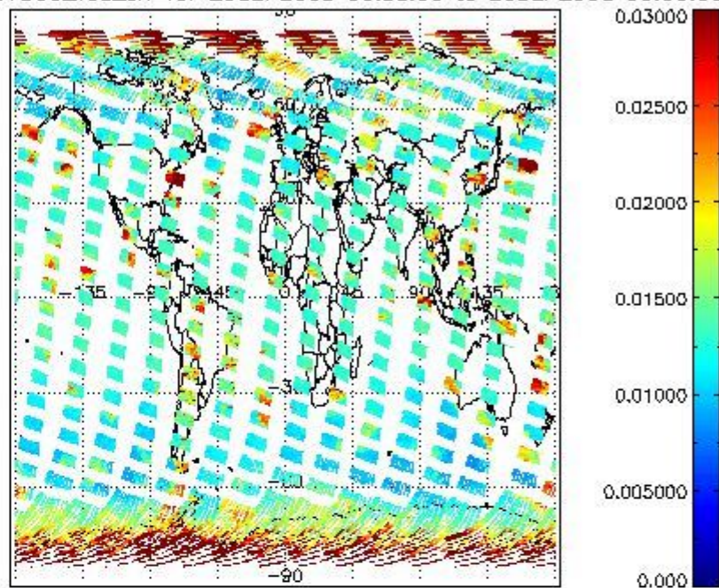
SCIOL2P_NADUV003_vcd_err for 25SEP2008 00:00:00 to 26SEP2008 00:00:00
