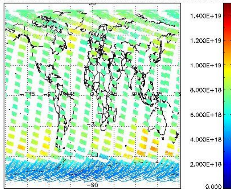
SCIOL2P_NADUV003_vcd for 25SEP2008 00:00:00 to 26SEP2008 00:00:00
