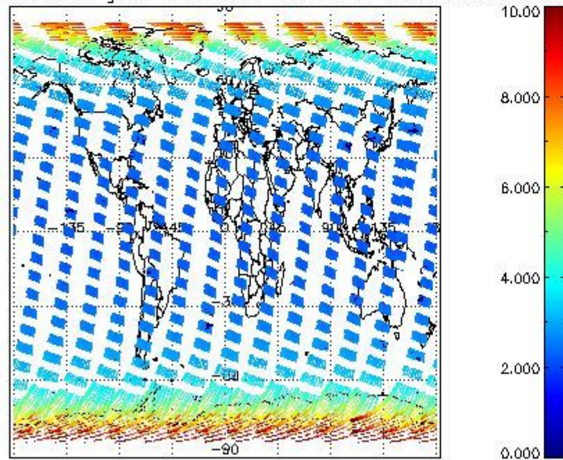
SCIOL2P_NADUV003_amf_gr for 25SEP2008 00:00:00 to 26SEP2008 00:00:00
