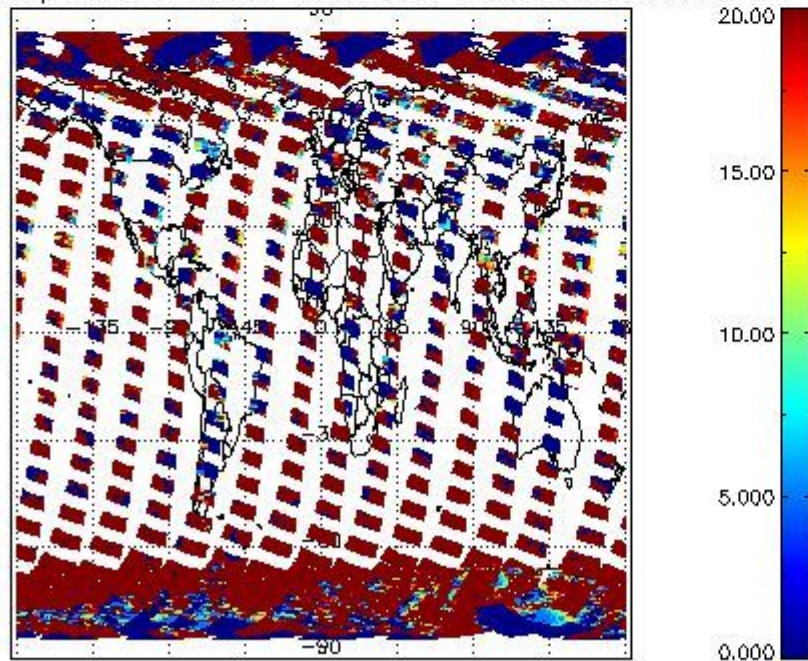
cL_opt_depth for 25SEP2008 00:00:00 to 26SEP2008 00:00:00
