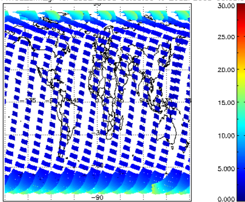
iCIOL2P_NADUV1NO2_amf_gr for 25SEP2008 00:00:00 to 26SEP2008 00:00:00
