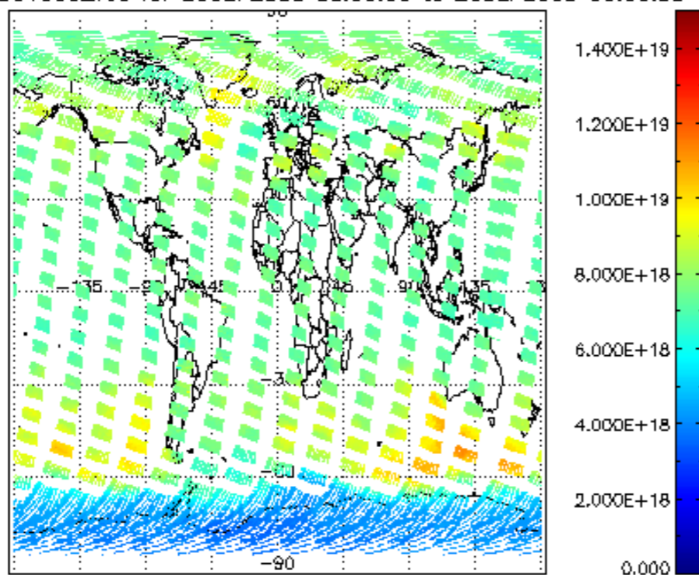
SCIOL2P_NADUV003_vcd for 25SEP2008 00:00:00 to 26SEP2008 00:00:00
