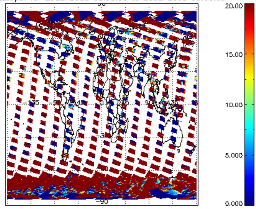
cl_opt_depth for 25SEP2008 00:00:00 to 26SEP2008 00:00:00
