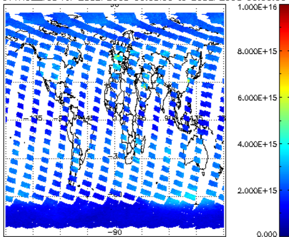
SCIOL2P_NADUV1NO2_vcd for 25SEP2008 00:00:00 to 26SEP2008 00:00:00
