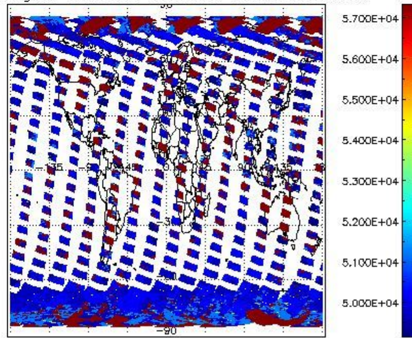
cloud_flags for 25SEP2008 00:00:00 to 26SEP2008 00:00:00
