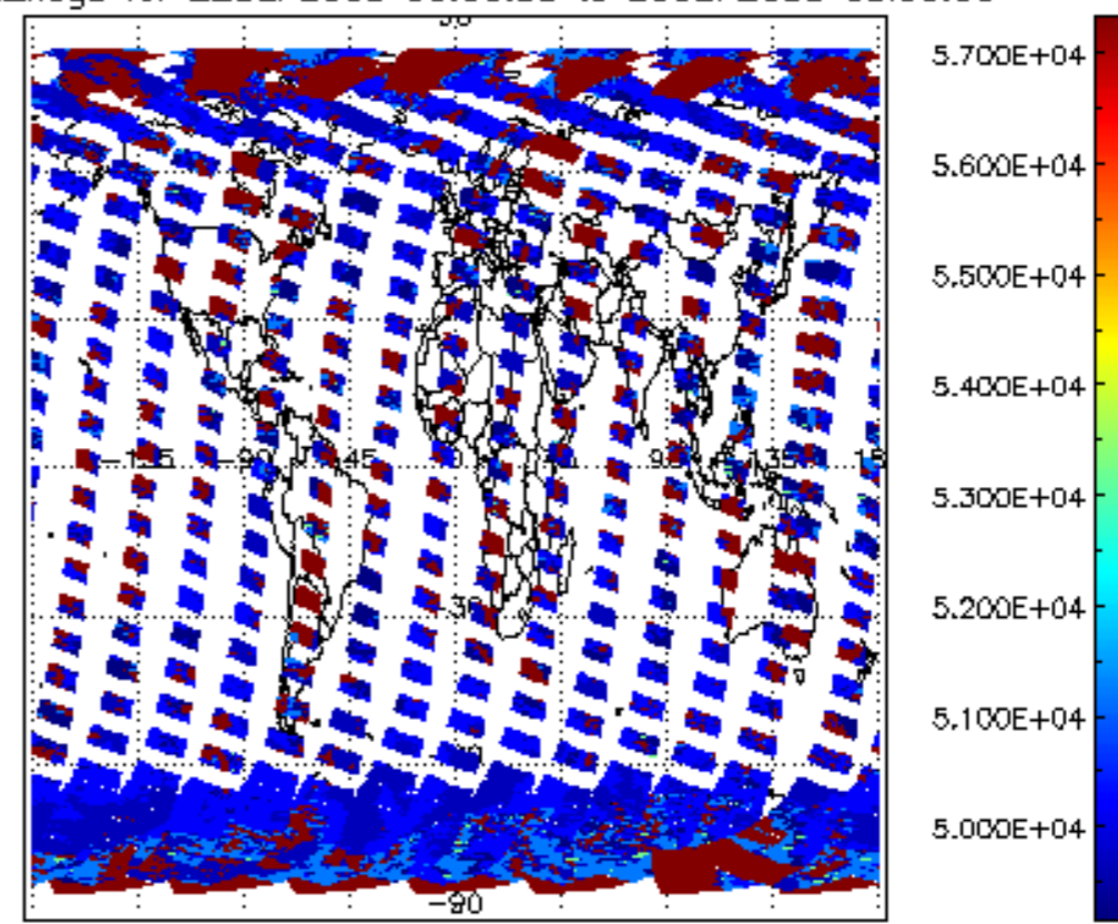
cloud_flags for 22SEP2008 00:00:00 to 23SEP2008 00:00:00
