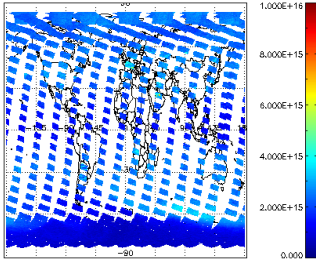
SCIOL2P_NADUV1NO2_vcd for 22SEP2008 00:00:00 to 23SEP2008 00:00:00
