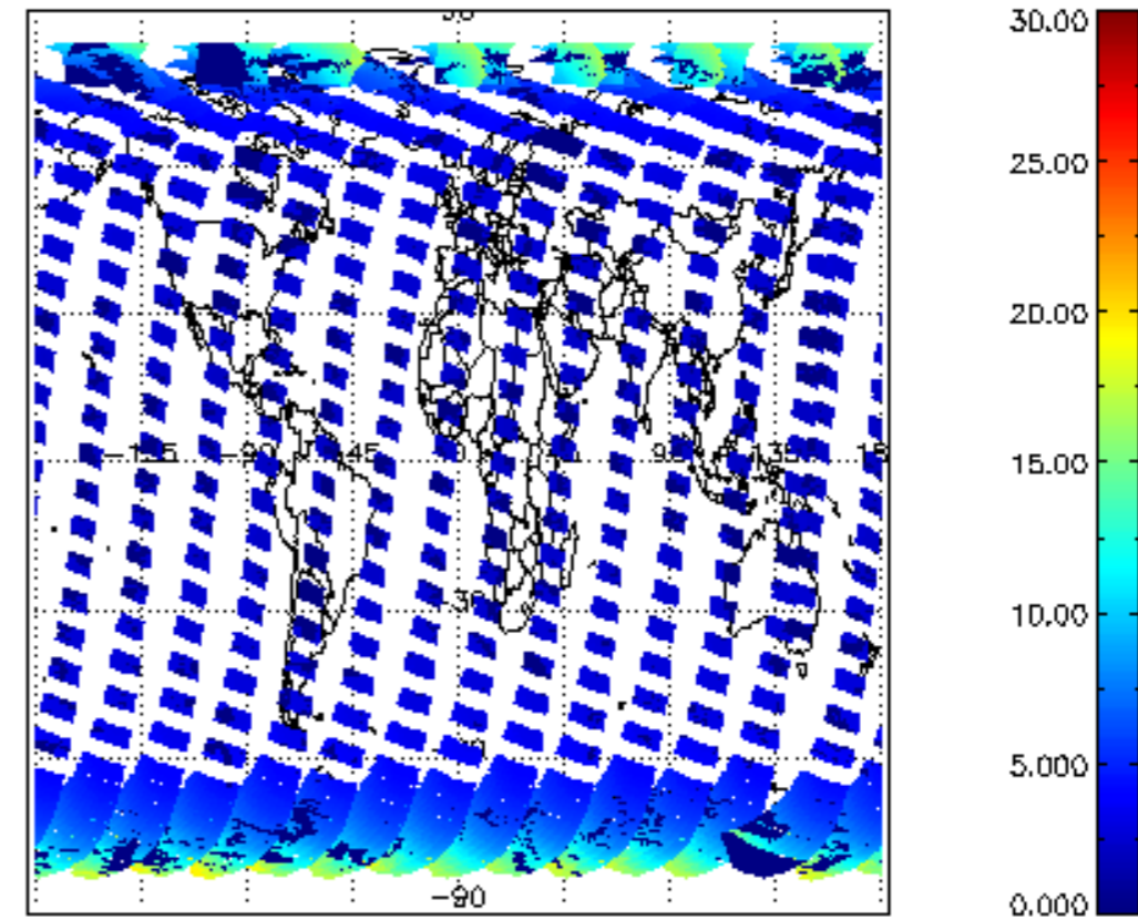
iCIOL2P_NADUV1NO2_amf_cl for 22SEP2008 00:00:00 to 23SEP2008 00:00:00
