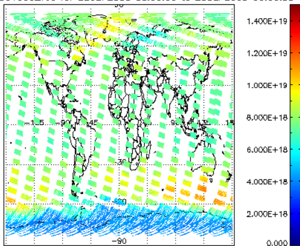
SCIOL2P_NADUV003_vcd for 22SEP2008 00:00:00 to 23SEP2008 00:00:00
