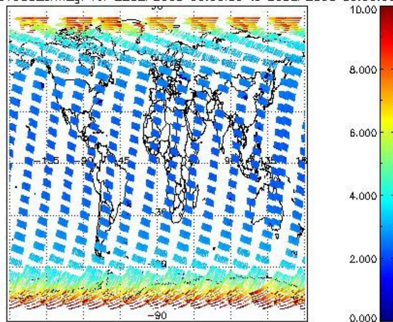
SCIOL2P_NADUV003_amf_gr for 22SEP2008 00:00:00 to 23SEP2008 00:00:00
