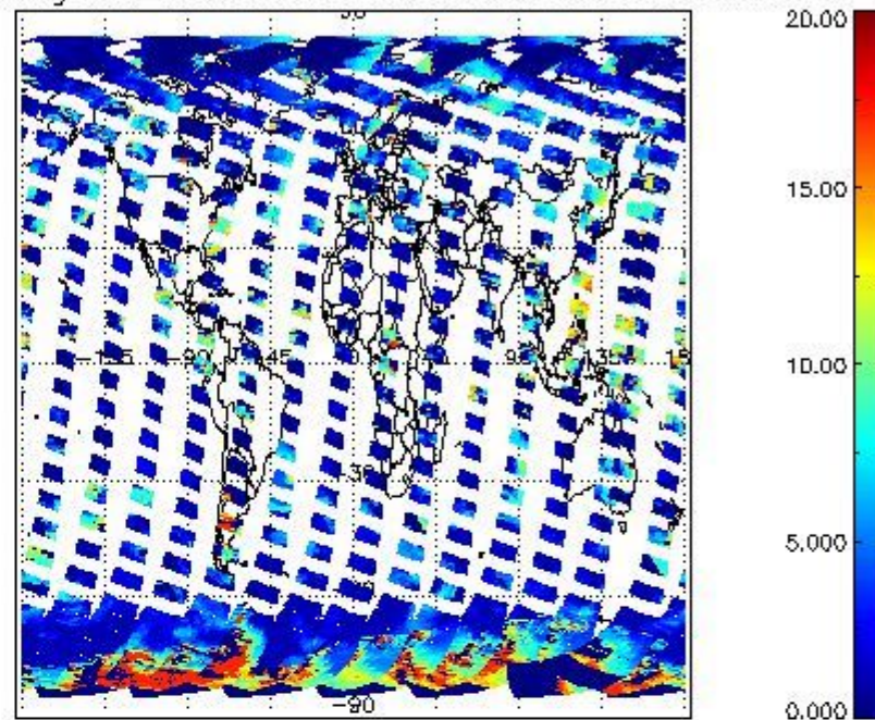
cL_top_height for 22SEP2008 00:00:00 to 23SEP2008 00:00:00
