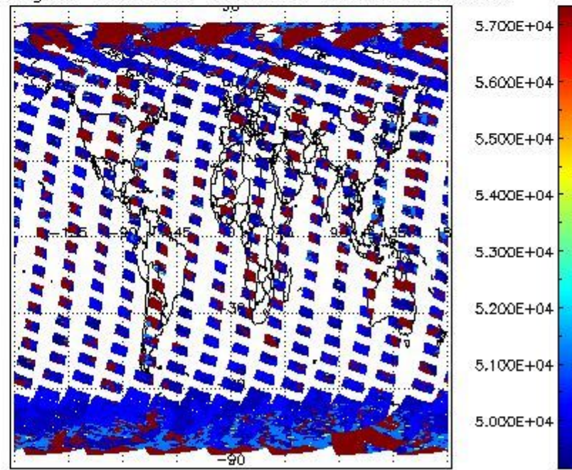
cloud_flags for 22SEP2008 00:00:00 to 23SEP2008 00:00:00
