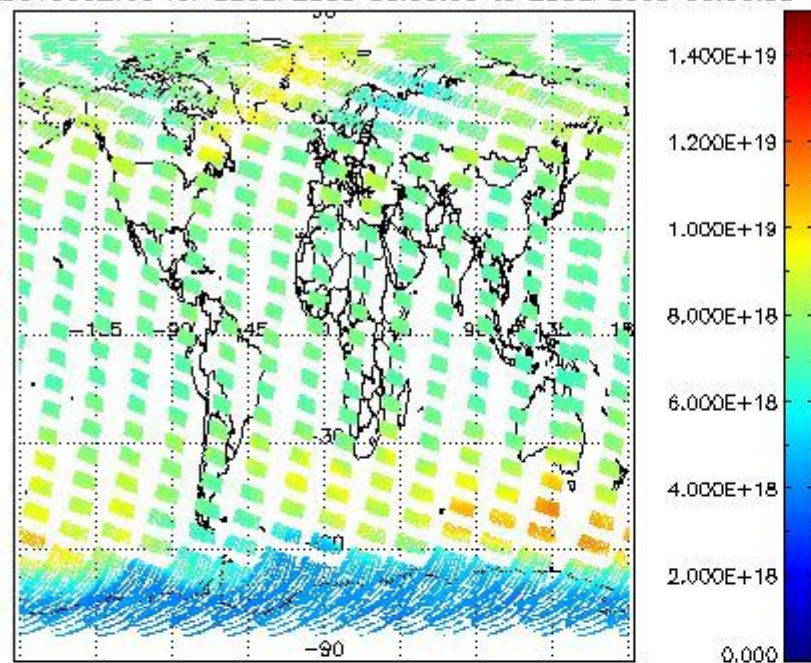
SCIOL2P_NADUV003_vcd for 22SEP2008 00:00:00 to 23SEP2008 00:00:00
