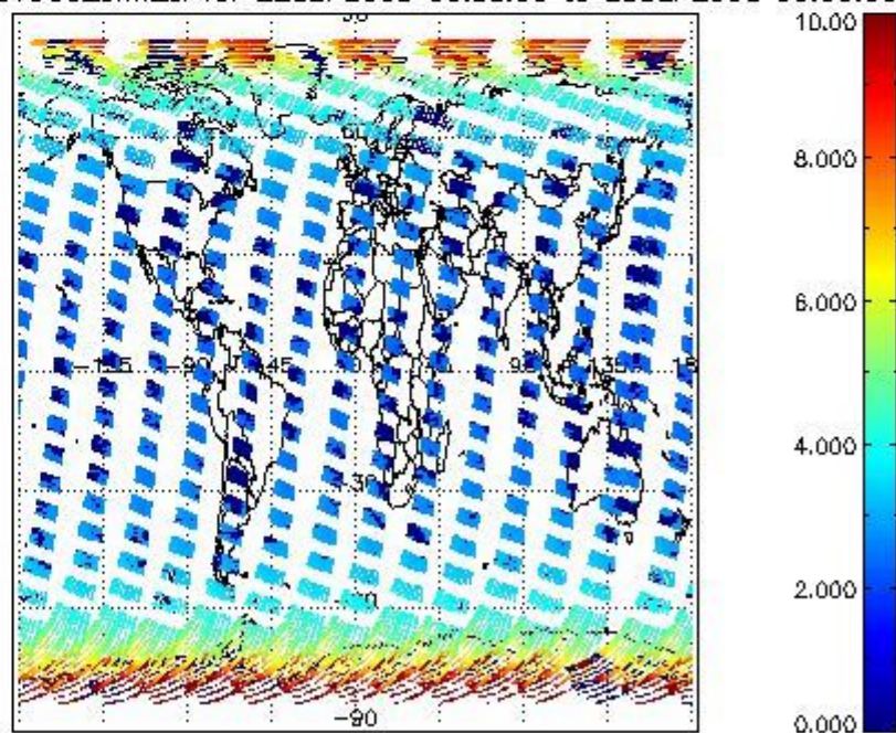
SCIOL2P_NADUV003_amf_cl for 22SEP2008 00:00:00 to 23SEP2008 00:00:00
