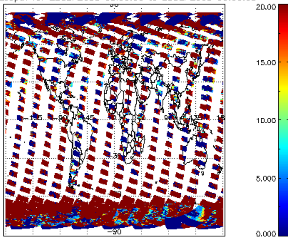
cl_opt_depth for 22SEP2008 00:00:00 to 23SEP2008 00:00:00
