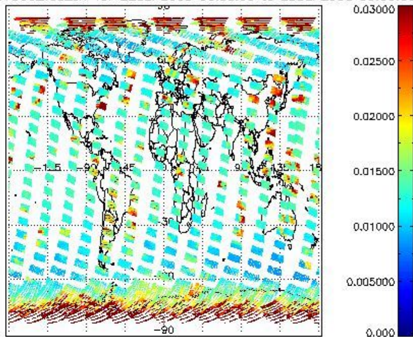
SCIOL2P_NADUV003_vcd_err for 22SEP2008 00:00:00 to 23SEP2008 00:00:00
