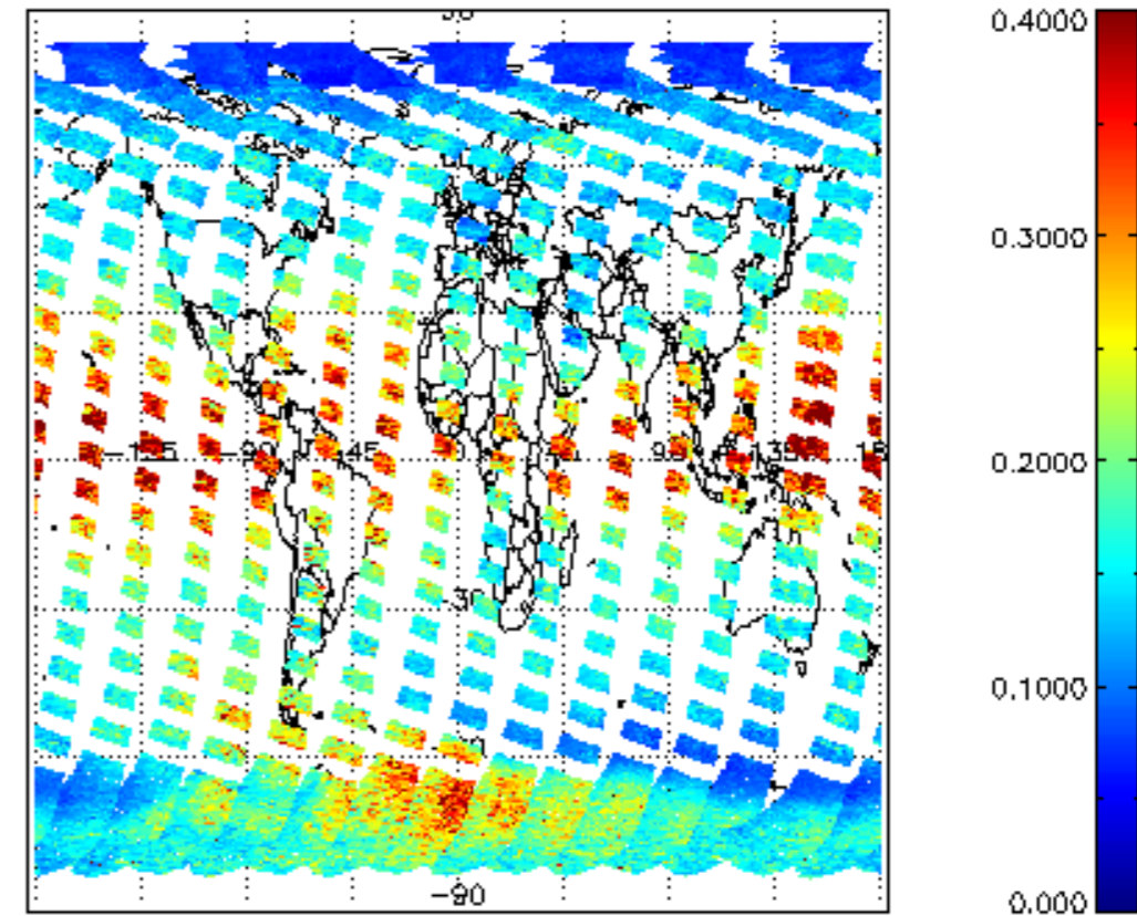
iCIOL2P_NADUV1NO2_vcd_err for 22SEP2008 00:00:00 to 23SEP2008 00:00:00
