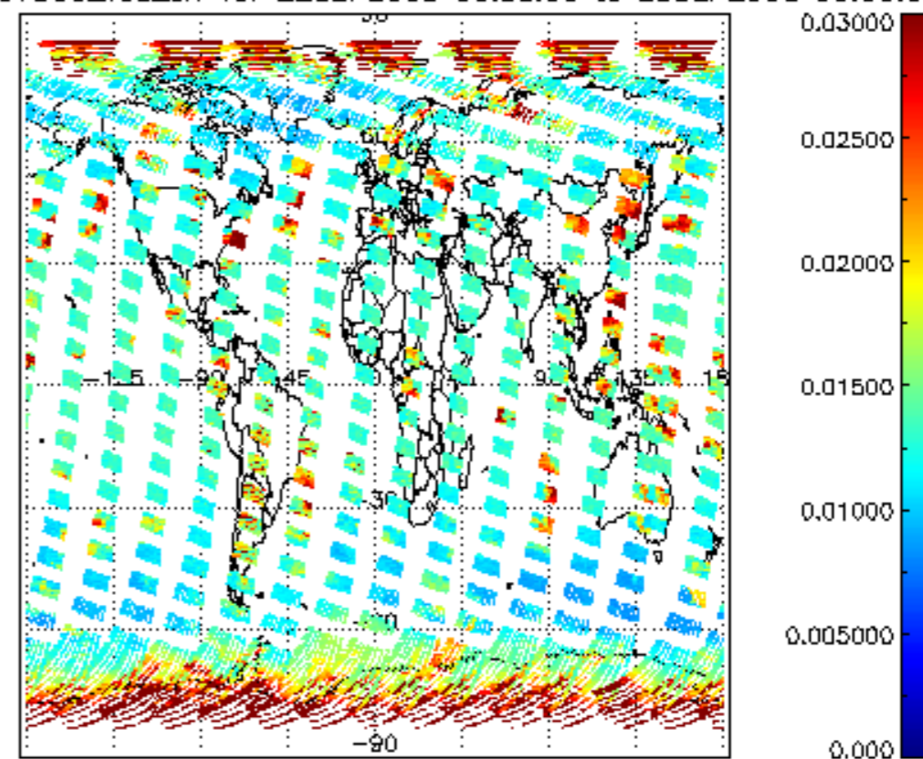
SCIOL2P_NADUV003_vcd_err for 22SEP2008 00:00:00 to 23SEP2008 00:00:00
