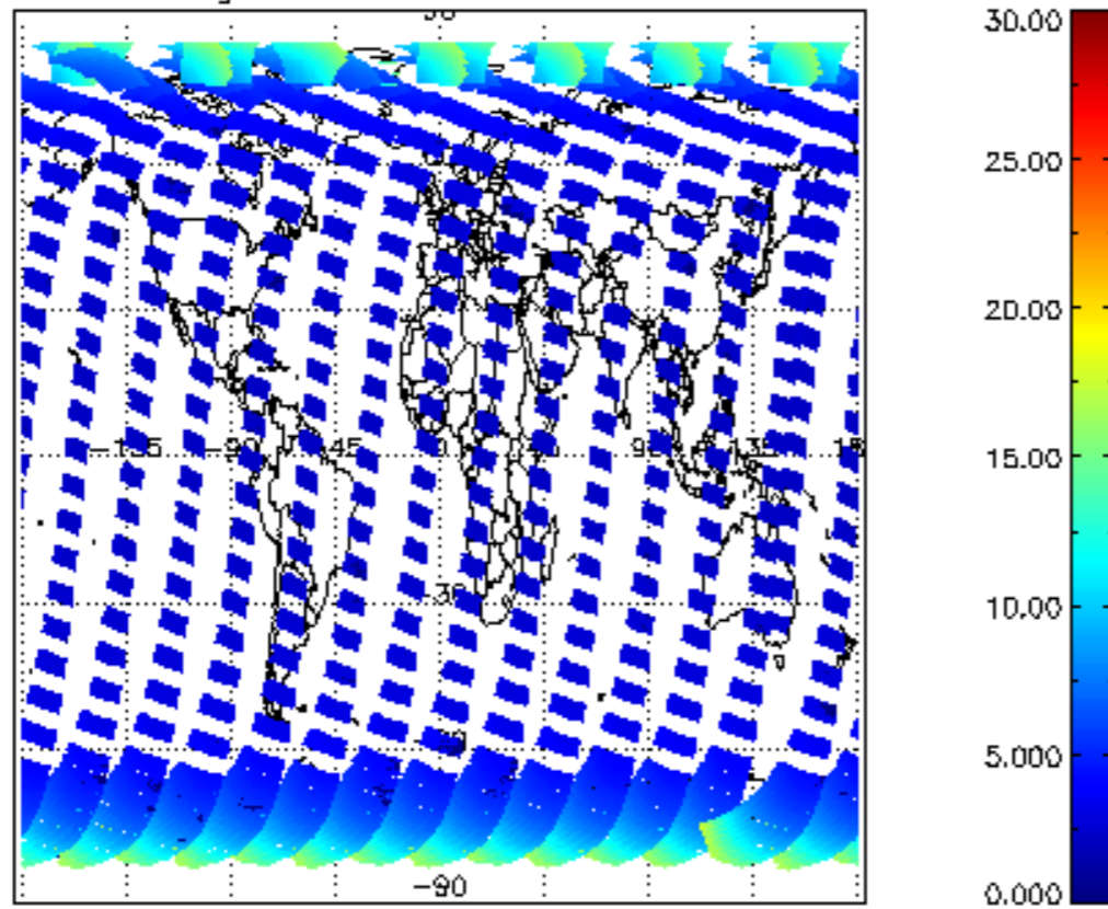
iCIOL2P_NADUV1NO2_amf_gr for 22SEP2008 00:00:00 to 23SEP2008 00:00:00
