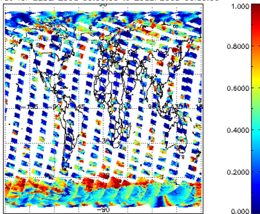
cl_frac for 22SEP2008 00:00:00 to 23SEP2008 00:00:00
