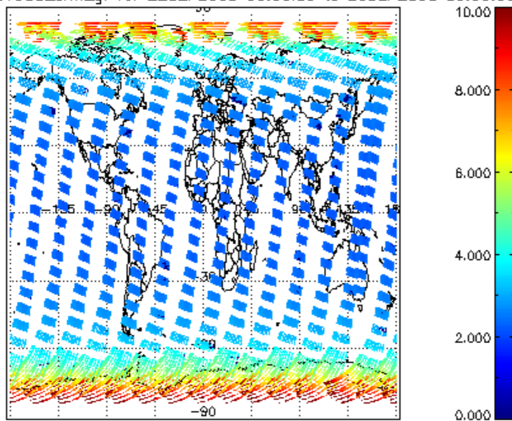
SCIOL2P_NADUV003_amf_gr for 22SEP2008 00:00:00 to 23SEP2008 00:00:00
