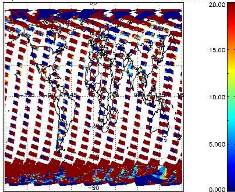
cL_opt_depth for 22SEP2008 00:00:00 to 23SEP2008 00:00:00
