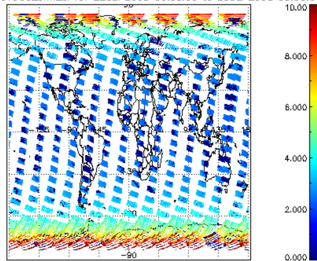
SCIOL2P_NADUV003_amf_cl for 22SEP2008 00:00:00 to 23SEP2008 00:00:00
