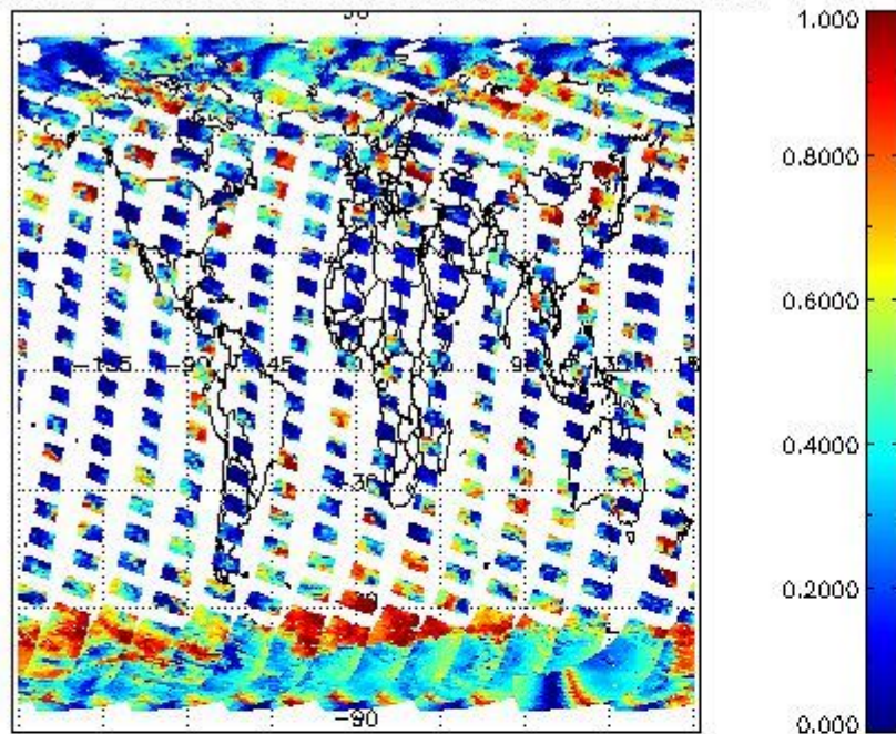
cL_frac for 22SEP2008 00:00:00 to 23SEP2008 00:00:00
