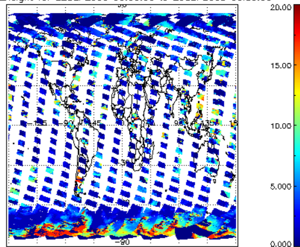
cl_top_height for 22SEP2008 00:00:00 to 23SEP2008 00:00:00
