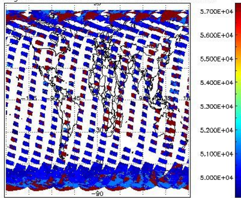
cloud_flags for 19SEP2008 00:00:00 to 20SEP2008 00:00:00
