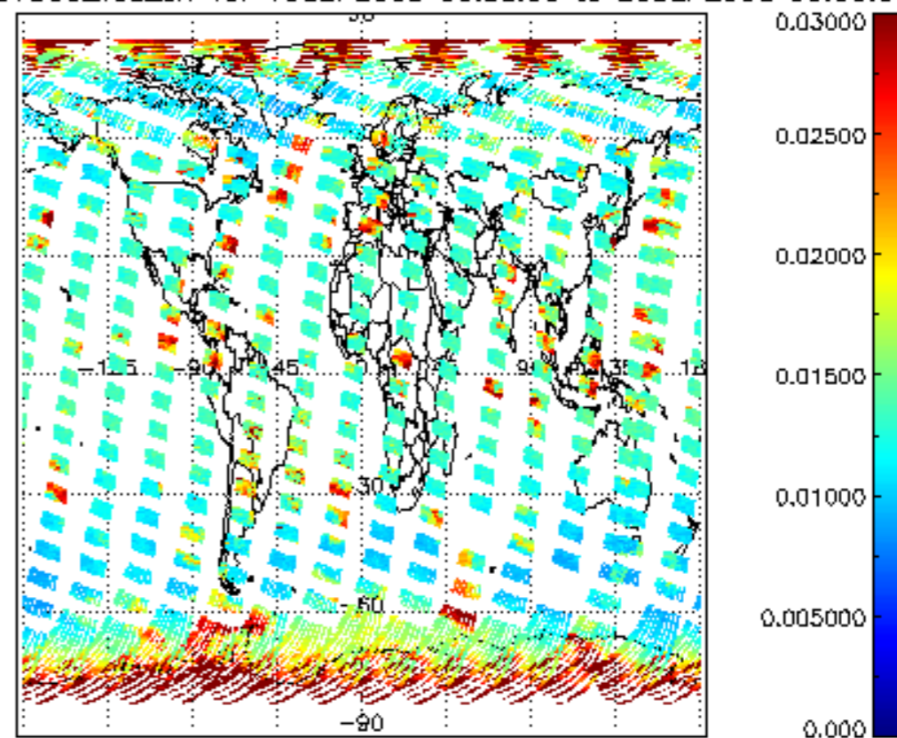
SCIOL2P_NADUV003_vcd_err for 19SEP2008 00:00:00 to 20SEP2008 00:00:00
