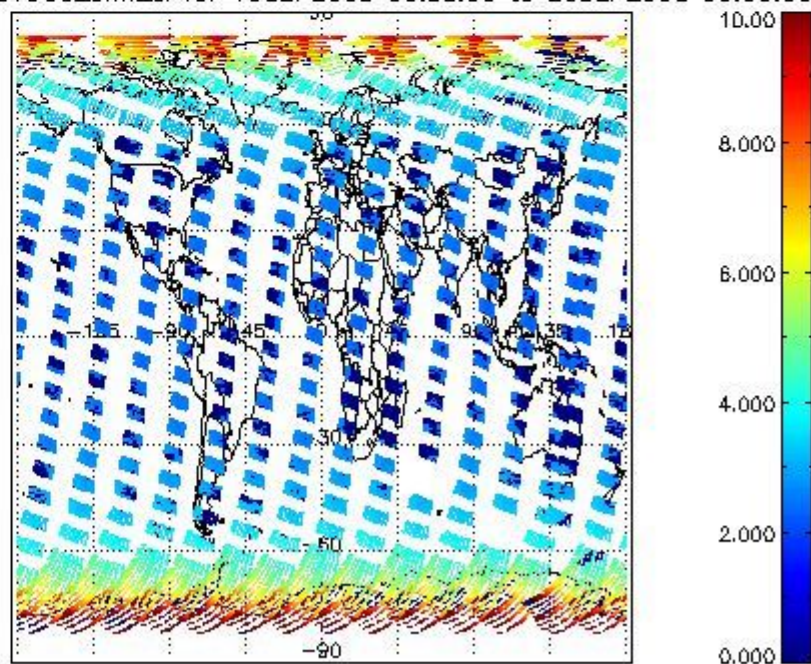
SCIOL2P_NADUV003_amf_cl for 19SEP2008 00:00:00 to 20SEP2008 00:00:00
