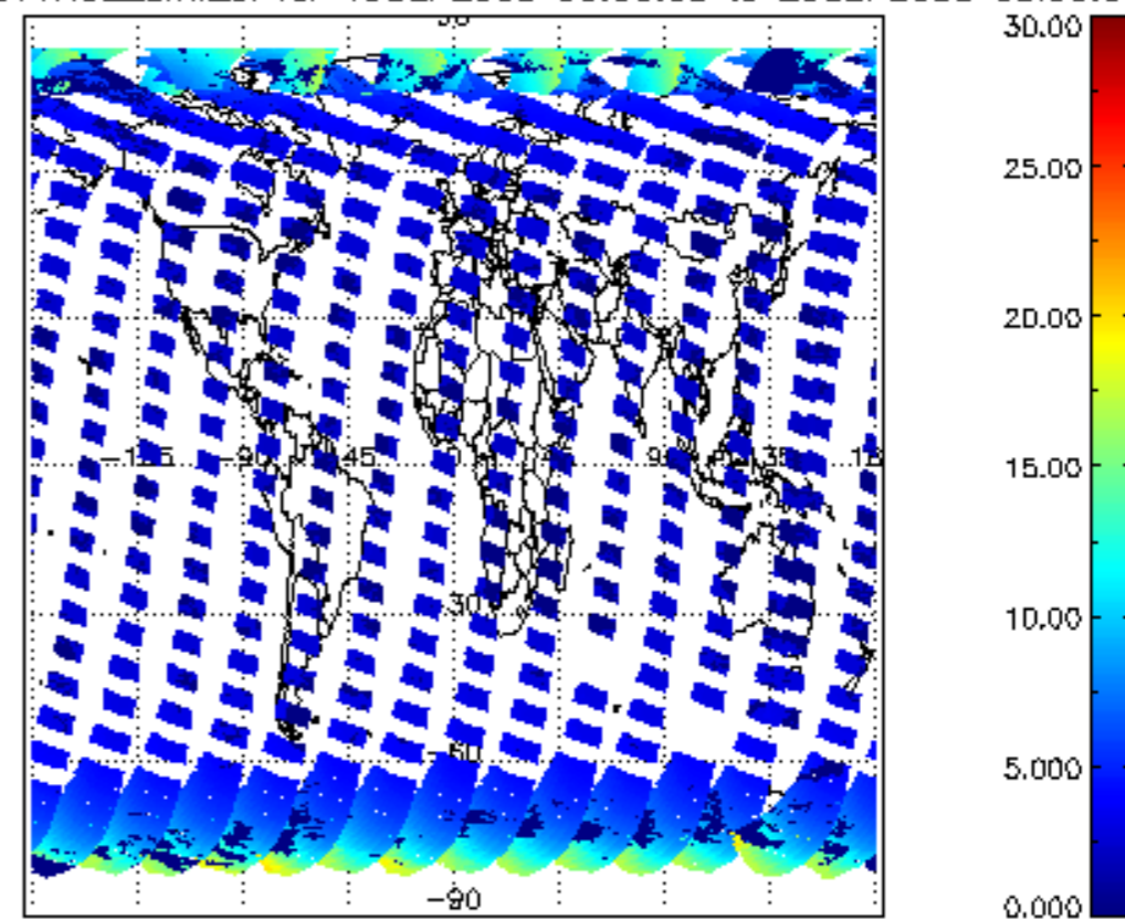
iCIOL2P_NADUV1NO2_amf_cl for 19SEP2008 00:00:00 to 20SEP2008 00:00:00
