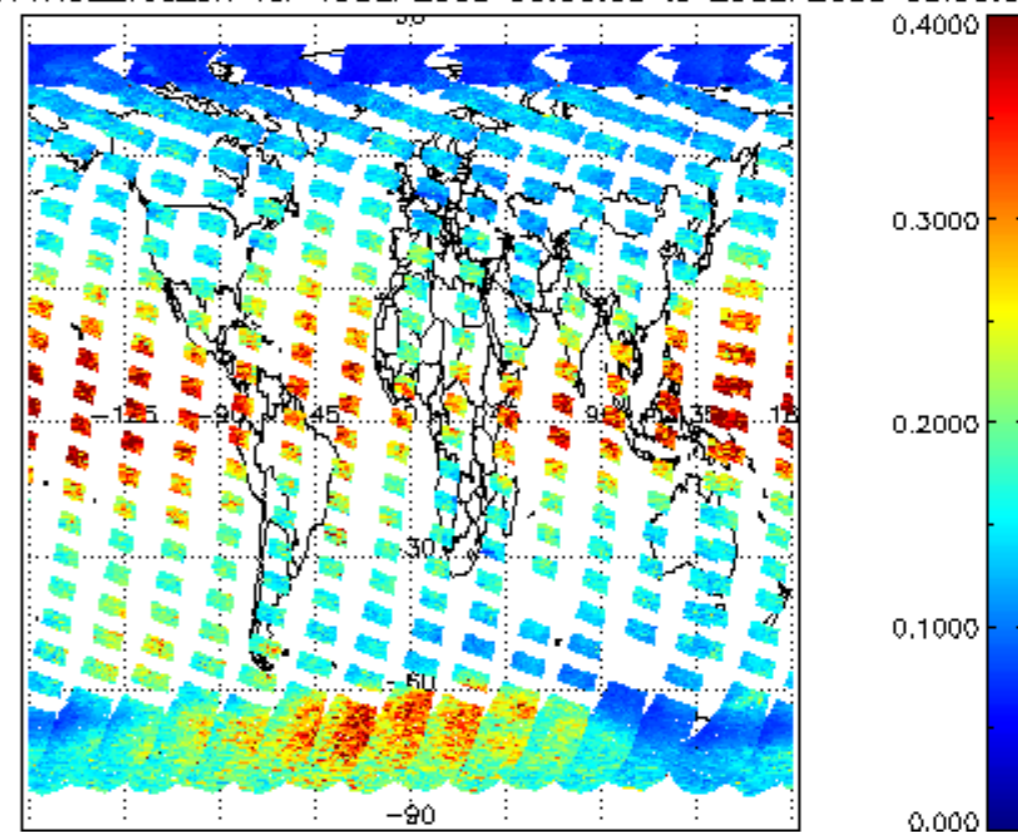
iCIOL2P_NADUV1NO2_vcd_err for 19SEP2008 00:00:00 to 20SEP2008 00:00:00
