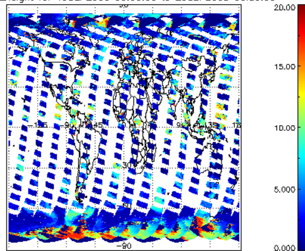
cl_top_height for 19SEP2008 00:00:00 to 20SEP2008 00:00:00
