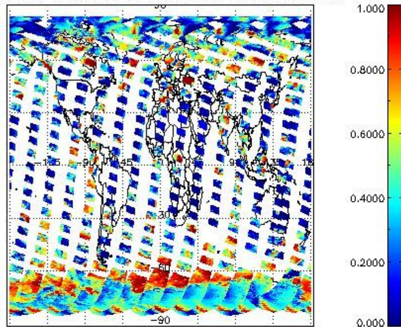
cL_frac for 19SEP2008 00:00:00 to 20SEP2008 00:00:00
