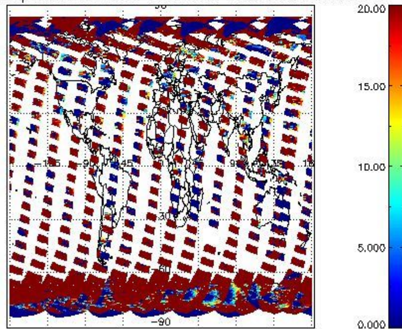
cL_opt_depth for 19SEP2008 00:00:00 to 20SEP2008 00:00:00
