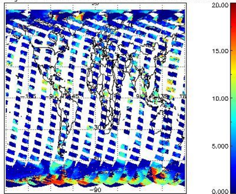
cL_top_height for 19SEP2008 00:00:00 to 20SEP2008 00:00:00
