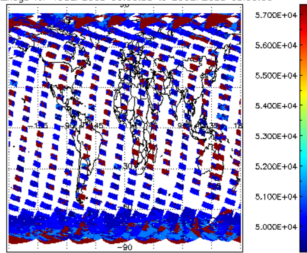
cloud_flags for 19SEP2008 00:00:00 to 20SEP2008 00:00:00
