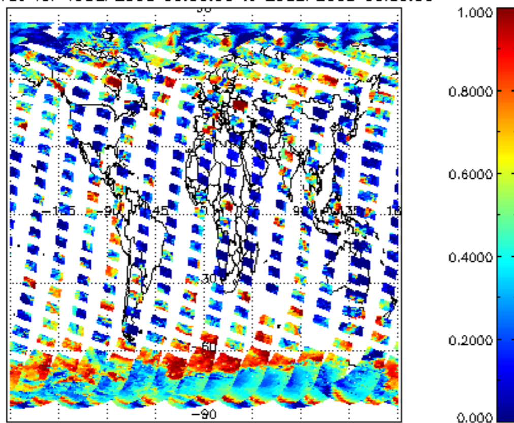
cl_frac for 19SEP2008 00:00:00 to 20SEP2008 00:00:00
