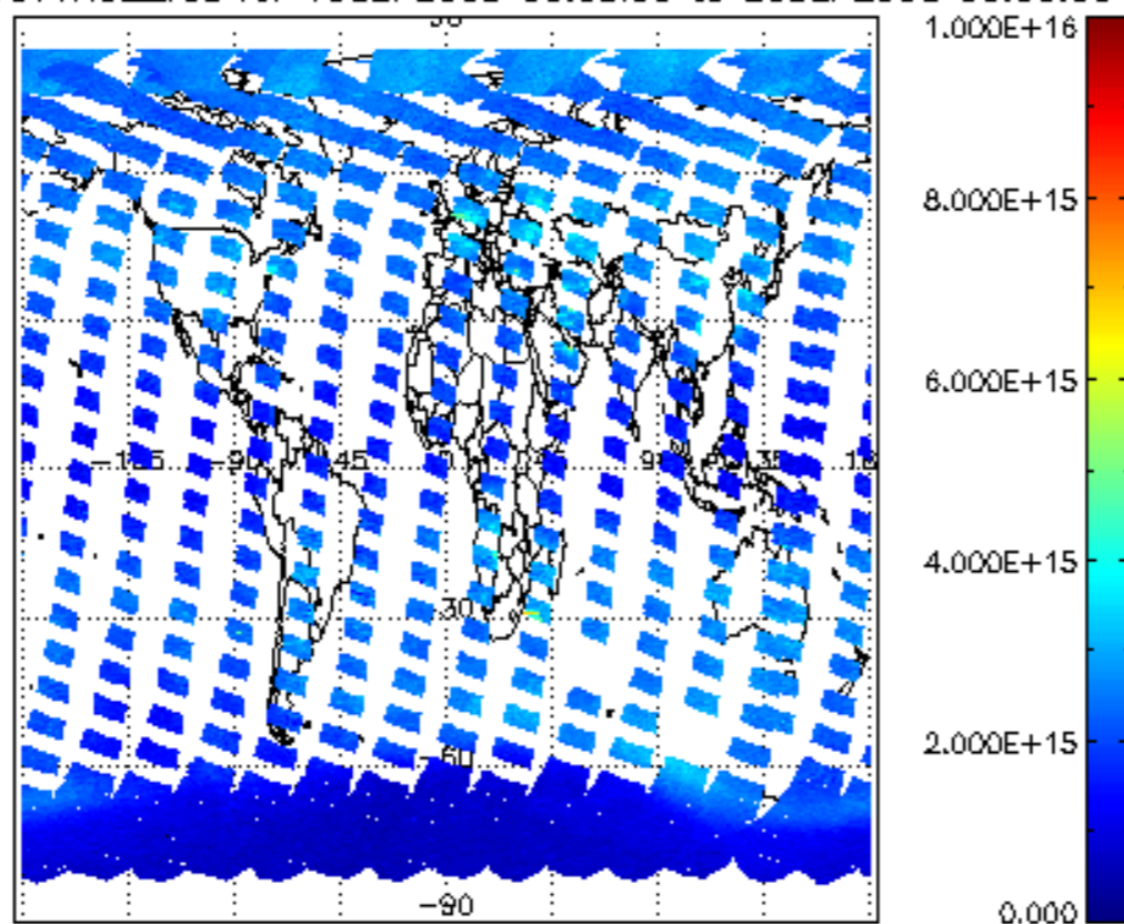
SCIOL2P_NADUV1NO2_vcd for 19SEP2008 00:00:00 to 20SEP2008 00:00:00
