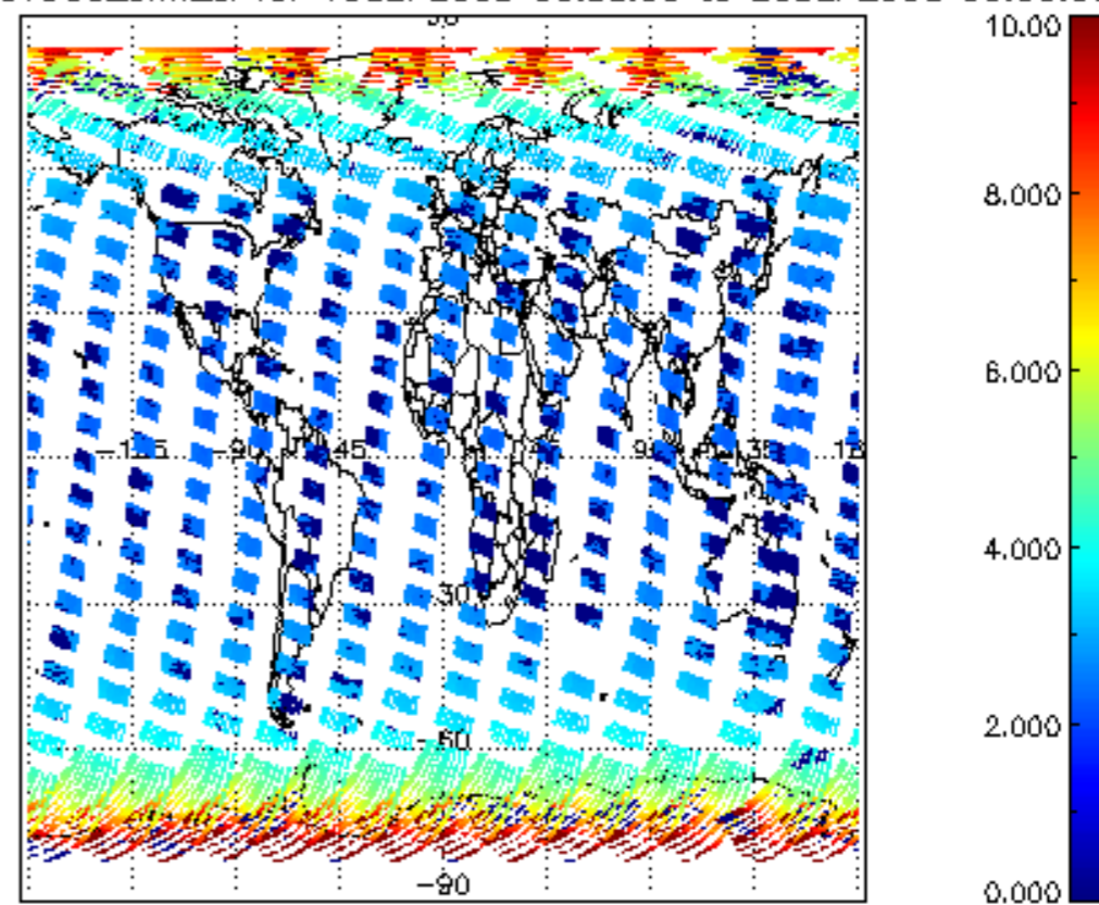
SCIOL2P_NADUV003_amf_cl for 19SEP2008 00:00:00 to 20SEP2008 00:00:00
