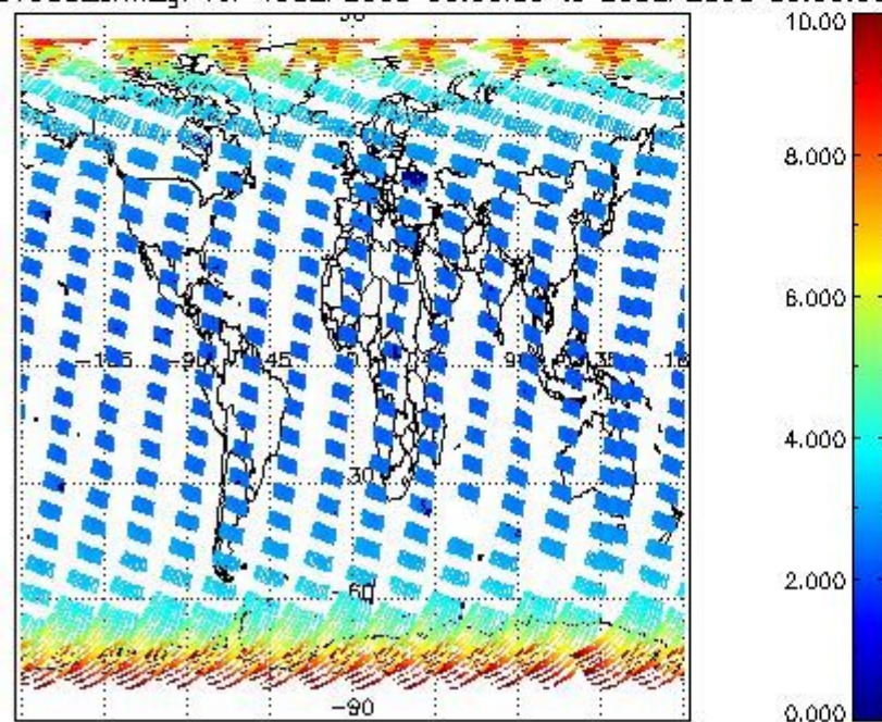
SCIOL2P_NADUV003_amf_gr for 19SEP2008 00:00:00 to 20SEP2008 00:00:00
