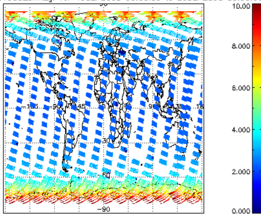
SCIOL2P_NADUV003_amf_gr for 19SEP2008 00:00:00 to 20SEP2008 00:00:00
