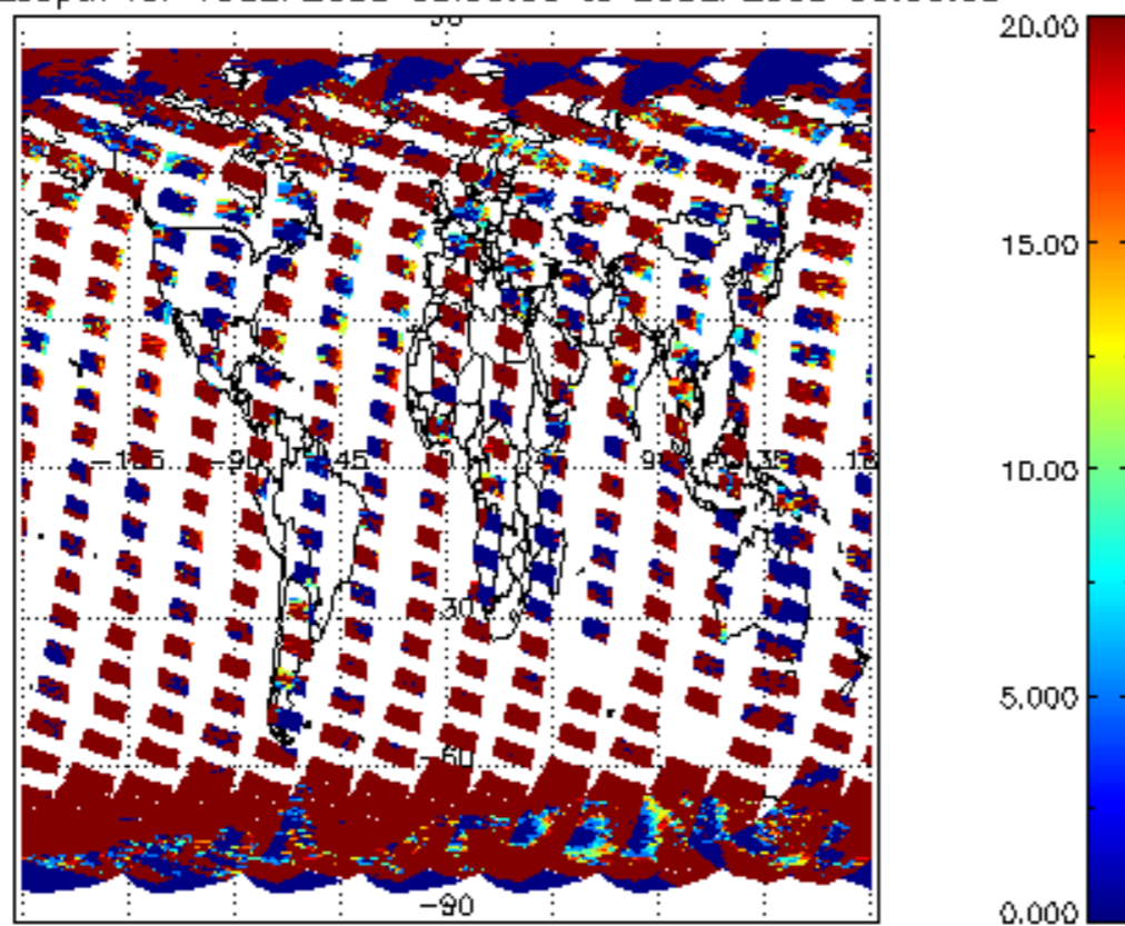
cl_opt_depth for 19SEP2008 00:00:00 to 20SEP2008 00:00:00
