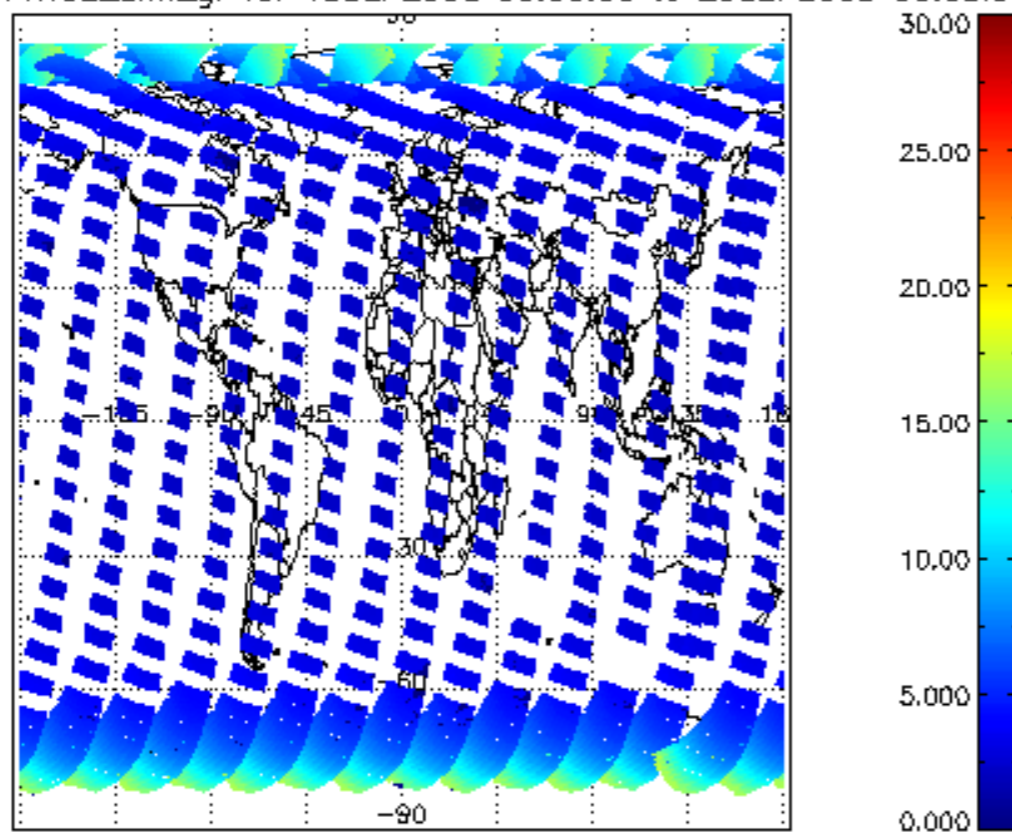
iCIOL2P_NADUV1NO2_amf_gr for 19SEP2008 00:00:00 to 20SEP2008 00:00:00
