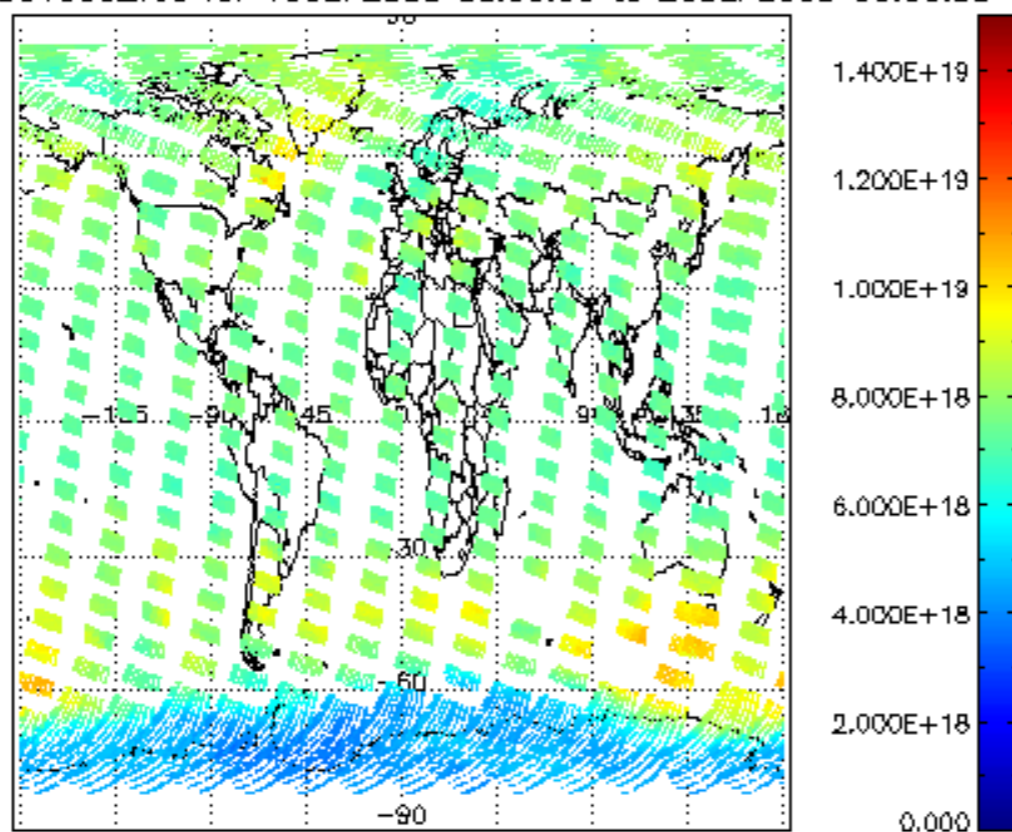
SCIOL2P_NADUV003_vcd for 19SEP2008 00:00:00 to 20SEP2008 00:00:00
