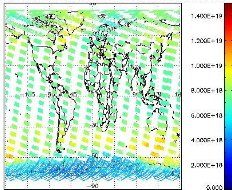
SCIOL2P_NADUV003_vcd for 19SEP2008 00:00:00 to 20SEP2008 00:00:00
