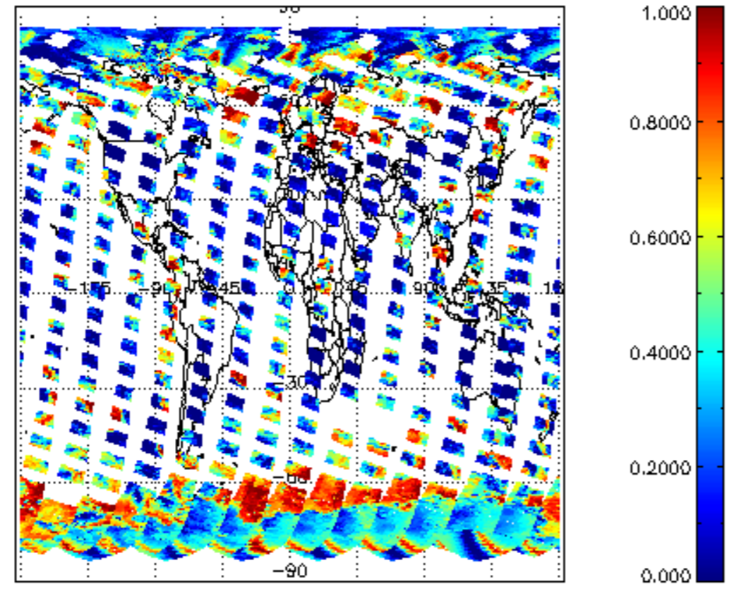
cl_frac for 16SEP2008 00:00:00 to 17SEP2008 00:00:00
