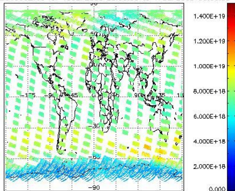
SCIOL2P_NADUV003_vcd for 16SEP2008 00:00:00 to 17SEP2008 00:00:00
