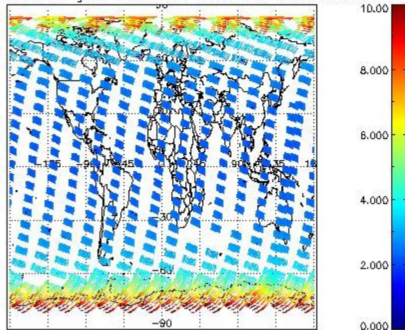
SCIOL2P_NADUV003_amf_gr for 16SEP2008 00:00:00 to 17SEP2008 00:00:00
