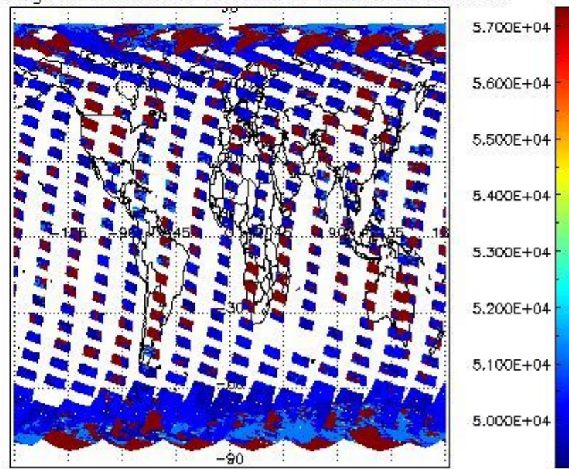
cloud_flags for 16SEP2008 00:00:00 to 17SEP2008 00:00:00
