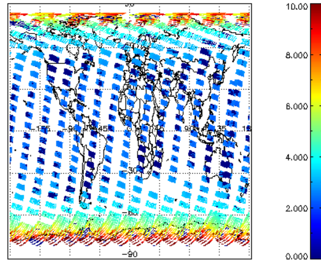
SCIOL2P_NADUV003_amf_cl for 16SEP2008 00:00:00 to 17SEP2008 00:00:00
