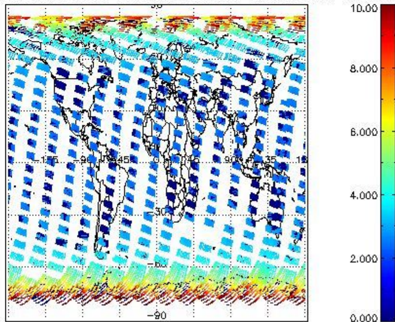
SCIOL2P_NADUV003_amf_cl for 16SEP2008 00:00:00 to 17SEP2008 00:00:00
