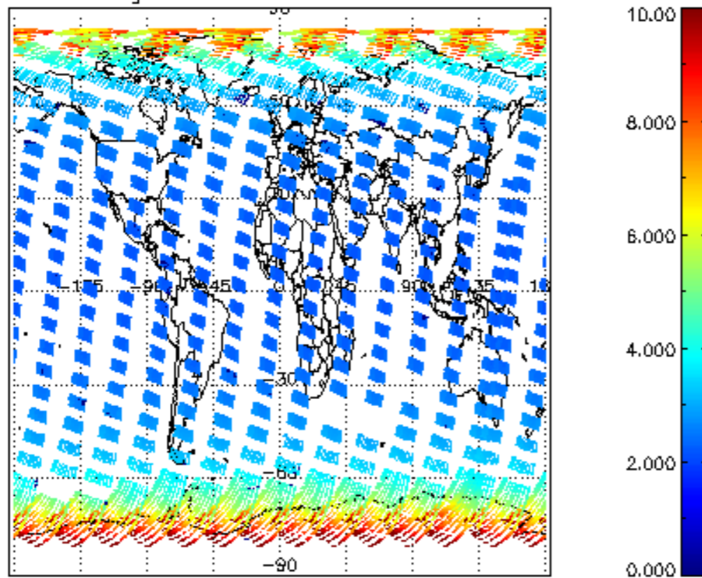
SCIOL2P_NADUV003_amf_gr for 16SEP2008 00:00:00 to 17SEP2008 00:00:00
