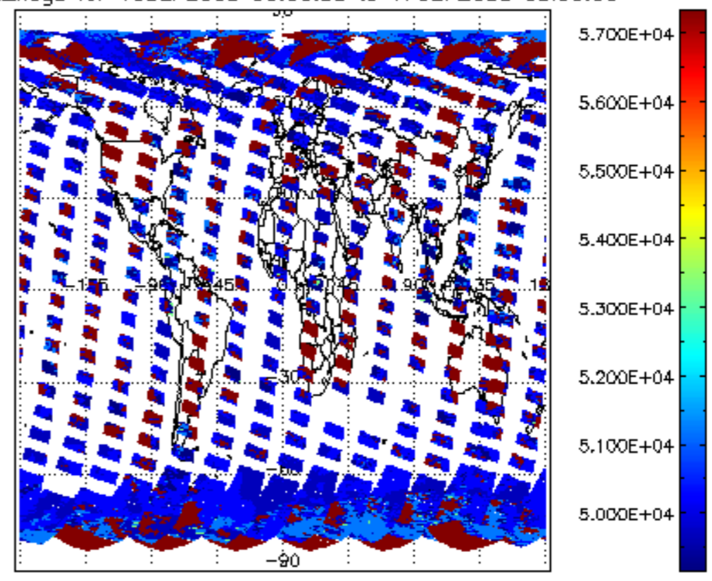
cloud_flags for 16SEP2008 00:00:00 to 17SEP2008 00:00:00
