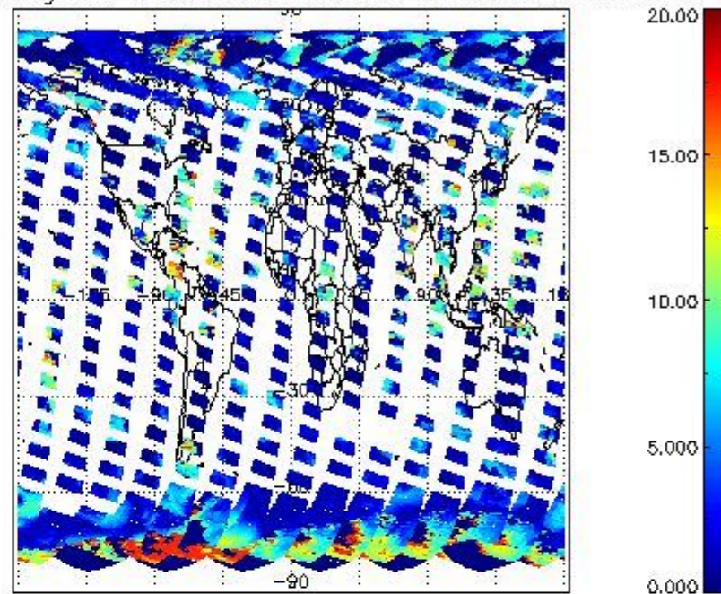
cL_top_height for 16SEP2008 00:00:00 to 17SEP2008 00:00:00
