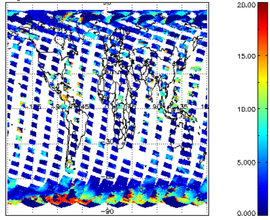
cl_top_height for 16SEP2008 00:00:00 to 17SEP2008 00:00:00
