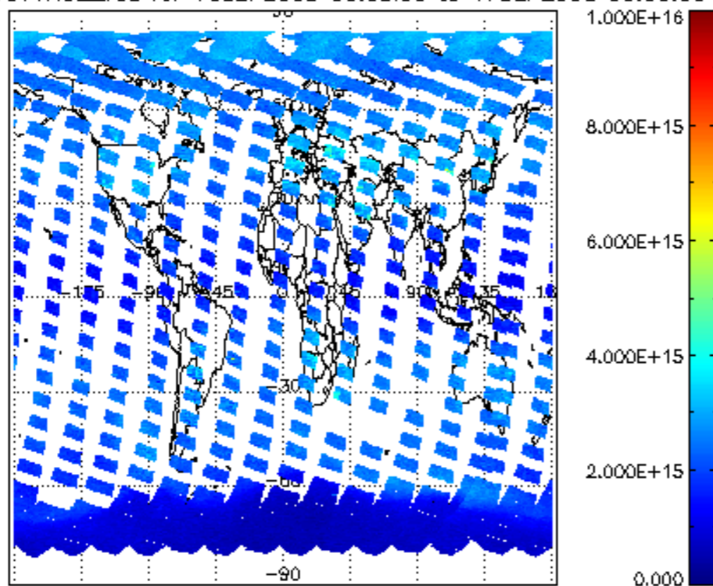
SCIOL2P_NADUV1NO2_vcd for 16SEP2008 00:00:00 to 17SEP2008 00:00:00
