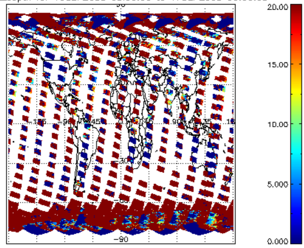
cl_opt_depth for 16SEP2008 00:00:00 to 17SEP2008 00:00:00
