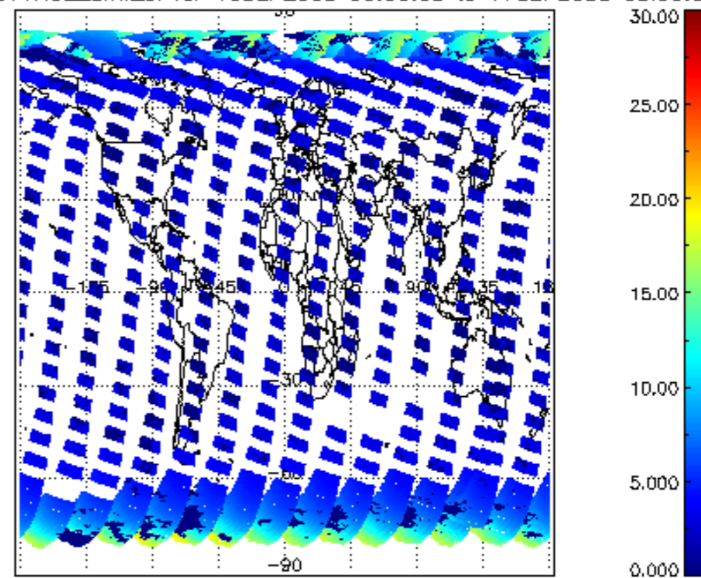
iCIOL2P_NADUV1NO2_amf_cl for 16SEP2008 00:00:00 to 17SEP2008 00:00:00
