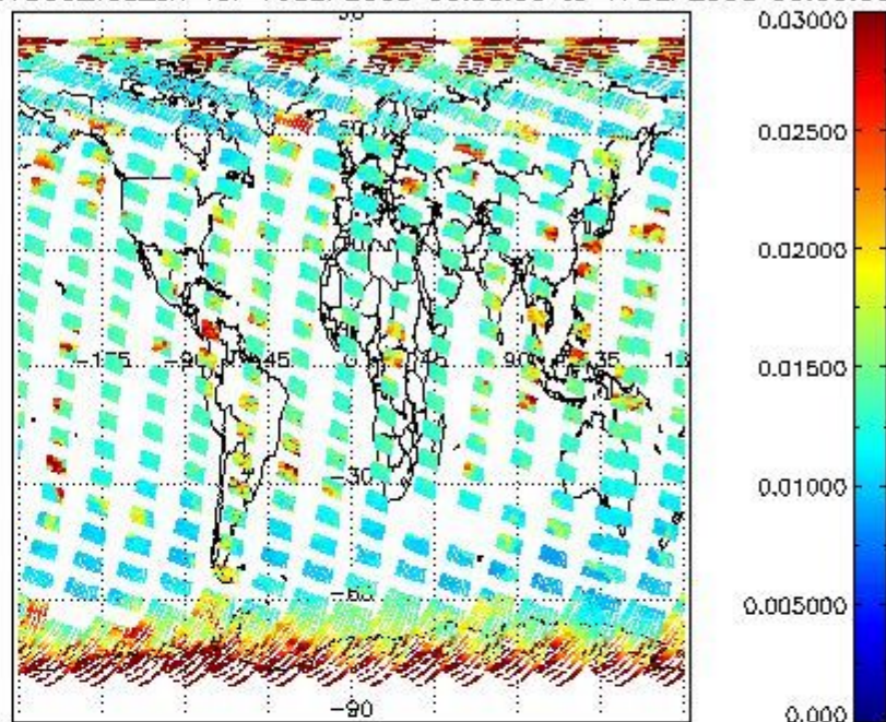
SCIOL2P_NADUV003_vcd_err for 16SEP2008 00:00:00 to 17SEP2008 00:00:00
