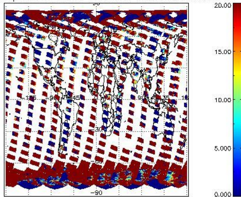
cL_opt_depth for 16SEP2008 00:00:00 to 17SEP2008 00:00:00
