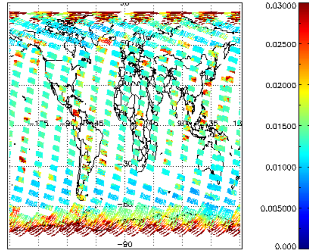
SCIOL2P_NADUV003_vcd_err for 16SEP2008 00:00:00 to 17SEP2008 00:00:00
