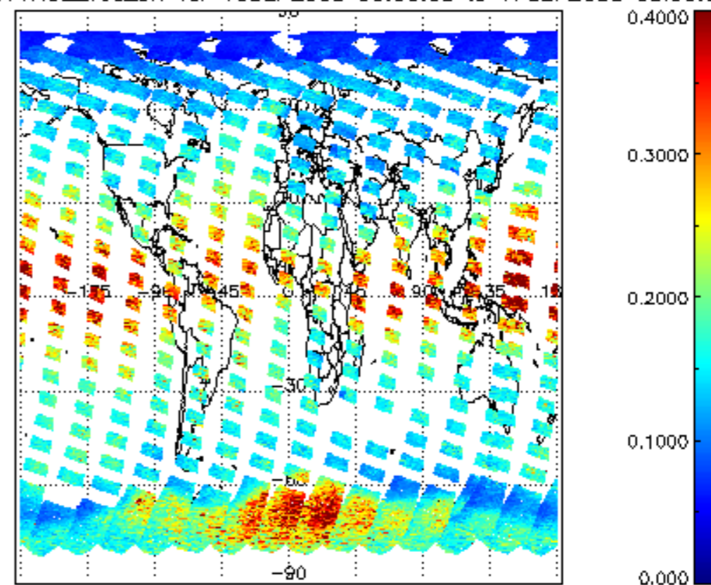
iCIOL2P_NADUV1NO2_vcd_err for 16SEP2008 00:00:00 to 17SEP2008 00:00:00
