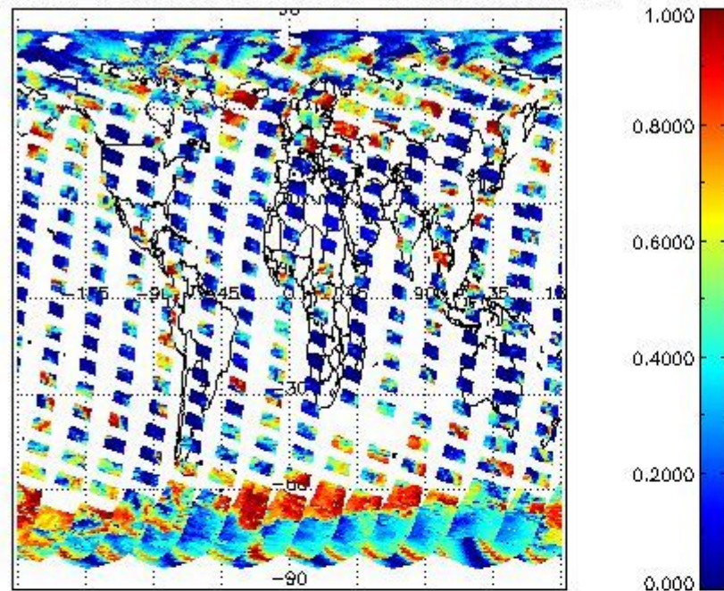
cL_frac for 16SEP2008 00:00:00 to 17SEP2008 00:00:00
