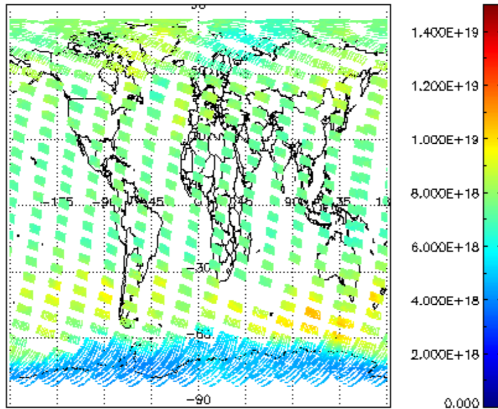
SCIOL2P_NADUV003_vcd for 16SEP2008 00:00:00 to 17SEP2008 00:00:00
