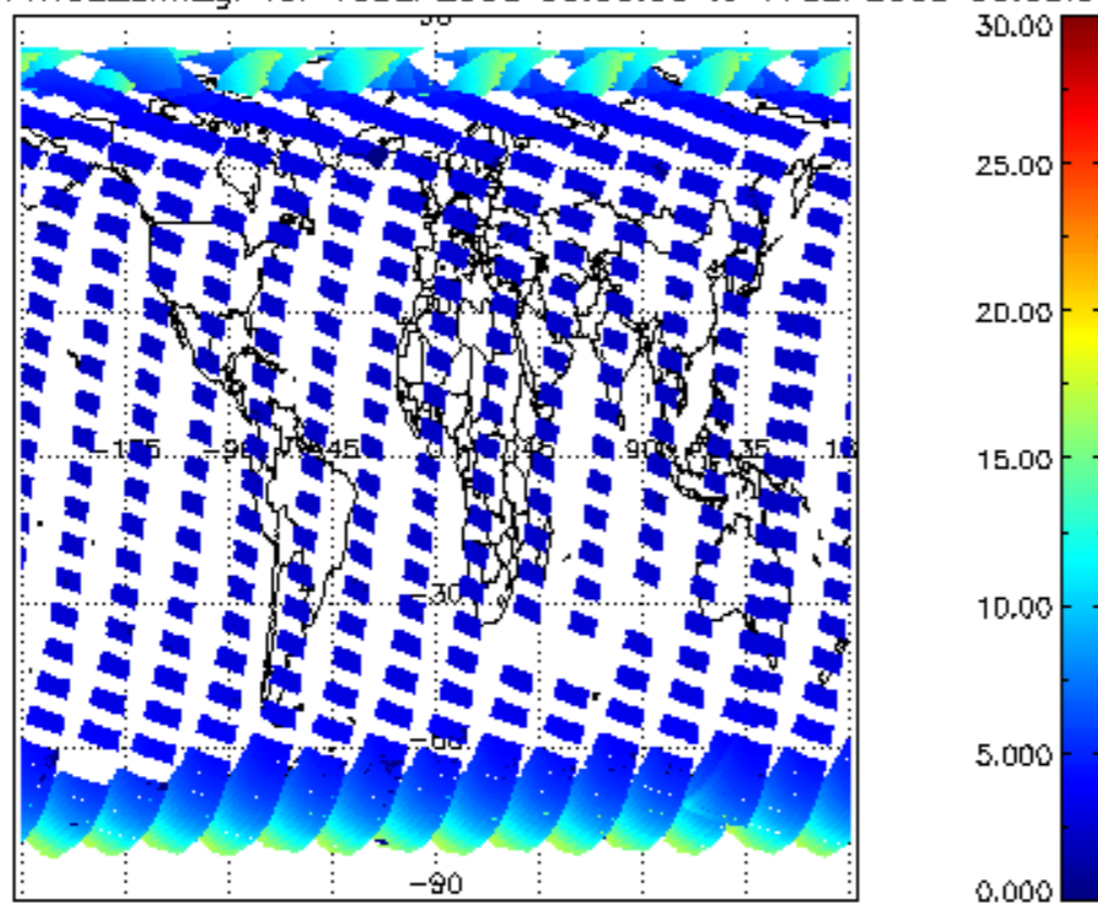
iCIOL2P_NADUV1NO2_amf_gr for 16SEP2008 00:00:00 to 17SEP2008 00:00:00
