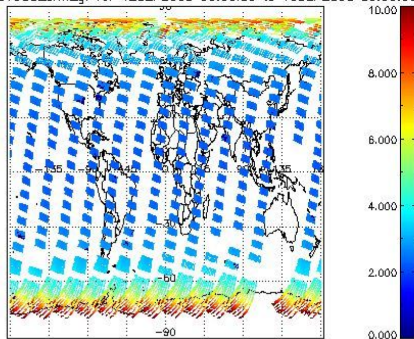
SCIOL2P_NADUV003_amf_gr for 12SEP2008 00:00:00 to 13SEP2008 00:00:00
