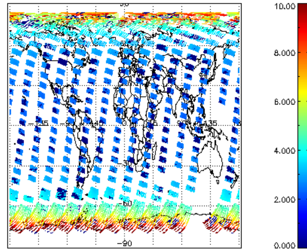
SCIOL2P_NADUV003_amf_cl for 12SEP2008 00:00:00 to 13SEP2008 00:00:00
