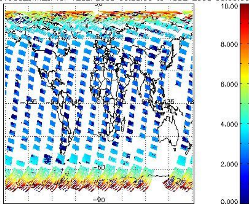
SCIOL2P_NADUV003_amf_cl for 12SEP2008 00:00:00 to 13SEP2008 00:00:00
