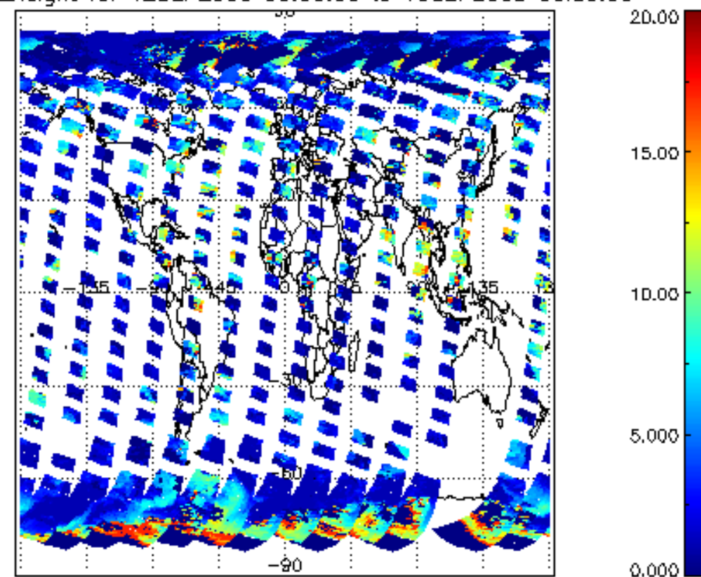
cL_top_height for 12SEP2008 00:00:00 to 13SEP2008 00:00:00
