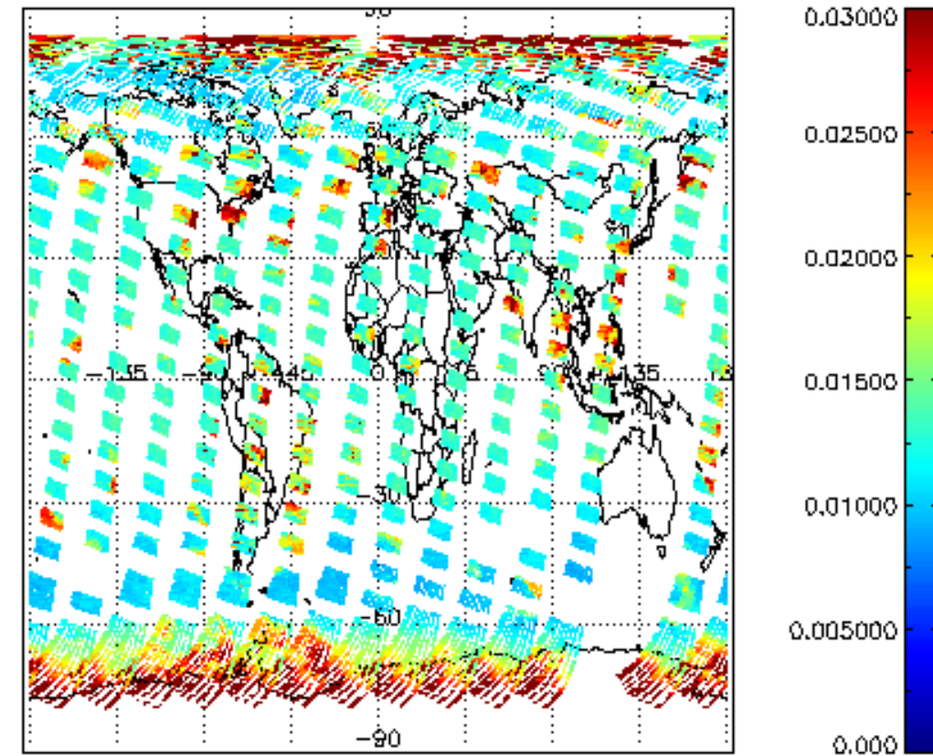
SCIOL2P_NADUV003_vcd_err for 12SEP2008 00:00:00 to 13SEP2008 00:00:00
