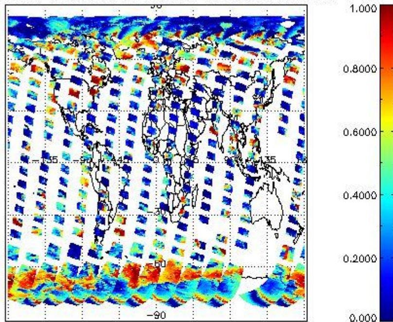
cL_frac for 12SEP2008 00:00:00 to 13SEP2008 00:00:00
