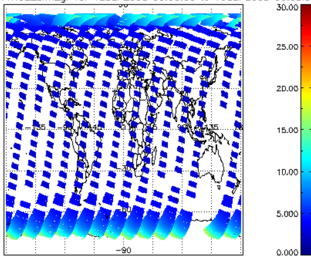
iCIOL2P_NADUV1NO2_amf_gr for 12SEP2008 00:00:00 to 13SEP2008 00:00:00
