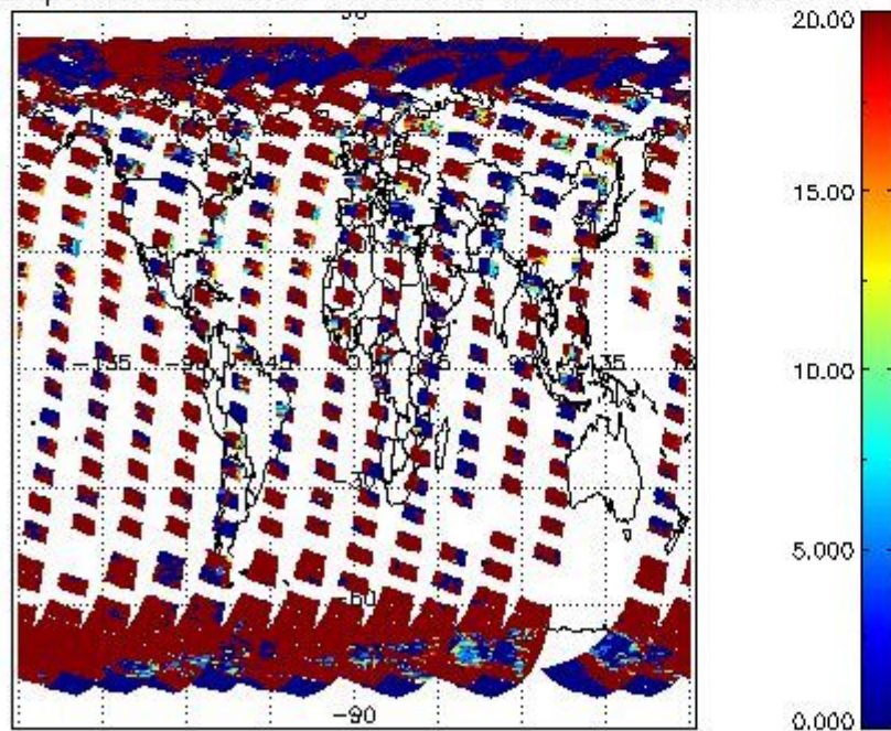
cL_opt_depth for 12SEP2008 00:00:00 to 13SEP2008 00:00:00
