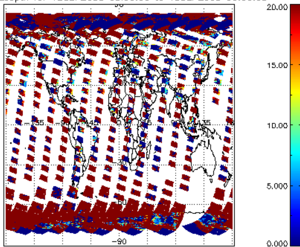
cL_opt_depth for 12SEP2008 00:00:00 to 13SEP2008 00:00:00
