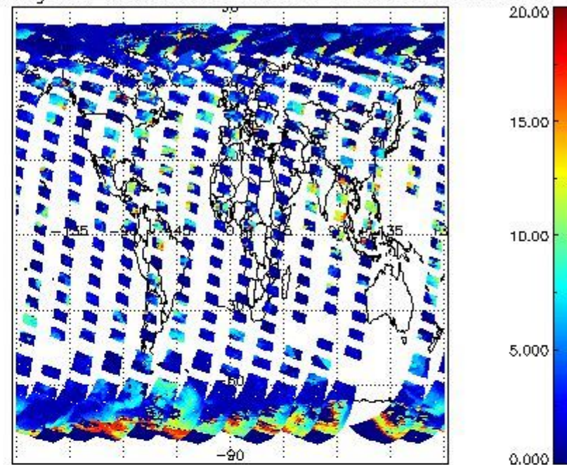
cL_top_height for 12SEP2008 00:00:00 to 13SEP2008 00:00:00
