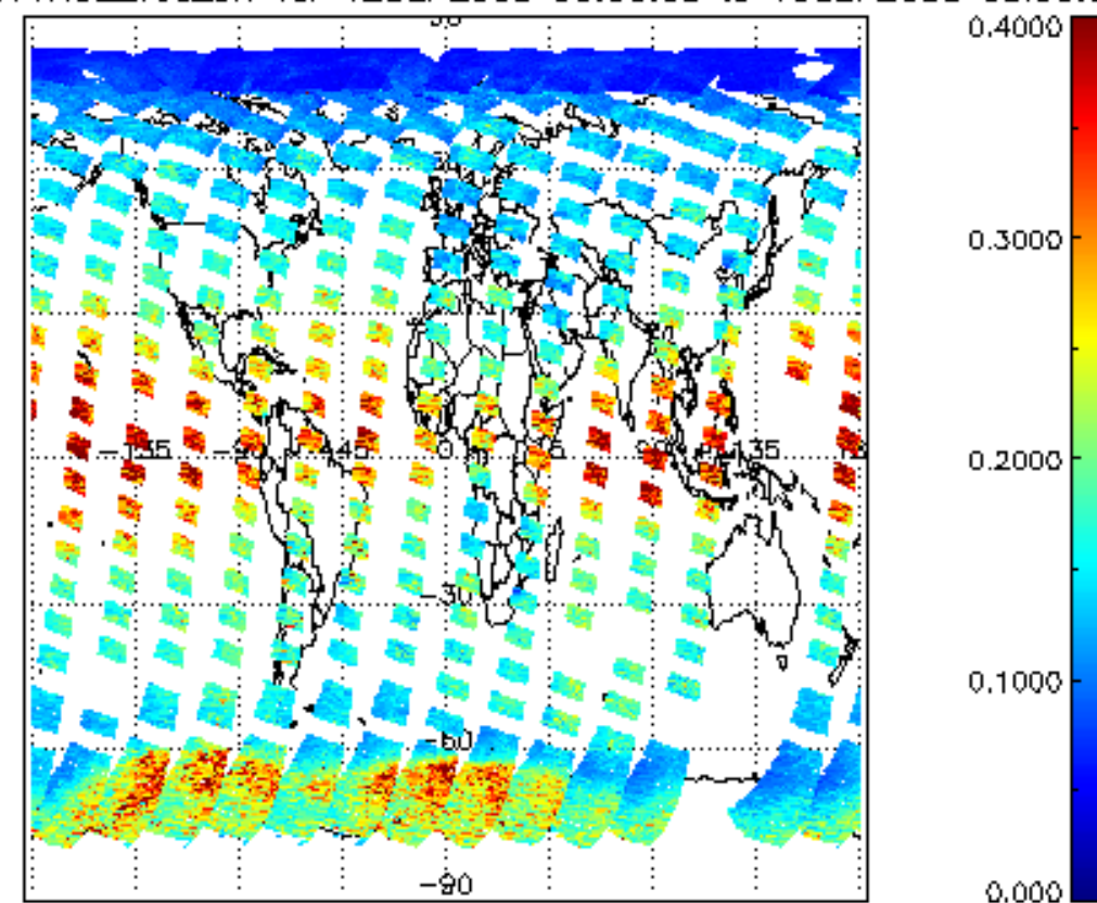
iCIOL2P_NADUV1NO2_vcd_err for 12SEP2008 00:00:00 to 13SEP2008 00:00:00
