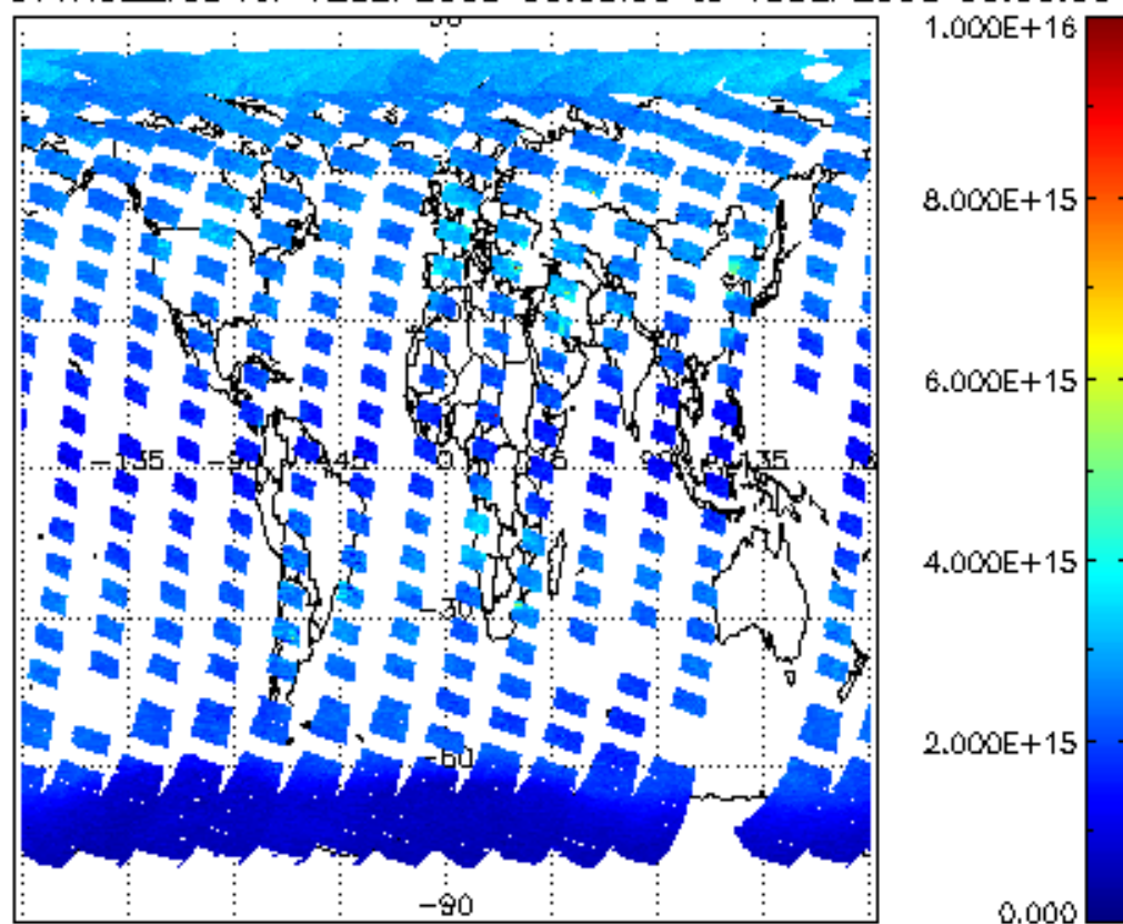
SCIOL2P_NADUV1NO2_vcd for 12SEP2008 00:00:00 to 13SEP2008 00:00:00
