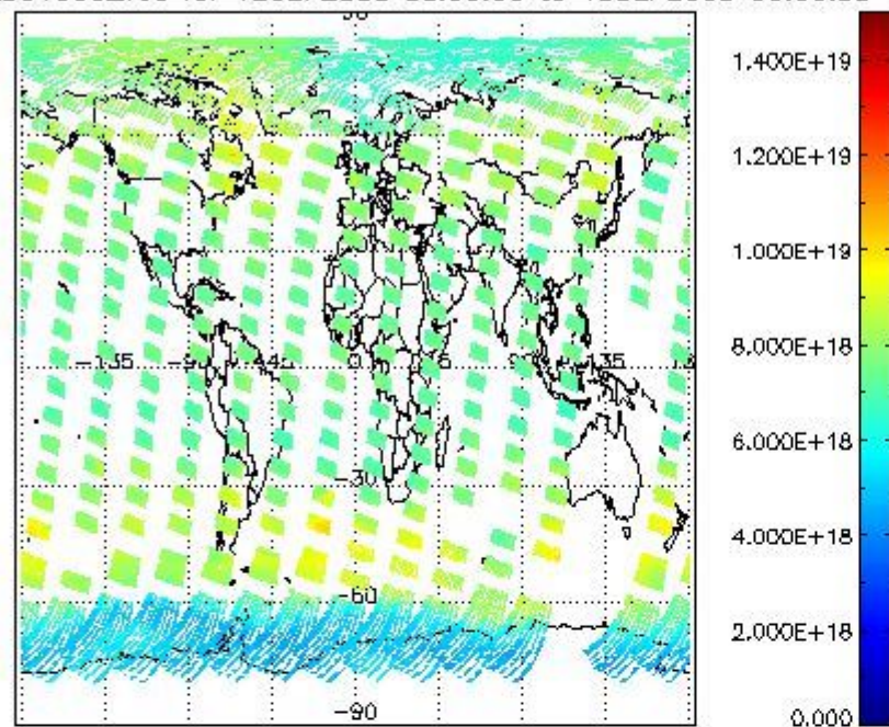
SCIOL2P_NADUV003_vcd for 12SEP2008 00:00:00 to 13SEP2008 00:00:00
