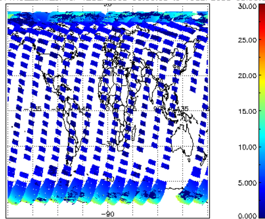
iCIOL2P_NADUV1NO2_amf_cl for 12SEP2008 00:00:00 to 13SEP2008 00:00:00
