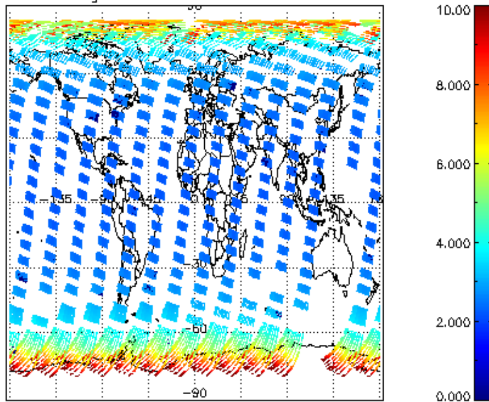
SCIOL2P_NADUV003_amf_gr for 12SEP2008 00:00:00 to 13SEP2008 00:00:00
