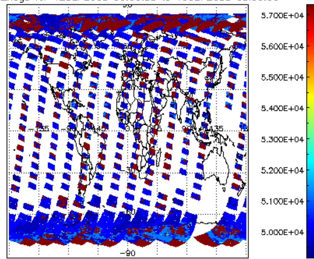
cloud_flags for 12SEP2008 00:00:00 to 13SEP2008 00:00:00
