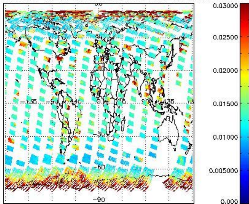
SCIOL2P_NADUV003_vcd_err for 12SEP2008 00:00:00 to 13SEP2008 00:00:00
