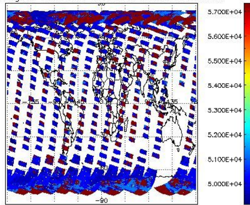
cloud_flags for 12SEP2008 00:00:00 to 13SEP2008 00:00:00
