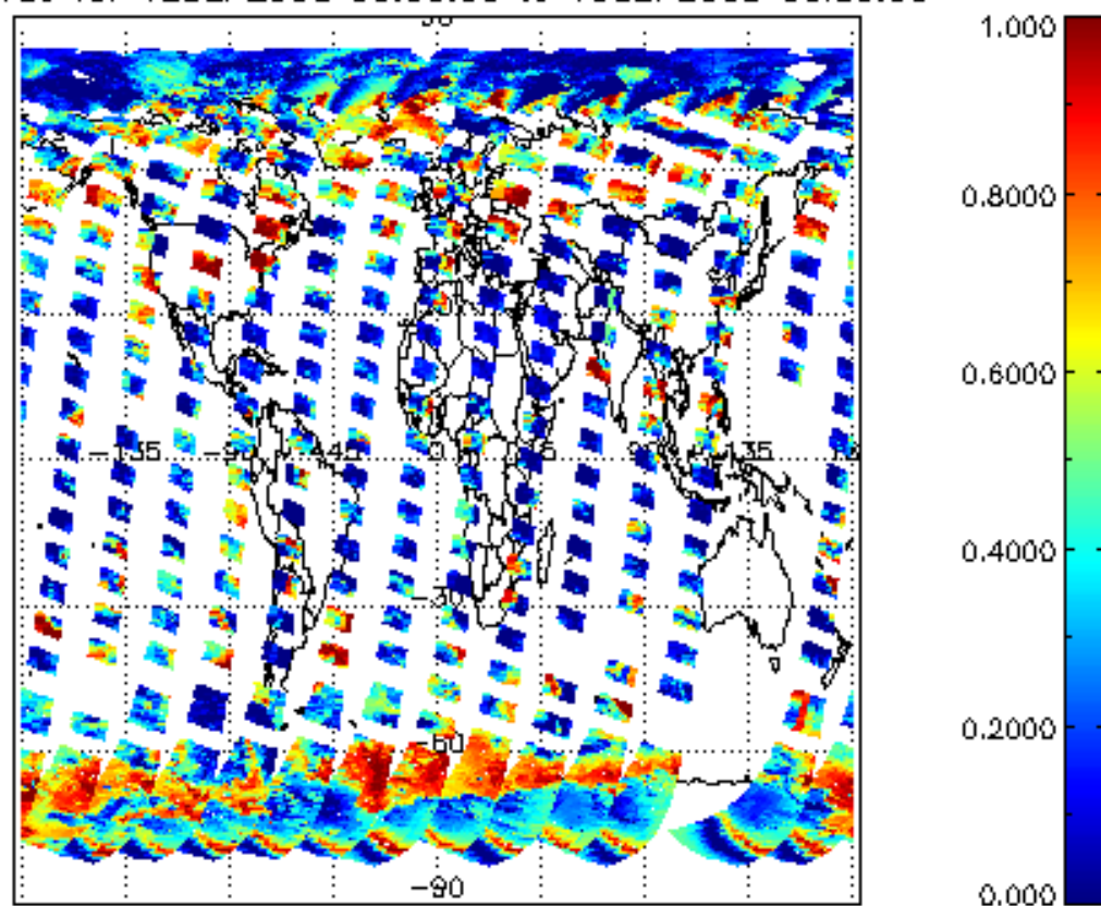
cL_frac for 12SEP2008 00:00:00 to 13SEP2008 00:00:00
