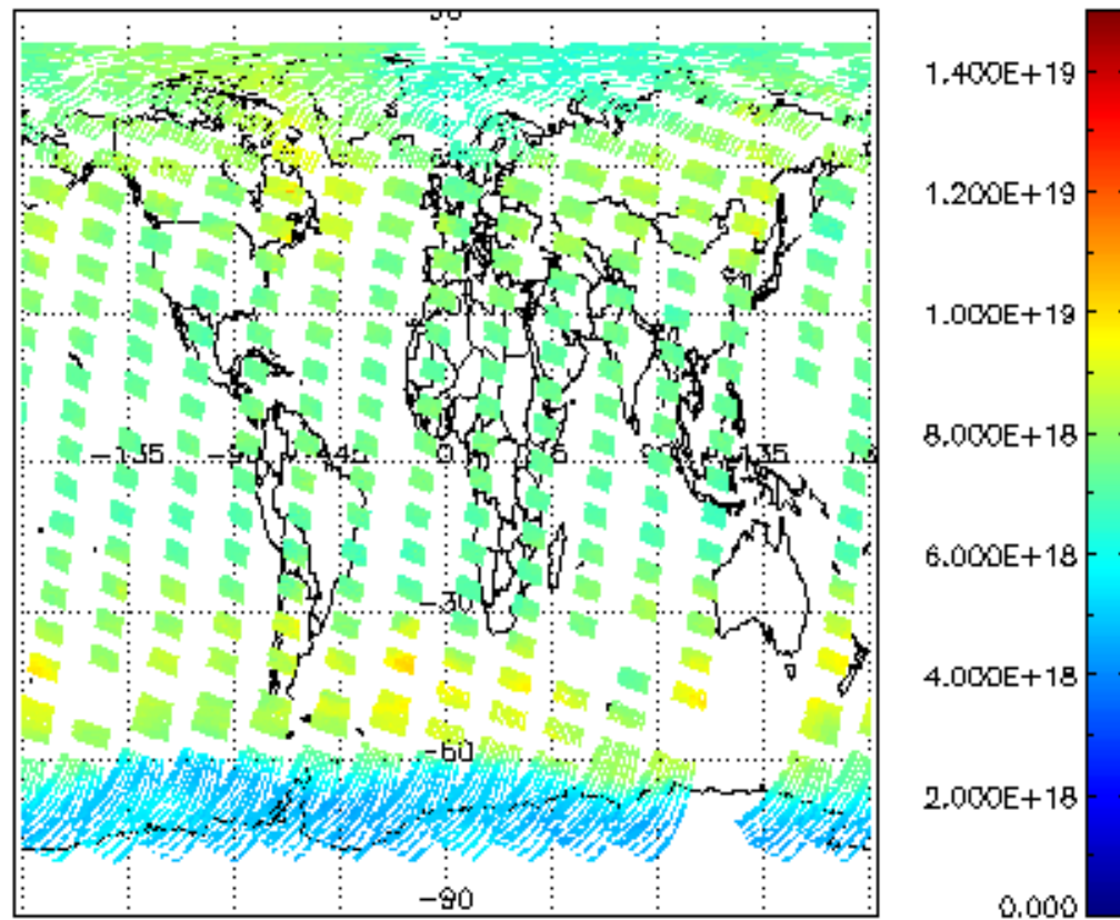
SCIOL2P_NADUV003_vcd for 12SEP2008 00:00:00 to 13SEP2008 00:00:00
