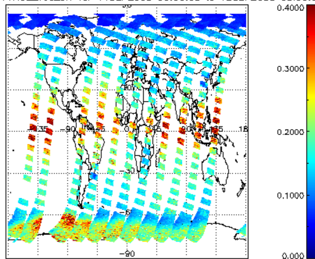
iCIOL2P_NADUV1NO2_vcd_err for 11SEP2008 00:00:00 to 12SEP2008 00:00:00
