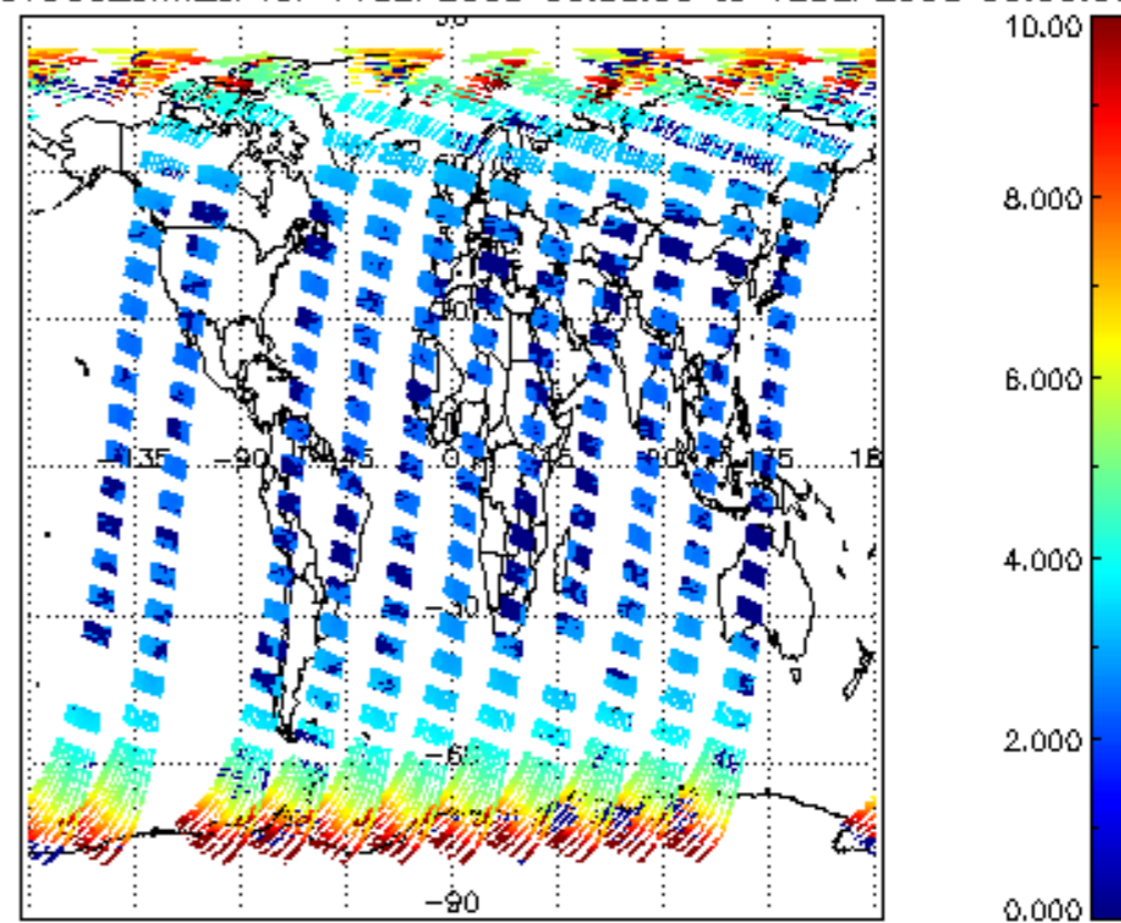
SCIOL2P_NADUV003_amf_cl for 11SEP2008 00:00:00 to 12SEP2008 00:00:00
