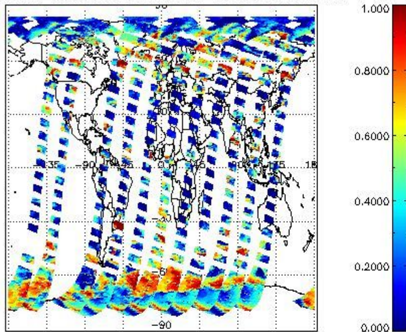
cLfrac for 11SEP2008 00:00:00 to 12SEP2008 00:00:00
