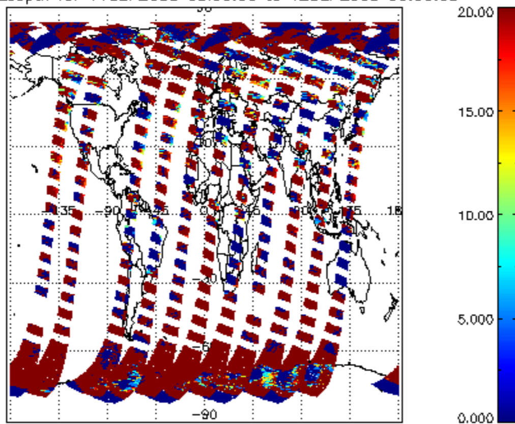
cl_opt_depth for 11SEP2008 00:00:00 to 12SEP2008 00:00:00
