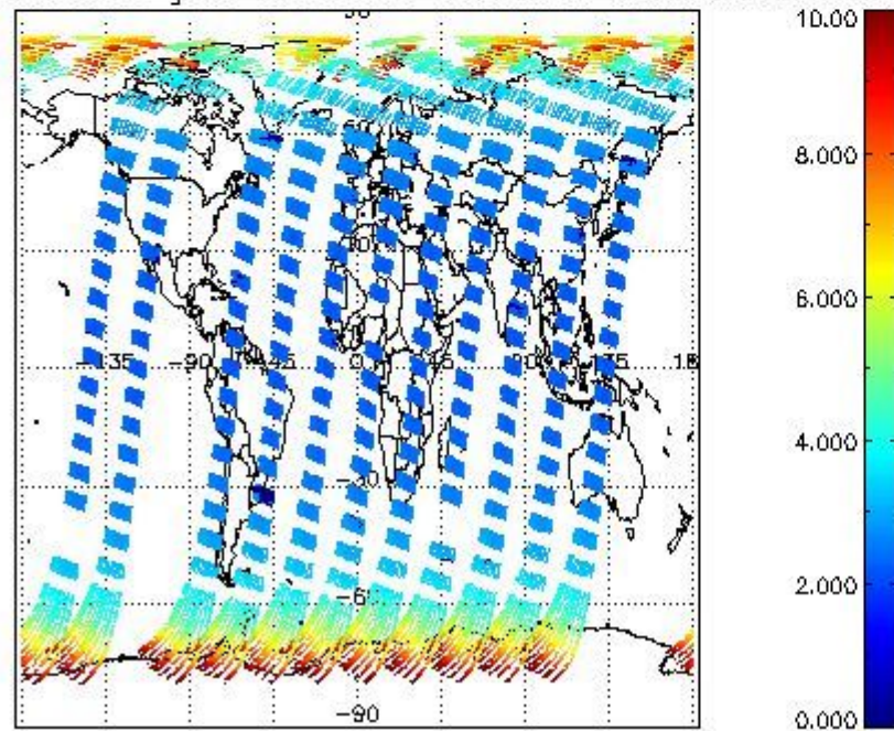
SCIOL2P_NADUV003_amf_gr for 11SEP2008 00:00:00 to 12SEP2008 00:00:00
