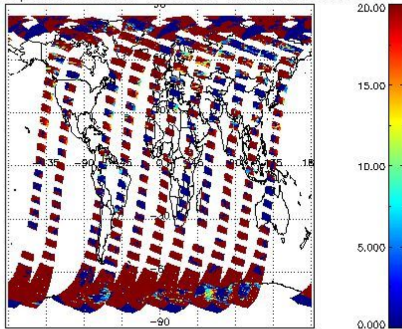
cLopt_depth for 11SEP2008 00:00:00 to 12SEP2008 00:00:00
