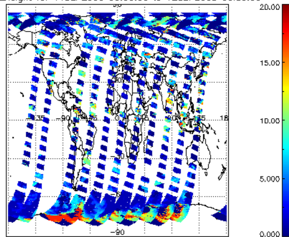
cl_top_height for 11SEP2008 00:00:00 to 12SEP2008 00:00:00
