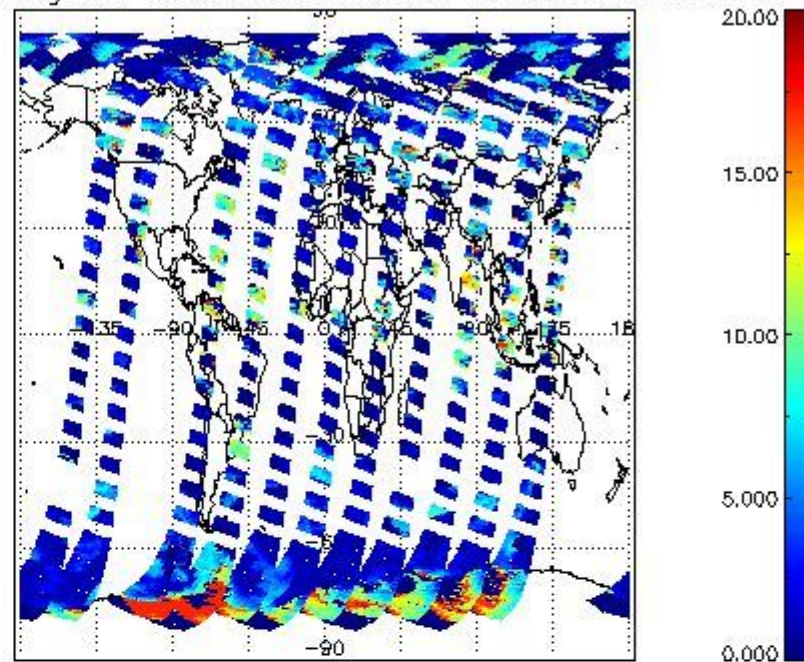
cL_top_height for 11SEP2008 00:00:00 to 12SEP2008 00:00:00
