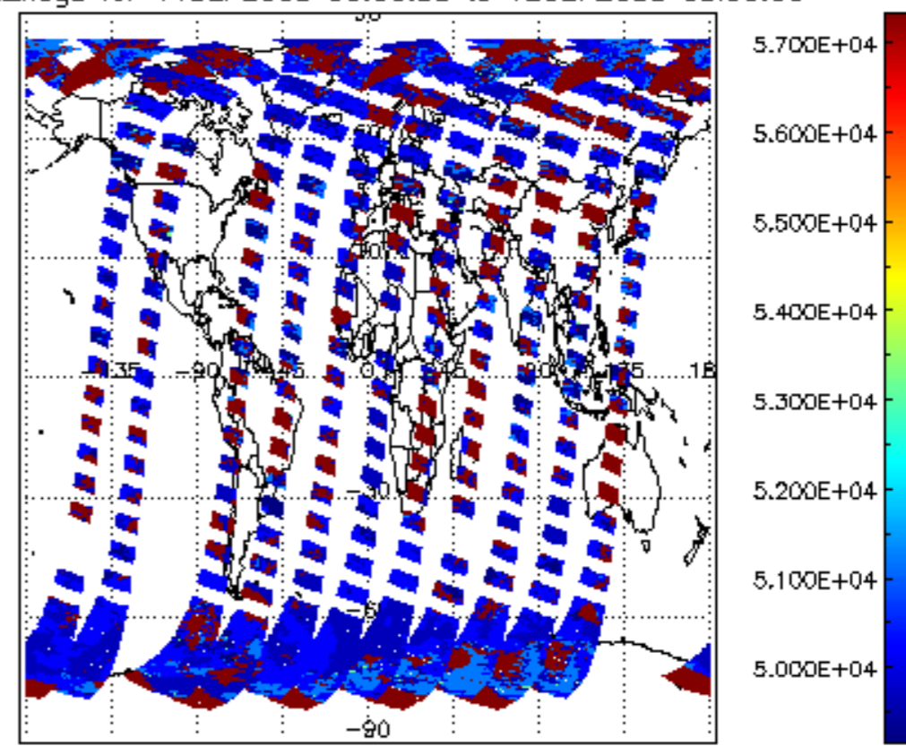
cloud_flags for 11SEP2008 00:00:00 to 12SEP2008 00:00:00
