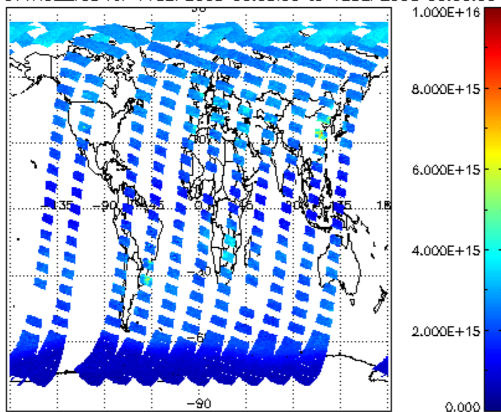
SCIOL2P_NADUV1NO2_vcd for 11SEP2008 00:00:00 to 12SEP2008 00:00:00
