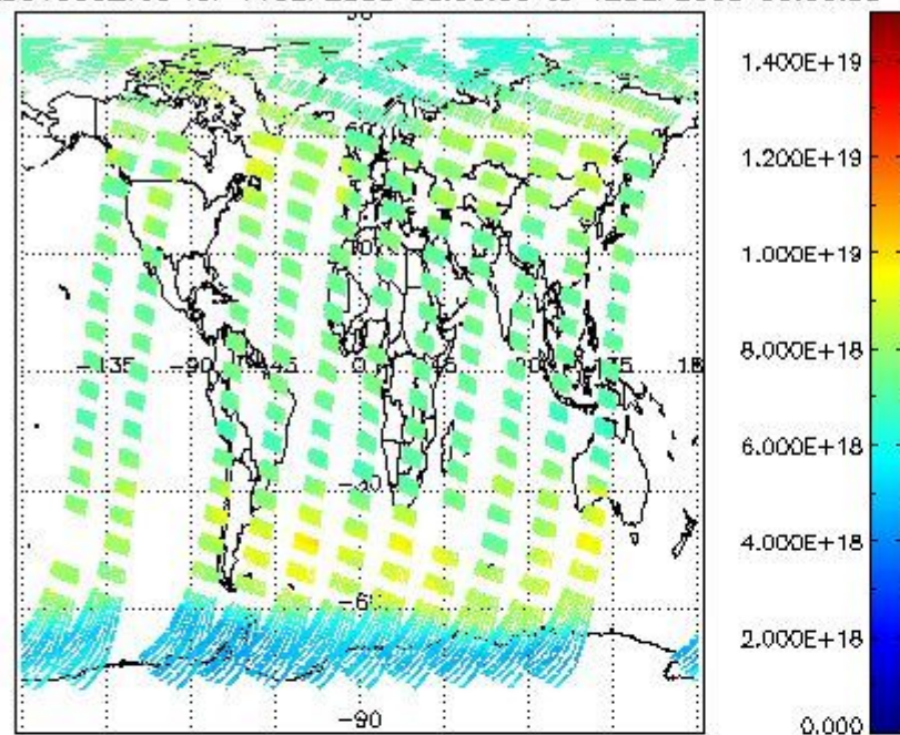
SCIOL2P_NADUV003_vcd for 11SEP2008 00:00:00 to 12SEP2008 00:00:00
