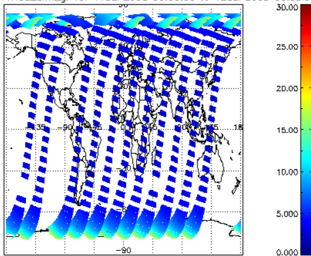
iCIOL2P_NADUV1NO2_amf_gr for 11SEP2008 00:00:00 to 12SEP2008 00:00:00
