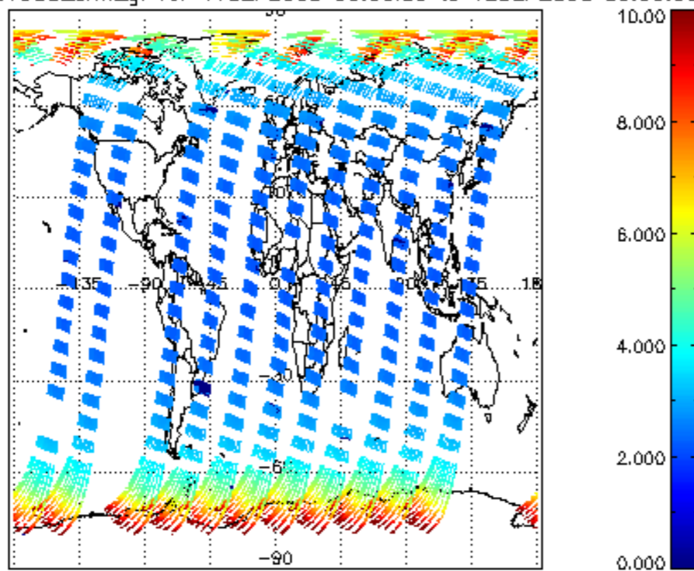
SCIOL2P_NADUV003_amf_gr for 11SEP2008 00:00:00 to 12SEP2008 00:00:00
