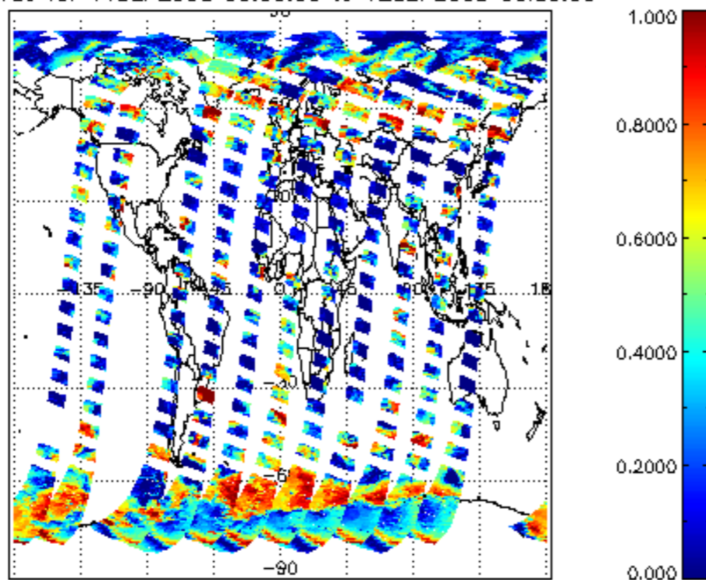
cl_frac for 11SEP2008 00:00:00 to 12SEP2008 00:00:00
