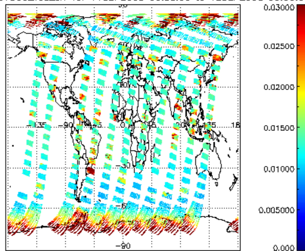
SCIOL2P_NADUV003_vcd_err for 11SEP2008 00:00:00 to 12SEP2008 00:00:00
