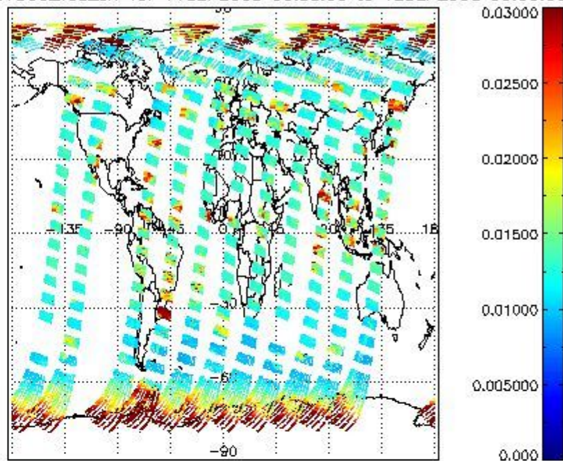
SCIOL2P_NADUV003_vcd_err for 11SEP2008 00:00:00 to 12SEP2008 00:00:00
