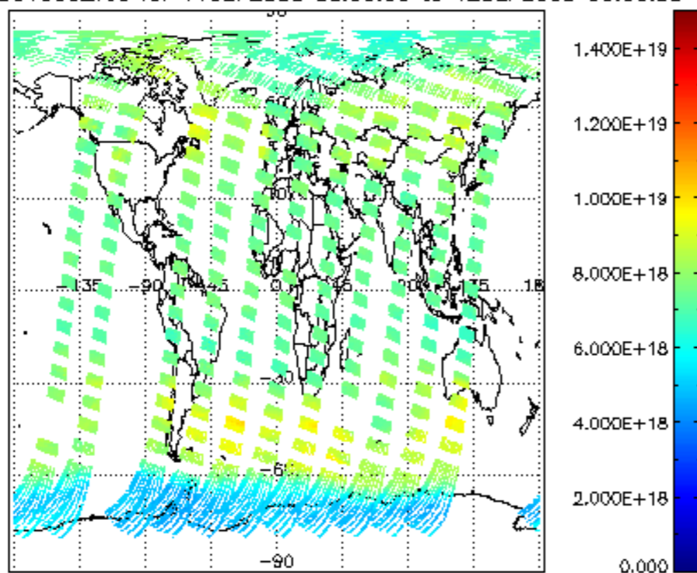
SCIOL2P_NADUV003_vcd for 11SEP2008 00:00:00 to 12SEP2008 00:00:00
