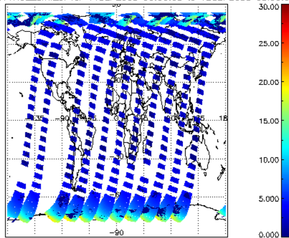
iCIOL2P_NADUV1NO2_amf_cl for 11SEP2008 00:00:00 to 12SEP2008 00:00:00
