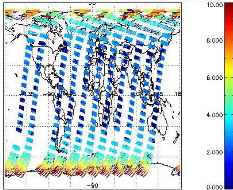
SCIOL2P_NADUV003_amf_cl for 11SEP2008 00:00:00 to 12SEP2008 00:00:00
