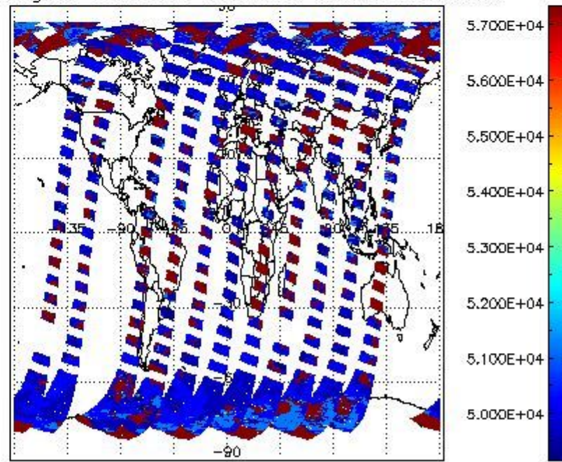
cloud_flags for 11SEP2008 00:00:00 to 12SEP2008 00:00:00
