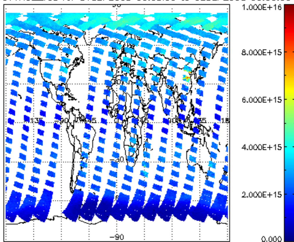
SCIOL2P_NADUV1NO2_vcd for 01SEP2008 00:00:00 to 02SEP2008 00:00:00
