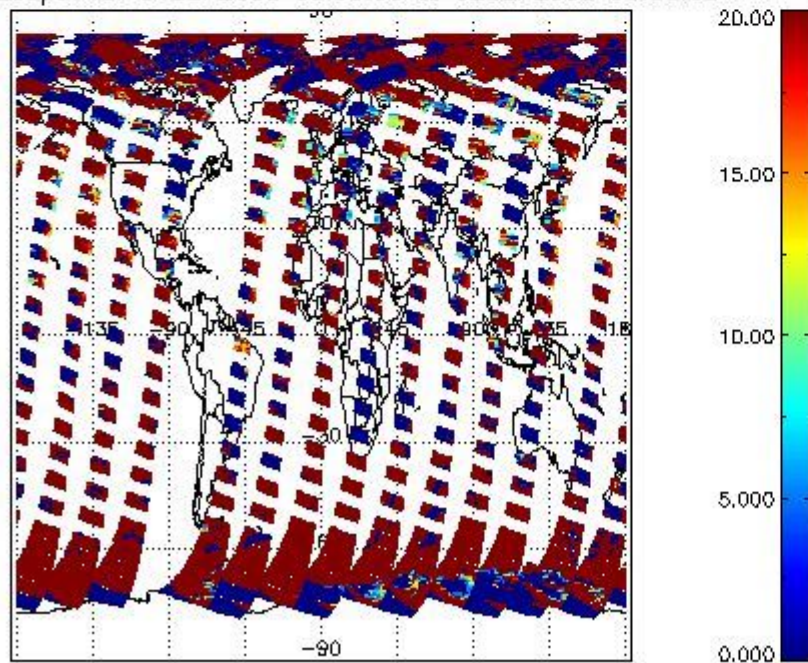
cL_opt_depth for 01SEP2008 00:00:00 to 02SEP2008 00:00:00
