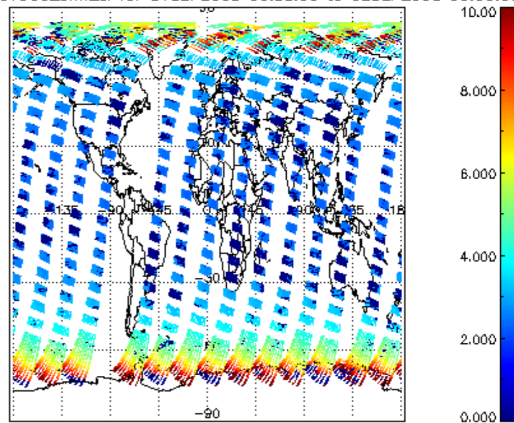
SCIOL2P_NADUV003_amf_cl for 01SEP2008 00:00:00 to 02SEP2008 00:00:00
