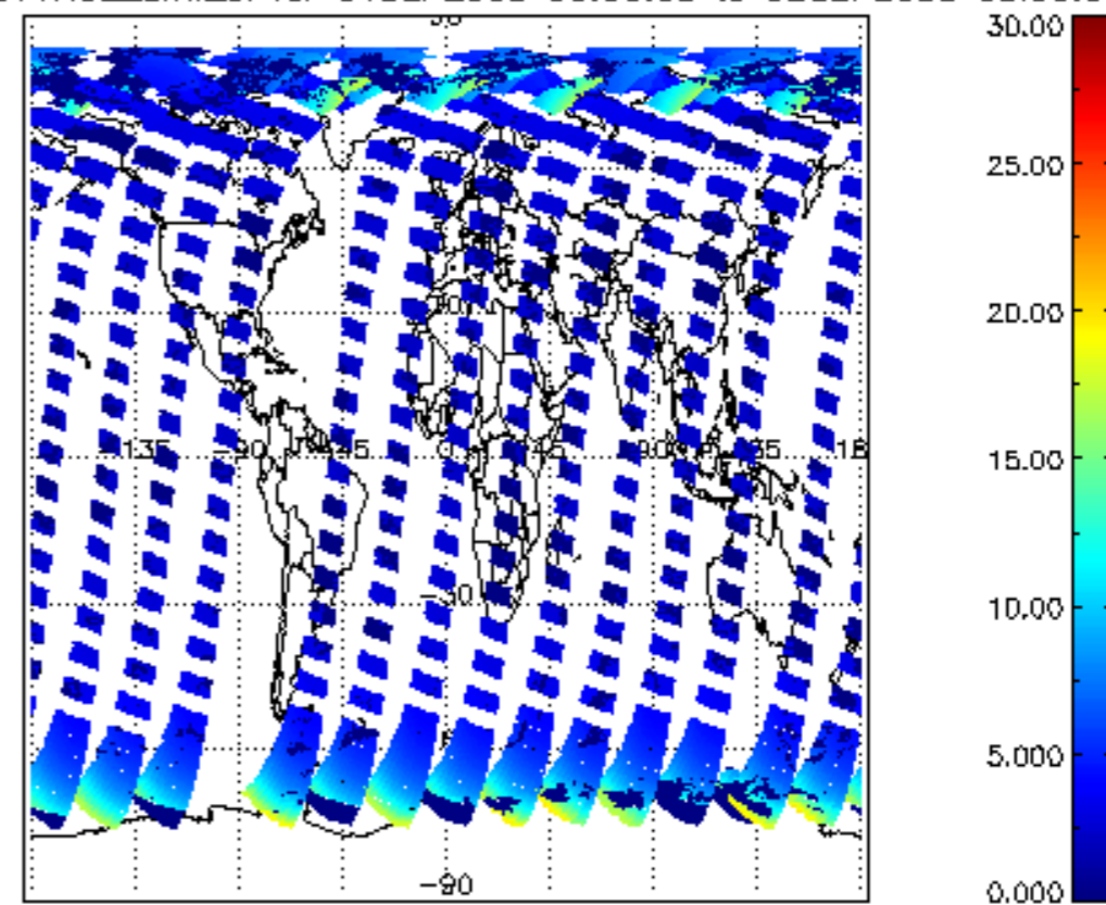
iCIOL2P_NADUV1NO2_amf_cl for 01SEP2008 00:00:00 to 02SEP2008 00:00:00
