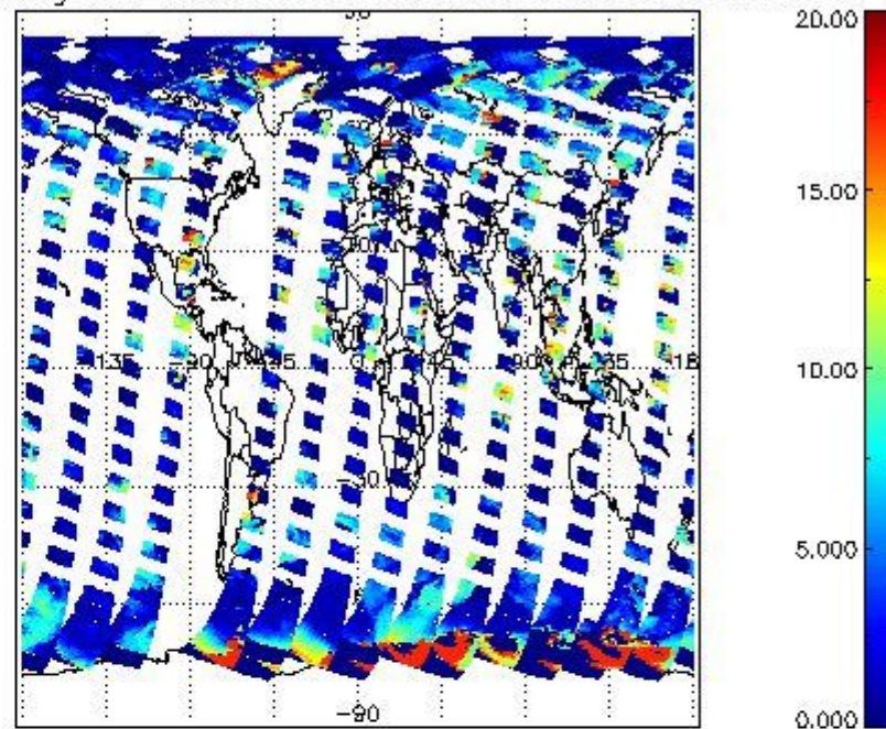
cL_top_height for 01SEP2008 00:00:00 to 02SEP2008 00:00:00
