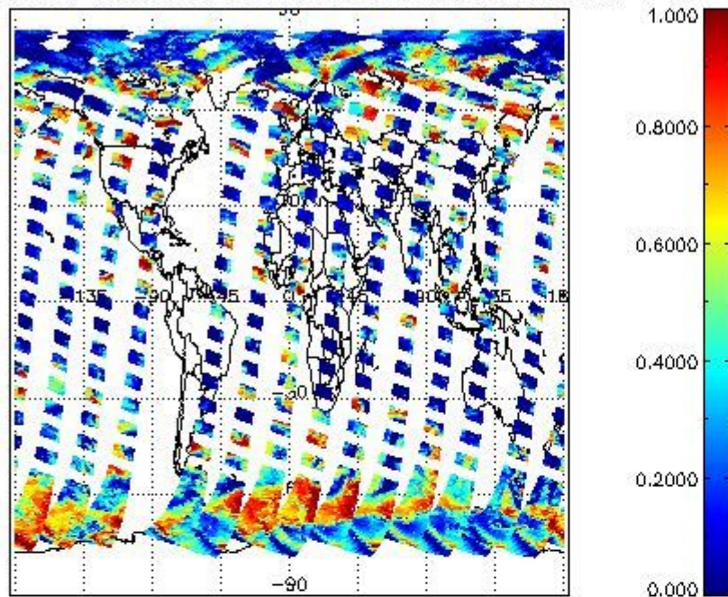
cL_frac for 01SEP2008 00:00:00 to 02SEP2008 00:00:00
