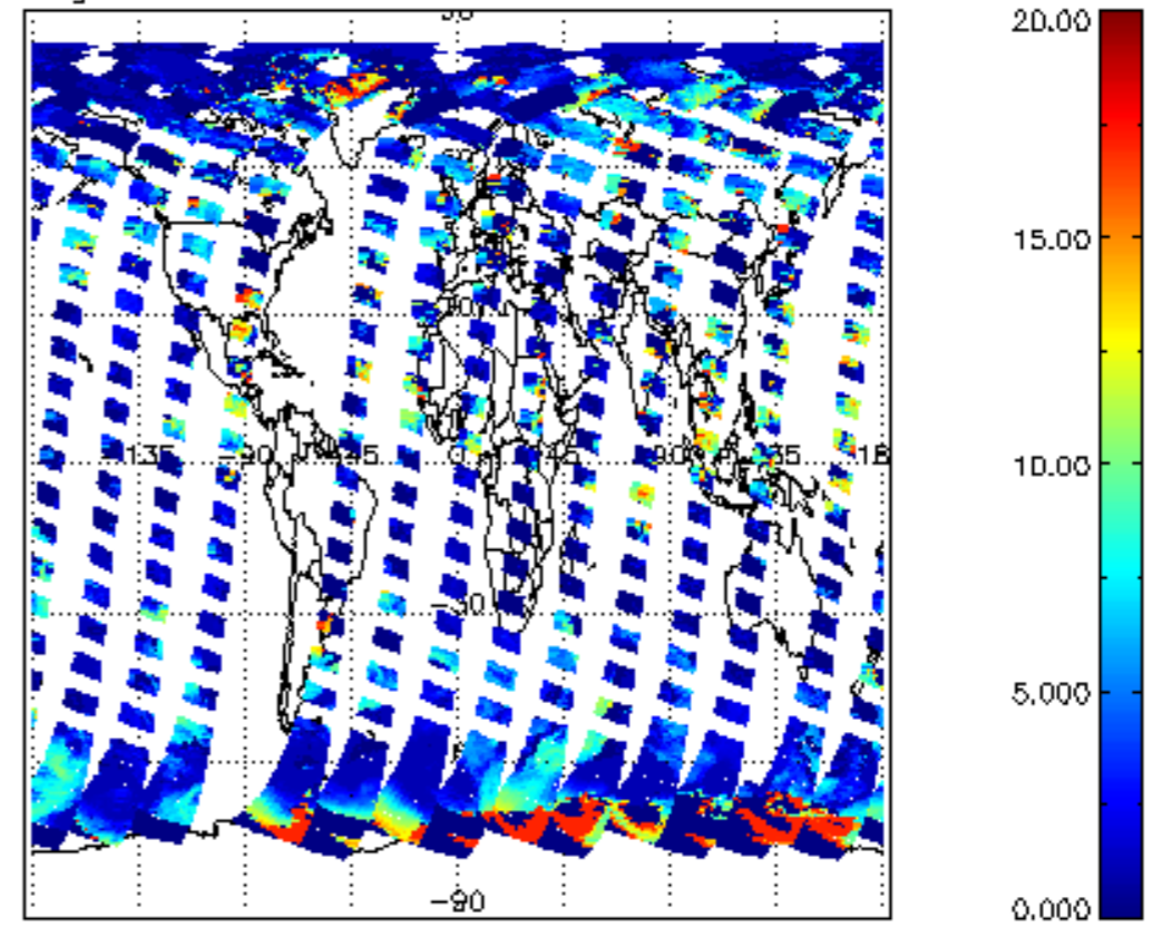
cl_top_height for 01SEP2008 00:00:00 to 02SEP2008 00:00:00
