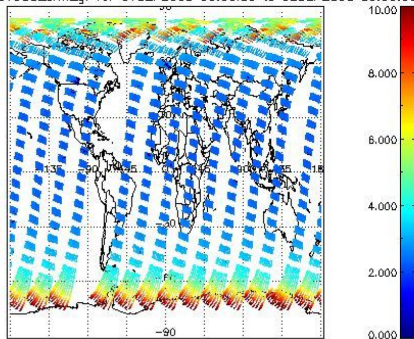
SCIOL2P_NADUV003_amf_gr for 01SEP2008 00:00:00 to 02SEP2008 00:00:00
