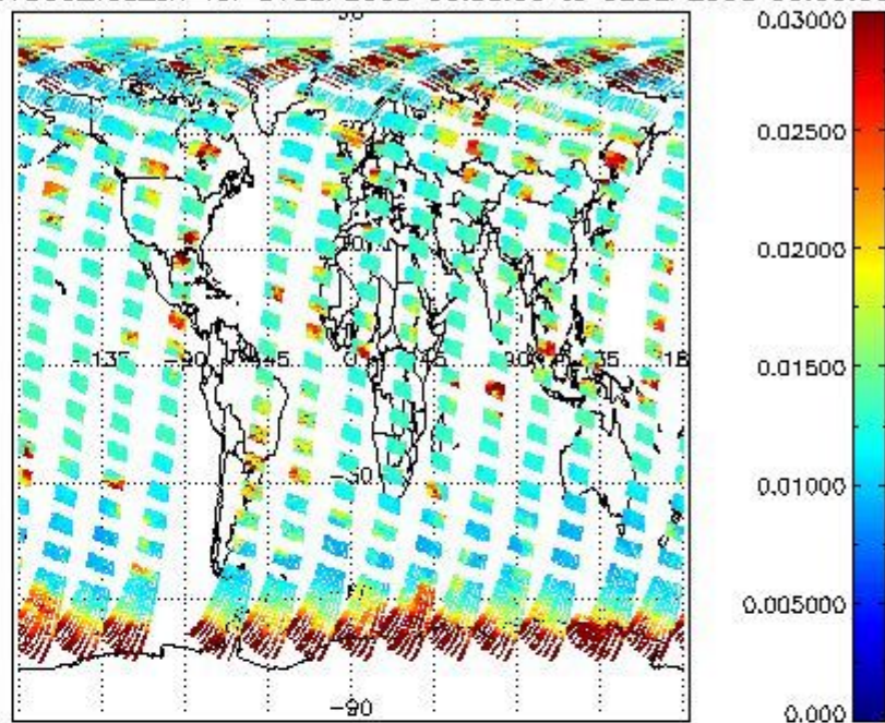
SCIOL2P_NADUV003_vcd_err for 01SEP2008 00:00:00 to 02SEP2008 00:00:00
