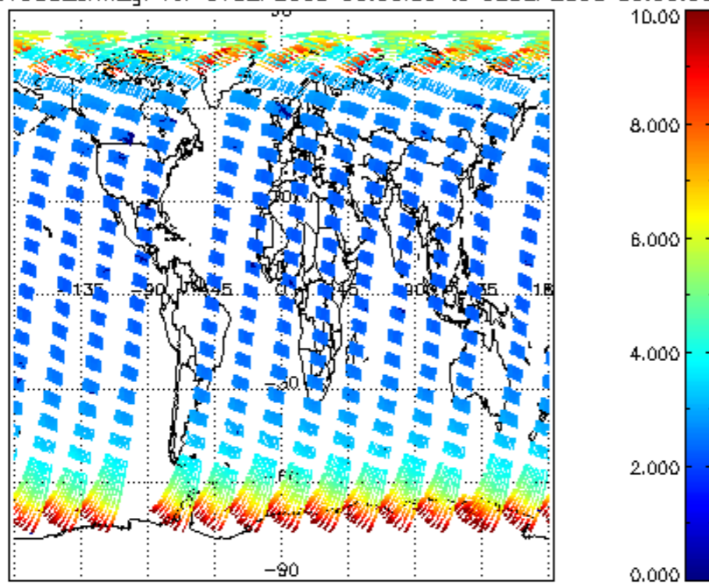
SCIOL2P_NADUV003_amf_gr for 01SEP2008 00:00:00 to 02SEP2008 00:00:00
