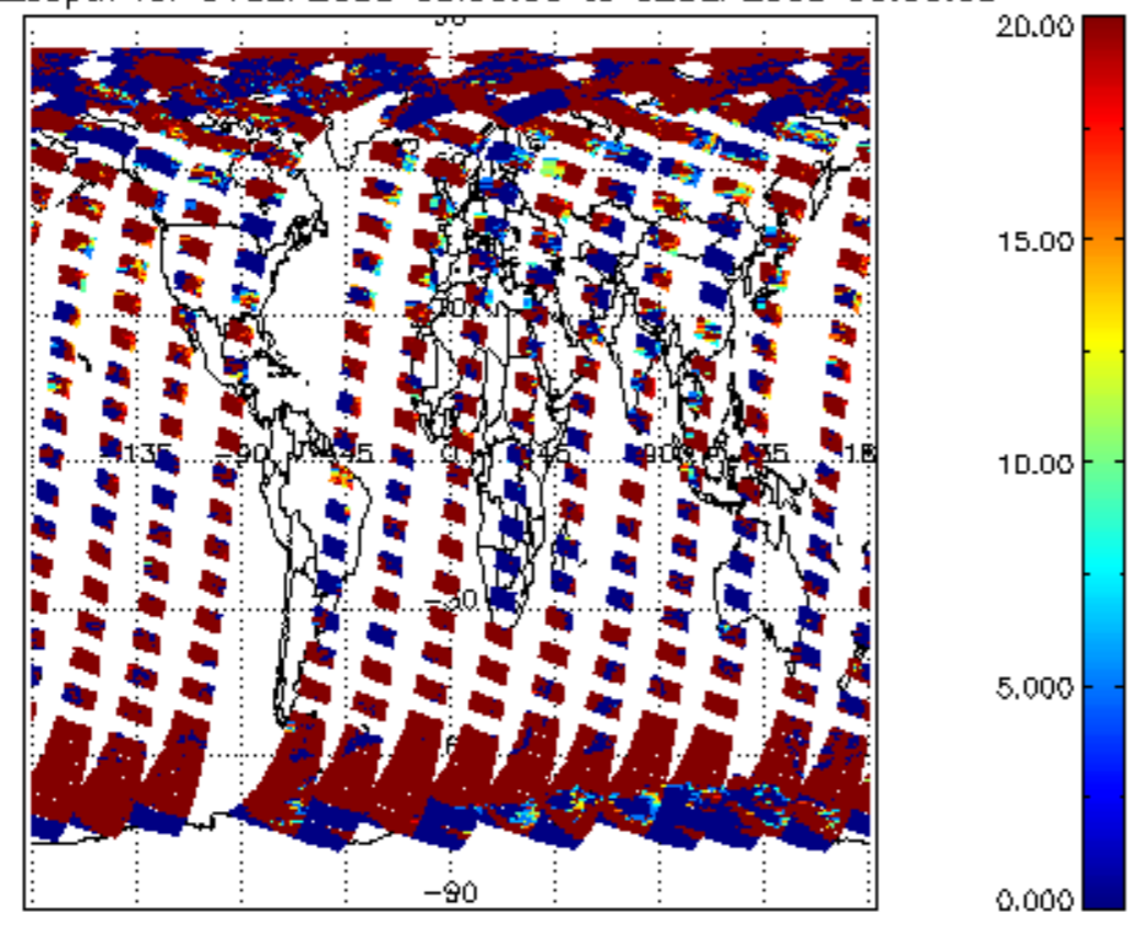
cl_opt_depth for 01SEP2008 00:00:00 to 02SEP2008 00:00:00
