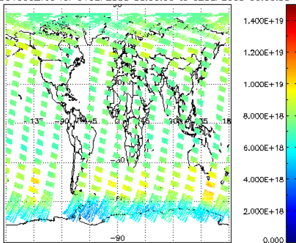
SCIOL2P_NADUV003_vcd for 01SEP2008 00:00:00 to 02SEP2008 00:00:00
