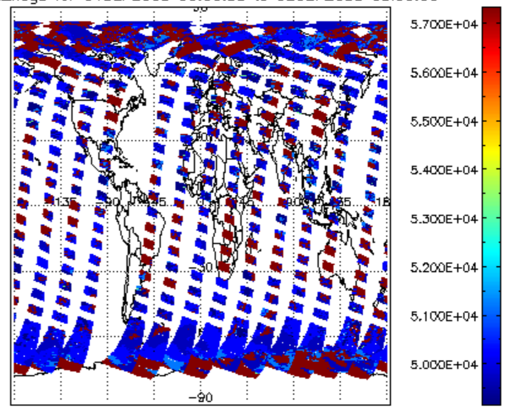
cloud_flags for 01SEP2008 00:00:00 to 02SEP2008 00:00:00
