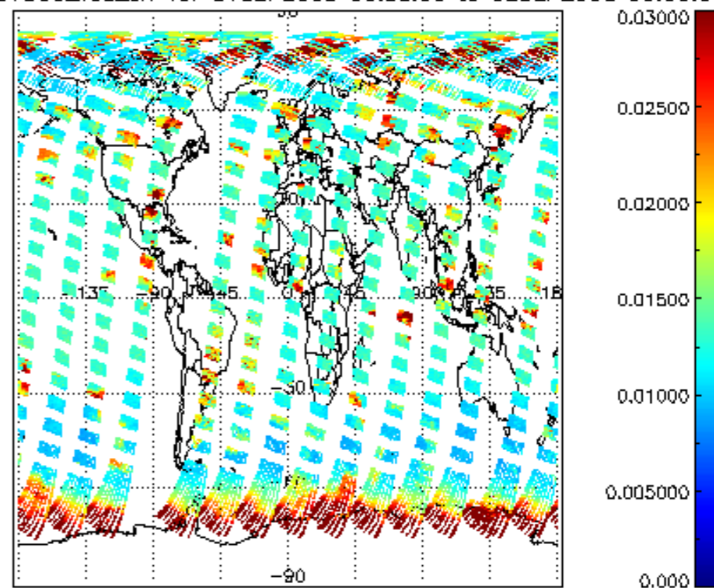
SCIOL2P_NADUV003_vcd_err for 01SEP2008 00:00:00 to 02SEP2008 00:00:00
