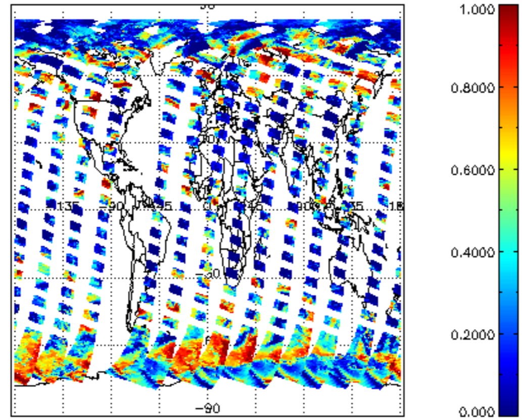
cl_frac for 01SEP2008 00:00:00 to 02SEP2008 00:00:00
