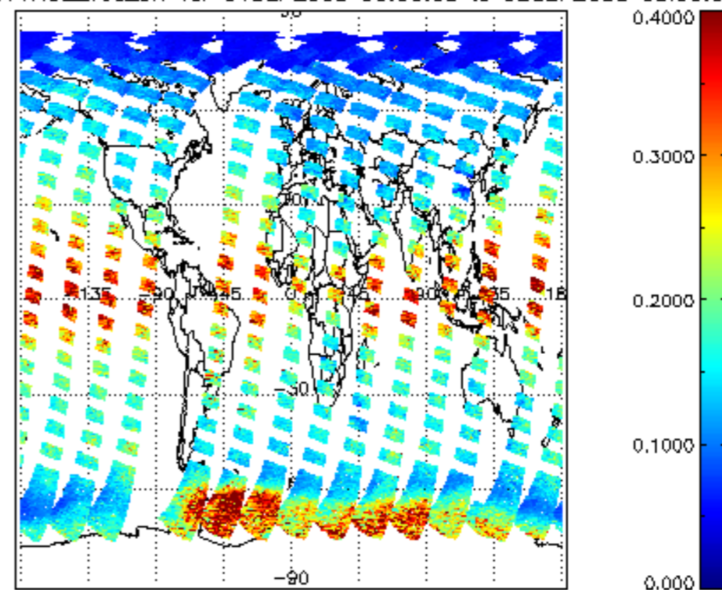
iCIOL2P_NADUV1NO2_vcd_err for 01SEP2008 00:00:00 to 02SEP2008 00:00:00
