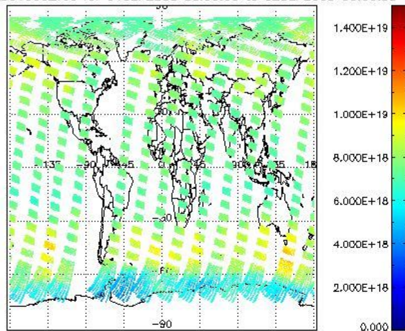
SCIOL2P_NADUV003_vcd for 01SEP2008 00:00:00 to 02SEP2008 00:00:00
