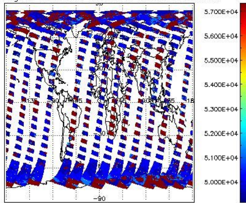
cloud_flags for 01SEP2008 00:00:00 to 02SEP2008 00:00:00
