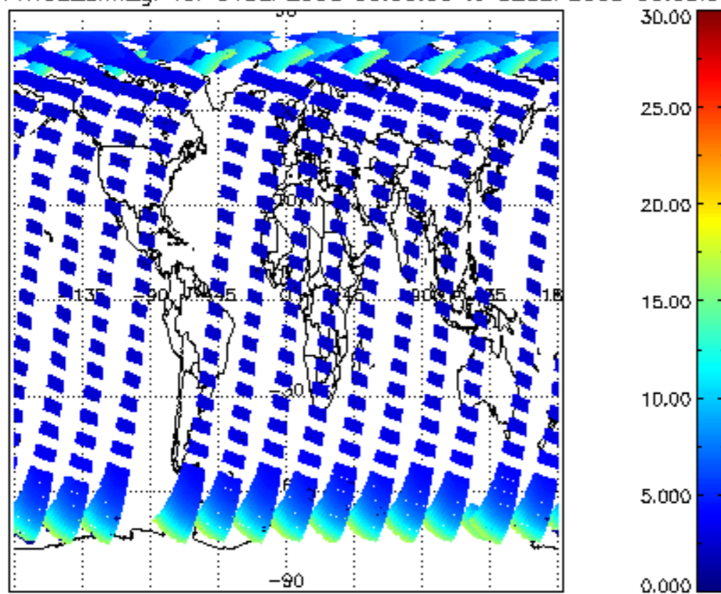
iCIOL2P_NADUV1NO2_amf_gr for 01SEP2008 00:00:00 to 02SEP2008 00:00:00
