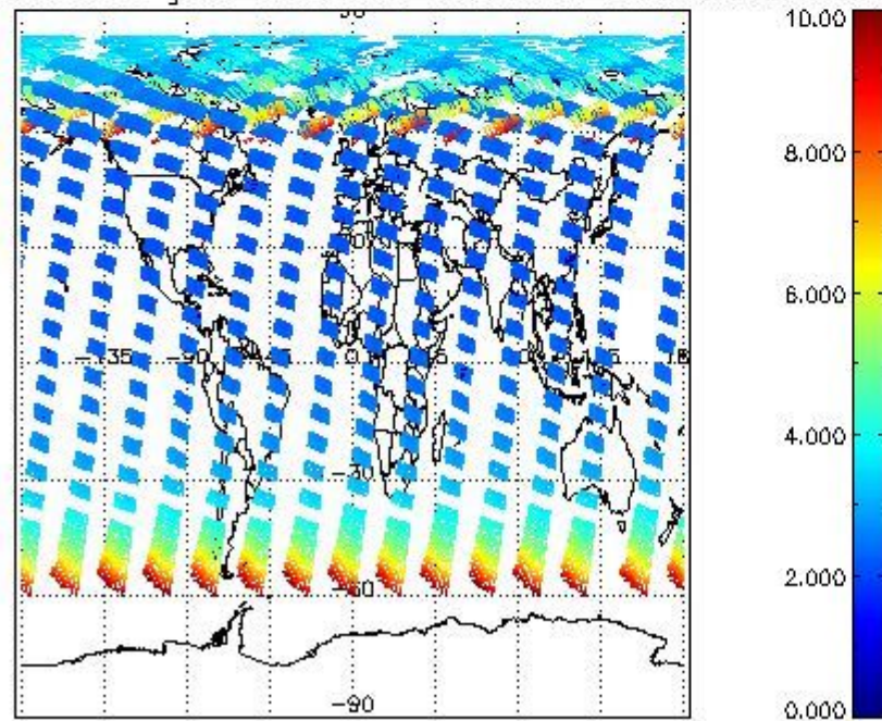
SCIOL2P_NADUV003_amf_gr for 27JUN2008 00:00:00 to 28JUN2008 00:00:00
