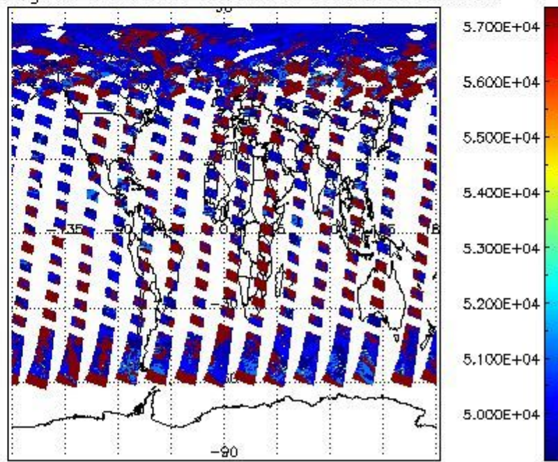
cloud_flags for 27JUN2008 00:00:00 to 28JUN2008 00:00:00
