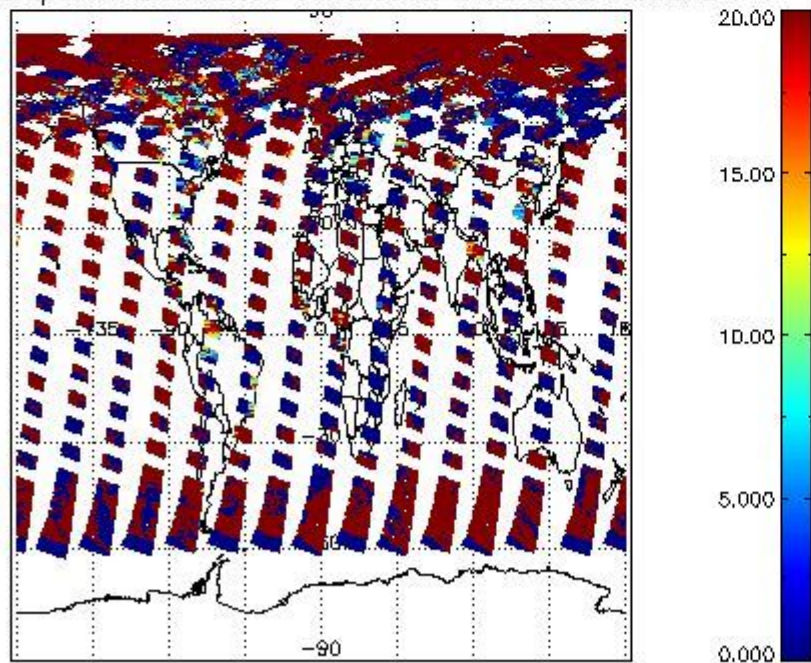
cL_opt_depth for 27JUN2008 00:00:00 to 28JUN2008 00:00:00
