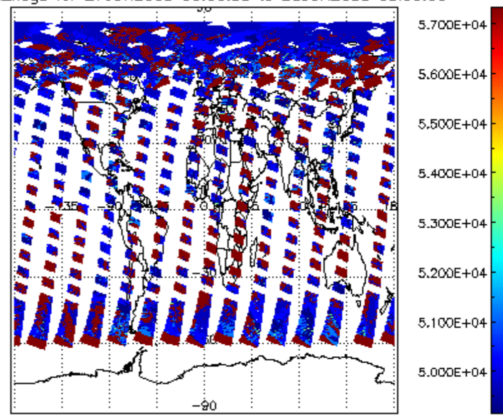
cloud_flags for 27JUN2008 00:00:00 to 28JUN2008 00:00:00
