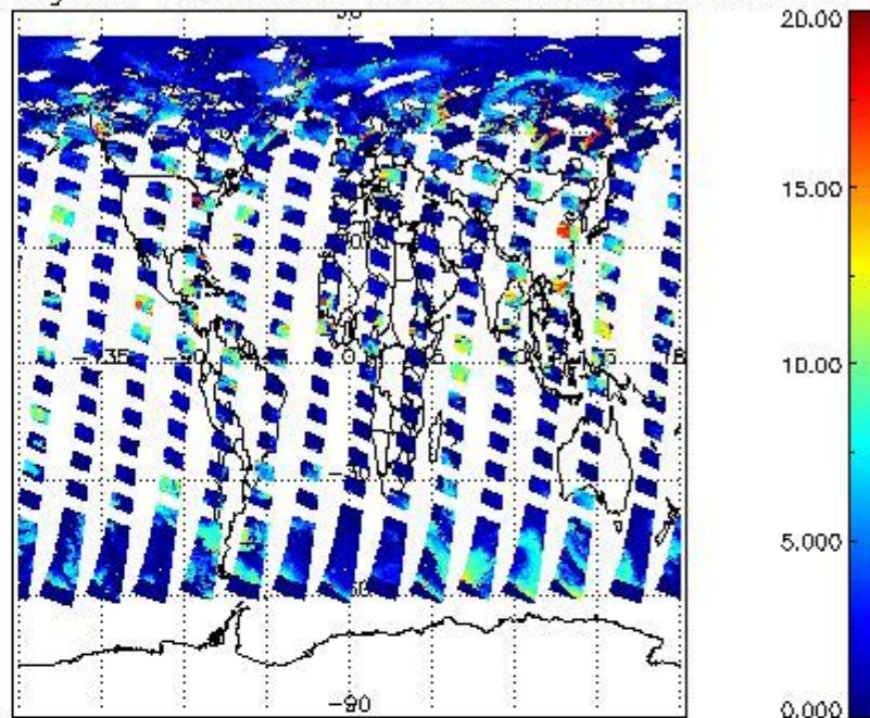
cL_top_height for 27JUN2008 00:00:00 to 28JUN2008 00:00:00
