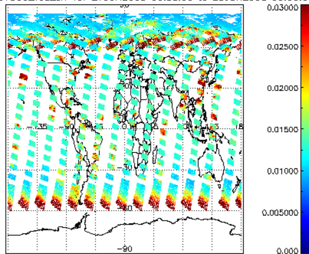
SCIOL2P_NADUV003_vcd_err for 27JUN2008 00:00:00 to 28JUN2008 00:00:00
