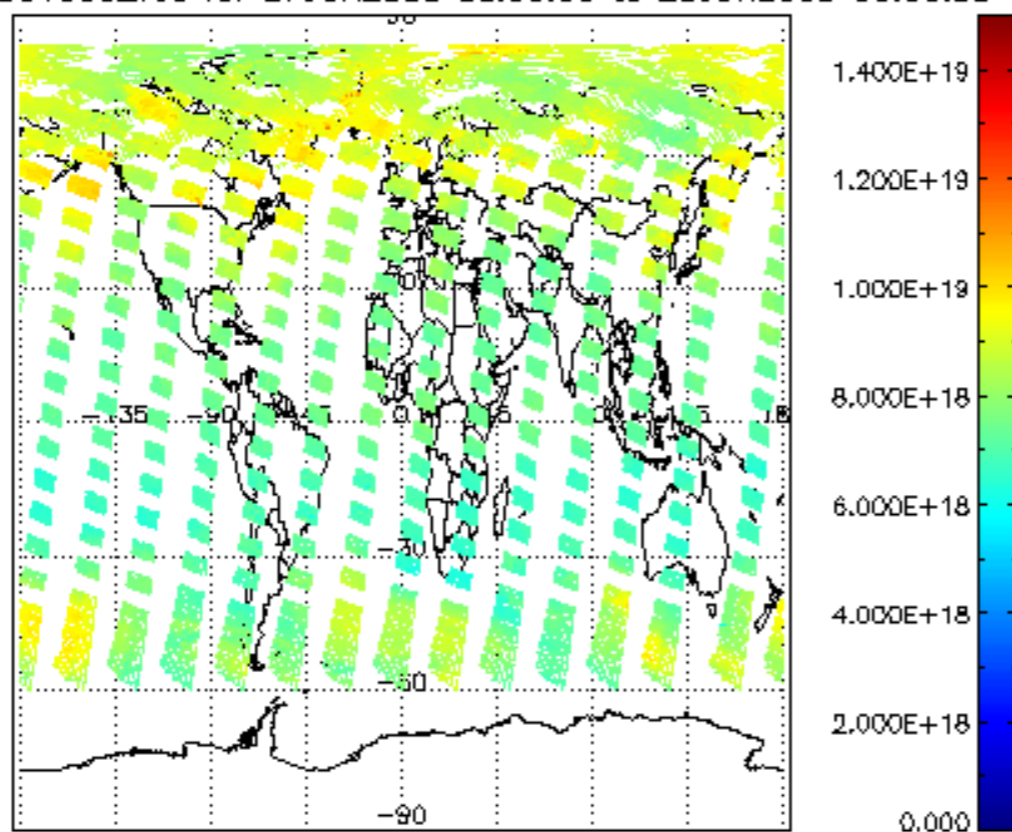
SCIOL2P_NADUV003_vcd for 27JUN2008 00:00:00 to 28JUN2008 00:00:00
