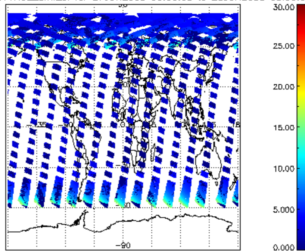
iCIOL2P_NADUV1NO2_amf_cl for 27JUN2008 00:00:00 to 28JUN2008 00:00:00
