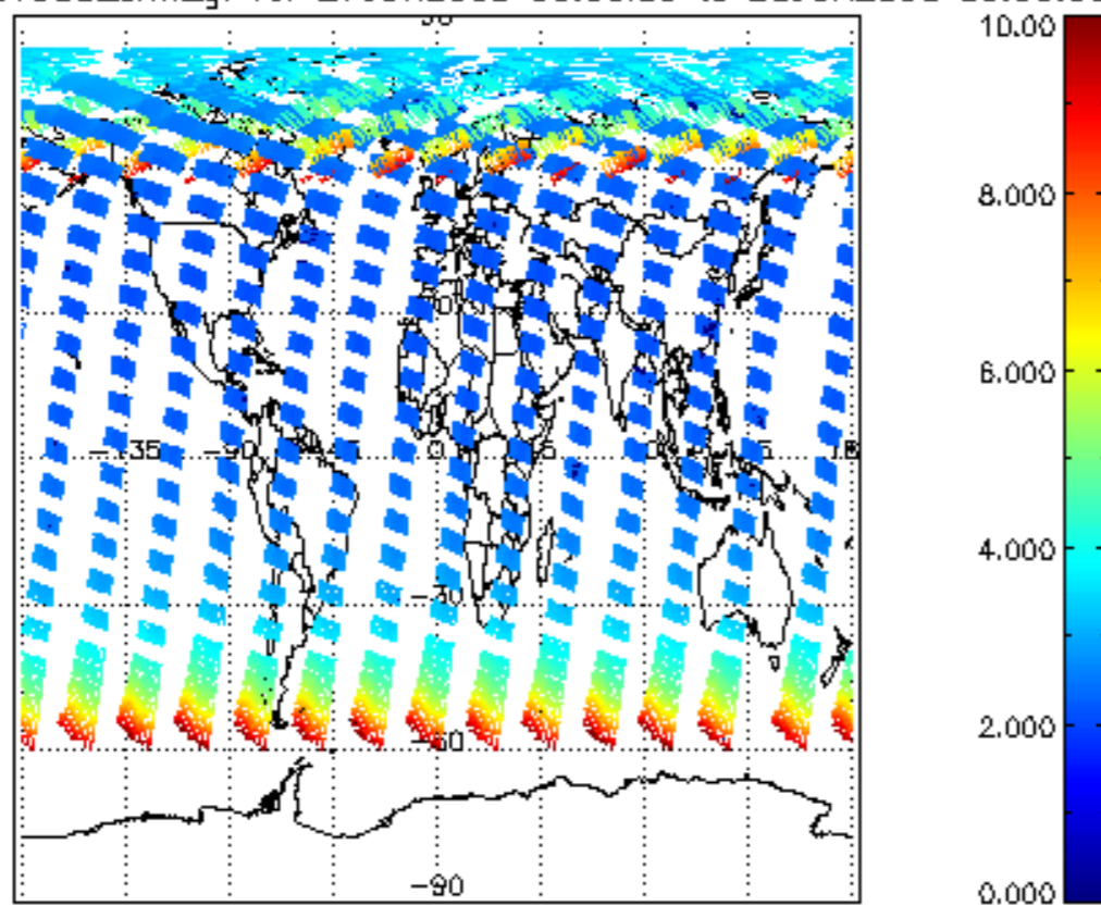
SCIOL2P_NADUV003_amf_gr for 27JUN2008 00:00:00 to 28JUN2008 00:00:00
