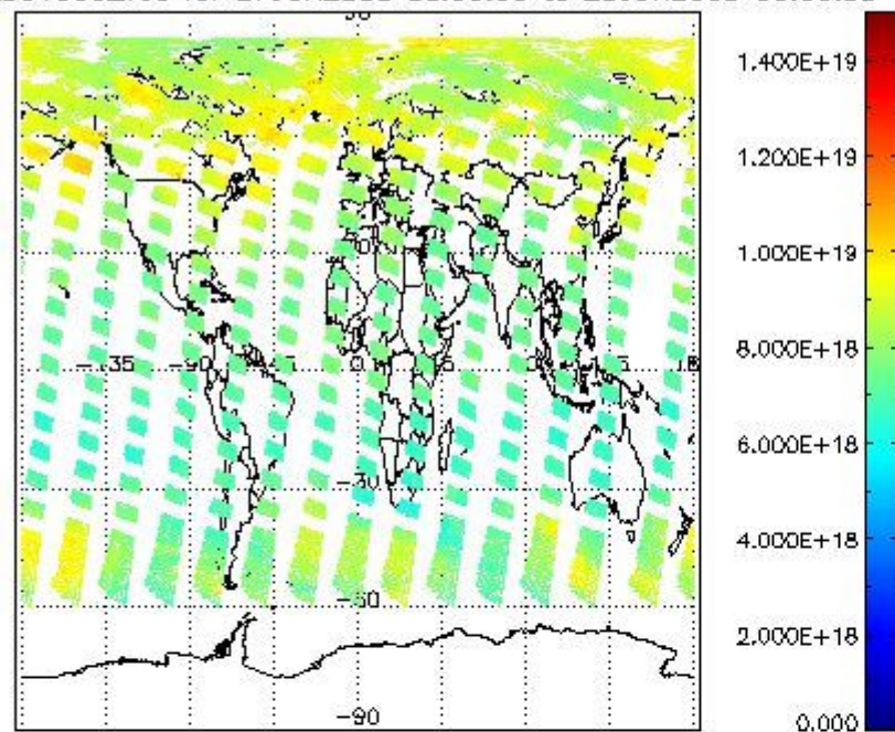
SCIOL2P_NADUV003_vcd for 27JUN2008 00:00:00 to 28JUN2008 00:00:00
