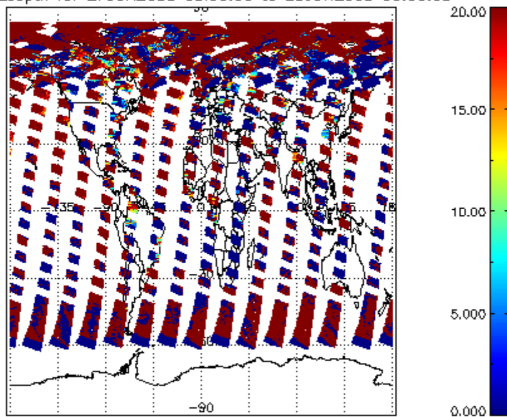
cl_opt_depth for 27JUN2008 00:00:00 to 28JUN2008 00:00:00
