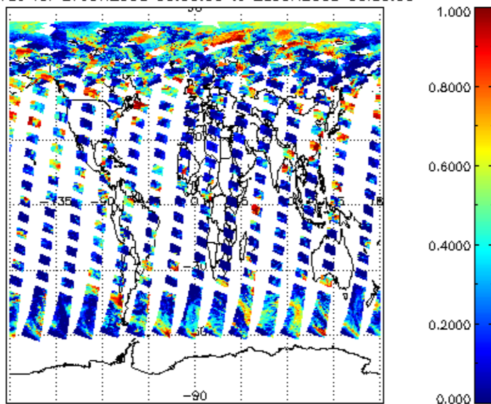
cl_frac for 27JUN2008 00:00:00 to 28JUN2008 00:00:00
