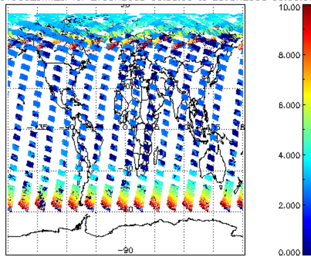
SCIOL2P_NADUV003_amf_cl for 27JUN2008 00:00:00 to 28JUN2008 00:00:00
