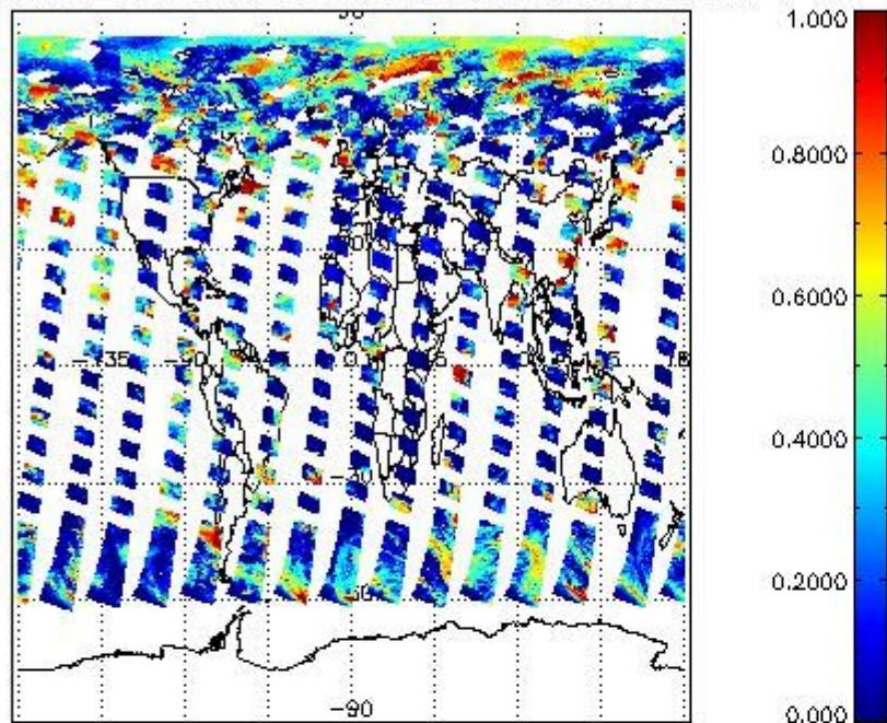
cL_frac for 27JUN2008 00:00:00 to 28JUN2008 00:00:00
