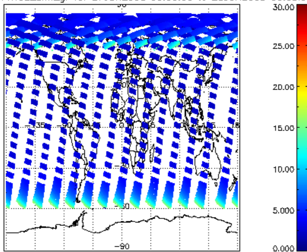
iCIOL2P_NADUV1NO2_amf_gr for 27JUN2008 00:00:00 to 28JUN2008 00:00:00
