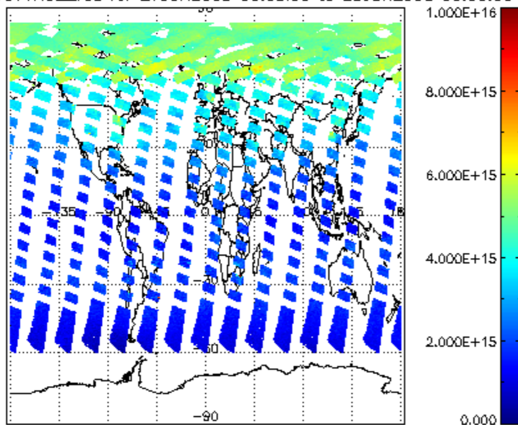
SCIOL2P_NADUV1NO2_vcd for 27JUN2008 00:00:00 to 28JUN2008 00:00:00
