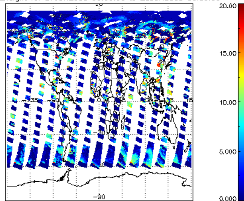
cl_top_height for 27JUN2008 00:00:00 to 28JUN2008 00:00:00
