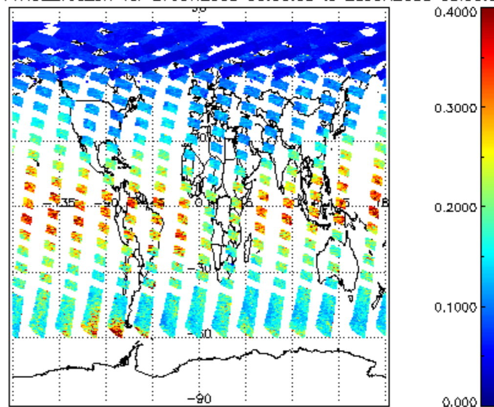
iCIOL2P_NADUV1NO2_vcd_err for 27JUN2008 00:00:00 to 28JUN2008 00:00:00
