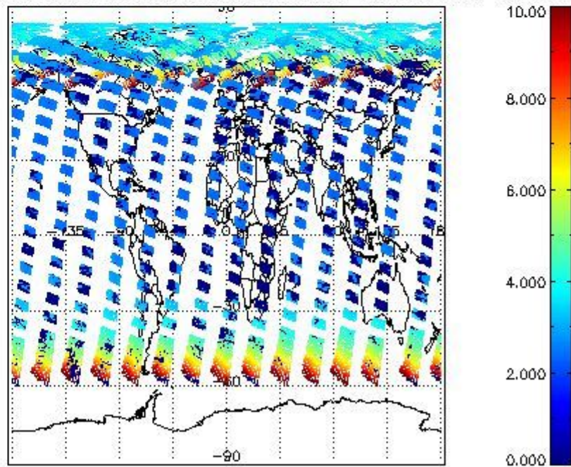
SCIOL2P_NADUV003_amf_cl for 27JUN2008 00:00:00 to 28JUN2008 00:00:00
