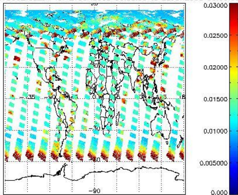
SCIOL2P_NADUV003_vcd_err for 27JUN2008 00:00:00 to 28JUN2008 00:00:00
