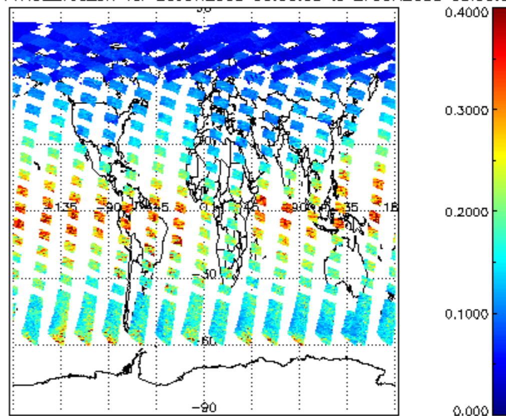
iCIOL2P_NADUV1NO2_vcd_err for 26JUN2008 00:00:00 to 27JUN2008 00:00:00
