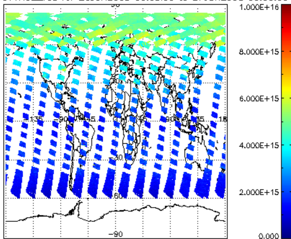
SCIOL2P_NADUV1NO2_vcd for 26JUN2008 00:00:00 to 27JUN2008 00:00:00
