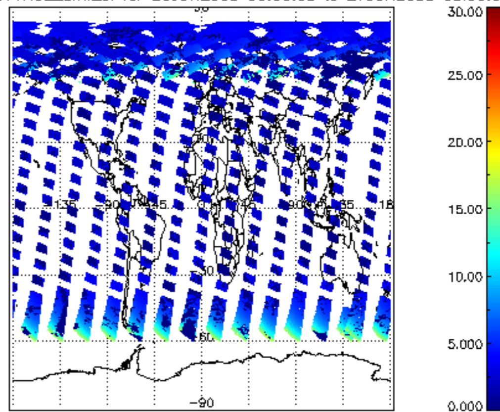
iCIOL2P_NADUV1NO2_amf_cl for 26JUN2008 00:00:00 to 27JUN2008 00:00:00
