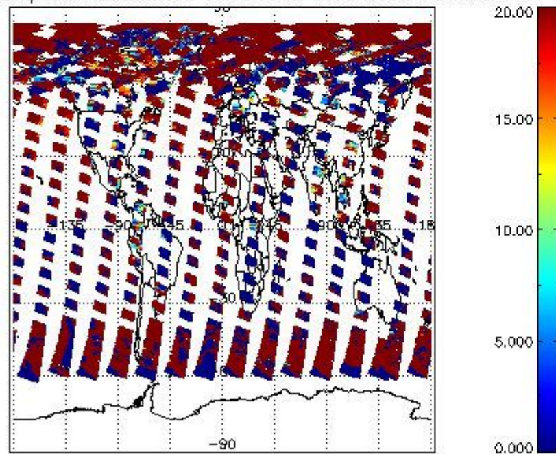
cL_opt_depth for 26JUN2008 00:00:00 to 27JUN2008 00:00:00
