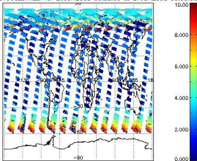
SCIOL2P_NADUV003_amf_cl for 26JUN2008 00:00:00 to 27JUN2008 00:00:00
