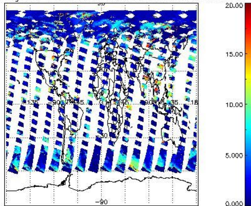
cL_top_height for 26JUN2008 00:00:00 to 27JUN2008 00:00:00
