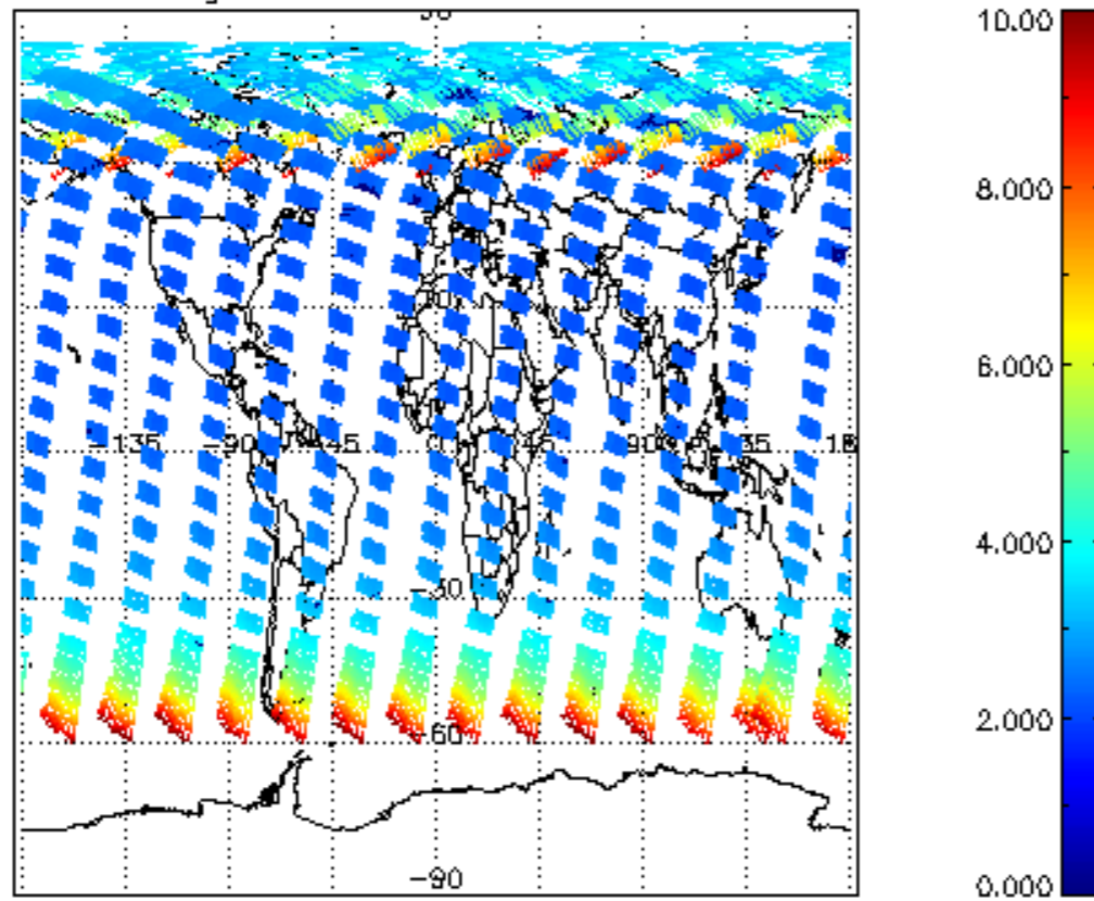
SCIOL2P_NADUV003_amf_gr for 26JUN2008 00:00:00 to 27JUN2008 00:00:00
