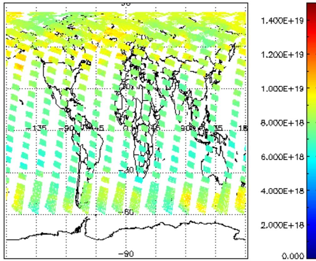
SCIOL2P_NADUV003_vcd for 26JUN2008 00:00:00 to 27JUN2008 00:00:00
