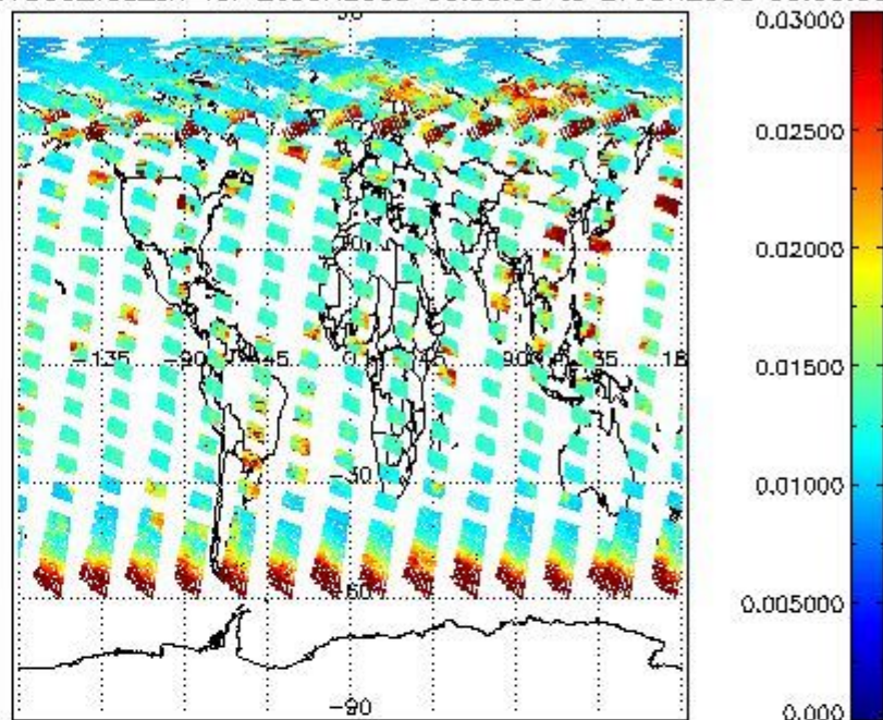
SCIOL2P_NADUV003_vcd_err for 26JUN2008 00:00:00 to 27JUN2008 00:00:00
