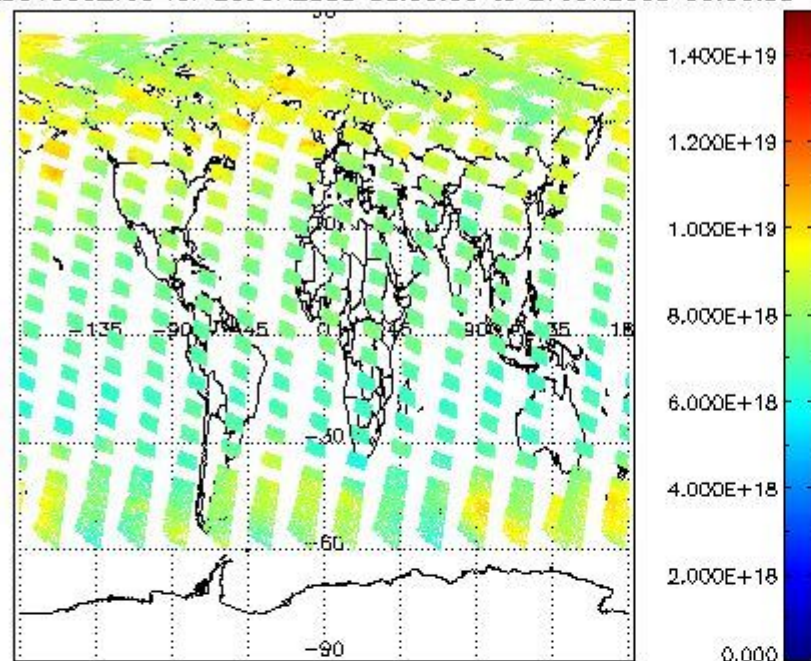
SCIOL2P_NADUV003_vcd for 26JUN2008 00:00:00 to 27JUN2008 00:00:00
