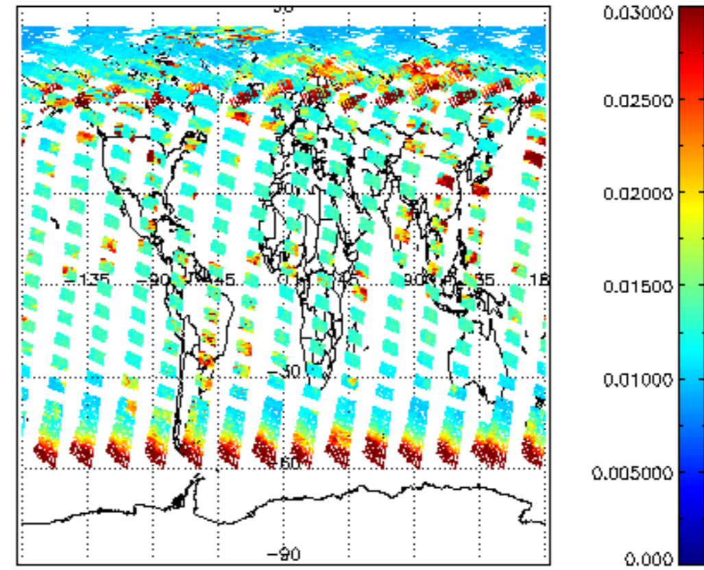
SCIOL2P_NADUV003_vcd_err for 26JUN2008 00:00:00 to 27JUN2008 00:00:00
