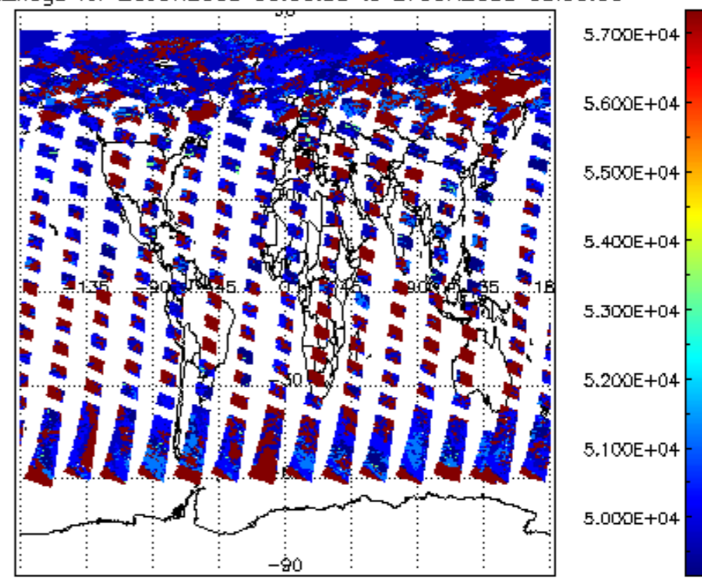
cloud_flags for 26JUN2008 00:00:00 to 27JUN2008 00:00:00
