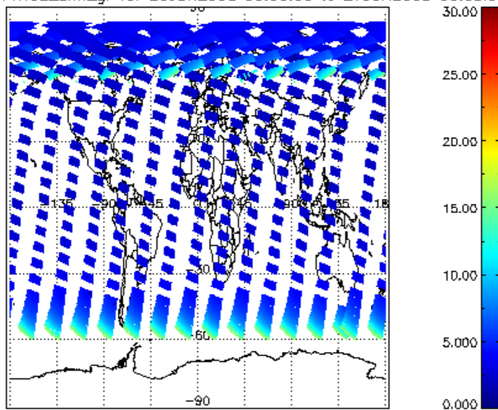
iCIOL2P_NADUV1NO2_amf_gr for 26JUN2008 00:00:00 to 27JUN2008 00:00:00
