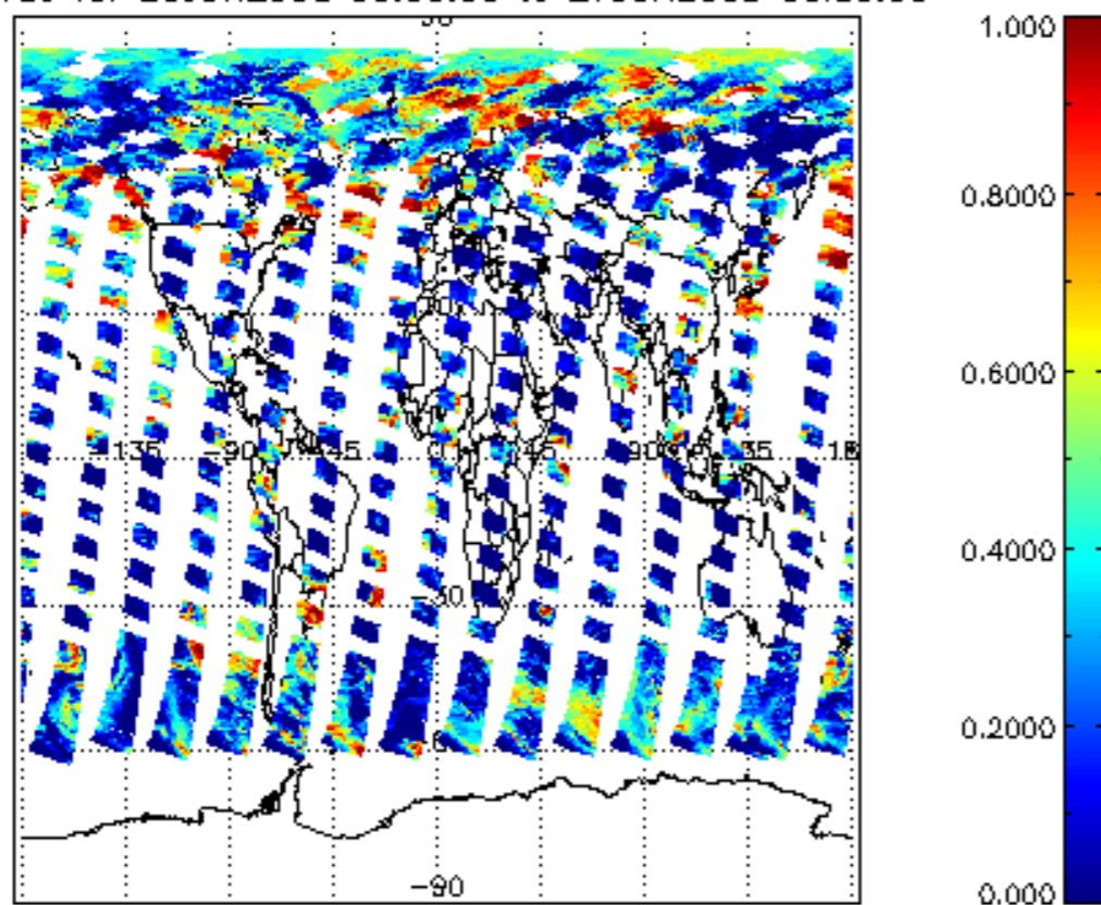
cl_frac for 26JUN2008 00:00:00 to 27JUN2008 00:00:00
