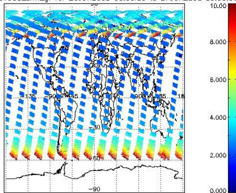
SCIOL2P_NADUV003_amf_gr for 26JUN2008 00:00:00 to 27JUN2008 00:00:00
