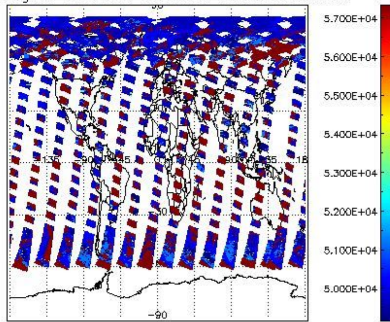
cloud_flags for 26JUN2008 00:00:00 to 27JUN2008 00:00:00
