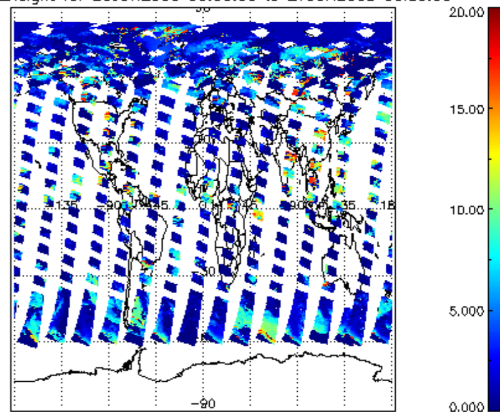
cl_top_height for 26JUN2008 00:00:00 to 27JUN2008 00:00:00
