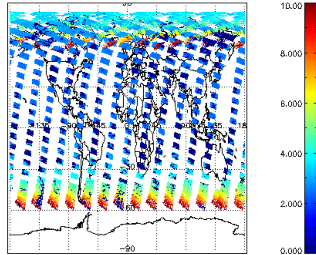
SCIOL2P_NADUV003_amf_cl for 26JUN2008 00:00:00 to 27JUN2008 00:00:00
