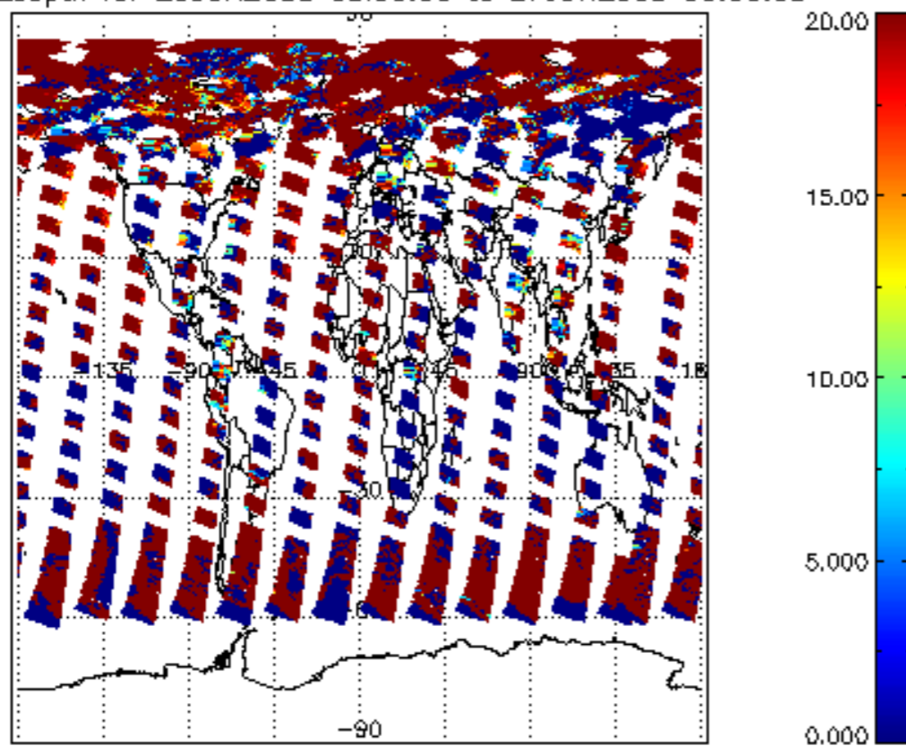
cl_opt_depth for 26JUN2008 00:00:00 to 27JUN2008 00:00:00
