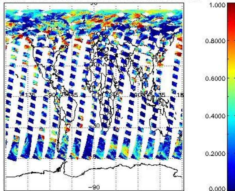
cL_frac for 26JUN2008 00:00:00 to 27JUN2008 00:00:00
